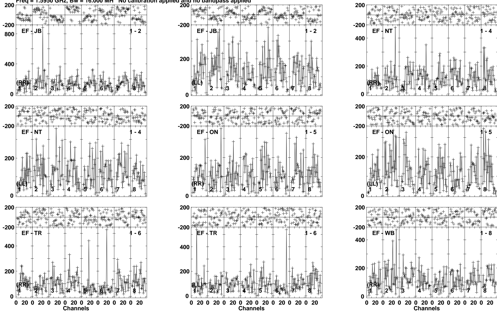
Lower frame: Micro Ampl Jy Top frame: Phas deg Vector averaged cross-power spectrum Baseline: EF (01) - JB (02) Timerange: 01/05:40:01 to 01/05:43:59
