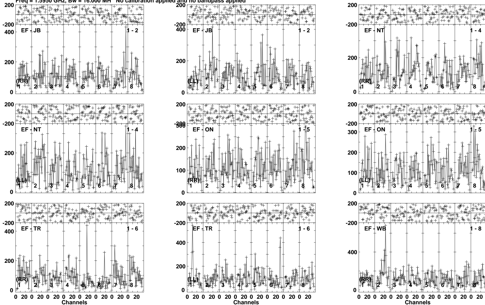
Lower frame: Micro Ampl Jy Top frame: Phas deg Vector averaged cross-power spectrum Baseline: EF (01) - JB (02) Timerange: 00:19:45:01 to 00:19:48:59
