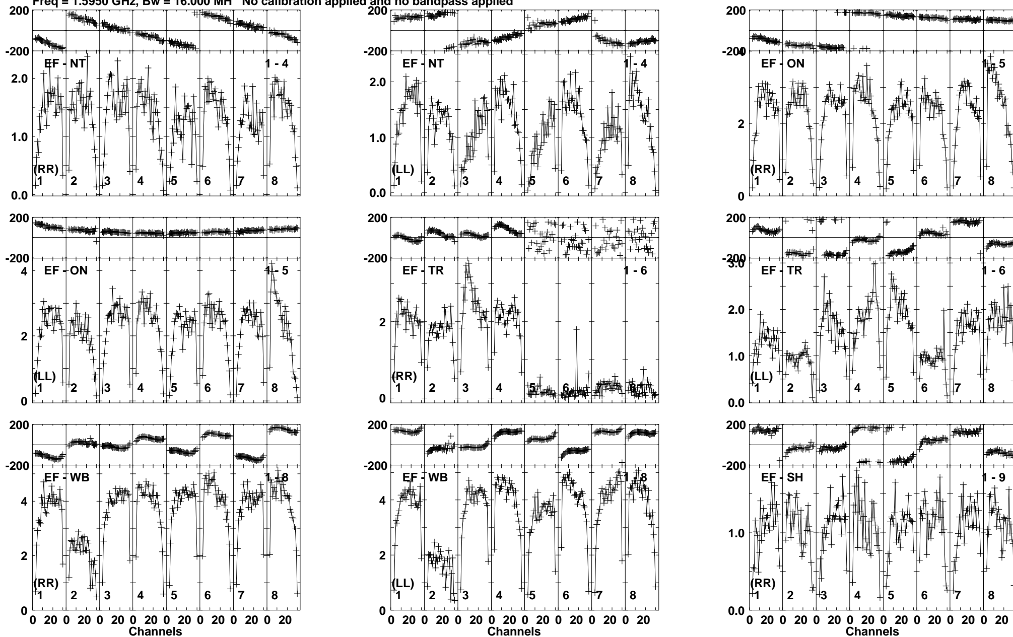
Lower frame: Milli Ampl Jy Top frame: Phas deg Vector averaged cross-power spectrum Baseline: EF (01) - NT (04) Timerange: 00:19:44:01 to 00:19:44:59
