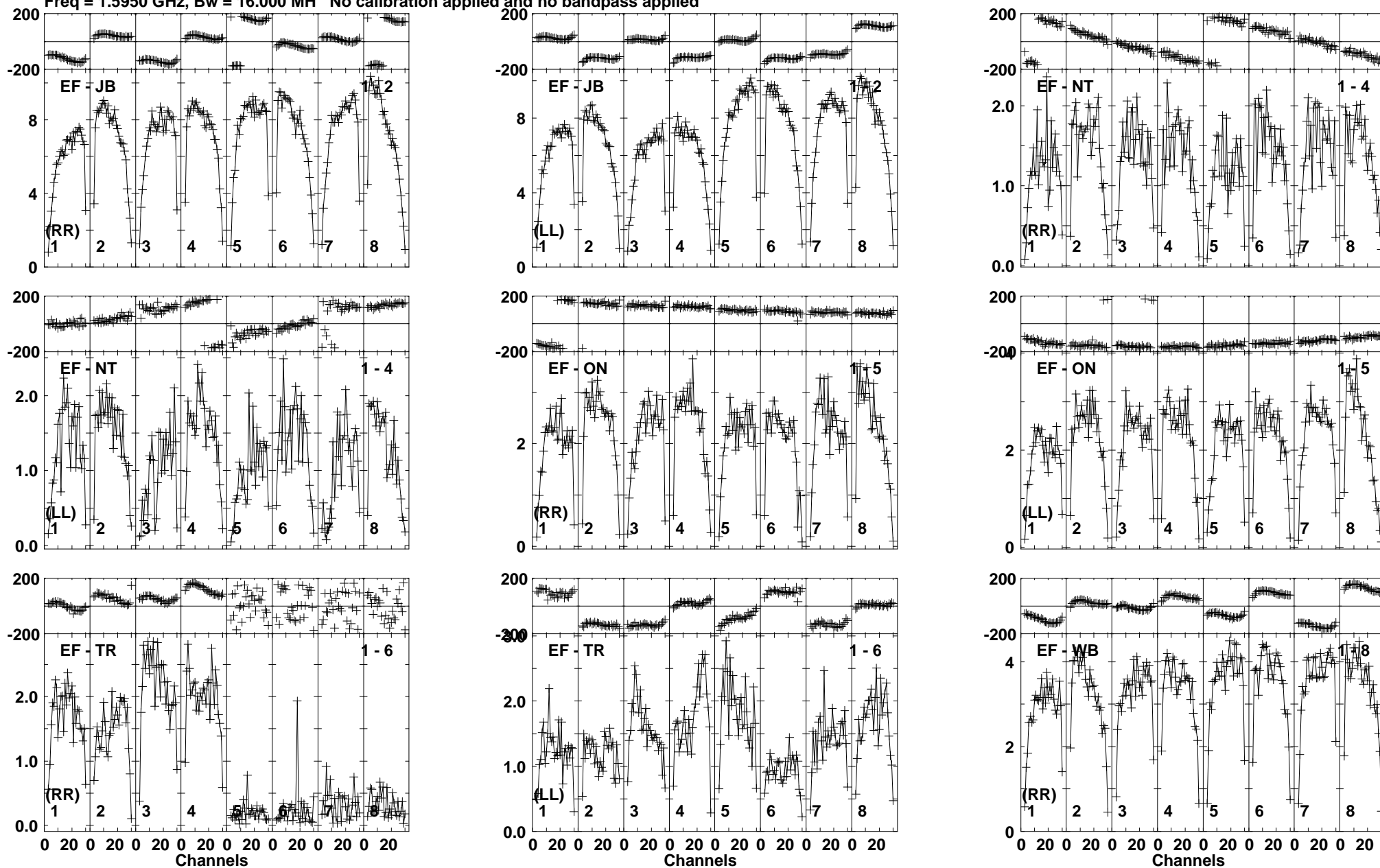
Lower frame: Milli Ampl Jy Top frame: Phas deg Vector averaged cross-power spectrum Baseline: EF (01) - JB (02) Timerange: 01/05:19:31 to 01/05:19:59
