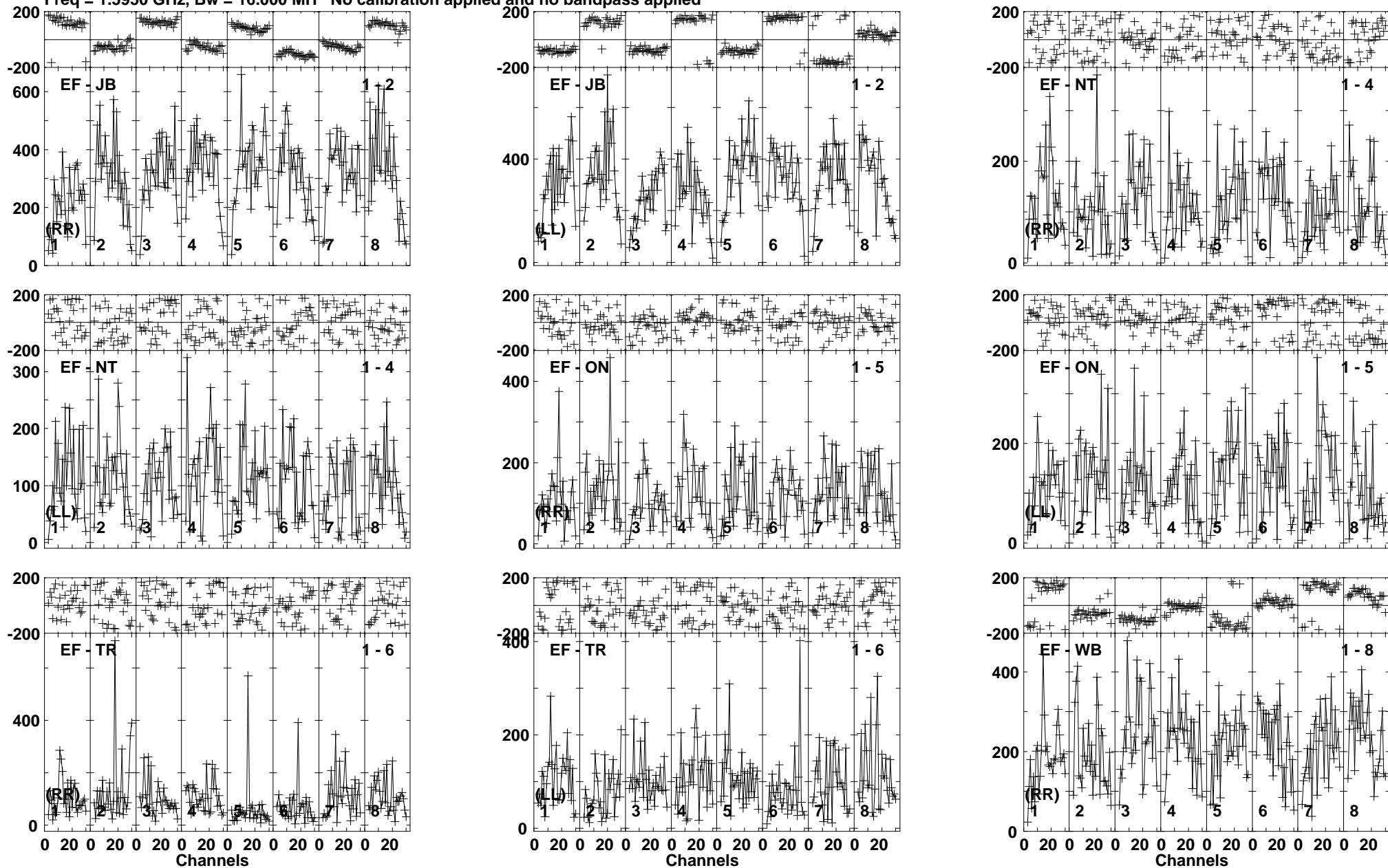
Lower frame: Micro Ampl Jy Top frame: Phas deg Vector averaged cross-power spectrum Baseline: EF (01) - JB (02) Timerange: 01/05:20:01 to 01/05:23:59
