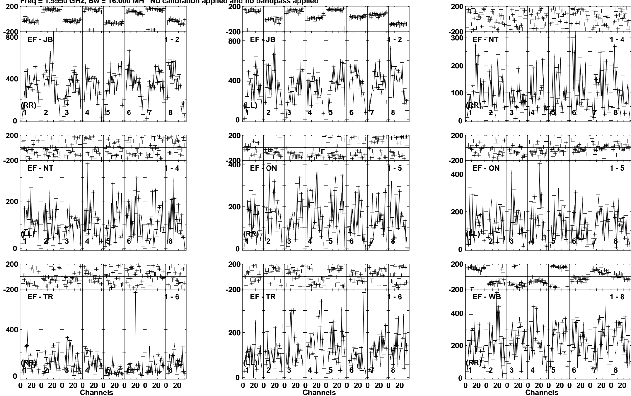
Lower frame: Micro Ampl Jy Top frame: Phas deg Vector averaged cross-power spectrum Baseline: EF (01) - JB (02) Timerange: 01/04:25:01 to 01/04:28:59
