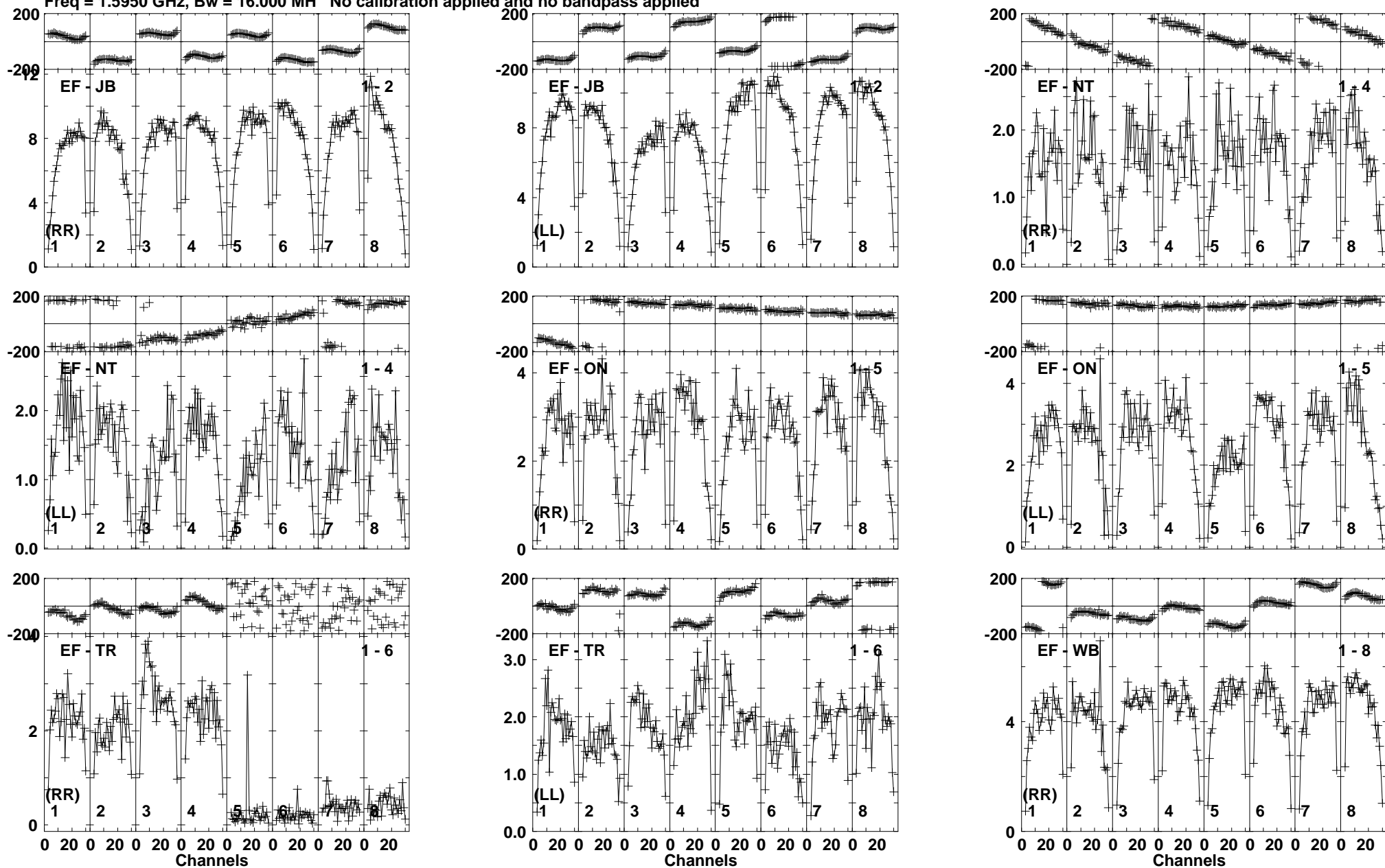
Lower frame: Milli Ampl Jy Top frame: Phas deg Vector averaged cross-power spectrum Baseline: EF (01) - JB (02) Timerange: 01/00:39:31 to 01/00:39:59
