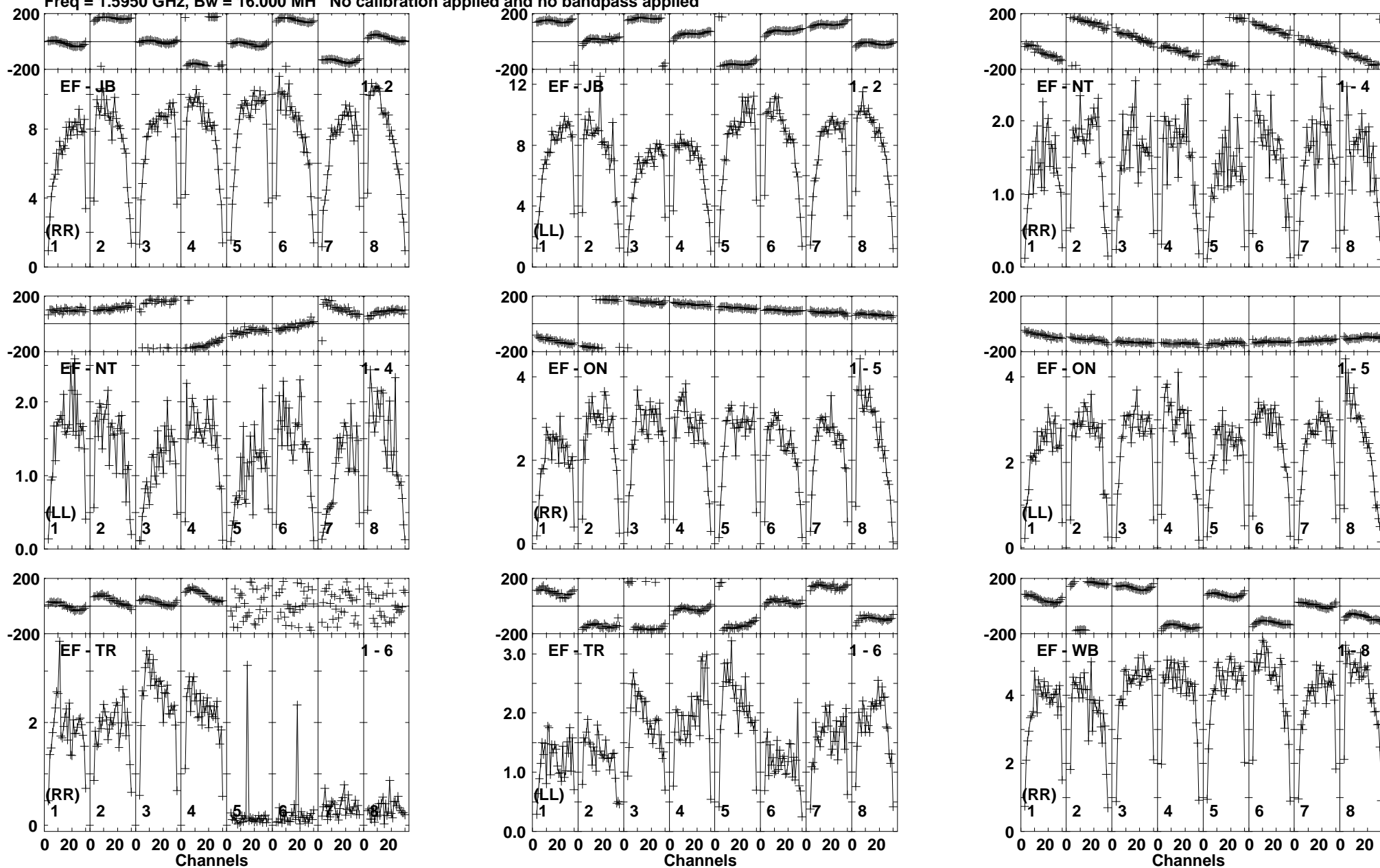
Lower frame: Milli Ampl Jy Top frame: Phas deg Vector averaged cross-power spectrum Baseline: EF (01) - JB (02) Timerange: 01/03:29:01 to 01/03:29:59
