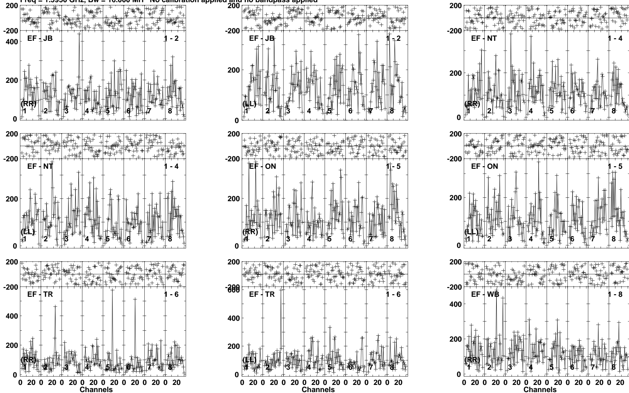
Lower frame: Micro Ampl Jy Top frame: Phas deg Vector averaged cross-power spectrum Baseline: EF (01) - JB (02) Timerange: 01/05:35:01 to 01/05:38:59
