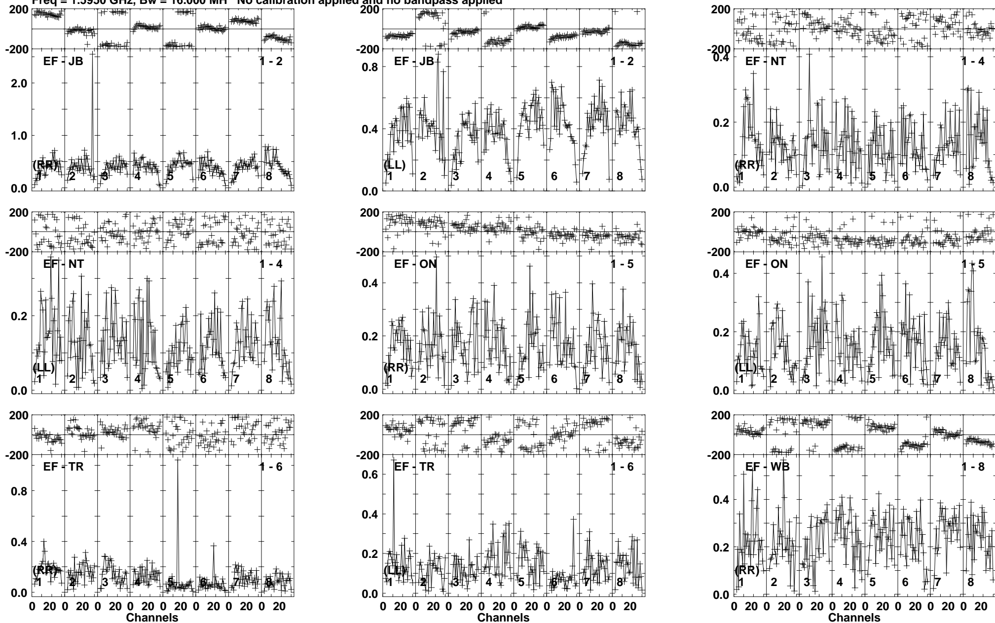
Lower frame: Milli Ampl Jy Top frame: Phas deg Vector averaged cross-power spectrum Baseline: EF (01) - JB (02) Timerange: 00/22:05:01 to 00/22:08:59
