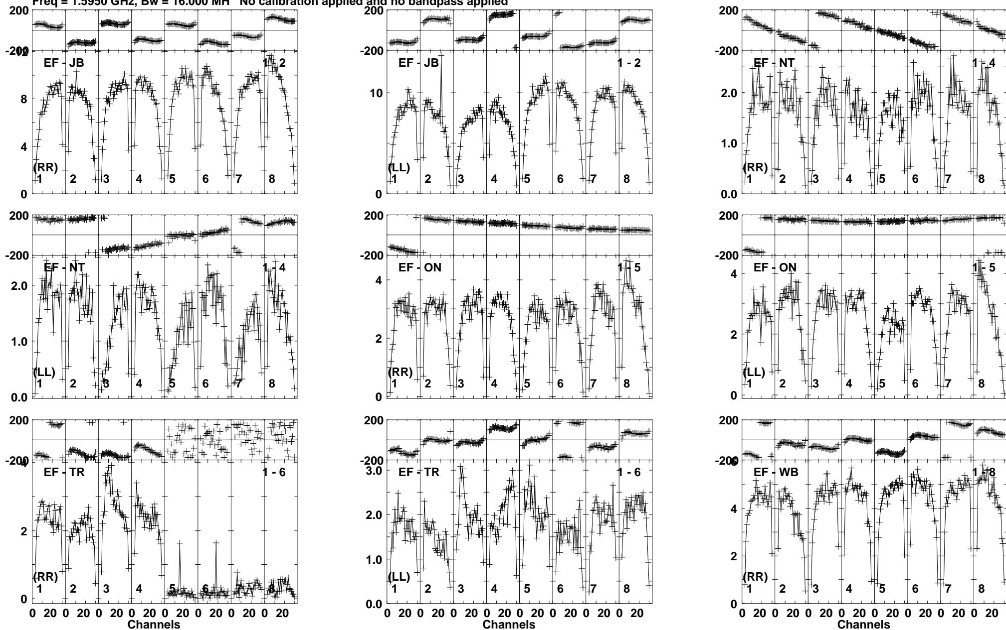
Lower frame: Milli Ampl Jy Top frame: Phas deg Vector averaged cross-power spectrum Baseline: EF (01) - JB (02) Timerange: 01/00:59:31 to 01/00:59:59
