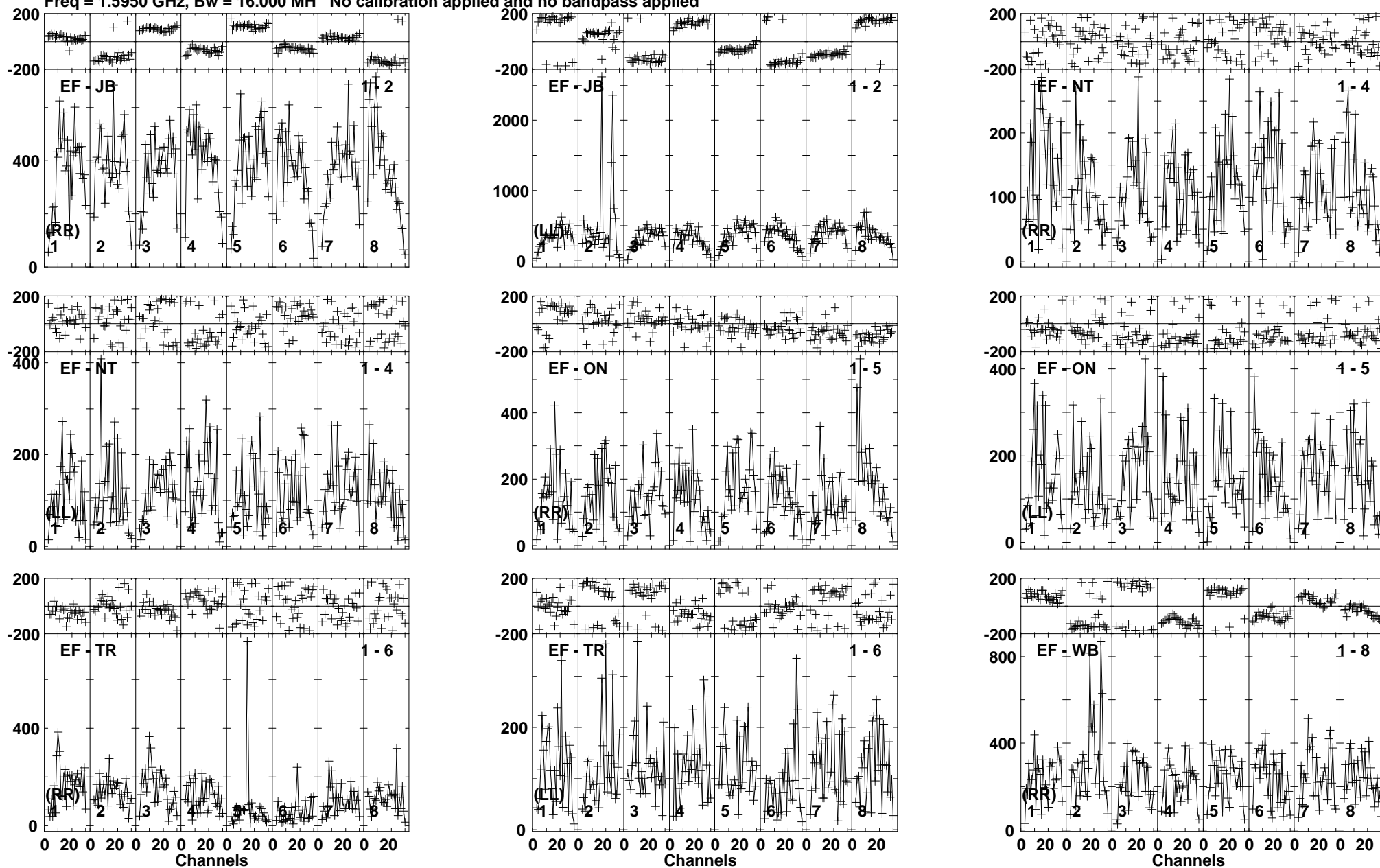
Lower frame: Micro Ampl Jy Top frame: Phas deg Vector averaged cross-power spectrum Baseline: EF (01) - JB (02) Timerange: 00/20:05:01 to 00/20:08:59
