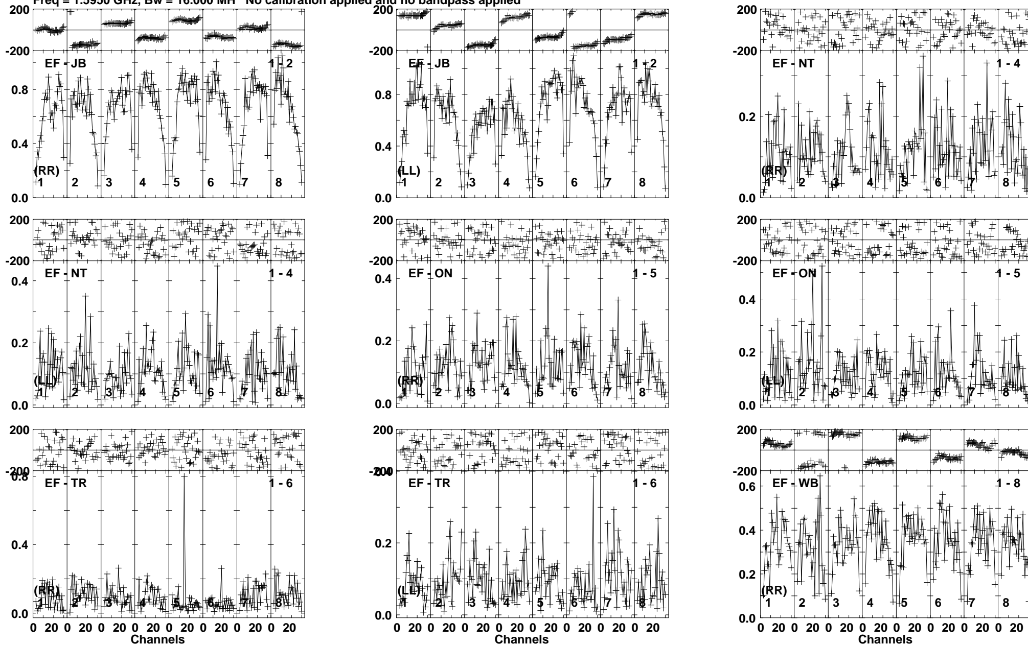
Lower frame: Milli Ampl Jy Top frame: Phas deg Vector averaged cross-power spectrum Baseline: EF (01) - JB (02) Timerange: 00/22:00:01 to 00/22:03:59
