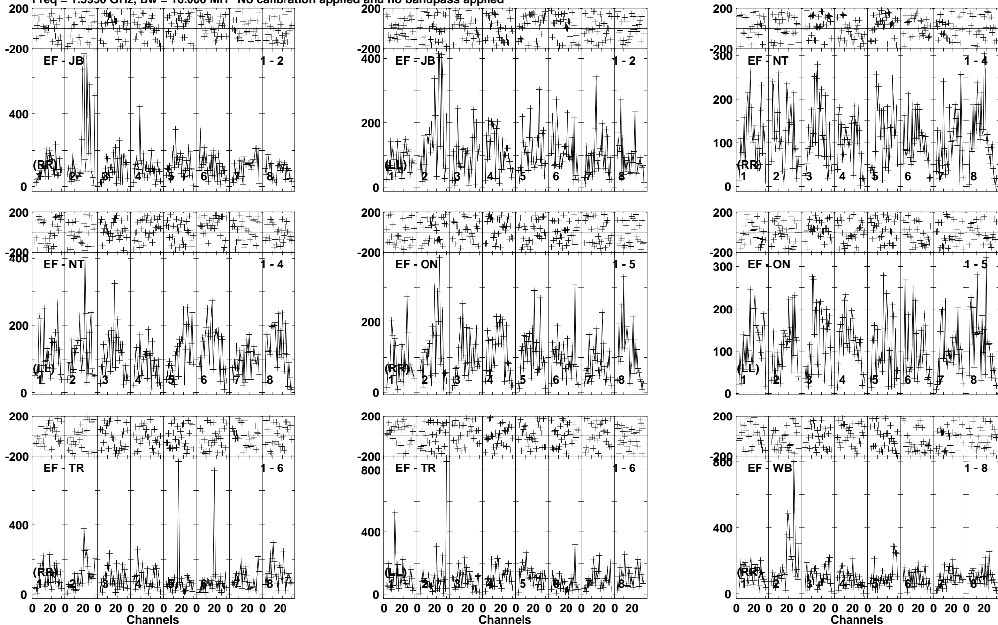
Lower frame: Micro Ampl Jy Top frame: Phas deg Vector averaged cross-power spectrum Baseline: EF (01) - JB (02) Timerange: 00:18:50:01 to 00:18:53:59
