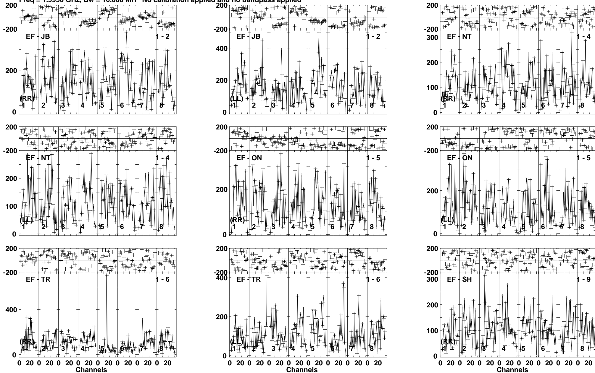
Lower frame: Micro Ampl Jy Top frame: Phas deg Vector averaged cross-power spectrum Baseline: EF (01) - JB (02) Timerange: 00/18:10:01 to 00/18:13:59
