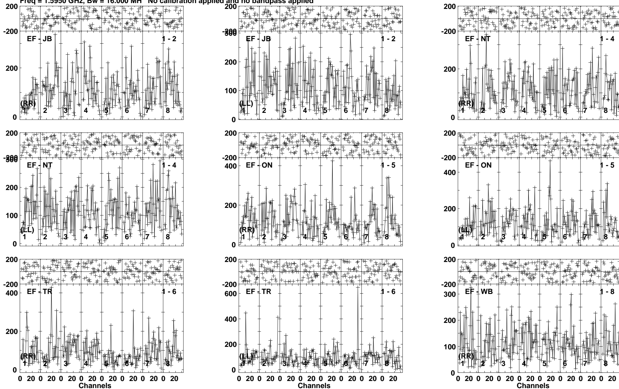
Lower frame: Micro Ampl Jy Top frame: Phas deg Vector averaged cross-power spectrum Baseline: EF (01) - JB (02) Timerange: 00:22:50:01 to 00:22:53:59
