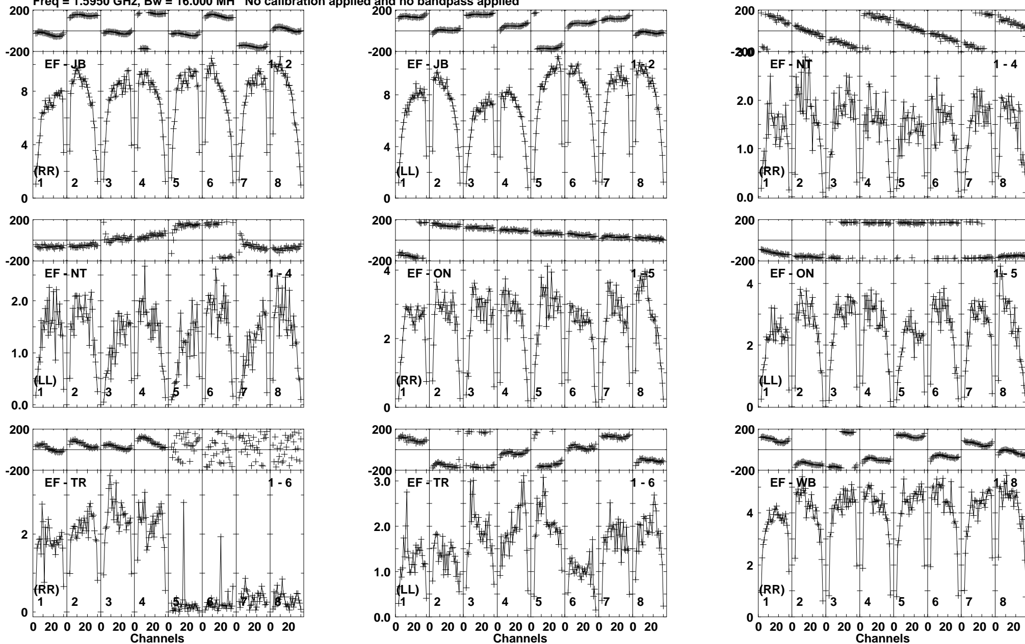
Lower frame: Milli Ampl Jy Top frame: Phas deg Vector averaged cross-power spectrum Baseline: EF (01) - JB (02) Timerange: 01/02:39:31 to 01/02:39:59
