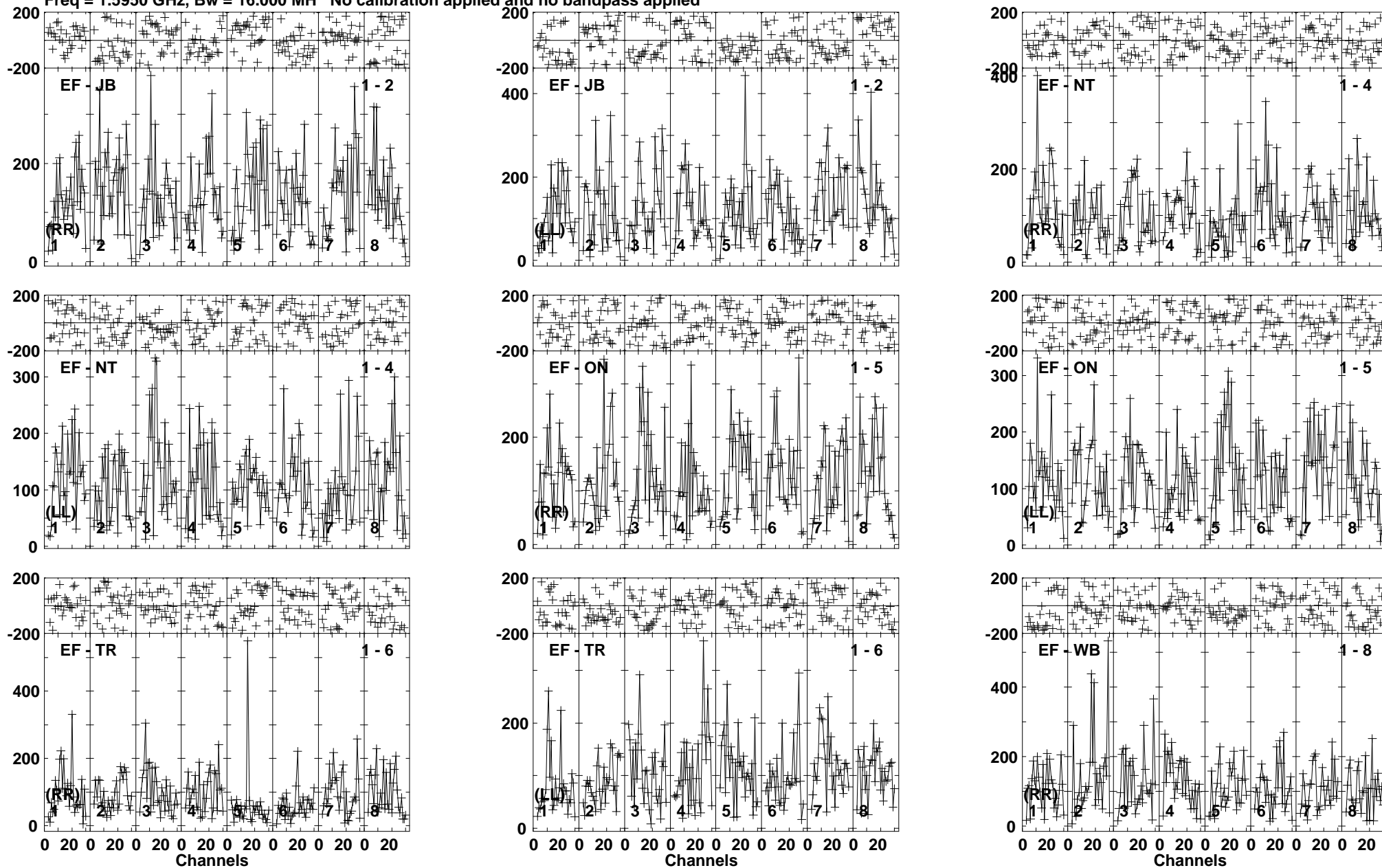
Lower frame: Micro Ampl Jy Top frame: Phas deg Vector averaged cross-power spectrum Baseline: EF (01) - JB (02) Timerange: 01/03:30:01 to 01/03:33:59
