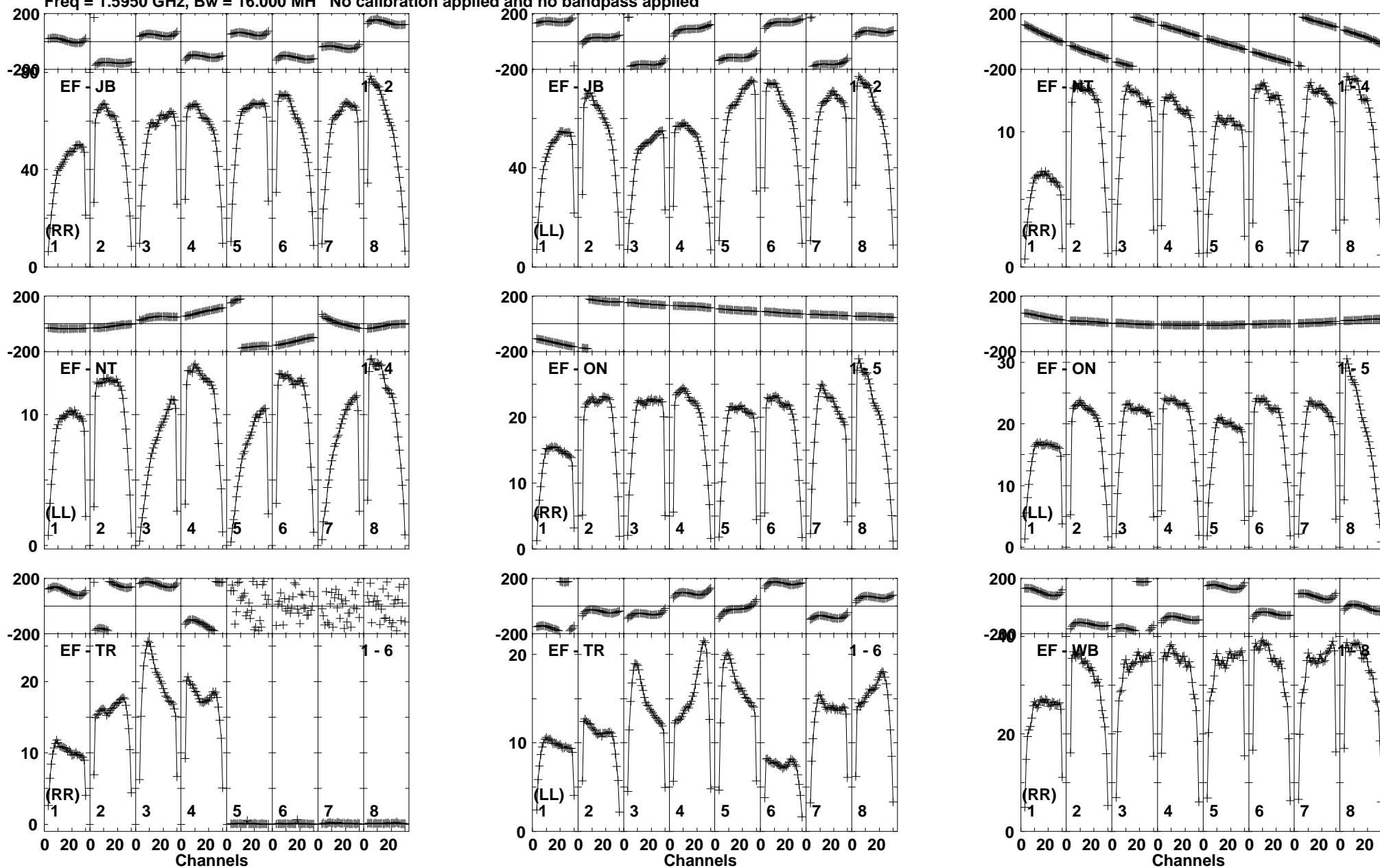
Lower frame: Milli Ampl Jy Top frame: Phas deg Vector averaged cross-power spectrum Baseline: EF (01) - JB (02) Timerange: 00/23:03:01 to 00/23:05:59
