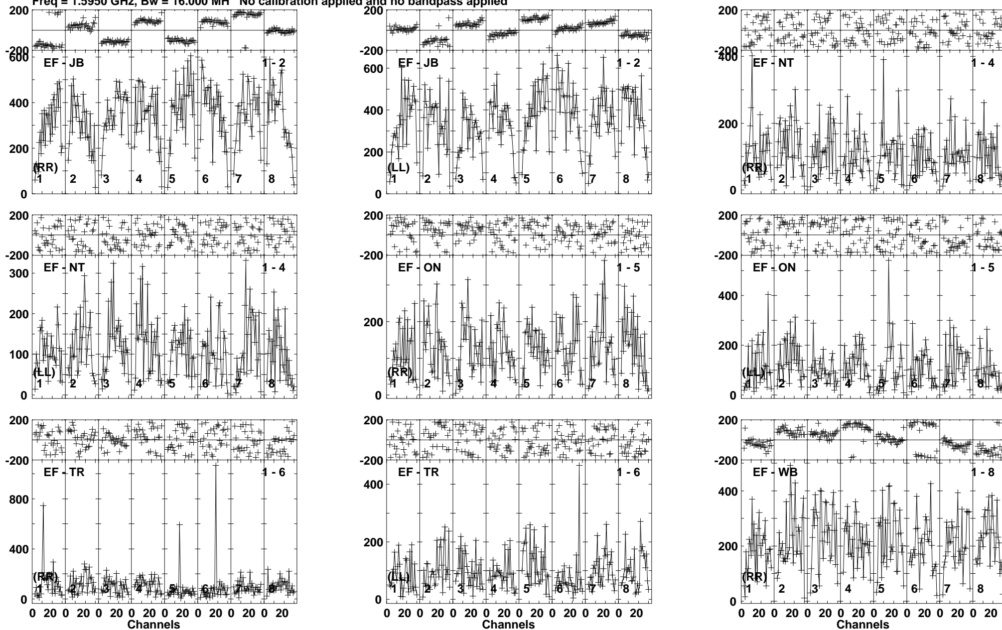
Lower frame: Micro Ampl Jy Top frame: Phas deg Vector averaged cross-power spectrum Baseline: EF (01) - JB (02) Timerange: 01/02:40:01 to 01/02:43:59
