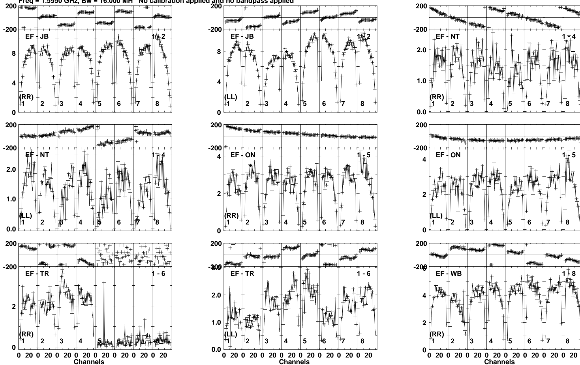
Lower frame: Milli Ampl Jy Top frame: Phas deg Vector averaged cross-power spectrum Baseline: EF (01) - JB (02) Timerange: 00/20:29:31 to 00/20:29:59
