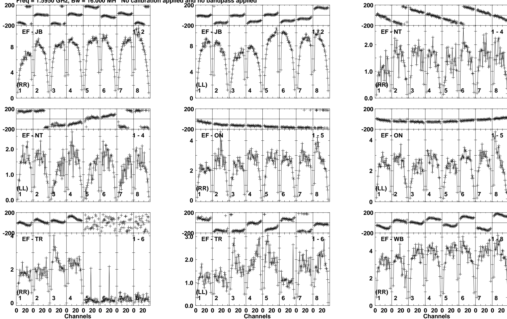
Lower frame: Milli Ampl Jy Top frame: Phas deg Vector averaged cross-power spectrum Baseline: EF (01) - JB (02) Timerange: 01/04:29:01 to 01/04:29:59
