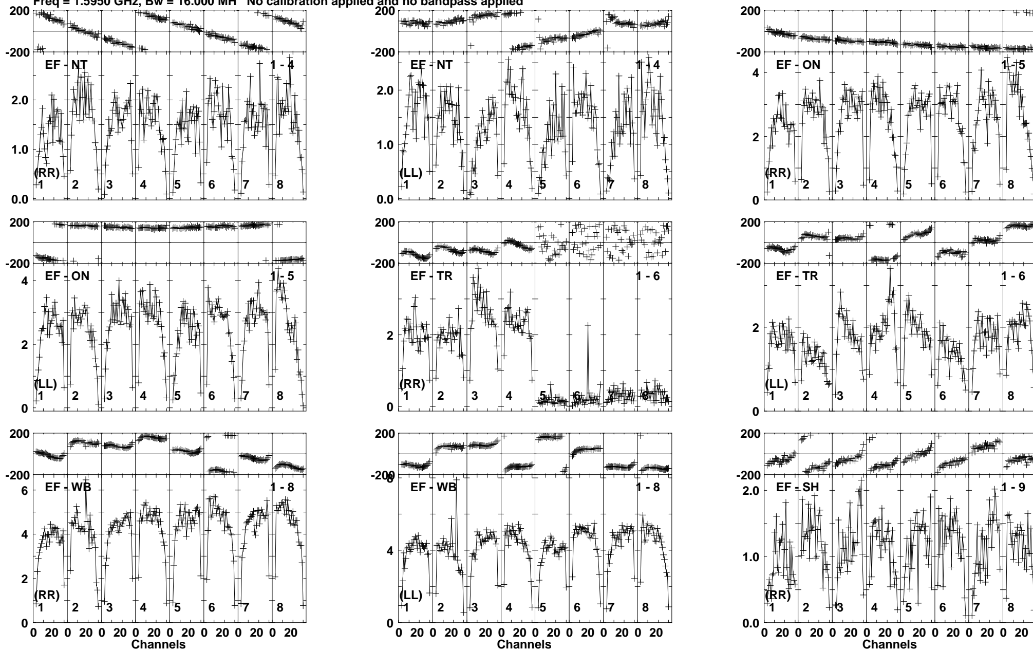
Lower frame: Milli Ampl Jy Top frame: Phas deg Vector averaged cross-power spectrum Baseline: EF (01) - NT (04) Timerange: 00:22:54:01 to 00:22:54:59
