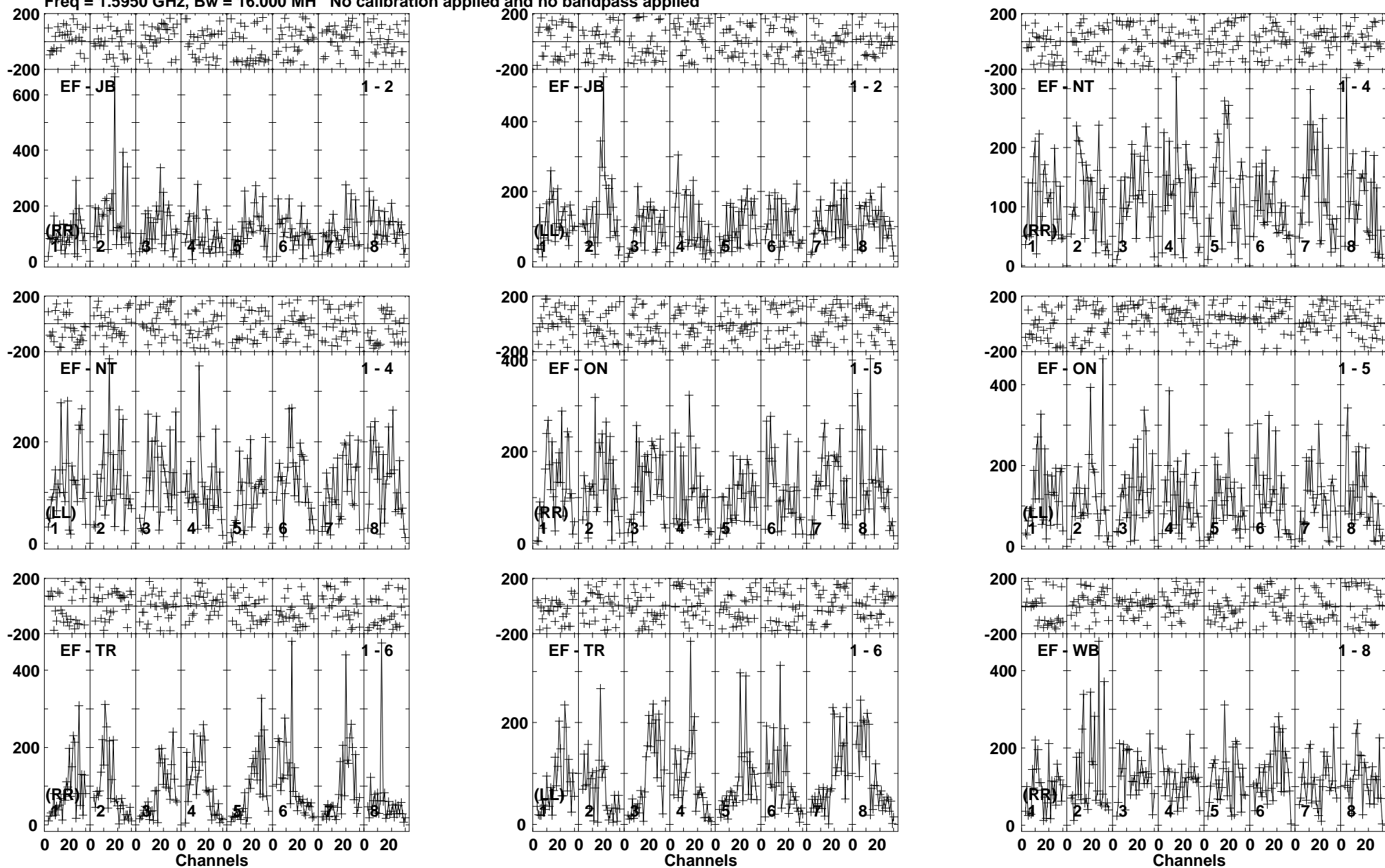
Lower frame: Micro Ampl Jy Top frame: Phas deg Vector averaged cross-power spectrum Baseline: EF (01) - JB (02) Timerange: 00/20:25:01 to 00/20:28:59
