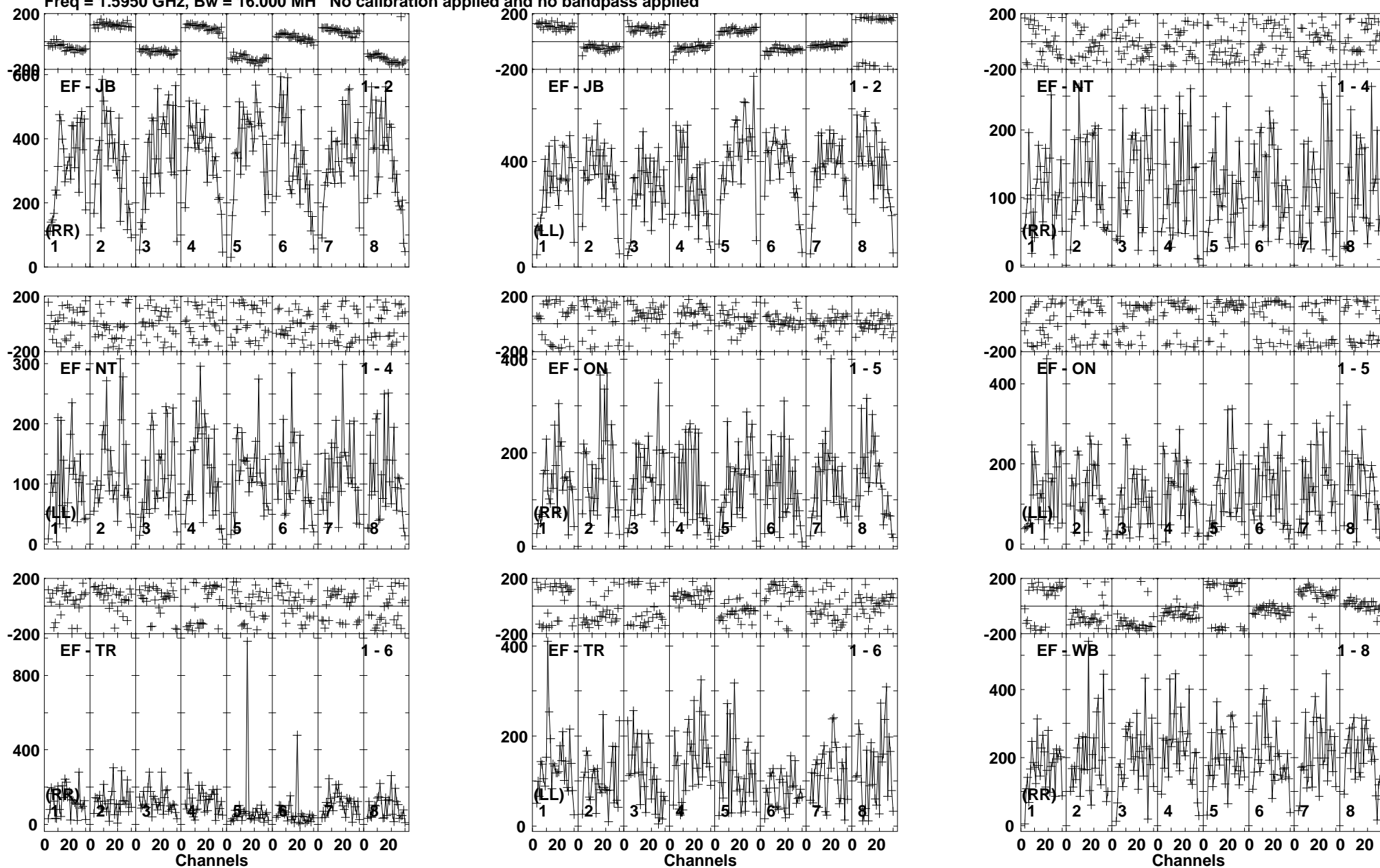
Lower frame: Micro Ampl Jy Top frame: Phas deg Vector averaged cross-power spectrum Baseline: EF (01) - JB (02) Timerange: 01/05:25:01 to 01/05:28:59
