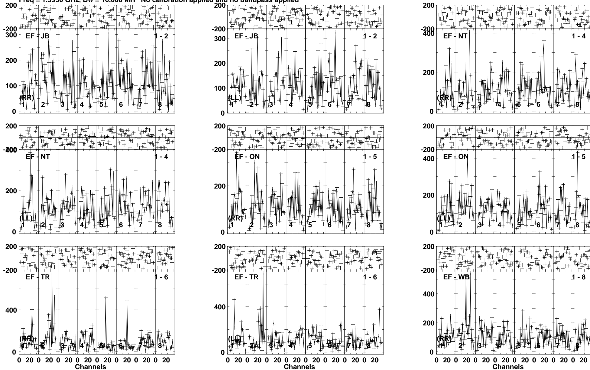
Lower frame: Micro Ampl Jy Top frame: Phas deg Vector averaged cross-power spectrum Baseline: EF (01) - JB (02) Timerange: 01/05:55:01 to 01/05:58:59
