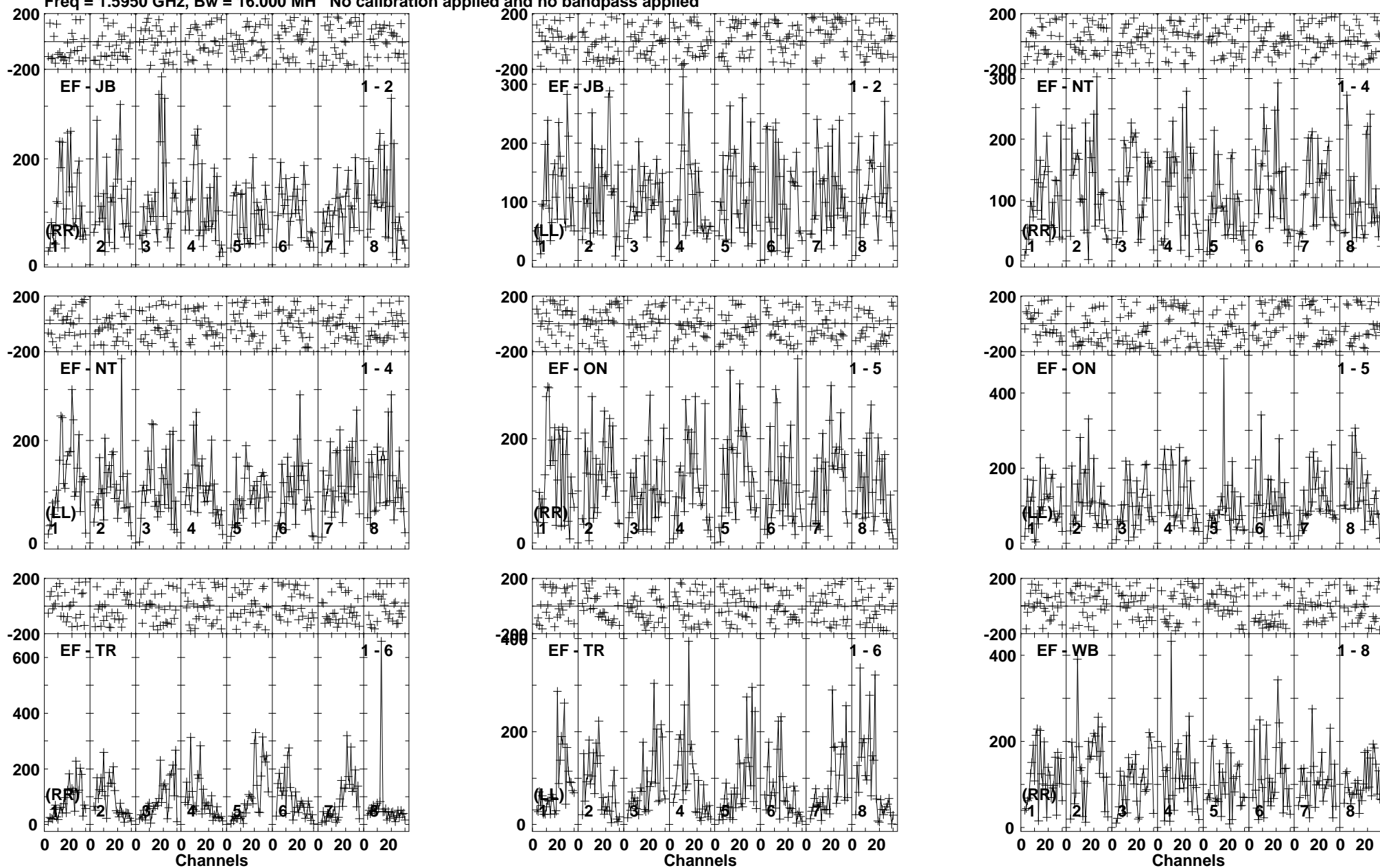
Lower frame: Micro Ampl Jy Top frame: Phas deg Vector averaged cross-power spectrum Baseline: EF (01) - JB (02) Timerange: 00/21:20:01 to 00/21:23:59
