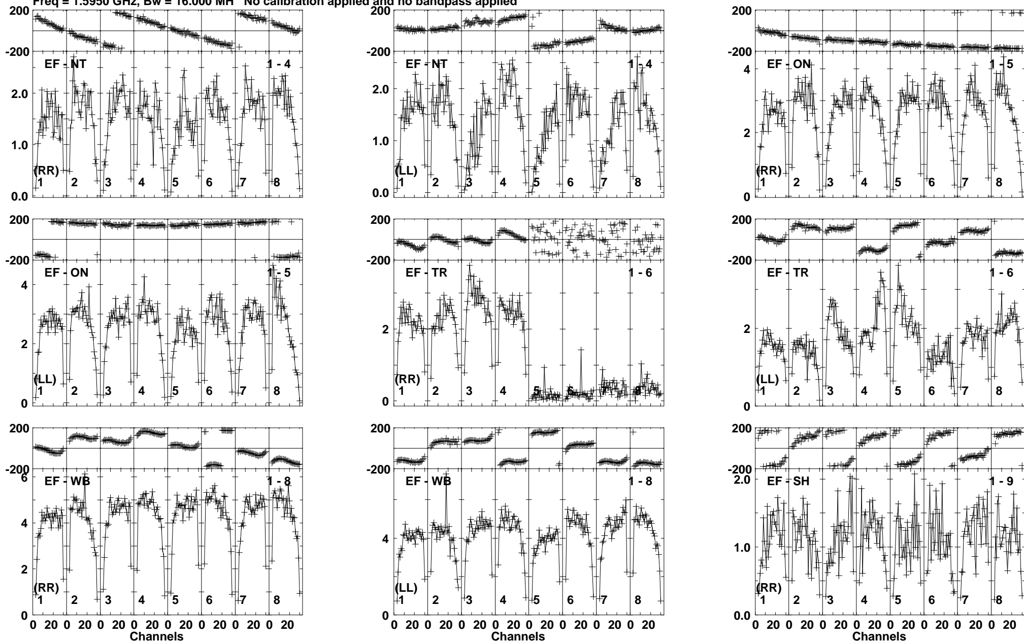
Lower frame: Milli Ampl Jy Top frame: Phas deg Vector averaged cross-power spectrum Baseline: EF (01) - NT (04) Timerange: 00/22:44:01 to 00/22:44:59
