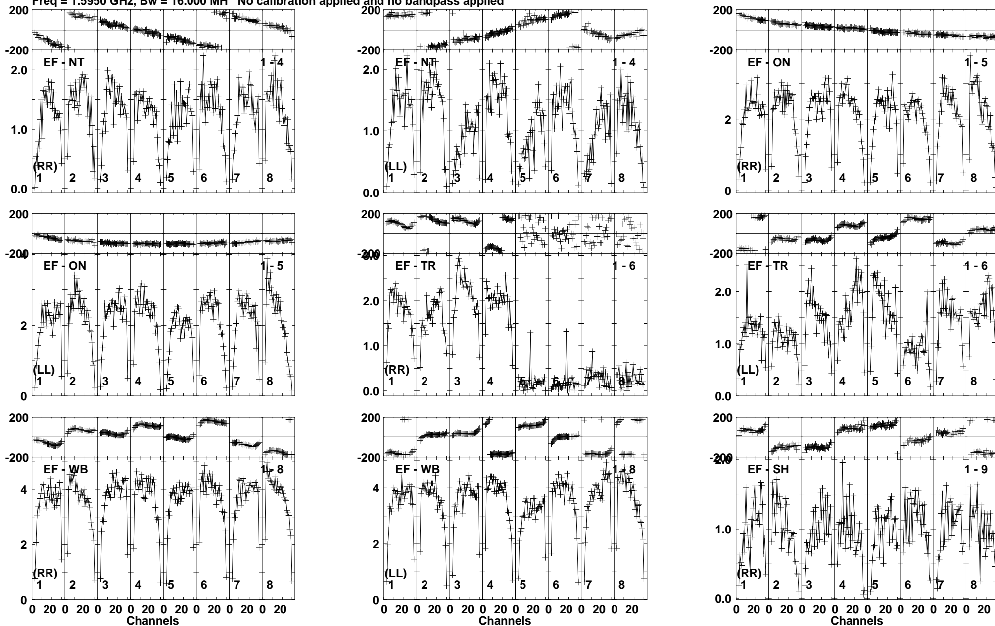
Lower frame: Milli Ampl Jy Top frame: Phas deg Vector averaged cross-power spectrum Baseline: EF (01) - NT (04) Timerange: 00:18:54:01 to 00:18:54:59
