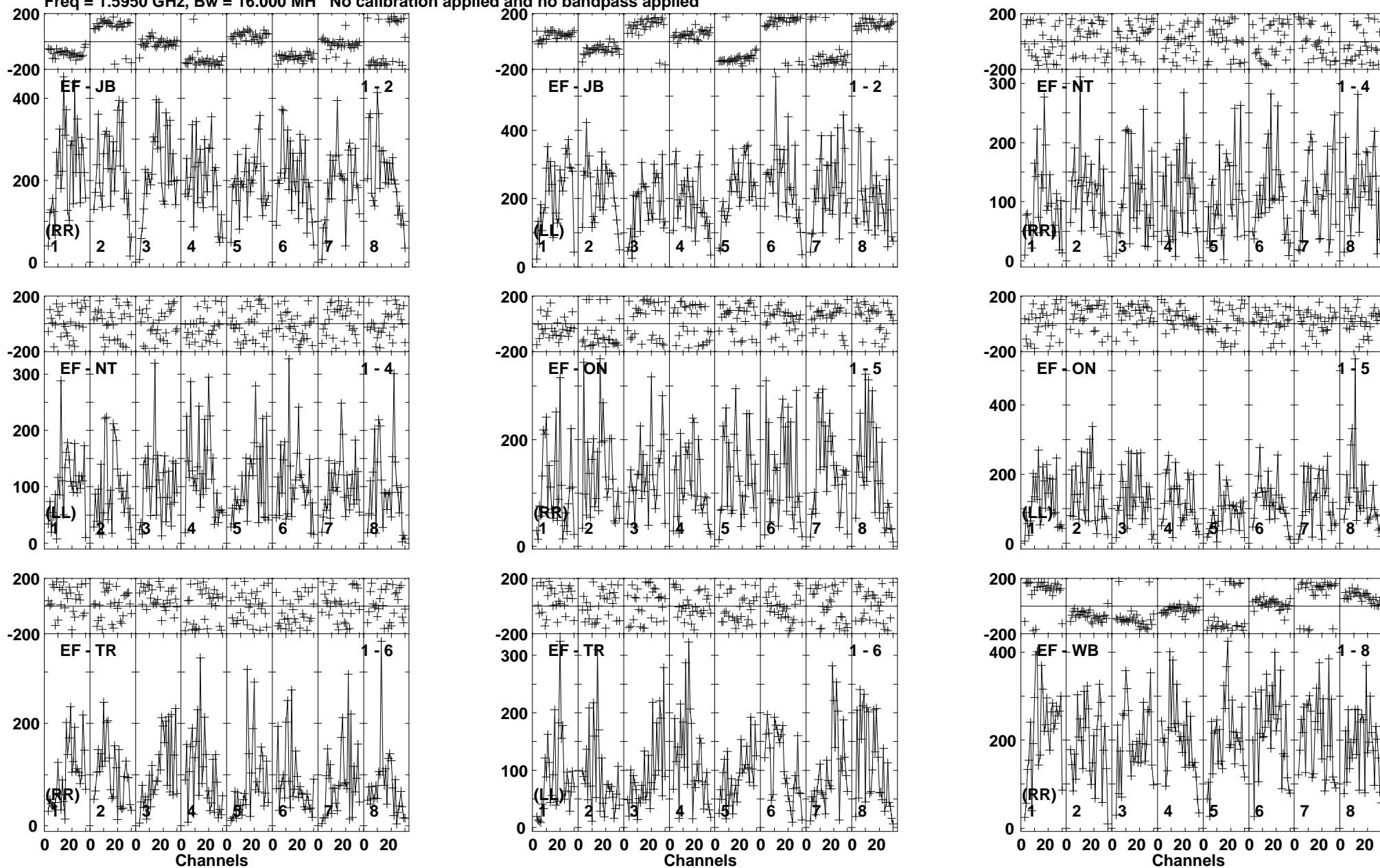
Lower frame: Micro Ampl Jy Top frame: Phas deg Vector averaged cross-power spectrum Baseline: EF (01) - JB (02) Timerange: 00/20:10:01 to 00/20:13:59
