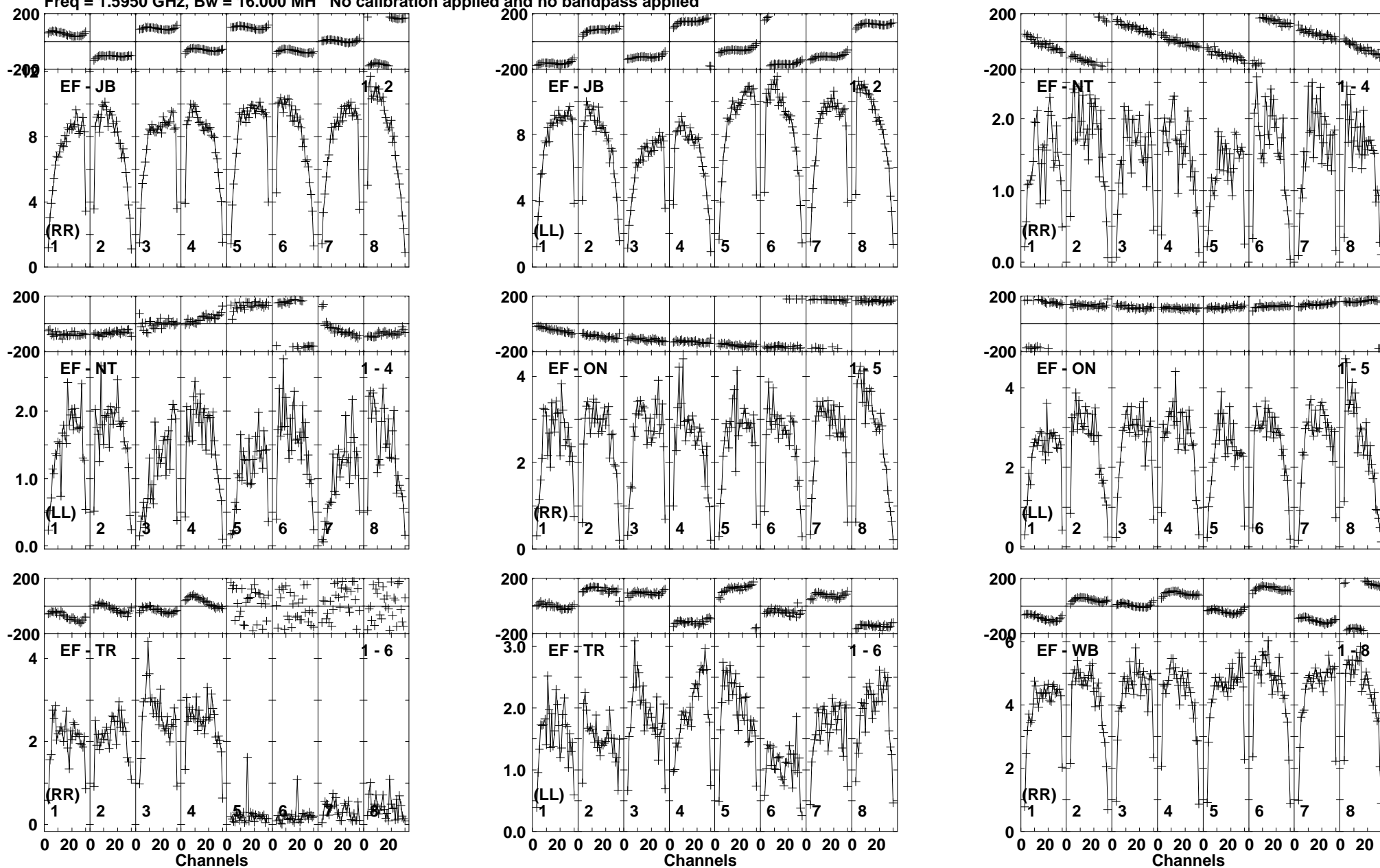
Lower frame: Milli Ampl Jy Top frame: Phas deg Vector averaged cross-power spectrum Baseline: EF (01) - JB (02) Timerange: 00/22:39:01 to 00/22:39:59
