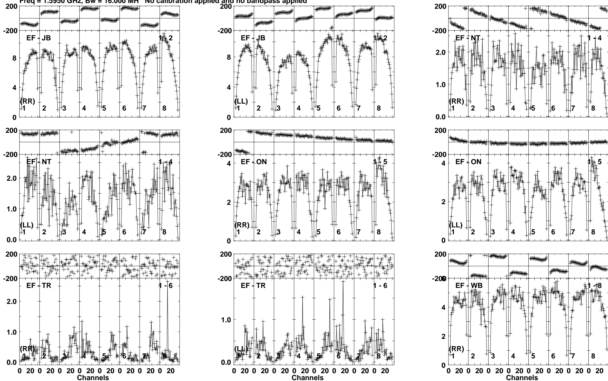
Lower frame: Milli Ampl Jy Top frame: Phas deg Vector averaged cross-power spectrum Baseline: EF (01) - JB (02) Timerange: 00/21:09:31 to 00/21:09:59
