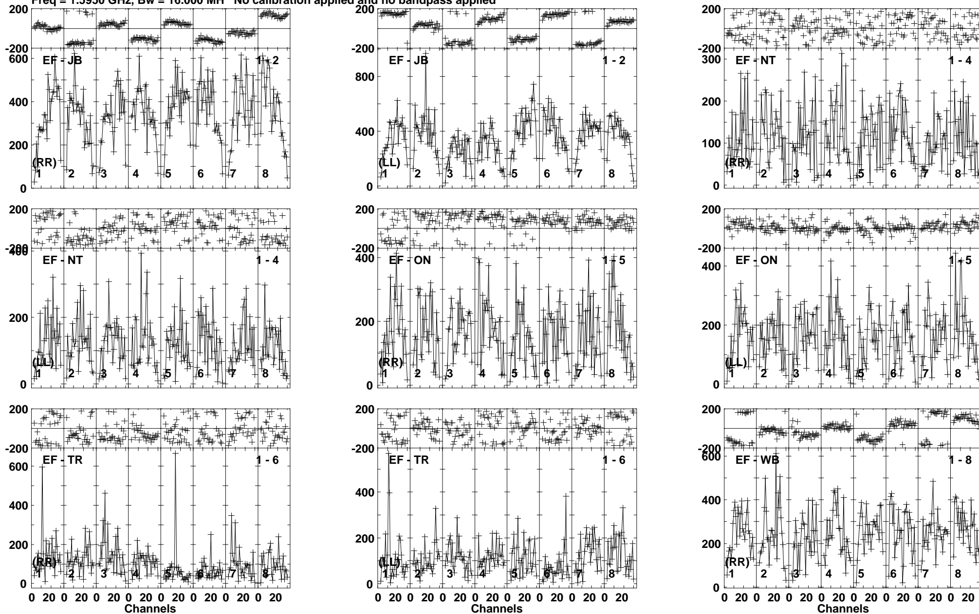
Lower frame: Micro Ampl Jy Top frame: Phas deg Vector averaged cross-power spectrum Baseline: EF (01) - JB (02) Timerange: 00/22:15:01 to 00/22:18:59
