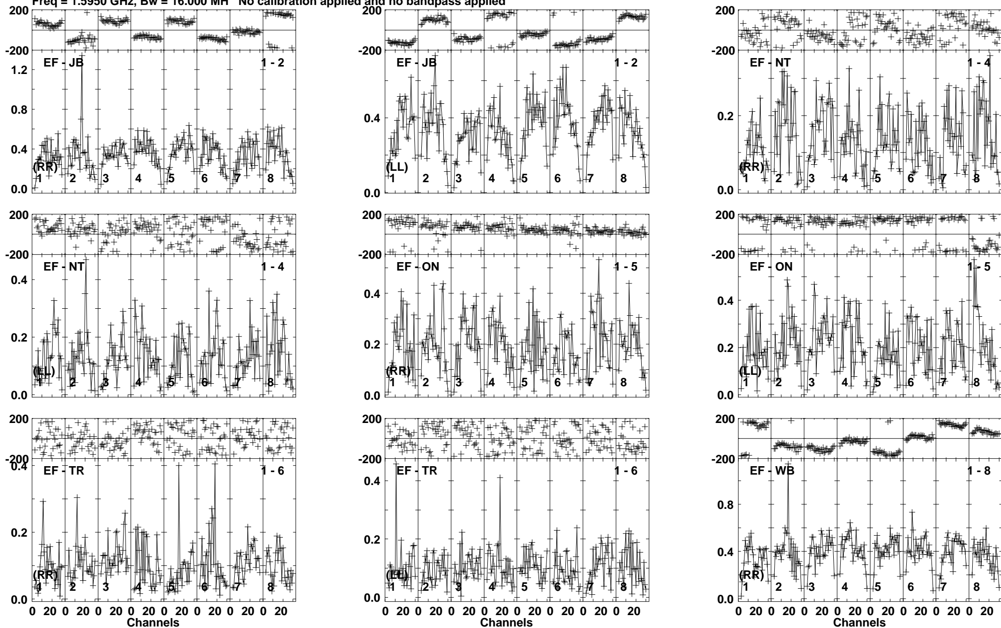
Lower frame: Milli Ampl Jy Top frame: Phas deg Vector averaged cross-power spectrum Baseline: EF (01) - JB (02) Timerange: 01/02:30:01 to 01/02:33:59
