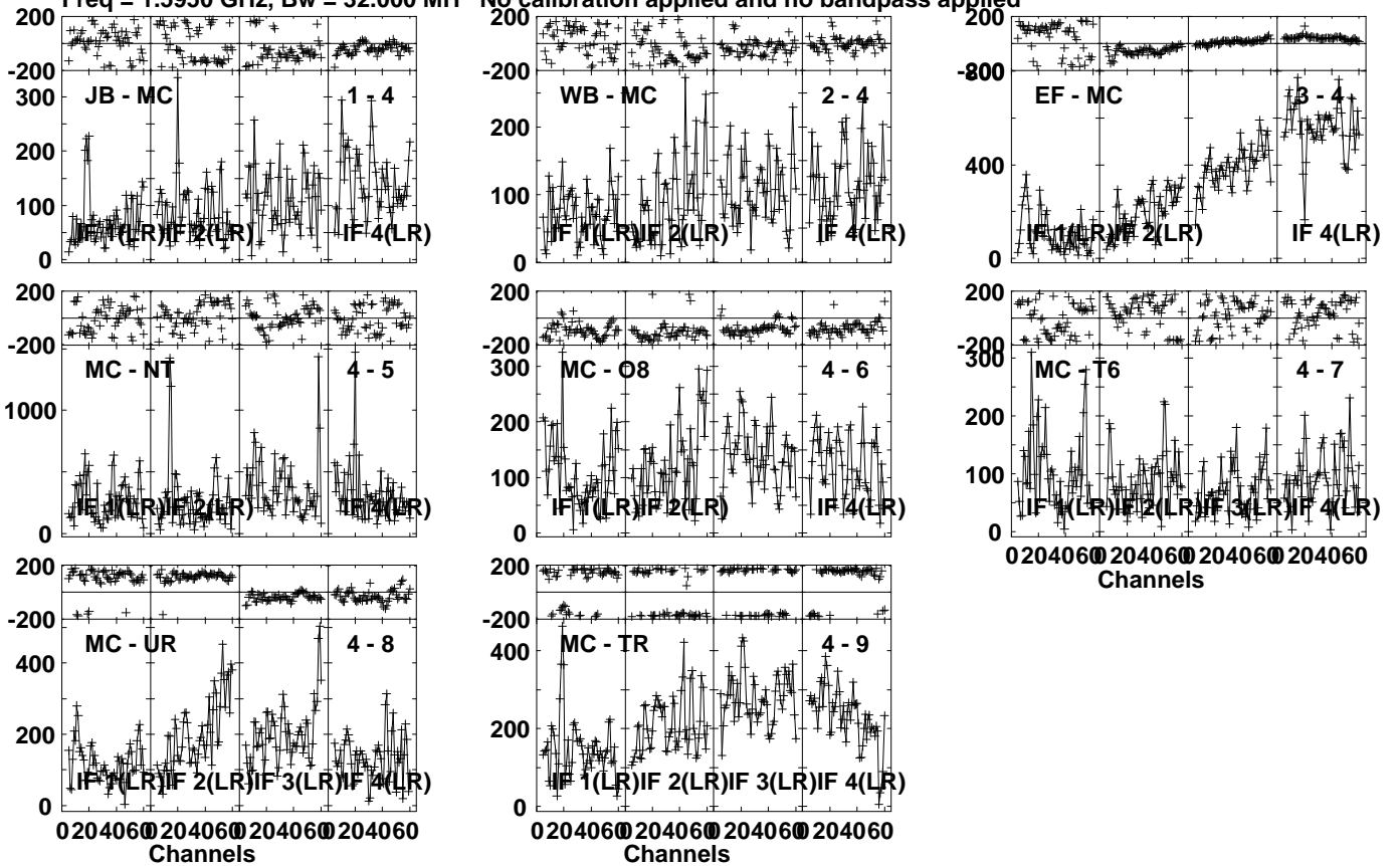
Lower frame: Micro Ampl Jy Top frame: Phas deg Vector averaged cross-power spectrum Several baselines displayed Timerange: 00/12:17:13 to 00/12:30:59
