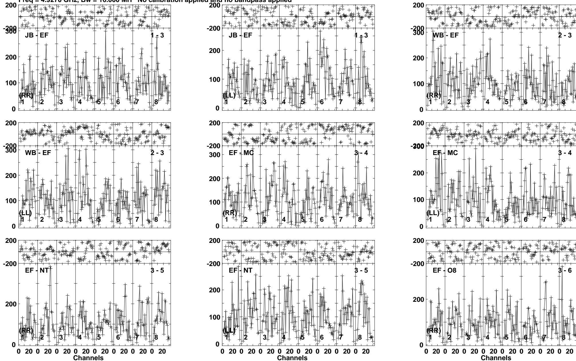
Lower frame: Micro Ampl Jy Top frame: Phas deg Vector averaged cross-power spectrum Baseline: JB (01) - EF (03) Timerange: 01/12:17:14 to 01/12:20:38
