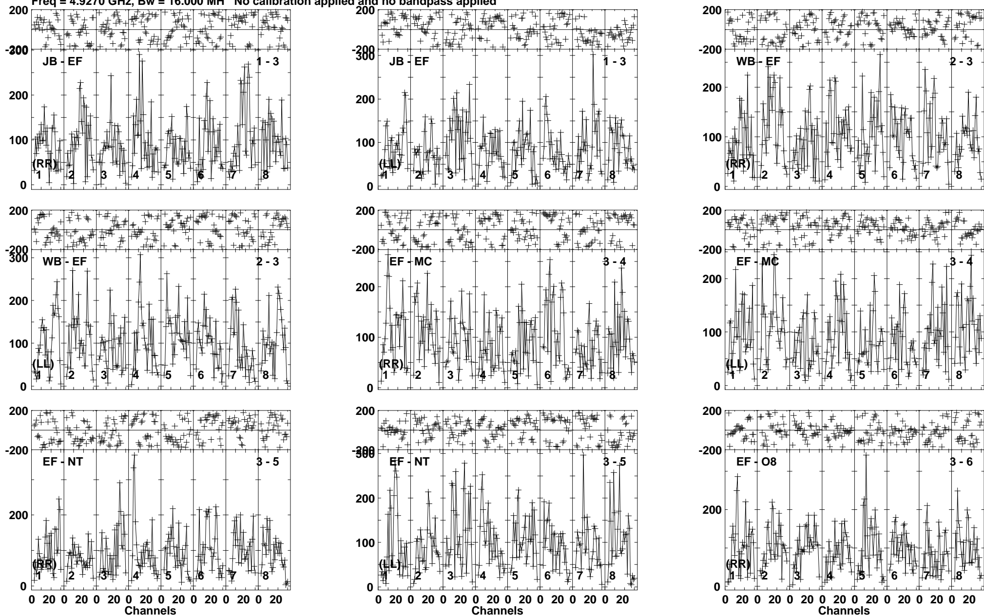
Lower frame: Micro Ampl Jy Top frame: Phas deg Vector averaged cross-power spectrum Baseline: JB (01) - EF (03) Timerange: 01/11:05:28 to 01/11:08:52
