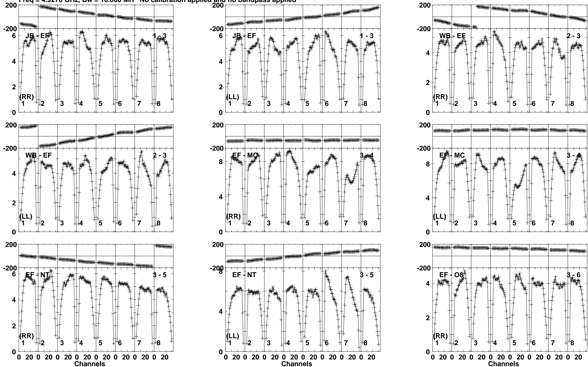
Lower frame: Milli Ampl Jy Top frame: Phas deg Vector averaged cross-power spectrum Baseline: JB (01) - EF (03) Timerange: 00/21:01:03 to 00/21:02:29
