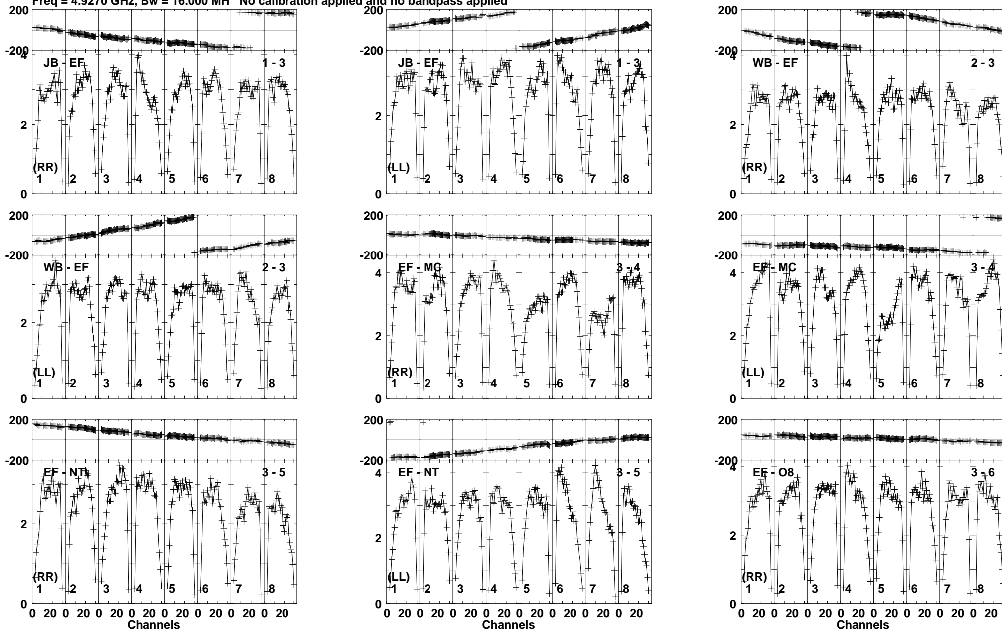
Lower frame: Milli Ampl Jy Top frame: Phas deg Vector averaged cross-power spectrum Baseline: JB (01) - EF (03) Timerange: 01/11:46:17 to 01/11:47:39
