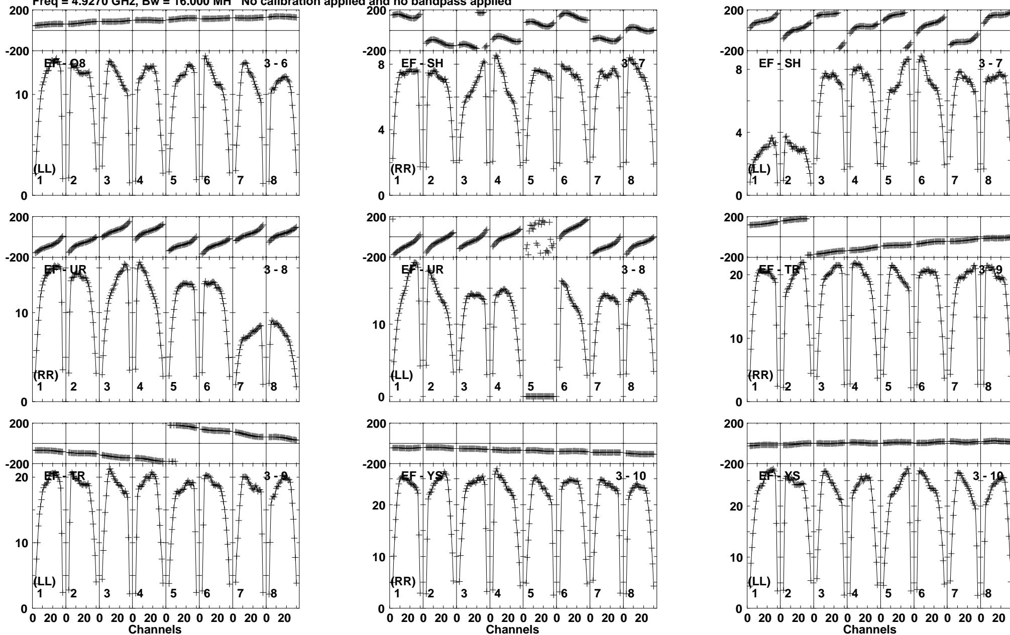
Lower frame: Milli Amply Jy Top frame: Phas deg Vector averaged cross-power spectrum Baseline: EF (03) - O8 (06) Timerange: 01/02:33:54 to 01/02:35:22
