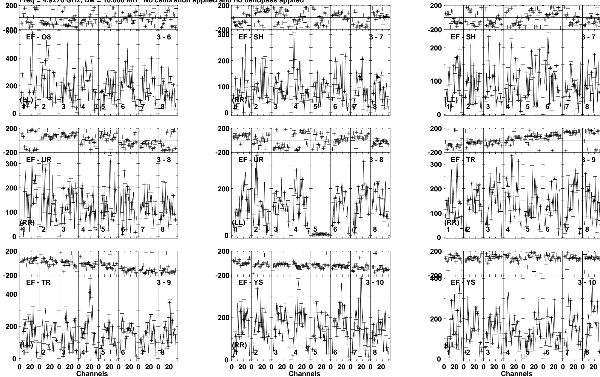
Lower frame: Micro Ampl Jy Top frame: Phas deg Vector averaged cross-power spectrum Baseline: EF (03) - O8 (06) Timerange: 01/00:45:31 to 01/00:48:53
