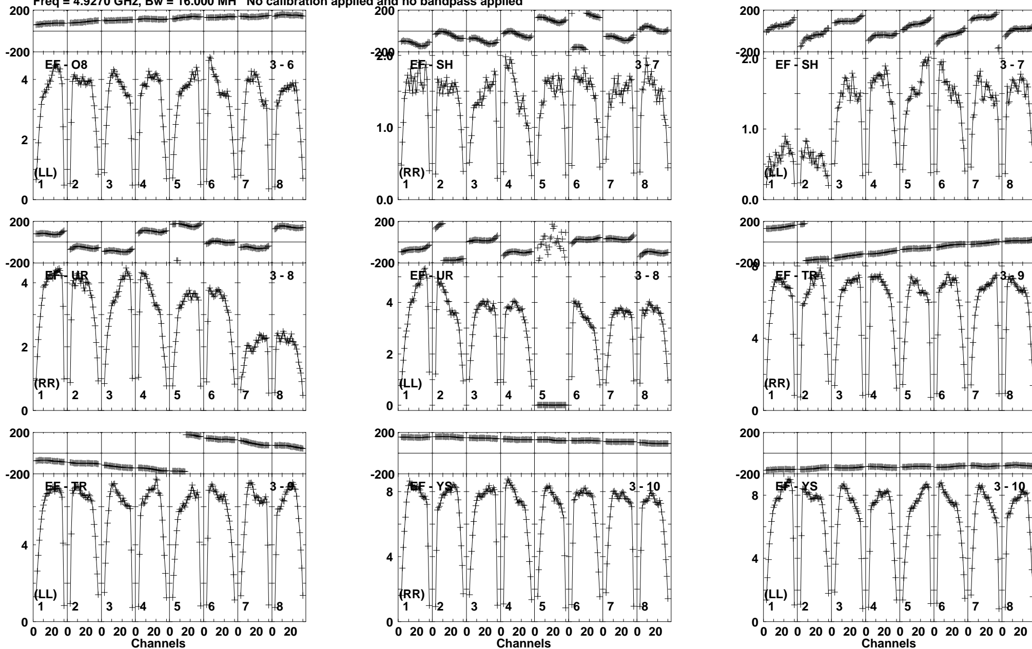
Lower frame: Milli Ampl Jy Top frame: Phas deg Vector averaged cross-power spectrum Baseline: EF (03) - O8 (06) Timerange: 00/21:52:27 to 00/21:53:53
