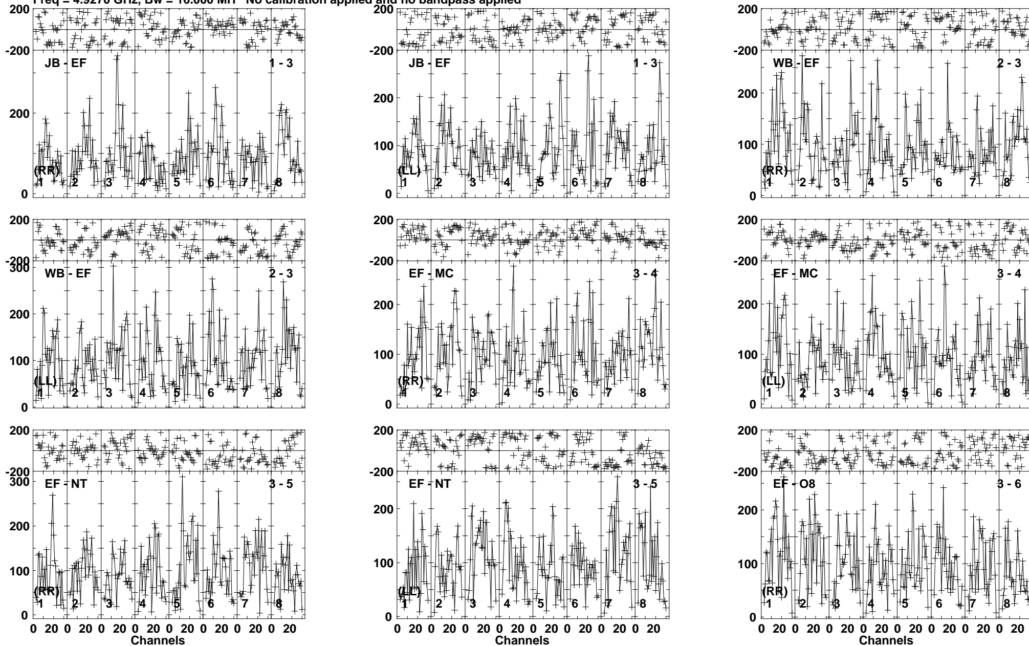
Lower frame: Micro Ampl Jy Top frame: Phas deg Vector averaged cross-power spectrum Baseline: JB (01) - EF (03) Timerange: 01/10:44:32 to 01/10:47:52
