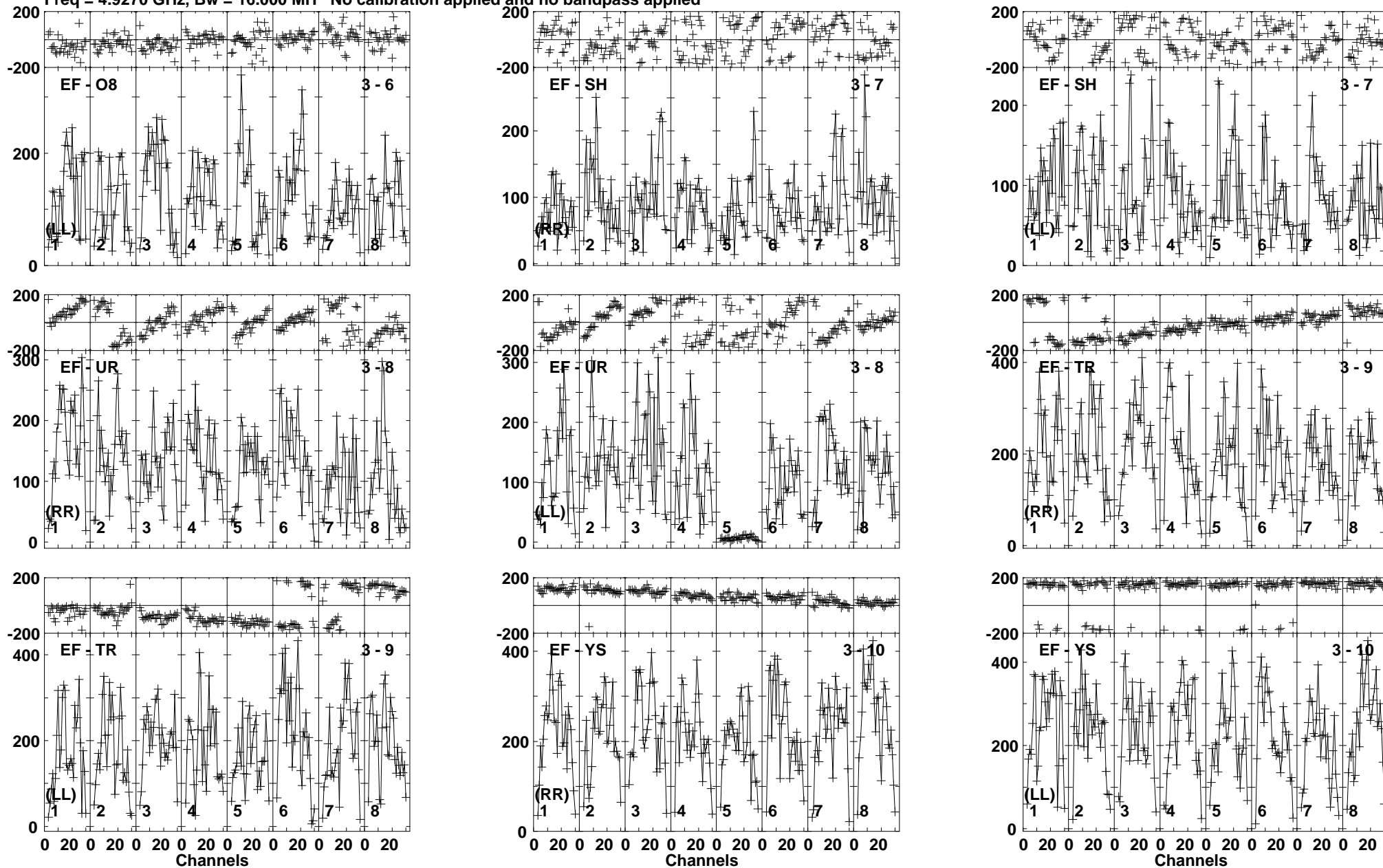
Lower frame: Micro Ampl Jy Top frame: Phas deg Vector averaged cross-power spectrum Baseline: EF (03) - O8 (06) Timerange: 01/03:23:30 to 01/03:26:52
