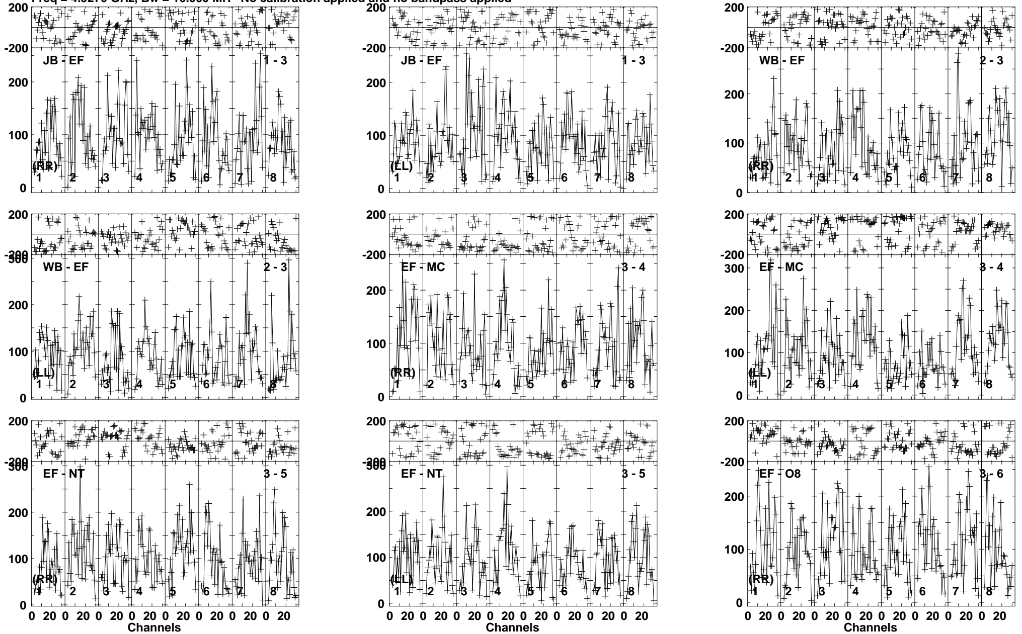
Lower frame: Micro Ampl Jy Top frame: Phas deg Vector averaged cross-power spectrum Baseline: JB (01) - EF (03) Timerange: 01/10:59:58 to 01/11:03:22
