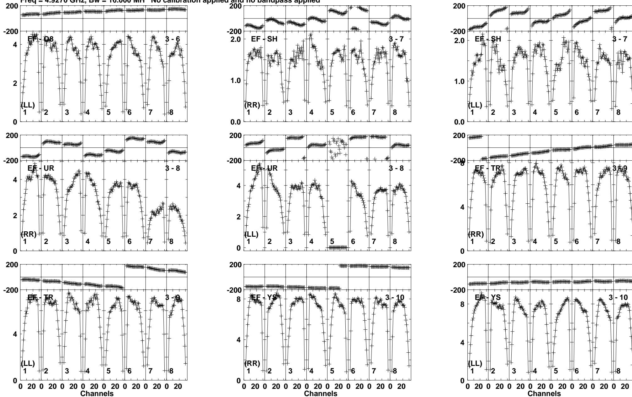
Lower frame: Milli Ampl Jy Top frame: Phas deg Vector averaged cross-power spectrum Baseline: EF (03) - O8 (06) Timerange: 00/21:47:02 to 00/21:48:22
