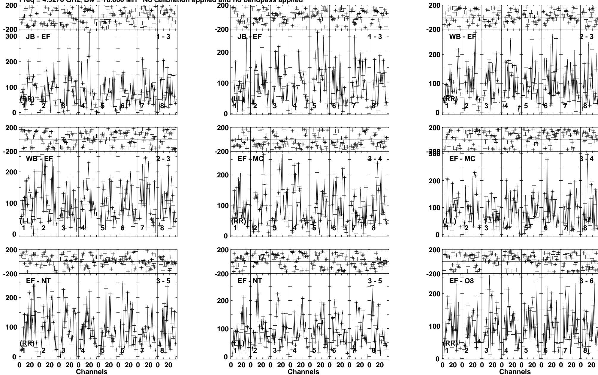
Lower frame: Micro Ampl Jy Top frame: Phas deg Vector averaged cross-power spectrum Baseline: JB (01) - EF (03) Timerange: 01/07:46:31 to 01/07:49:51
