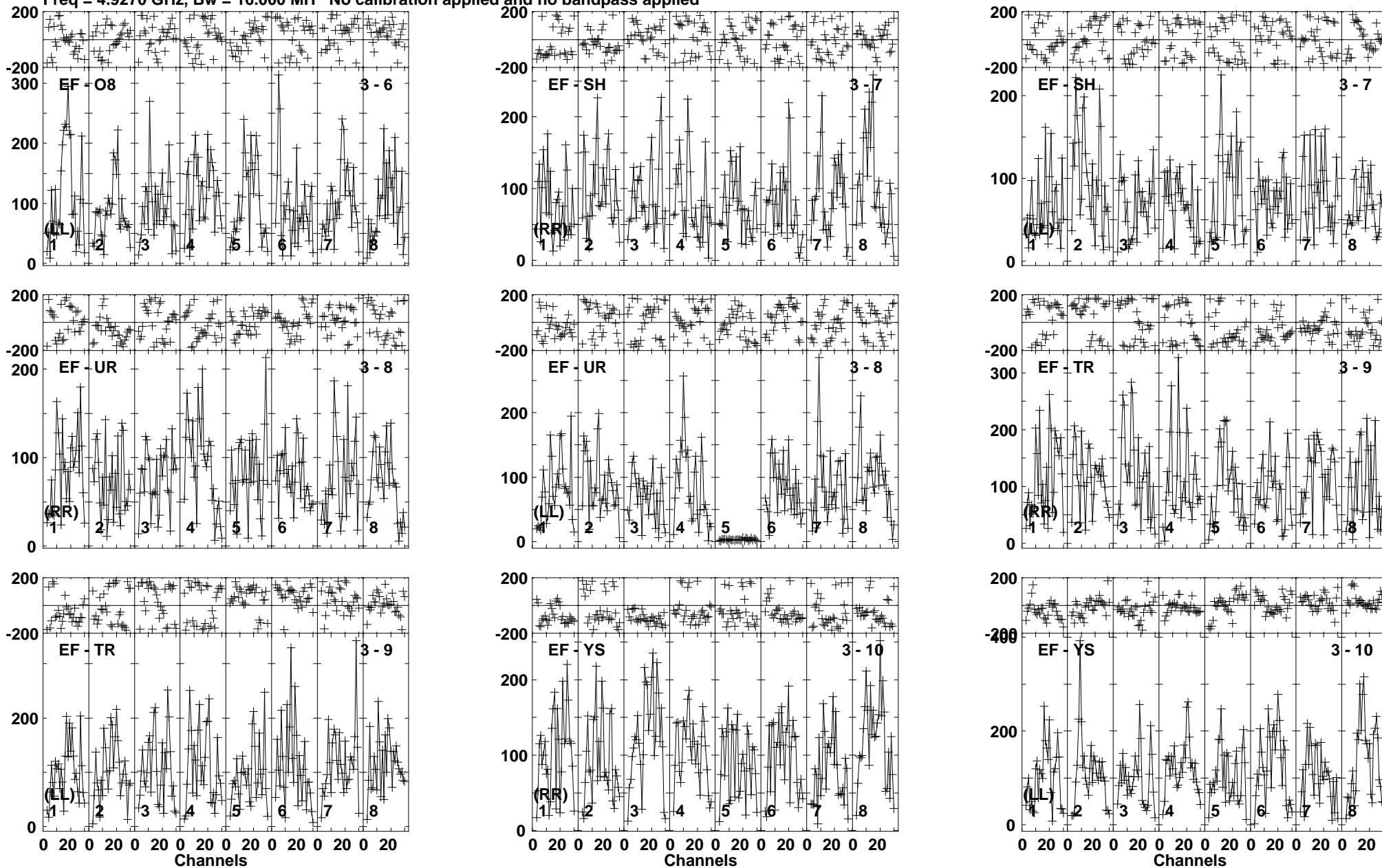
Lower frame: Micro Ampl Jy Top frame: Phas deg Vector averaged cross-power spectrum Baseline: EF (03) - O8 (06) Timerange: 01/01:27:59 to 01/01:31:21
