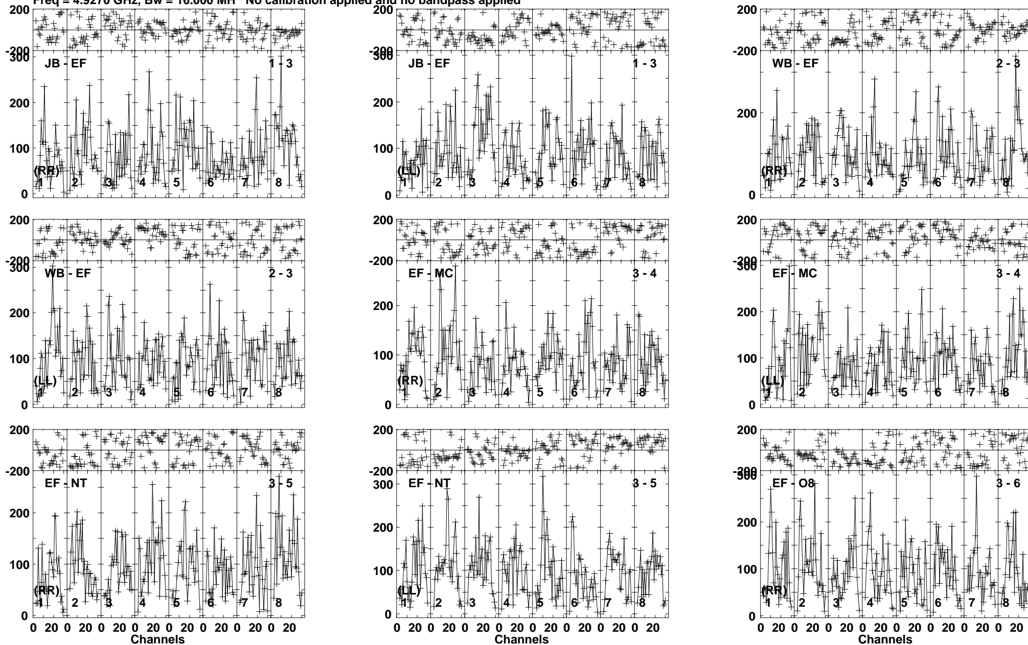
Lower frame: Micro Ampl Jy Top frame: Phas deg Vector averaged cross-power spectrum Baseline: JB (01) - EF (03) Timerange: 01/10:39:02 to 01/10:42:22
