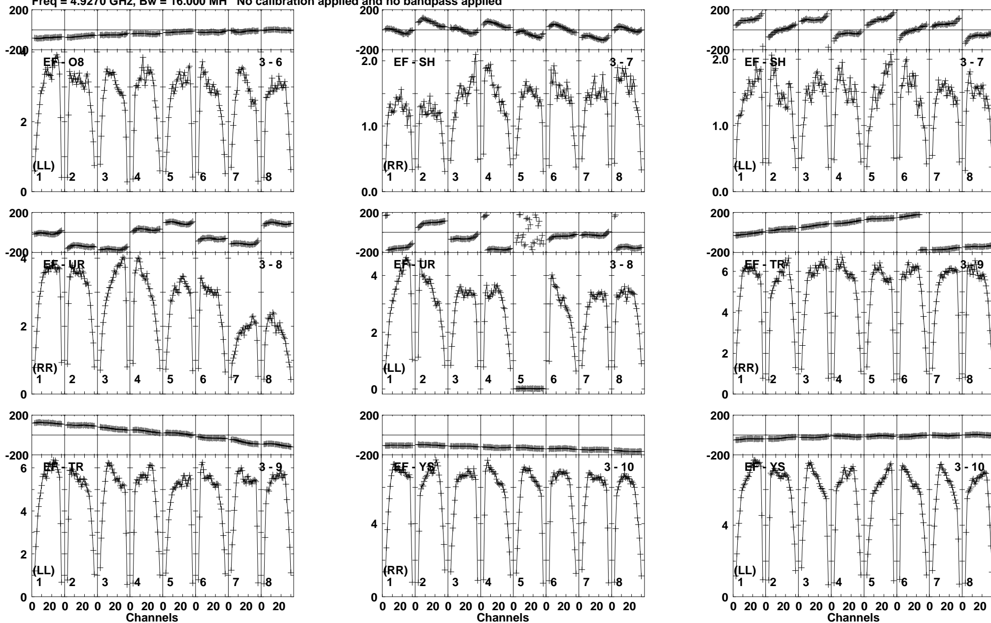
Lower frame: Milli Ampl Jy Top frame: Phas deg Vector averaged cross-power spectrum Baseline: EF (03) - O8 (06) Timerange: 00/20:24:35 to 00/20:25:59
