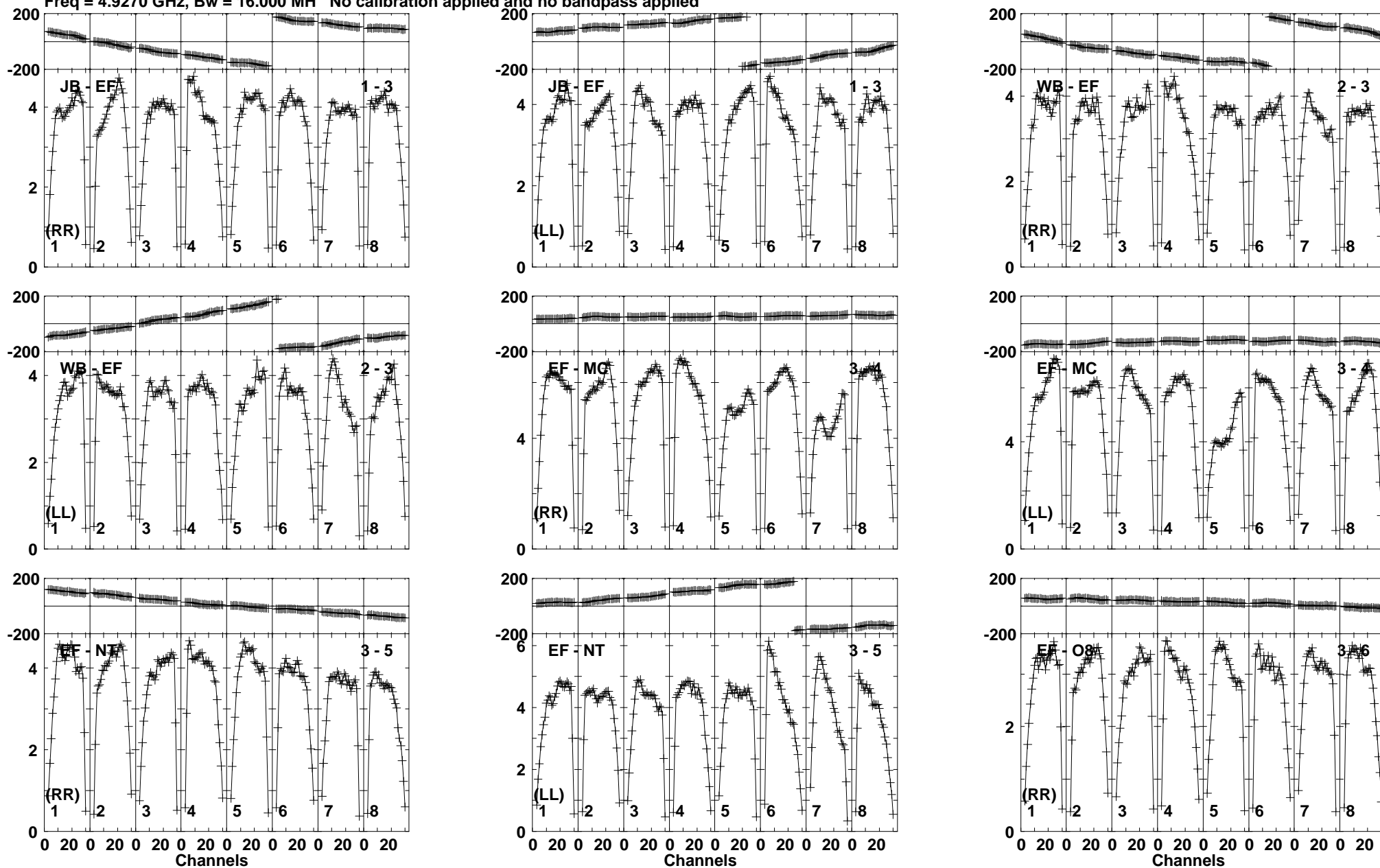
Lower frame: Milli Ampl Jy Top frame: Phas deg Vector averaged cross-power spectrum Baseline: JB (01) - EF (03) Timerange: 00/19:51:03 to 00/19:52:29
