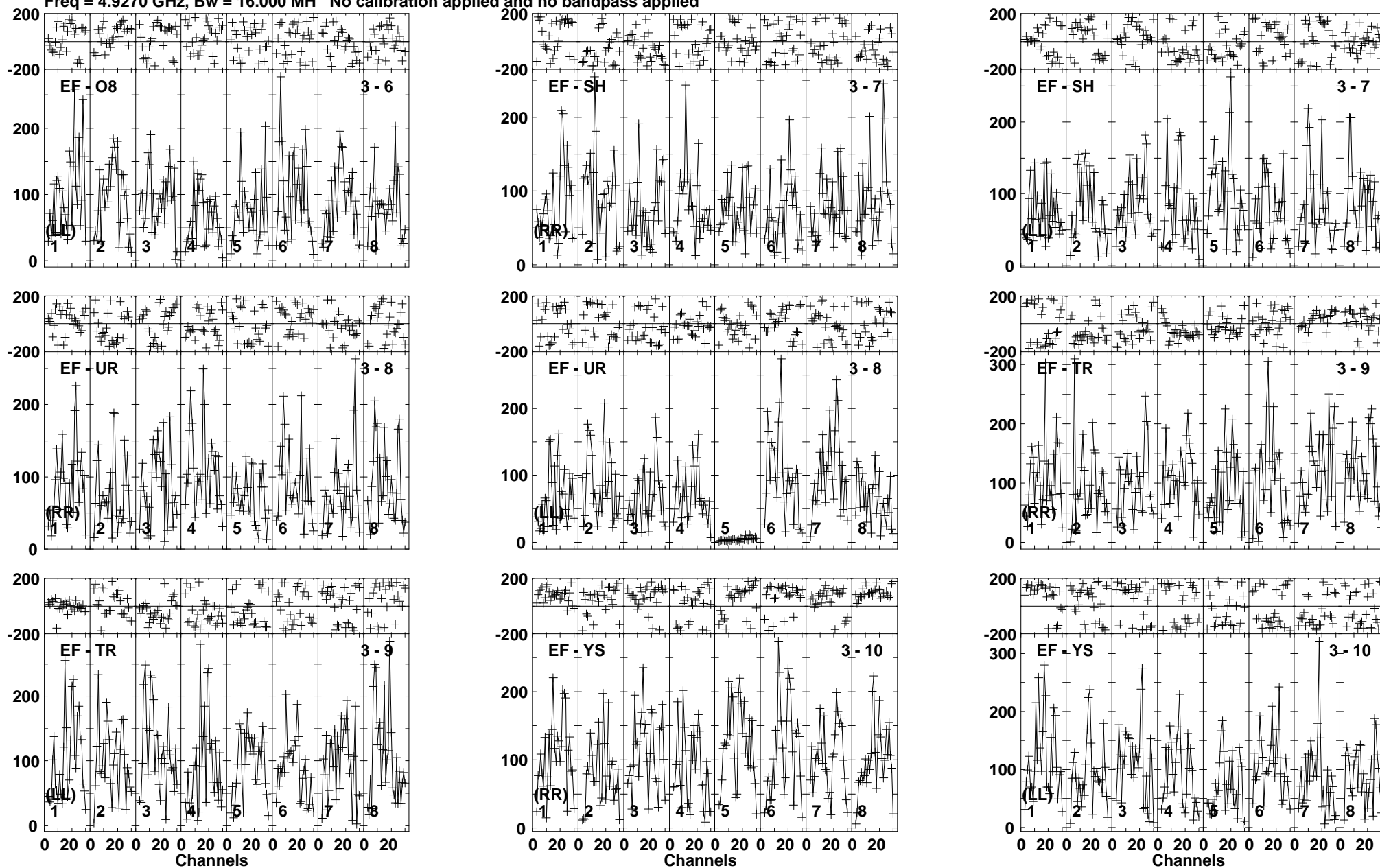
Lower frame: Micro Ampl Jy Top frame: Phas deg Vector averaged cross-power spectrum Baseline: EF (03) - O8 (06) Timerange: 01/01:17:29 to 01/01:20:51
