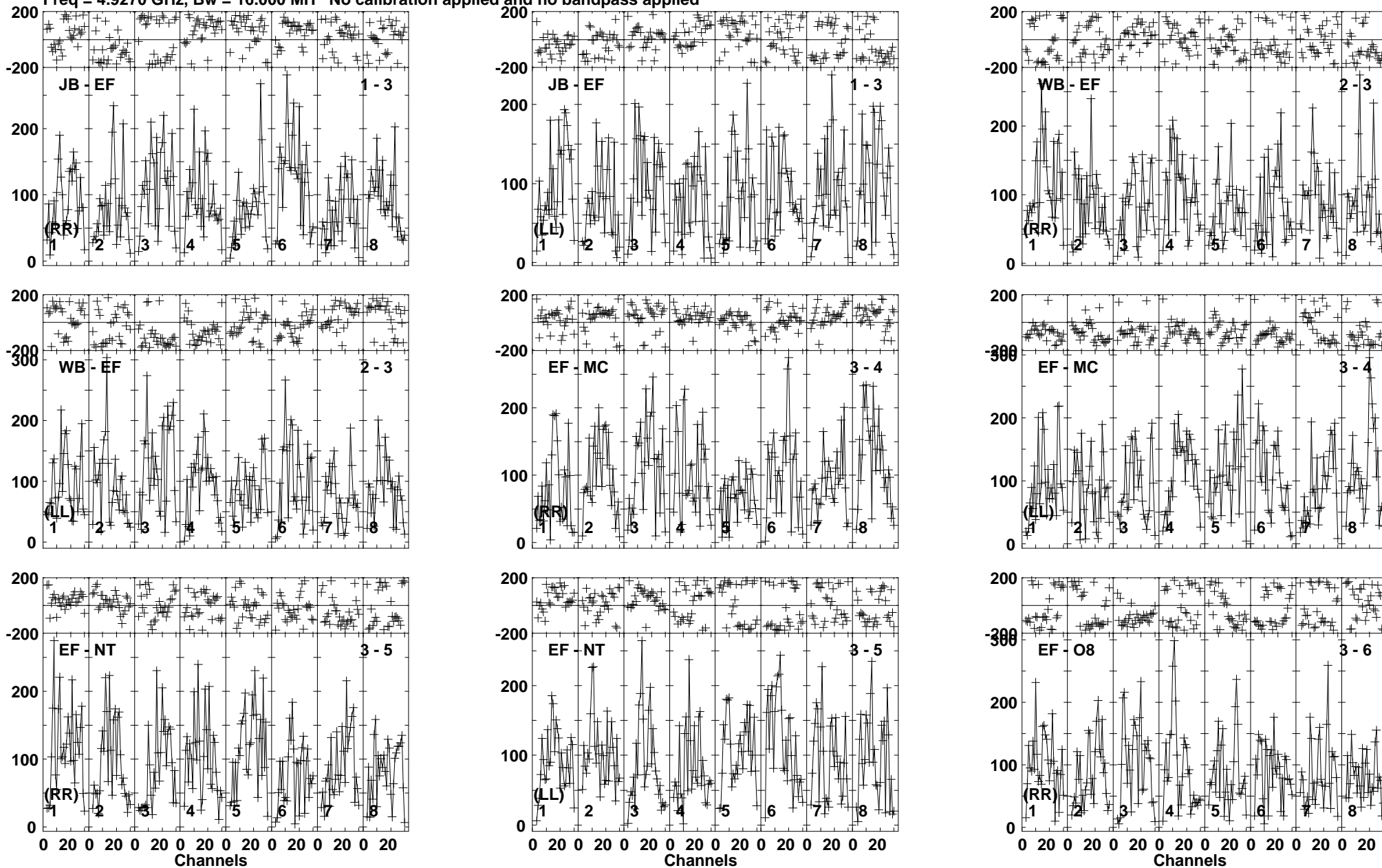
Lower frame: Micro Ampl Jy Top frame: Phas deg Vector averaged cross-power spectrum Baseline: JB (01) - EF (03) Timerange: 01/04:51:59 to 01/04:55:21
