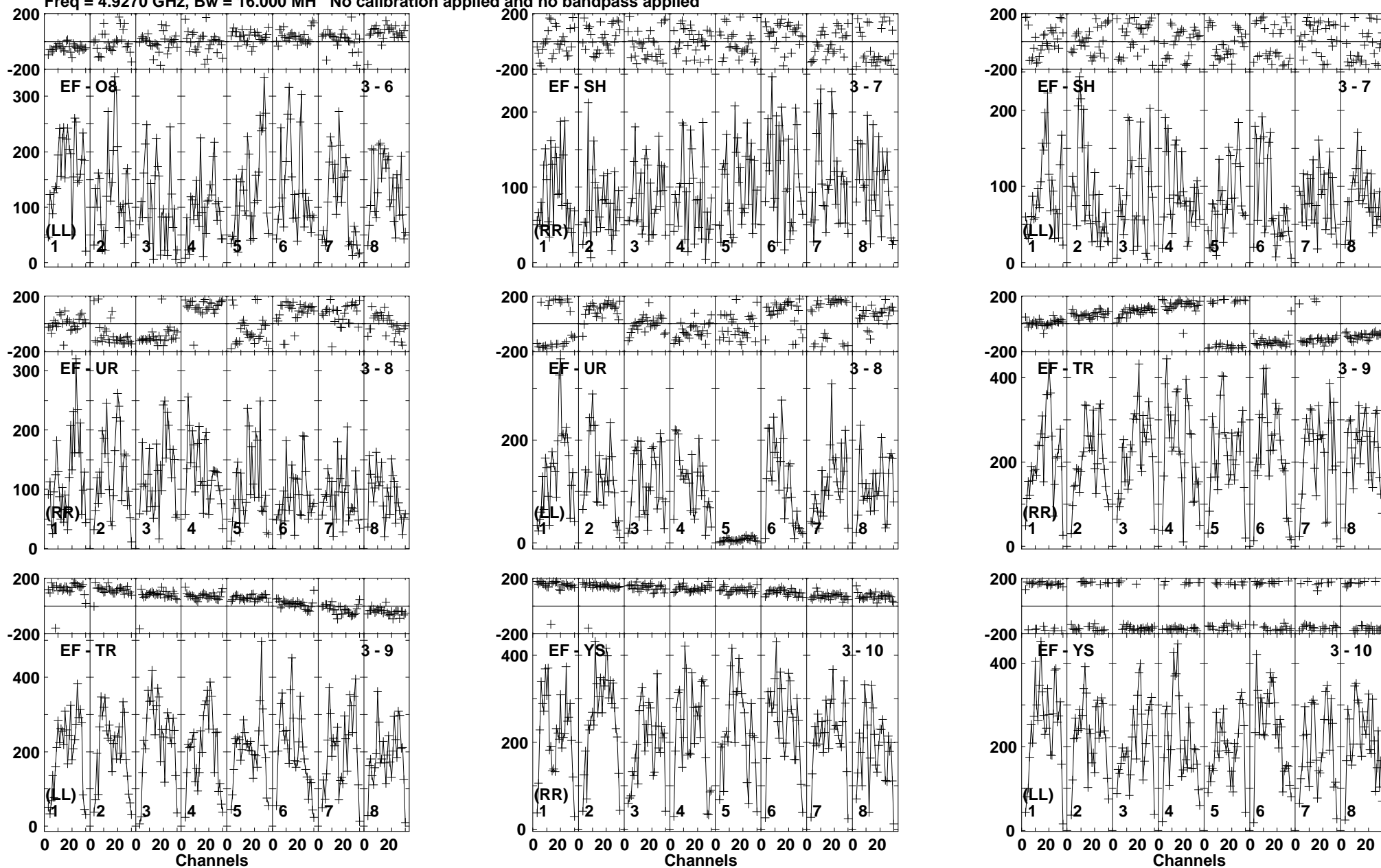
Lower frame: Micro Ampl Jy Top frame: Phas deg Vector averaged cross-power spectrum Baseline: EF (03) - O8 (06) Timerange: 01/04:20:30 to 01/04:23:52
