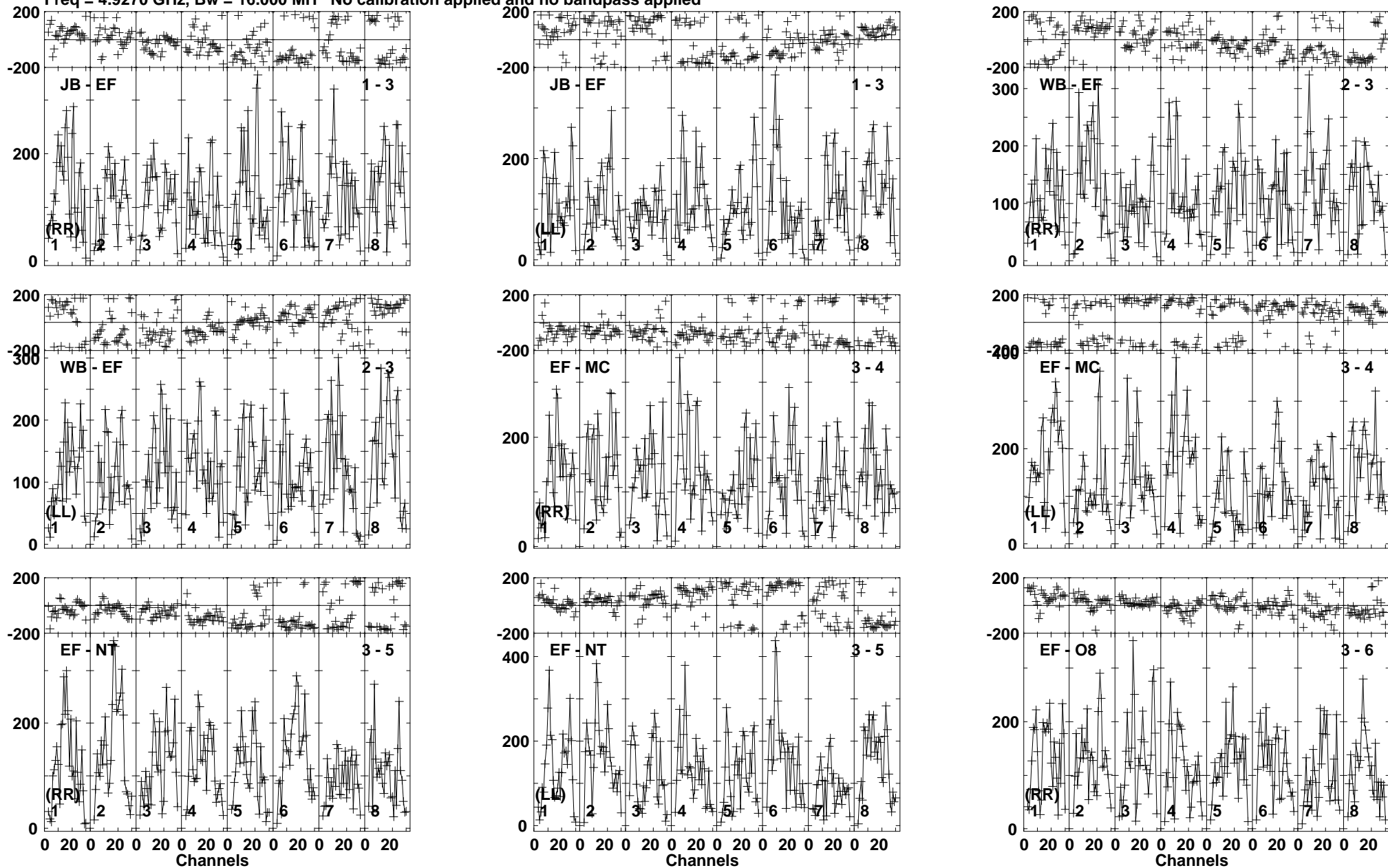
Lower frame: Micro Ampl Jy Top frame: Phas deg Vector averaged cross-power spectrum Baseline: JB (01) - EF (03) Timerange: 01/11:32:17 to 01/11:35:39
