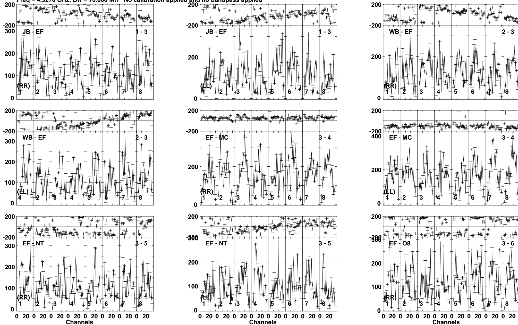
Lower frame: Micro Ampl Jy Top frame: Phas deg Vector averaged cross-power spectrum Baseline: JB (01) - EF (03) Timerange: 01/01:54:00 to 01/01:57:22
