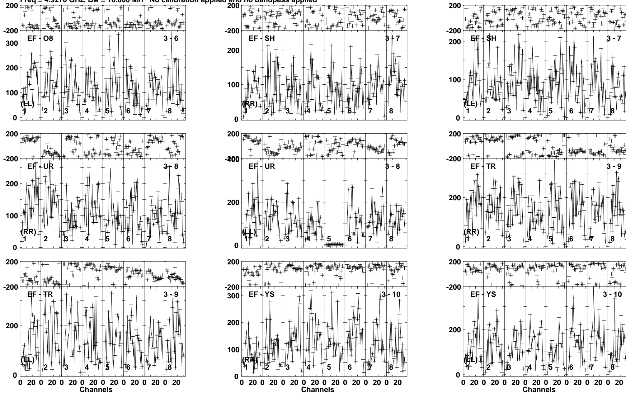
Lower frame: Micro Ampl Jy Top frame: Phas deg Vector averaged cross-power spectrum Baseline: EF (03) - O8 (06) Timerange: 01/11:42:47 to 01/11:46:09
