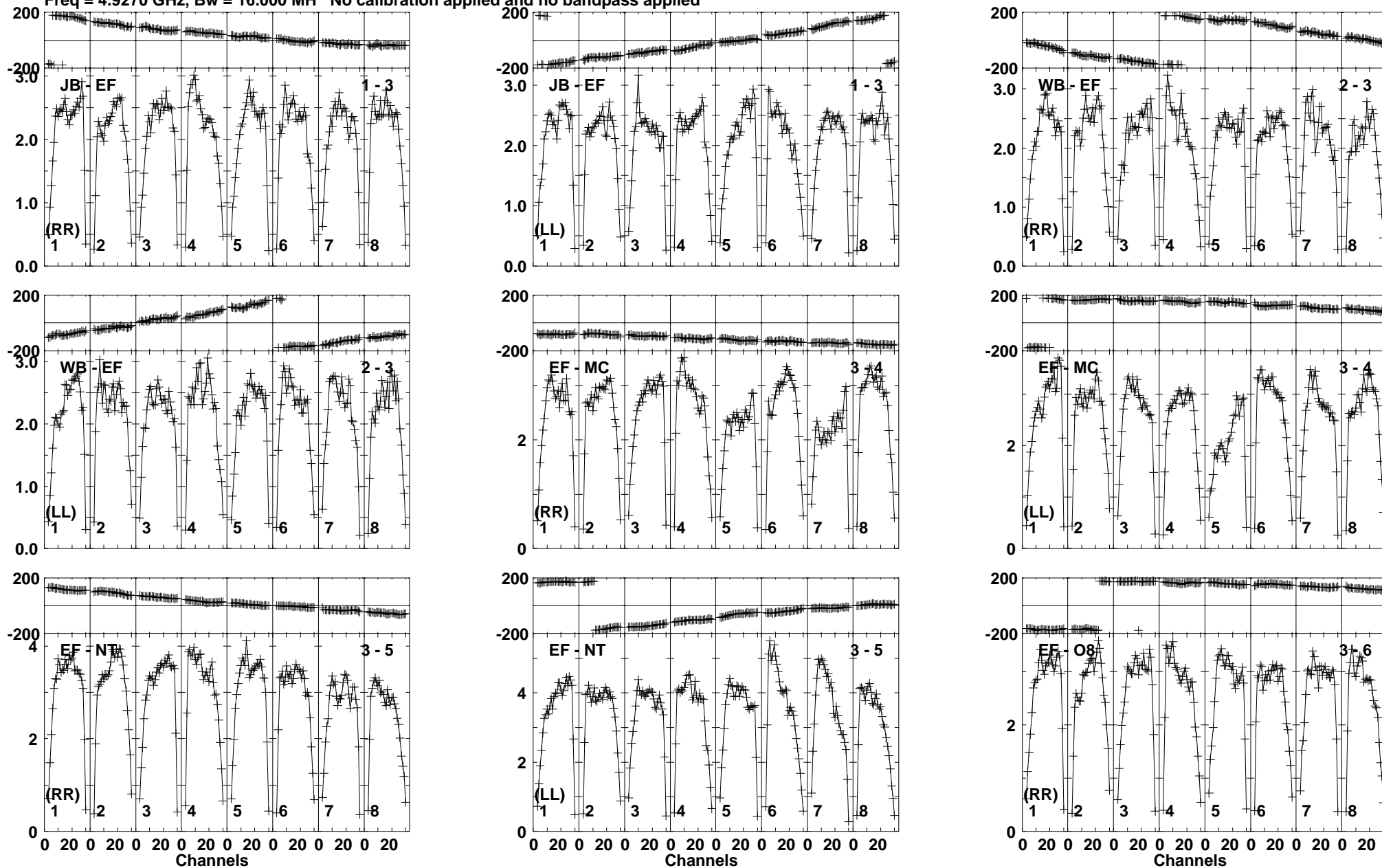
Lower frame: Milli Ampl Jy Top frame: Phas deg Vector averaged cross-power spectrum Baseline: JB (01) - EF (03) Timerange: 01/10:37:32 to 01/10:38:52
