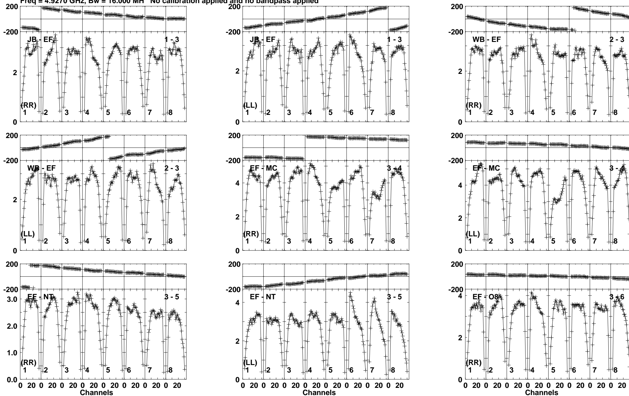
Lower frame: Milli Ampl Jy Top frame: Phas deg Vector averaged cross-power spectrum Baseline: JB (01) - EF (03) Timerange: 01/11:20:13 to 01/11:21:39
