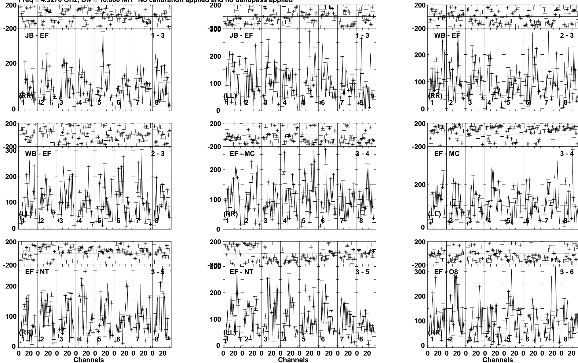
Lower frame: Micro Ampl Jy Top frame: Phas deg Vector averaged cross-power spectrum Baseline: JB (01) - EF (03) Timerange: 01/05:02:30 to 01/05:05:52
