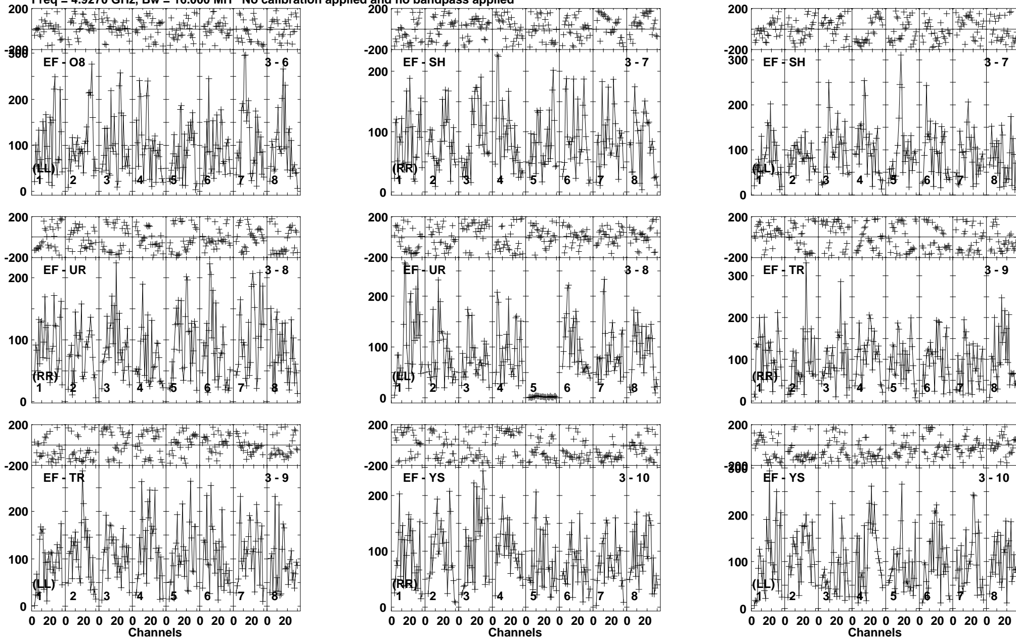
Lower frame: Micro Ampl Jy Top frame: Phas deg Vector averaged cross-power spectrum Baseline: EF (03) - O8 (06) Timerange: 01/09:23:31 to 01/09:26:51
