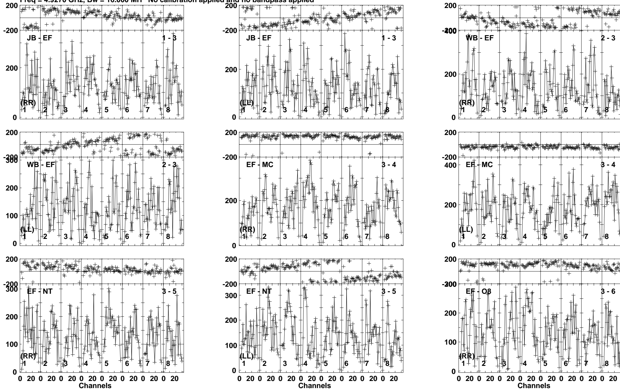
Lower frame: Micro Ampl Jy Top frame: Phas deg Vector averaged cross-power spectrum Baseline: JB (01) - EF (03) Timerange: 01/03:28:30 to 01/03:31:52
