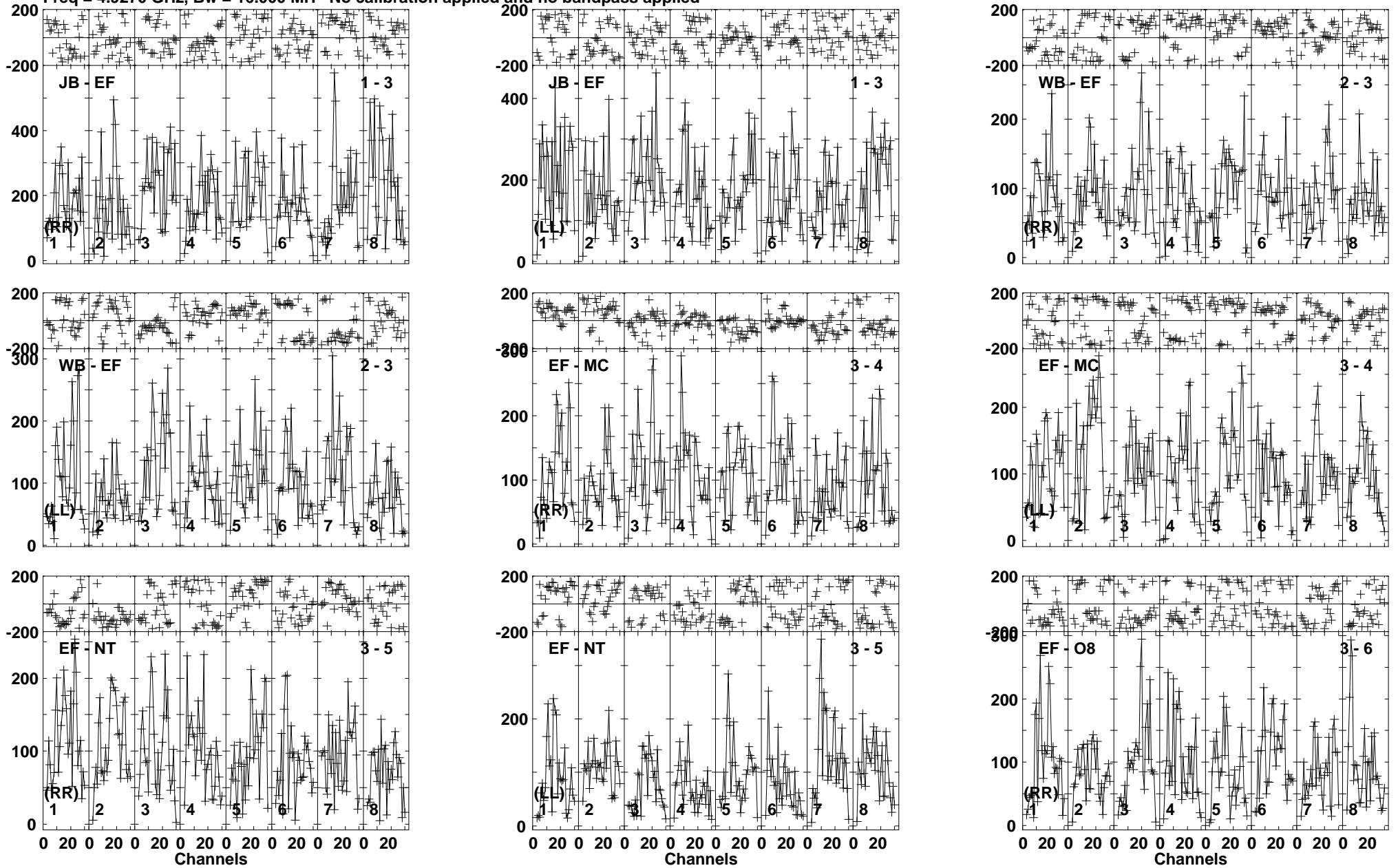
Lower frame: Micro Ampl Jy Top frame: Phas deg Vector averaged cross-power spectrum Baseline: JB (01) - EF (03) Timerange: 01/12:38:13 to 01/12:41:39
