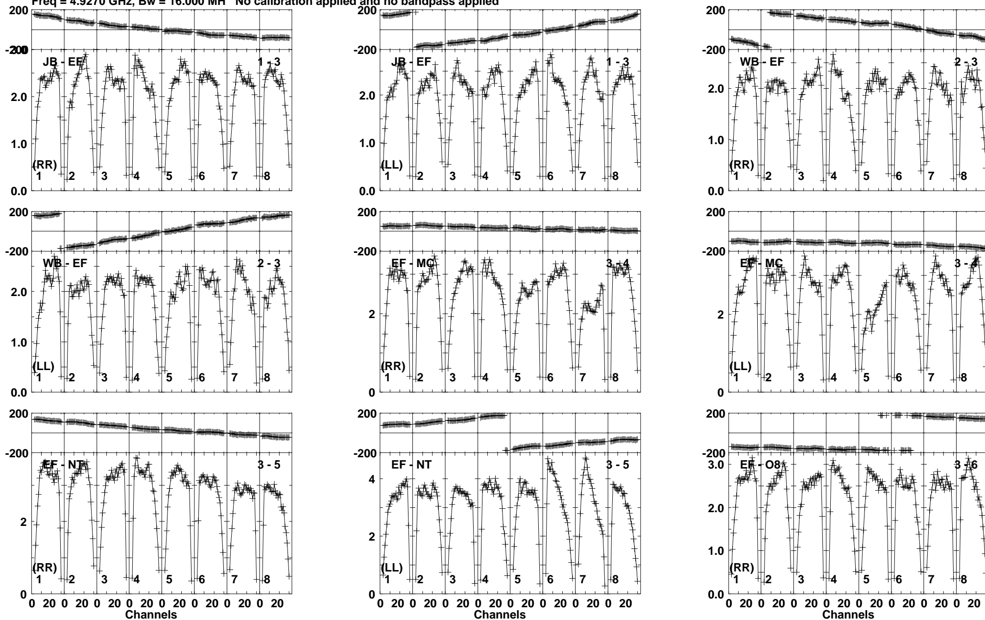
Lower frame: Milli Ampl Jy Top frame: Phas deg Vector averaged cross-power spectrum Baseline: JB (01) - EF (03) Timerange: 01/07:31:24 to 01/07:32:52
