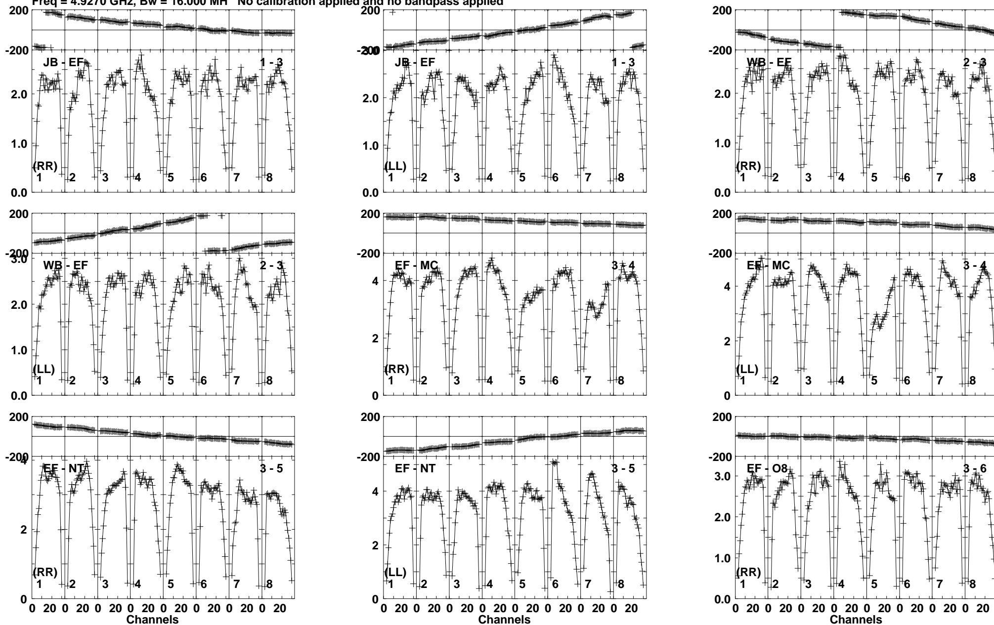
Lower frame: Milli Ampl Jy Top frame: Phas deg Vector averaged cross-power spectrum Baseline: JB (01) - EF (03) Timerange: 01/11:14:24 to 01/11:15:52
