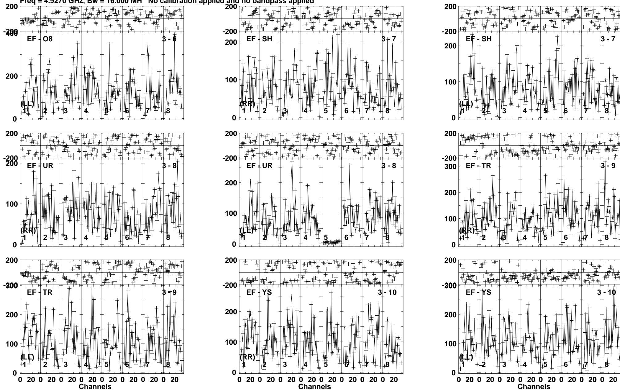
Lower frame: Micro Ampl Jy Top frame: Phas deg Vector averaged cross-power spectrum Baseline: EF (03) - O8 (06) Timerange: 01/01:22:59 to 01/01:26:21
