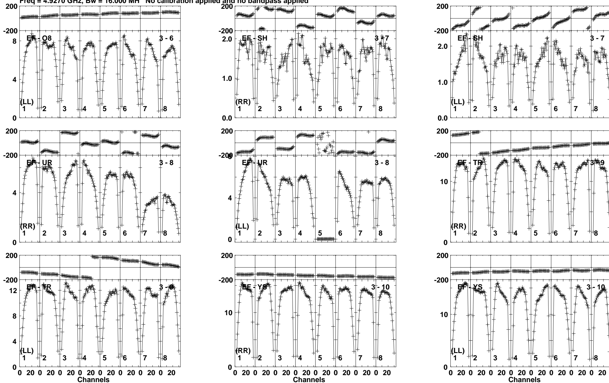
Lower frame: Milli Amply Jy Top frame: Phas deg Vector averaged cross-power spectrum Baseline: EF (03) - O8 (06) Timerange: 01/04:08:30 to 01/04:09:52
