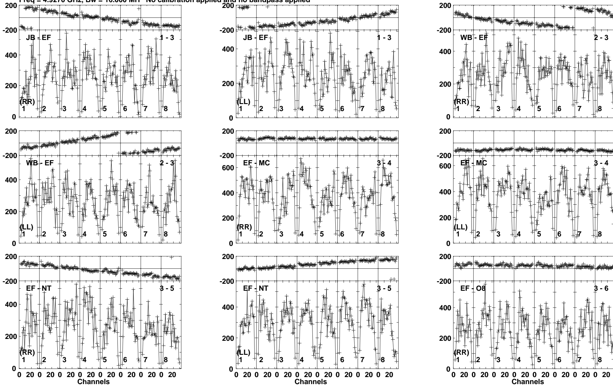
Lower frame: Micro Ampl Jy Top frame: Phas deg Vector averaged cross-power spectrum Baseline: JB (01) - EF (03) Timerange: 00/21:05:05 to 00/21:08:29
