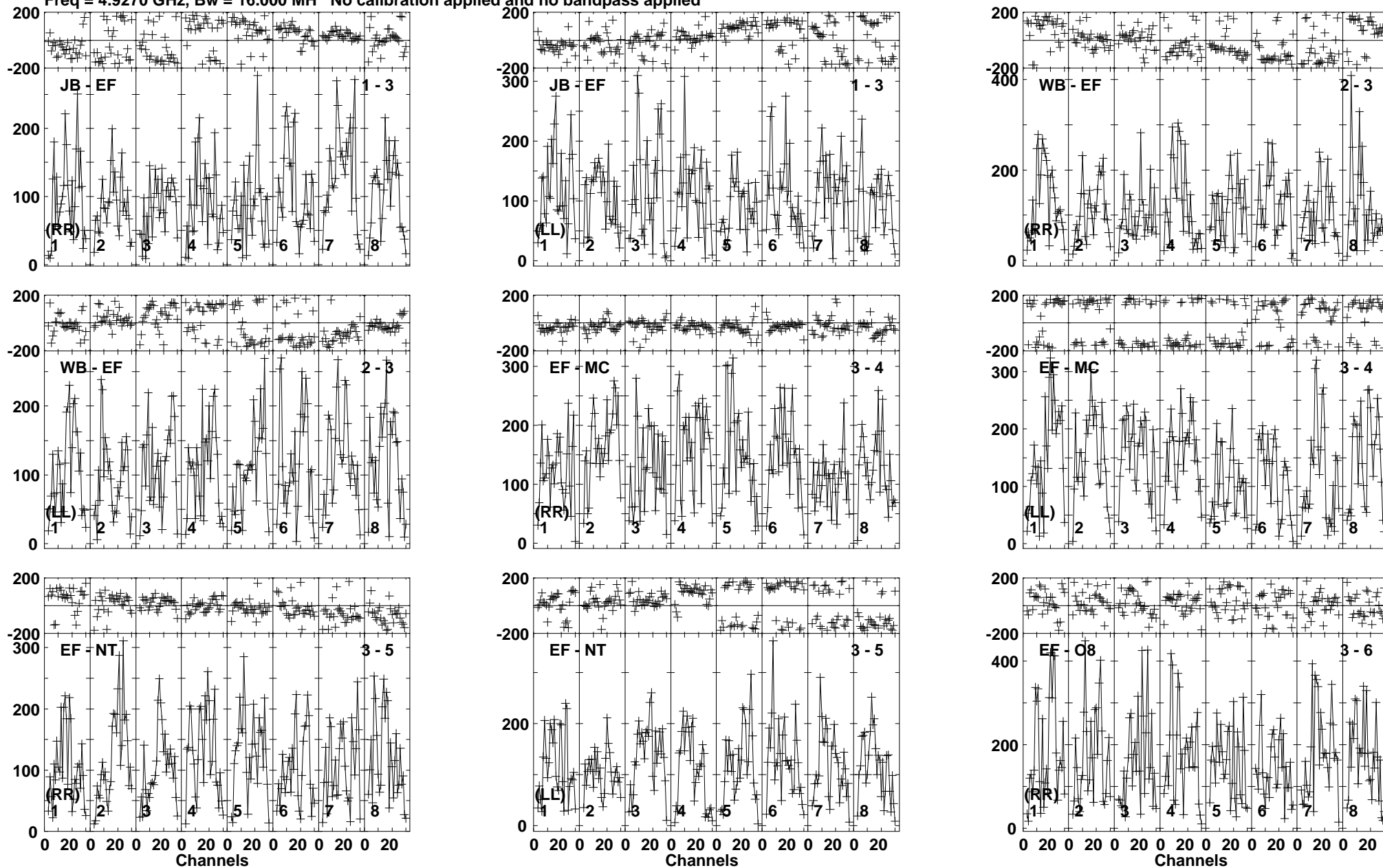
Lower frame: Micro Ampl Jy Top frame: Phas deg Vector averaged cross-power spectrum Baseline: JB (01) - EF (03) Timerange: 01/00:45:31 to 01/00:48:53
