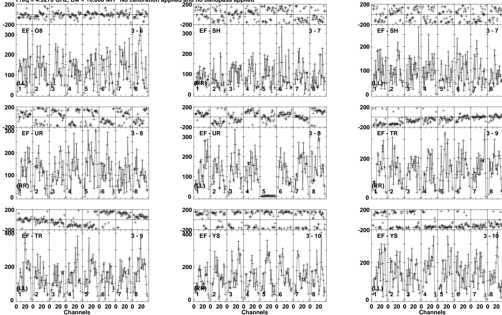
Lower frame: Micro Ampl Jy Top frame: Phas deg Vector averaged cross-power spectrum Baseline: EF (03) - O8 (06) Timerange: 01/09:43:30 to 01/09:46:52
