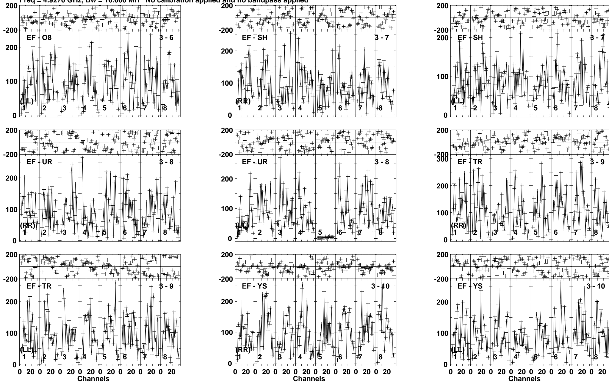
Lower frame: Micro Ampl Jy Top frame: Phas deg Vector averaged cross-power spectrum Baseline: EF (03) - O8 (06) Timerange: 01/12:38:13 to 01/12:41:39
