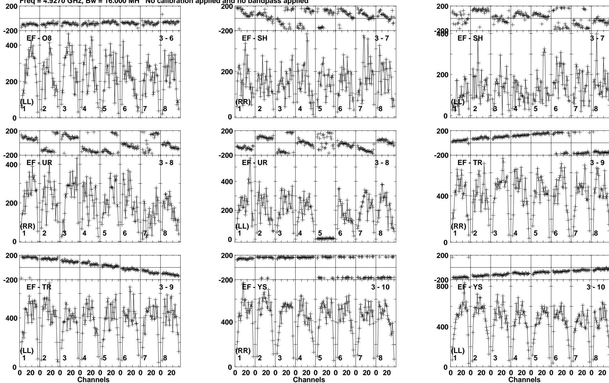
Lower frame: Micro Ampl Jy Top frame: Phas deg Vector averaged cross-power spectrum Baseline: EF (03) - O8 (06) Timerange: 00/20:46:38 to 00/20:49:58
