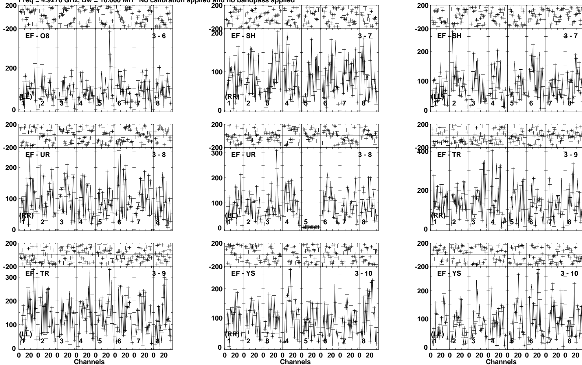
Lower frame: Micro Ampl Jy Top frame: Phas deg Vector averaged cross-power spectrum Baseline: EF (03) - O8 (06) Timerange: 01/11:10:28 to 01/11:13:52
