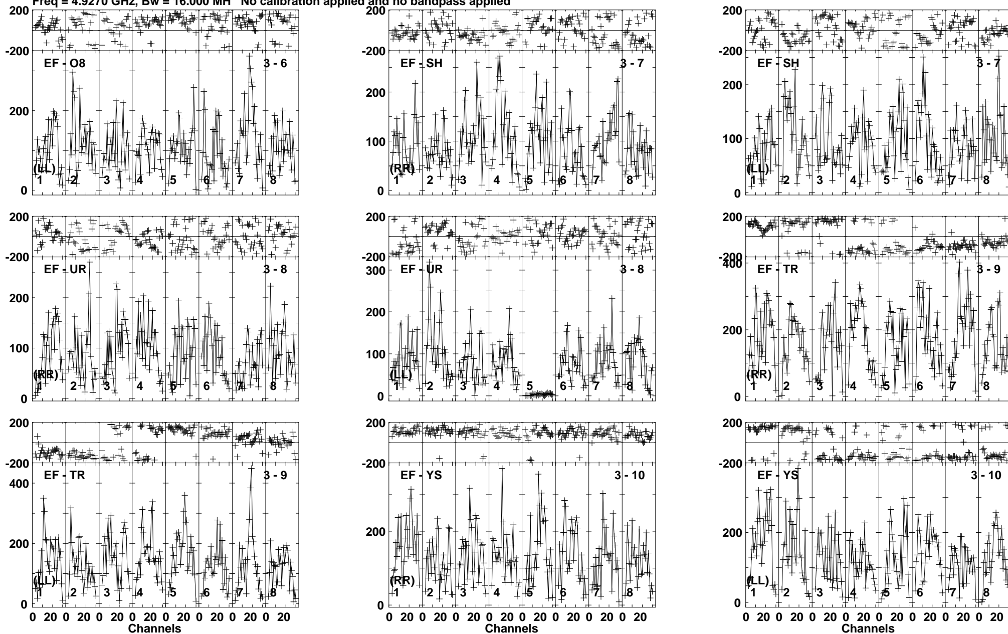
Lower frame: Micro Ampl Jy Top frame: Phas deg Vector averaged cross-power spectrum Baseline: EF (03) - O8 (06) Timerange: 01/06:47:57 to 01/06:51:21
