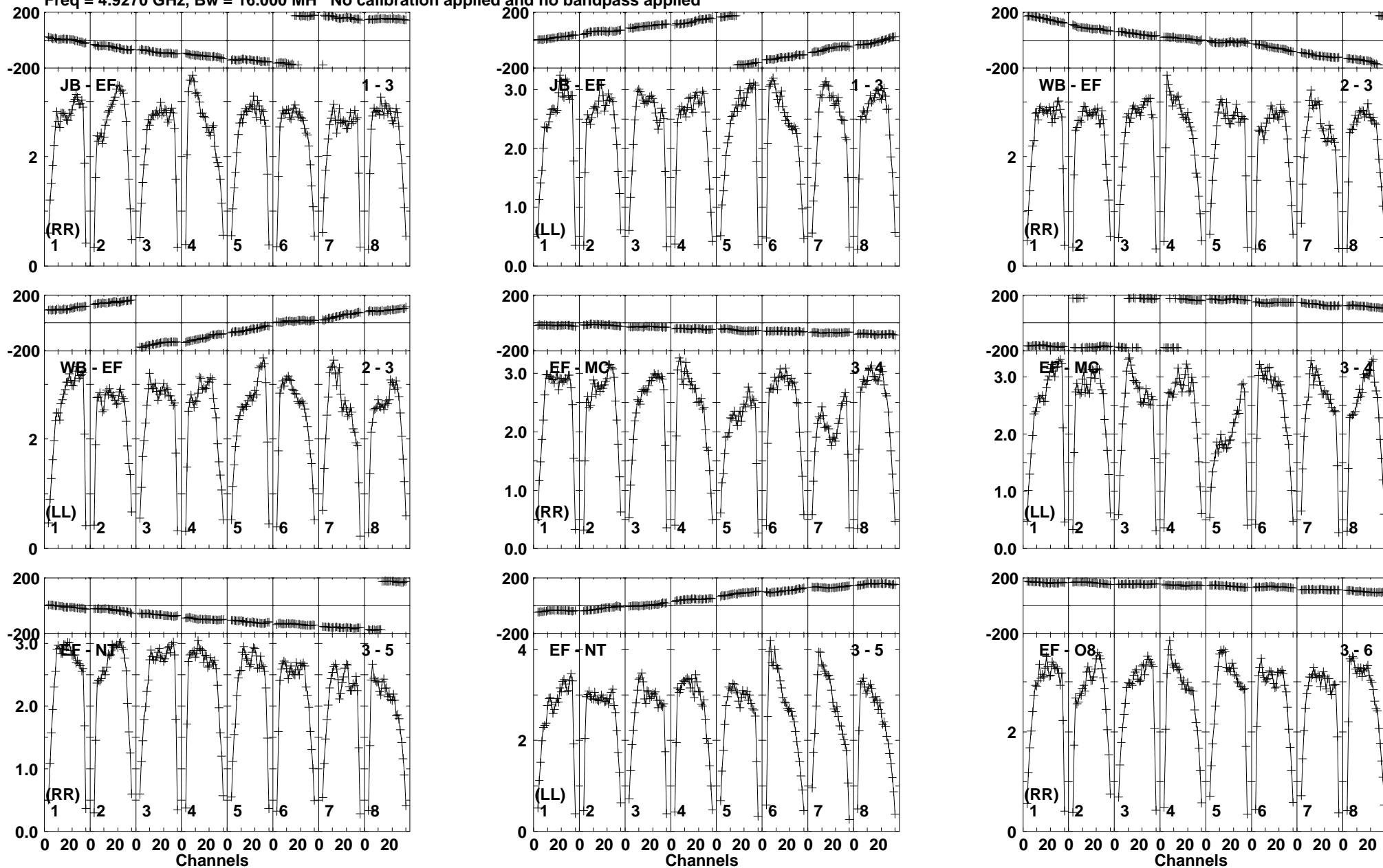
Lower frame: Milli Ampl Jy Top frame: Phas deg Vector averaged cross-power spectrum Baseline: JB (01) - EF (03) Timerange: 01/09:41:56 to 01/09:43:22
