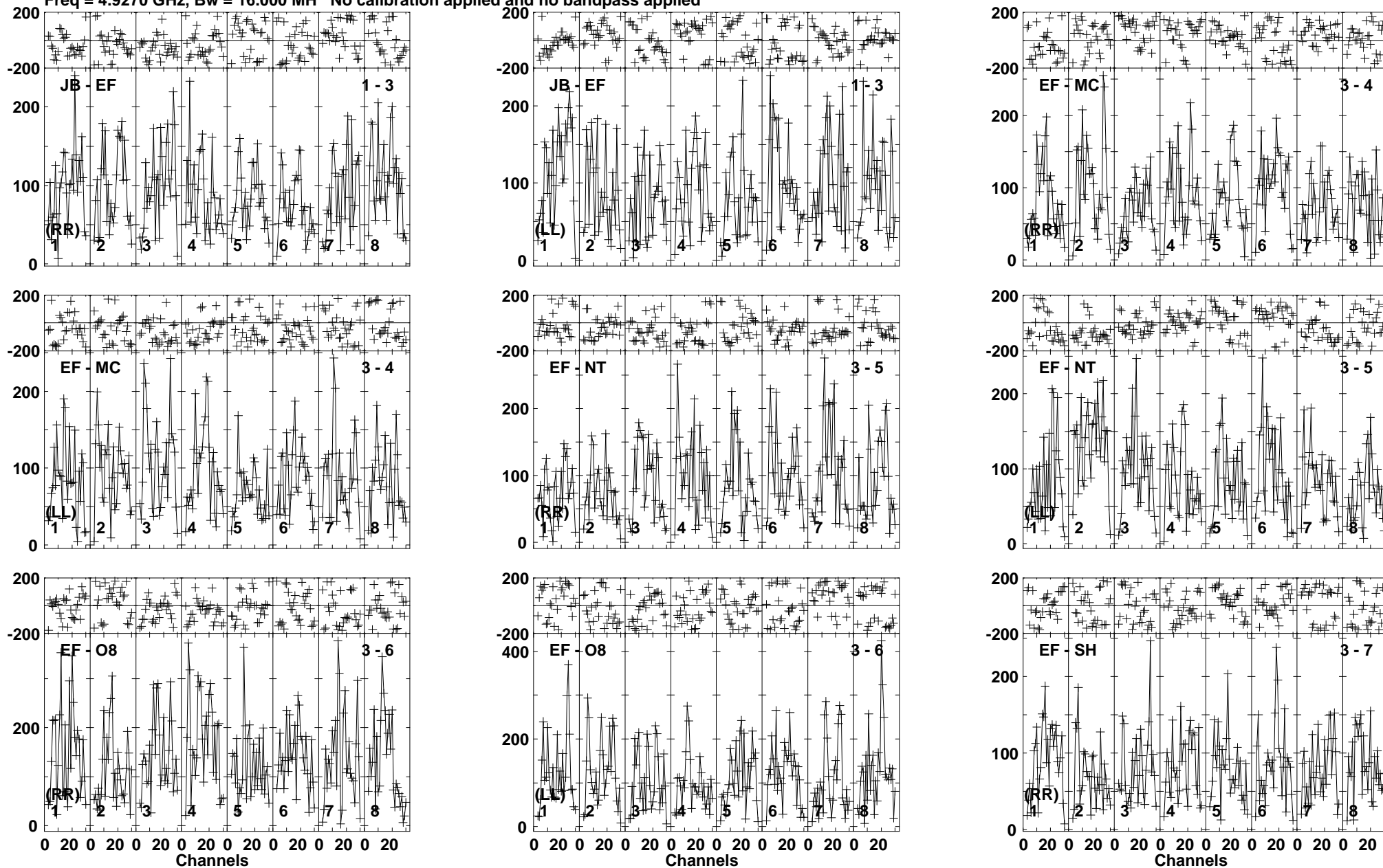
Lower frame: Micro Ampl Jy Top frame: Phas deg Vector averaged cross-power spectrum Baseline: JB (01) - EF (03) Timerange: 01/05:55:00 to 01/05:58:22
