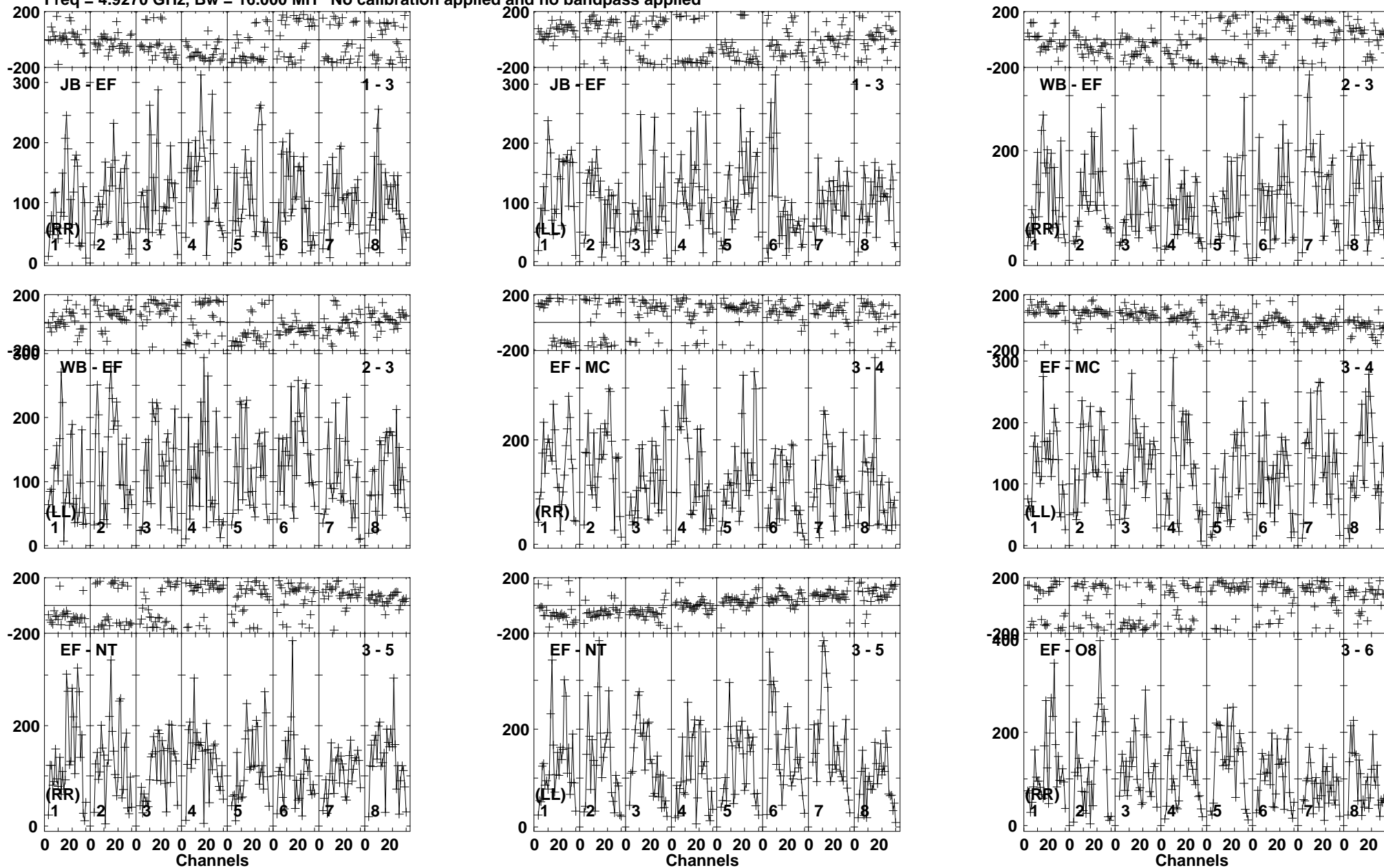
Lower frame: Micro Ampl Jy Top frame: Phas deg Vector averaged cross-power spectrum Baseline: JB (01) - EF (03) Timerange: 01/11:47:45 to 01/11:51:09
