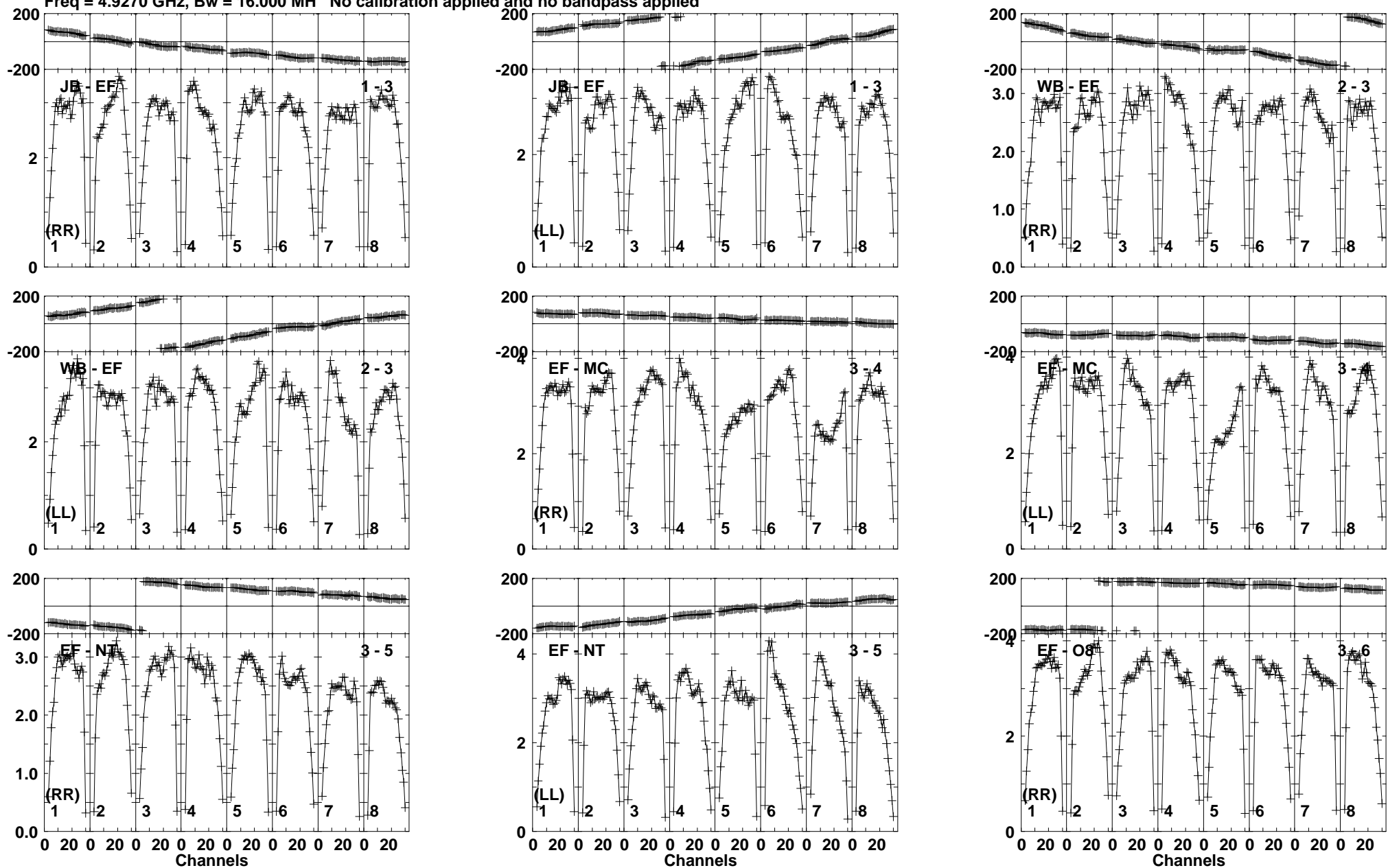
Lower frame: Milli Ampl Jy Top frame: Phas deg Vector averaged cross-power spectrum Baseline: JB (01) - EF (03) Timerange: 01/10:13:26 to 01/10:14:52
