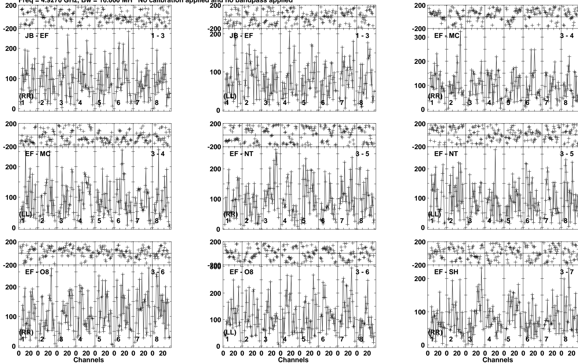
Lower frame: Micro Ampl Jy Top frame: Phas deg Vector averaged cross-power spectrum Baseline: JB (01) - EF (03) Timerange: 01/05:39:30 to 01/05:42:52
