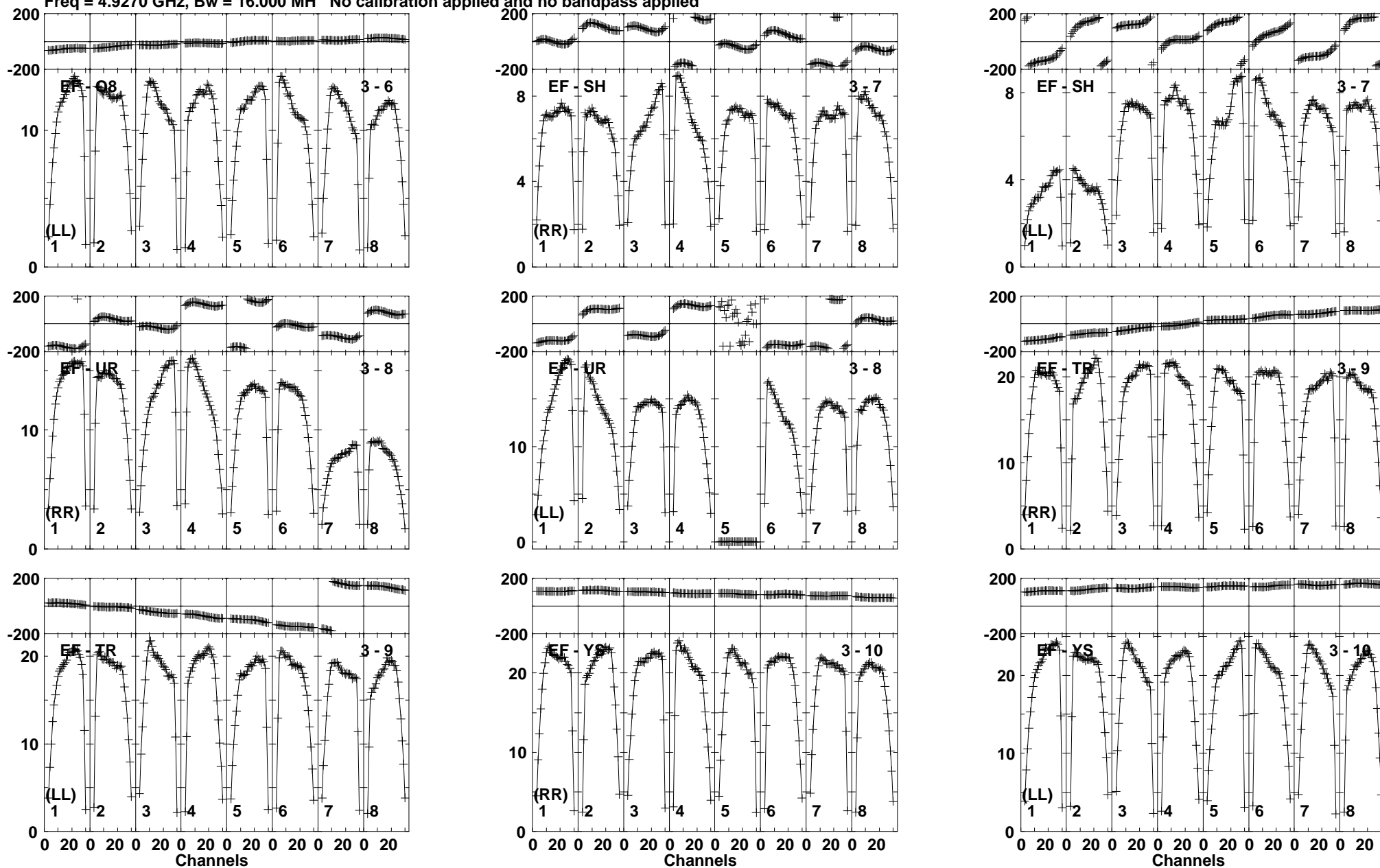
Lower frame: Milli Amply Jy Top frame: Phas deg Vector averaged cross-power spectrum Baseline: EF (03) - O8 (06) Timerange: 01/05:06:00 to 01/05:07:22
