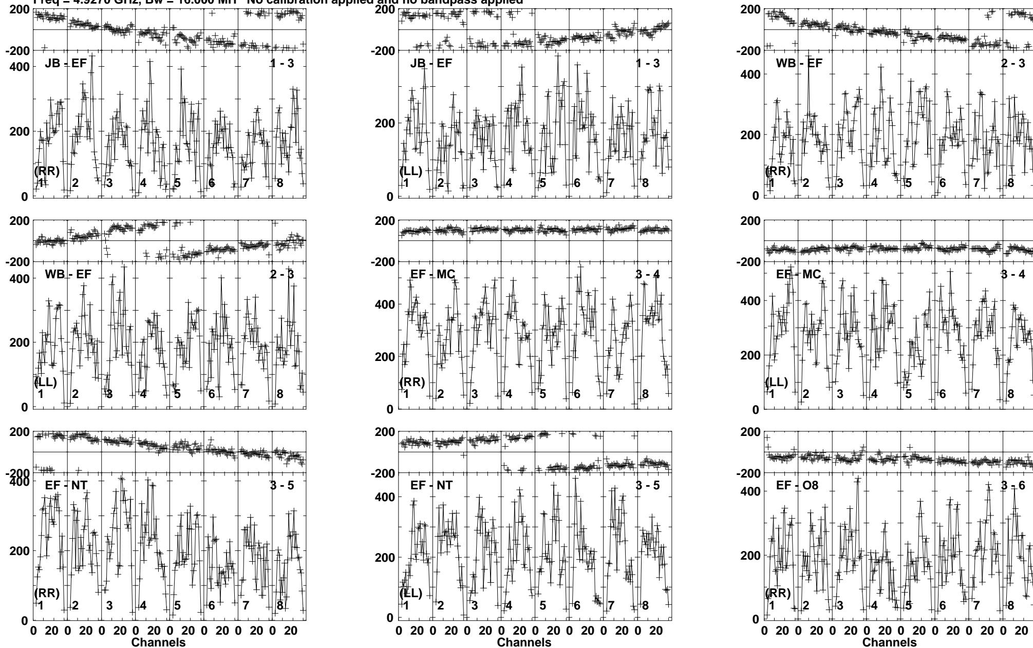
Lower frame: Micro Ampl Jy Top frame: Phas deg Vector averaged cross-power spectrum Baseline: JB (01) - EF (03) Timerange: 00/20:05:35 to 00/20:08:59
