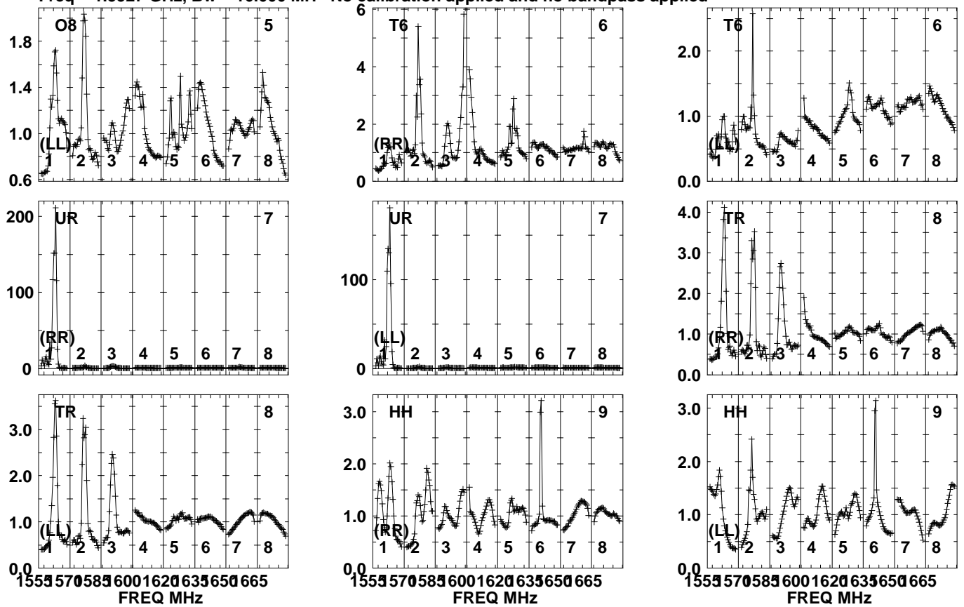
Lower frame: Real Jy Auto-corr total-power spectrum Antenna: * Timerange: 00/03:53:31 to 00/03:54:59
