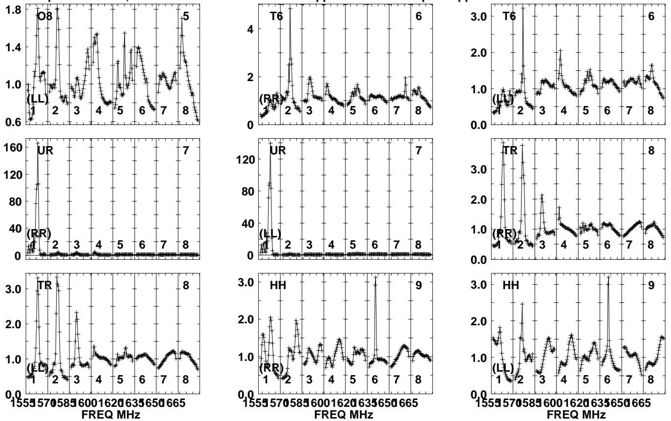
Lower frame: Real Jy Auto-corr total-power spectrum Antenna: * Timerange: 00/02:43:31 to 00/02:44:59
