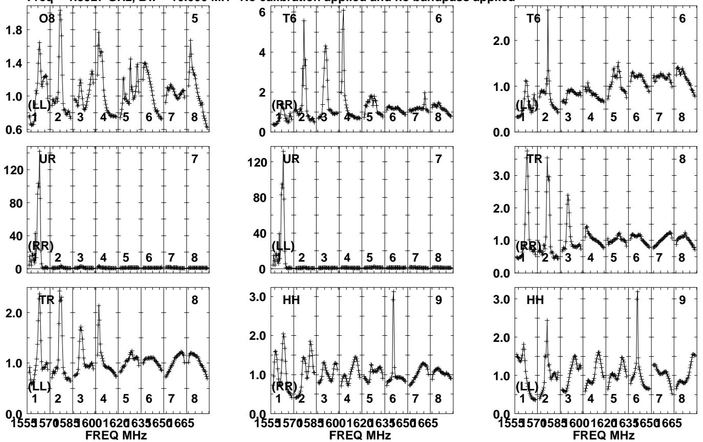
Lower frame: Real Jy Auto-corr total-power spectrum Antenna: * Timerange: 00/02:30:01 to 00/02:33:29
