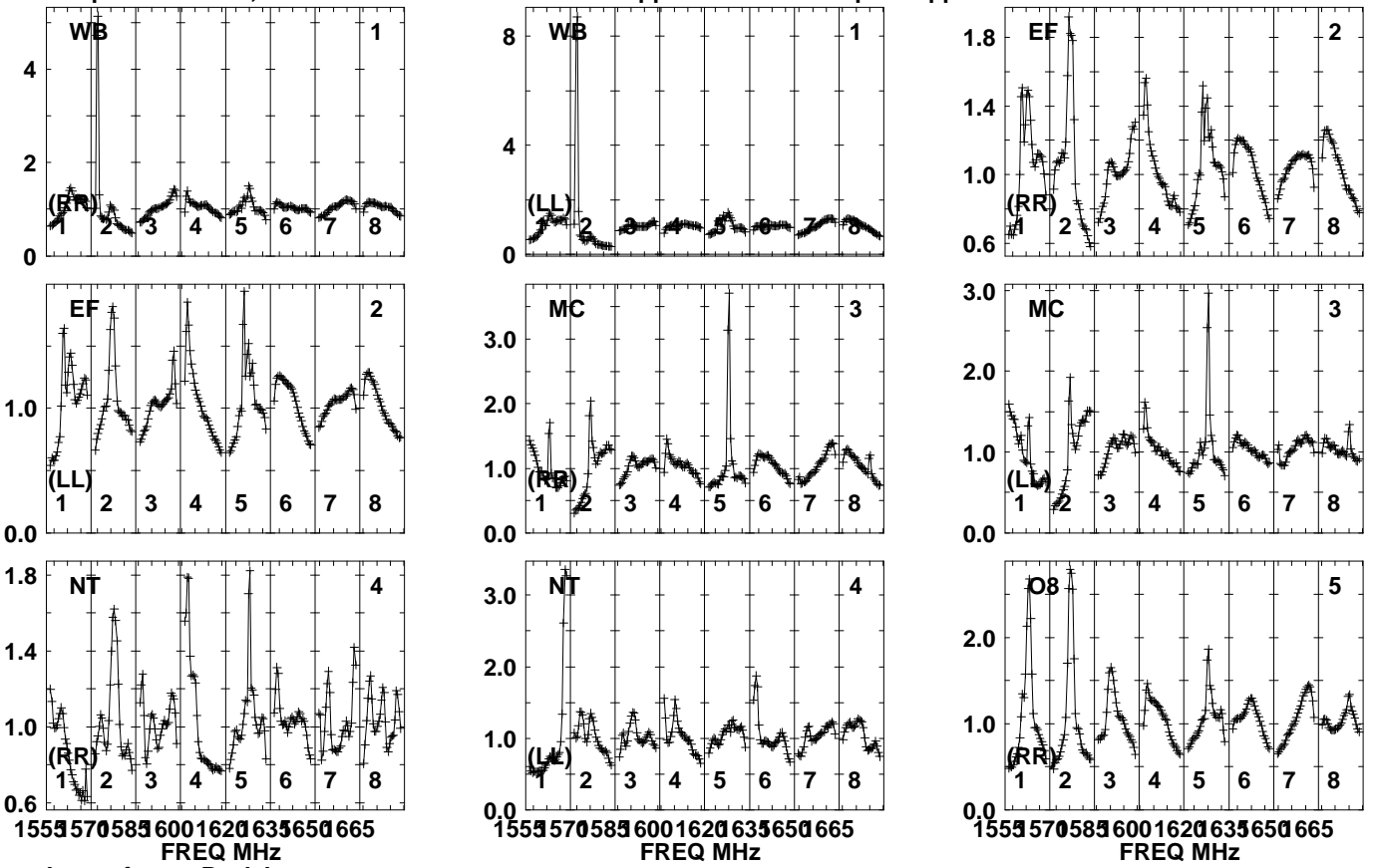
Lower frame: Real Jy Auto-corr total-power spectrum Antenna: * Timerange: 00/02:04:01 to 00/02:04:59
