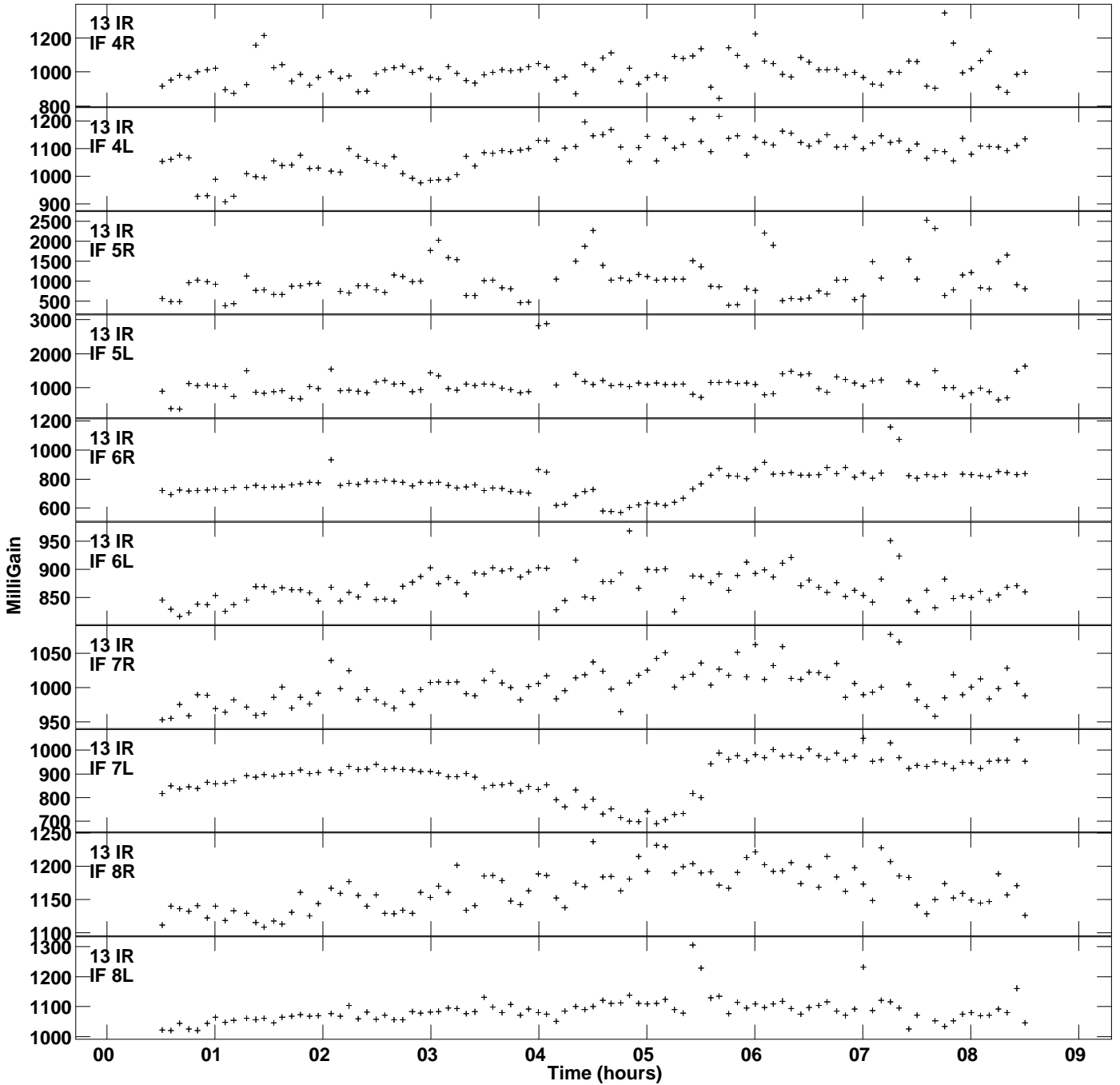
Plot file version 16 created 01-FEB-2023 16:37:45 Gain amp vs UTC time for J1748+3404.MULTI.1 SN 2 Rpol & Lpol IF 1 - 8
