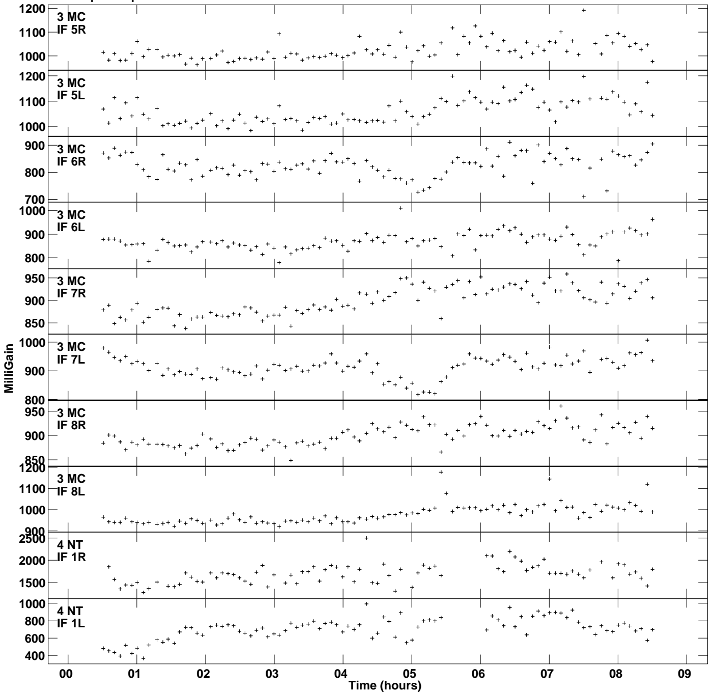
Plot file version 5 created 01-FEB-2023 16:37:45 Gain amp vs UTC time for J1748+3404.MULTI.1 SN 2 Rpol & Lpol IF 1 - 8
