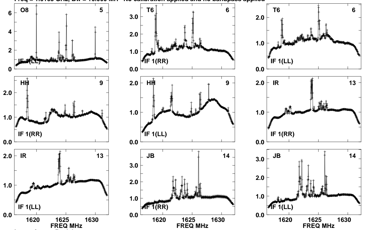
Lower frame: Real Jy Auto-corr total-power spectrum Antenna: * Timerange: 00/04:39:21 to 00/04:40:49
