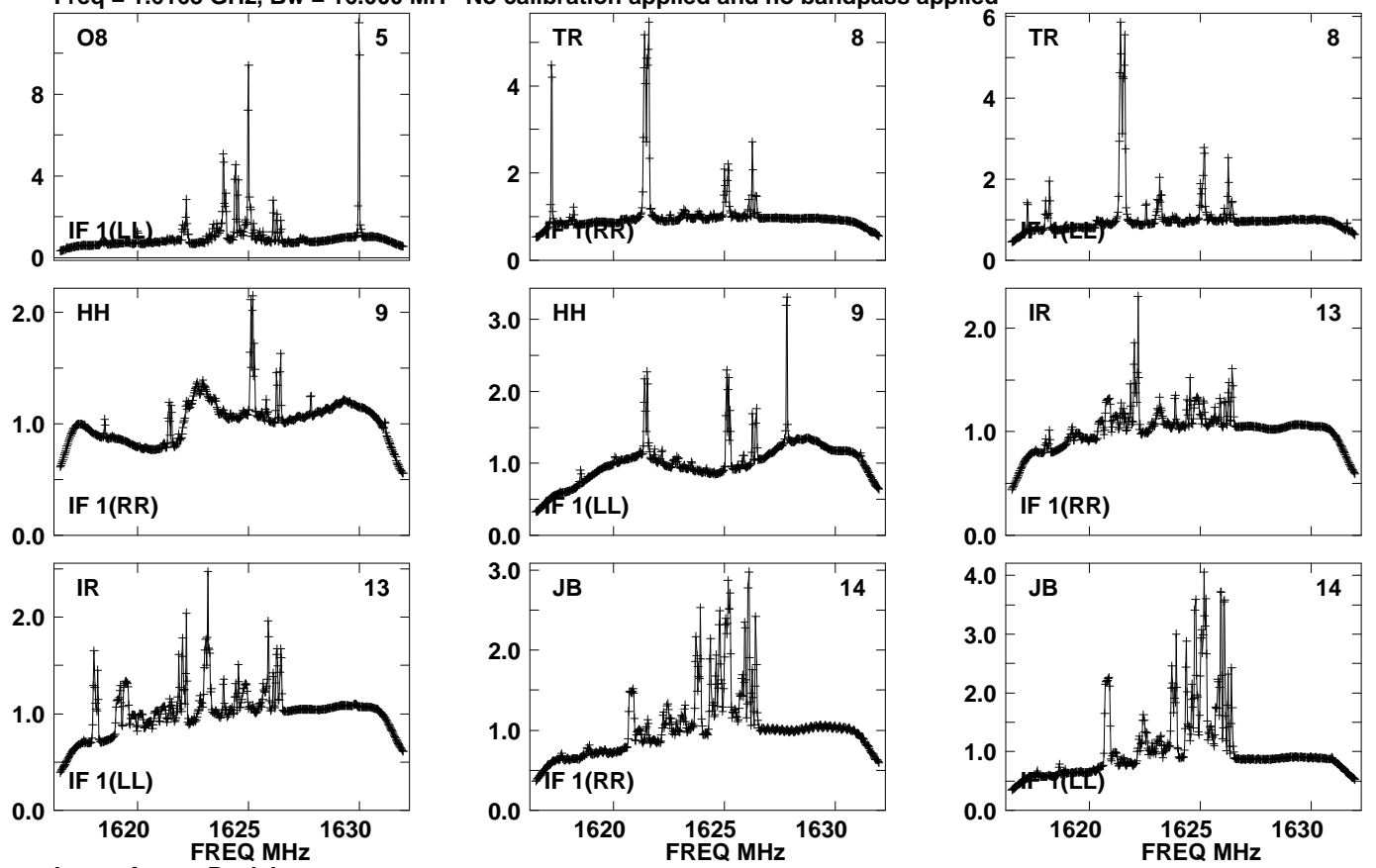
Lower frame: Real Jy Auto-corr total-power spectrum Antenna: * Timerange: 00/08:19:21 to 00/08:20:49
