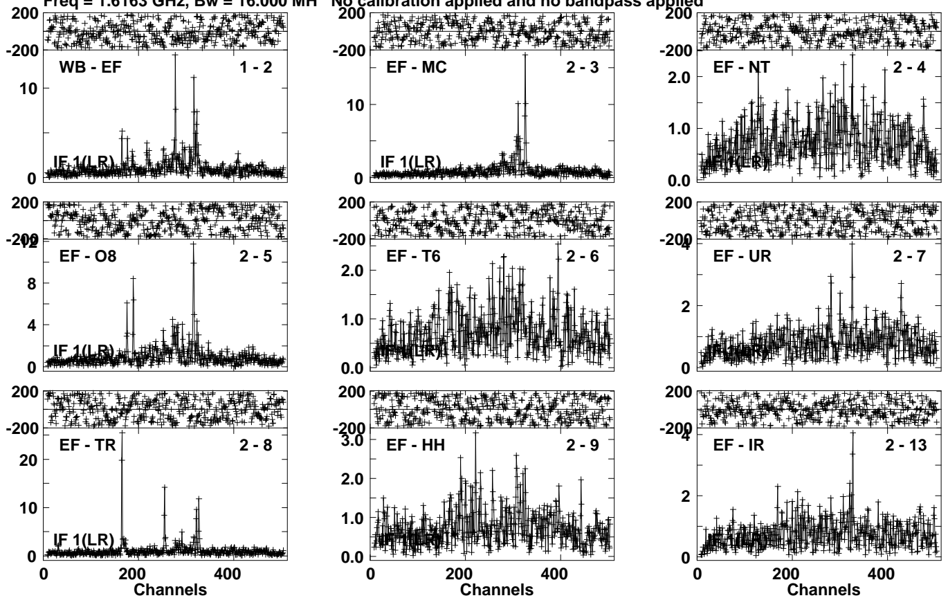
Lower frame: Milli Ampl Jy Top frame: Phas deg Vector averaged cross-power spectrum Several baselines displayed Timerange: 00/03:55:01 to 00/03:58:29
