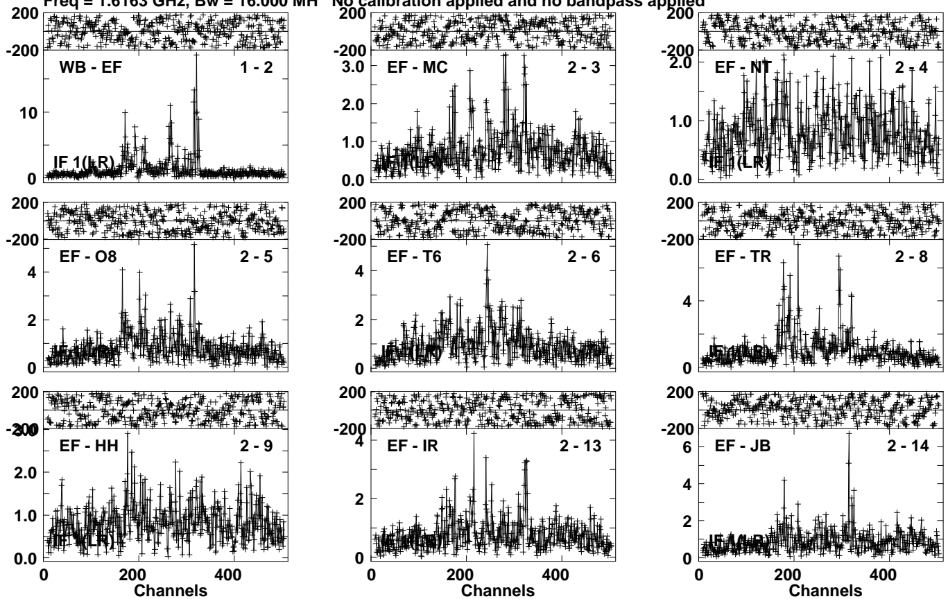
Lower frame: Milli Ampl Jy Top frame: Phas deg Vector averaged cross-power spectrum Several baselines displayed Timerange: 00/05:00:51 to 00/05:04:19
