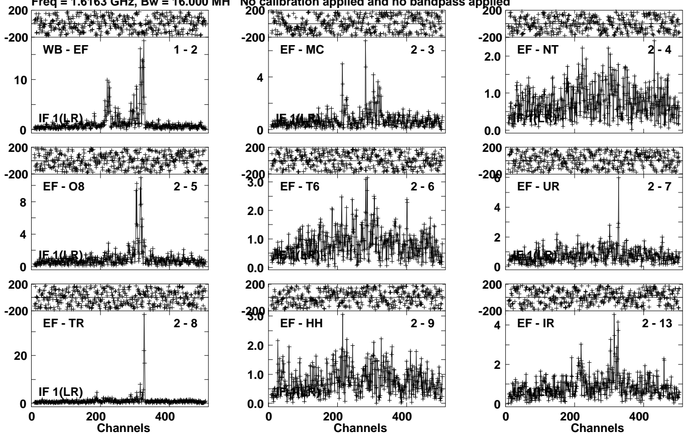
Lower frame: Milli Ampl Jy Top frame: Phas deg Vector averaged cross-power spectrum Several baselines displayed Timerange: 00/03:10:01 to 00/03:13:29
