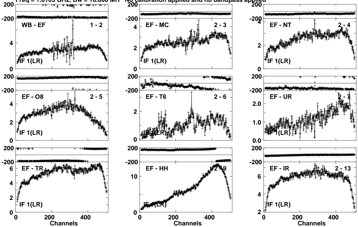
Lower frame: Milli Ampl Jy Top frame: Phas deg Vector averaged cross-power spectrum Several baselines displayed Timerange: 00/01:12:36 to 00/01:15:34
