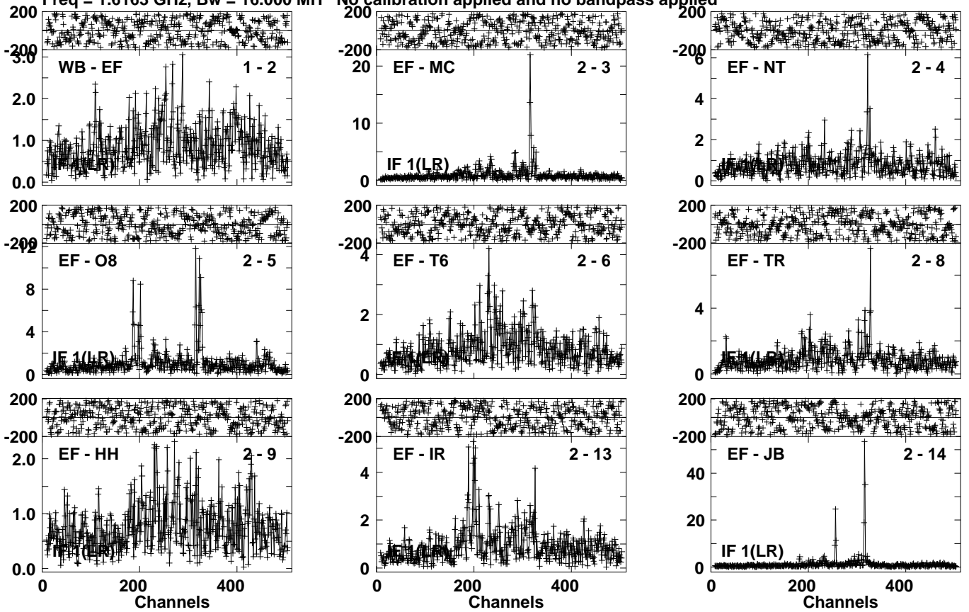
Lower frame: Milli Ampl Jy Top frame: Phas deg Vector averaged cross-power spectrum Several baselines displayed Timerange: 00/05:30:51 to 00/05:34:19
