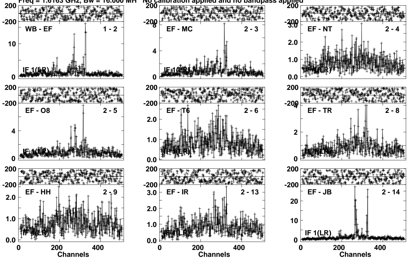
Lower frame: Milli Ampl Jy Top frame: Phas deg Vector averaged cross-power spectrum Several baselines displayed Timerange: 00/05:05:51 to 00/05:09:19
