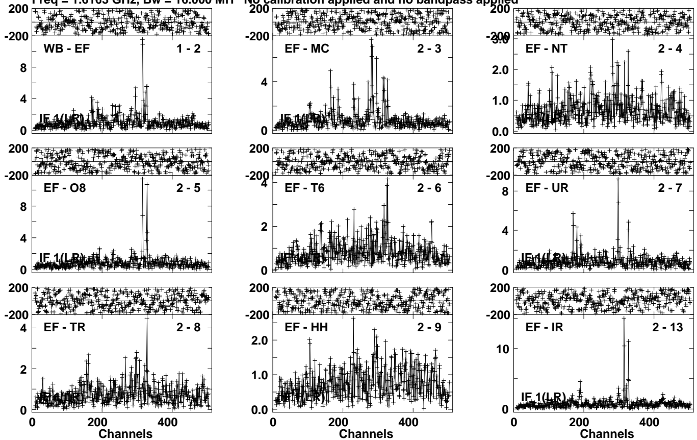
Lower frame: Milli Ampl Jy Top frame: Phas deg Vector averaged cross-power spectrum Several baselines displayed Timerange: 00/02:25:01 to 00/02:28:29
