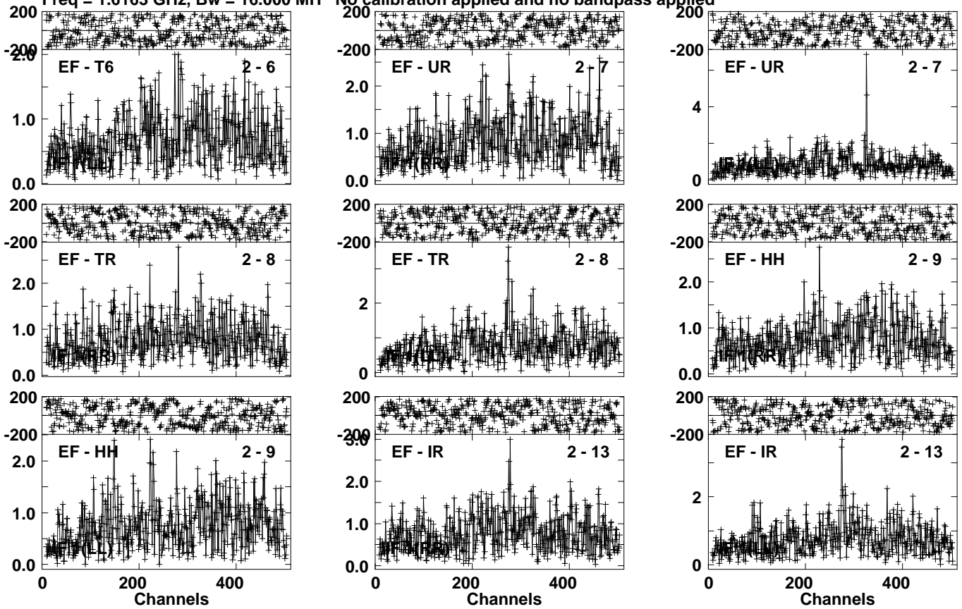
Lower frame: Milli Ampl Jy Top frame: Phas deg Vector averaged cross-power spectrum Several baselines displayed Timerange: 00/03:25:01 to 00/03:28:29
