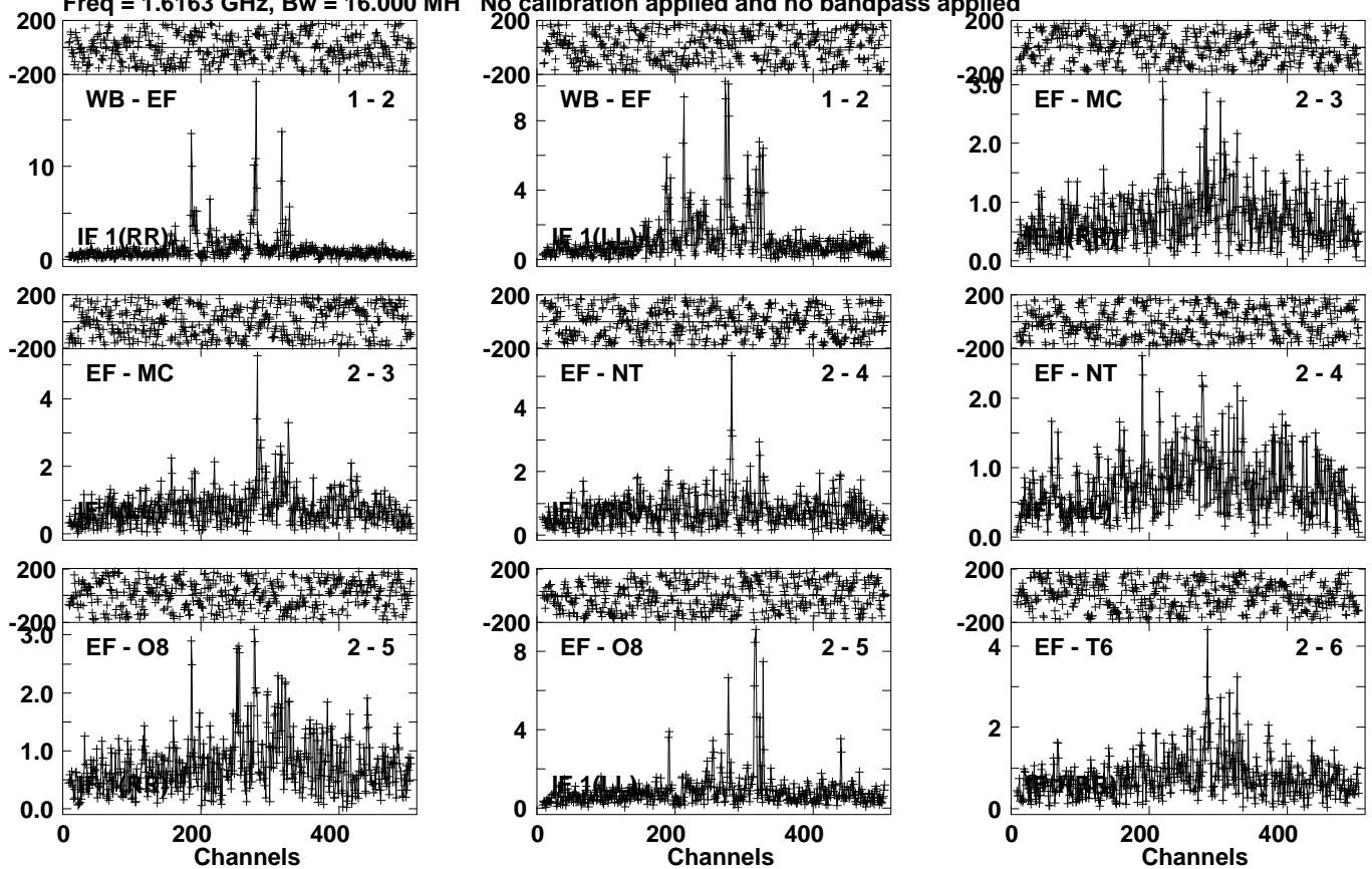
Lower frame: Milli Ampl Jy Top frame: Phas deg Vector averaged cross-power spectrum Several baselines displayed Timerange: 00/03:30:01 to 00/03:33:29
