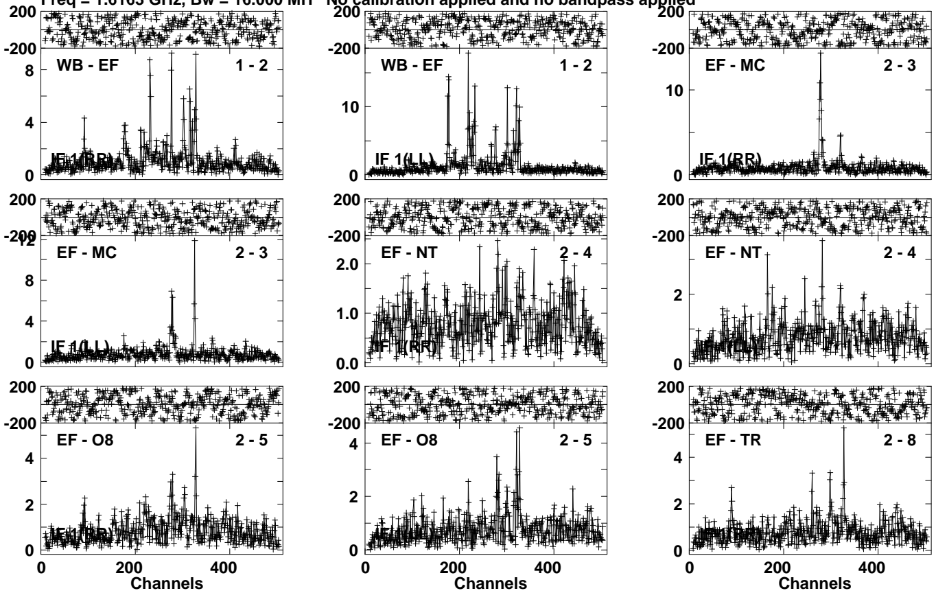
Lower frame: Milli Ampl Jy Top frame: Phas deg Vector averaged cross-power spectrum Several baselines displayed Timerange: 00/06:15:51 to 00/06:19:19
