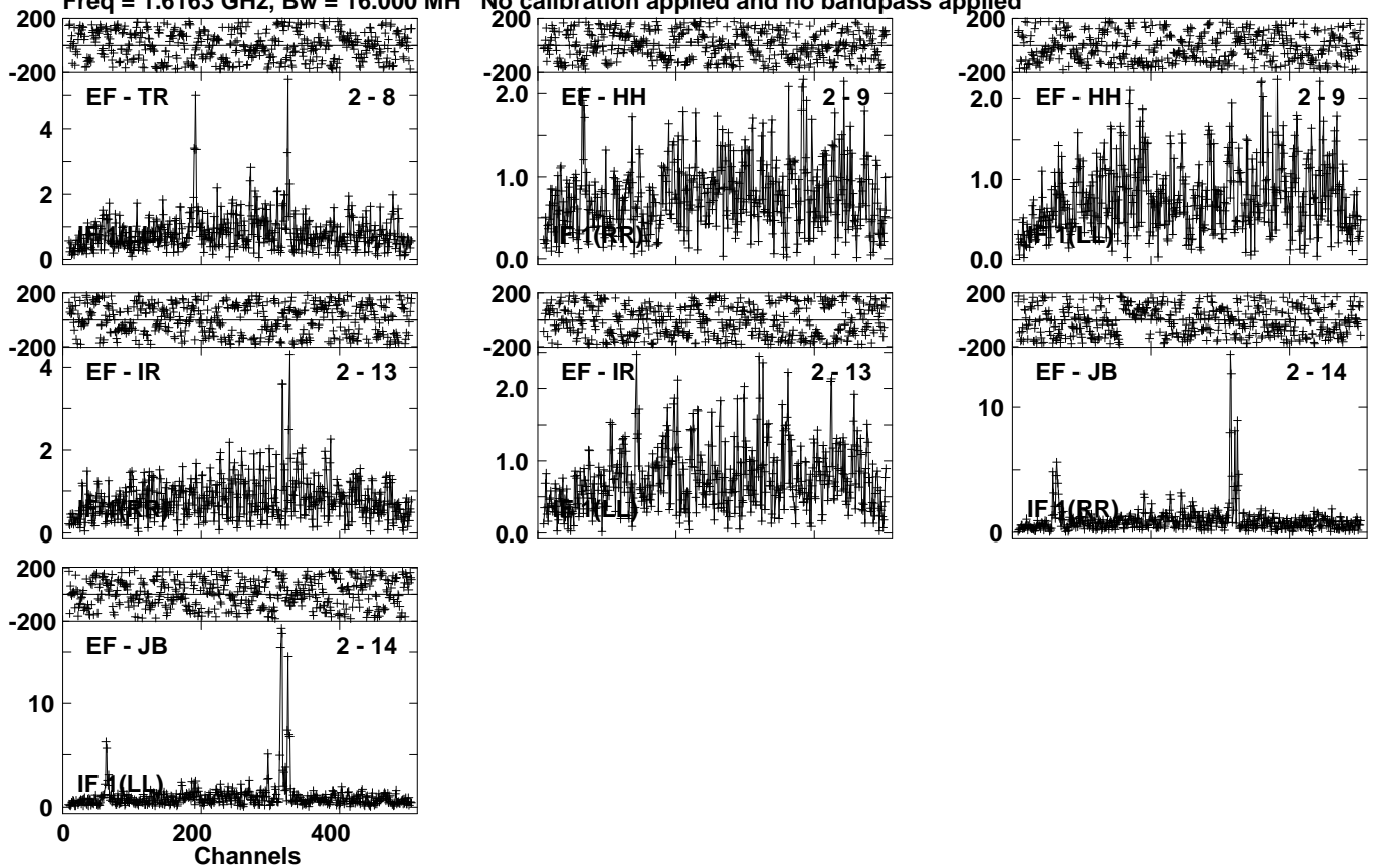
Lower frame: Milli Ampl Jy Top frame: Phas deg Vector averaged cross-power spectrum Several baselines displayed Timerange: 00/08:20:51 to 00/08:24:19
