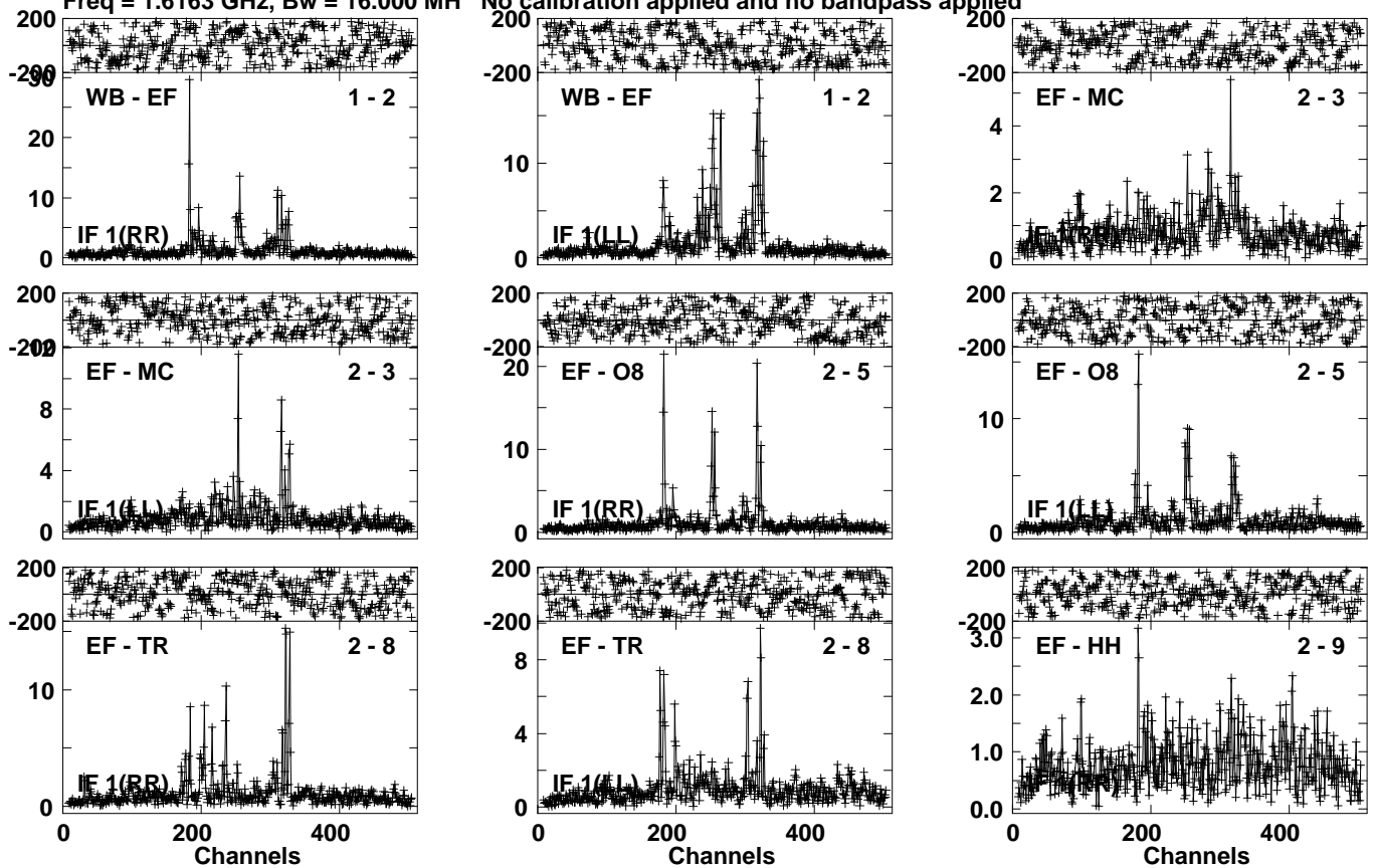
Lower frame: Milli Ampl Jy Top frame: Phas deg Vector averaged cross-power spectrum Several baselines displayed Timerange: 00/05:50:51 to 00/05:54:19
