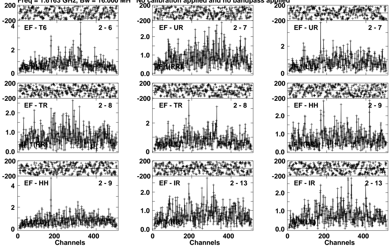
Lower frame: Milli Ampl Jy Top frame: Phas deg Vector averaged cross-power spectrum Several baselines displayed Timerange: 00/04:20:51 to 00/04:24:19
