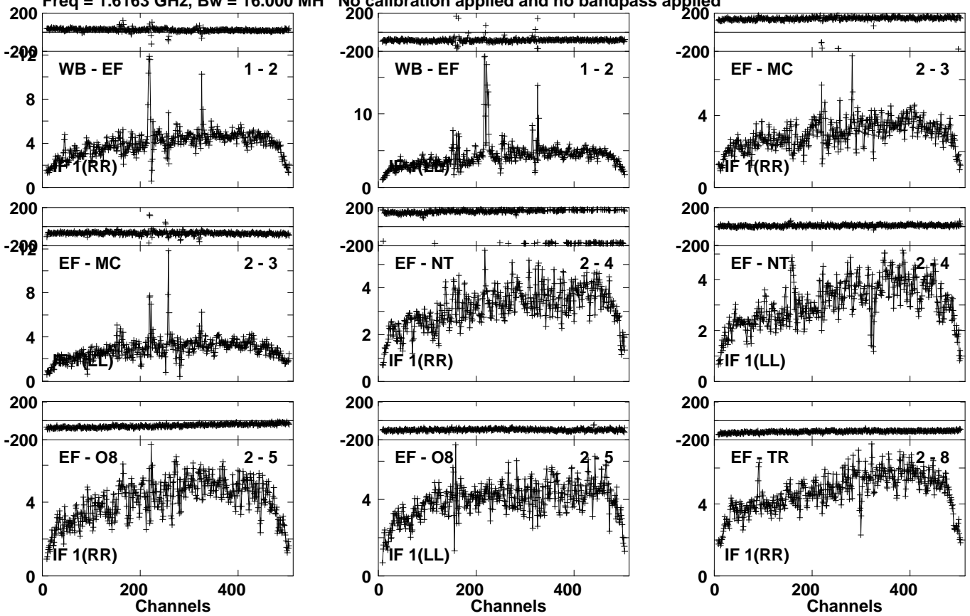
Lower frame: Milli Ampl Jy Top frame: Phas deg Vector averaged cross-power spectrum Several baselines displayed Timerange: 00/06:44:51 to 00/06:45:49
