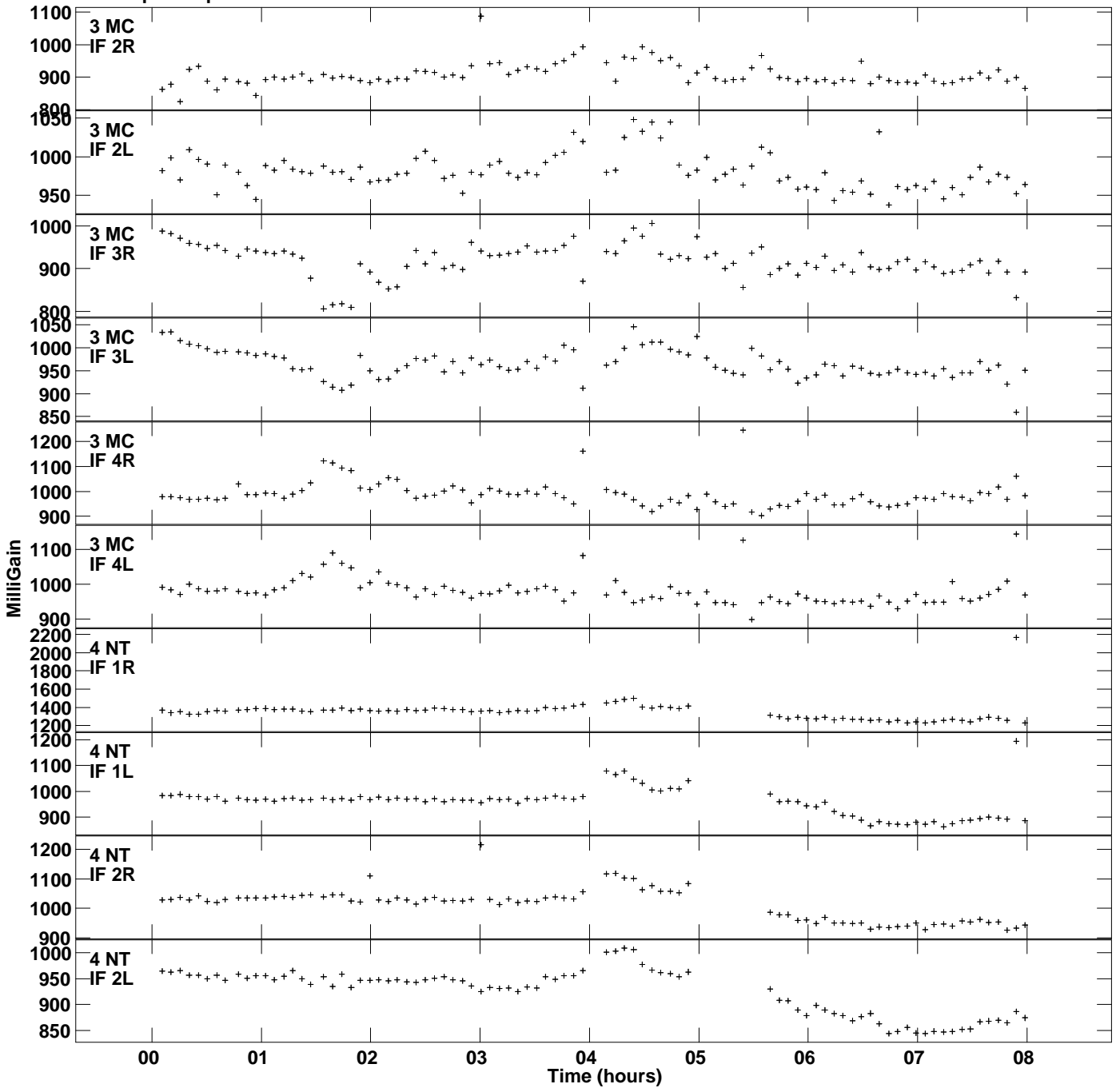
Plot file version 2 created 24-NOV-2022 15:13:12 Gain amp vs UTC time for J1748+3404.MULTI.1 SN 2 Rpol & Lpol IF 1 - 4
