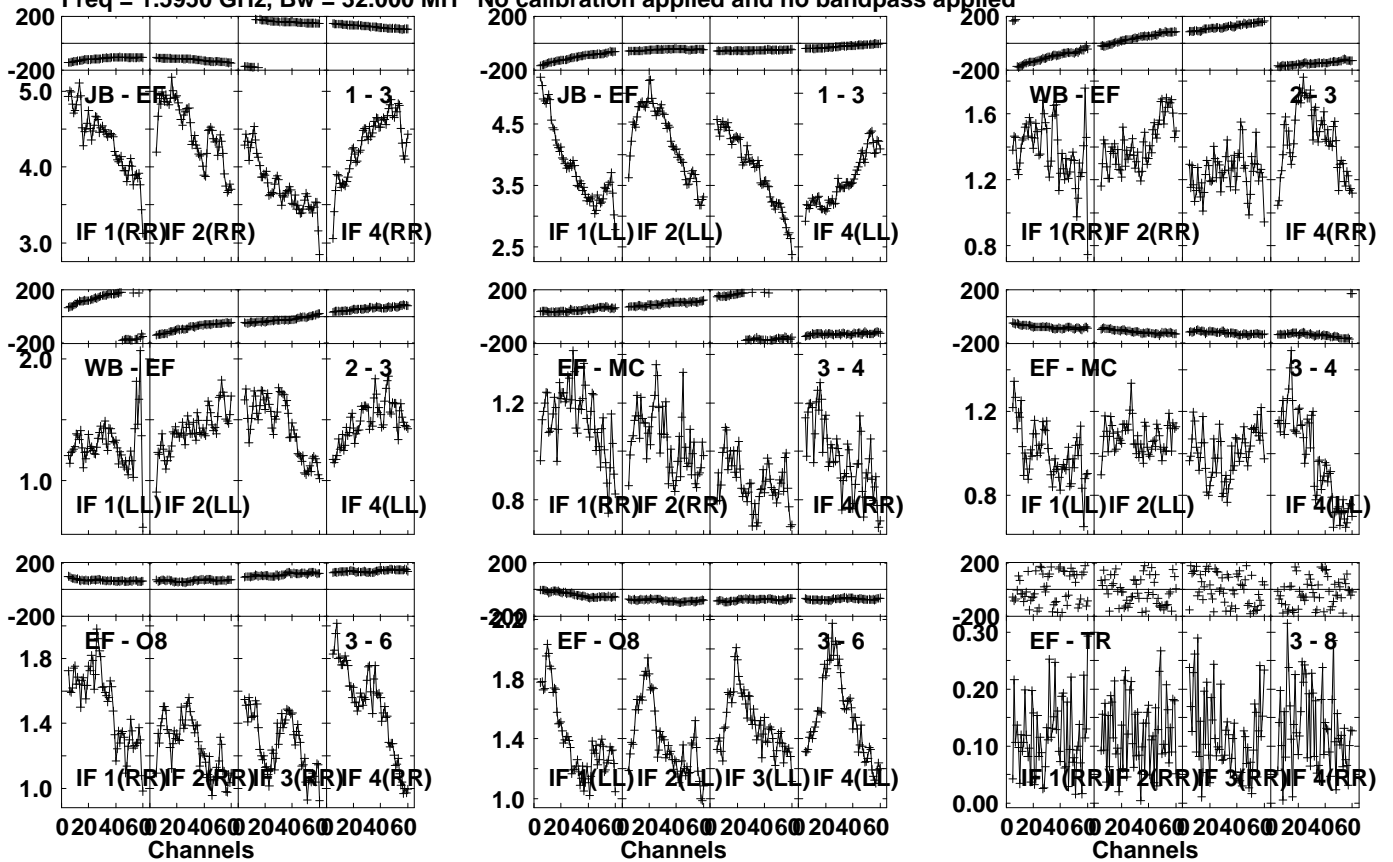
Lower frame: Milli Ampl Jy Top frame: Phas deg Vector averaged cross-power spectrum Several baselines displayed Timerange: 00:15:31:31 to 00:15:32:59
