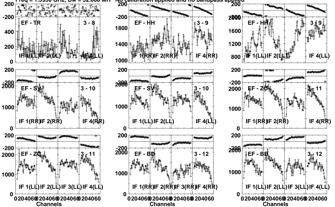
Lower frame: Micro Ampl Jy Top frame: Phas deg Vector averaged cross-power spectrum Several baselines displayed Timerange: 00/07:45:01 to 00/07:46:29
