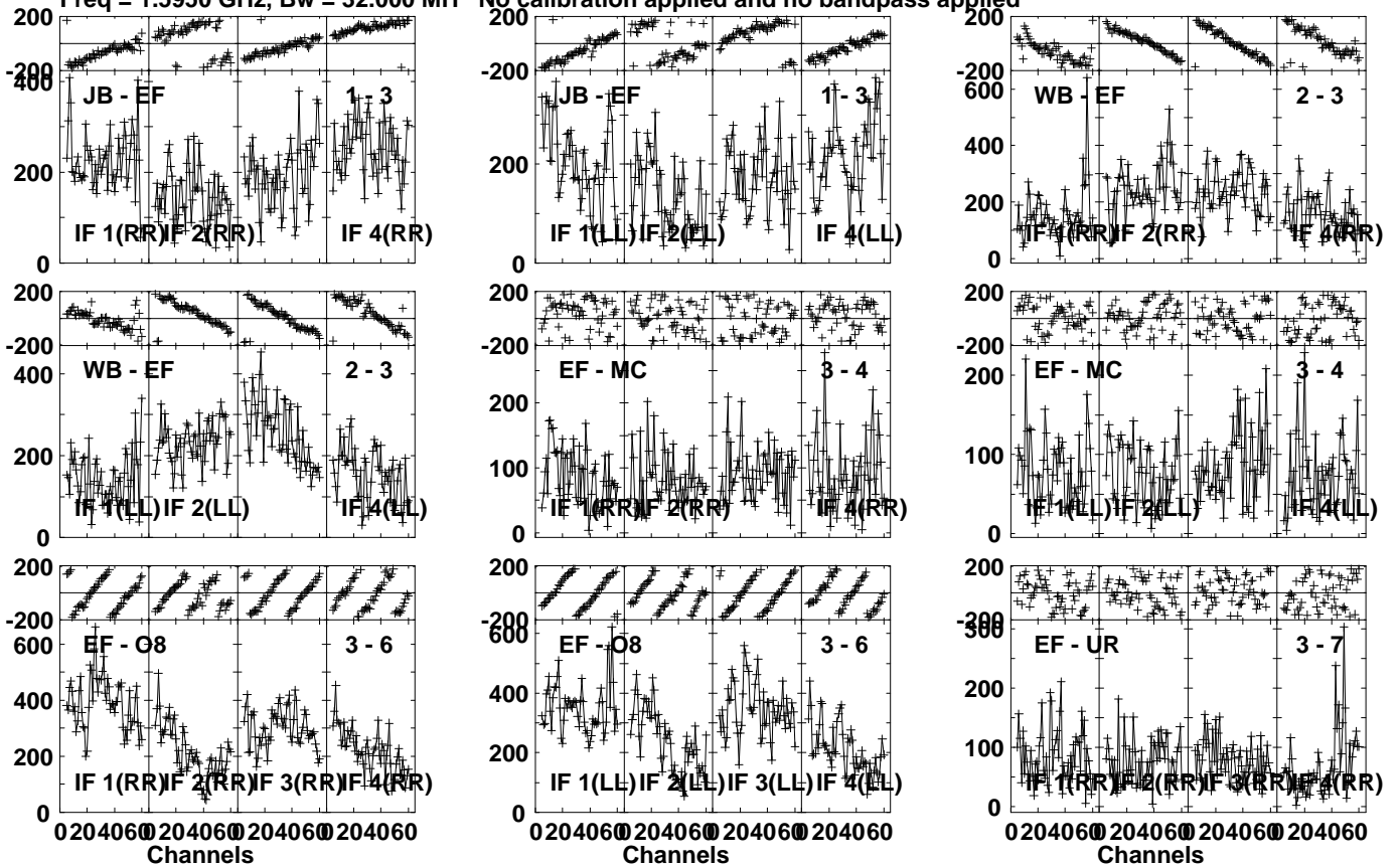
Lower frame: Micro Ampl Jy Top frame: Phas deg Vector averaged cross-power spectrum Several baselines displayed Timerange: 00/07:36:01 to 00/07:39:29
