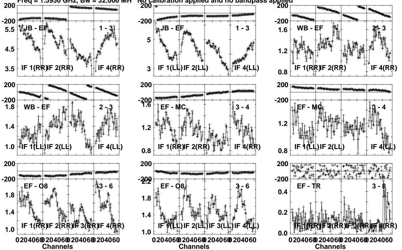
Lower frame: Milli Ampl Jy Top frame: Phas deg Vector averaged cross-power spectrum Several baselines displayed Timerange: 00/06:47:31 to 00/06:48:59
