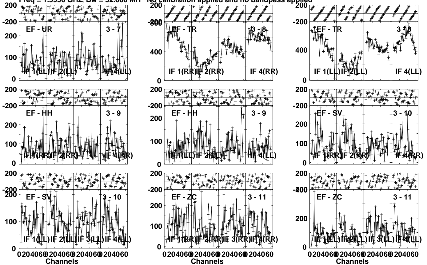
Lower frame: Micro Ampl Jy Top frame: Phas deg Vector averaged cross-power spectrum Several baselines displayed Timerange: 00/09:41:31 to 00/09:44:59
