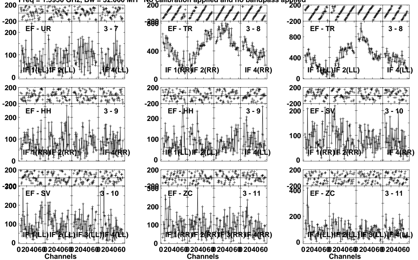
Lower frame: Micro Ampl Jy Top frame: Phas deg Vector averaged cross-power spectrum Several baselines displayed Timerange: 00/09:47:01 to 00/09:50:29
