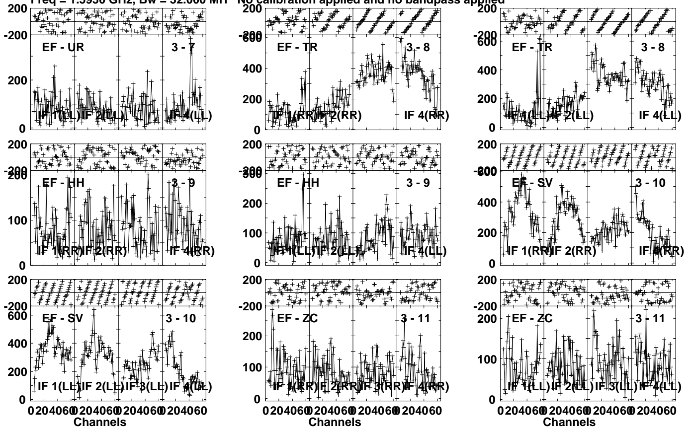
Lower frame: Micro Ampl Jy Top frame: Phas deg Vector averaged cross-power spectrum Several baselines displayed Timerange: 00/08:23:31 to 00/08:26:59
