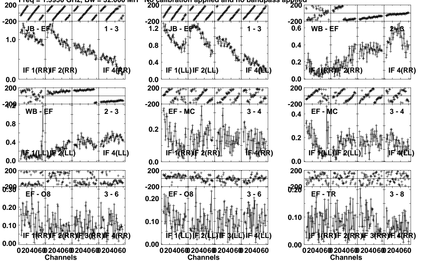
Lower frame: Milli Ampl Jy Top frame: Phas deg Vector averaged cross-power spectrum Several baselines displayed Timerange: 00/12:24:31 to 00/12:27:59
