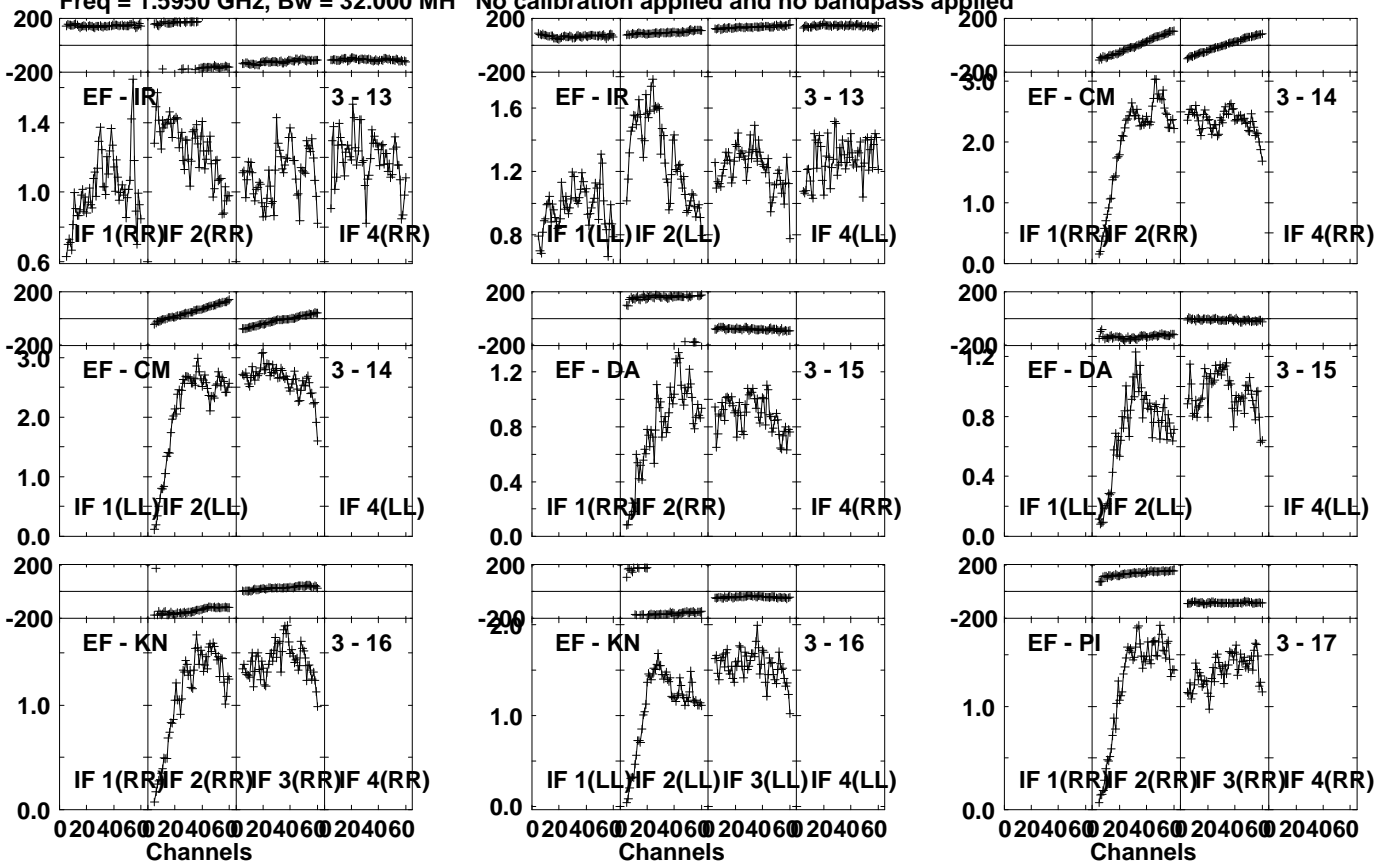
Lower frame: Milli Ampl Jy Top frame: Phas deg Vector averaged cross-power spectrum Several baselines displayed Timerange: 00/10:01:01 to 00/10:02:29
