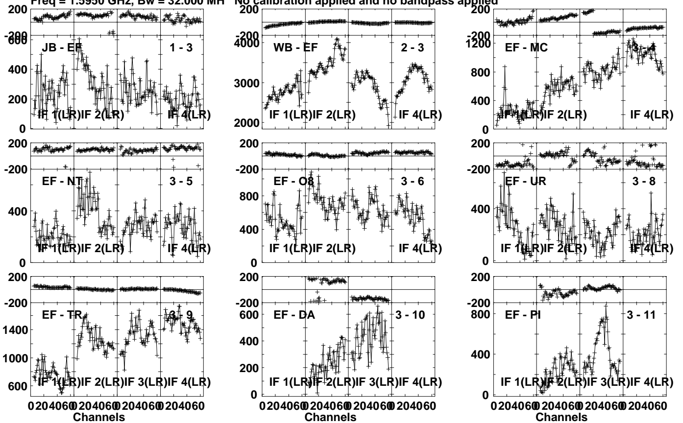
Lower frame: Micro Ampl Jy Top frame: Phas deg Vector averaged cross-power spectrum Several baselines displayed Timerange: 00/12:44:56 to 00/12:46:12
