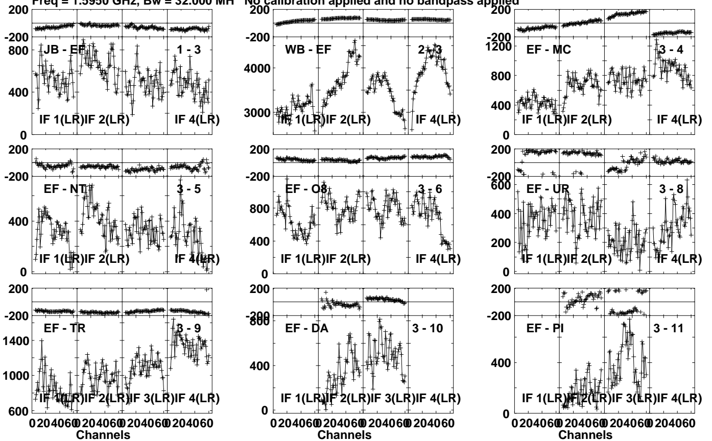
Lower frame: Micro Ampl Jy Top frame: Phas deg Vector averaged cross-power spectrum Several baselines displayed Timerange: 00/14:12:21 to 00/14:13:27
