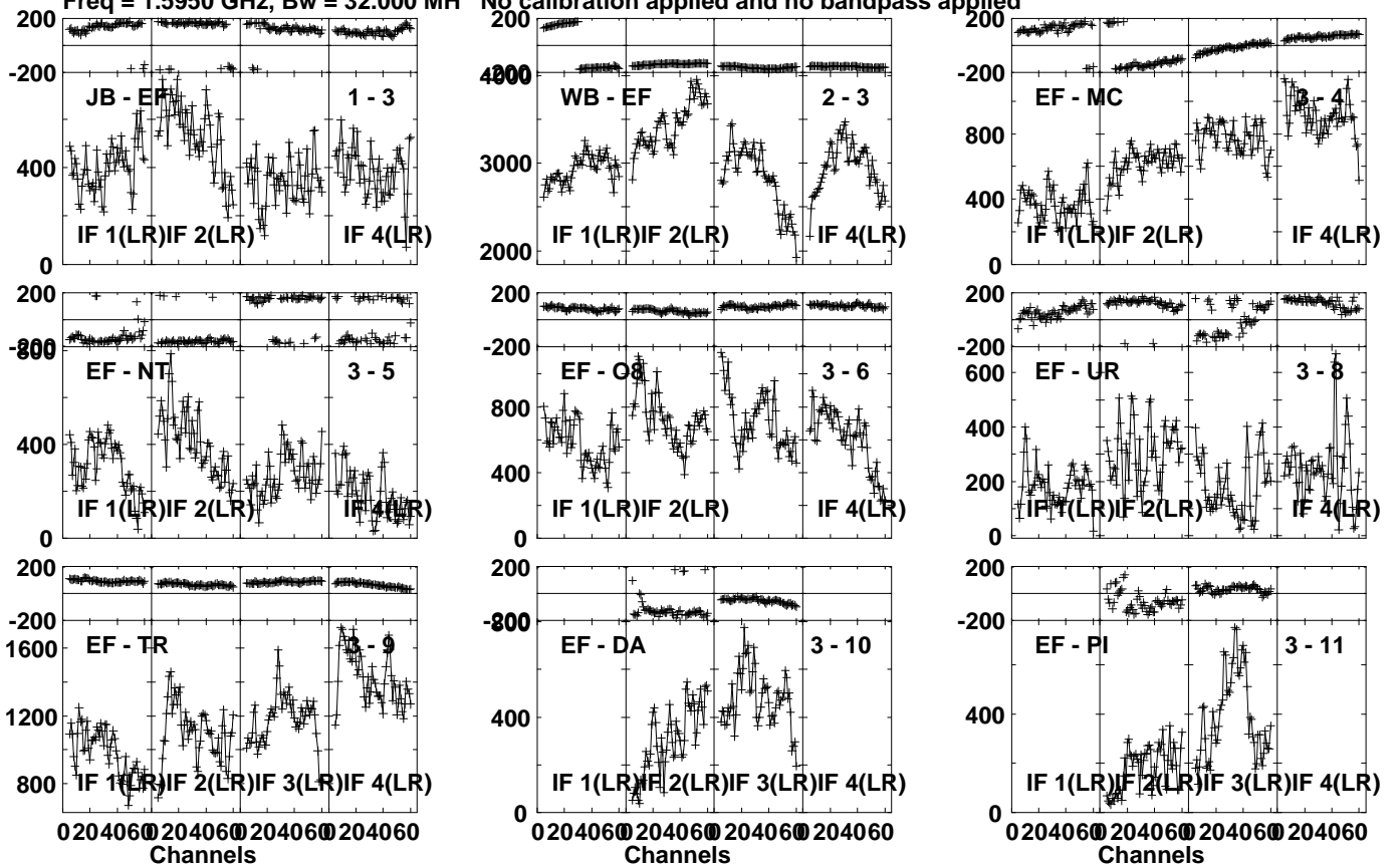
Lower frame: Micro Ampl Jy Top frame: Phas deg Vector averaged cross-power spectrum Several baselines displayed Timerange: 00/13:44:07 to 00/13:45:13
