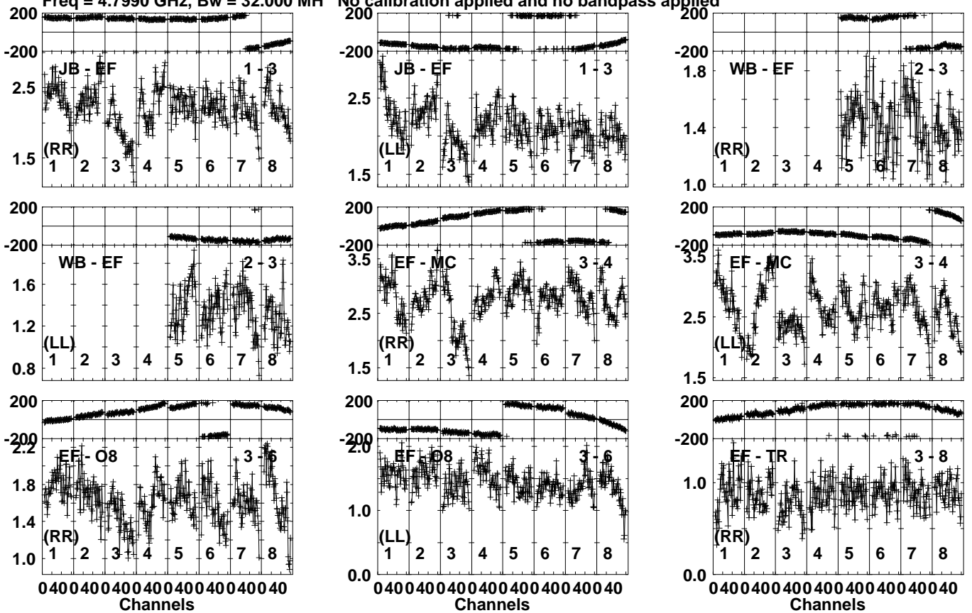
Lower frame: Milli Ampl Jy Top frame: Phas deg Vector averaged cross-power spectrum Several baselines displayed Timerange: 00/23:53:21 to 00/23:54:49
