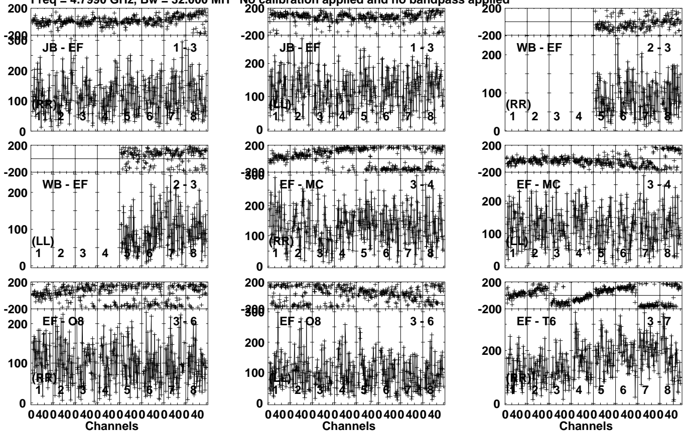
Lower frame: Micro Ampl Jy Top frame: Phas deg Vector averaged cross-power spectrum Several baselines displayed Timerange: 01/03:40:51 to 01/03:44:19
