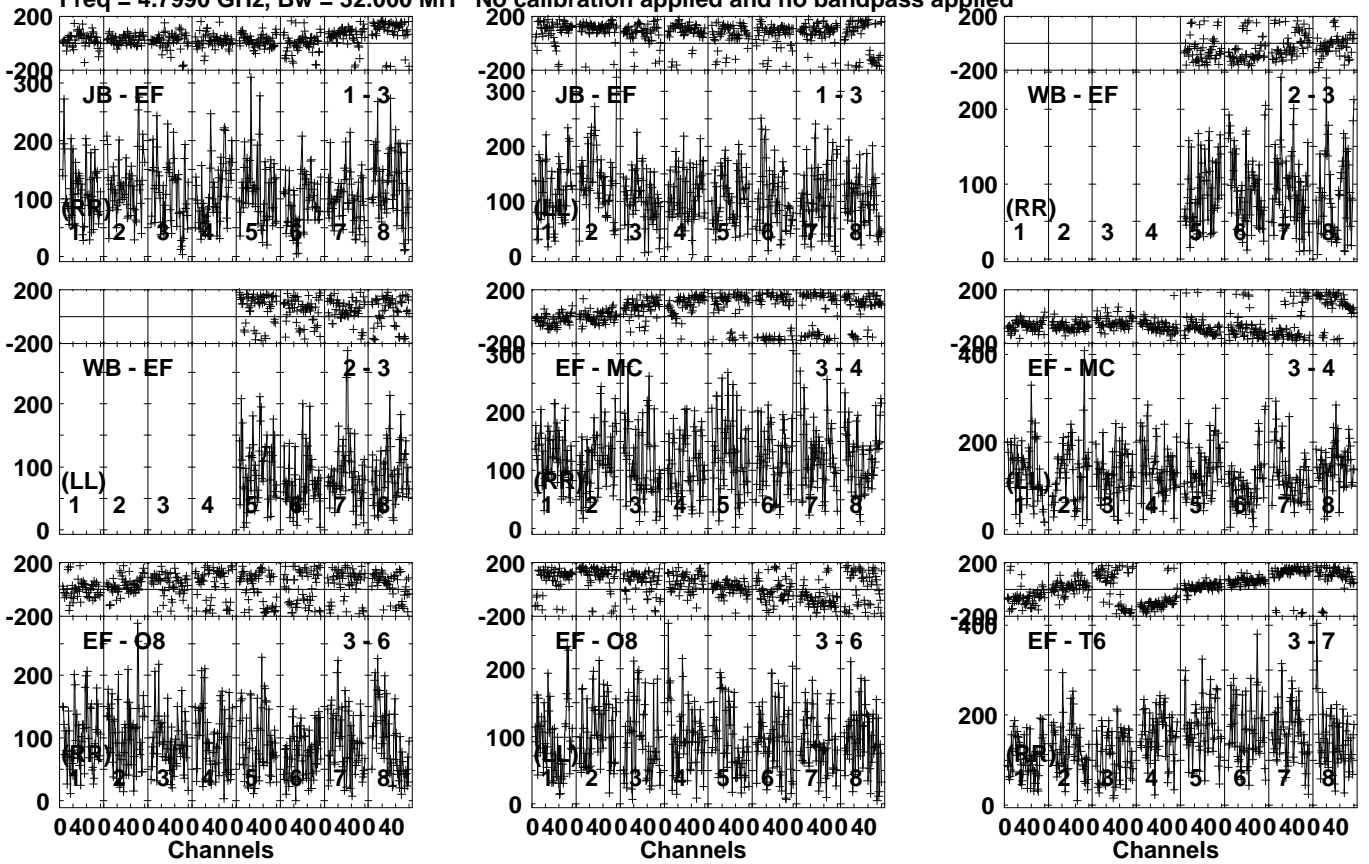
Lower frame: Micro Ampl Jy Top frame: Phas deg Vector averaged cross-power spectrum Several baselines displayed Timerange: 01/04:00:51 to 01/04:04:19
