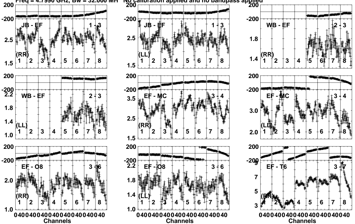
Lower frame: Milli Ampl Jy Top frame: Phas deg Vector averaged cross-power spectrum Several baselines displayed Timerange: 01/05:56:21 to 01/05:57:19
