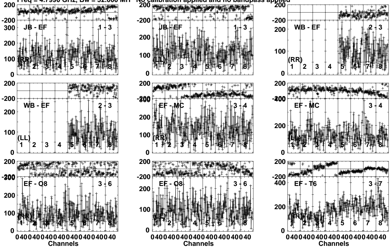
Lower frame: Micro Ampl Jy Top frame: Phas deg Vector averaged cross-power spectrum Several baselines displayed Timerange: 01/03:05:21 to 01/03:08:49
