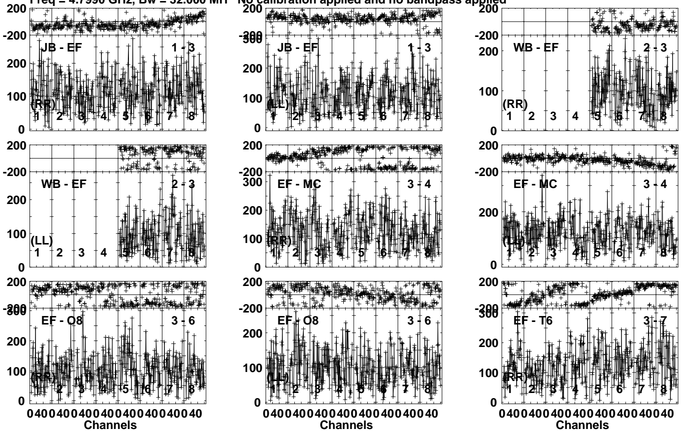
Lower frame: Micro Ampl Jy Top frame: Phas deg Vector averaged cross-power spectrum Several baselines displayed Timerange: 01/06:27:21 to 01/06:30:49
