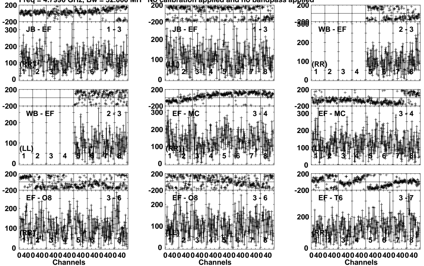
Lower frame: Micro Ampl Jy Top frame: Phas deg Vector averaged cross-power spectrum Several baselines displayed Timerange: 01/06:47:51 to 01/06:51:19
