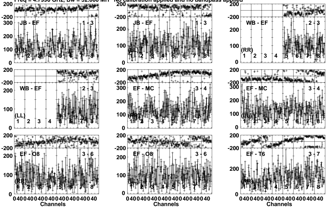
Lower frame: Micro Ampl Jy Top frame: Phas deg Vector averaged cross-power spectrum Several baselines displayed Timerange: 01/04:36:21 to 01/04:39:49
