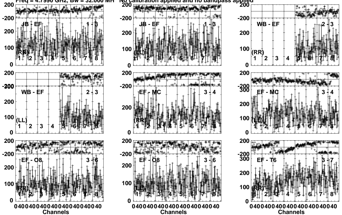
Lower frame: Micro Ampl Jy Top frame: Phas deg Vector averaged cross-power spectrum Several baselines displayed Timerange: 01/03:50:51 to 01/03:54:19
