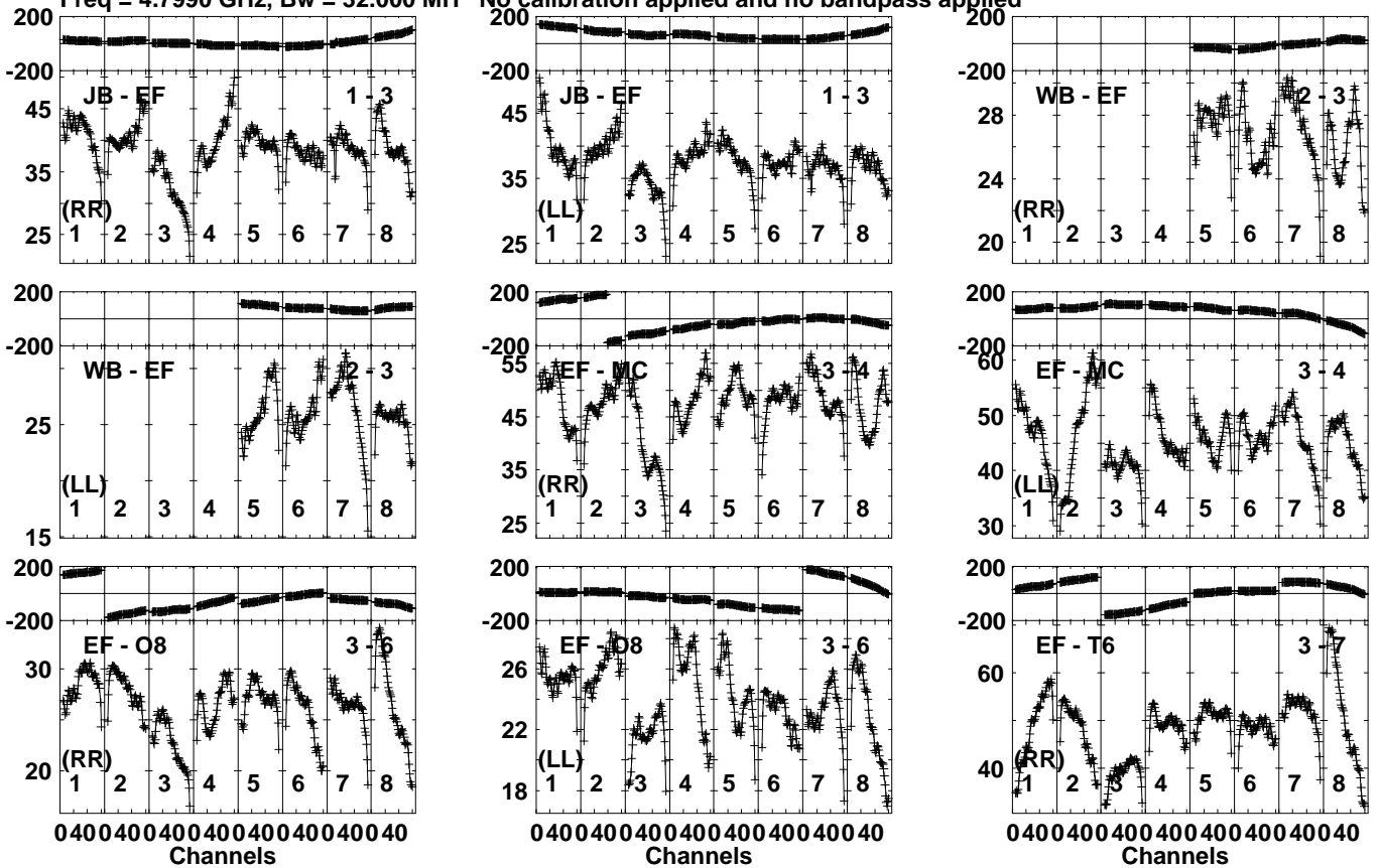
Lower frame: Milli Ampl Jy Top frame: Phas deg Vector averaged cross-power spectrum Several baselines displayed Timerange: 00/19:35:21 to 00/19:38:19
