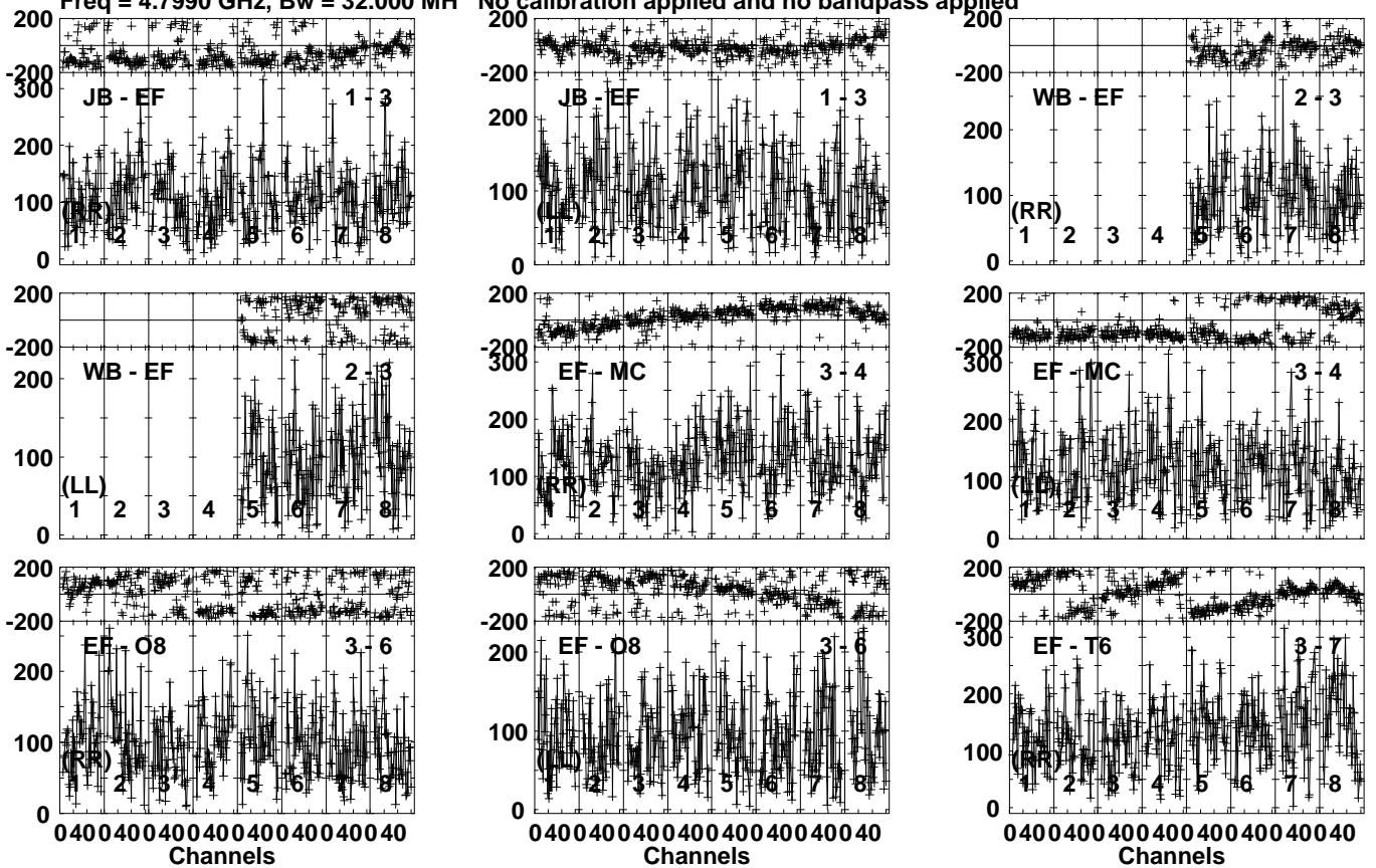
Lower frame: Micro Ampl Jy Top frame: Phas deg Vector averaged cross-power spectrum Several baselines displayed Timerange: 01/05:57:21 to 01/06:00:49
