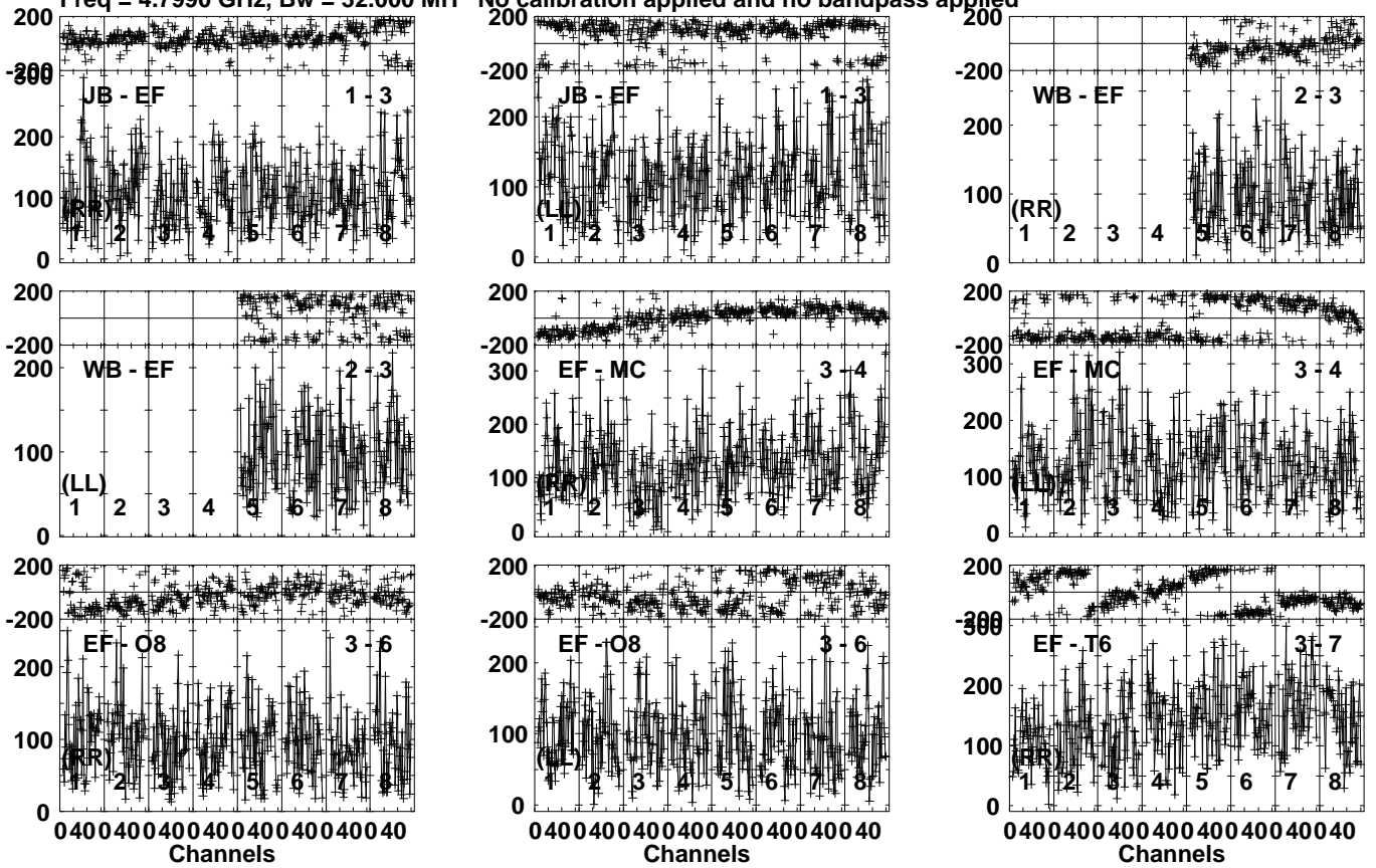
Lower frame: Micro Ampl Jy Top frame: Phas deg Vector averaged cross-power spectrum Several baselines displayed Timerange: 01/05:01:21 to 01/05:04:49
