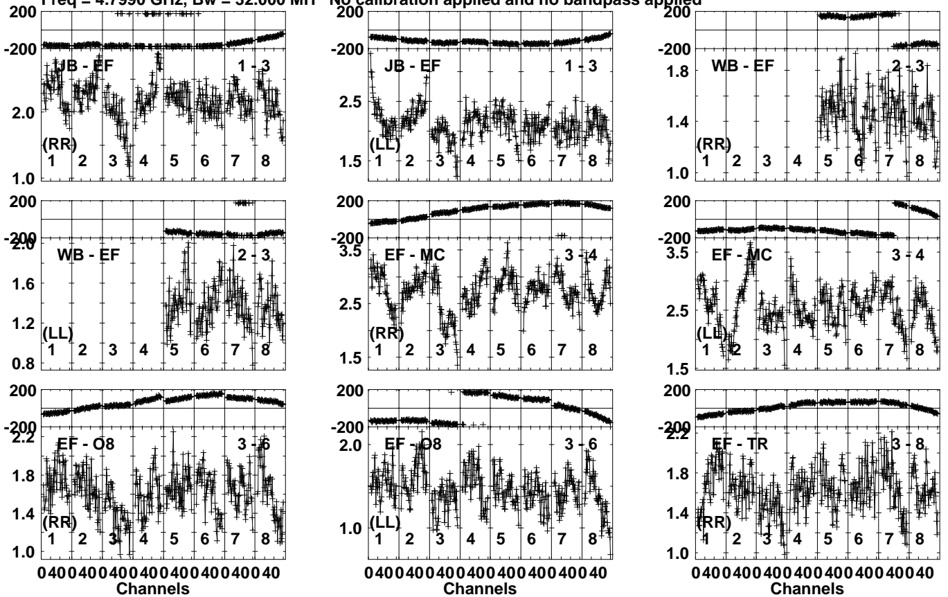
Lower frame: Milli Ampl Jy Top frame: Phas deg Vector averaged cross-power spectrum Several baselines displayed Timerange: 01/00:08:51 to 01/00:09:49
