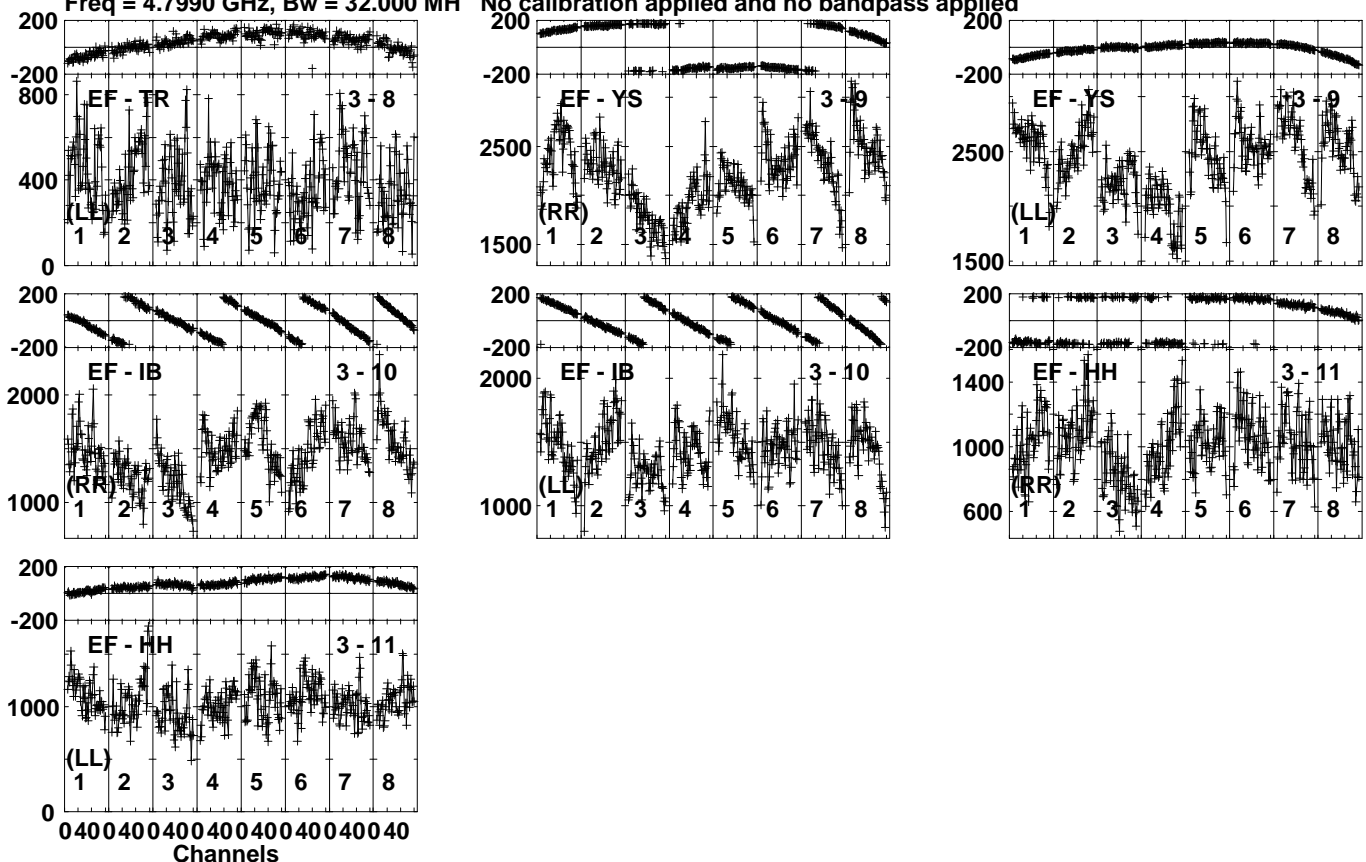
Lower frame: Micro Ampl Jy Top frame: Phas deg Vector averaged cross-power spectrum Several baselines displayed Timerange: 01/01:44:21 to 01/01:45:49
