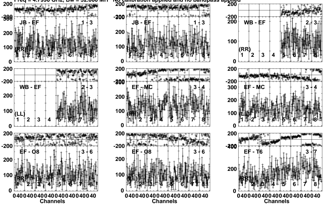
Lower frame: Micro Ampl Jy Top frame: Phas deg Vector averaged cross-power spectrum Several baselines displayed Timerange: 01/03:30:51 to 01/03:34:19
