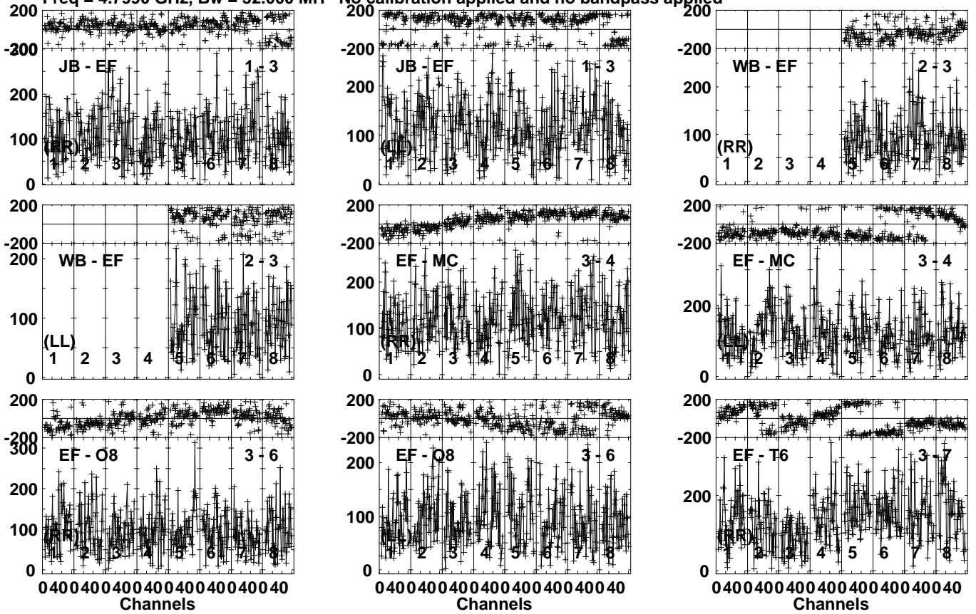
Lower frame: Micro Ampl Jy Top frame: Phas deg Vector averaged cross-power spectrum Several baselines displayed Timerange: 01/04:41:21 to 01/04:44:49
