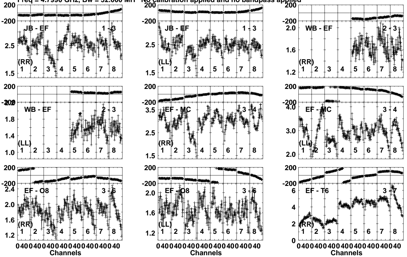
Lower frame: Milli Ampl Jy Top frame: Phas deg Vector averaged cross-power spectrum Several baselines displayed Timerange: 01/03:59:21 to 01/04:00:49
