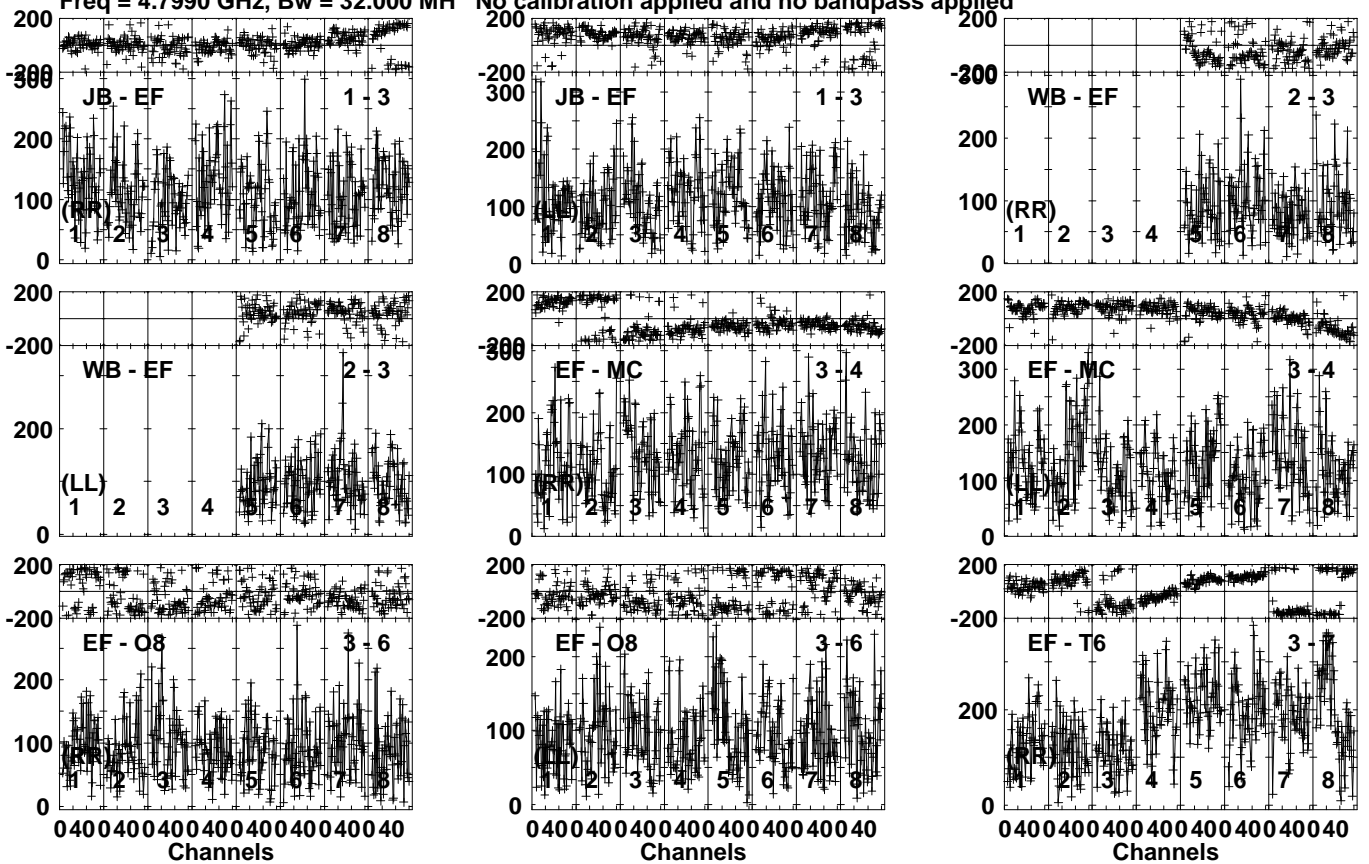
Lower frame: Micro Ampl Jy Top frame: Phas deg Vector averaged cross-power spectrum Several baselines displayed Timerange: 01/02:40:21 to 01/02:43:49
