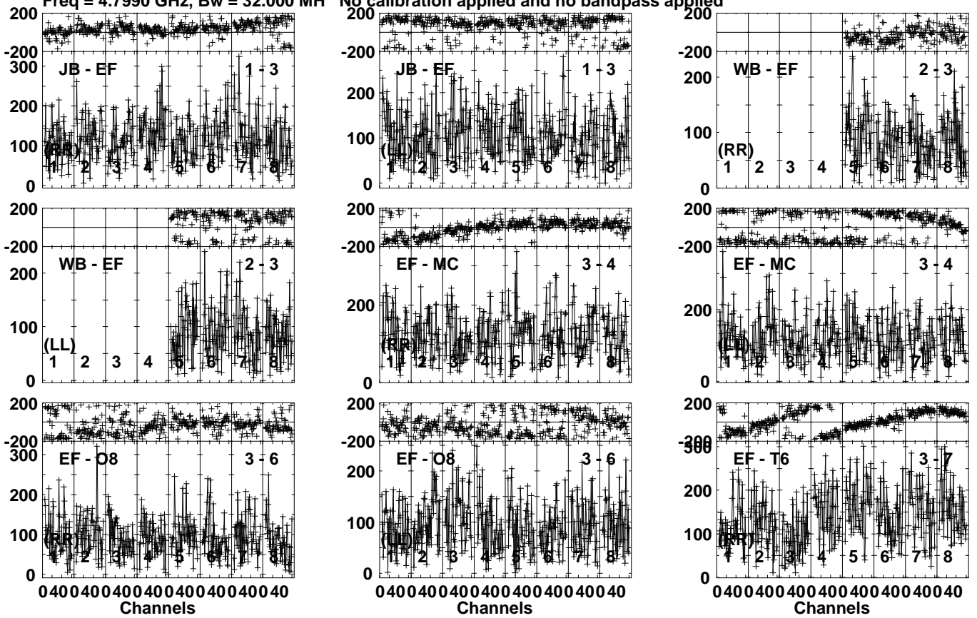
Lower frame: Micro Ampl Jy Top frame: Phas deg Vector averaged cross-power spectrum Several baselines displayed Timerange: 01/05:06:21 to 01/05:09:49
