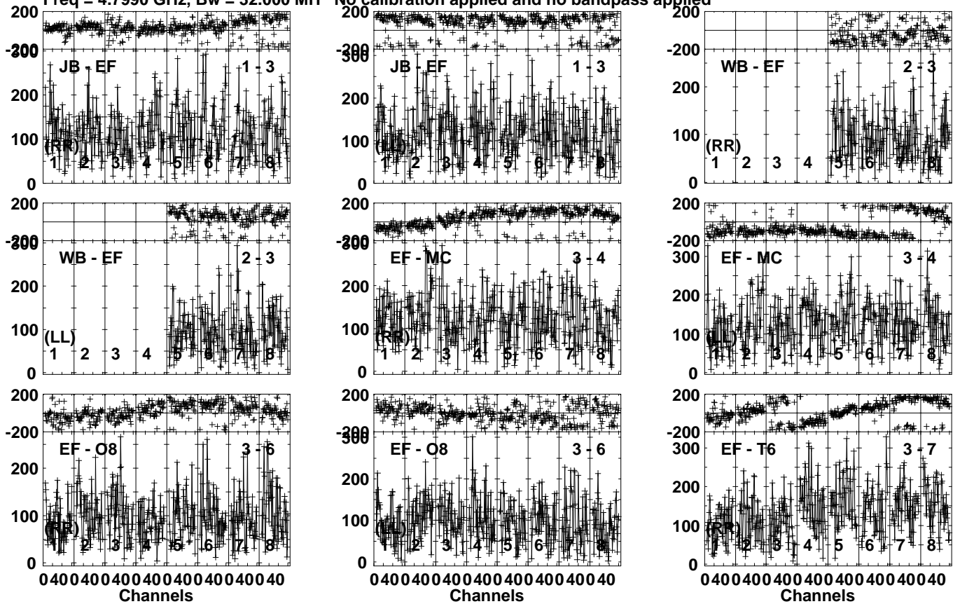
Lower frame: Micro Ampl Jy Top frame: Phas deg Vector averaged cross-power spectrum Several baselines displayed Timerange: 01/04:26:21 to 01/04:29:49
