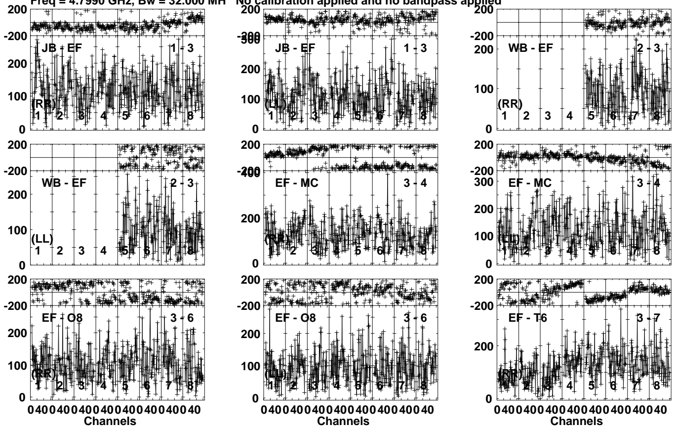
Lower frame: Micro Ampl Jy Top frame: Phas deg Vector averaged cross-power spectrum Several baselines displayed Timerange: 01/05:42:21 to 01/05:45:49
