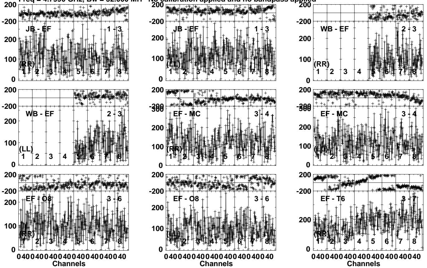
Lower frame: Micro Ampl Jy Top frame: Phas deg Vector averaged cross-power spectrum Several baselines displayed Timerange: 01/02:20:21 to 01/02:23:49
