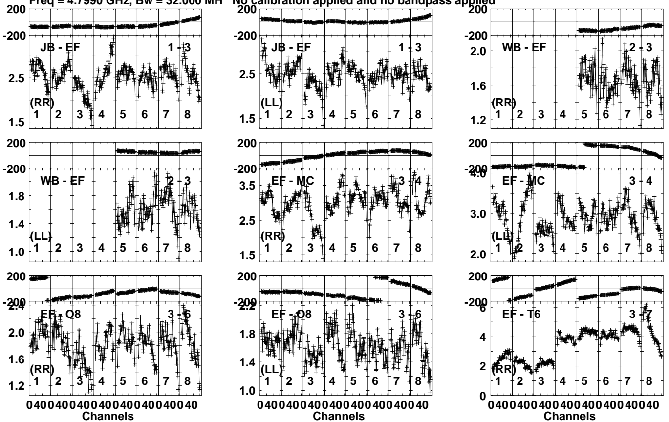
Lower frame: Milli Ampl Jy Top frame: Phas deg Vector averaged cross-power spectrum Several baselines displayed Timerange: 01/03:29:21 to 01/03:30:49
