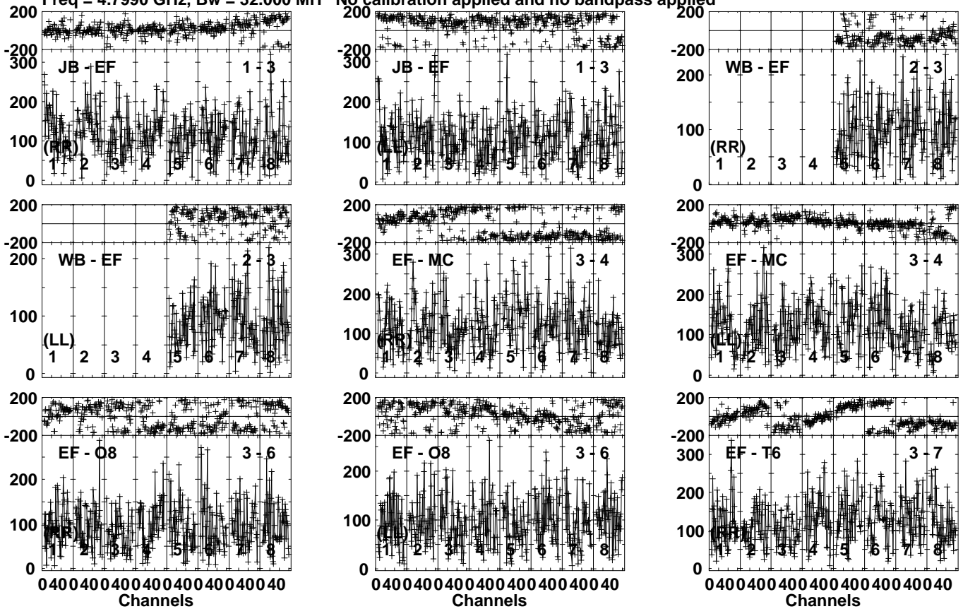
Lower frame: Micro Ampl Jy Top frame: Phas deg Vector averaged cross-power spectrum Several baselines displayed Timerange: 01/06:22:21 to 01/06:25:49
