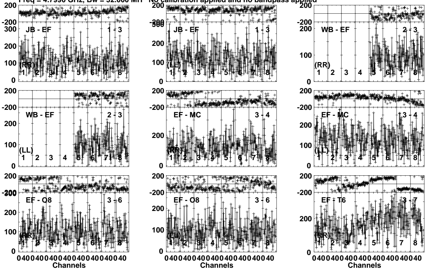
Lower frame: Micro Ampl Jy Top frame: Phas deg Vector averaged cross-power spectrum Several baselines displayed Timerange: 01/02:50:21 to 01/02:53:49
