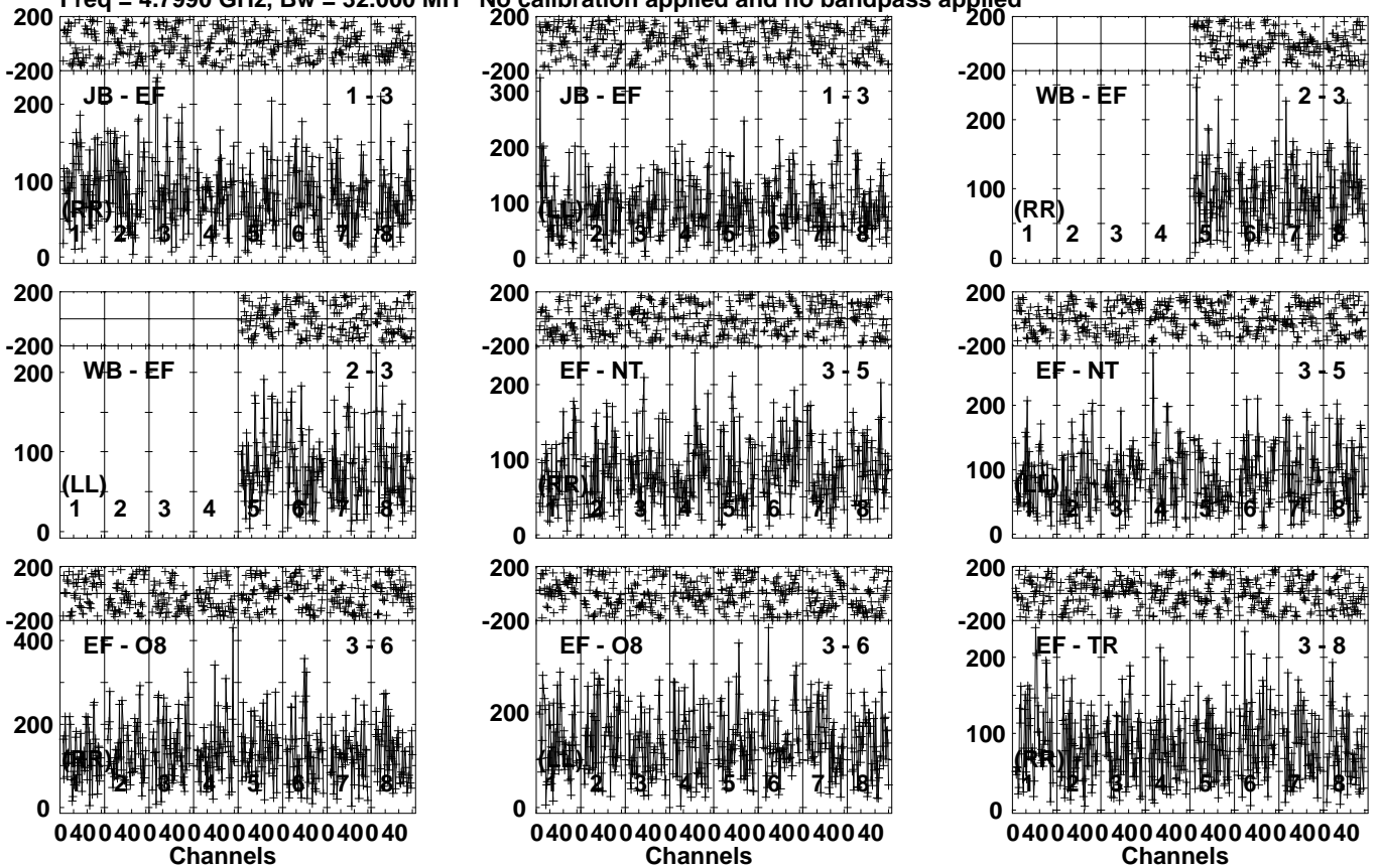
Lower frame: Micro Ampl Jy Top frame: Phas deg Vector averaged cross-power spectrum Several baselines displayed Timerange: 01/02:58:01 to 01/03:01:29
