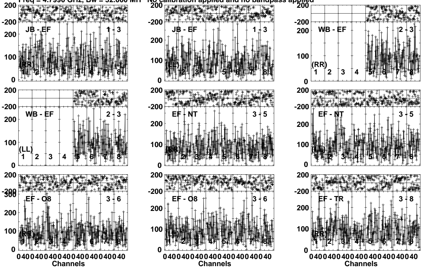
Lower frame: Micro Ampl Jy Top frame: Phas deg Vector averaged cross-power spectrum Several baselines displayed Timerange: 01/08:24:31 to 01/08:27:59
