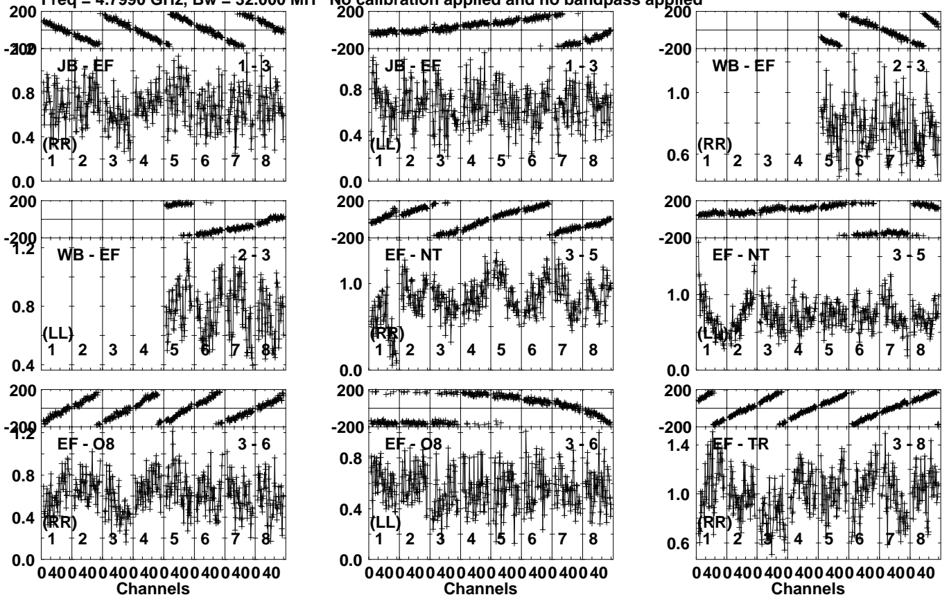
Lower frame: Milli Ampl Jy Top frame: Phas deg Vector averaged cross-power spectrum Several baselines displayed Timerange: 01/08:13:31 to 01/08:14:29
