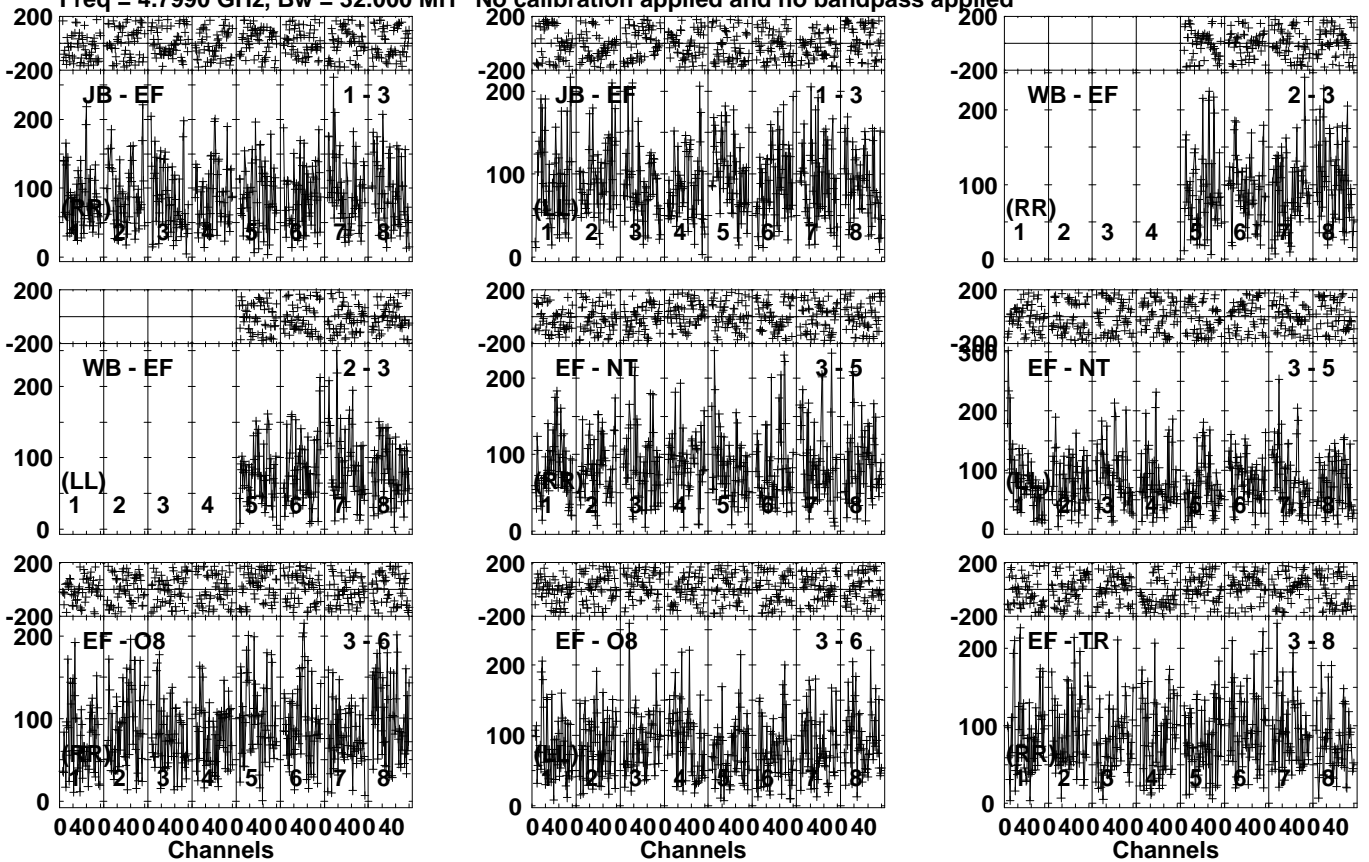
Lower frame: Micro Ampl Jy Top frame: Phas deg Vector averaged cross-power spectrum Several baselines displayed Timerange: 00/22:49:31 to 00/22:52:59
