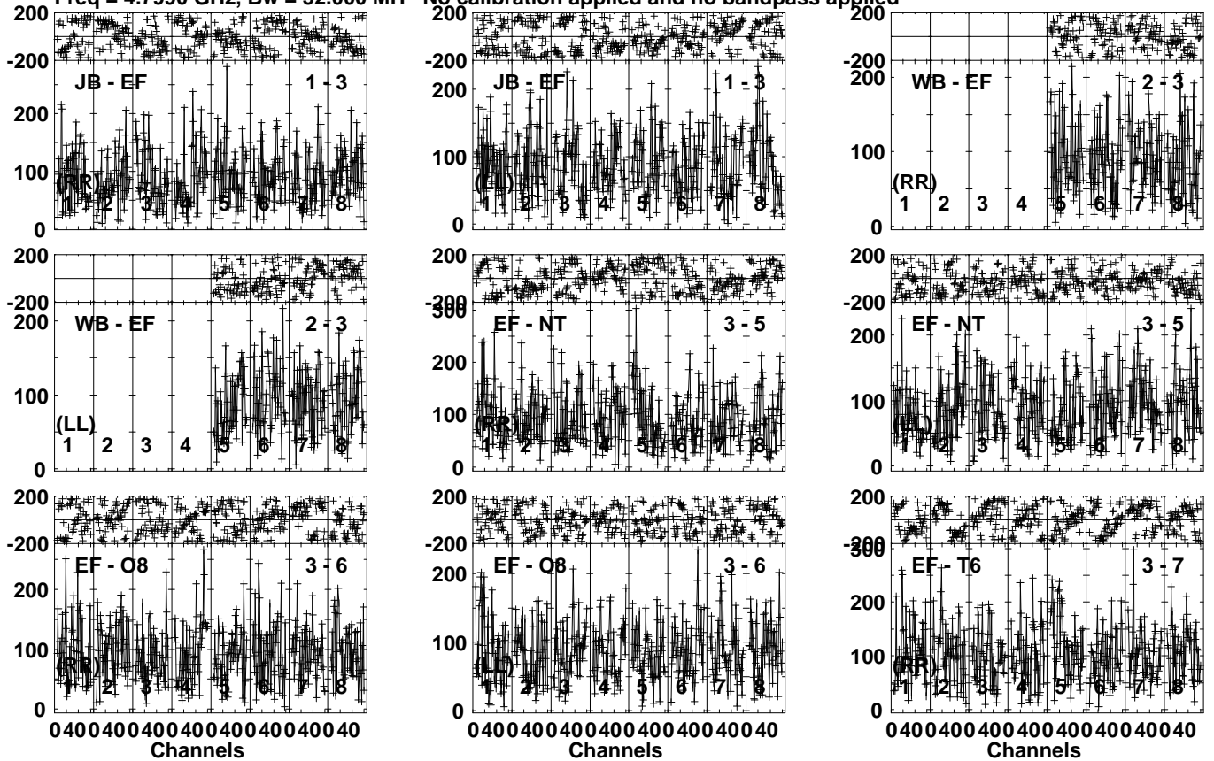
Lower frame: Micro Ampl Jy Top frame: Phas deg Vector averaged cross-power spectrum Several baselines displayed Timerange: 01/05:14:31 to 01/05:17:59
