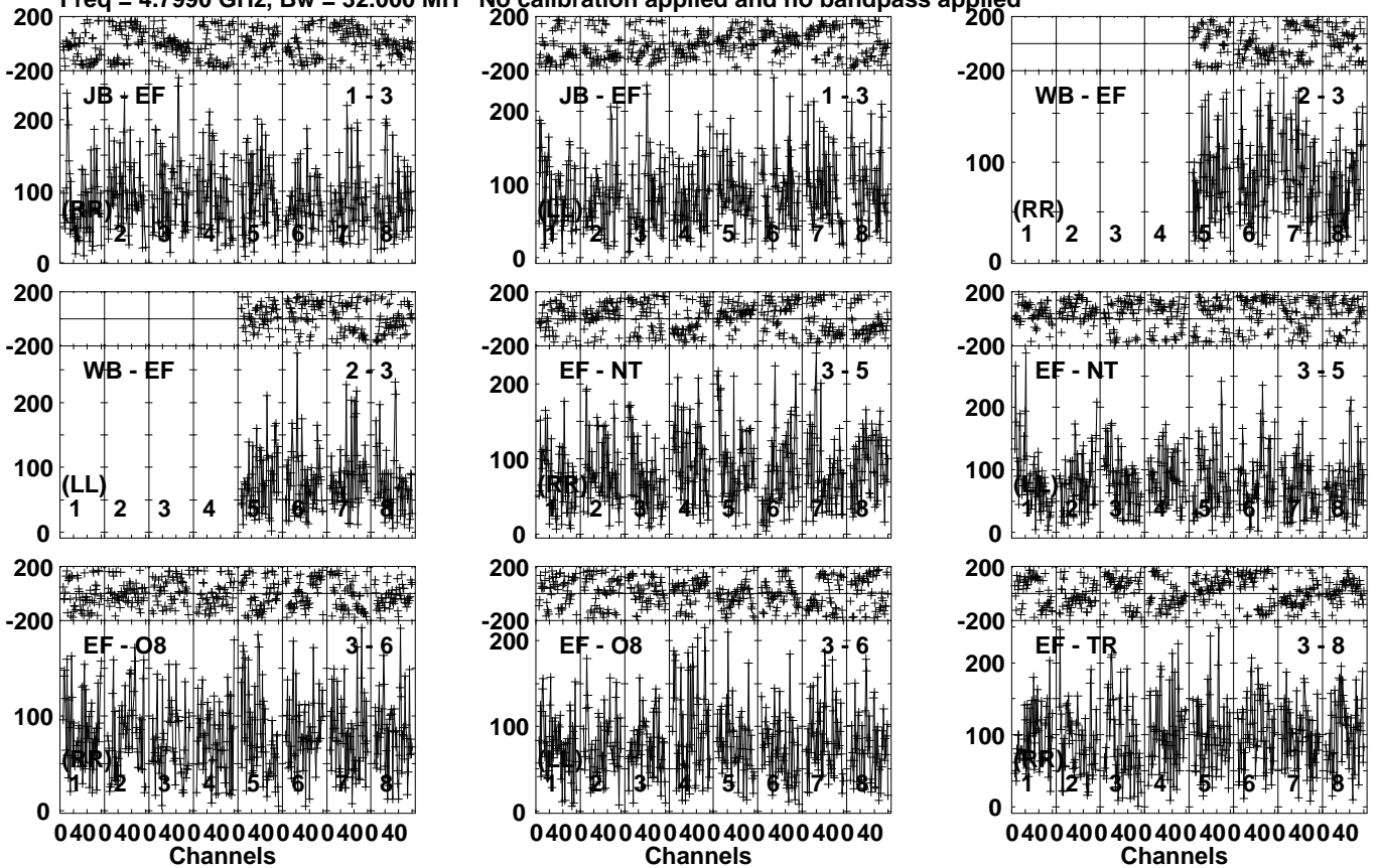
Lower frame: Micro Ampl Jy Top frame: Phas deg Vector averaged cross-power spectrum Several baselines displayed Timerange: 01/07:29:31 to 01/07:32:59
