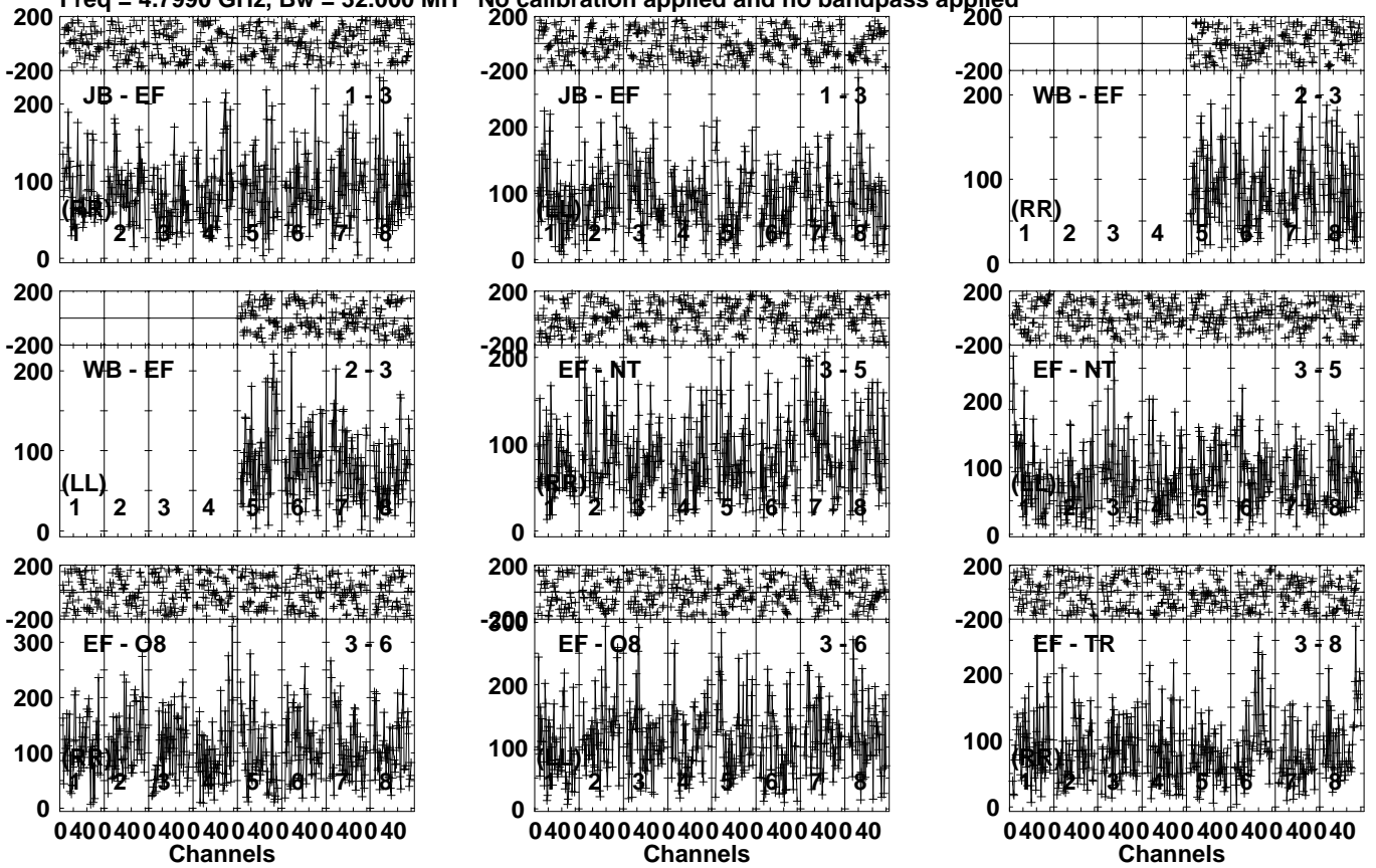
Lower frame: Micro Ampl Jy Top frame: Phas deg Vector averaged cross-power spectrum Several baselines displayed Timerange: 01/03:33:01 to 01/03:36:29
