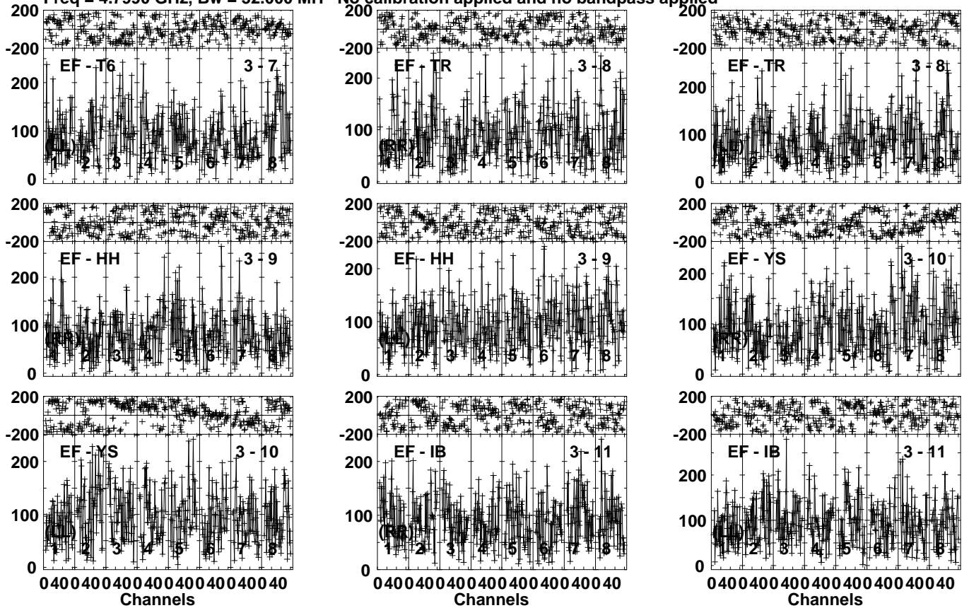
Lower frame: Micro Ampl Jy Top frame: Phas deg Vector averaged cross-power spectrum Several baselines displayed Timerange: 01/05:39:31 to 01/05:42:59
