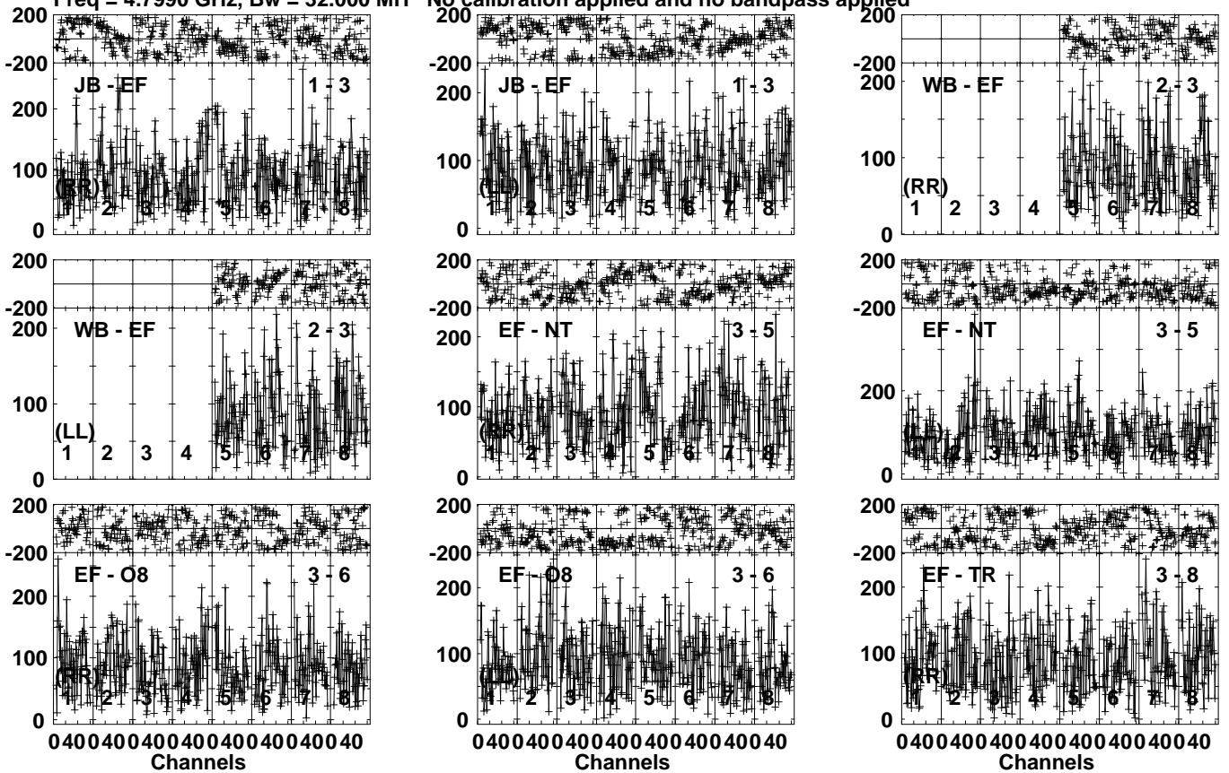
Lower frame: Micro Ampl Jy Top frame: Phas deg Vector averaged cross-power spectrum Several baselines displayed Timerange: 01/06:29:31 to 01/06:32:59
