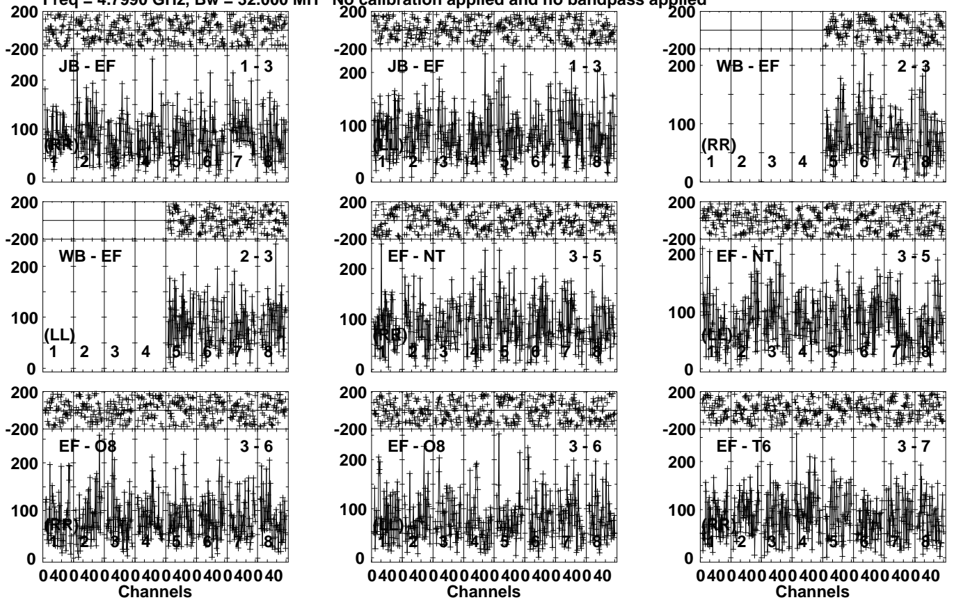
Lower frame: Micro Ampl Jy Top frame: Phas deg Vector averaged cross-power spectrum Several baselines displayed Timerange: 00/20:39:31 to 00/20:42:59
