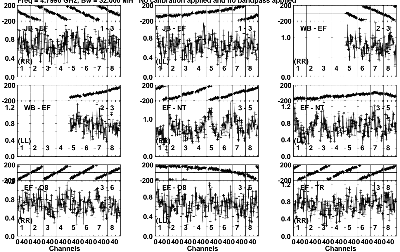
Lower frame: Milli Ampl Jy Top frame: Phas deg Vector averaged cross-power spectrum Several baselines displayed Timerange: 01/07:48:01 to 01/07:49:29
