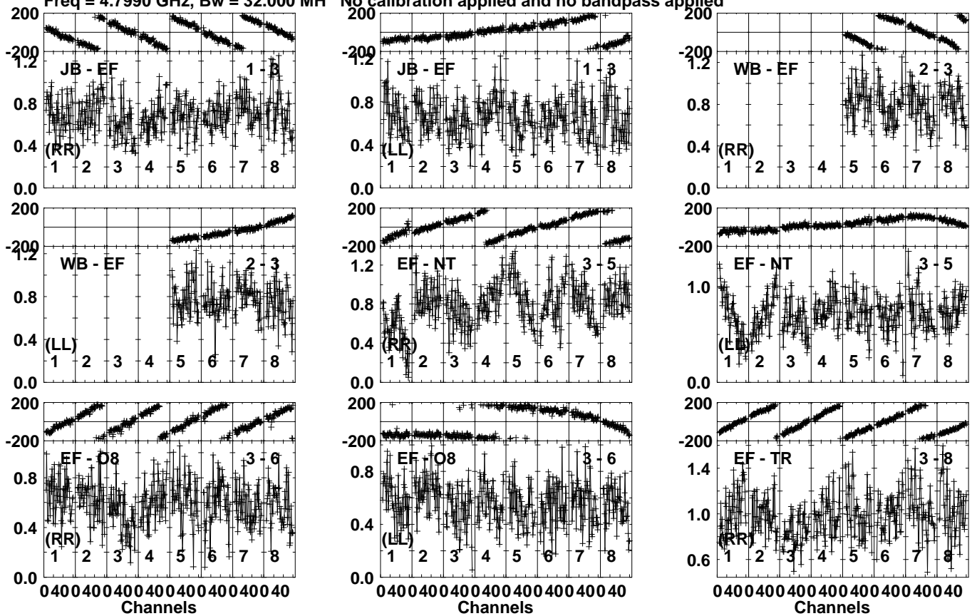
Lower frame: Milli Ampl Jy Top frame: Phas deg Vector averaged cross-power spectrum Several baselines displayed Timerange: 01/08:03:31 to 01/08:04:29
