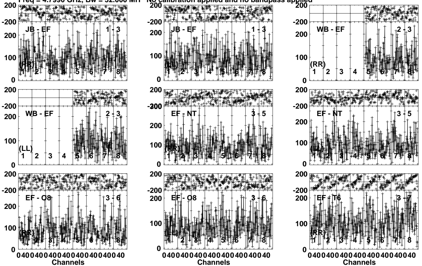
Lower frame: Micro Ampl Jy Top frame: Phas deg Vector averaged cross-power spectrum Several baselines displayed Timerange: 01/05:19:31 to 01/05:22:59
