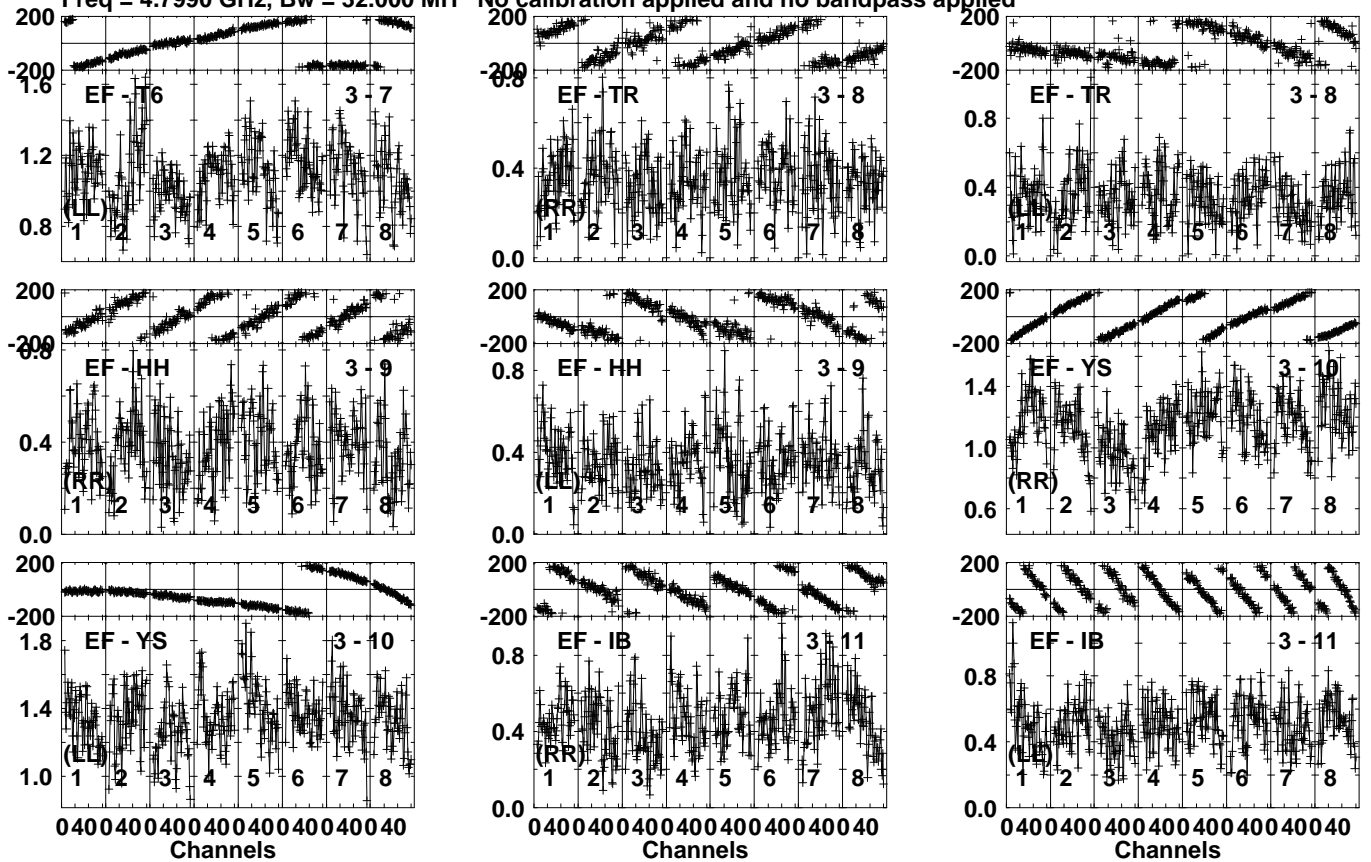
Lower frame: Milli Ampl Jy Top frame: Phas deg Vector averaged cross-power spectrum Several baselines displayed Timerange: 01/06:03:31 to 01/06:04:29
