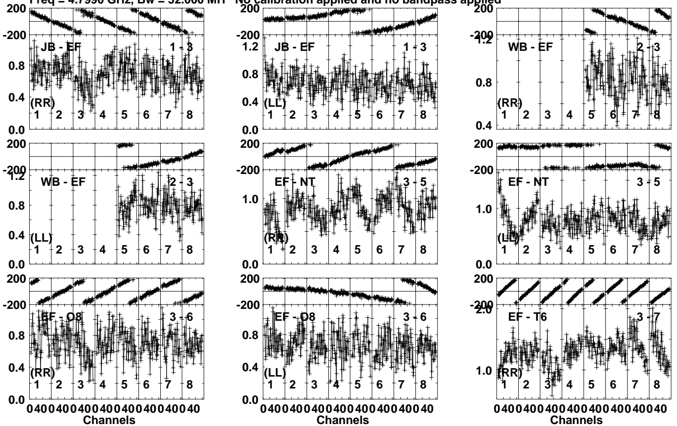
Lower frame: Milli Ampl Jy Top frame: Phas deg Vector averaged cross-power spectrum Several baselines displayed Timerange: 01/05:33:31 to 01/05:34:29
