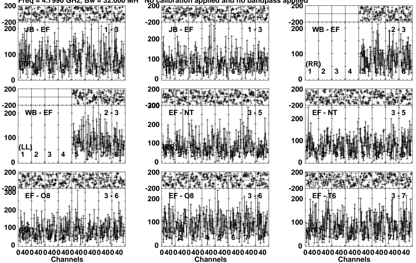
Lower frame: Micro Ampl Jy Top frame: Phas deg Vector averaged cross-power spectrum Several baselines displayed Timerange: 00/21:29:31 to 00/21:32:59
