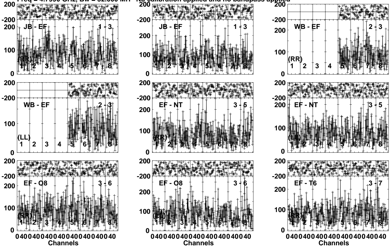
Lower frame: Micro Ampl Jy Top frame: Phas deg Vector averaged cross-power spectrum Several baselines displayed Timerange: 00/21:54:31 to 00/21:57:59
