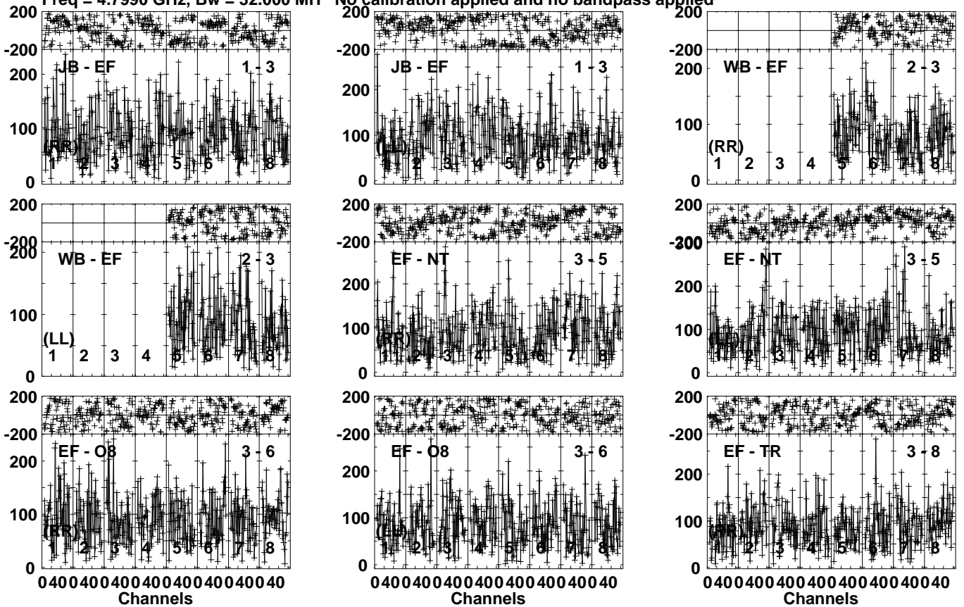
Lower frame: Micro Ampl Jy Top frame: Phas deg Vector averaged cross-power spectrum Several baselines displayed Timerange: 01/09:09:31 to 01/09:12:59
