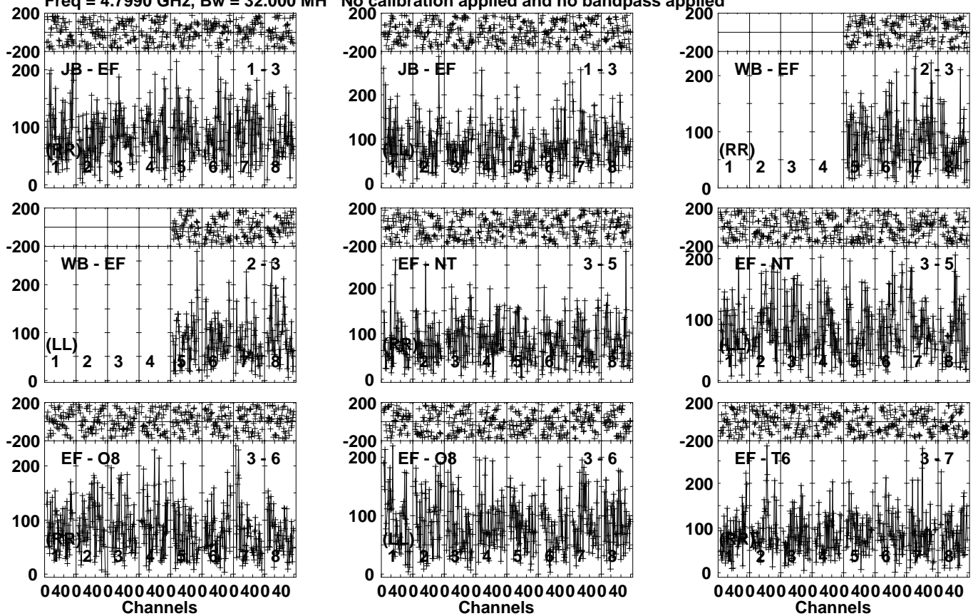
Lower frame: Micro Ampl Jy Top frame: Phas deg Vector averaged cross-power spectrum Several baselines displayed Timerange: 00/21:24:31 to 00/21:27:59
