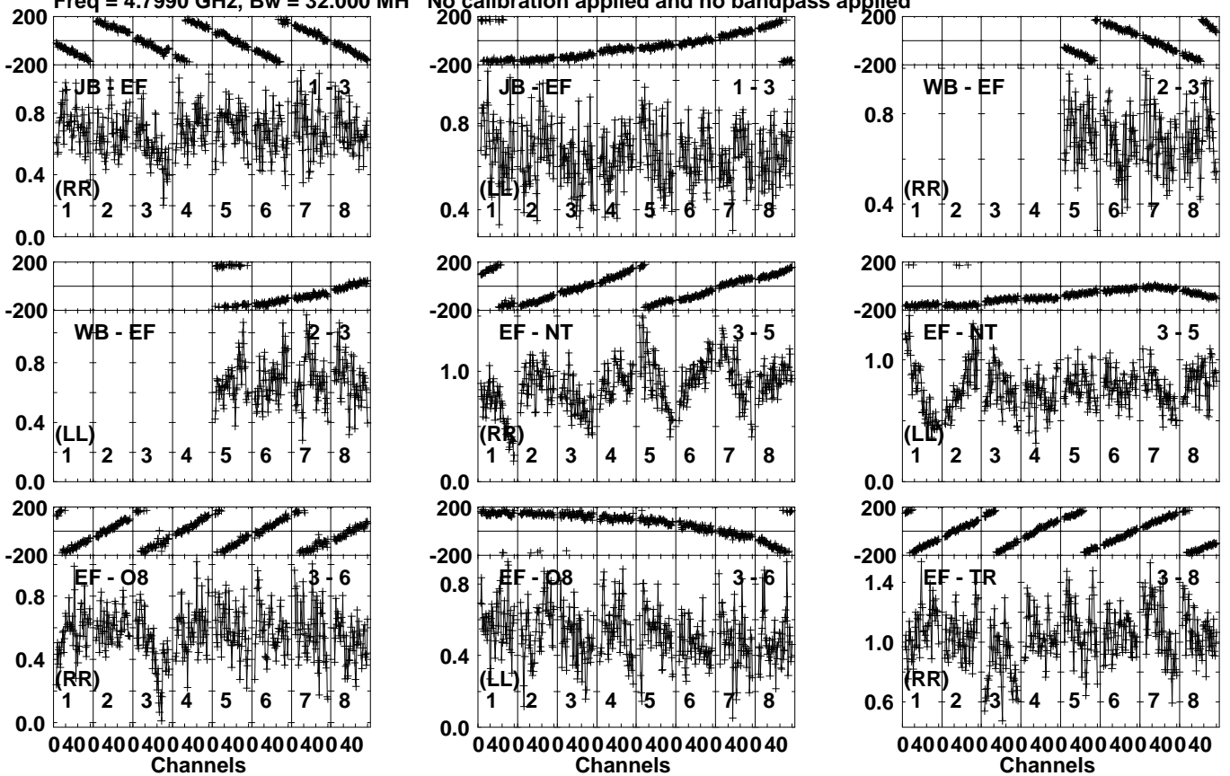
Lower frame: Milli Ampl Jy Top frame: Phas deg Vector averaged cross-power spectrum Several baselines displayed Timerange: 01/08:43:31 to 01/08:44:29
