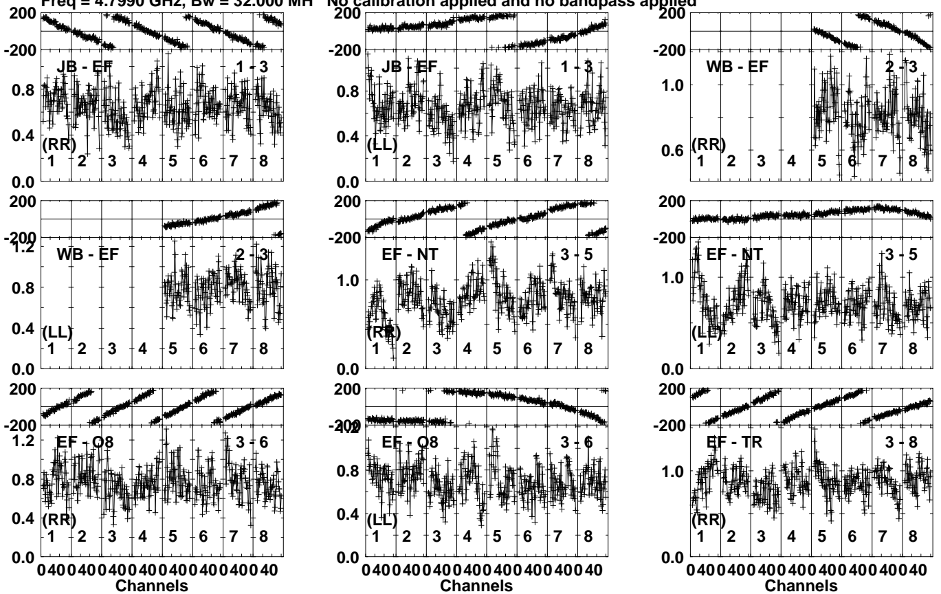
Lower frame: Milli Ampl Jy Top frame: Phas deg Vector averaged cross-power spectrum Several baselines displayed Timerange: 01/06:38:01 to 01/06:39:29
