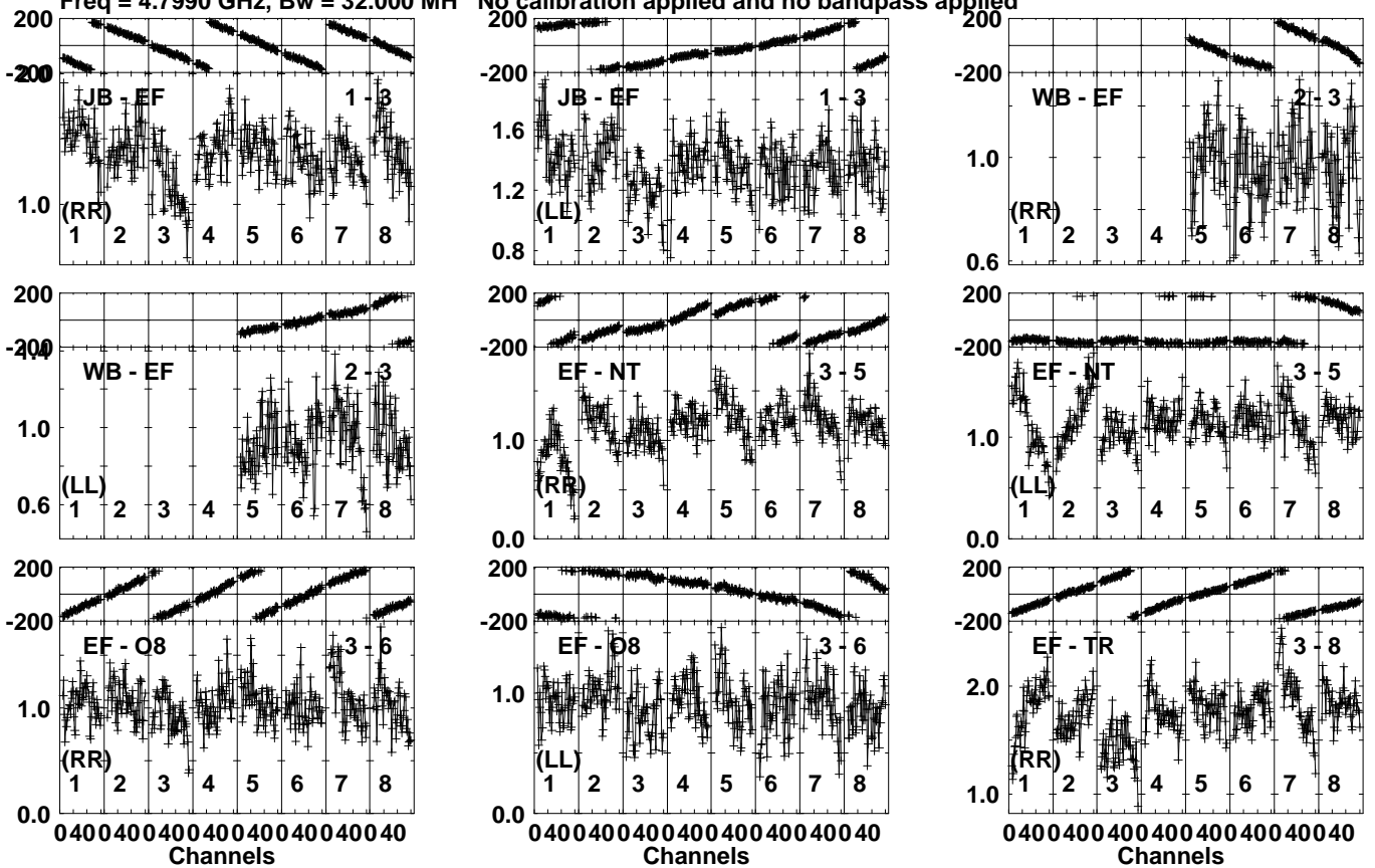
Lower frame: Milli Ampl Jy Top frame: Phas deg Vector averaged cross-power spectrum Several baselines displayed Timerange: 01/00:46:31 to 01/00:47:59
