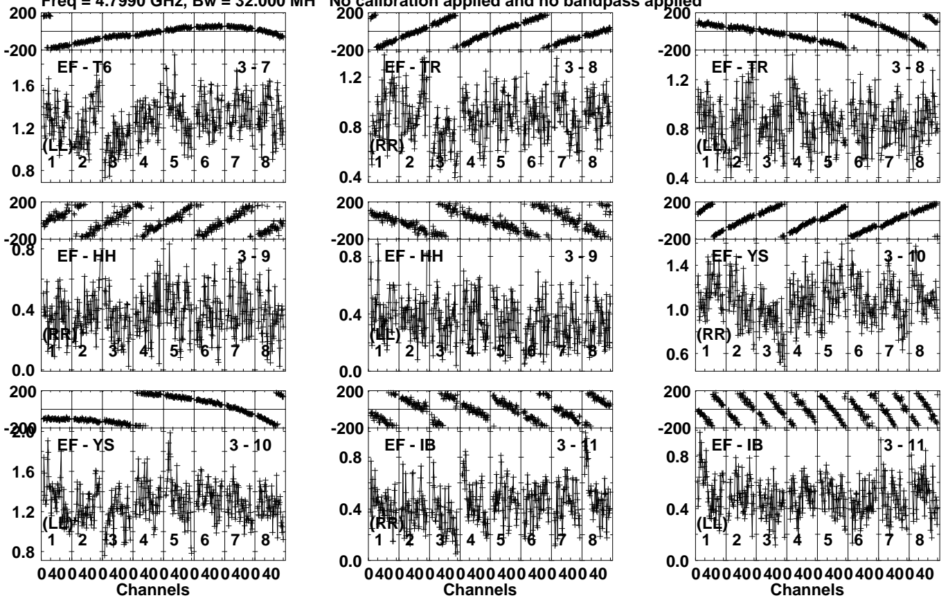
Lower frame: Milli Ampl Jy Top frame: Phas deg Vector averaged cross-power spectrum Several baselines displayed Timerange: 01/05:23:31 to 01/05:24:29
