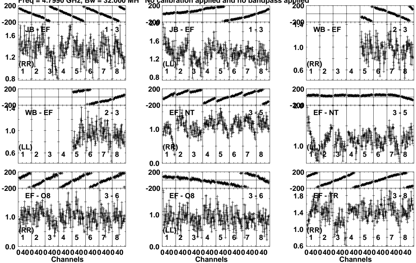
Lower frame: Milli Ampl Jy Top frame: Phas deg Vector averaged cross-power spectrum Several baselines displayed Timerange: 01/02:06:31 to 01/02:07:59
