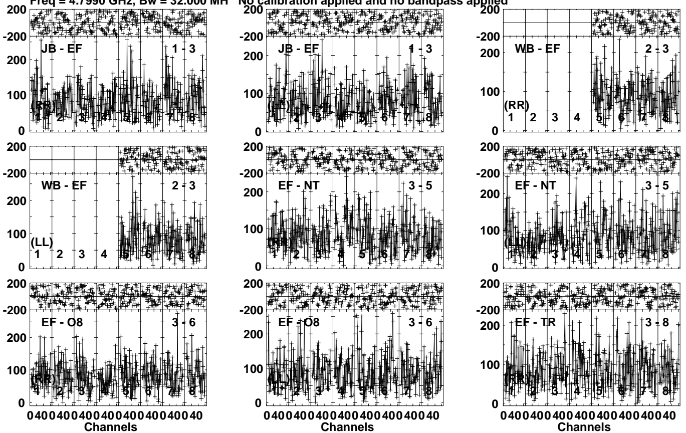
Lower frame: Micro Ampl Jy Top frame: Phas deg Vector averaged cross-power spectrum Several baselines displayed Timerange: 00/23:29:31 to 00/23:32:59
