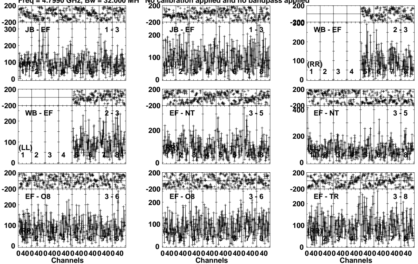
Lower frame: Micro Ampl Jy Top frame: Phas deg Vector averaged cross-power spectrum Several baselines displayed Timerange: 01/07:44:31 to 01/07:47:59
