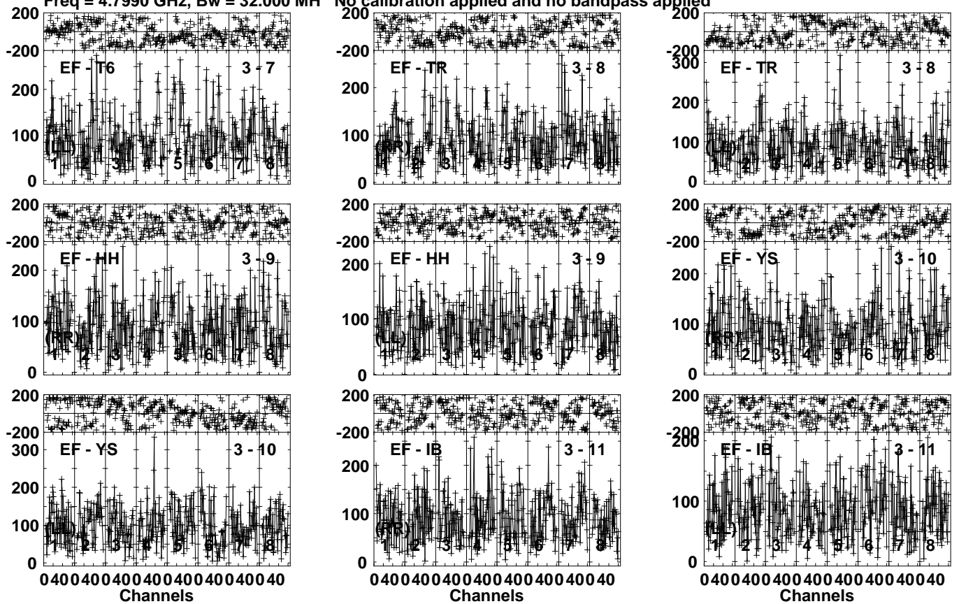
Lower frame: Micro Ampl Jy Top frame: Phas deg Vector averaged cross-power spectrum Several baselines displayed Timerange: 01/05:34:31 to 01/05:37:59
