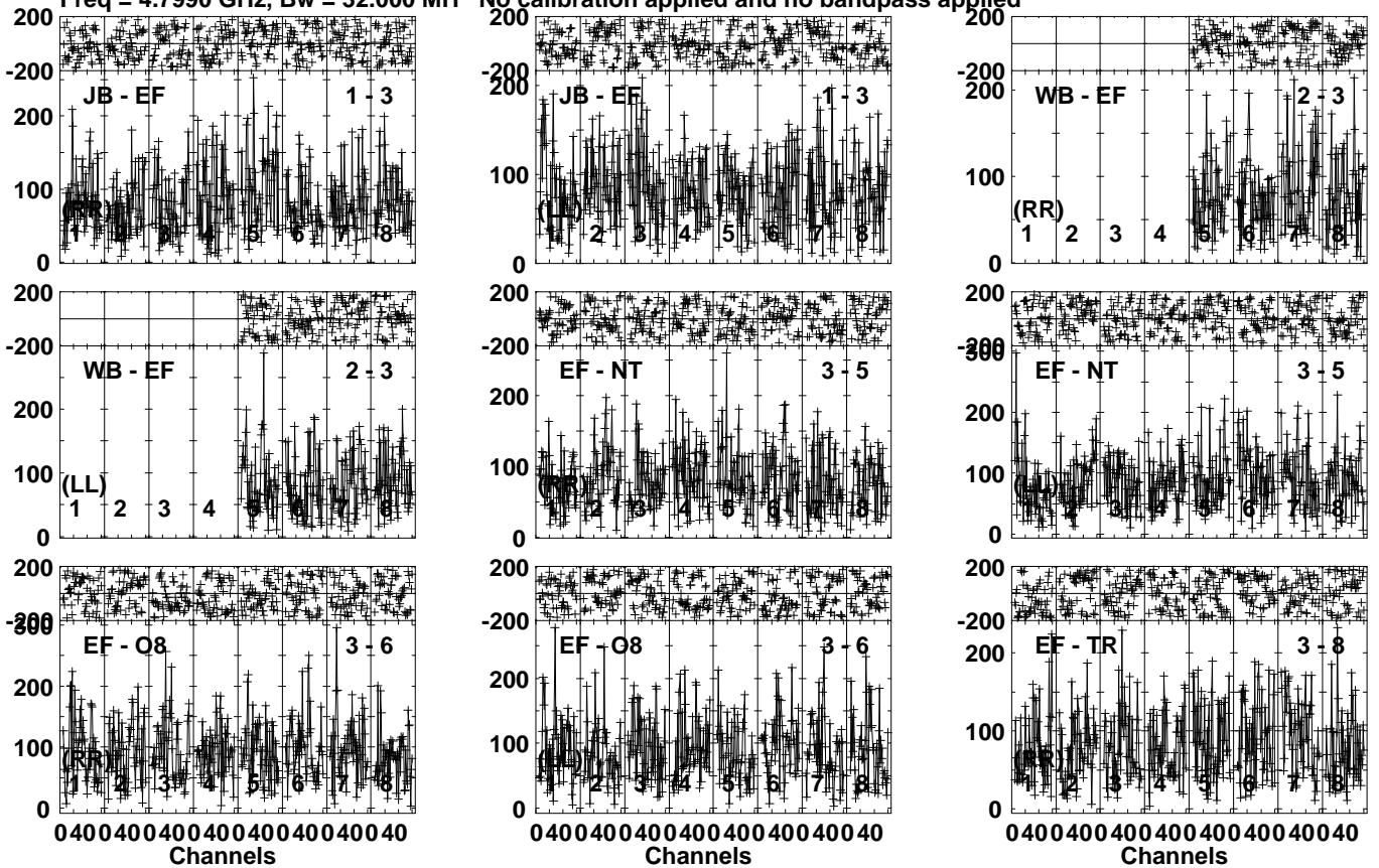
Lower frame: Micro Ampl Jy Top frame: Phas deg Vector averaged cross-power spectrum Several baselines displayed Timerange: 01/00:43:01 to 01/00:46:29
