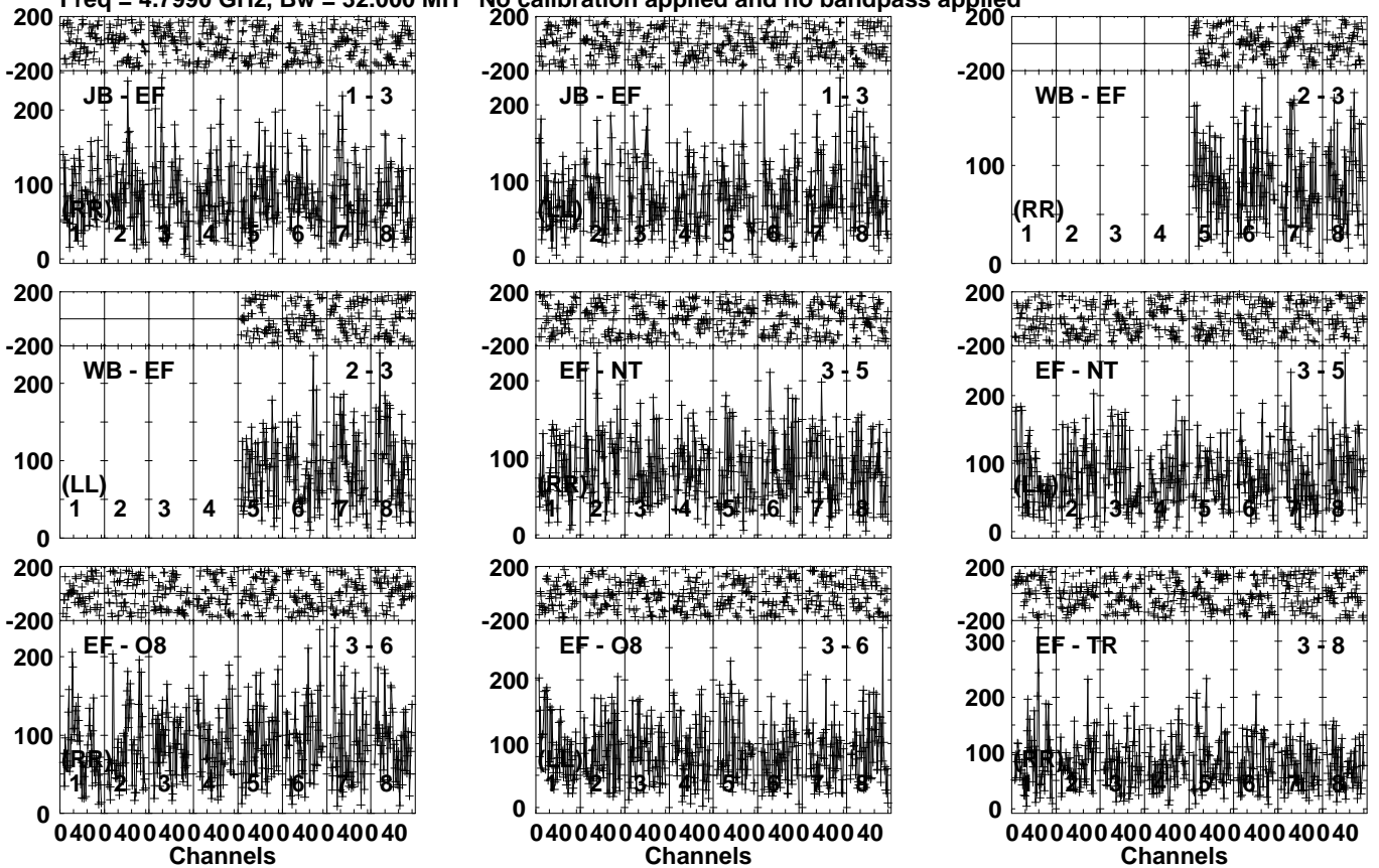
Lower frame: Micro Ampl Jy Top frame: Phas deg Vector averaged cross-power spectrum Several baselines displayed Timerange: 00/23:39:31 to 00/23:42:59
