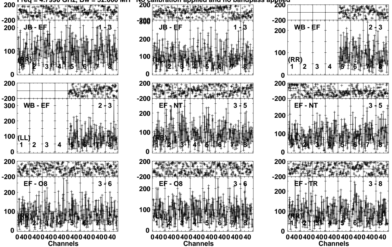
Lower frame: Micro Ampl Jy Top frame: Phas deg Vector averaged cross-power spectrum Several baselines displayed Timerange: 01/07:54:31 to 01/07:57:59
