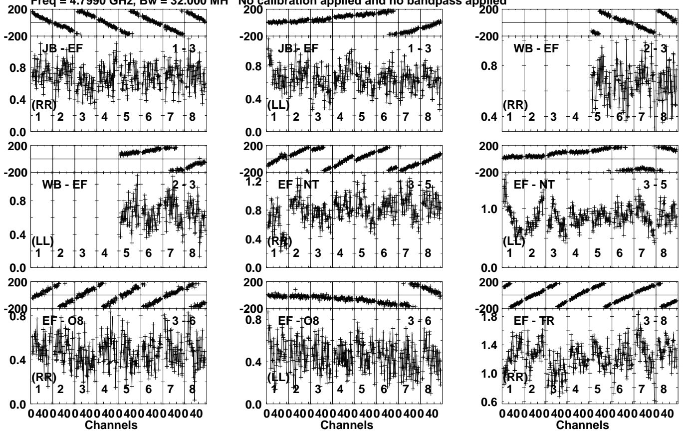
Lower frame: Milli Ampl Jy Top frame: Phas deg Vector averaged cross-power spectrum Several baselines displayed Timerange: 01/09:38:01 to 01/09:39:29
