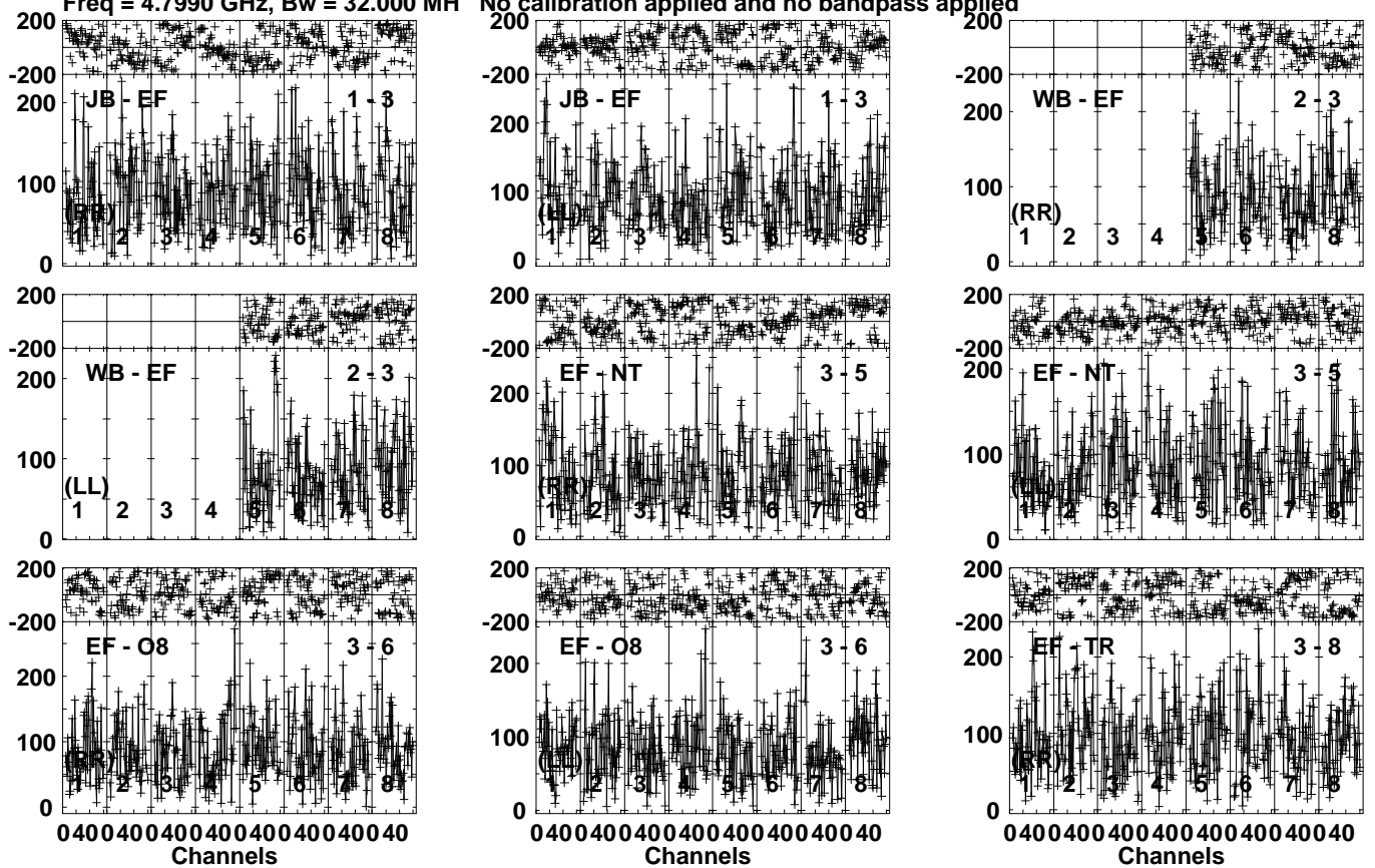
Lower frame: Micro Ampl Jy Top frame: Phas deg Vector averaged cross-power spectrum Several baselines displayed Timerange: 01/06:39:31 to 01/06:42:59
