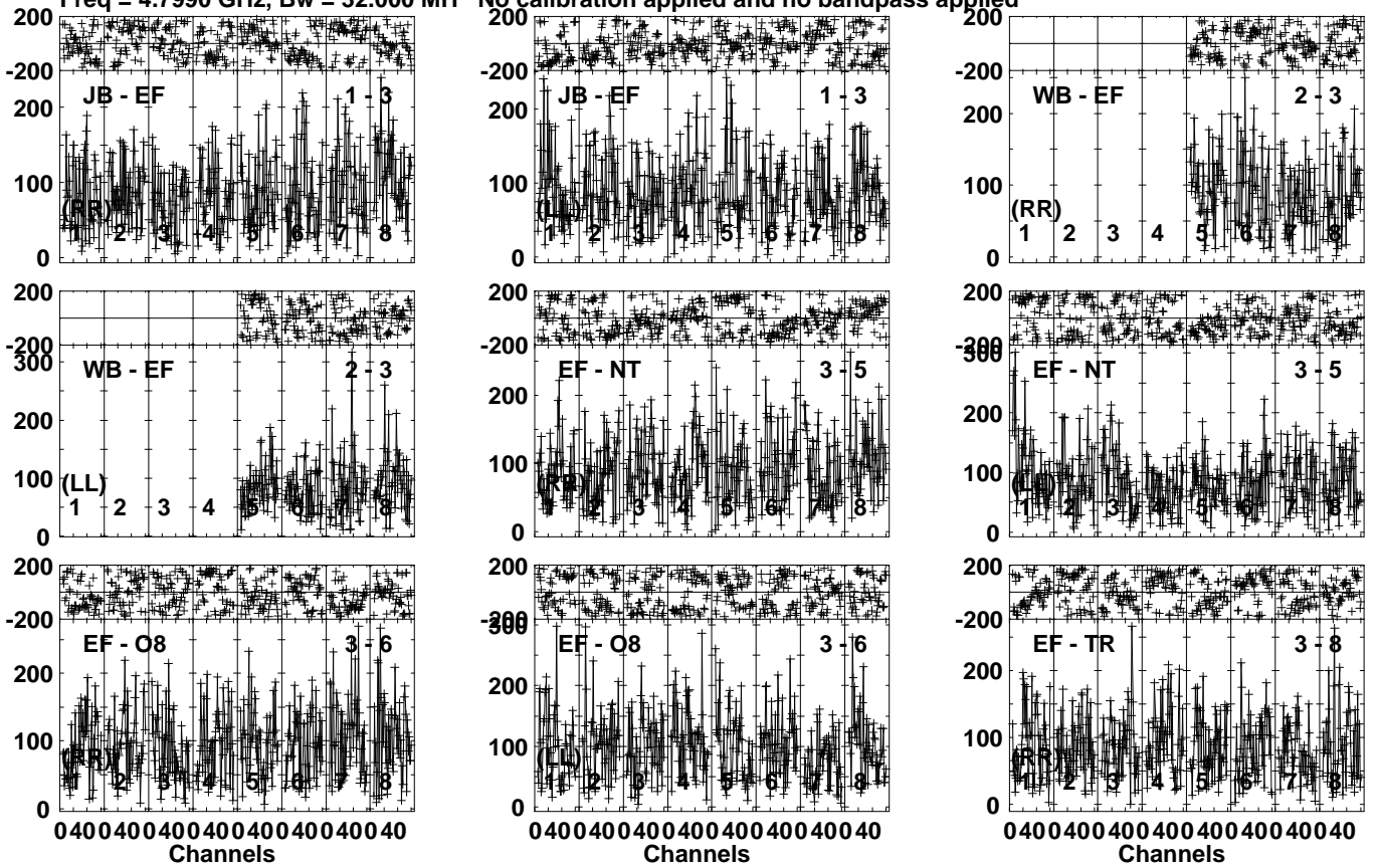
Lower frame: Micro Ampl Jy Top frame: Phas deg Vector averaged cross-power spectrum Several baselines displayed Timerange: 01/08:39:31 to 01/08:42:59
