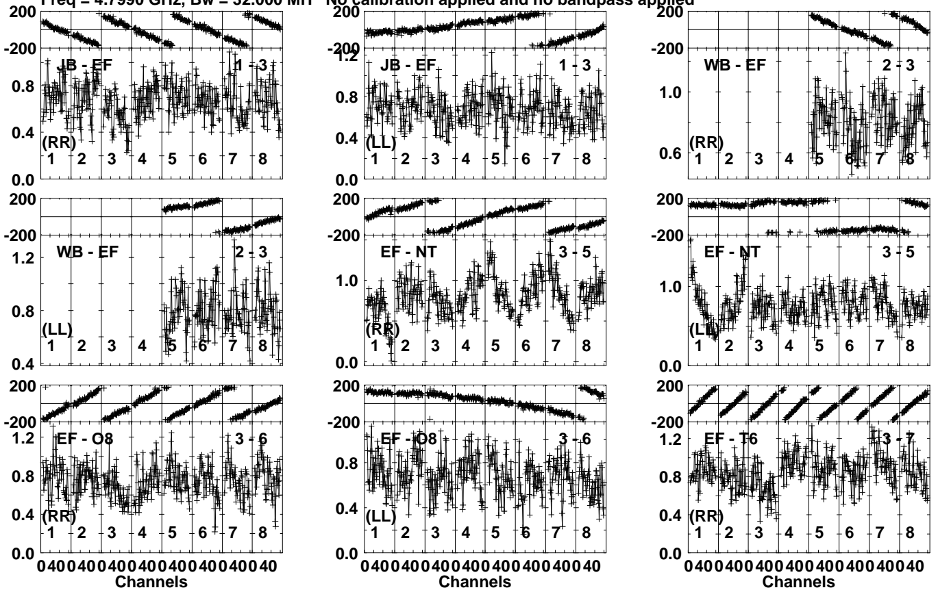
Lower frame: Milli Ampl Jy Top frame: Phas deg Vector averaged cross-power spectrum Several baselines displayed Timerange: 01/05:58:01 to 01/05:59:29
