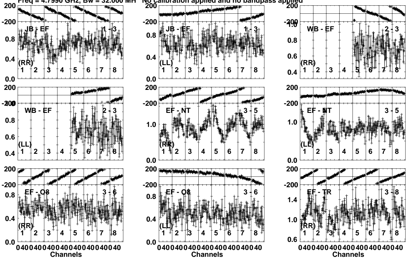
Lower frame: Milli Ampl Jy Top frame: Phas deg Vector averaged cross-power spectrum Several baselines displayed Timerange: 01/09:13:31 to 01/09:14:29
