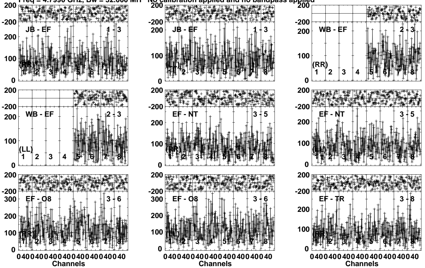
Lower frame: Micro Ampl Jy Top frame: Phas deg Vector averaged cross-power spectrum Several baselines displayed Timerange: 01/03:23:01 to 01/03:26:29
