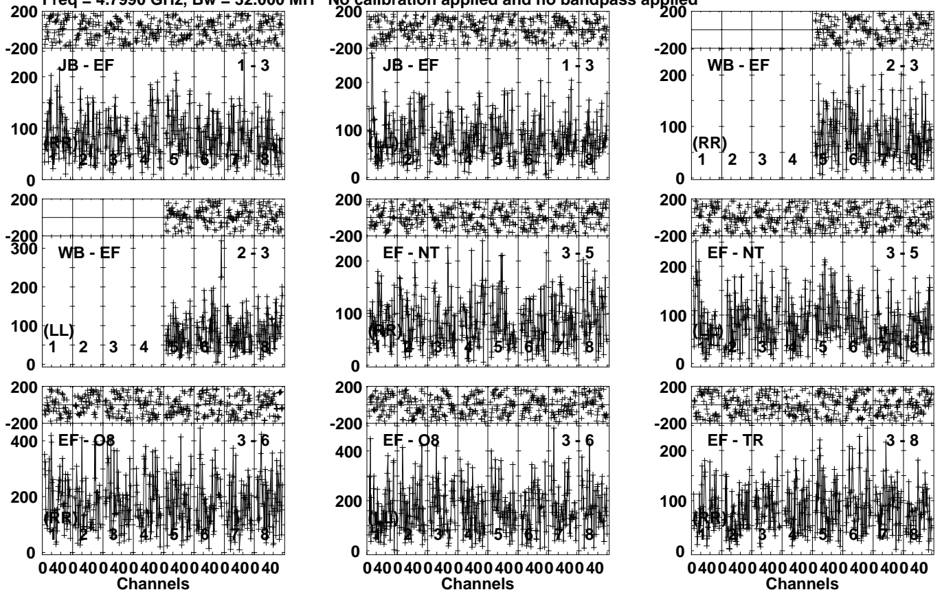
Lower frame: Micro Ampl Jy Top frame: Phas deg Vector averaged cross-power spectrum Several baselines displayed Timerange: 01/01:18:01 to 01/01:21:29
