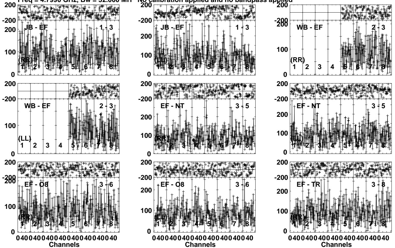
Lower frame: Micro Ampl Jy Top frame: Phas deg Vector averaged cross-power spectrum Several baselines displayed Timerange: 01/06:54:31 to 01/06:57:59
