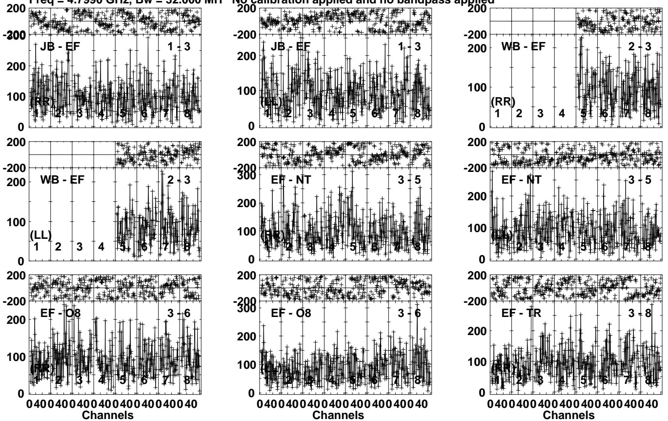
Lower frame: Micro Ampl Jy Top frame: Phas deg Vector averaged cross-power spectrum Several baselines displayed Timerange: 01/07:59:31 to 01/08:02:59
