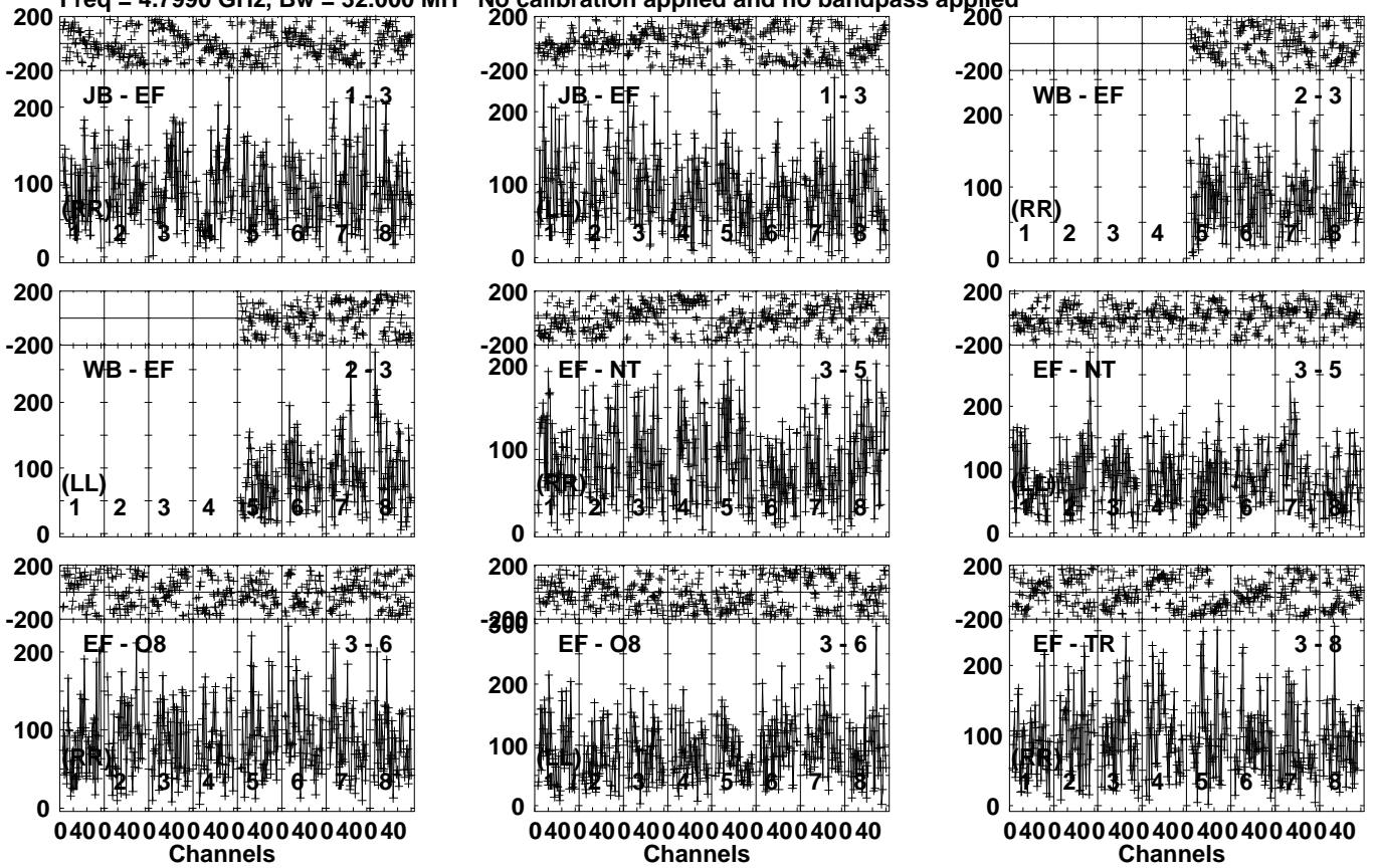
Lower frame: Micro Ampl Jy Top frame: Phas deg Vector averaged cross-power spectrum Several baselines displayed Timerange: 01/06:49:31 to 01/06:52:59
