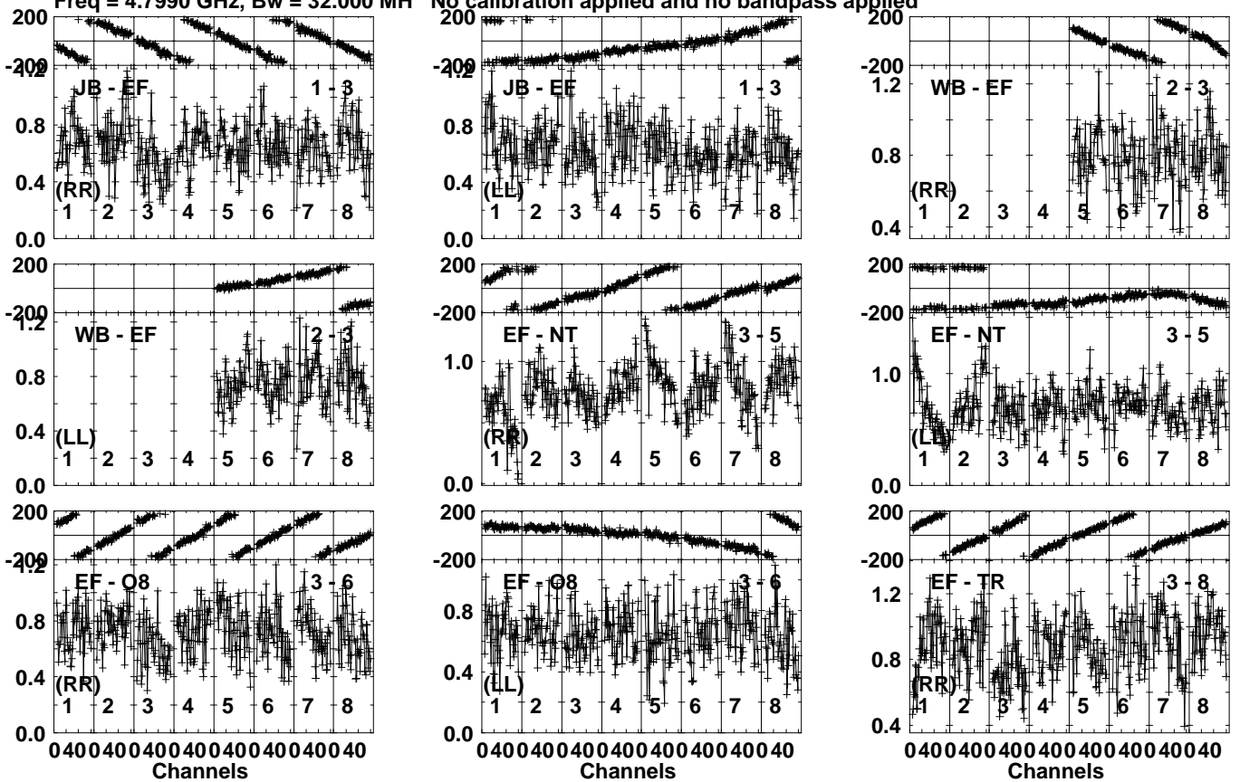
Lower frame: Milli Ampl Jy Top frame: Phas deg Vector averaged cross-power spectrum Several baselines displayed Timerange: 01/07:38:01 to 01/07:39:29
