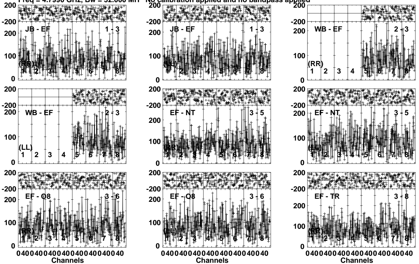
Lower frame: Micro Ampl Jy Top frame: Phas deg Vector averaged cross-power spectrum Several baselines displayed Timerange: 00/23:19:31 to 00/23:22:59
