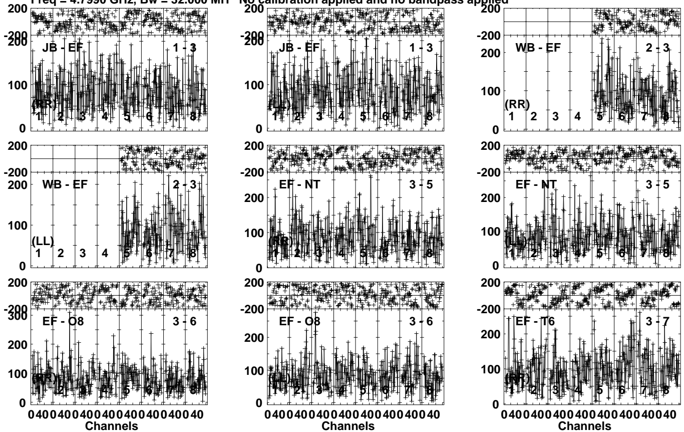
Lower frame: Micro Ampl Jy Top frame: Phas deg Vector averaged cross-power spectrum Several baselines displayed Timerange: 01/04:04:31 to 01/04:07:59
