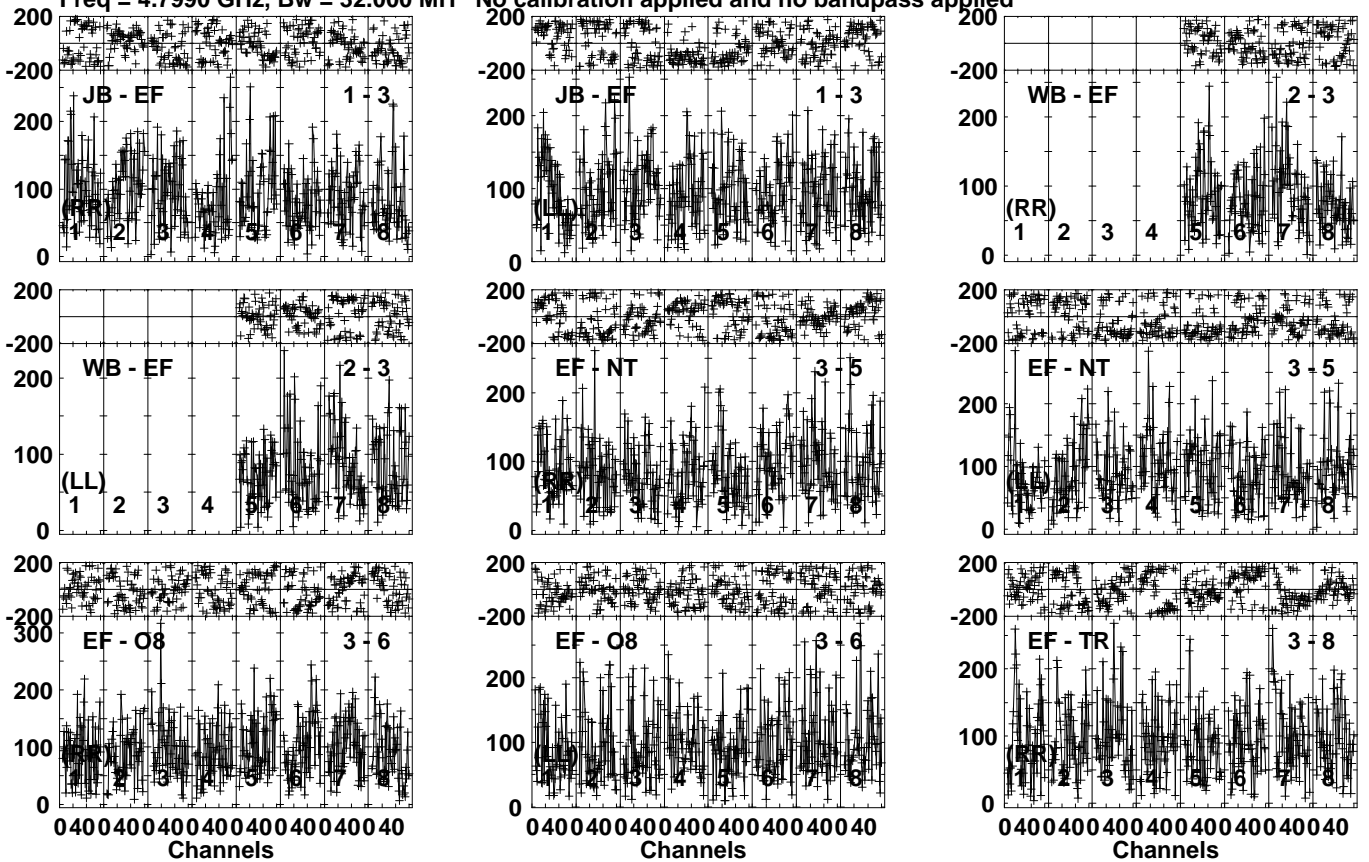
Lower frame: Micro Ampl Jy Top frame: Phas deg Vector averaged cross-power spectrum Several baselines displayed Timerange: 01/08:49:31 to 01/08:52:59
