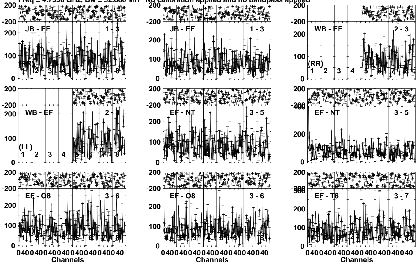
Lower frame: Micro Ampl Jy Top frame: Phas deg Vector averaged cross-power spectrum Several baselines displayed Timerange: 00/20:09:31 to 00/20:12:59
