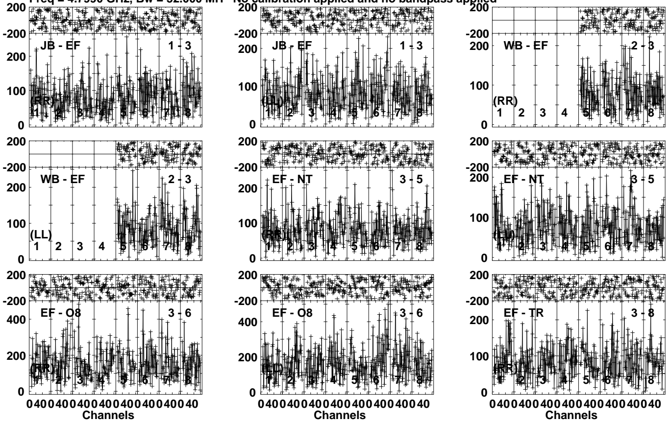
Lower frame: Micro Ampl Jy Top frame: Phas deg Vector averaged cross-power spectrum Several baselines displayed Timerange: 01/01:33:01 to 01/01:36:29
