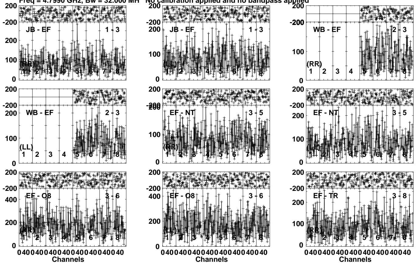
Lower frame: Micro Ampl Jy Top frame: Phas deg Vector averaged cross-power spectrum Several baselines displayed Timerange: 01/02:23:01 to 01/02:26:29
