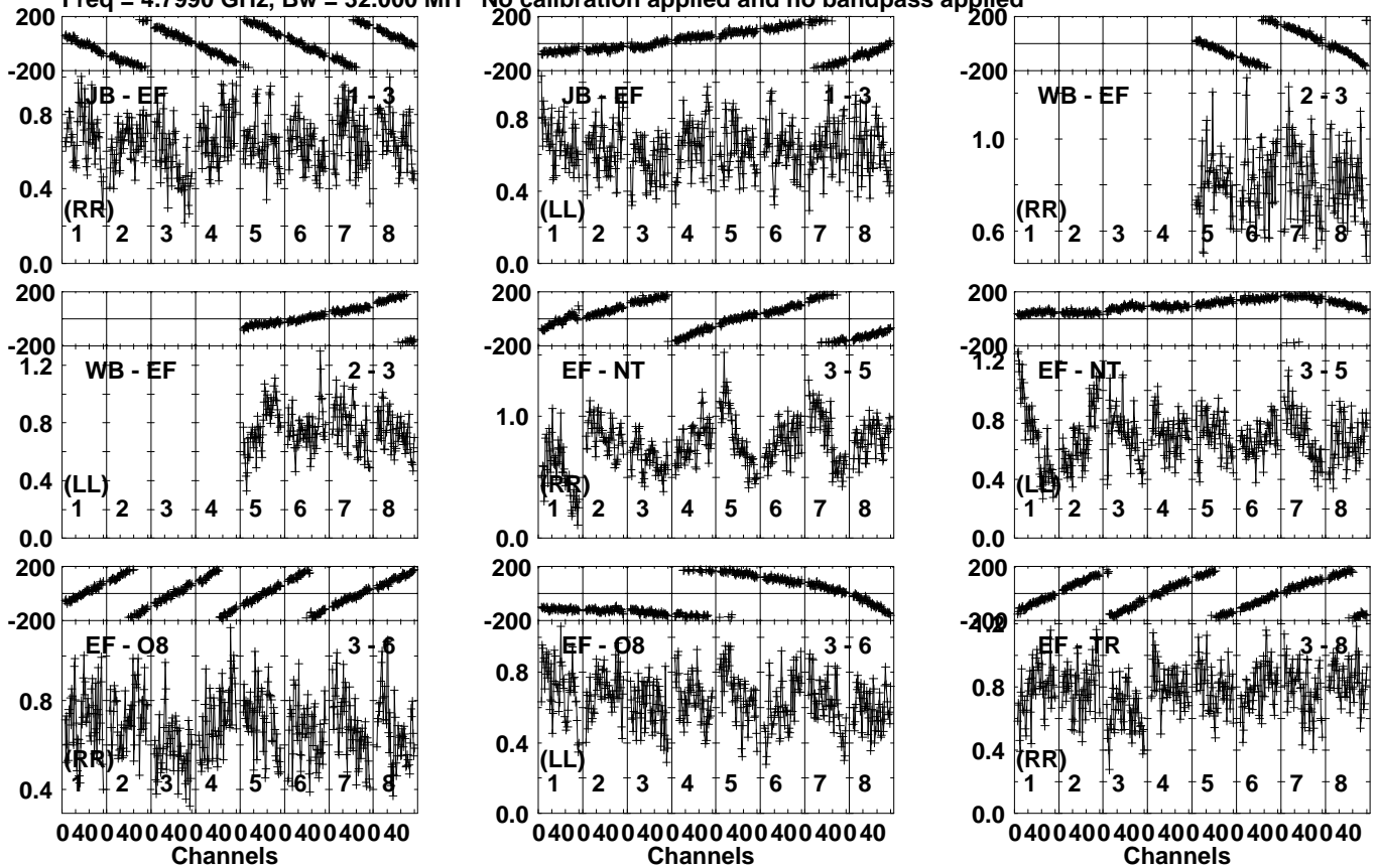
Lower frame: Milli Ampl Jy Top frame: Phas deg Vector averaged cross-power spectrum Several baselines displayed Timerange: 01/06:53:31 to 01/06:54:29
