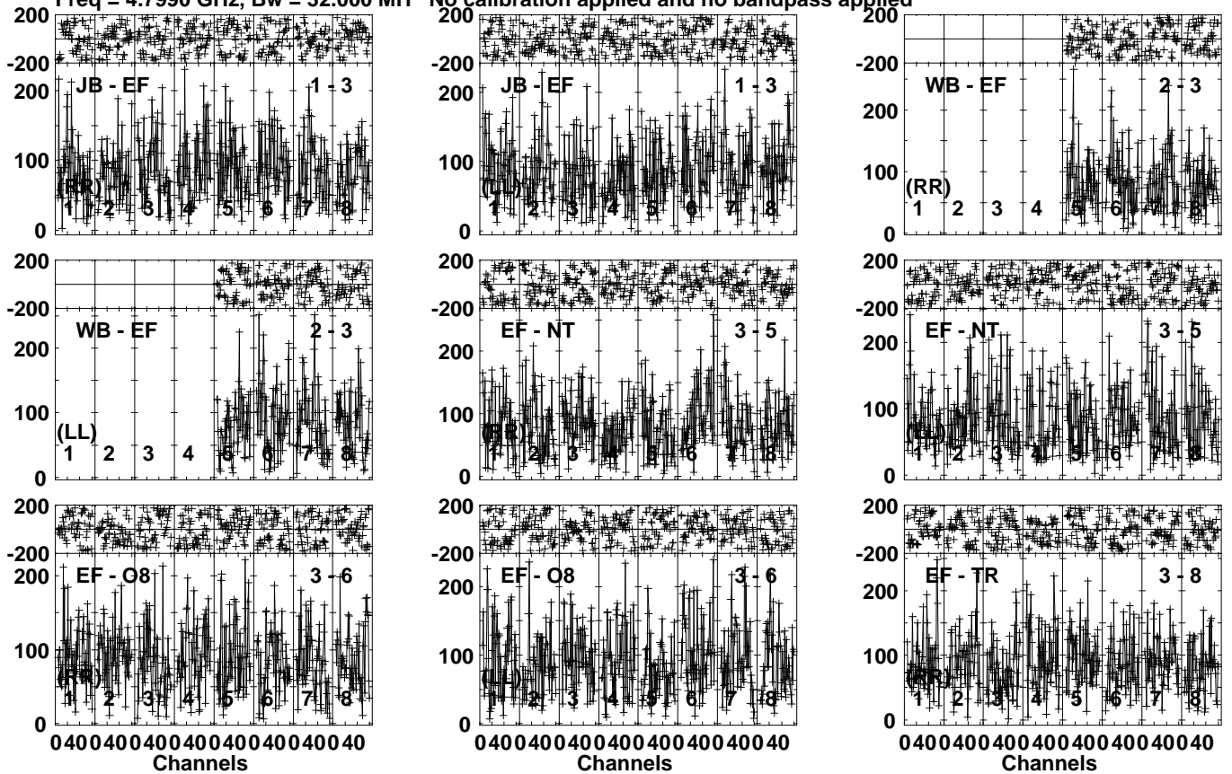
Lower frame: Micro Ampl Jy Top frame: Phas deg Vector averaged cross-power spectrum Several baselines displayed Timerange: 00/22:34:31 to 00/22:37:59
