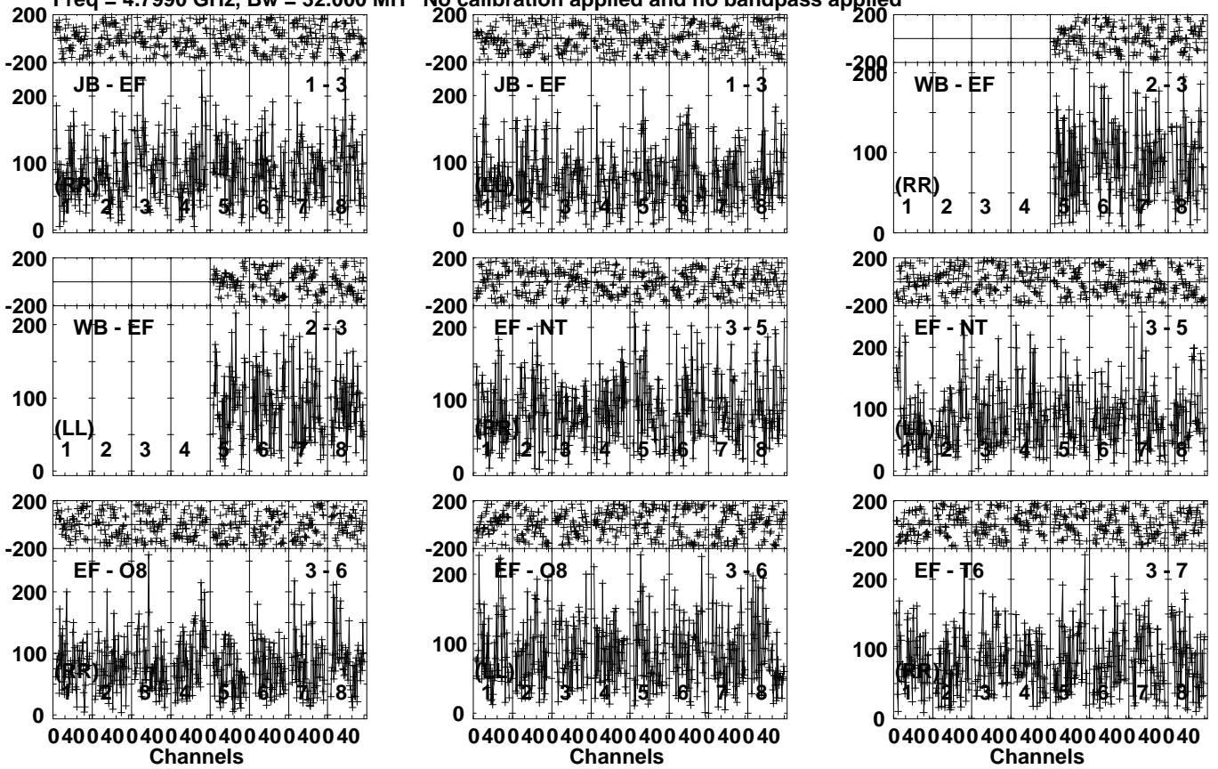
Lower frame: Micro Ampl Jy Top frame: Phas deg Vector averaged cross-power spectrum Several baselines displayed Timerange: 00/21:19:31 to 00/21:22:59
