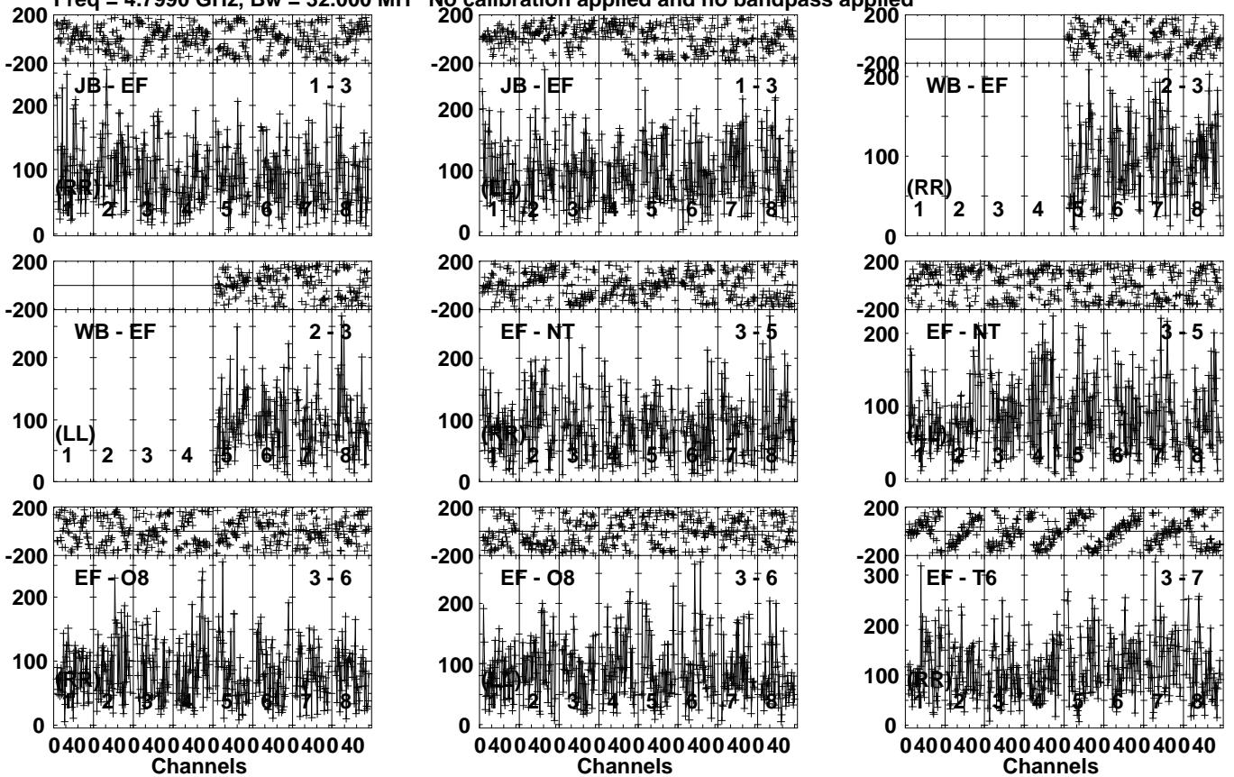
Lower frame: Micro Ampl Jy Top frame: Phas deg Vector averaged cross-power spectrum Several baselines displayed Timerange: 01/04:54:31 to 01/04:57:59
