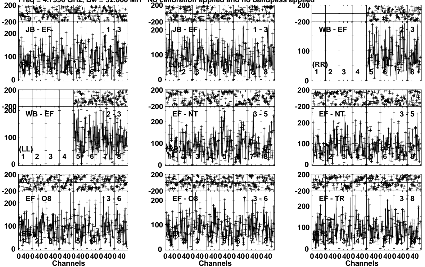
Lower frame: Micro Ampl Jy Top frame: Phas deg Vector averaged cross-power spectrum Several baselines displayed Timerange: 01/07:04:31 to 01/07:07:59
