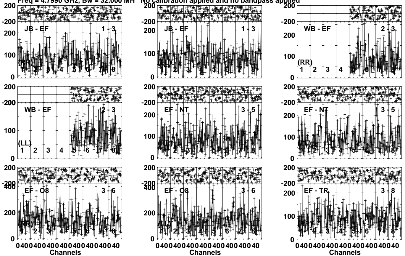
Lower frame: Micro Ampl Jy Top frame: Phas deg Vector averaged cross-power spectrum Several baselines displayed Timerange: 01/01:53:01 to 01/01:56:29
