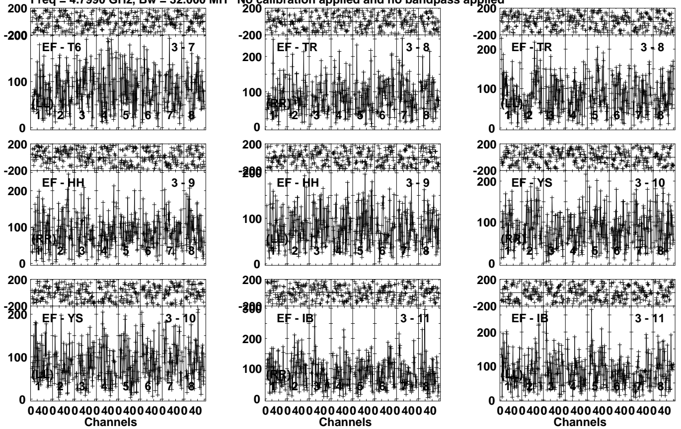
Lower frame: Micro Ampl Jy Top frame: Phas deg Vector averaged cross-power spectrum Several baselines displayed Timerange: 00/22:04:31 to 00/22:07:59
