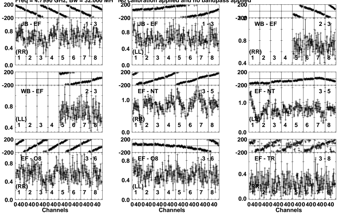
Lower frame: Milli Ampl Jy Top frame: Phas deg Vector averaged cross-power spectrum Several baselines displayed Timerange: 01/08:28:01 to 01/08:29:29
