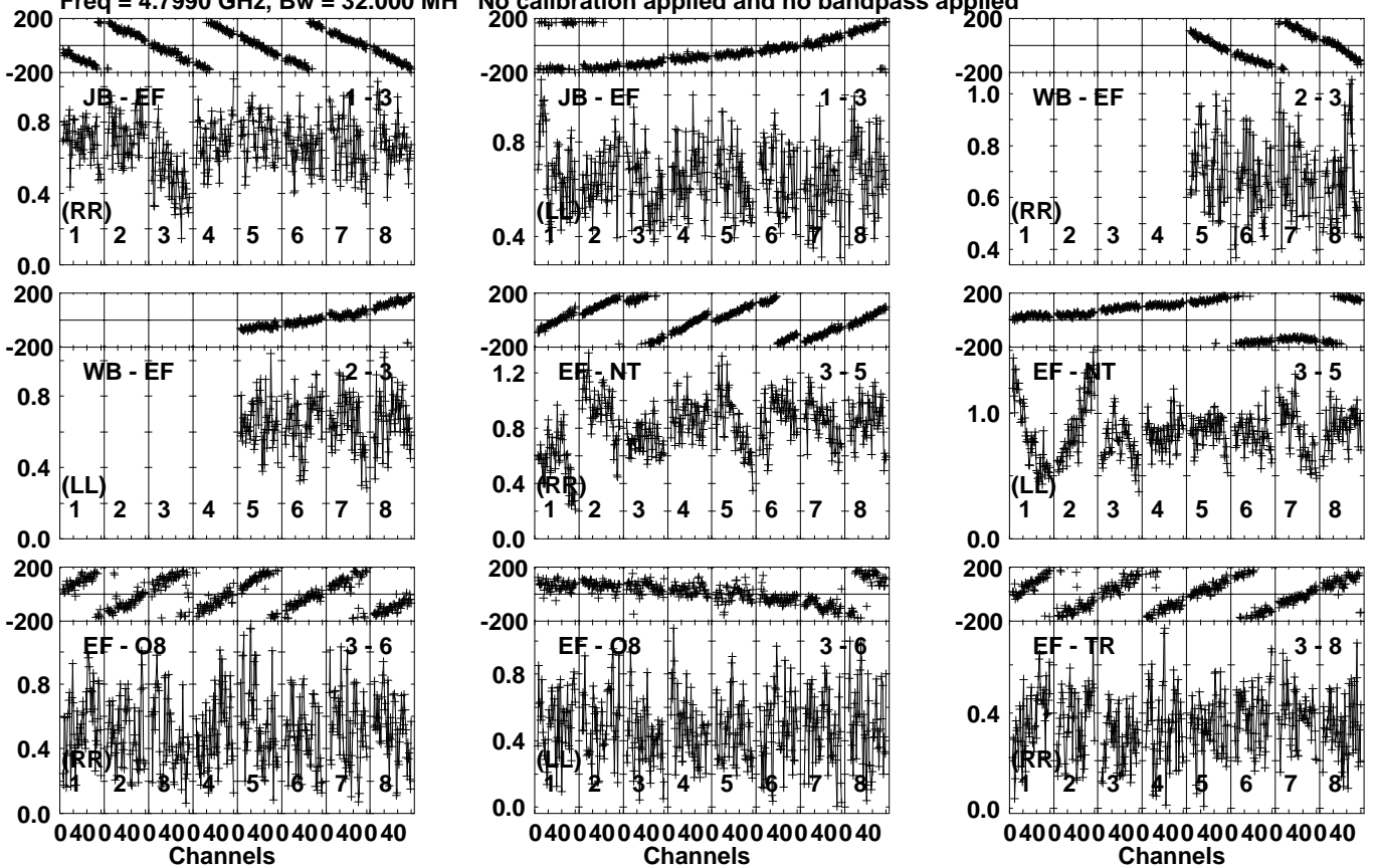
Lower frame: Milli Ampl Jy Top frame: Phas deg Vector averaged cross-power spectrum Several baselines displayed Timerange: 01/09:53:01 to 01/09:54:29
