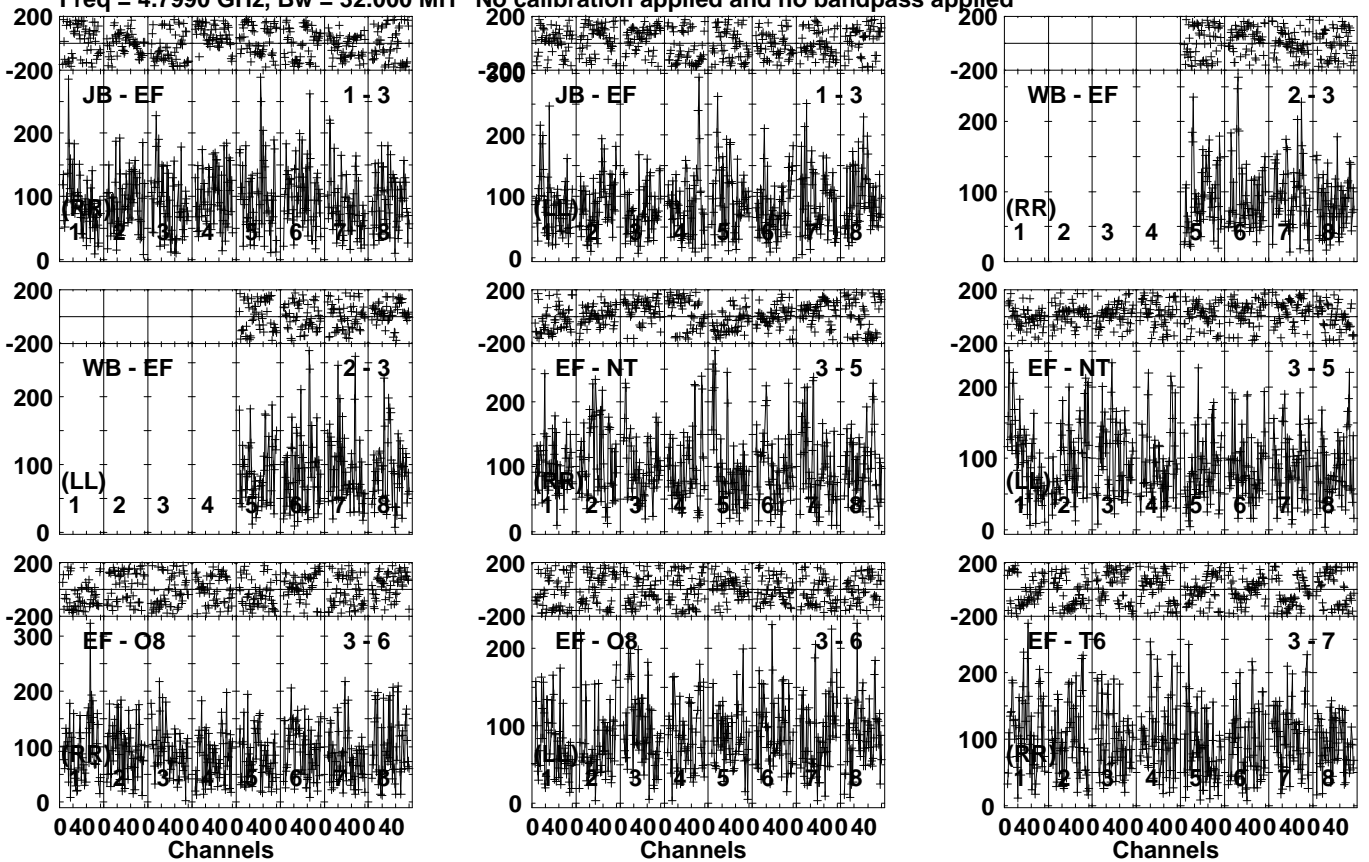
Lower frame: Micro Ampl Jy Top frame: Phas deg Vector averaged cross-power spectrum Several baselines displayed Timerange: 01/05:29:31 to 01/05:32:59
