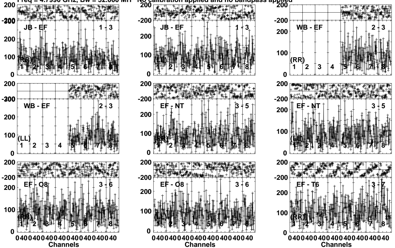
Lower frame: Micro Ampl Jy Top frame: Phas deg Vector averaged cross-power spectrum Several baselines displayed Timerange: 01/04:59:31 to 01/05:02:59
