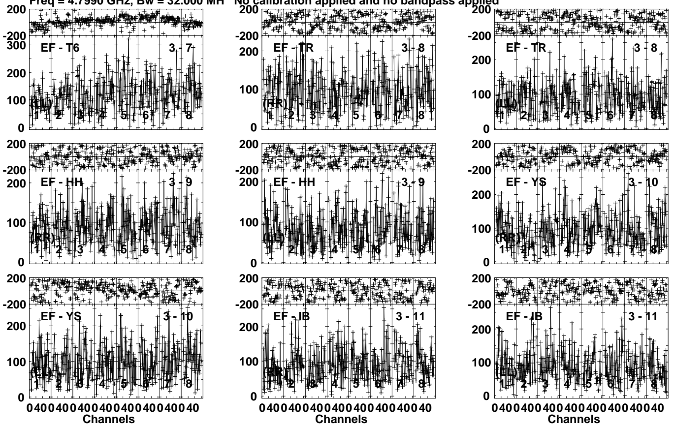
Lower frame: Micro Ampl Jy Top frame: Phas deg Vector averaged cross-power spectrum Several baselines displayed Timerange: 01/04:39:31 to 01/04:42:59
