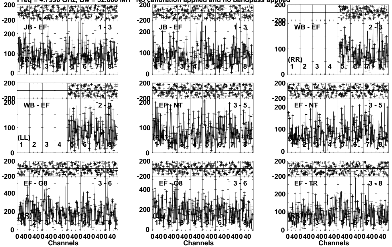
Lower frame: Micro Ampl Jy Top frame: Phas deg Vector averaged cross-power spectrum Several baselines displayed Timerange: 01/02:33:01 to 01/02:36:29
