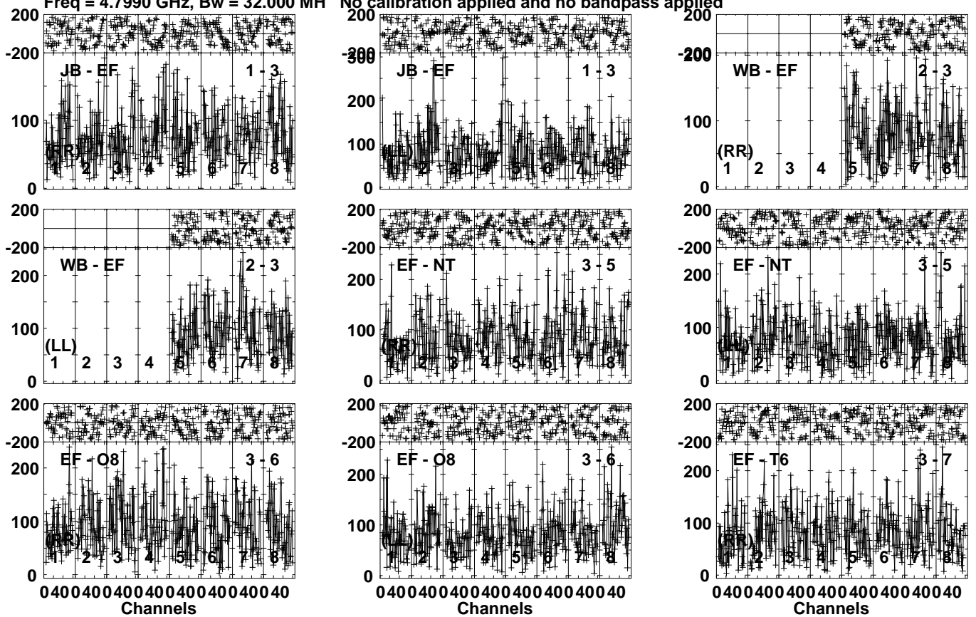
Lower frame: Micro Ampl Jy Top frame: Phas deg Vector averaged cross-power spectrum Several baselines displayed Timerange: 00/21:59:31 to 00/22:02:59
