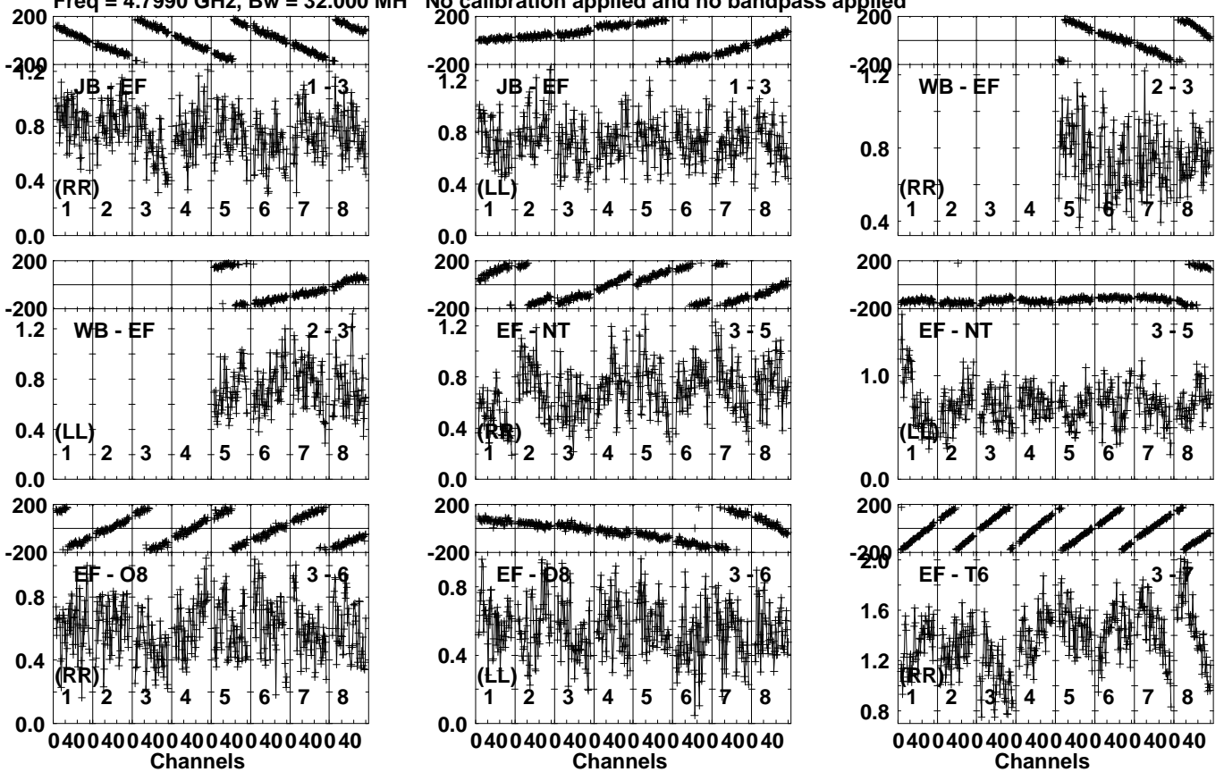
Lower frame: Milli Ampl Jy Top frame: Phas deg Vector averaged cross-power spectrum Several baselines displayed Timerange: 01/04:08:01 to 01/04:09:29
