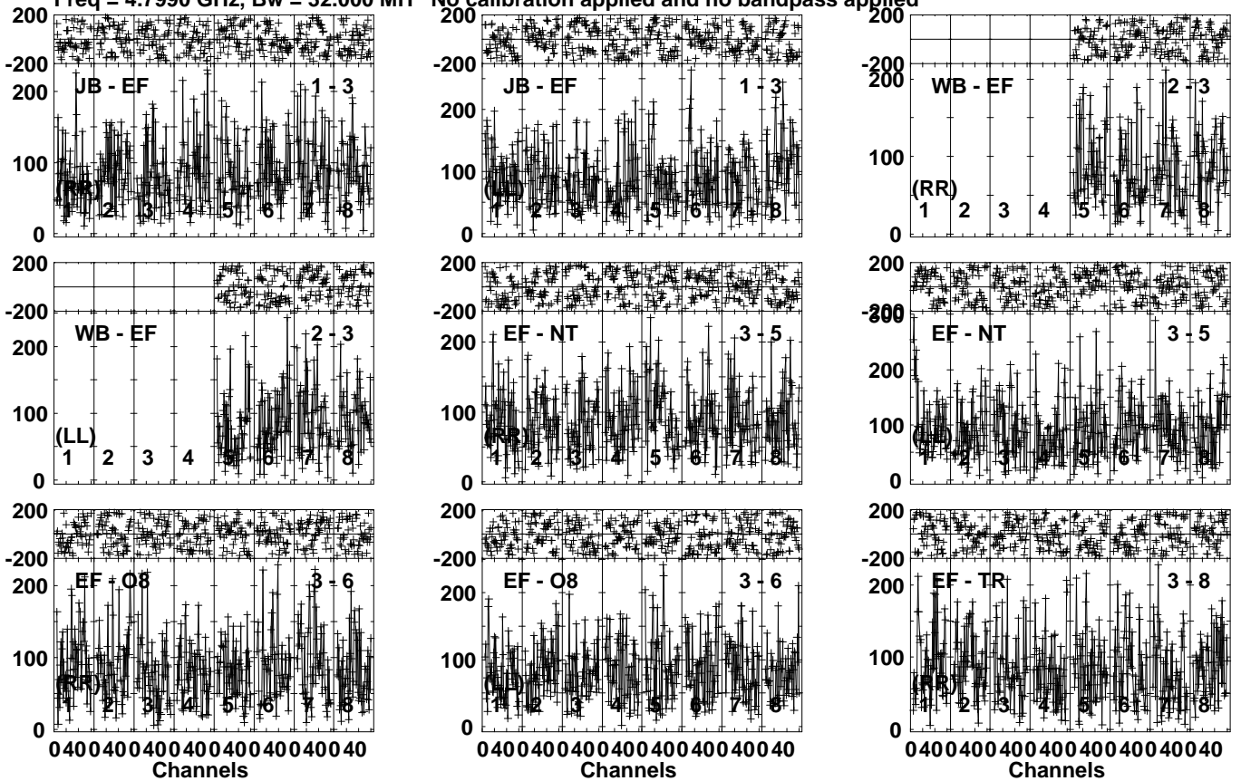
Lower frame: Micro Ampl Jy Top frame: Phas deg Vector averaged cross-power spectrum Several baselines displayed Timerange: 00/23:24:31 to 00/23:27:59
