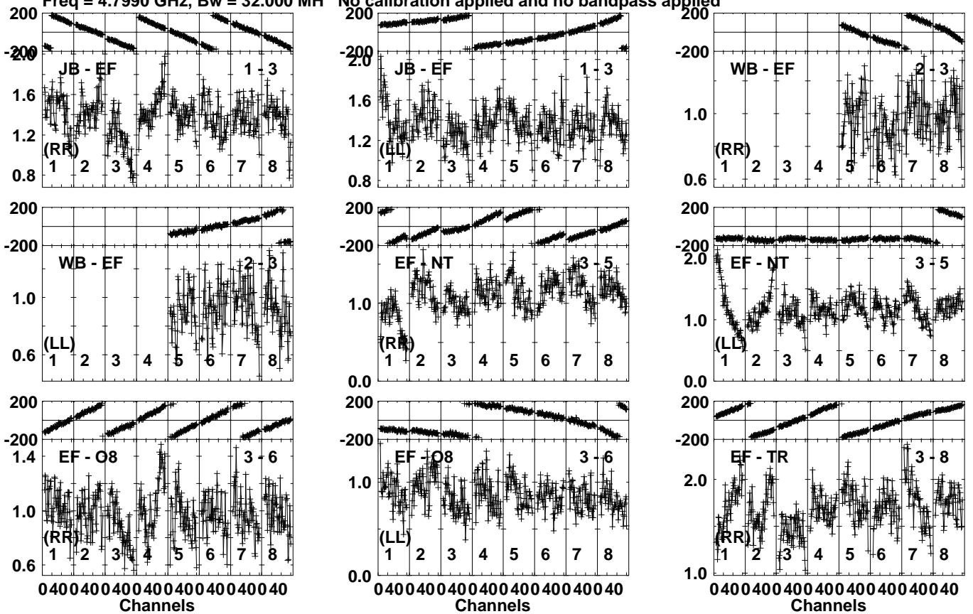
Lower frame: Milli Ampl Jy Top frame: Phas deg Vector averaged cross-power spectrum Several baselines displayed Timerange: 01/01:42:01 to 01/01:42:59
