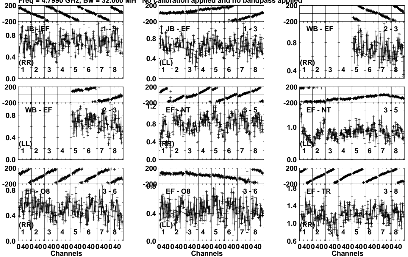
Lower frame: Milli Ampl Jy Top frame: Phas deg Vector averaged cross-power spectrum Several baselines displayed Timerange: 01/09:28:01 to 01/09:29:29
