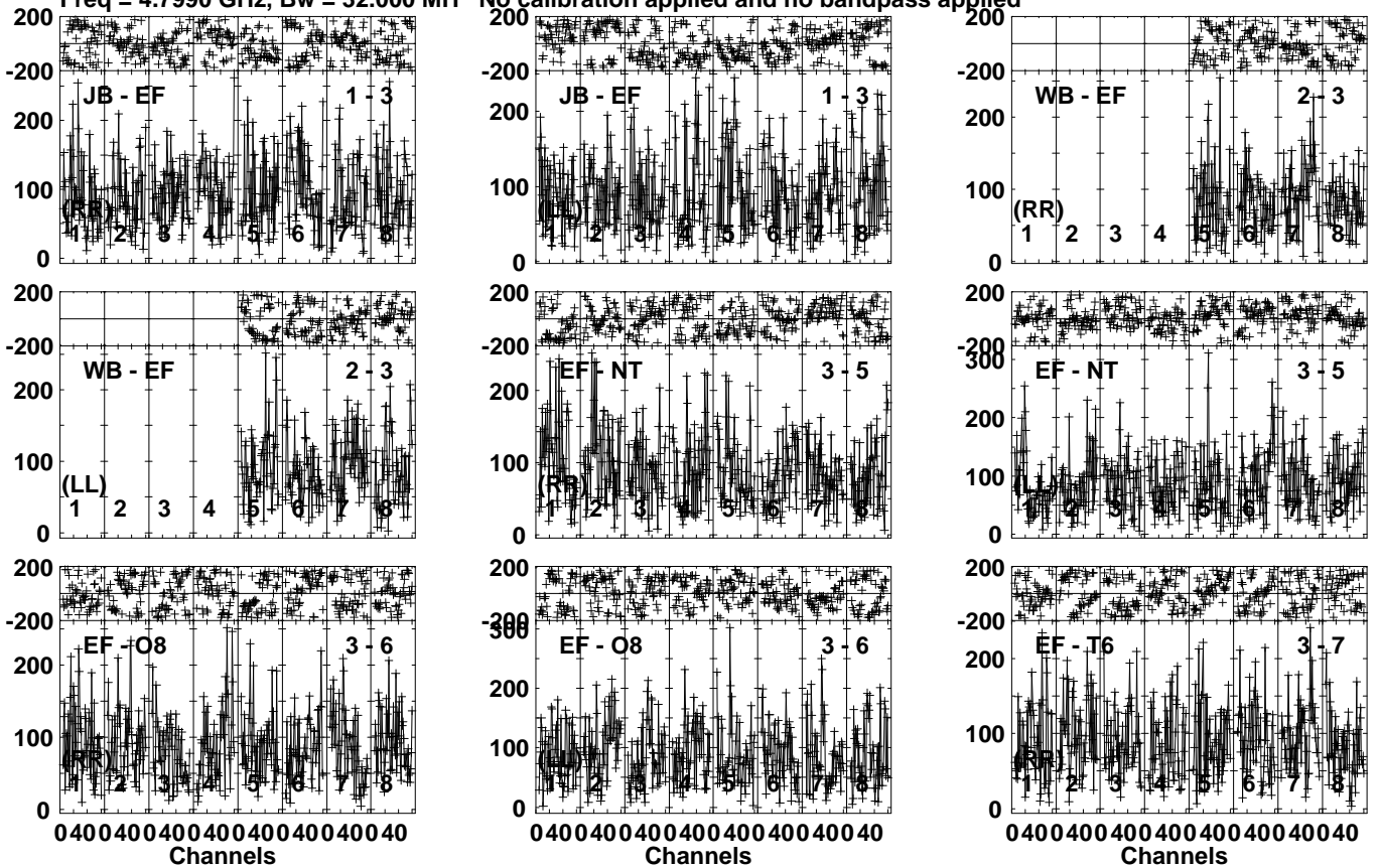
Lower frame: Micro Ampl Jy Top frame: Phas deg Vector averaged cross-power spectrum Several baselines displayed Timerange: 01/05:24:31 to 01/05:27:59
