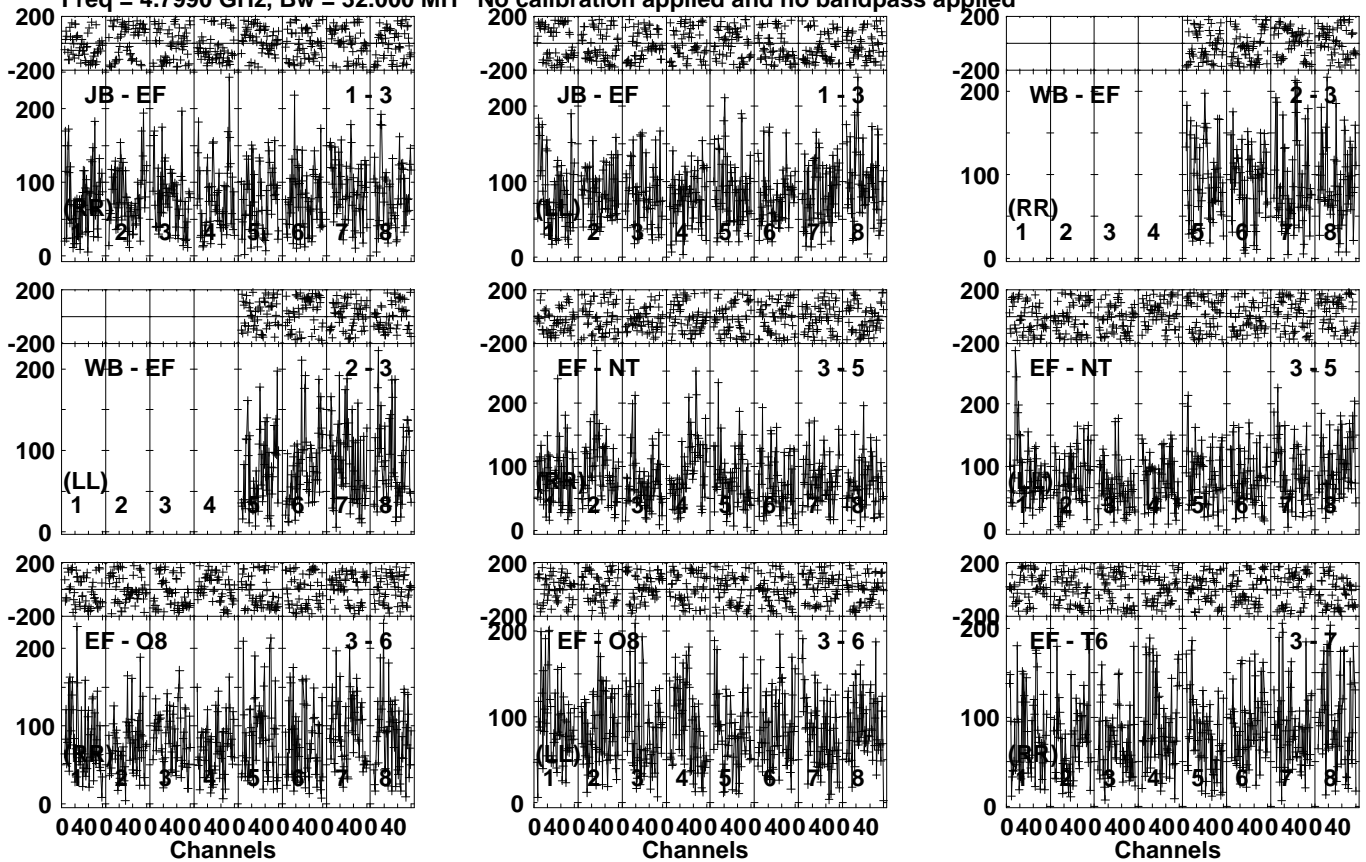
Lower frame: Micro Ampl Jy Top frame: Phas deg Vector averaged cross-power spectrum Several baselines displayed Timerange: 00/21:39:31 to 00/21:42:59
