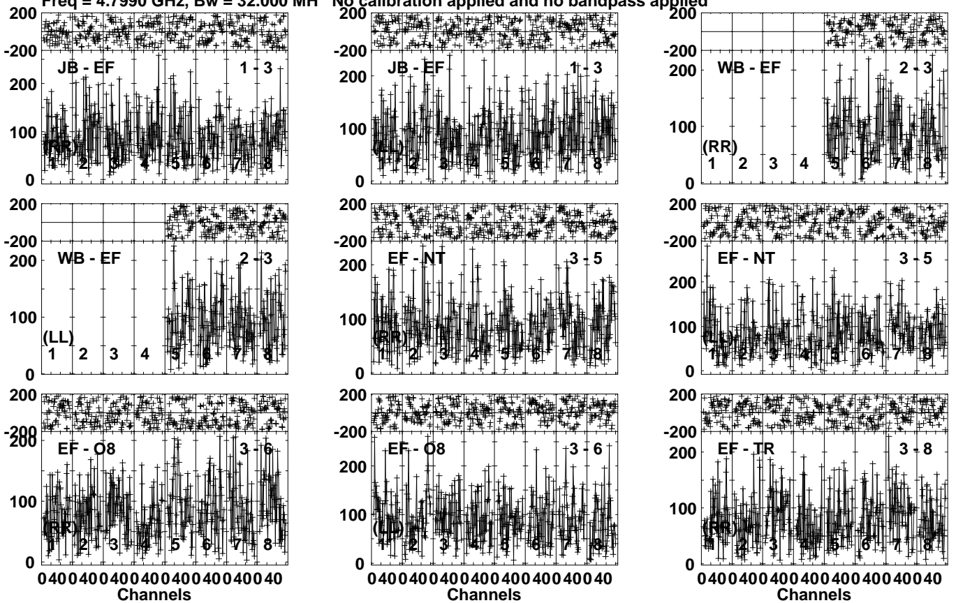
Lower frame: Micro Ampl Jy Top frame: Phas deg Vector averaged cross-power spectrum Several baselines displayed Timerange: 00/22:44:31 to 00/22:47:59
