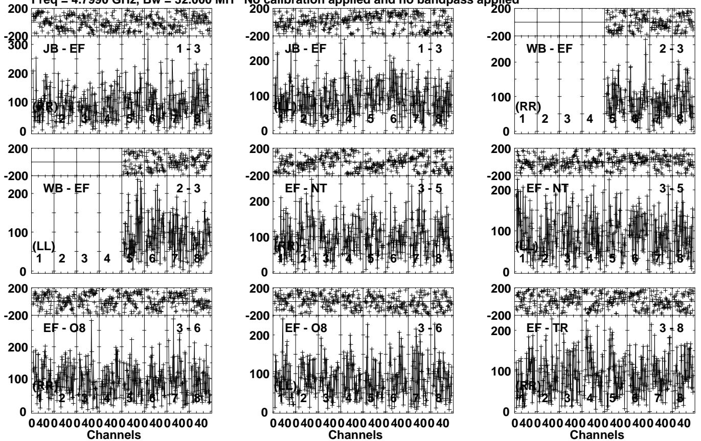
Lower frame: Micro Ampl Jy Top frame: Phas deg Vector averaged cross-power spectrum Several baselines displayed Timerange: 01/08:04:31 to 01/08:07:59
