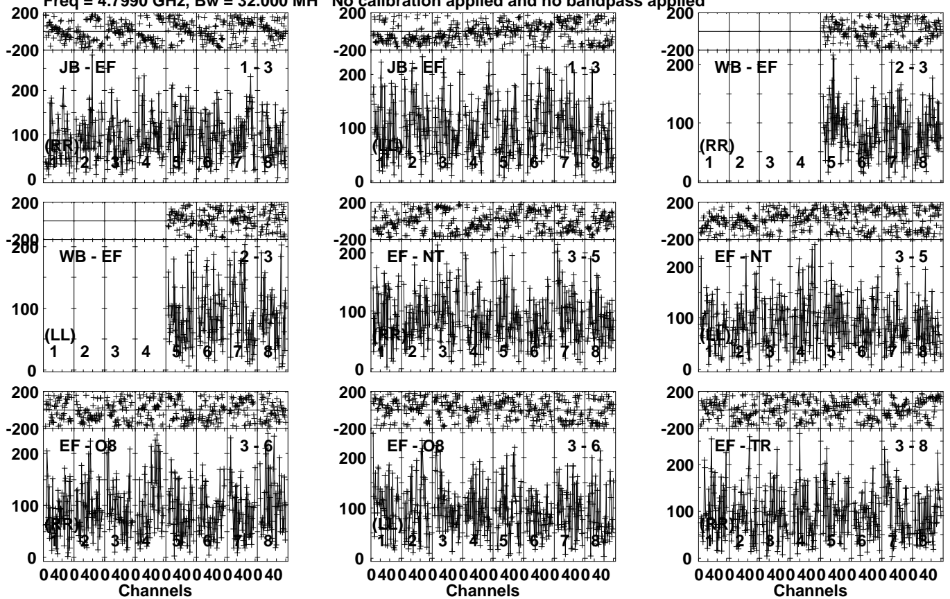
Lower frame: Micro Ampl Jy Top frame: Phas deg Vector averaged cross-power spectrum Several baselines displayed Timerange: 01/09:49:31 to 01/09:52:59
