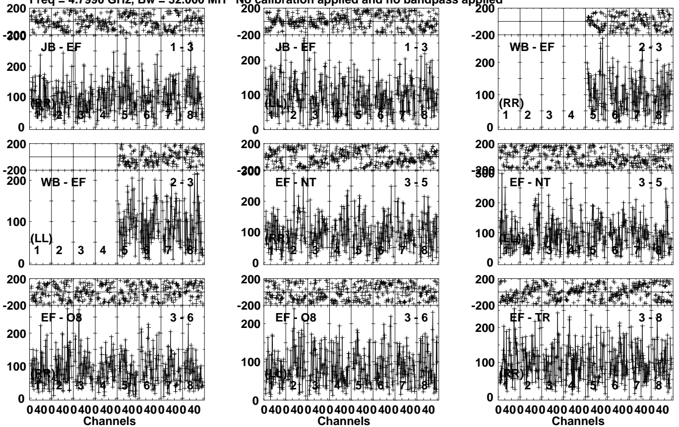
Lower frame: Micro Ampl Jy Top frame: Phas deg Vector averaged cross-power spectrum Several baselines displayed Timerange: 01/07:49:31 to 01/07:52:59
