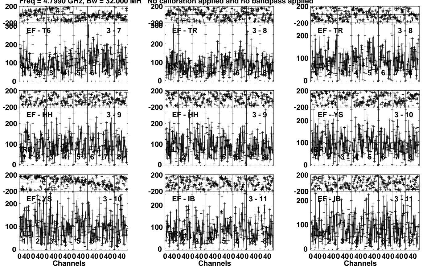
Lower frame: Micro Ampl Jy Top frame: Phas deg Vector averaged cross-power spectrum Several baselines displayed Timerange: 01/05:49:31 to 01/05:52:59
