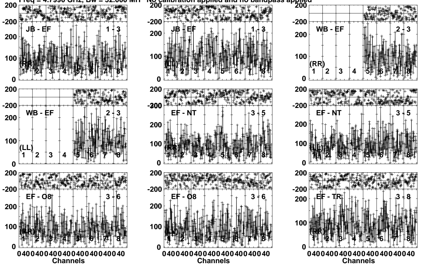
Lower frame: Micro Ampl Jy Top frame: Phas deg Vector averaged cross-power spectrum Several baselines displayed Timerange: 01/08:19:31 to 01/08:22:59
