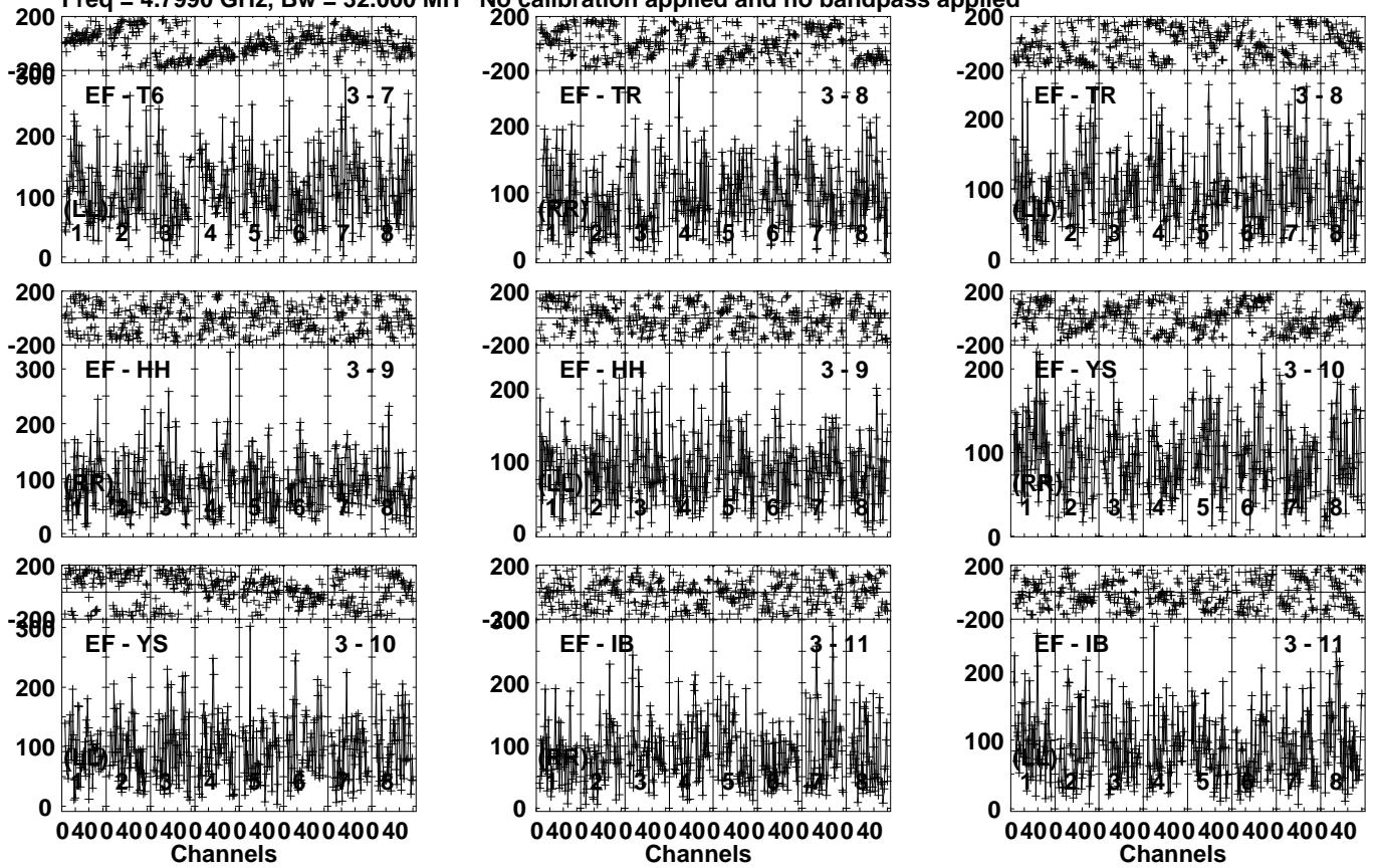
Lower frame: Micro Ampl Jy Top frame: Phas deg Vector averaged cross-power spectrum Several baselines displayed Timerange: 01/05:54:31 to 01/05:57:59
