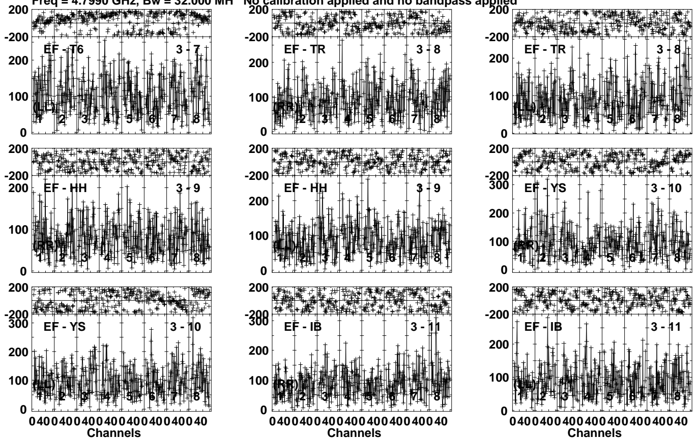
Lower frame: Micro Ampl Jy Top frame: Phas deg Vector averaged cross-power spectrum Several baselines displayed Timerange: 01/04:44:31 to 01/04:47:59
