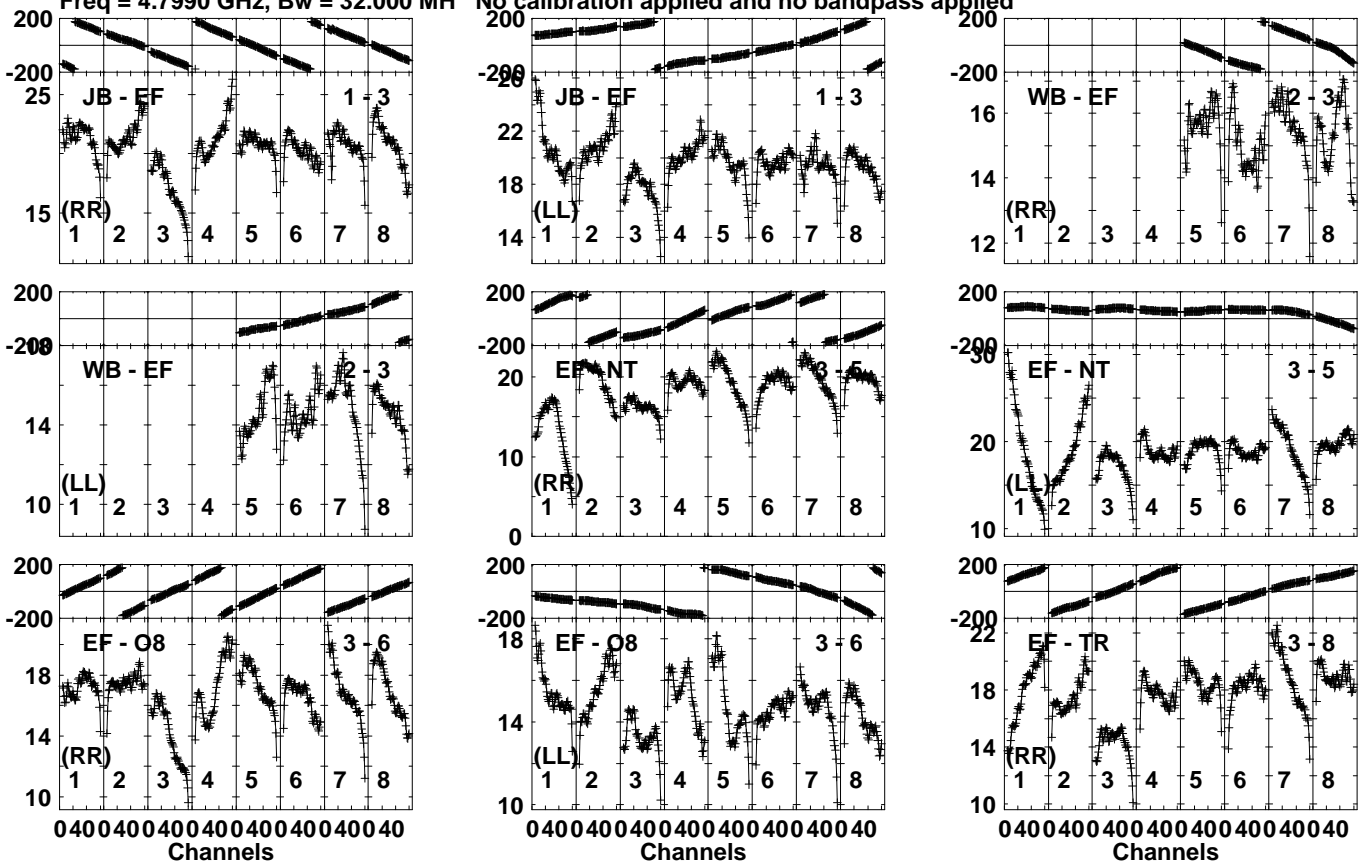
Lower frame: Milli Ampl Jy Top frame: Phas deg Vector averaged cross-power spectrum Several baselines displayed Timerange: 01/00:11:31 to 01/00:14:29
