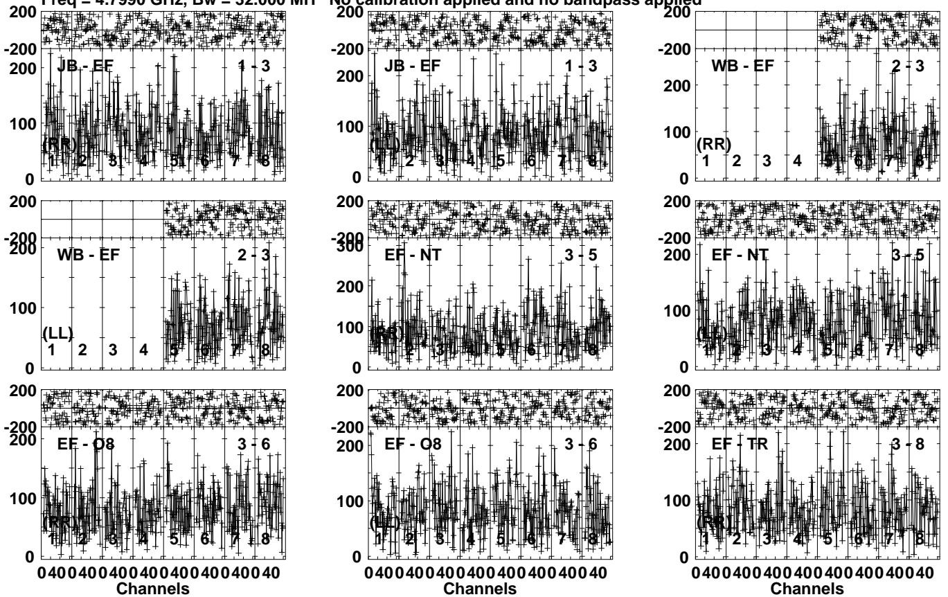
Lower frame: Micro Ampl Jy Top frame: Phas deg Vector averaged cross-power spectrum Several baselines displayed Timerange: 00/23:49:31 to 00/23:52:59
