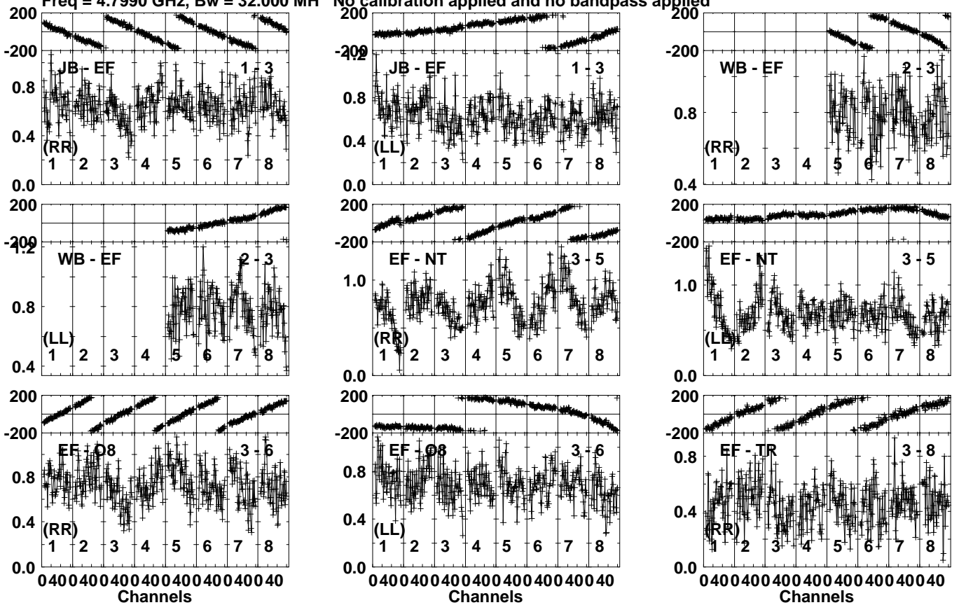
Lower frame: Milli Ampl Jy Top frame: Phas deg Vector averaged cross-power spectrum Several baselines displayed Timerange: 01/06:43:31 to 01/06:44:29
