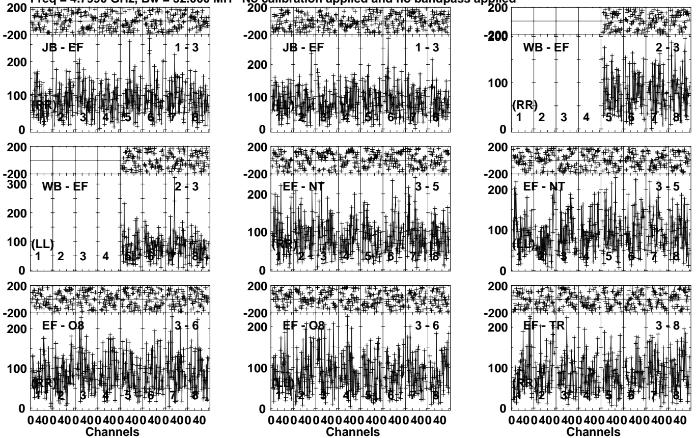
Lower frame: Micro Ampl Jy Top frame: Phas deg Vector averaged cross-power spectrum Several baselines displayed Timerange: 00/23:09:31 to 00/23:12:59
