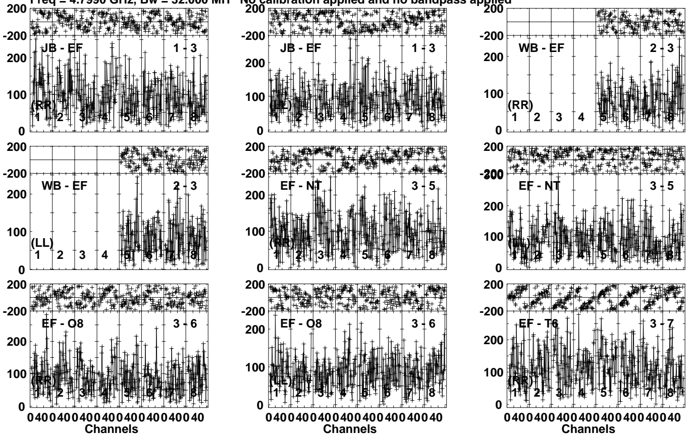
Lower frame: Micro Ampl Jy Top frame: Phas deg Vector averaged cross-power spectrum Several baselines displayed Timerange: 01/04:34:31 to 01/04:37:59
