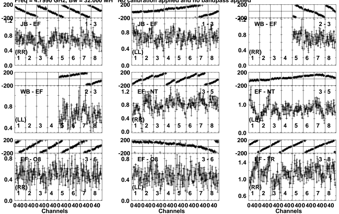
Lower frame: Milli Ampl Jy Top frame: Phas deg Vector averaged cross-power spectrum Several baselines displayed Timerange: 01/09:23:31 to 01/09:24:29
