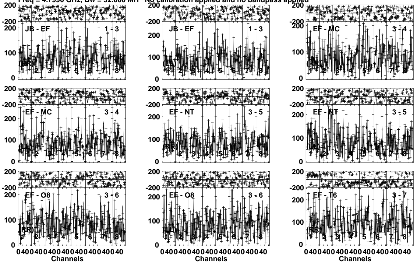
Lower frame: Micro Ampl Jy Top frame: Phas deg Vector averaged cross-power spectrum Several baselines displayed Timerange: 00/13:09:01 to 00/13:12:29
