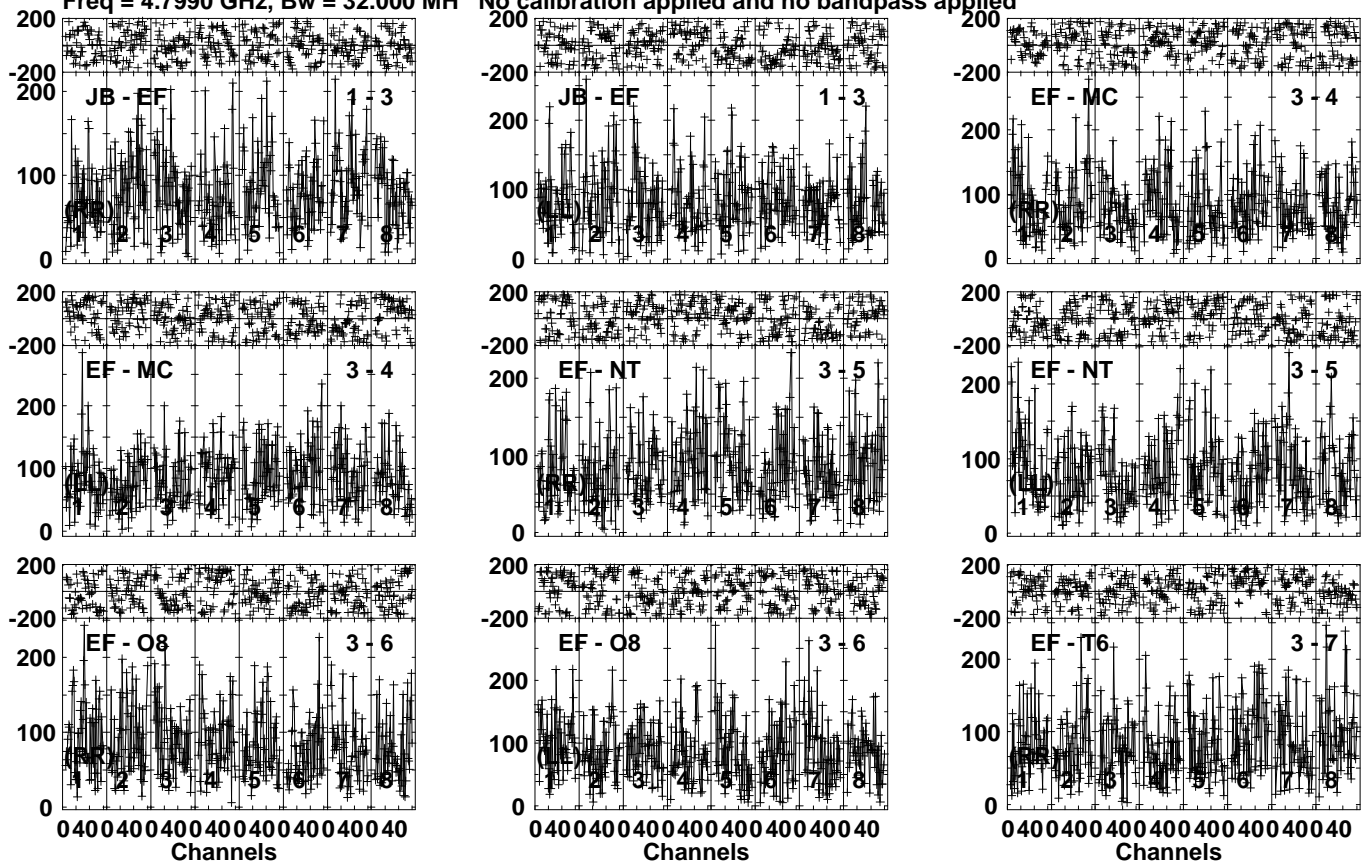
Lower frame: Micro Ampl Jy Top frame: Phas deg Vector averaged cross-power spectrum Several baselines displayed Timerange: 00/14:14:01 to 00/14:17:29
