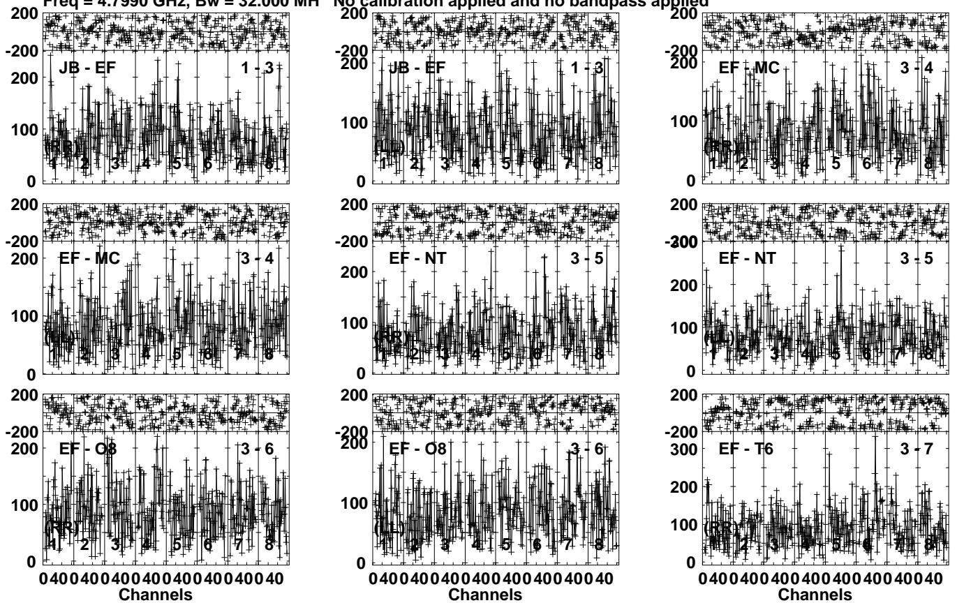
Lower frame: Micro Ampl Jy Top frame: Phas deg Vector averaged cross-power spectrum Several baselines displayed Timerange: 00/13:59:01 to 00/14:02:29
