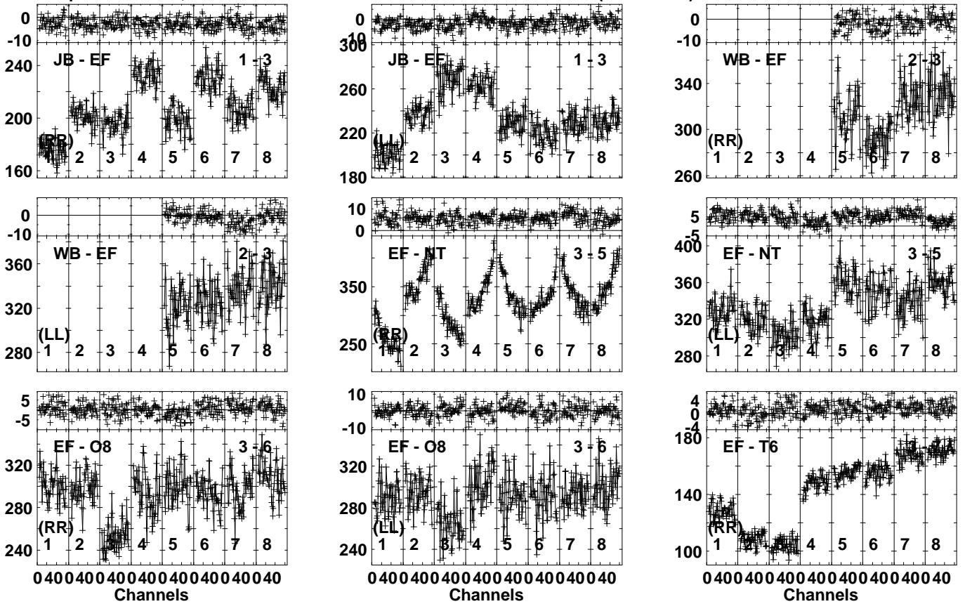
Lower frame: Milli Ampl Jy Top frame: Phas deg Vector averaged cross-power spectrum Several baselines displayed Timerange: 00:15:07:01 to 00:15:07:59
