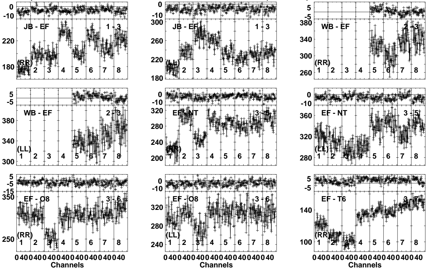
Lower frame: Milli Ampl Jy Top frame: Phas deg Vector averaged cross-power spectrum Several baselines displayed Timerange: 00/17:27:21 to 00/17:28:49
