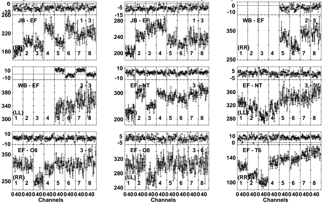
Lower frame: Milli Ampl Jy Top frame: Phas deg Vector averaged cross-power spectrum Several baselines displayed Timerange: 00:17:42:51 to 00:17:43:49
