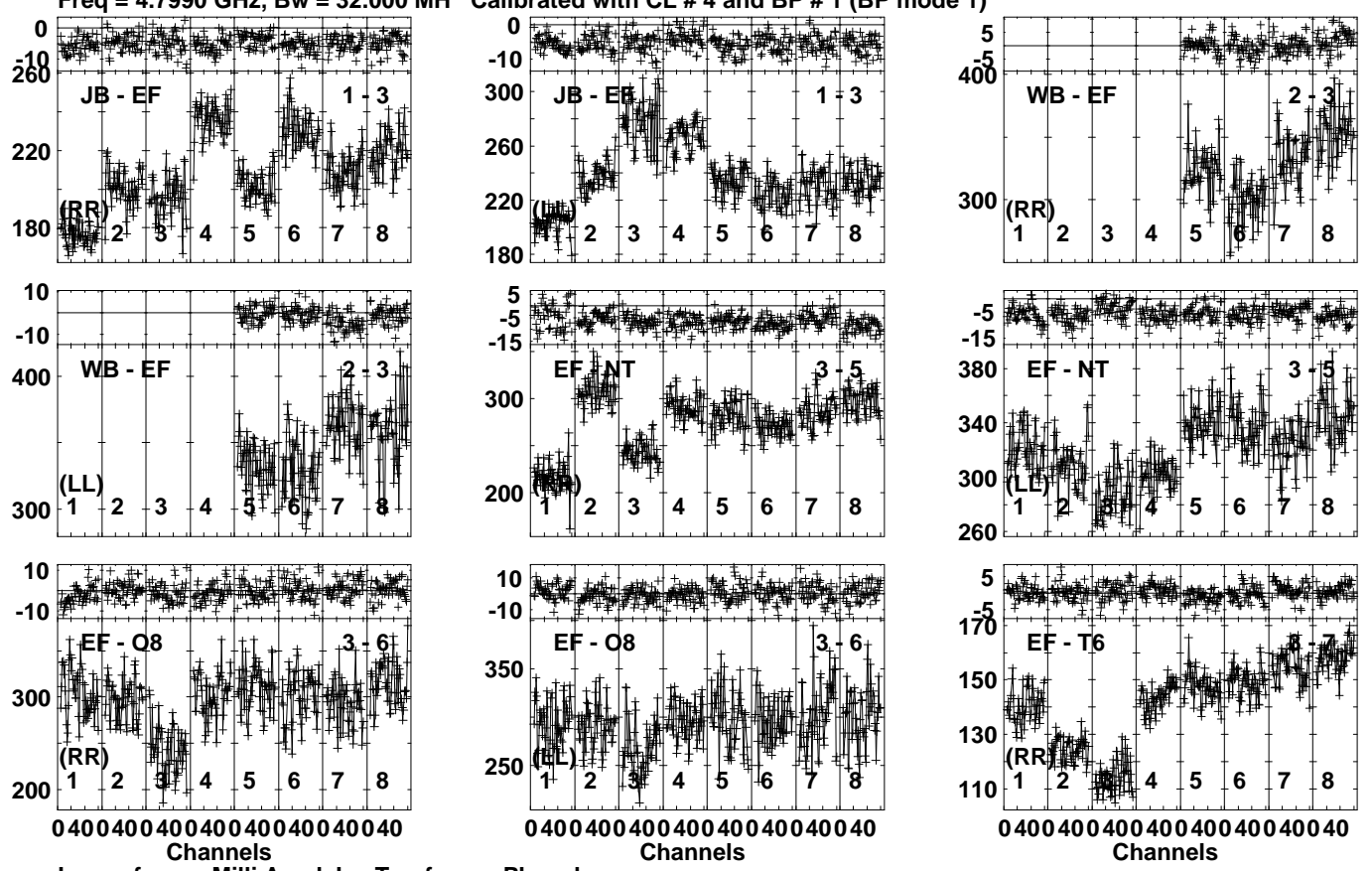
Lower frame: Milli Ampl Jy Top frame: Phas deg Vector averaged cross-power spectrum Several baselines displayed Timerange: 00/18:22:51 to 00/18:23:49
