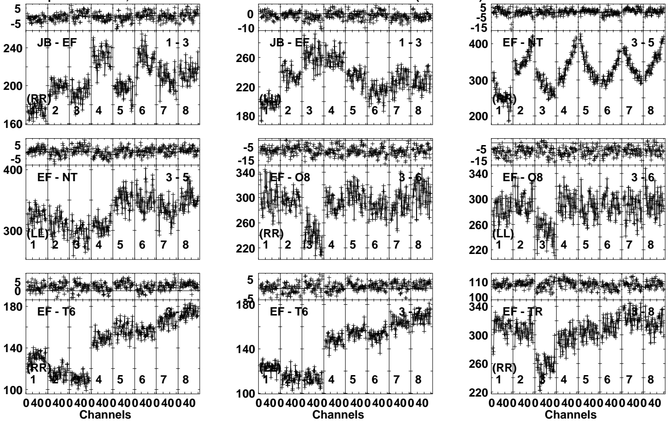
Lower frame: Milli Ampl Jy Top frame: Phas deg Vector averaged cross-power spectrum Several baselines displayed Timerange: 00/14:41:31 to 00/14:42:59
