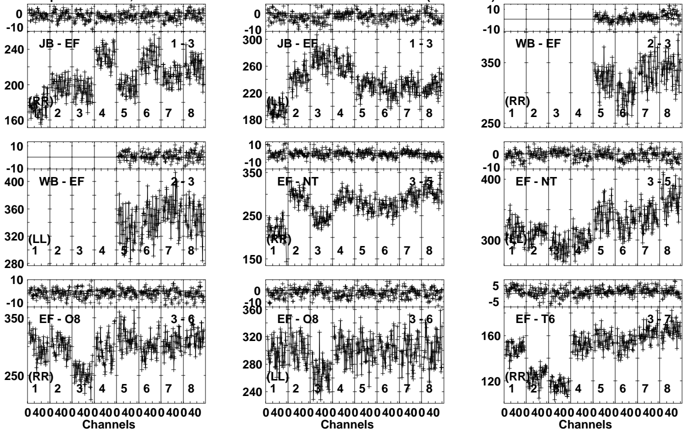
Lower frame: Milli Ampl Jy Top frame: Phas deg Vector averaged cross-power spectrum Several baselines displayed Timerange: 00/18:32:51 to 00/18:33:49
