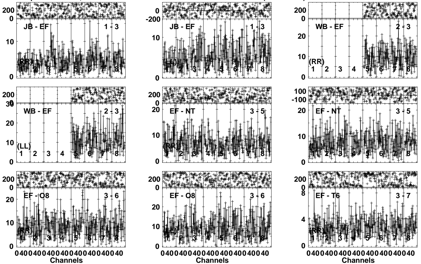
Lower frame: Milli Ampl Jy Top frame: Phas deg Vector averaged cross-power spectrum Several baselines displayed Timerange: 00/17:48:51 to 00/17:52:19
