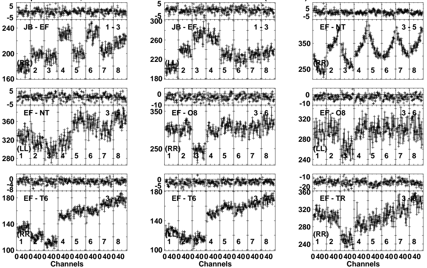
Lower frame: Milli Ampl Jy Top frame: Phas deg Vector averaged cross-power spectrum Several baselines displayed Timerange: 00/14:27:01 to 00/14:27:59
