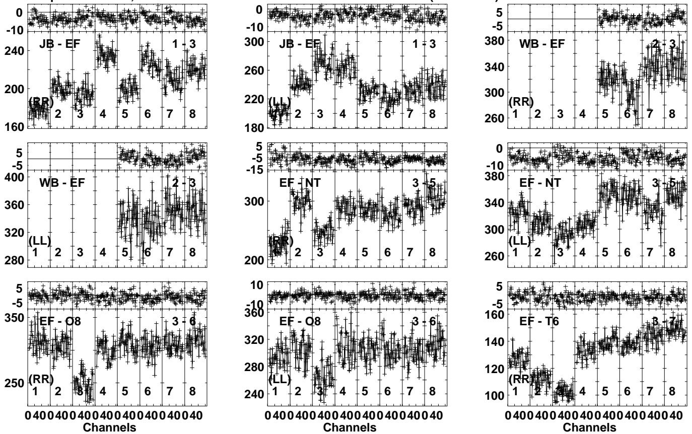
Lower frame: Milli Ampl Jy Top frame: Phas deg Vector averaged cross-power spectrum Several baselines displayed Timerange: 00/17:52:51 to 00/17:53:49
