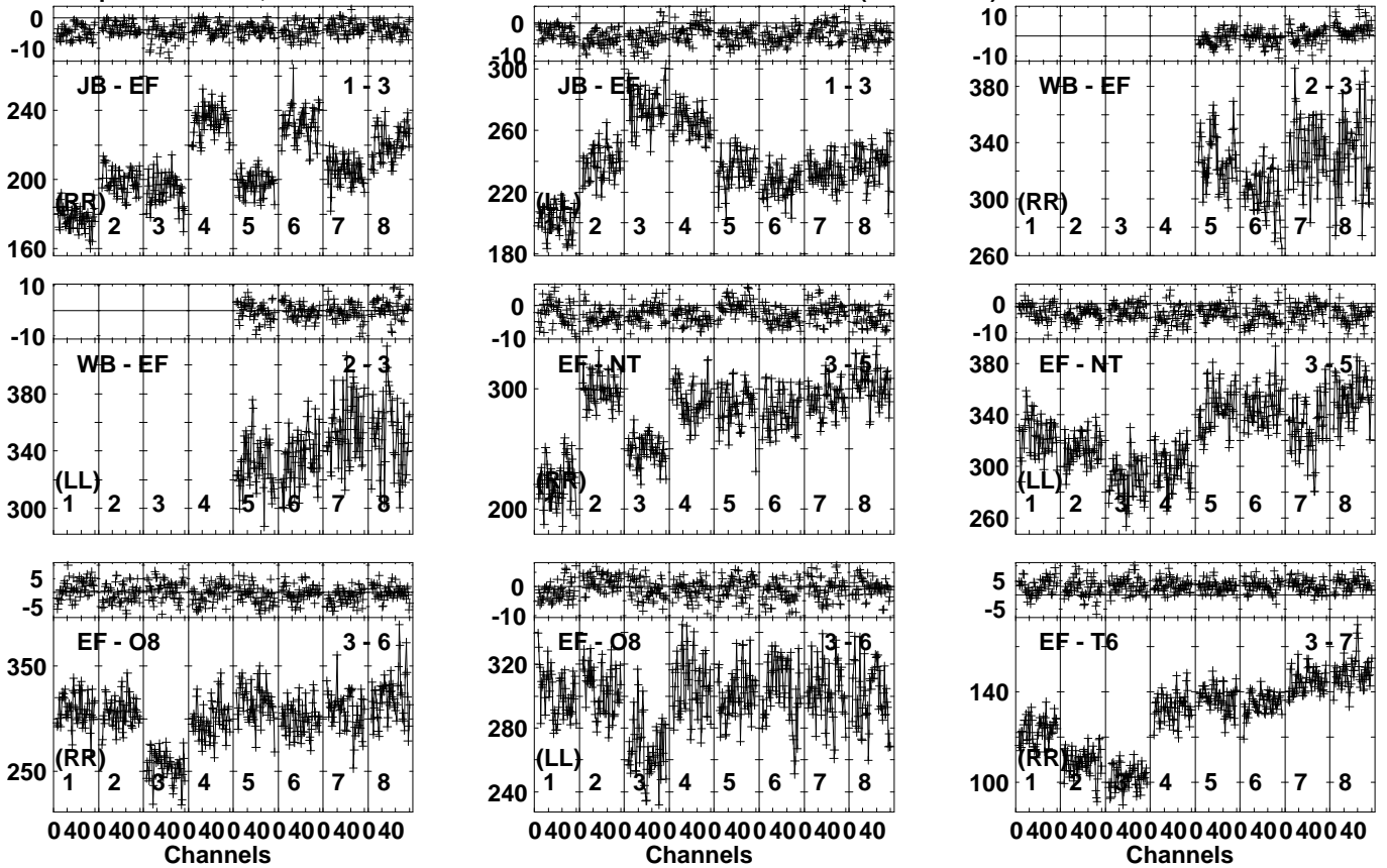
Lower frame: Milli Ampl Jy Top frame: Phas deg Vector averaged cross-power spectrum Several baselines displayed Timerange: 00:17:32:51 to 00:17:33:49
