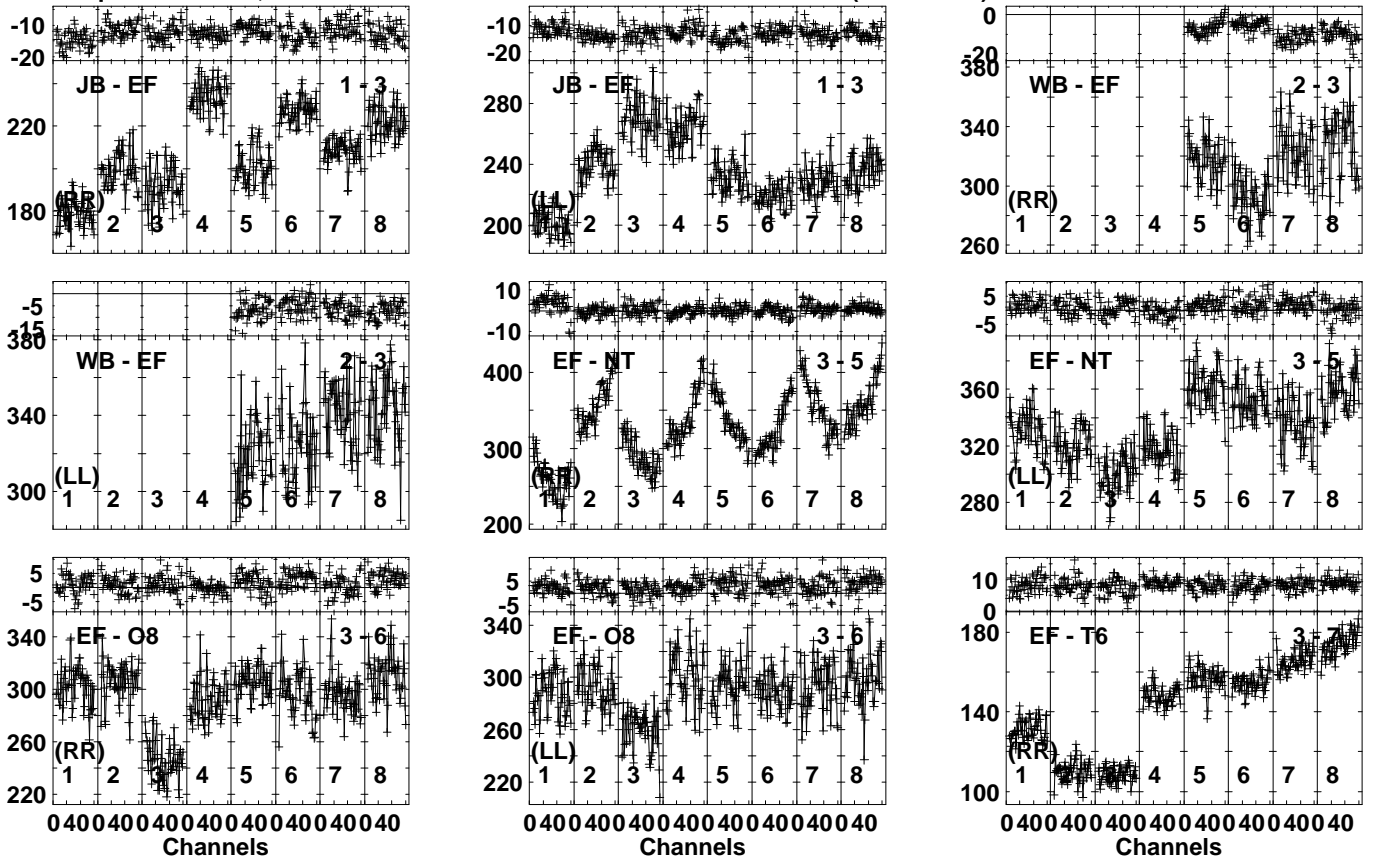
Lower frame: Milli Ampl Jy Top frame: Phas deg Vector averaged cross-power spectrum Several baselines displayed Timerange: 00/15:01:31 to 00/15:02:59
