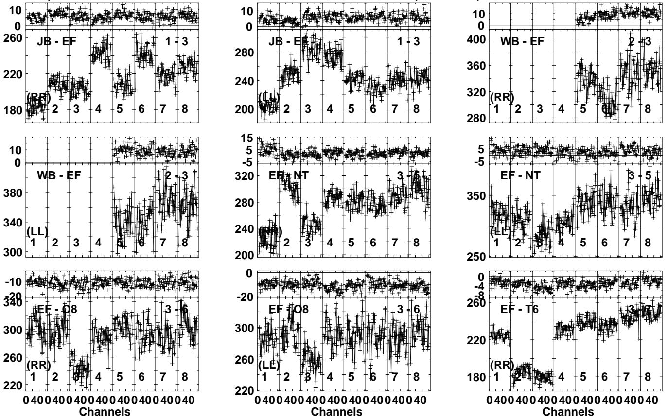
Lower frame: Milli Ampl Jy Top frame: Phas deg Vector averaged cross-power spectrum Several baselines displayed Timerange: 00/19:37:21 to 00/19:38:49
