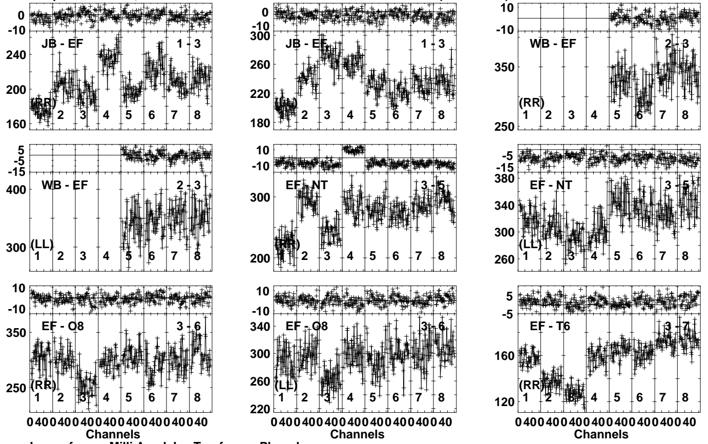
Lower frame: Milli Ampl Jy Top frame: Phas deg Vector averaged cross-power spectrum Several baselines displayed Timerange: 00/18:42:51 to 00/18:43:49
