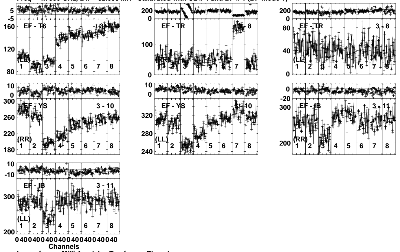
Lower frame: Milli Ampl Jy Top frame: Phas deg Vector averaged cross-power spectrum Several baselines displayed Timerange: 00/16:31:31 to 00/16:32:59
