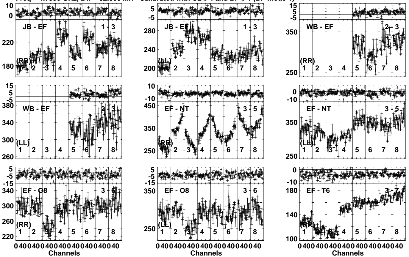
Lower frame: Milli Ampl Jy Top frame: Phas deg Vector averaged cross-power spectrum Several baselines displayed Timerange: 00/14:47:01 to 00/14:47:59
