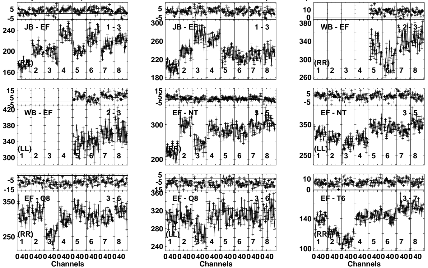
Lower frame: Milli Ampl Jy Top frame: Phas deg Vector averaged cross-power spectrum Several baselines displayed Timerange: 00/18:17:21 to 00/18:18:49
