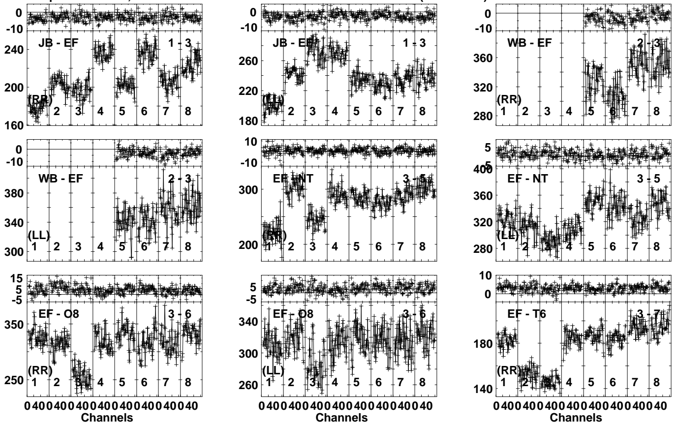
Lower frame: Milli Ampl Jy Top frame: Phas deg Vector averaged cross-power spectrum Several baselines displayed Timerange: 00:19:02:51 to 00:19:03:49
