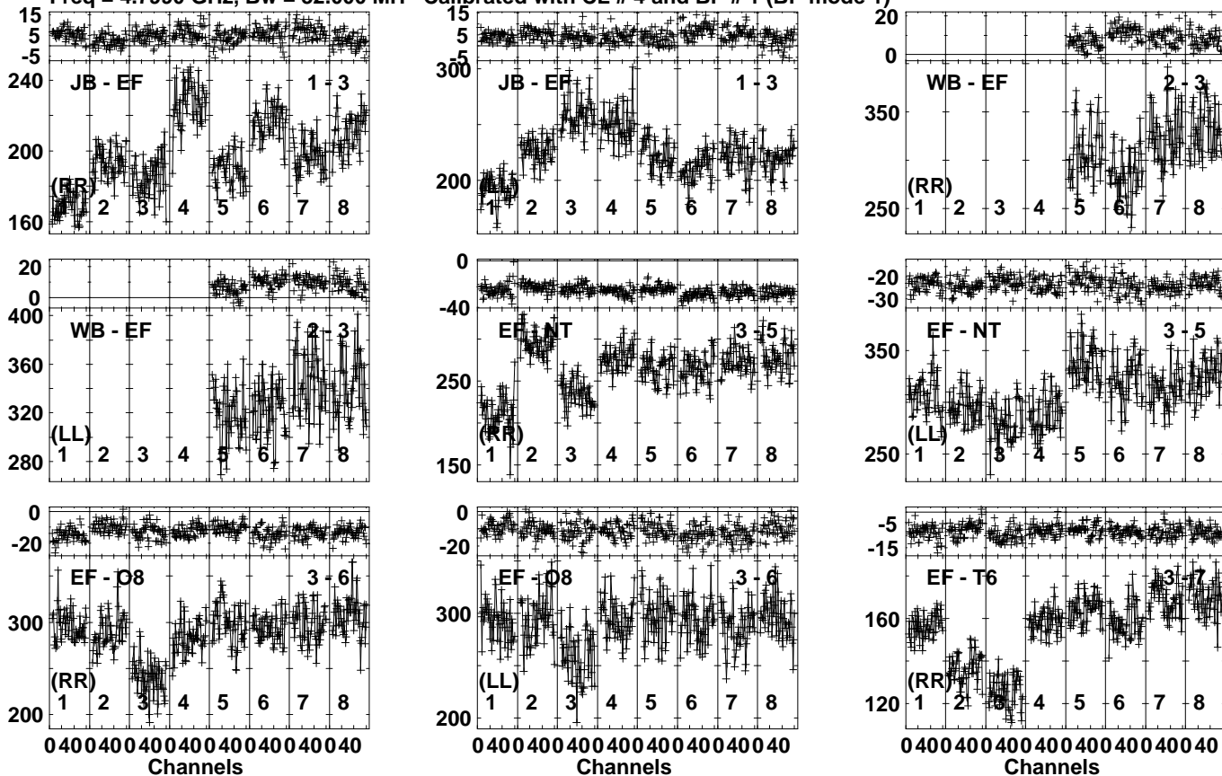
Lower frame: Milli Ampl Jy Top frame: Phas deg Vector averaged cross-power spectrum Several baselines displayed Timerange: 00/18:47:21 to 00/18:48:49
