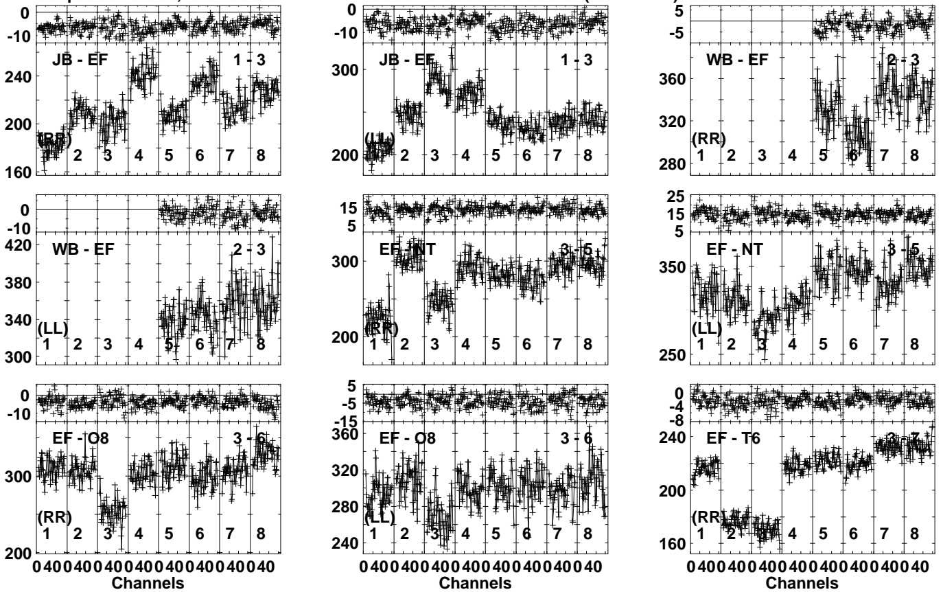
Lower frame: Milli Ampl Jy Top frame: Phas deg Vector averaged cross-power spectrum Several baselines displayed Timerange: 00/19:27:21 to 00/19:28:49
