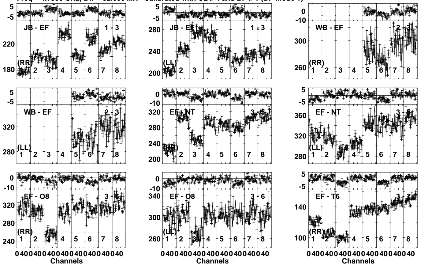
Lower frame: Milli Ampl Jy Top frame: Phas deg Vector averaged cross-power spectrum Several baselines displayed Timerange: 00/17:22:51 to 00/17:23:49
