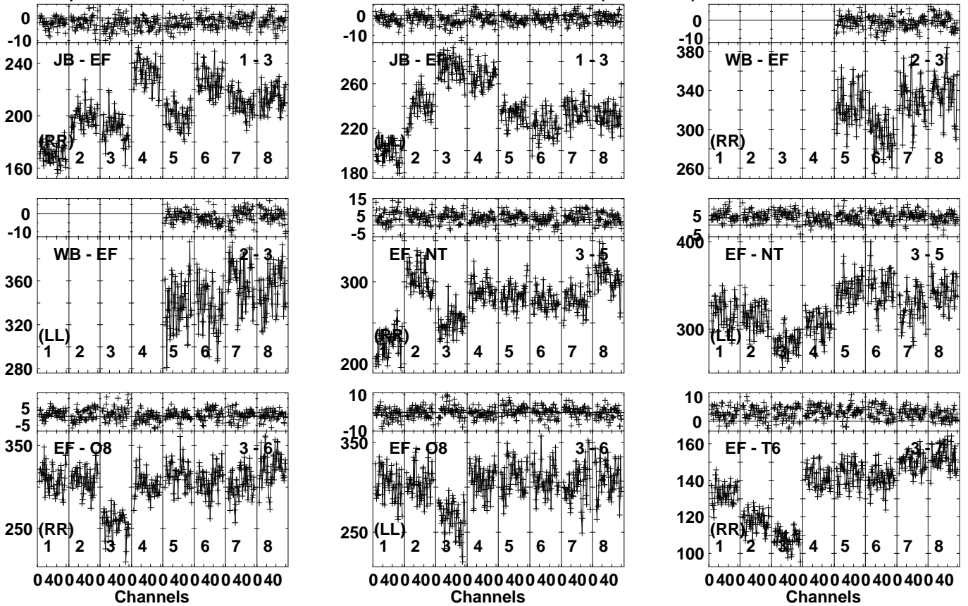
Lower frame: Milli Ampl Jy Top frame: Phas deg Vector averaged cross-power spectrum Several baselines displayed Timerange: 00/18:12:51 to 00/18:13:49
