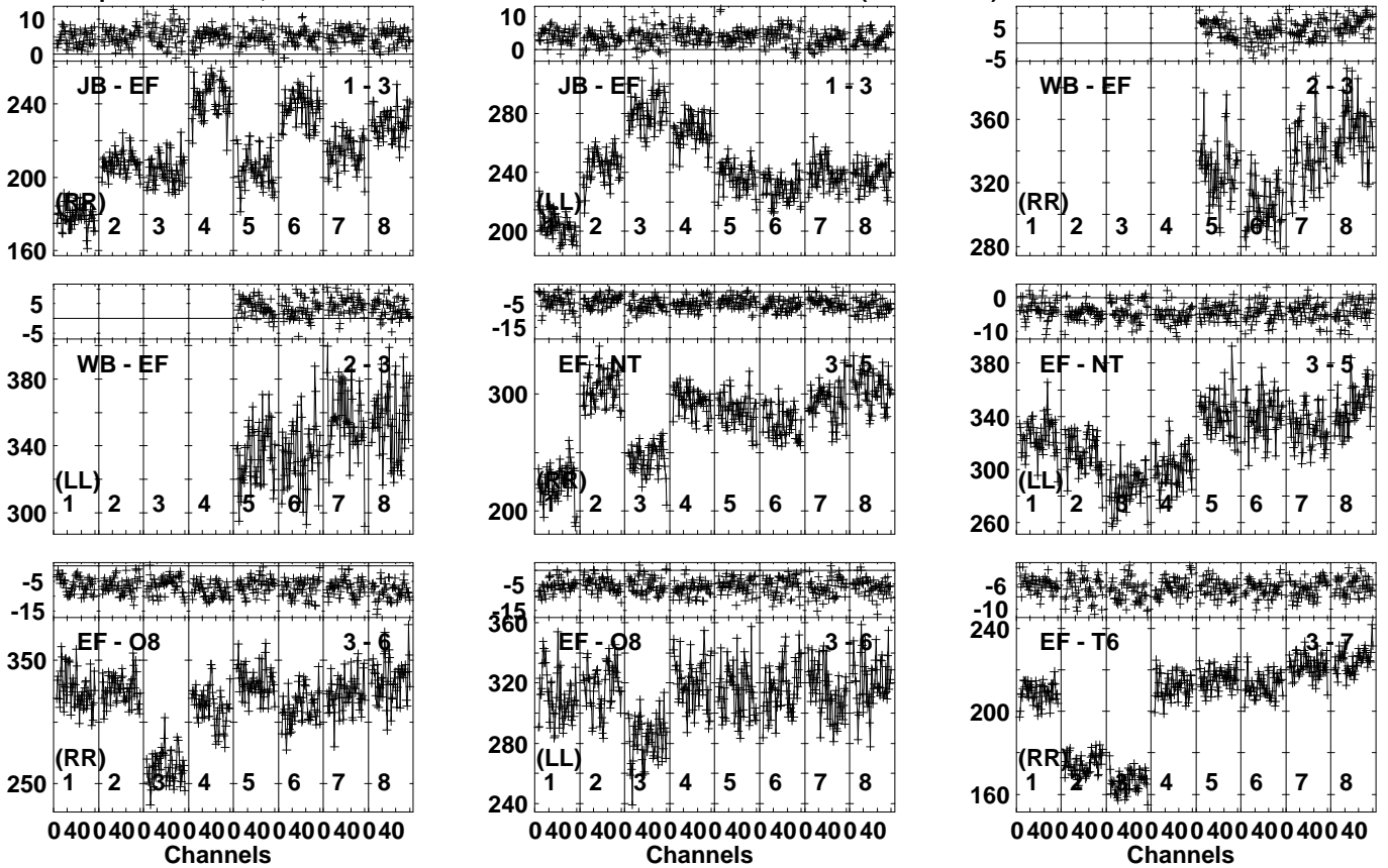
Lower frame: Milli Ampl Jy Top frame: Phas deg Vector averaged cross-power spectrum Several baselines displayed Timerange: 00/19:22:51 to 00/19:23:49
