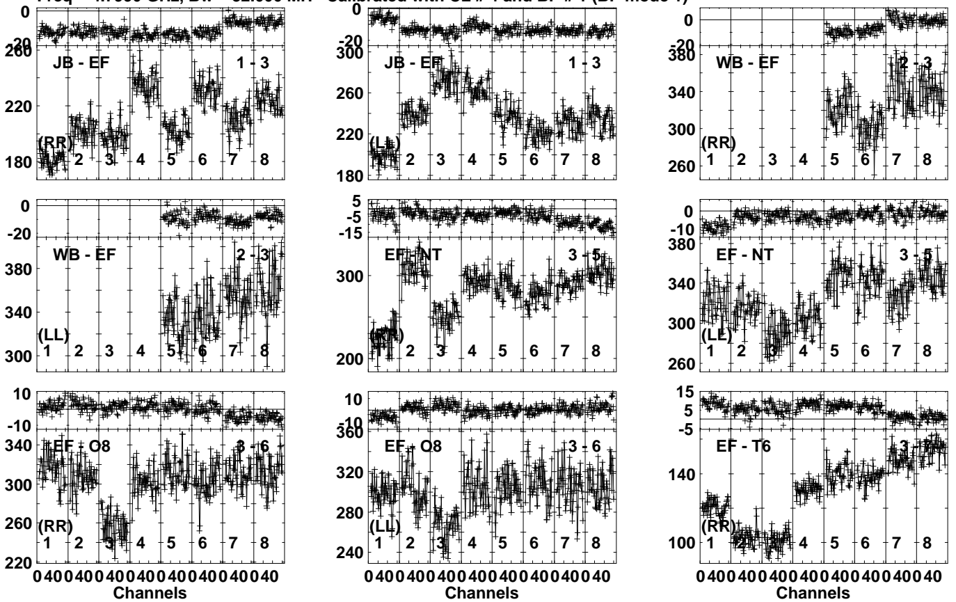
Lower frame: Milli Ampl Jy Top frame: Phas deg Vector averaged cross-power spectrum Several baselines displayed Timerange: 00/17:01:31 to 00/17:02:59
