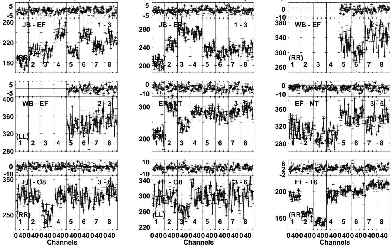
Lower frame: Milli Ampl Jy Top frame: Phas deg Vector averaged cross-power spectrum Several baselines displayed Timerange: 00/19:12:51 to 00/19:13:49
