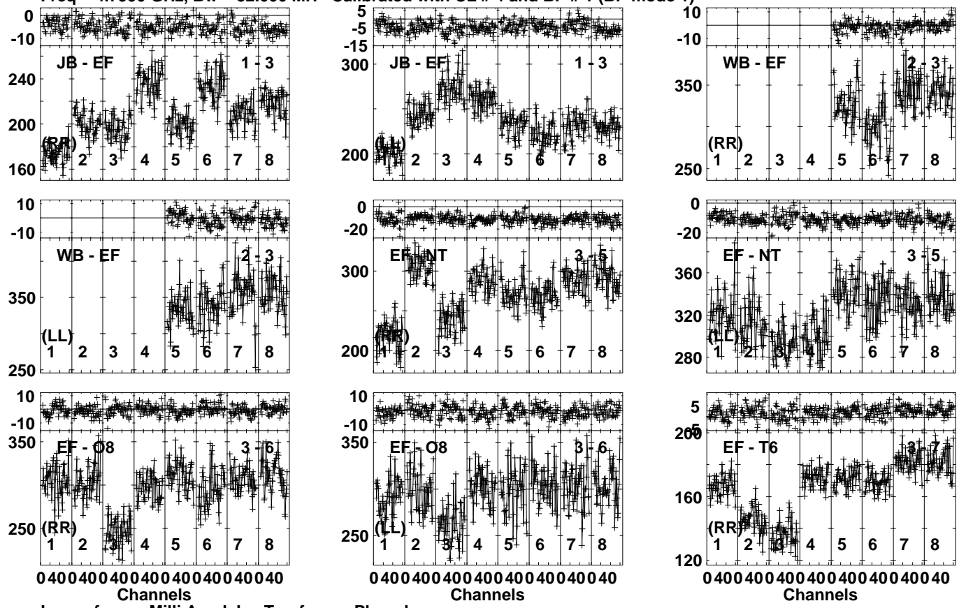
Lower frame: Milli Ampl Jy Top frame: Phas deg Vector averaged cross-power spectrum Several baselines displayed Timerange: 00:18:52:51 to 00:18:53:49
