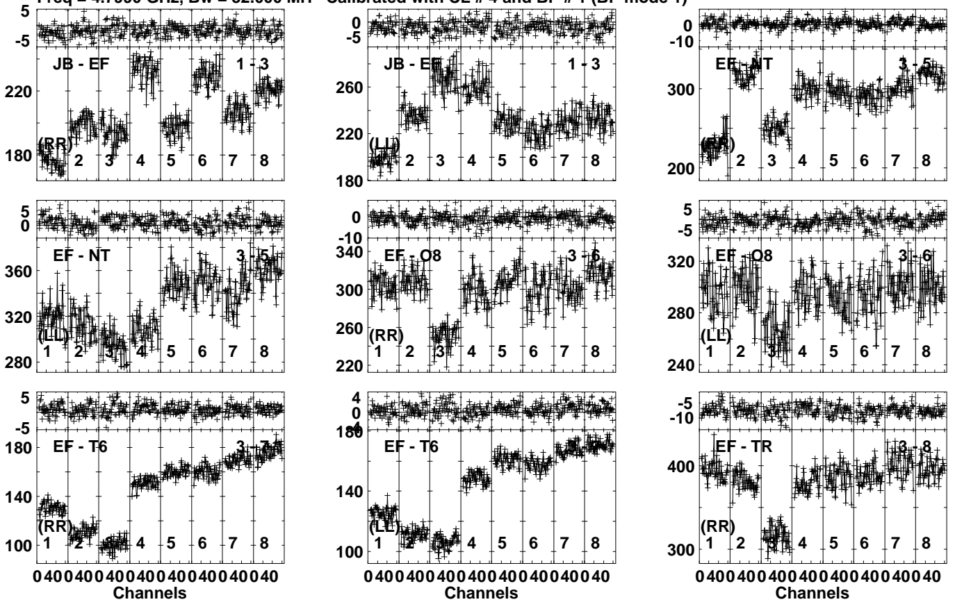
Lower frame: Milli Ampl Jy Top frame: Phas deg Vector averaged cross-power spectrum Several baselines displayed Timerange: 00/14:17:01 to 00/14:17:59
