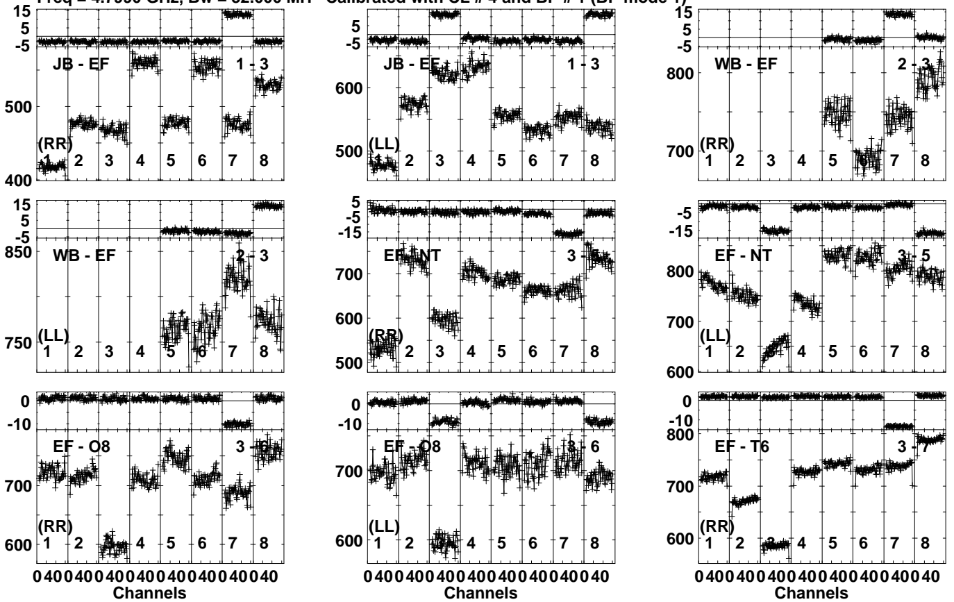
Lower frame: Milli Ampl Jy Top frame: Phas deg Vector averaged cross-power spectrum Several baselines displayed Timerange: 00/19:49:31 to 00/19:52:29
