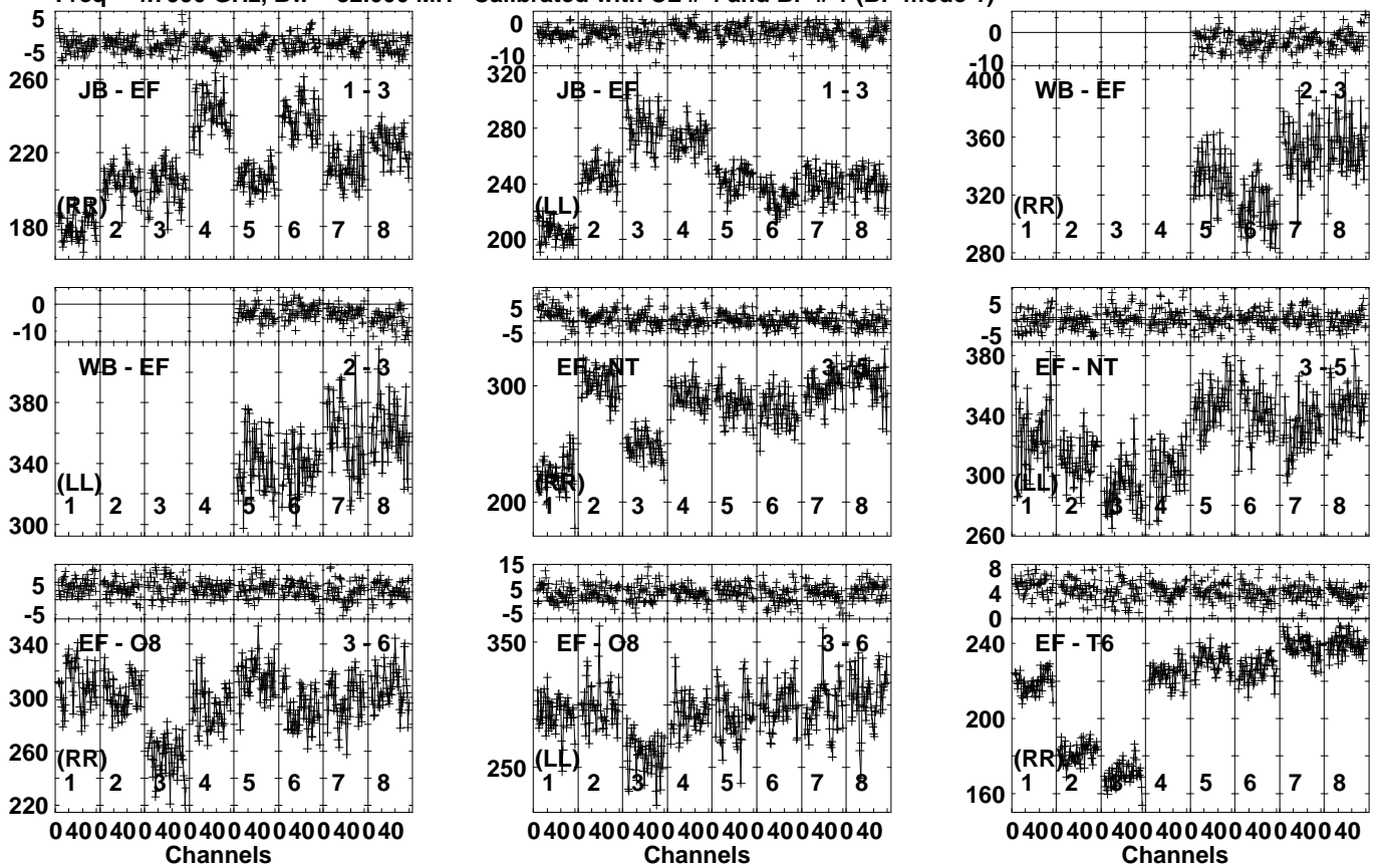
Lower frame: Milli Ampl Jy Top frame: Phas deg Vector averaged cross-power spectrum Several baselines displayed Timerange: 00/19:32:51 to 00/19:33:49
