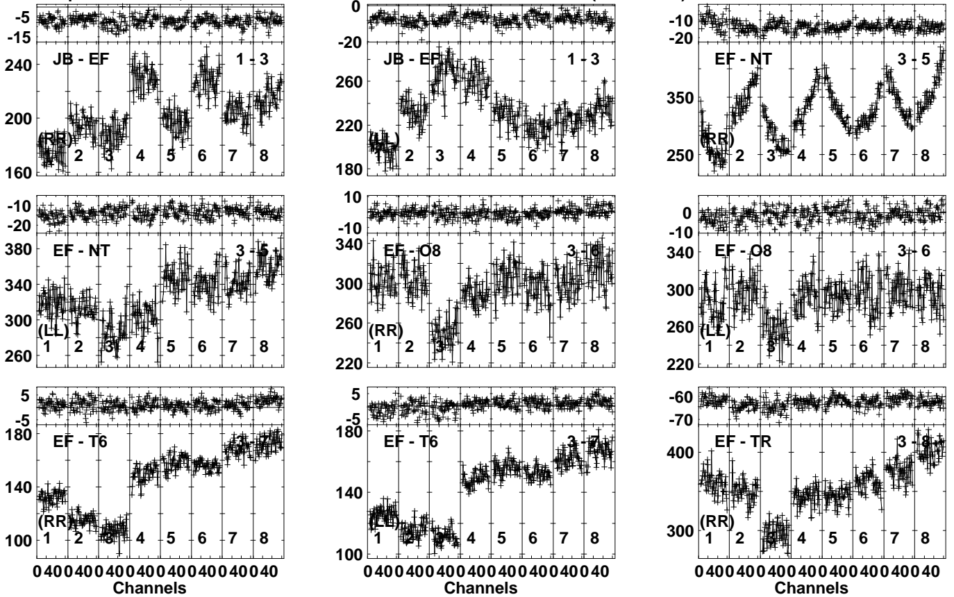
Lower frame: Milli Ampl Jy Top frame: Phas deg Vector averaged cross-power spectrum Several baselines displayed Timerange: 00/14:31:31 to 00/14:32:59
