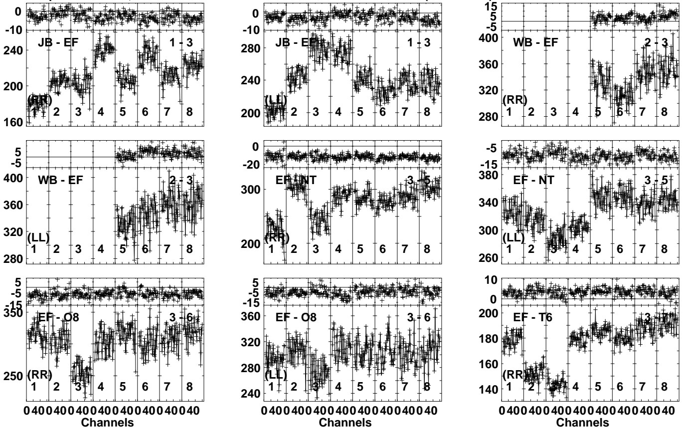
Lower frame: Milli Ampl Jy Top frame: Phas deg Vector averaged cross-power spectrum Several baselines displayed Timerange: 00:18:57:21 to 00:18:58:49
