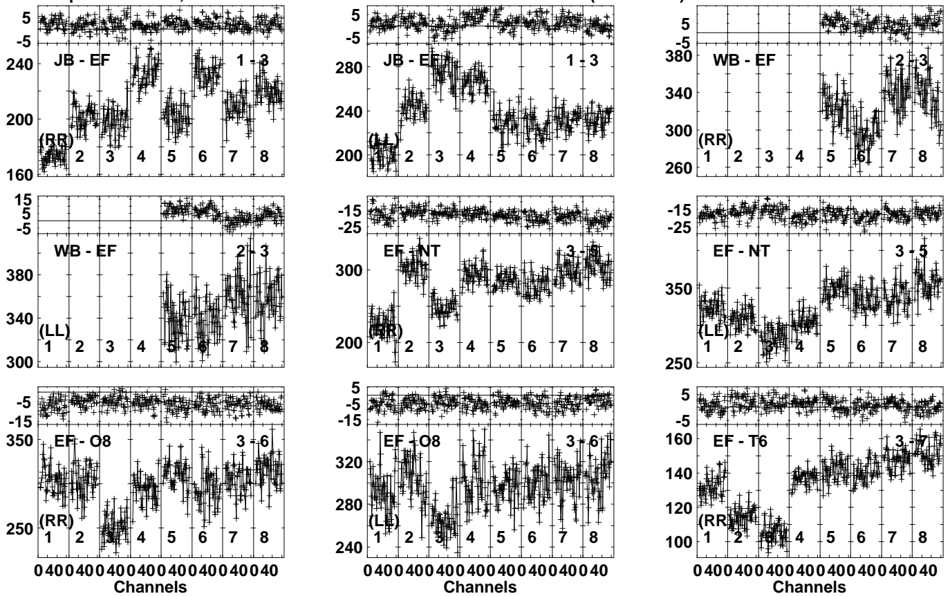
Lower frame: Milli Ampl Jy Top frame: Phas deg Vector averaged cross-power spectrum Several baselines displayed Timerange: 00:18:07:21 to 00:18:08:49
