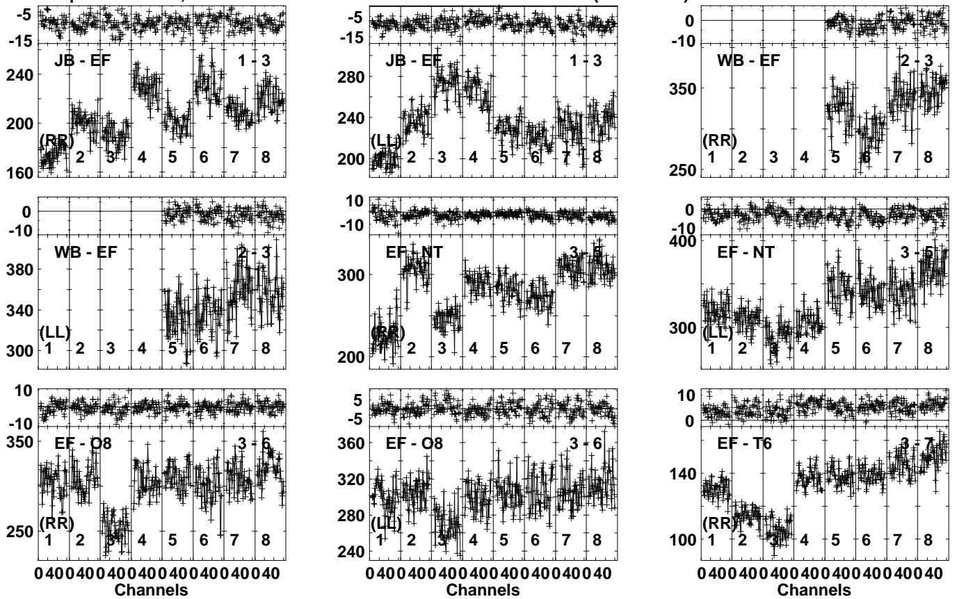
Lower frame: Milli Ampl Jy Top frame: Phas deg Vector averaged cross-power spectrum Several baselines displayed Timerange: 00/18:02:51 to 00/18:03:49
