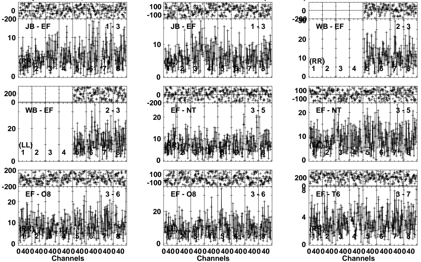
Lower frame: Milli Ampl Jy Top frame: Phas deg Vector averaged cross-power spectrum Several baselines displayed Timerange: 00/19:18:51 to 00/19:22:19
