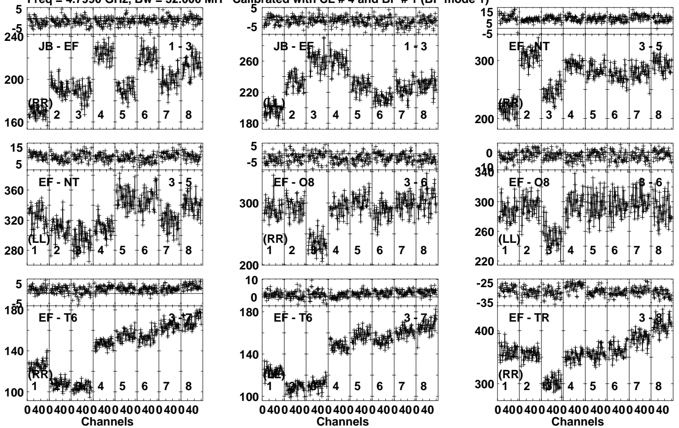
Lower frame: Milli Ampl Jy Top frame: Phas deg Vector averaged cross-power spectrum Several baselines displayed Timerange: 00/14:11:31 to 00/14:12:59
