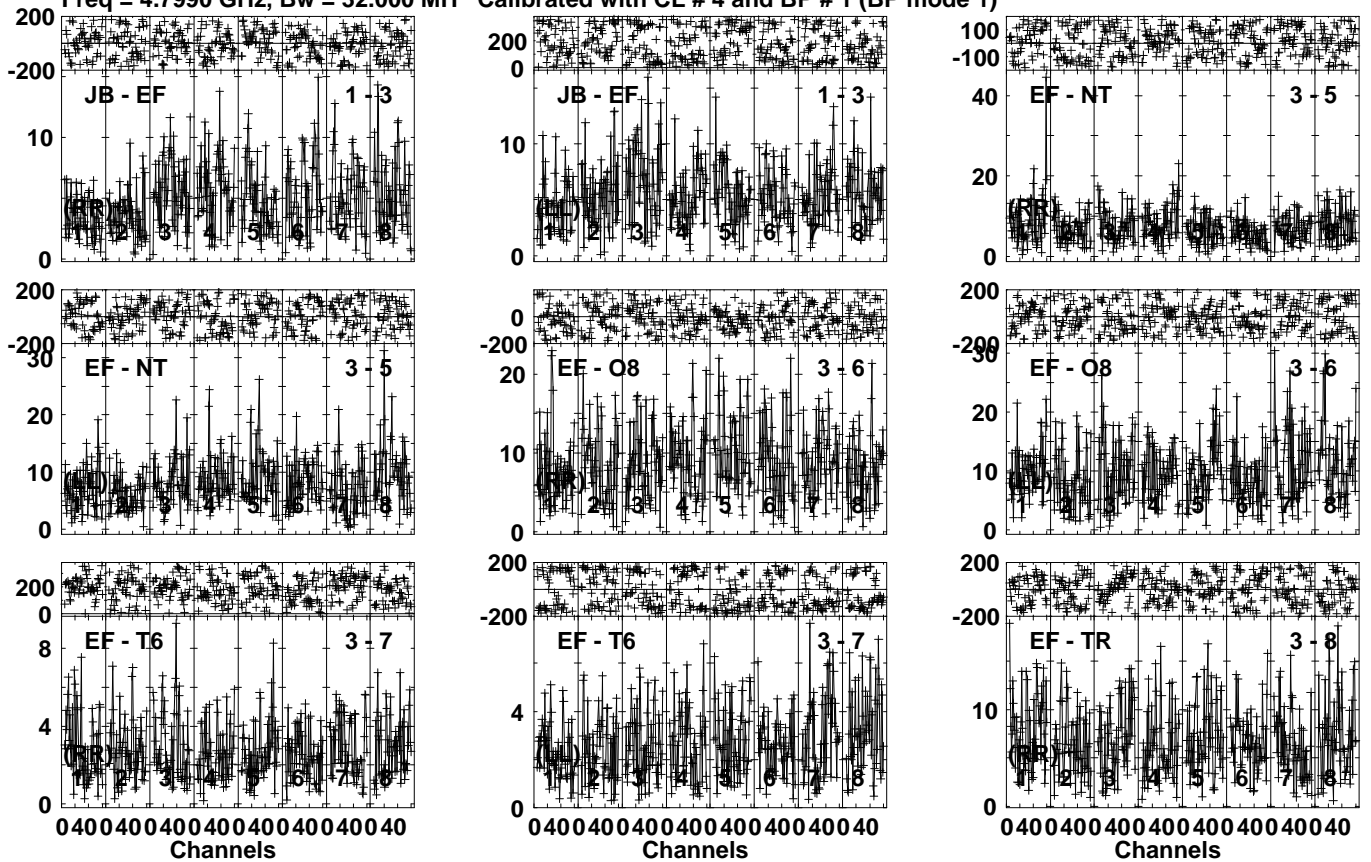
Lower frame: Milli Ampl Jy Top frame: Phas deg Vector averaged cross-power spectrum Several baselines displayed Timerange: 00/14:33:01 to 00/14:36:29
