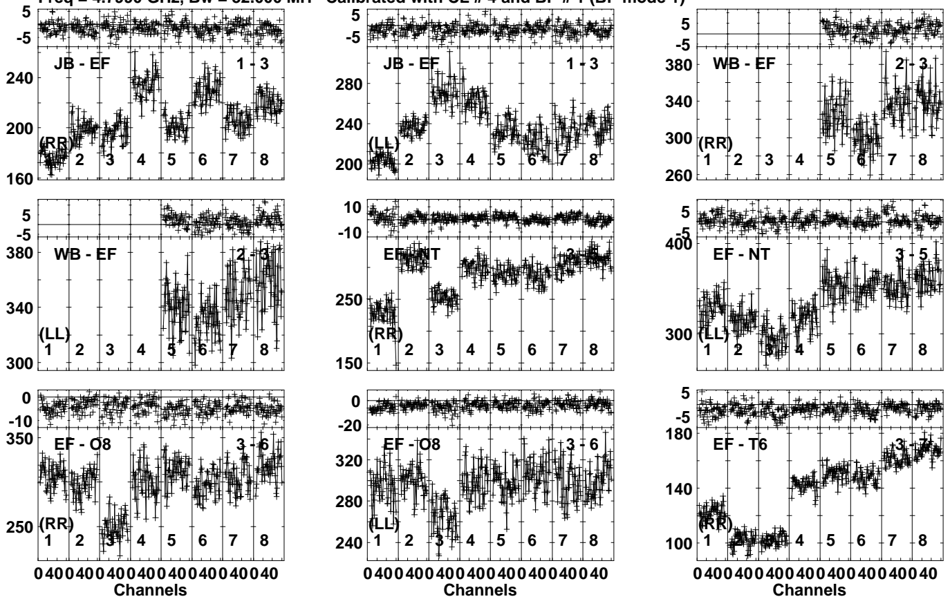
Lower frame: Milli Ampl Jy Top frame: Phas deg Vector averaged cross-power spectrum Several baselines displayed Timerange: 00:16:07:01 to 00:16:07:59
