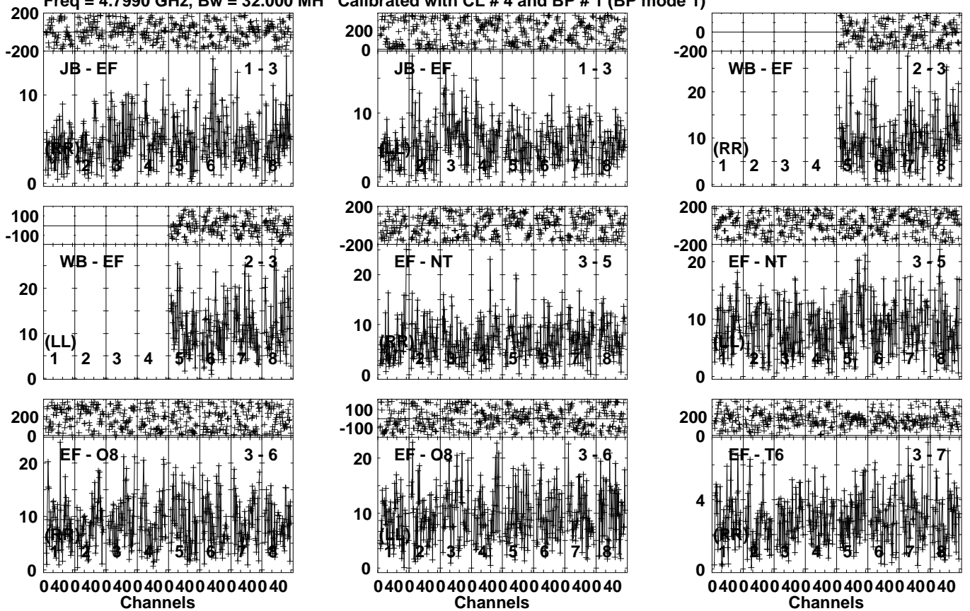
Lower frame: Milli Ampl Jy Top frame: Phas deg Vector averaged cross-power spectrum Several baselines displayed Timerange: 00/15:03:01 to 00/15:06:29
