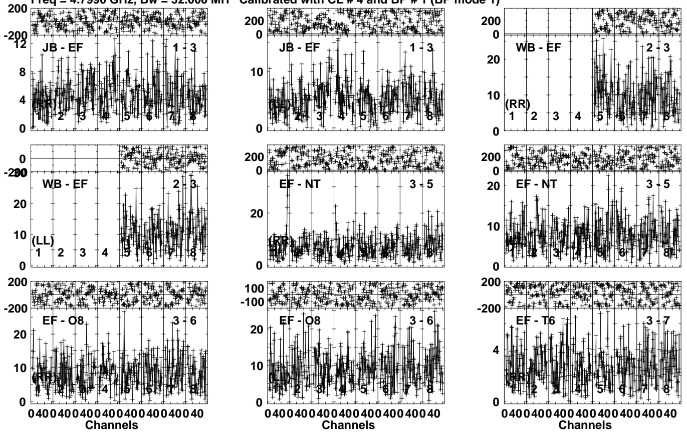
Lower frame: Milli Ampl Jy Top frame: Phas deg Vector averaged cross-power spectrum Several baselines displayed Timerange: 00/15:43:01 to 00/15:46:29
