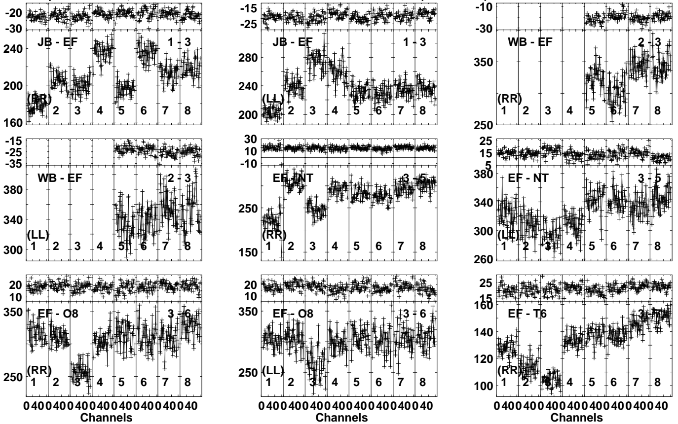
Lower frame: Milli Ampl Jy Top frame: Phas deg Vector averaged cross-power spectrum Several baselines displayed Timerange: 00/17:47:21 to 00/17:48:49
