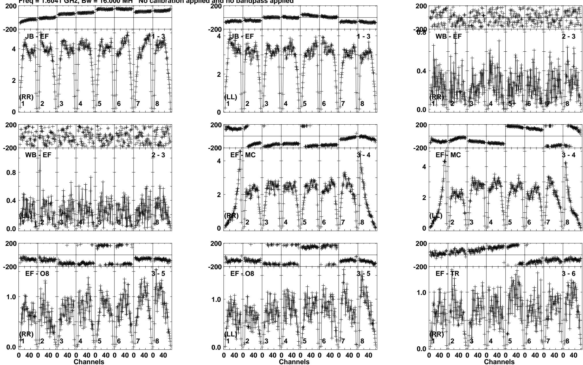
Lower frame: Milli Ampl Jy Top frame: Phas deg Vector averaged cross-power spectrum Baseline: JB (01) - EF (03) Timerange: 01/00:17:46 to 01/00:19:14
