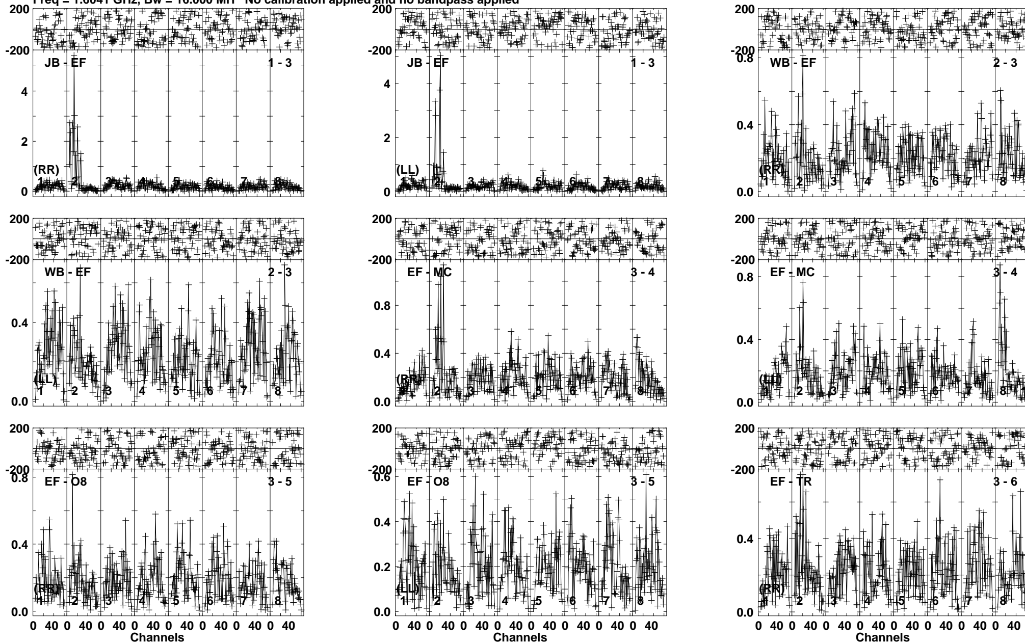
Lower frame: Milli Ampl Jy Top frame: Phas deg Vector averaged cross-power spectrum Baseline: JB (01) - EF (03) Timerange: 00:22:09:01 to 00:22:10:43
