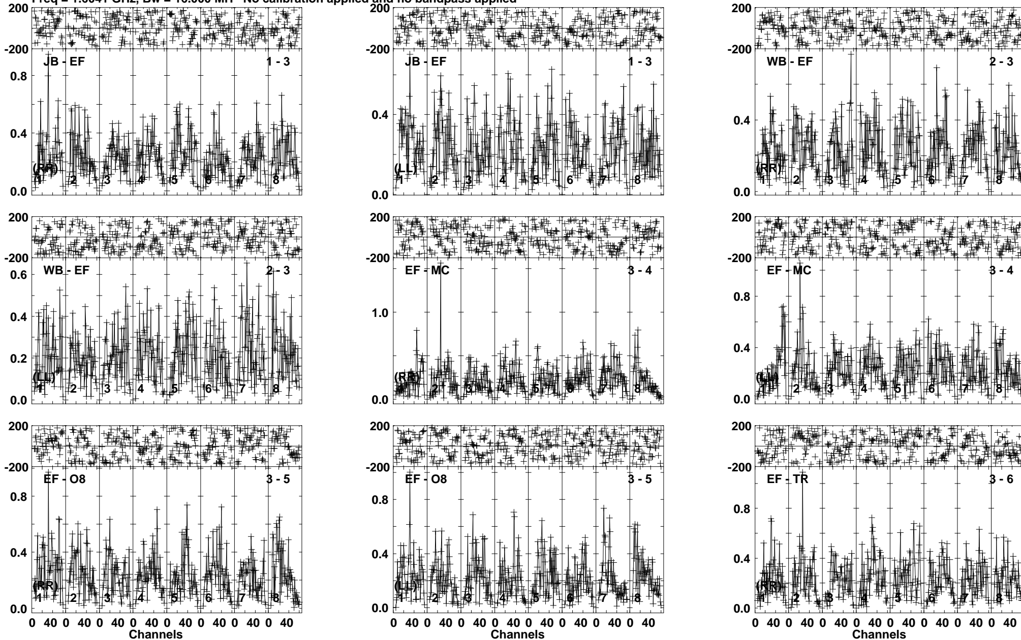
Lower frame: Milli Ampl Jy Top frame: Phas deg Vector averaged cross-power spectrum Baseline: JB (01) - EF (03) Timerange: 01/00:22:31 to 01/00:24:13
