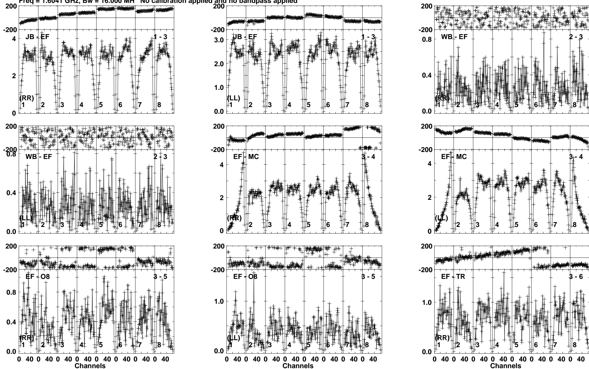
Lower frame: Milli Ampl Jy Top frame: Phas deg Vector averaged cross-power spectrum Baseline: JB (01) - EF (03) Timerange: 01/01:52:01 to 01/01:53:29
