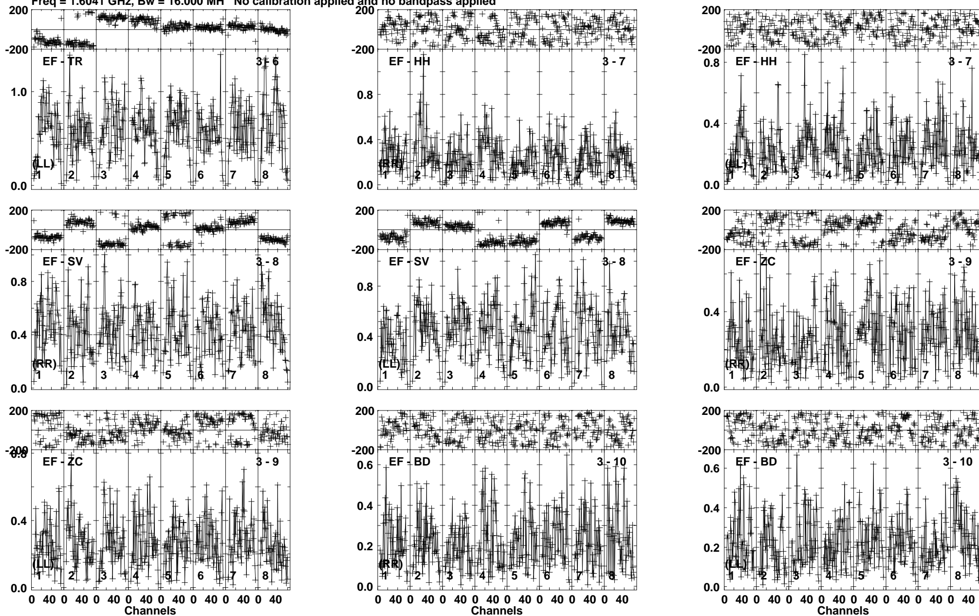
Lower frame: Milli Ampl Jy Top frame: Phas deg Vector averaged cross-power spectrum Baseline: EF (03) - TR (06) Timerange: 00/23:22:46 to 00/23:24:14
