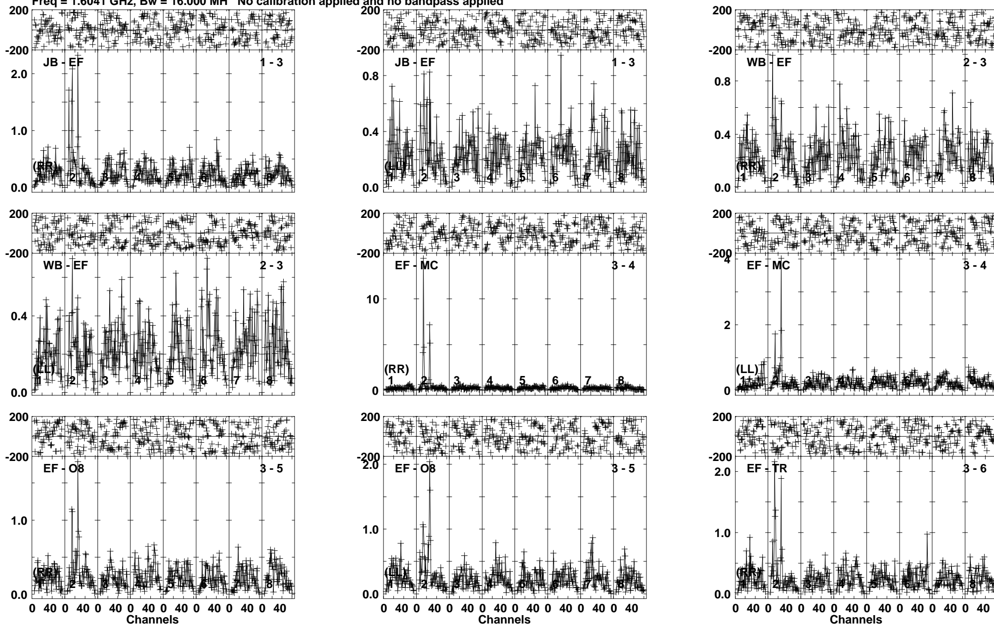
Lower frame: Milli Ampl Jy Top frame: Phas deg Vector averaged cross-power spectrum Baseline: JB (01) - EF (03) Timerange: 00/22:32:31 to 00/22:34:13
