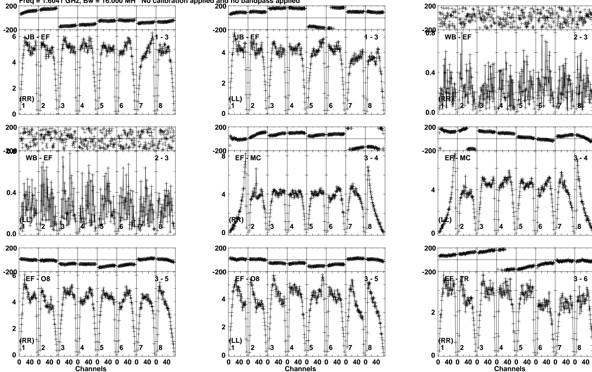
Lower frame: Milli Ampl Jy Top frame: Phas deg Vector averaged cross-power spectrum Baseline: JB (01) - EF (03) Timerange: 01/01:48:46 to 01/01:50:14
