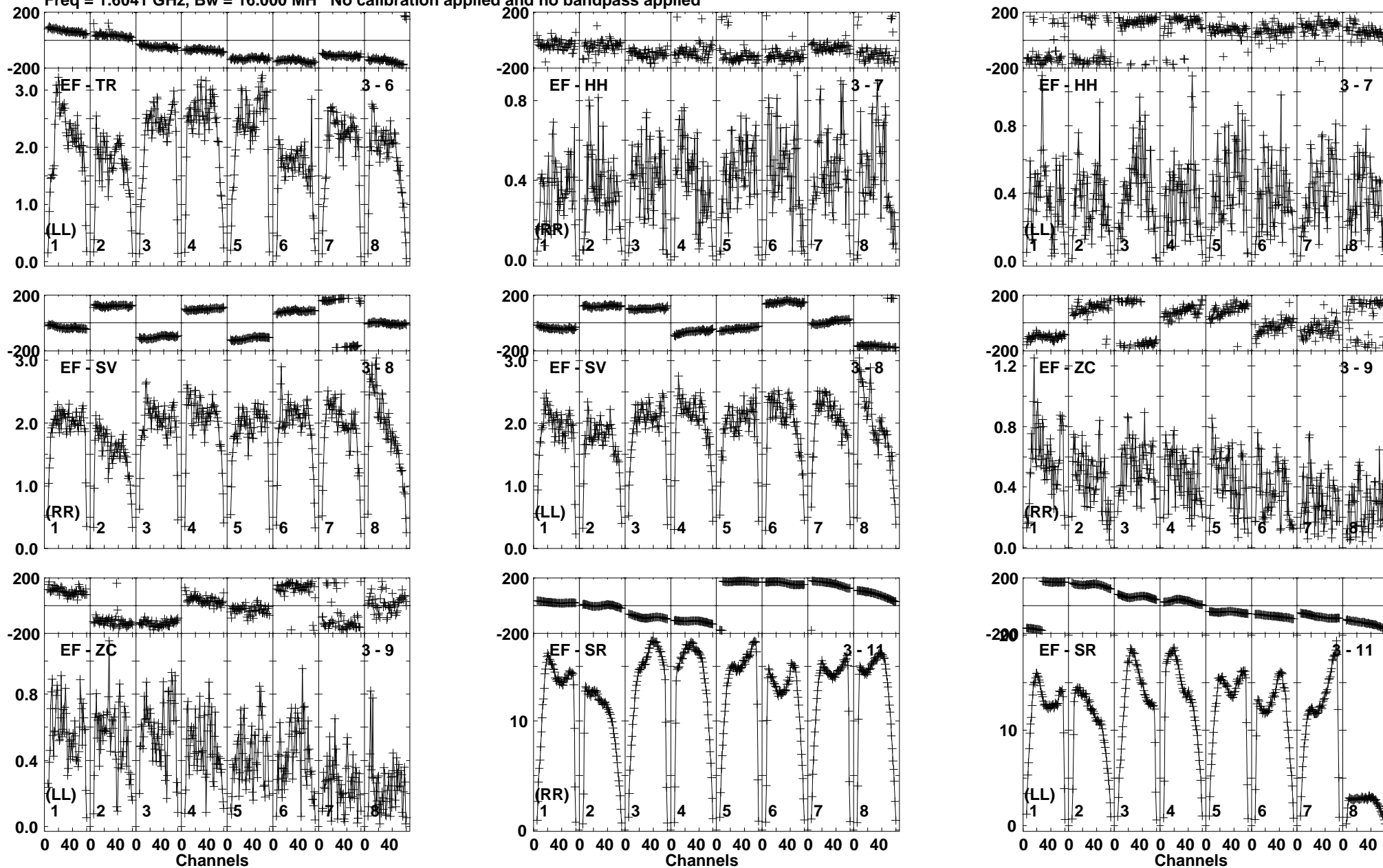
Lower frame: Milli Ampl Jy Top frame: Phas deg Vector averaged cross-power spectrum Baseline: EF (03) - TR (06) Timerange: 01/01:35:01 to 01/01:36:29
