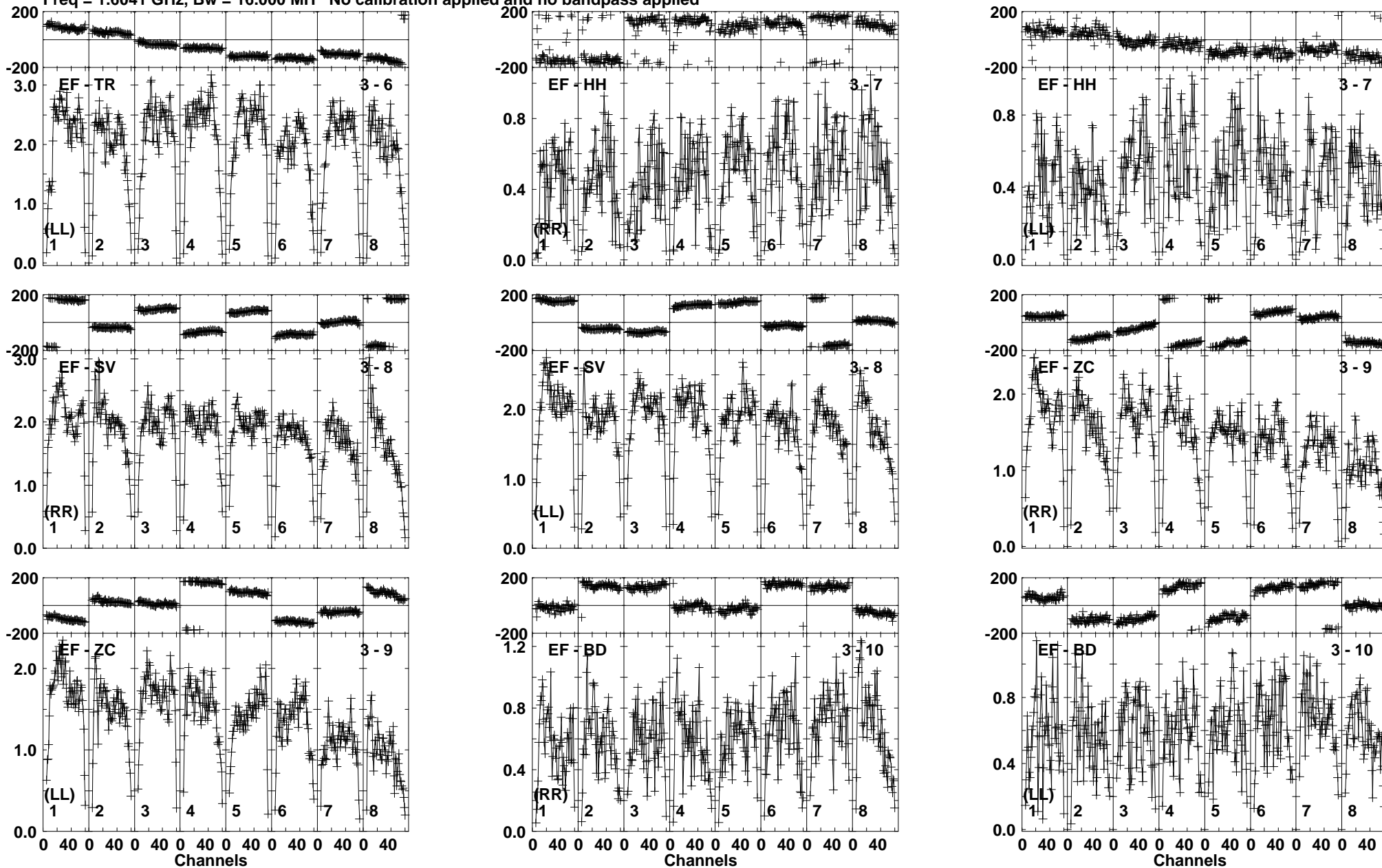
Lower frame: Milli Ampl Jy Top frame: Phas deg Vector averaged cross-power spectrum Baseline: EF (03) - TR (06) Timerange: 00/23:47:01 to 00/23:48:29
