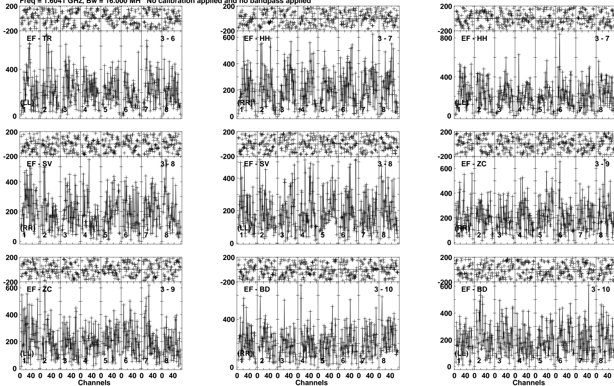
Lower frame: Micro Ampl Jy Top frame: Phas deg Vector averaged cross-power spectrum Baseline: EF (03) - TR (06) Timerange: 01/00:41:31 to 01/00:43:13
