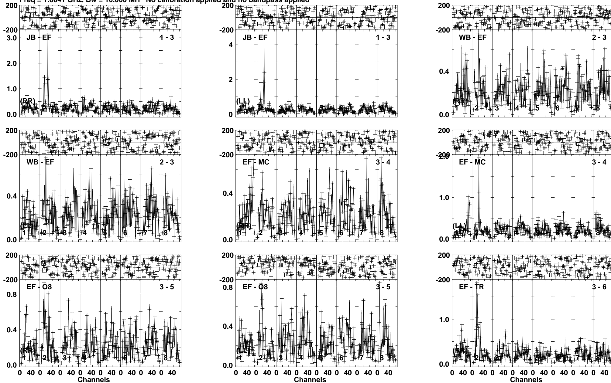
Lower frame: Milli Ampl Jy Top frame: Phas deg Vector averaged cross-power spectrum Baseline: JB (01) - EF (03) Timerange: 01/01:15:31 to 01/01:17:13
