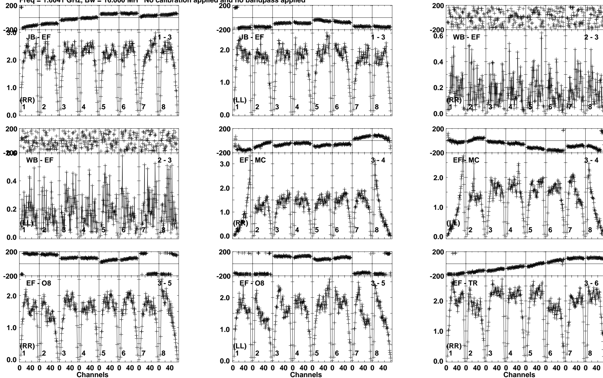
Lower frame: Milli Ampl Jy Top frame: Phas deg Vector averaged cross-power spectrum Baseline: JB (01) - EF (03) Timerange: 01/02:26:46 to 01/02:28:14
