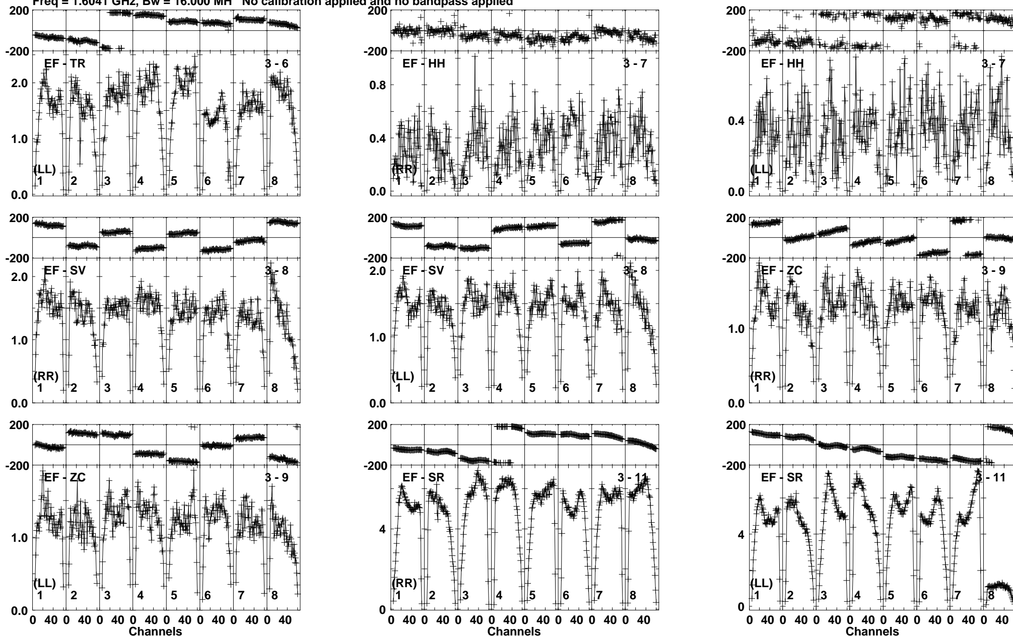
Lower frame: Milli Amply Jy Top frame: Phas deg Vector averaged cross-power spectrum Baseline: EF (03) - TR (06) Timerange: 01/01:59:16 to 01/02:00:44
