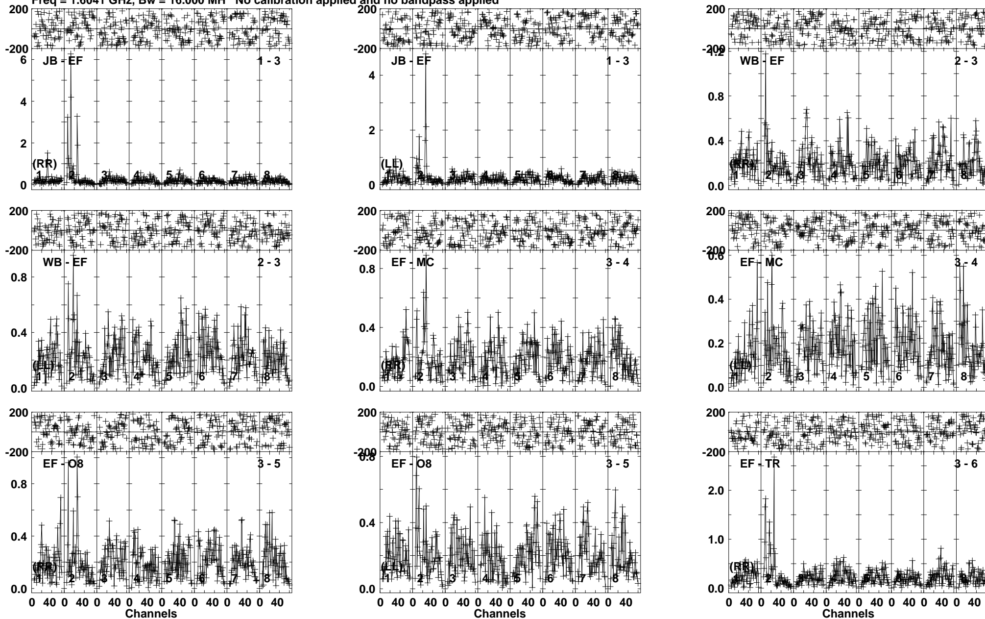
Lower frame: Milli Ampl Jy Top frame: Phas deg Vector averaged cross-power spectrum Baseline: JB (01) - EF (03) Timerange: 00:22:53:31 to 00:22:55:13
