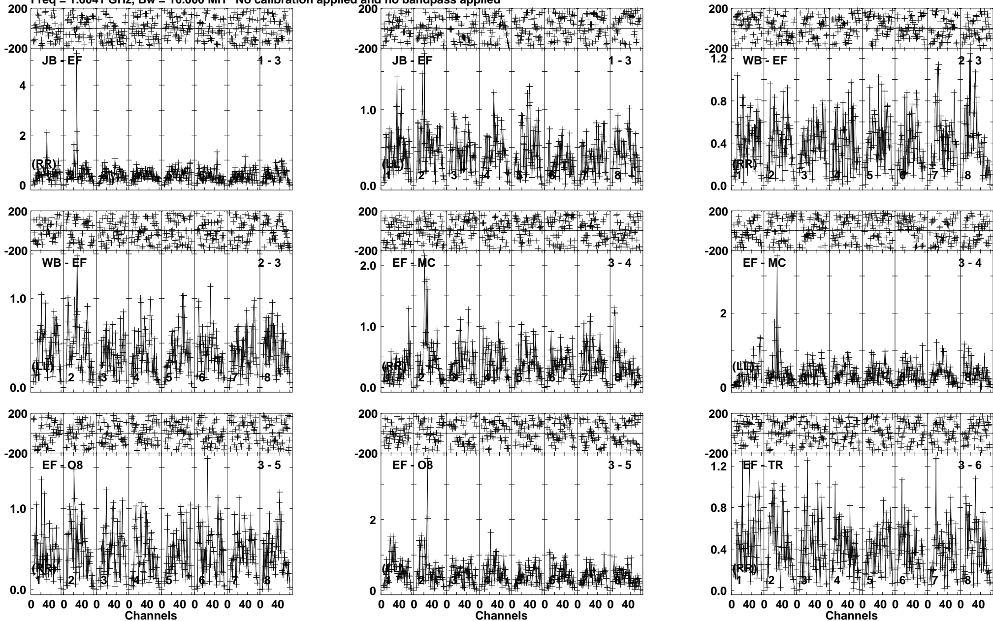
Lower frame: Milli Ampl Jy Top frame: Phas deg Vector averaged cross-power spectrum Baseline: JB (01) - EF (03) Timerange: 00:22:04:01 to 00:22:06:43
