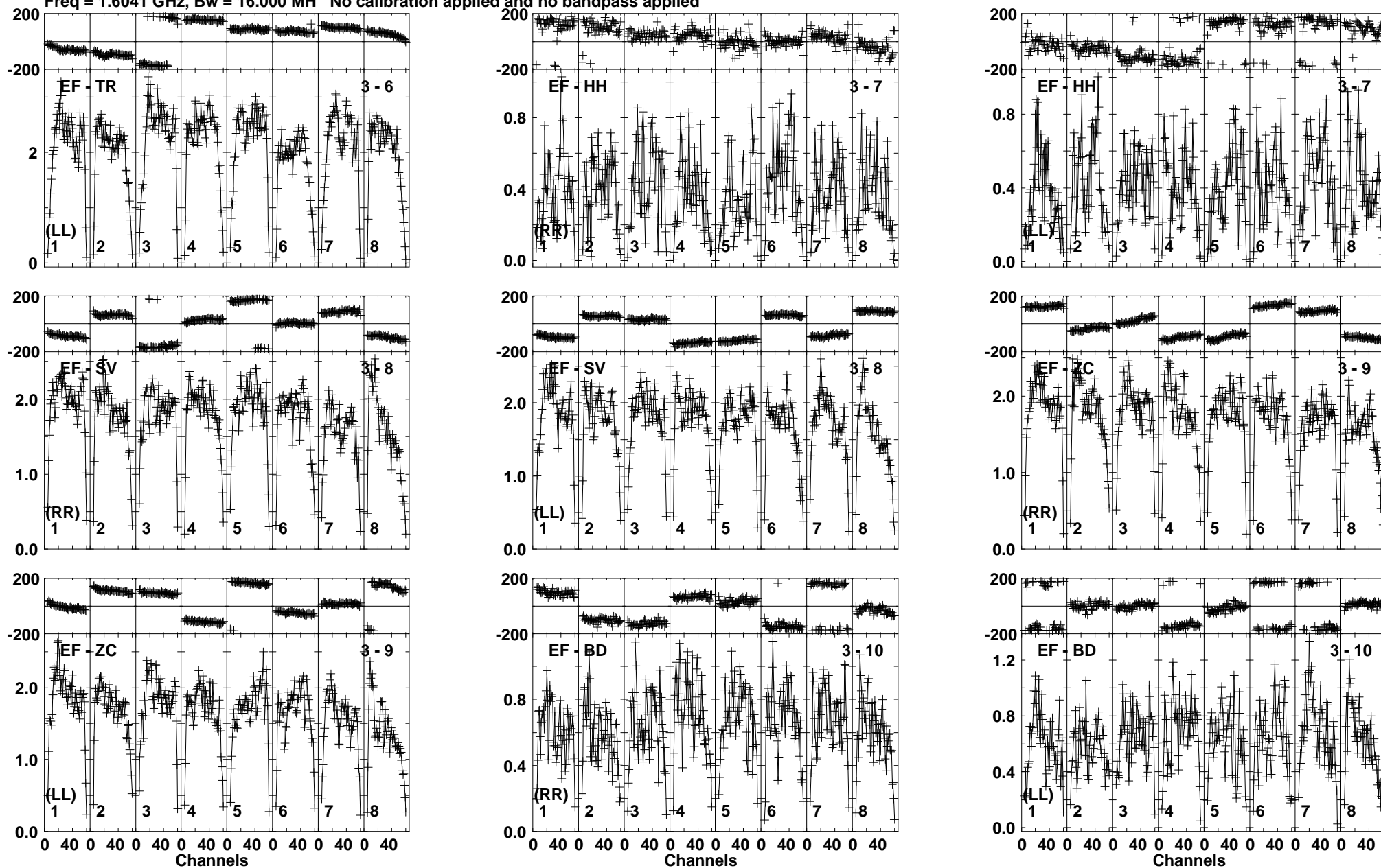
Lower frame: Milli Ampl Jy Top frame: Phas deg Vector averaged cross-power spectrum Baseline: EF (03) - TR (06) Timerange: 00/23:05:46 to 00/23:07:14
