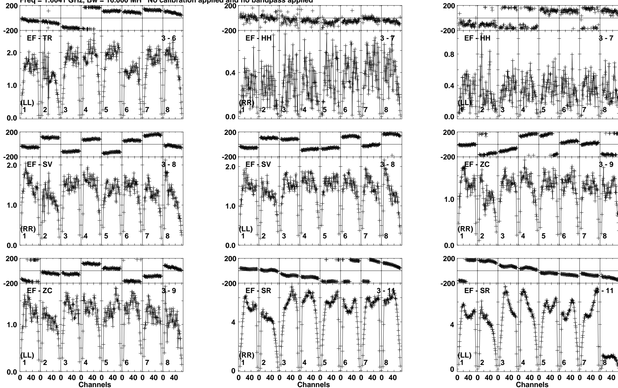
Lower frame: Milli Amply Jy Top frame: Phas deg Vector averaged cross-power spectrum Baseline: EF (03) - TR (06) Timerange: 01/01:45:31 to 01/01:46:59
