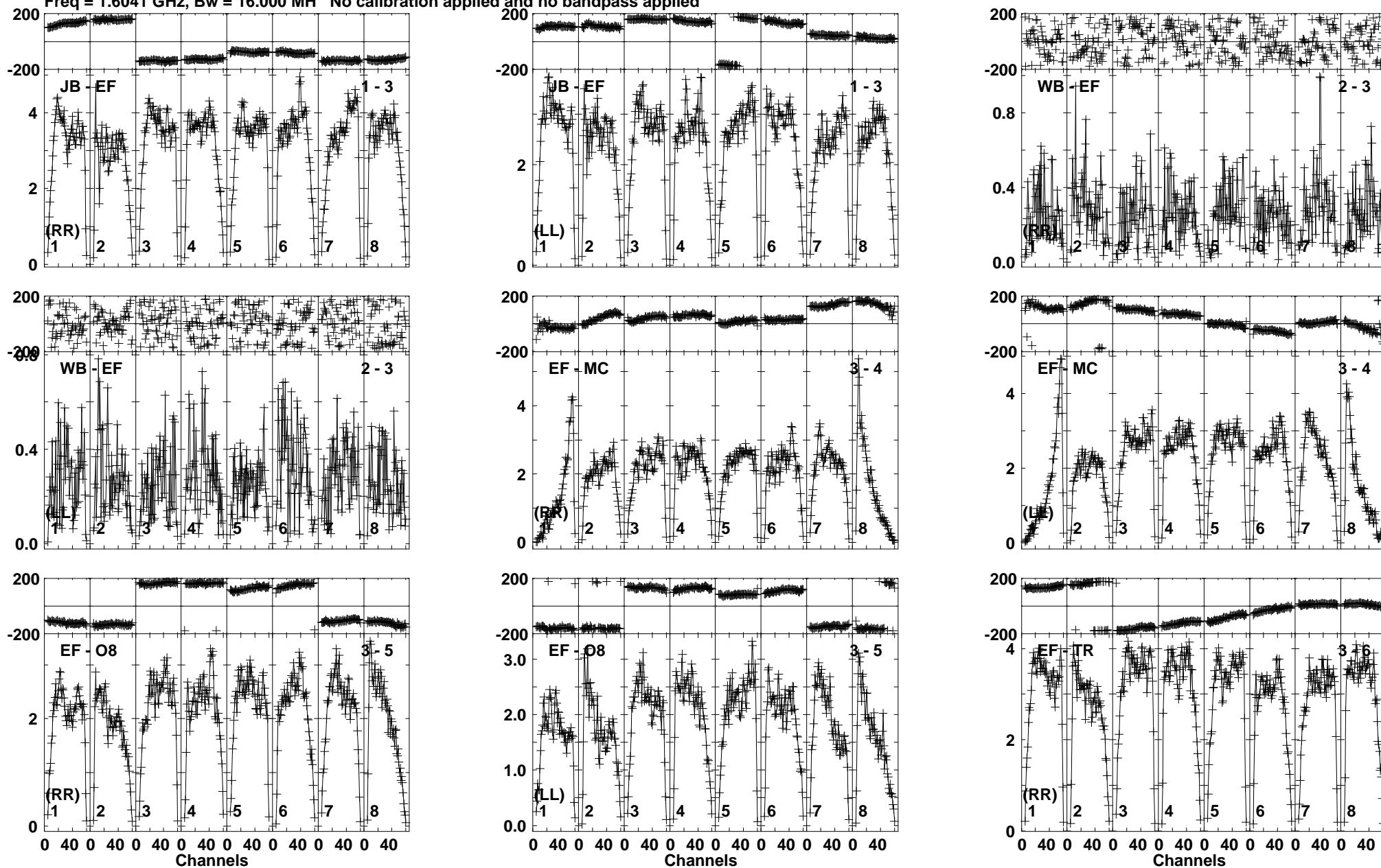
Lower frame: Milli Ampl Jy Top frame: Phas deg Vector averaged cross-power spectrum Baseline: JB (01) - EF (03) Timerange: 00/23:12:16 to 00/23:13:44
