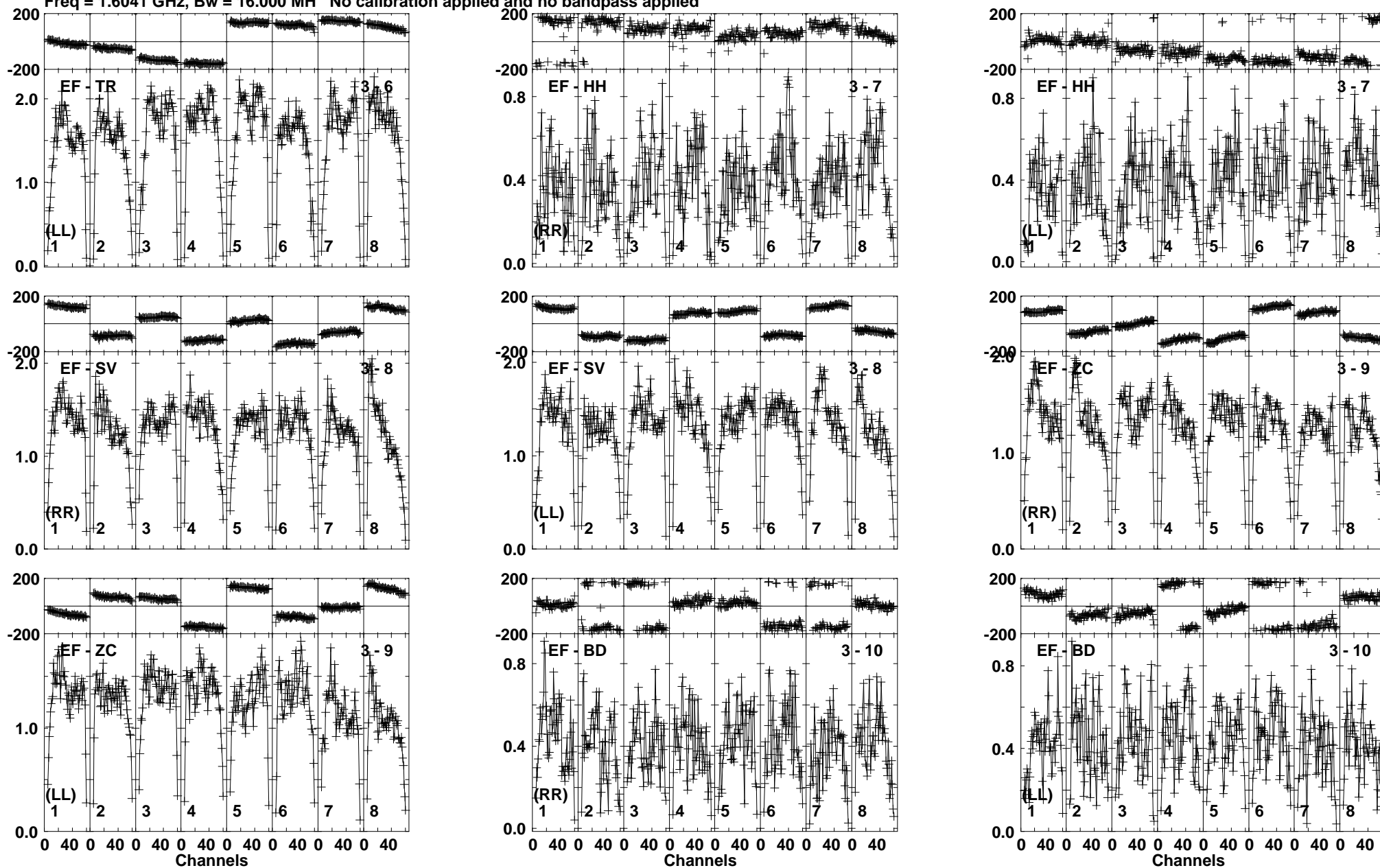
Lower frame: Milli Ampl Jy Top frame: Phas deg Vector averaged cross-power spectrum Baseline: EF (03) - TR (06) Timerange: 01/00:11:16 to 01/00:12:44
