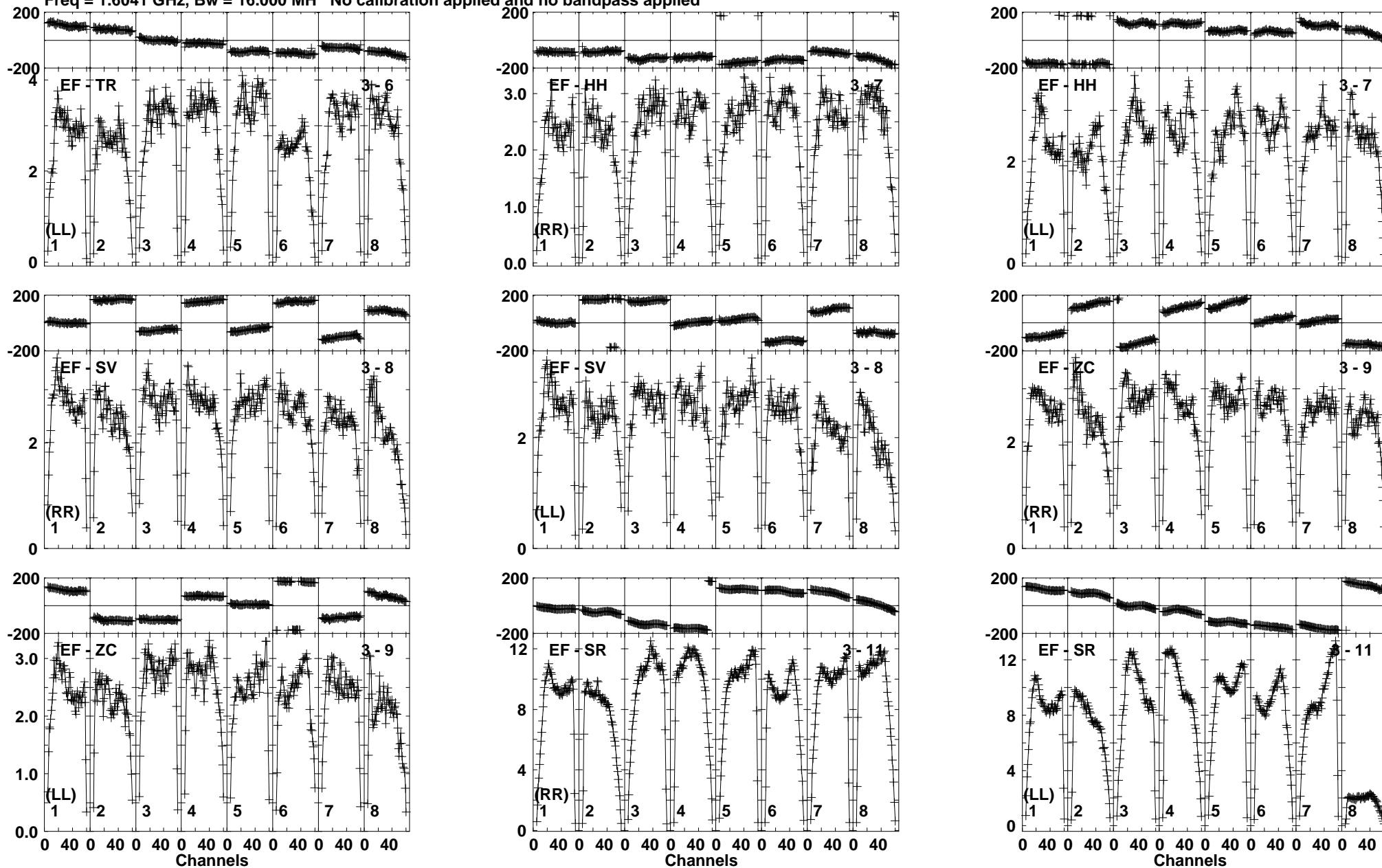
Lower frame: Milli Ampl Jy Top frame: Phas deg Vector averaged cross-power spectrum Baseline: EF (03) - TR (06) Timerange: 01/02:50:16 to 01/02:51:44
