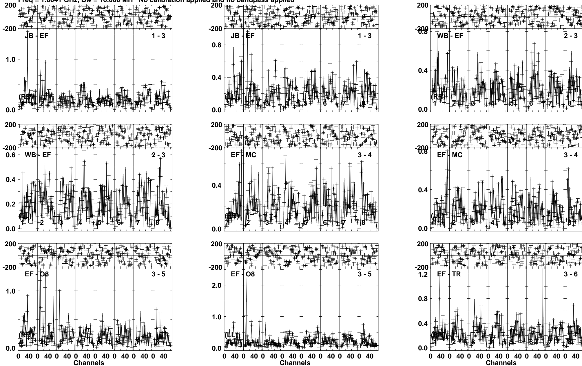
Lower frame: Milli Ampl Jy Top frame: Phas deg Vector averaged cross-power spectrum Baseline: JB (01) - EF (03) Timerange: 01/02:51:46 to 01/02:53:28
