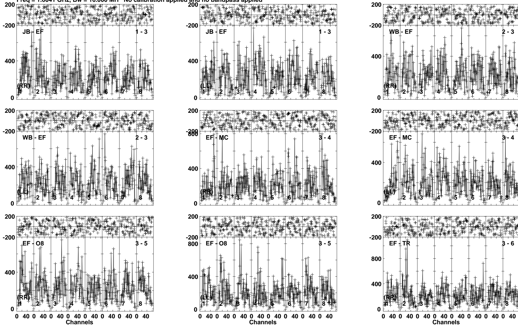
Lower frame: Micro Ampl Jy Top frame: Phas deg Vector averaged cross-power spectrum Baseline: JB (01) - EF (03) Timerange: 01/00:05:31 to 01/00:07:13
