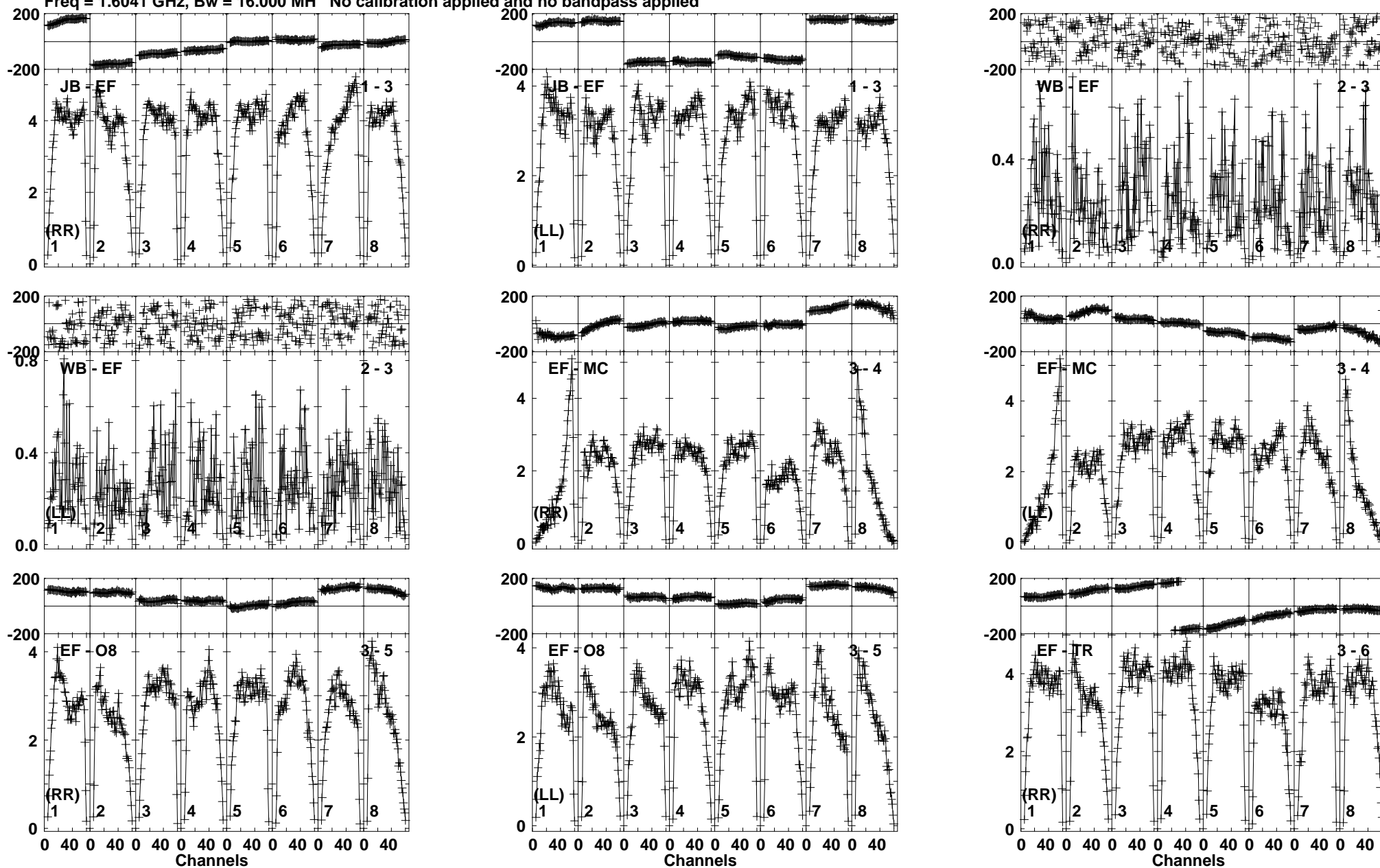
Lower frame: Milli Ampl Jy Top frame: Phas deg Vector averaged cross-power spectrum Baseline: JB (01) - EF (03) Timerange: 01/02:36:31 to 01/02:37:59
