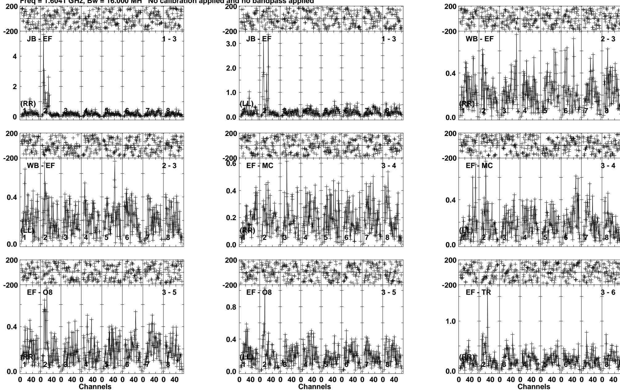
Lower frame: Milli Ampl Jy Top frame: Phas deg Vector averaged cross-power spectrum Baseline: JB (01) - EF (03) Timerange: 00:22:36:31 to 00:22:38:13
