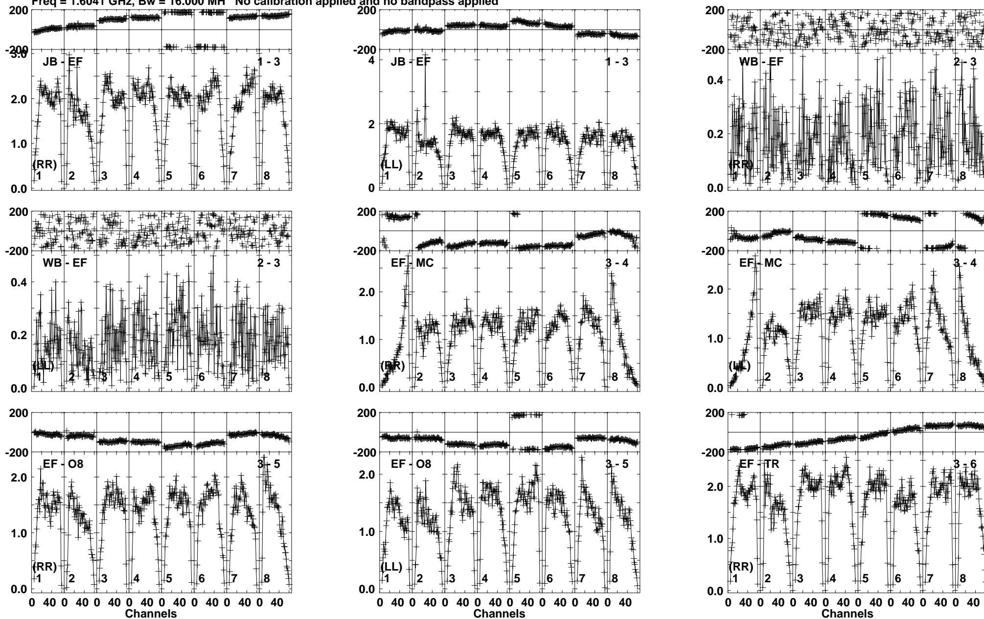
Lower frame: Milli Ampl Jy Top frame: Phas deg Vector averaged cross-power spectrum Baseline: JB (01) - EF (03) Timerange: 00/23:30:01 to 00/23:31:29
