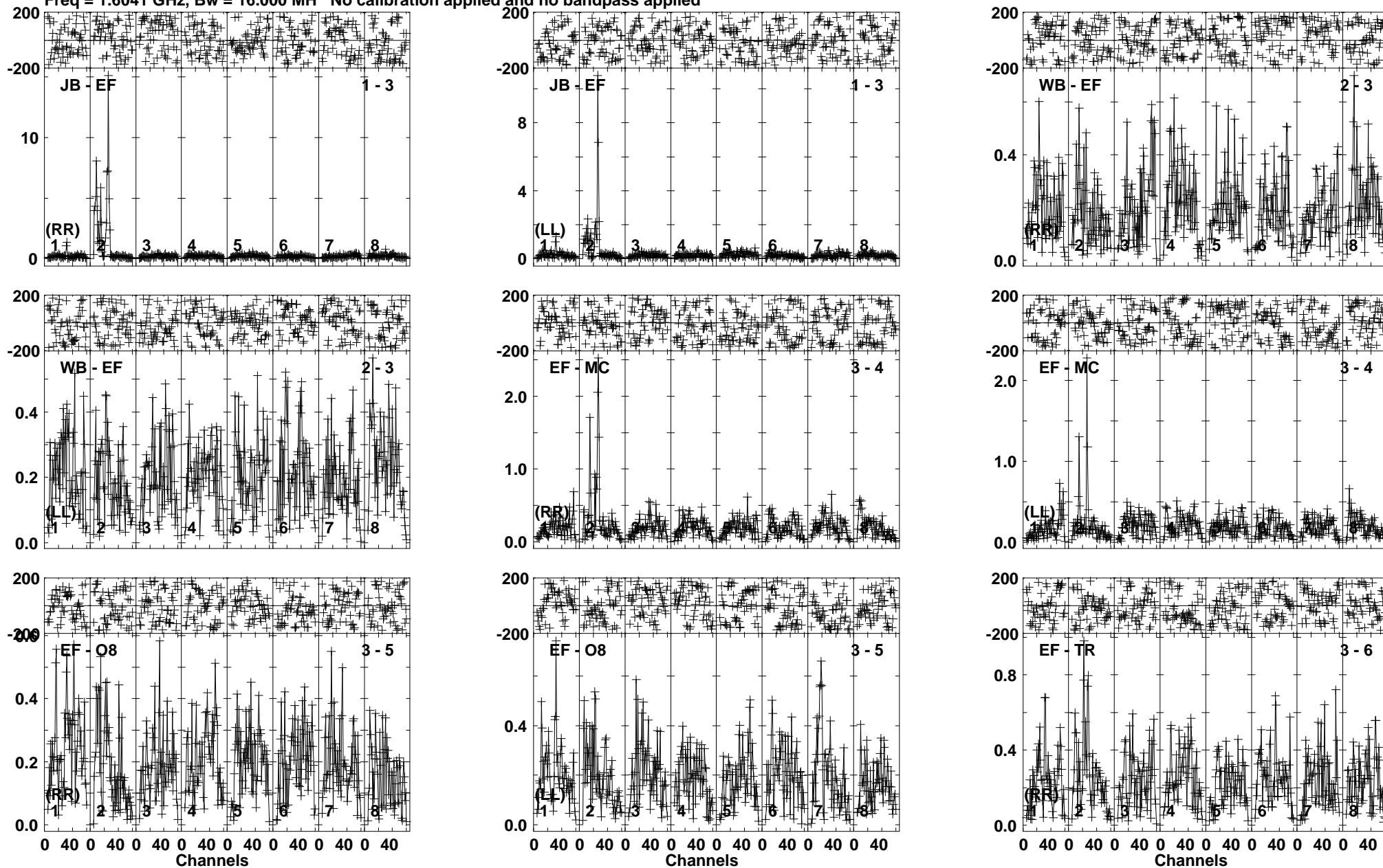
Lower frame: Milli Ampl Jy Top frame: Phas deg Vector averaged cross-power spectrum Baseline: JB (01) - EF (03) Timerange: 00/22:26:01 to 00/22:27:43
