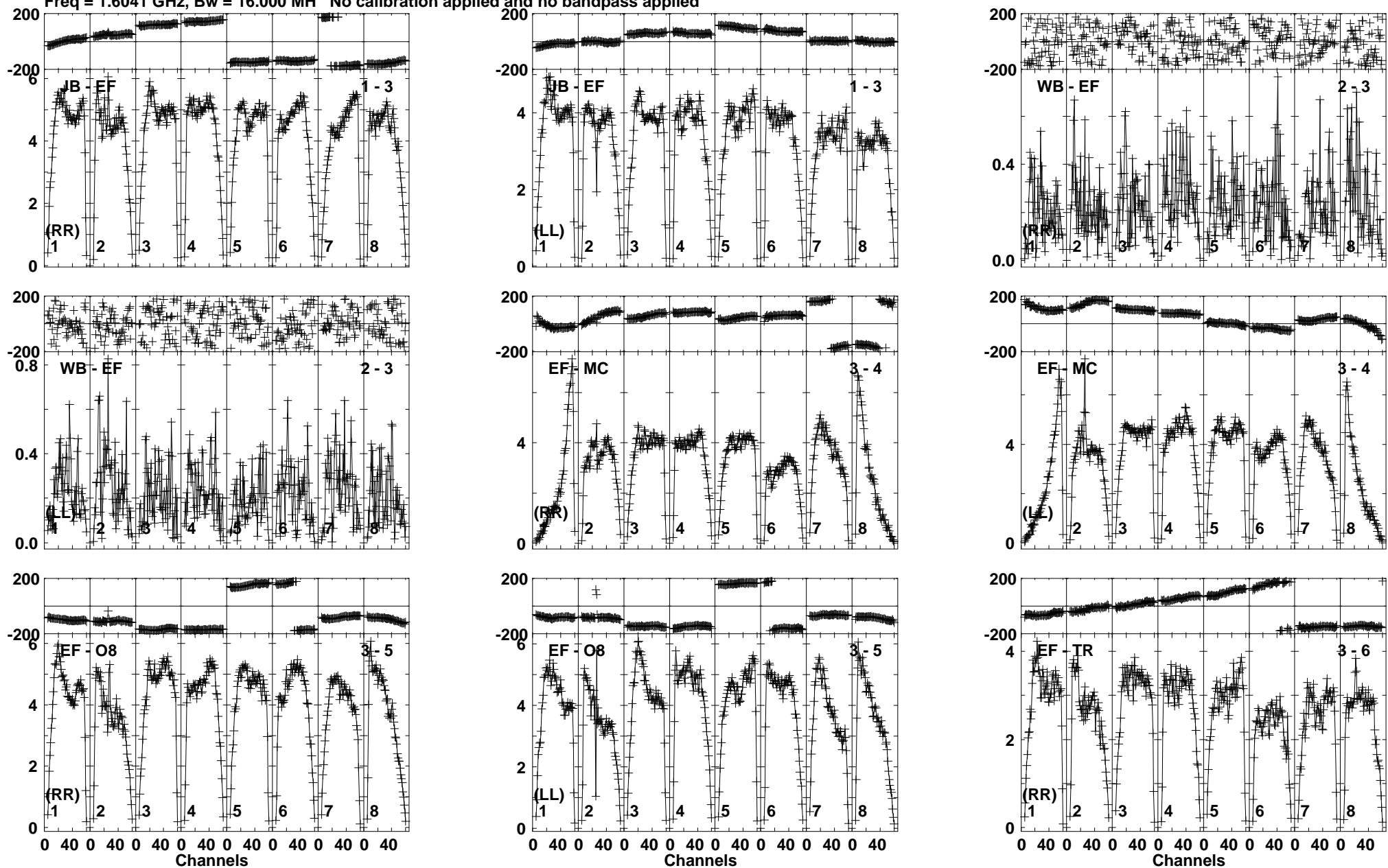
Lower frame: Milli Ampl Jy Top frame: Phas deg Vector averaged cross-power spectrum Baseline: JB (01) - EF (03) Timerange: 01/02:16:16 to 01/02:17:44
