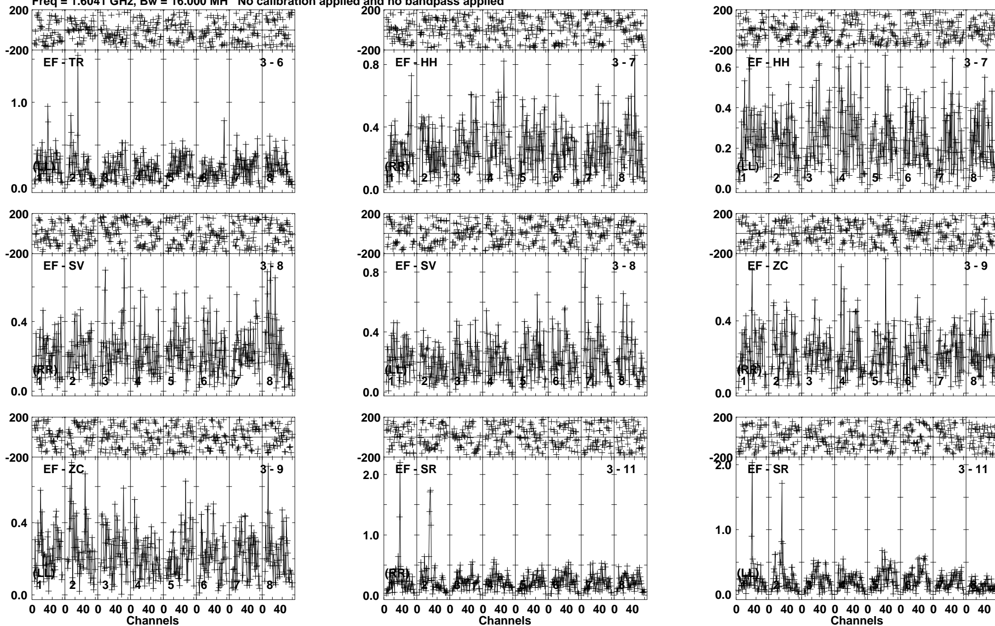
Lower frame: Milli Ampl Jy Top frame: Phas deg Vector averaged cross-power spectrum Baseline: EF (03) - TR (06) Timerange: 01/02:24:16 to 01/02:25:58
