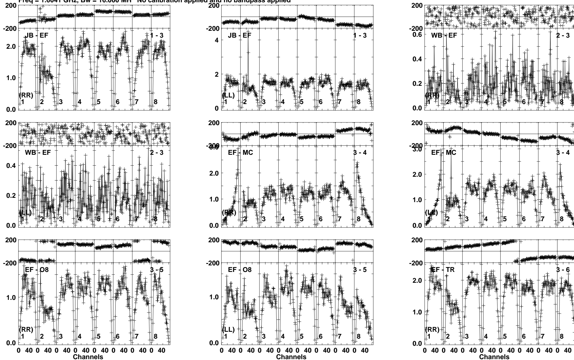
Lower frame: Milli Ampl Jy Top frame: Phas deg Vector averaged cross-power spectrum Baseline: JB (01) - EF (03) Timerange: 00:22:35:01 to 00:22:36:29
