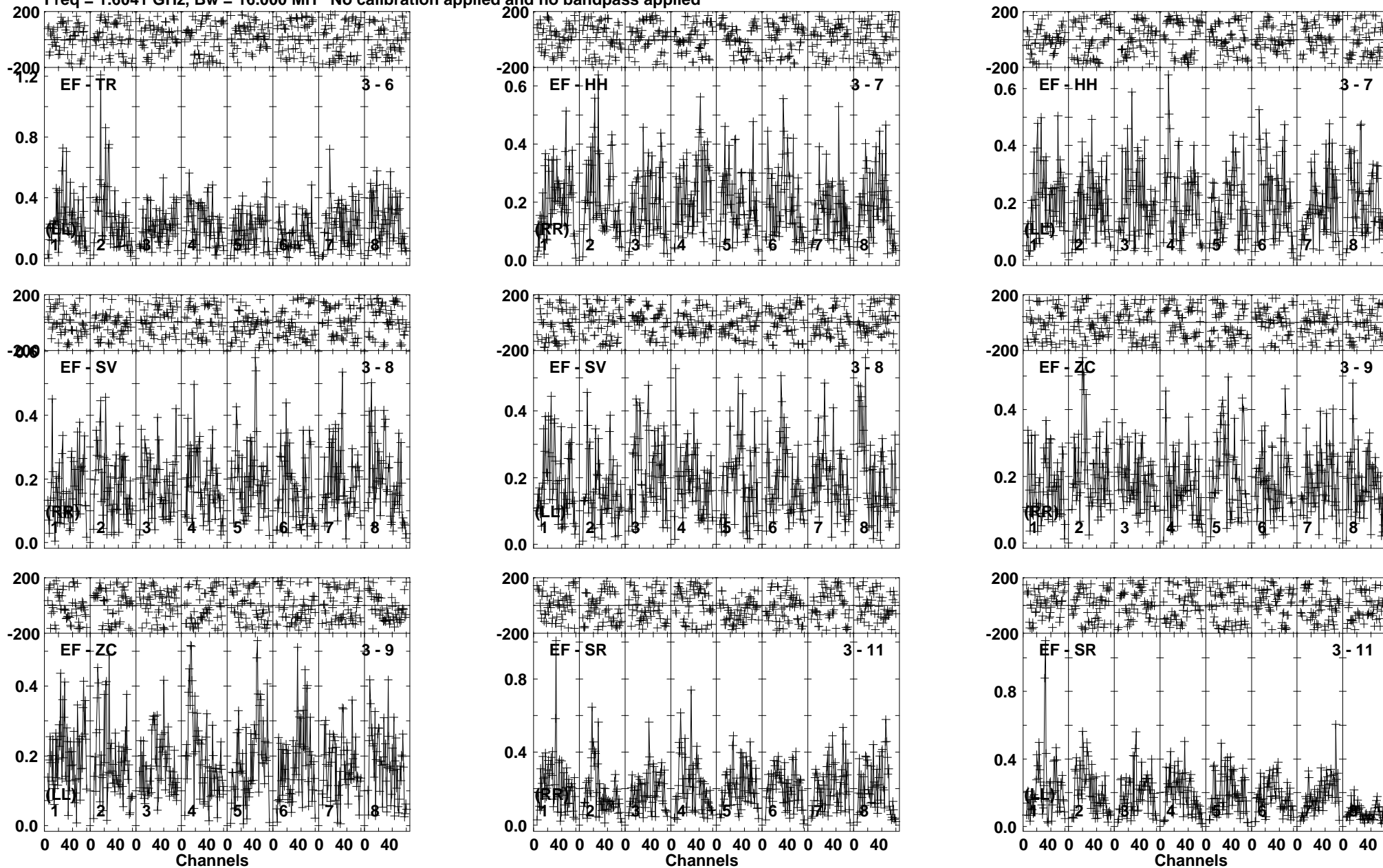
Lower frame: Milli Ampl Jy Top frame: Phas deg Vector averaged cross-power spectrum Baseline: EF (03) - TR (06) Timerange: 01/01:19:31 to 01/01:21:13
