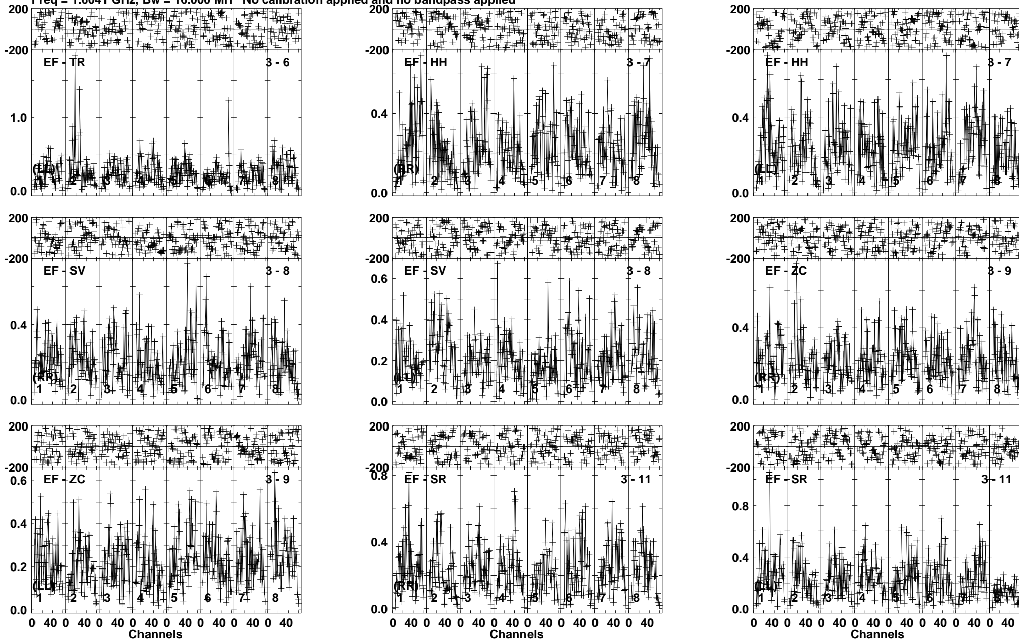
Lower frame: Milli Ampl Jy Top frame: Phas deg Vector averaged cross-power spectrum Baseline: EF (03) - TR (06) Timerange: 01/02:38:01 to 01/02:39:43
