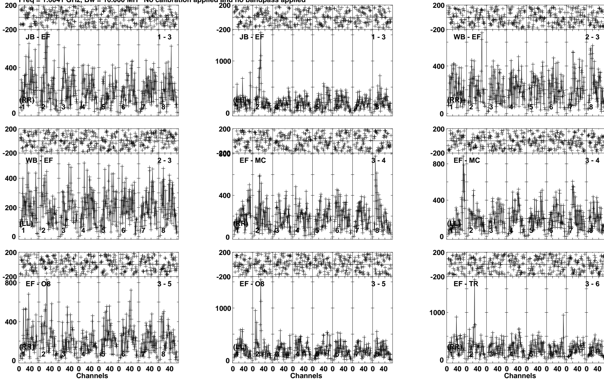
Lower frame: Micro Ampl Jy Top frame: Phas deg Vector averaged cross-power spectrum Baseline: JB (01) - EF (03) Timerange: 01/00:44:46 to 01/00:46:28
