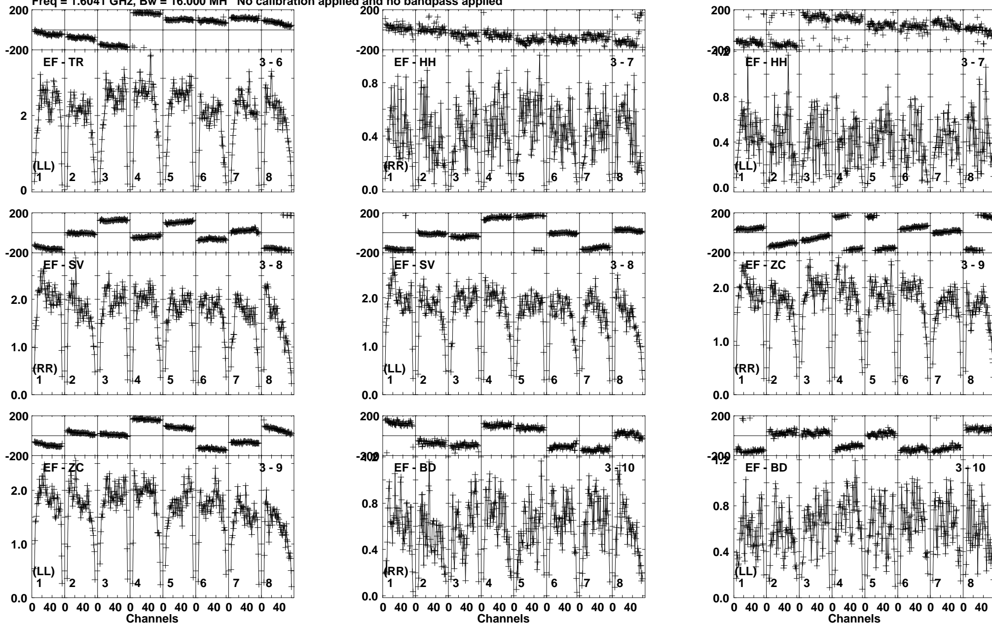
Lower frame: Milli Ampl Jy Top frame: Phas deg Vector averaged cross-power spectrum Baseline: EF (03) - TR (06) Timerange: 00/23:19:31 to 00/23:20:59
