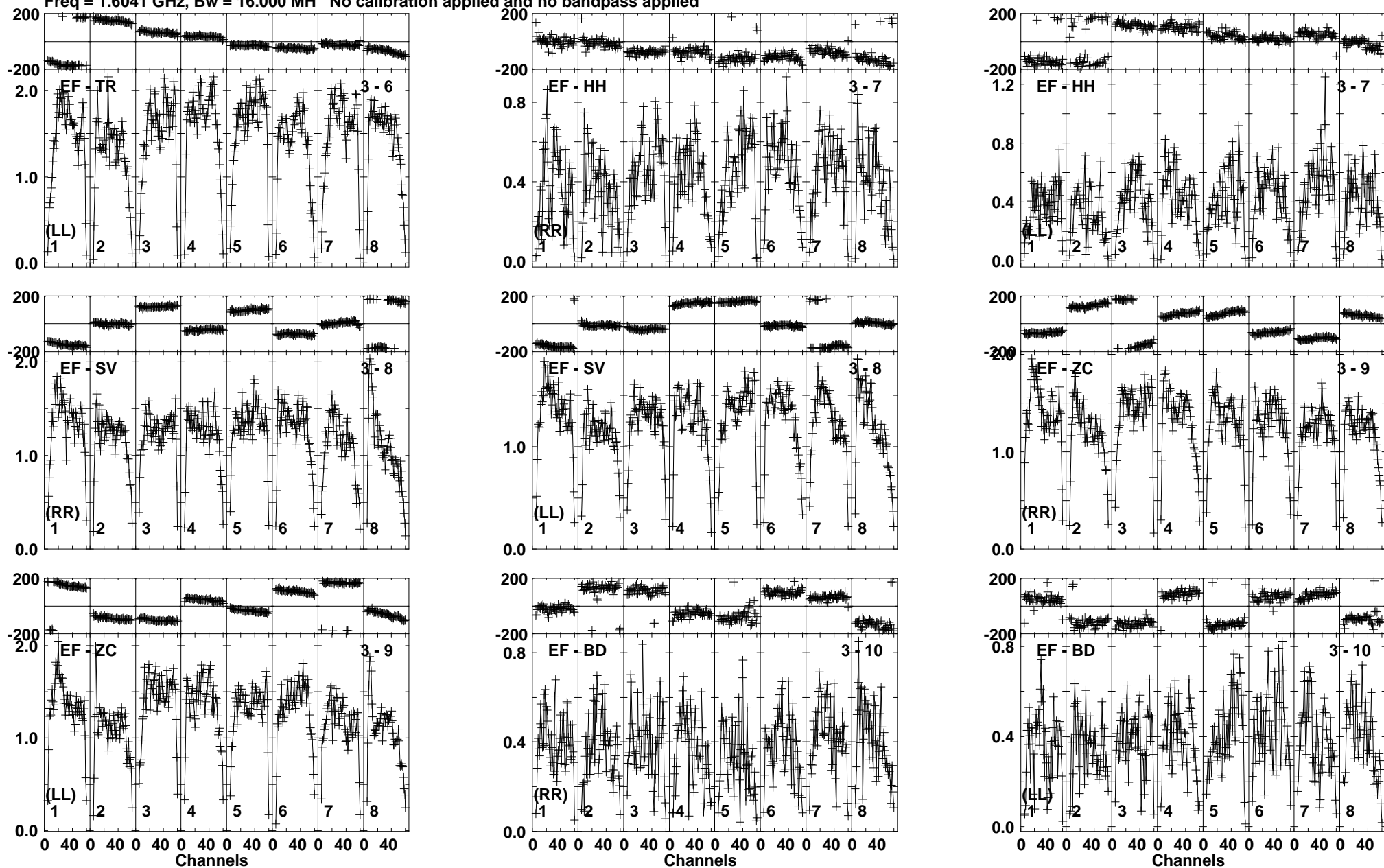
Lower frame: Milli Ampl Jy Top frame: Phas deg Vector averaged cross-power spectrum Baseline: EF (03) - TR (06) Timerange: 00/23:30:01 to 00/23:31:29
