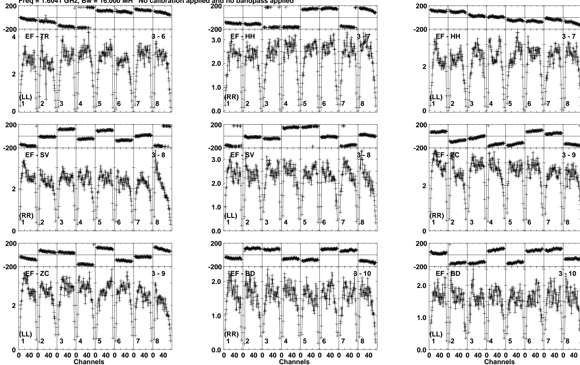
Lower frame: Milli Ampl Jy Top frame: Phas deg Vector averaged cross-power spectrum Baseline: EF (03) - TR (06) Timerange: 00/23:39:46 to 00/23:41:14
