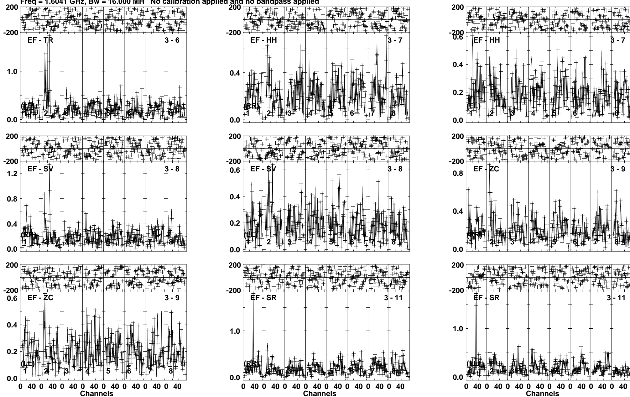
Lower frame: Milli Ampl Jy Top frame: Phas deg Vector averaged cross-power spectrum Baseline: EF (03) - TR (06) Timerange: 01/01:53:31 to 01/01:55:13
