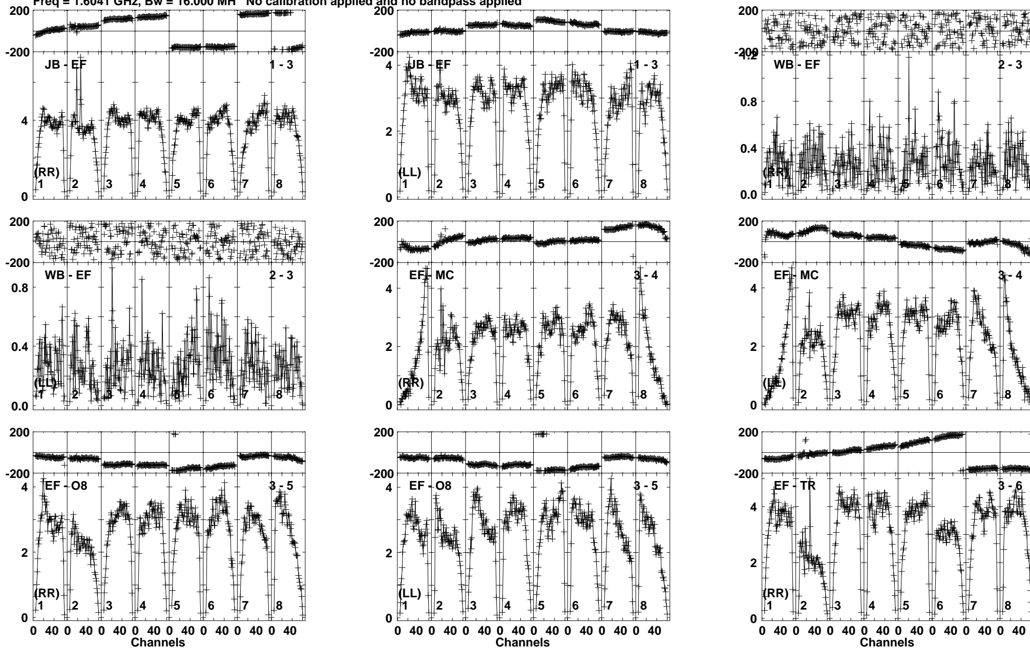
Lower frame: Milli Ampl Jy Top frame: Phas deg Vector averaged cross-power spectrum Baseline: JB (01) - EF (03) Timerange: 01/01:27:46 to 01/01:29:14
