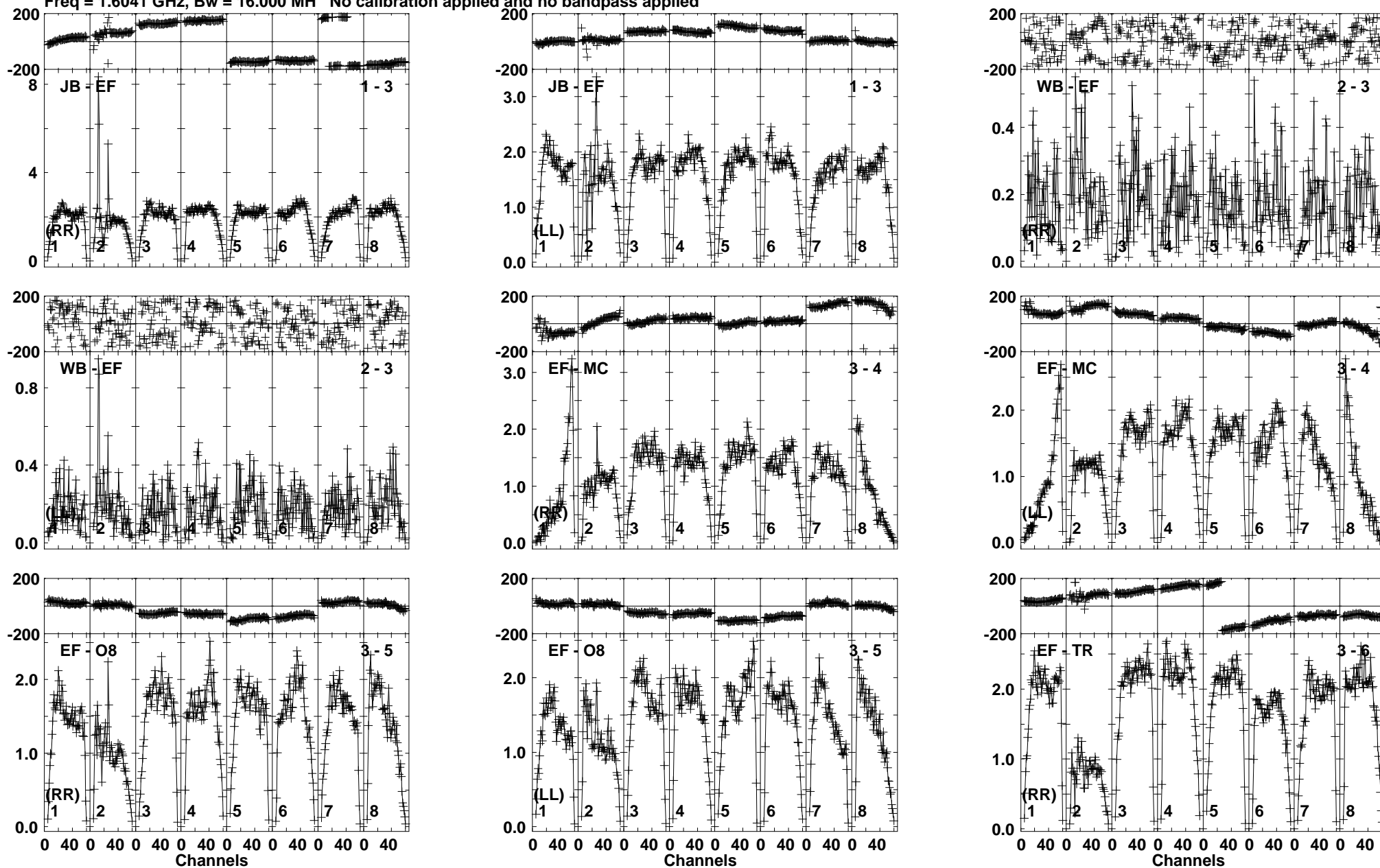
Lower frame: Milli Ampl Jy Top frame: Phas deg Vector averaged cross-power spectrum Baseline: JB (01) - EF (03) Timerange: 01/01:18:01 to 01/01:19:29
