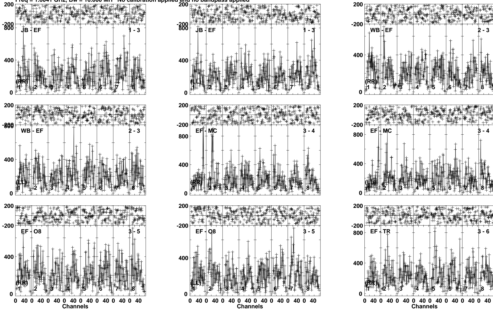
Lower frame: Micro Ampl Jy Top frame: Phas deg Vector averaged cross-power spectrum Baseline: JB (01) - EF (03) Timerange: 01/02:07:16 to 01/02:08:58
