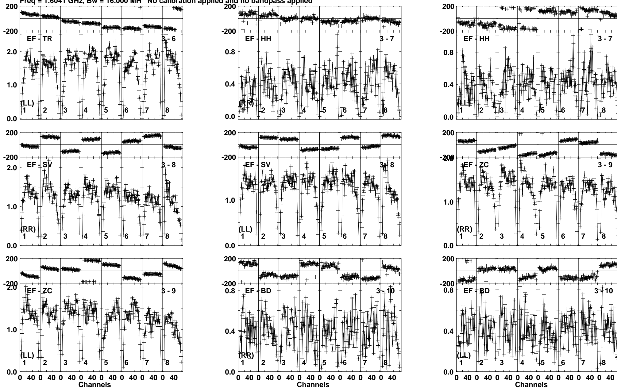
Lower frame: Milli Ampl Jy Top frame: Phas deg Vector averaged cross-power spectrum Baseline: EF (03) - TR (06) Timerange: 00/23:43:46 to 00/23:45:14
