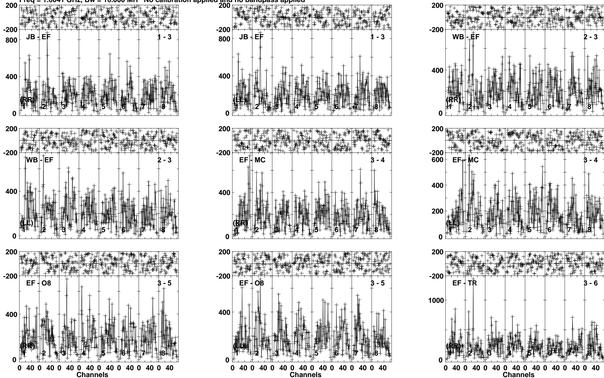
Lower frame: Micro Ampl Jy Top frame: Phas deg Vector averaged cross-power spectrum Baseline: JB (01) - EF (03) Timerange: 01/00:38:16 to 01/00:39:58
