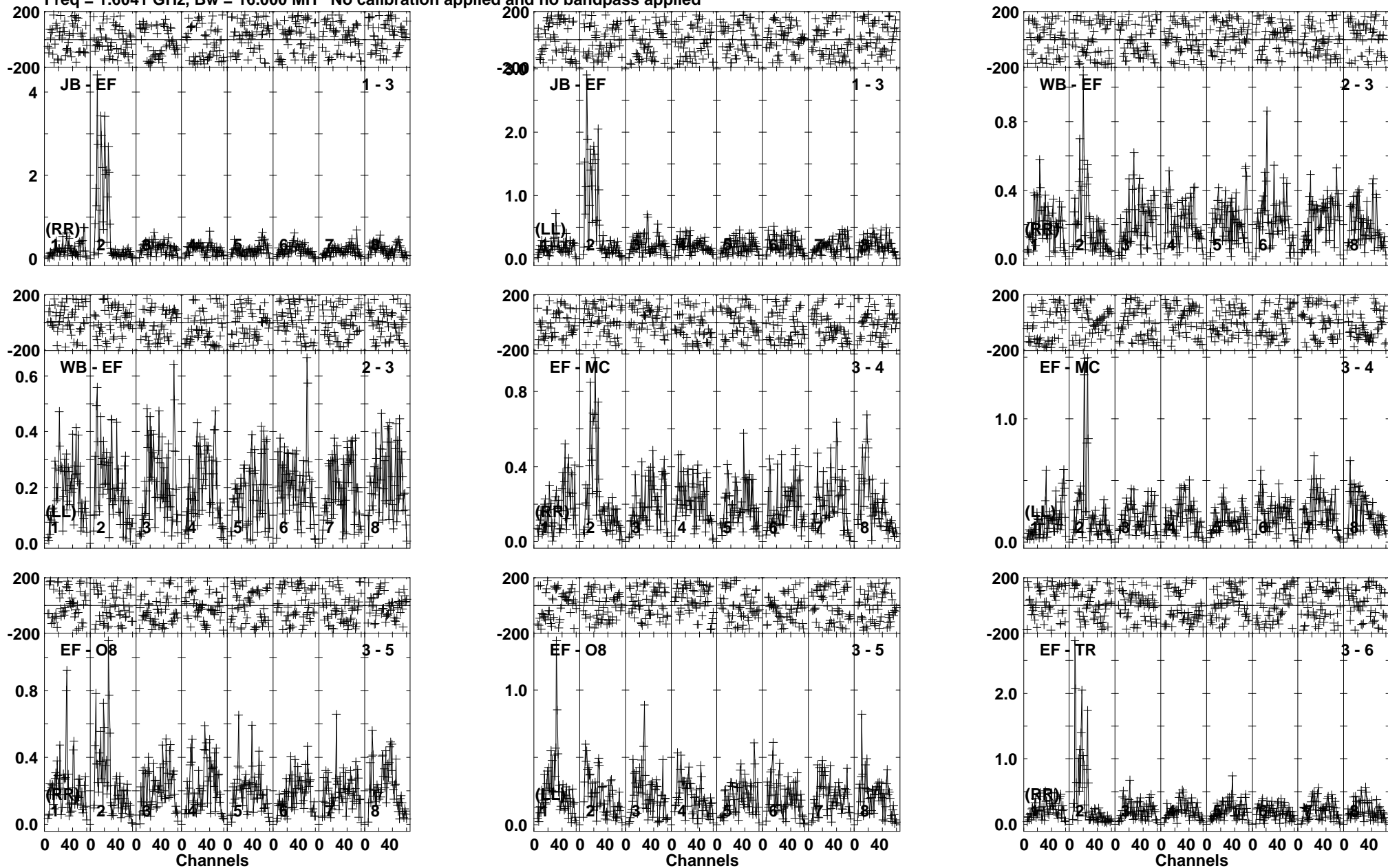
Lower frame: Milli Ampl Jy Top frame: Phas deg Vector averaged cross-power spectrum Baseline: JB (01) - EF (03) Timerange: 01/01:26:01 to 01/01:27:43
