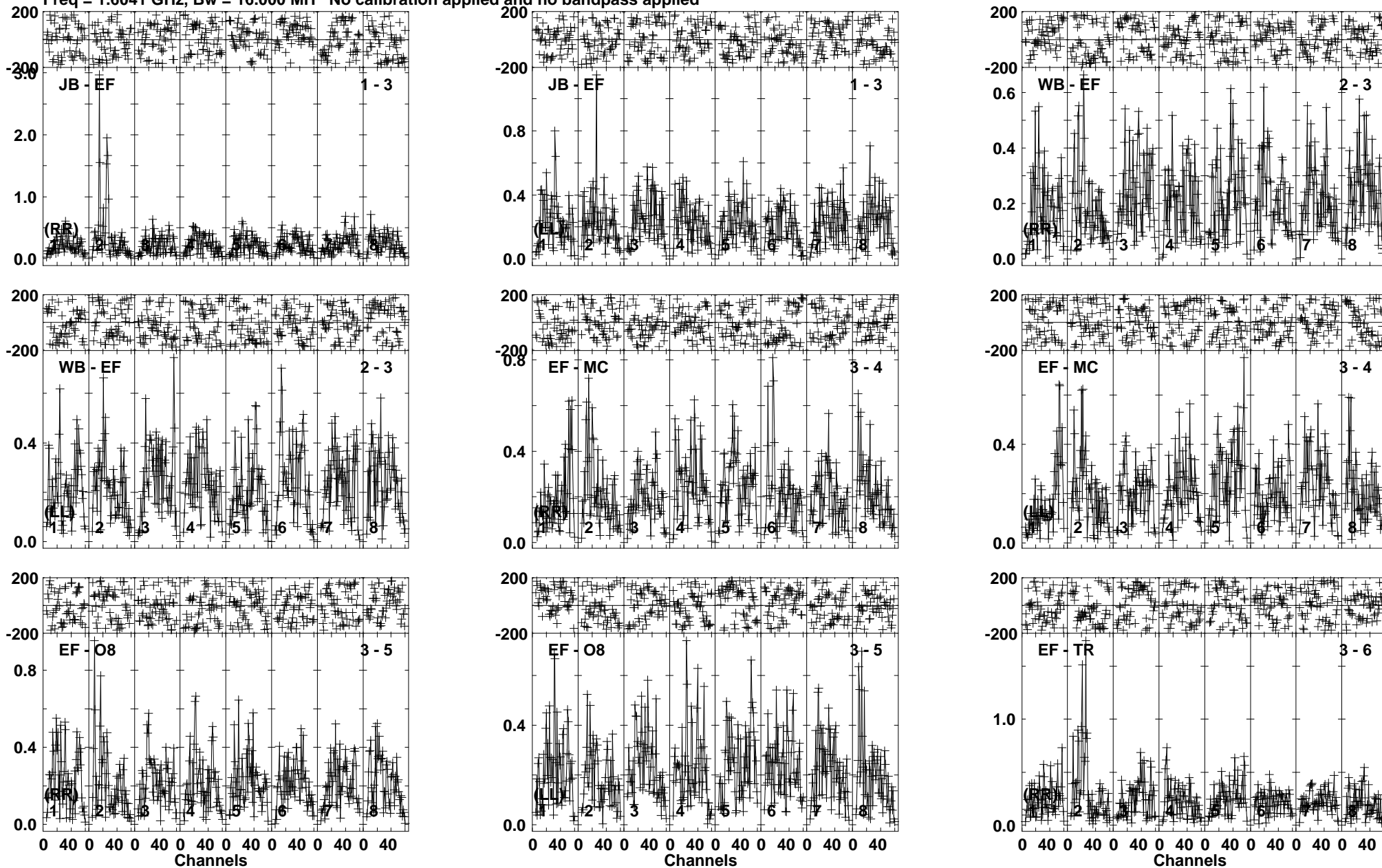
Lower frame: Milli Ampl Jy Top frame: Phas deg Vector averaged cross-power spectrum Baseline: JB (01) - EF (03) Timerange: 01/02:10:31 to 01/02:12:13
