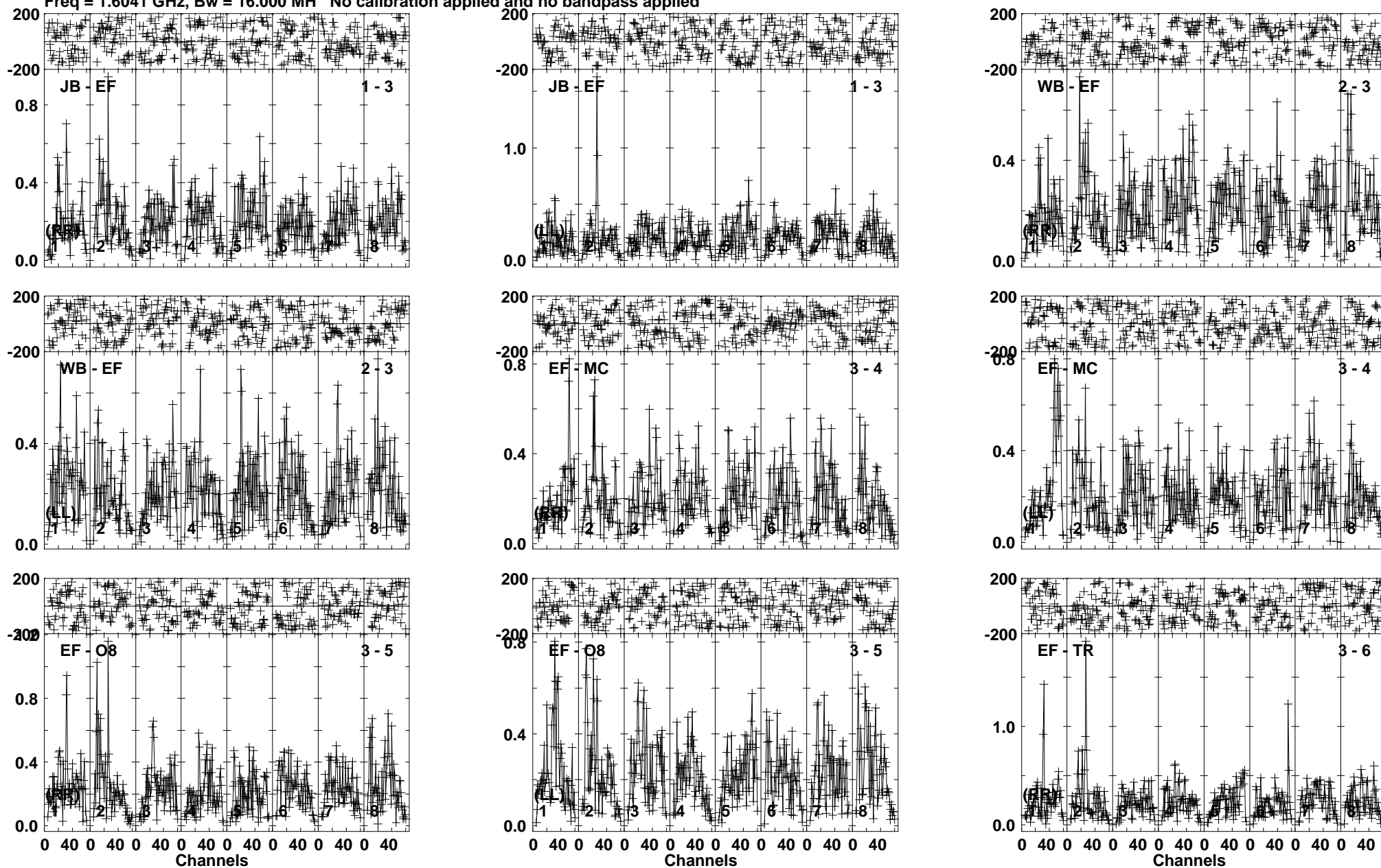
Lower frame: Milli Ampl Jy Top frame: Phas deg Vector averaged cross-power spectrum Baseline: JB (01) - EF (03) Timerange: 01/02:28:16 to 01/02:29:58
