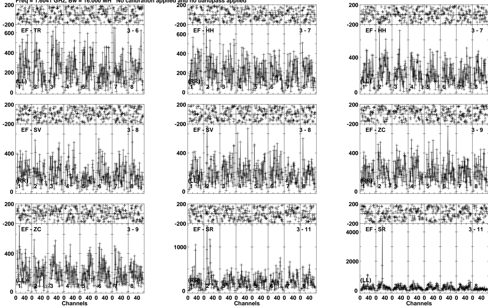
Lower frame: Micro Ampl Jy Top frame: Phas deg Vector averaged cross-power spectrum Baseline: EF (03) - TR (06) Timerange: 01/02:07:16 to 01/02:08:58
