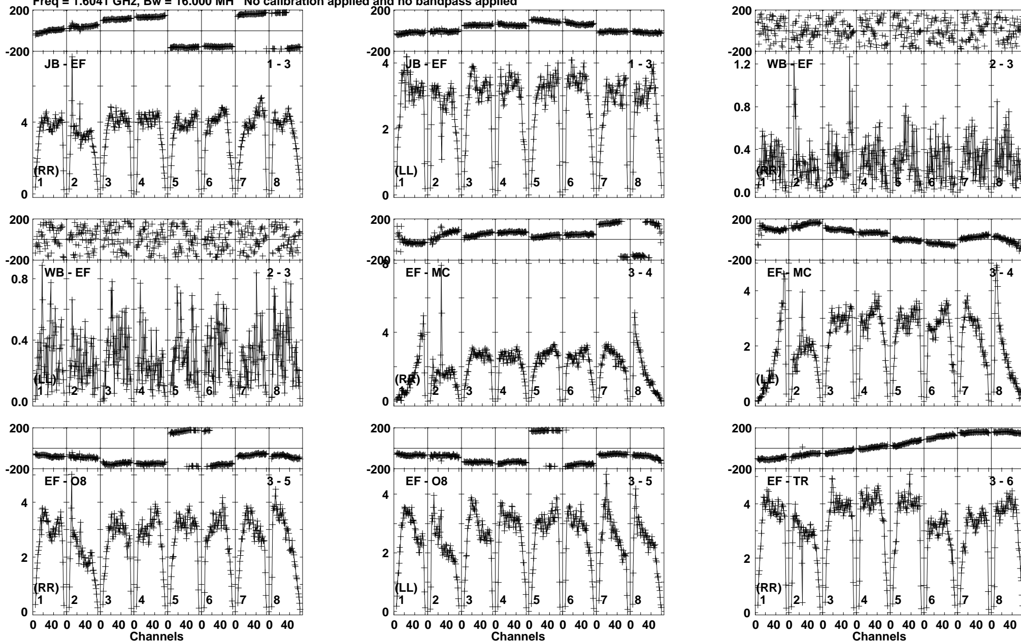
Lower frame: Milli Ampl Jy Top frame: Phas deg Vector averaged cross-power spectrum Baseline: JB (01) - EF (03) Timerange: 01/01:55:16 to 01/01:56:44
