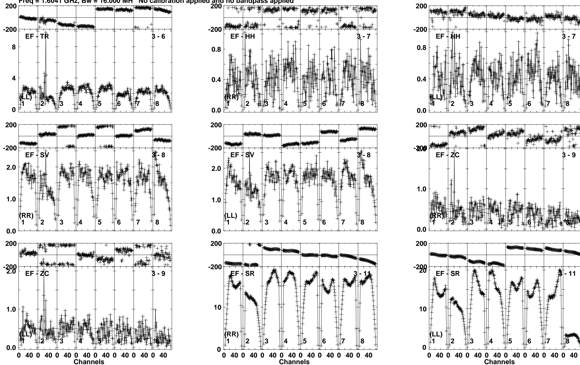
Lower frame: Milli Ampl Jy Top frame: Phas deg Vector averaged cross-power spectrum Baseline: EF (03) - TR (06) Timerange: 01/02:02:31 to 01/02:03:59
