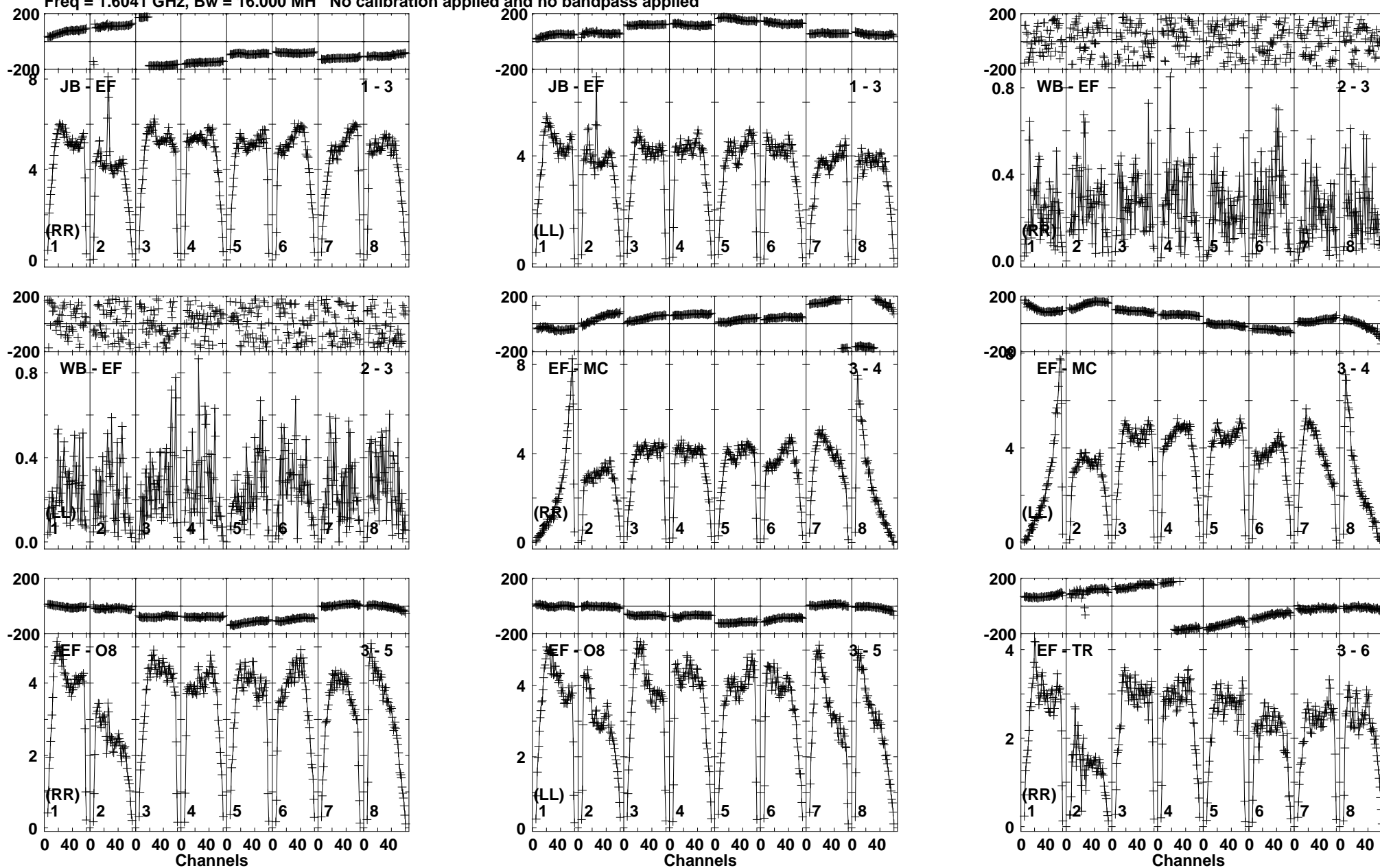
Lower frame: Milli Ampl Jy Top frame: Phas deg Vector averaged cross-power spectrum Baseline: JB (01) - EF (03) Timerange: 01/01:35:01 to 01/01:36:29
