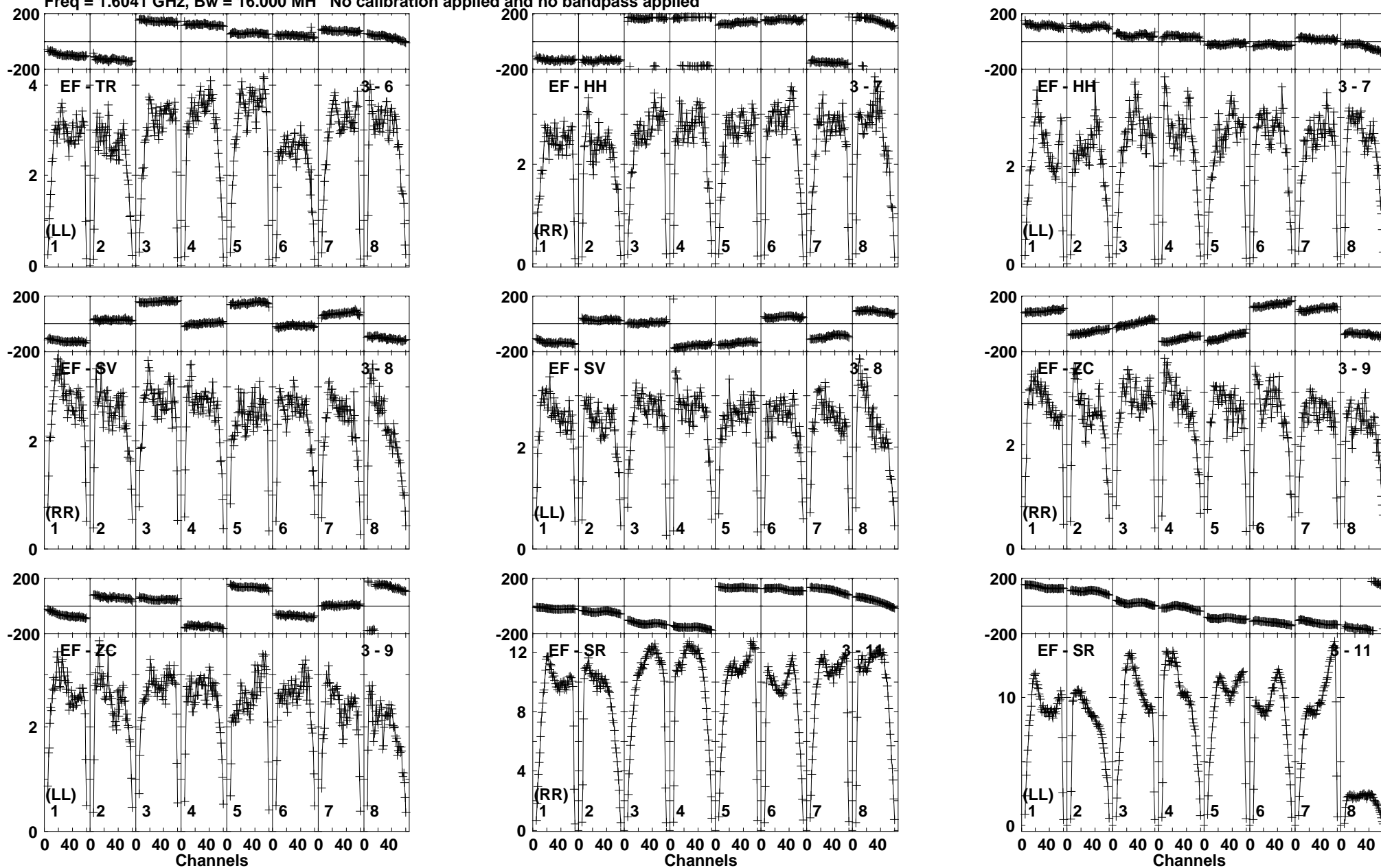
Lower frame: Milli Ampl Jy Top frame: Phas deg Vector averaged cross-power spectrum Baseline: EF (03) - TR (06) Timerange: 01/01:41:31 to 01/01:42:59
