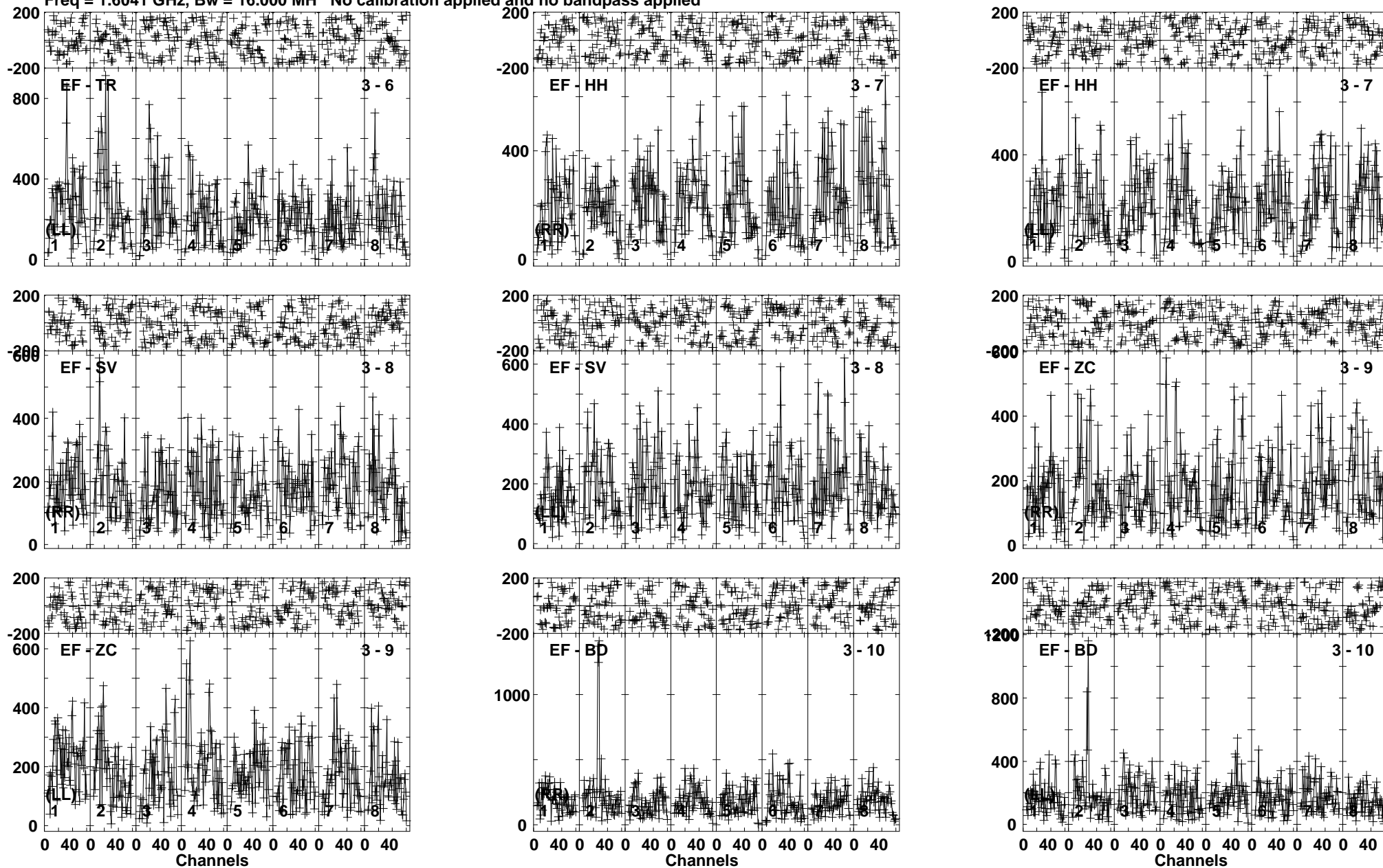
Lower frame: Micro Ampl Jy Top frame: Phas deg Vector averaged cross-power spectrum Baseline: EF (03) - TR (06) Timerange: 00/22:22:46 to 00/22:24:28
