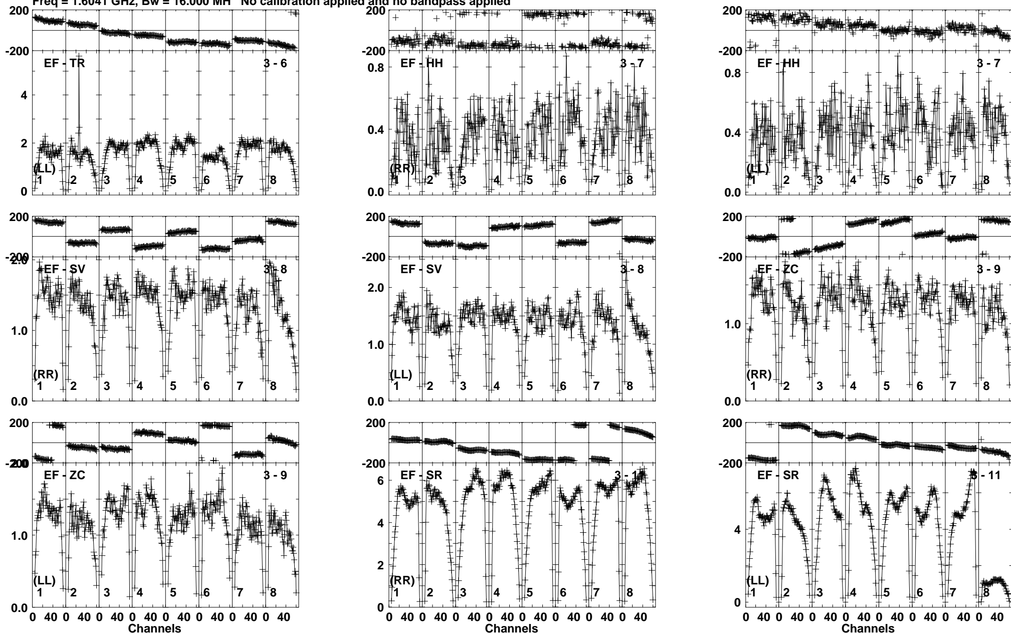
Lower frame: Milli Ampl Jy Top frame: Phas deg Vector averaged cross-power spectrum Baseline: EF (03) - TR (06) Timerange: 01/01:04:16 to 01/01:05:44
