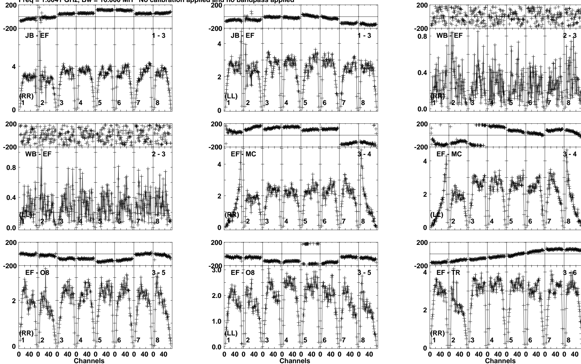
Lower frame: Milli Ampl Jy Top frame: Phas deg Vector averaged cross-power spectrum Baseline: JB (01) - EF (03) Timerange: 00:22:44:46 to 00:22:46:14
