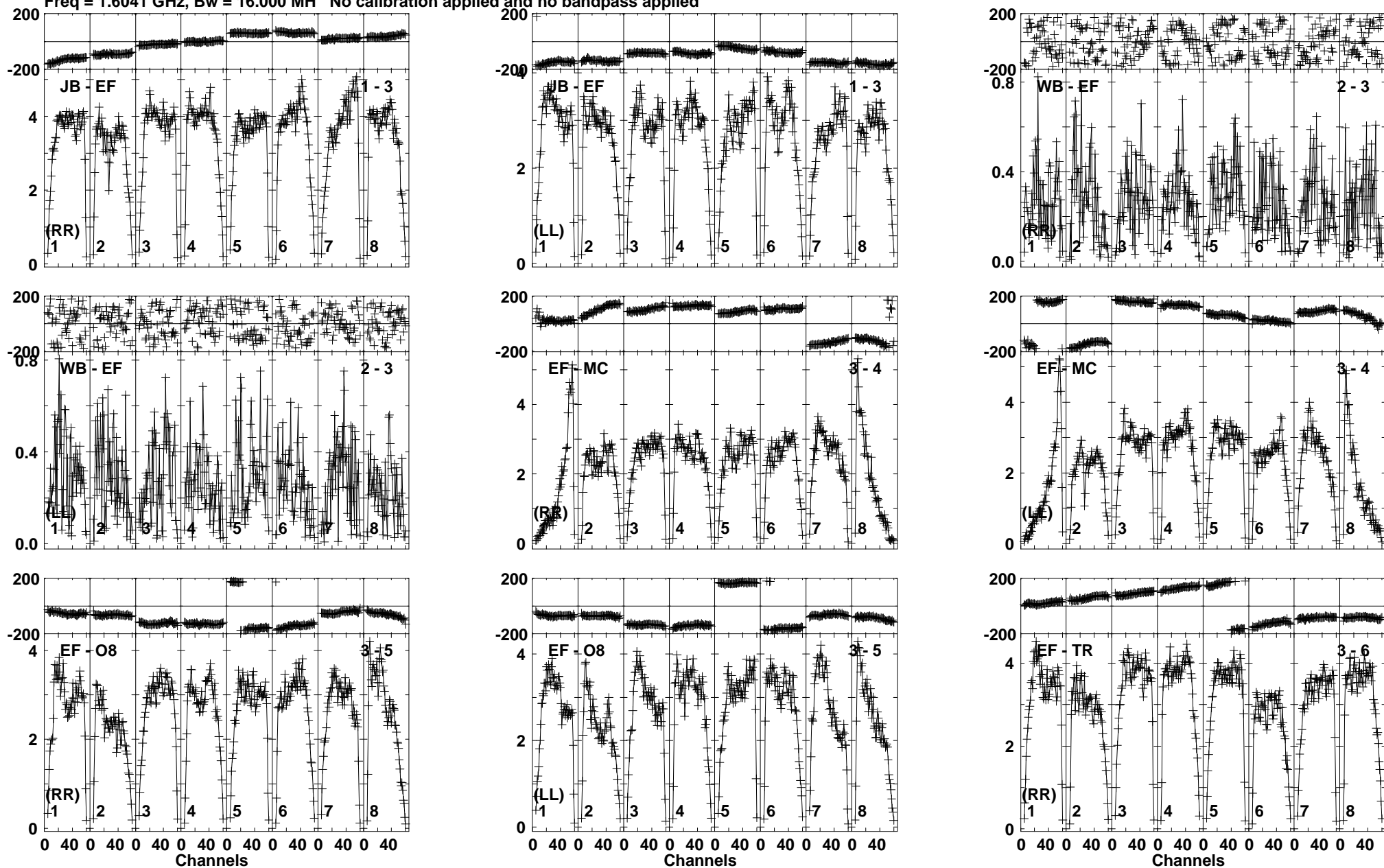
Lower frame: Milli Ampl Jy Top frame: Phas deg Vector averaged cross-power spectrum Baseline: JB (01) - EF (03) Timerange: 01/00:46:31 to 01/00:47:59
