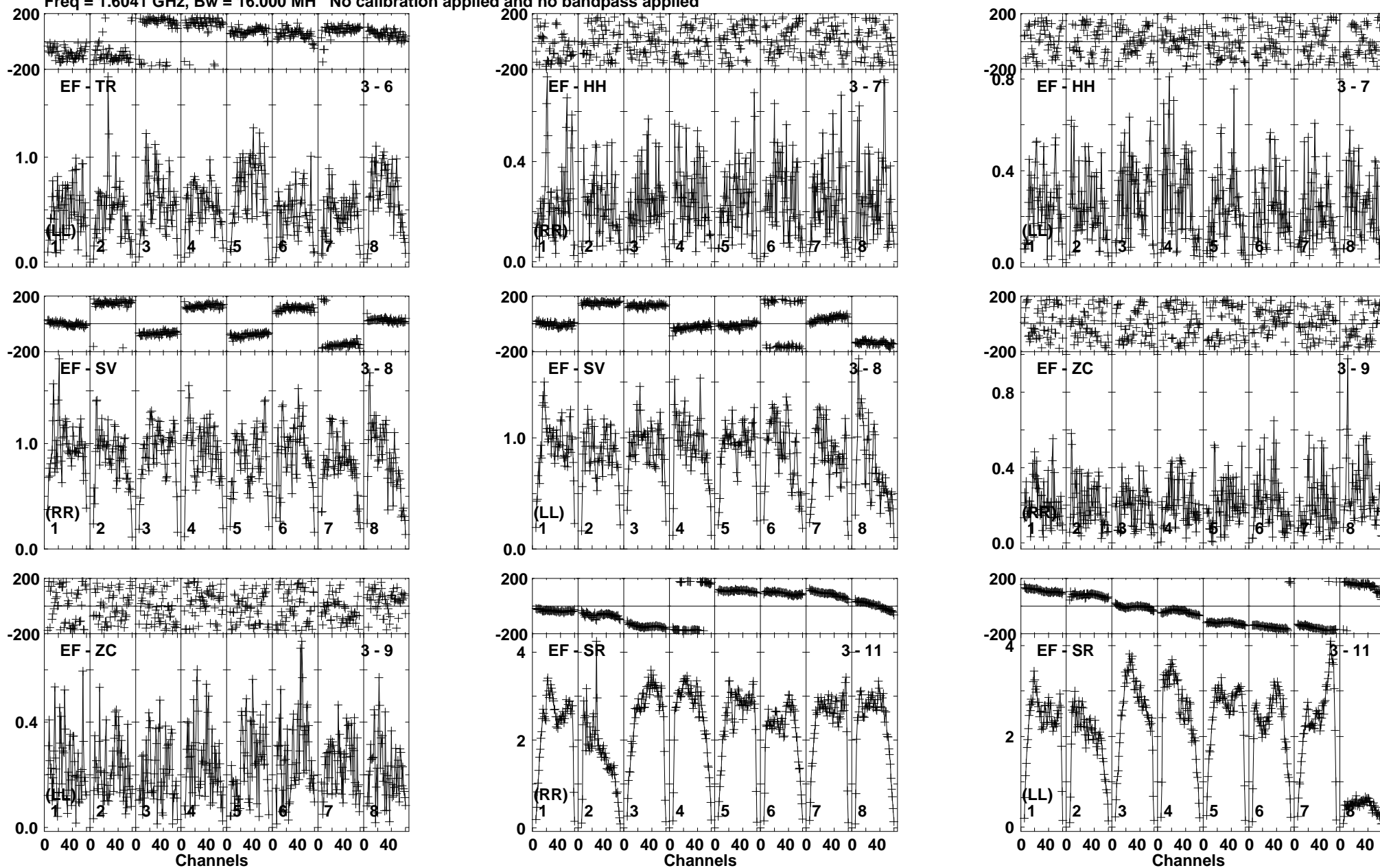
Lower frame: Milli Ampl Jy Top frame: Phas deg Vector averaged cross-power spectrum Baseline: EF (03) - TR (06) Timerange: 01/02:05:46 to 01/02:07:14
