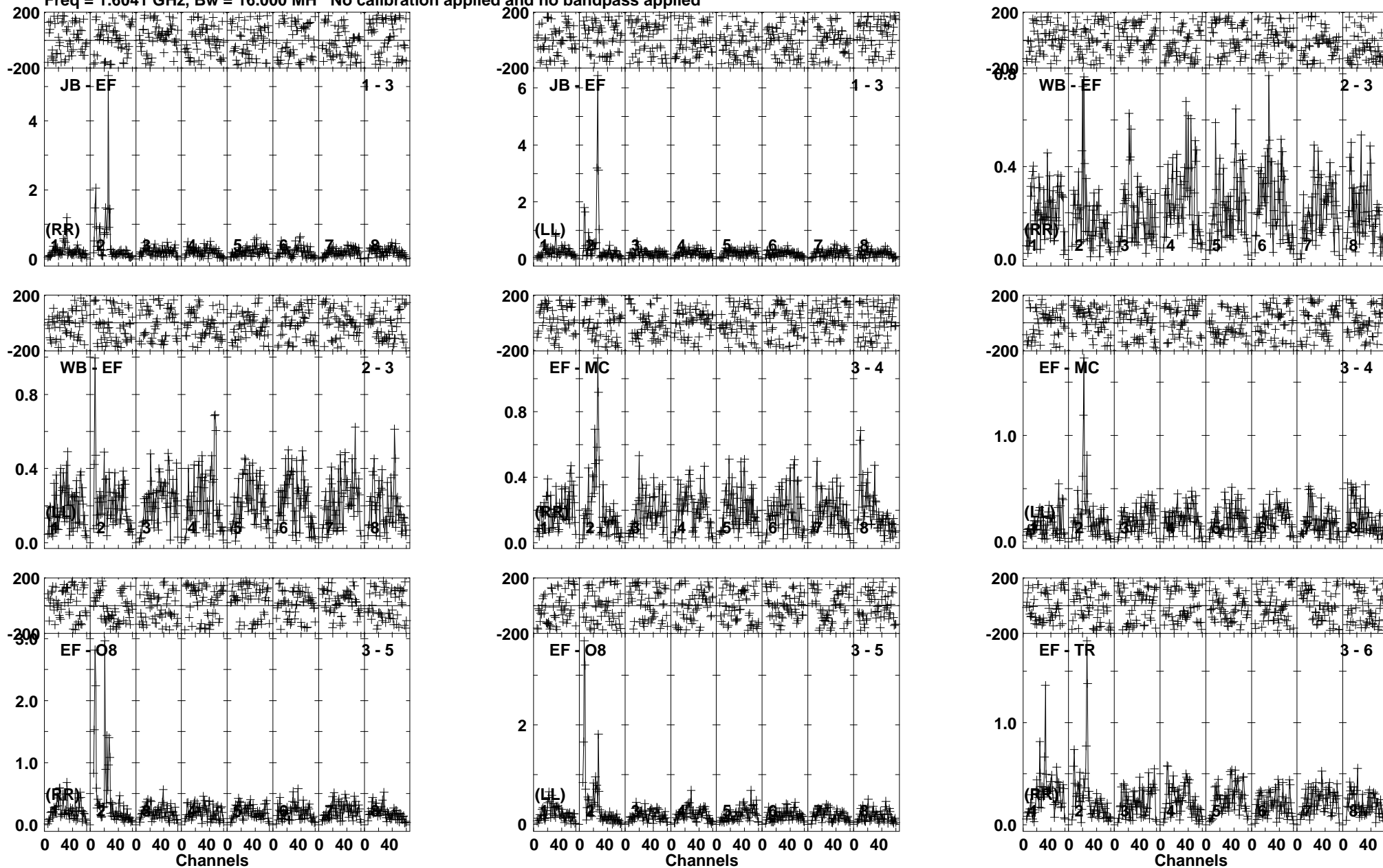
Lower frame: Milli Ampl Jy Top frame: Phas deg Vector averaged cross-power spectrum Baseline: JB (01) - EF (03) Timerange: 01/02:31:31 to 01/02:33:13
