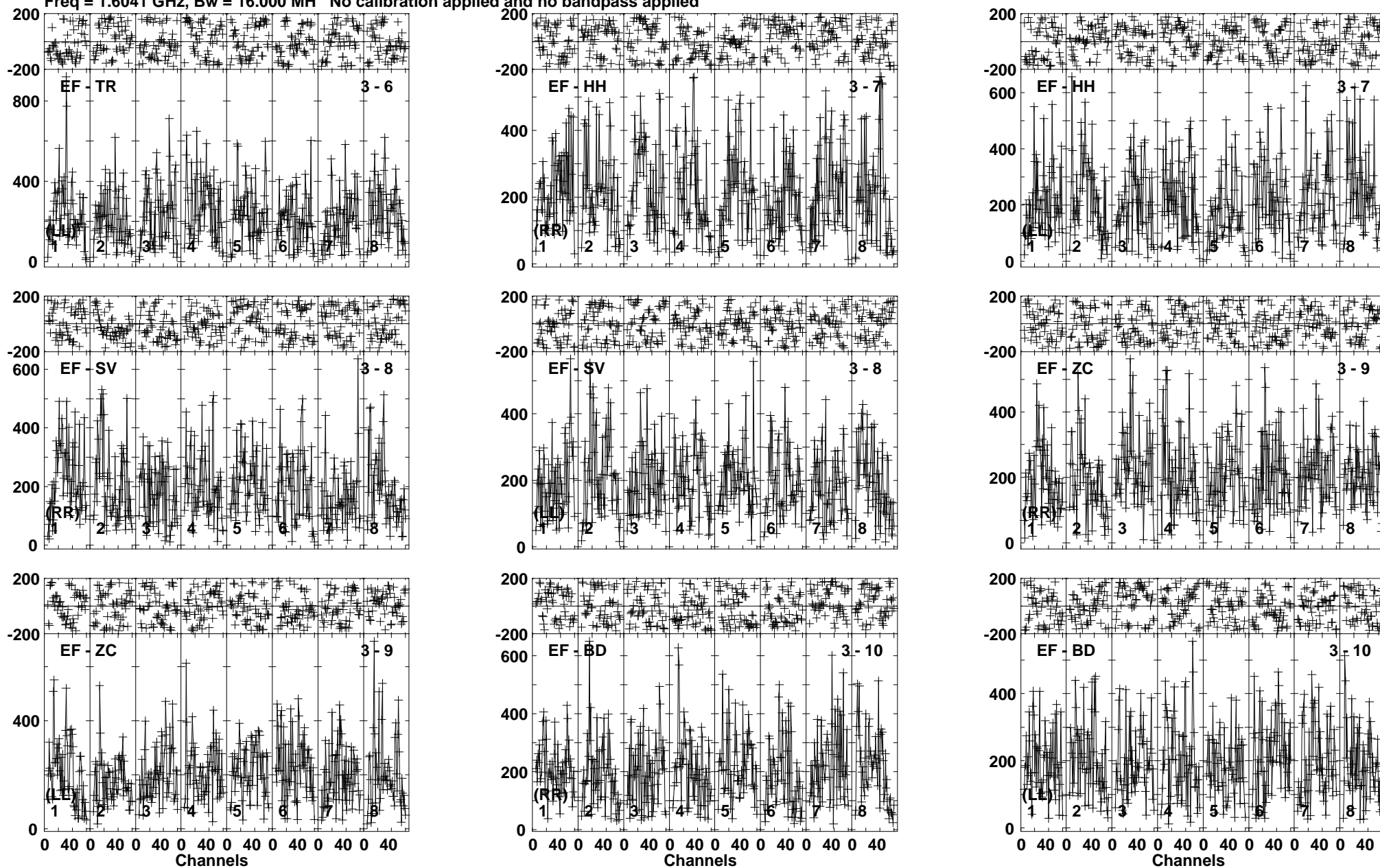
Lower frame: Micro Ampl Jy Top frame: Phas deg Vector averaged cross-power spectrum Baseline: EF (03) - TR (06) Timerange: 00/23:24:16 to 00/23:25:58
