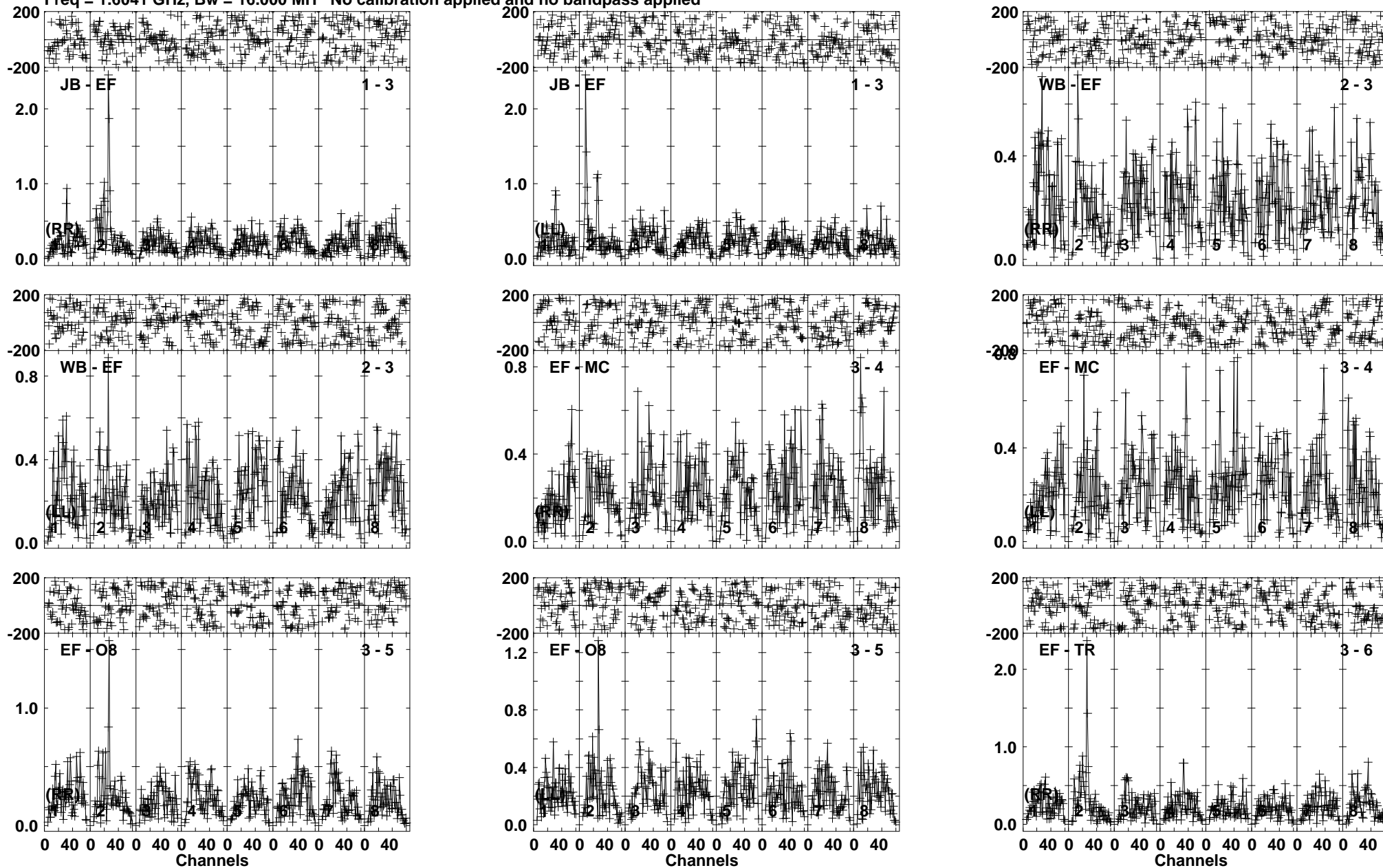
Lower frame: Milli Ampl Jy Top frame: Phas deg Vector averaged cross-power spectrum Baseline: JB (01) - EF (03) Timerange: 01/00:48:01 to 01/00:49:43
