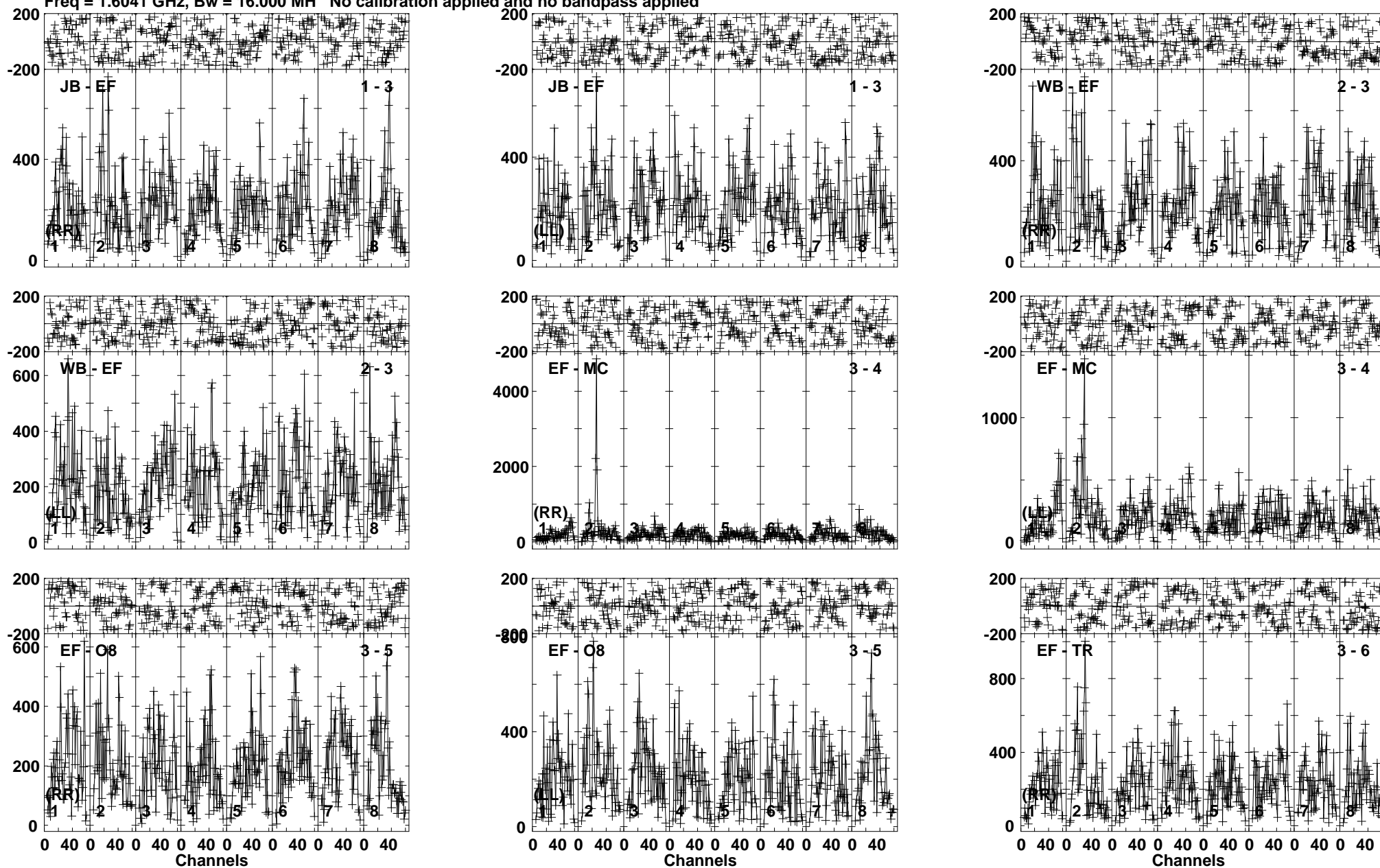
Lower frame: Micro Ampl Jy Top frame: Phas deg Vector averaged cross-power spectrum Baseline: JB (01) - EF (03) Timerange: 01/01:39:46 to 01/01:41:28
