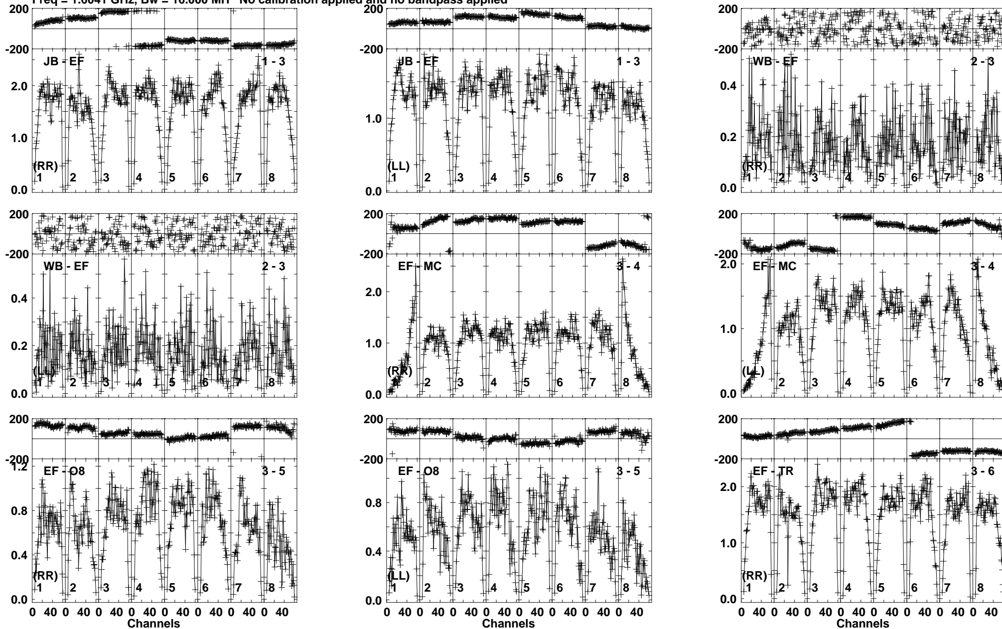
Lower frame: Milli Ampl Jy Top frame: Phas deg Vector averaged cross-power spectrum Baseline: JB (01) - EF (03) Timerange: 00/22:21:16 to 00/22:22:44
