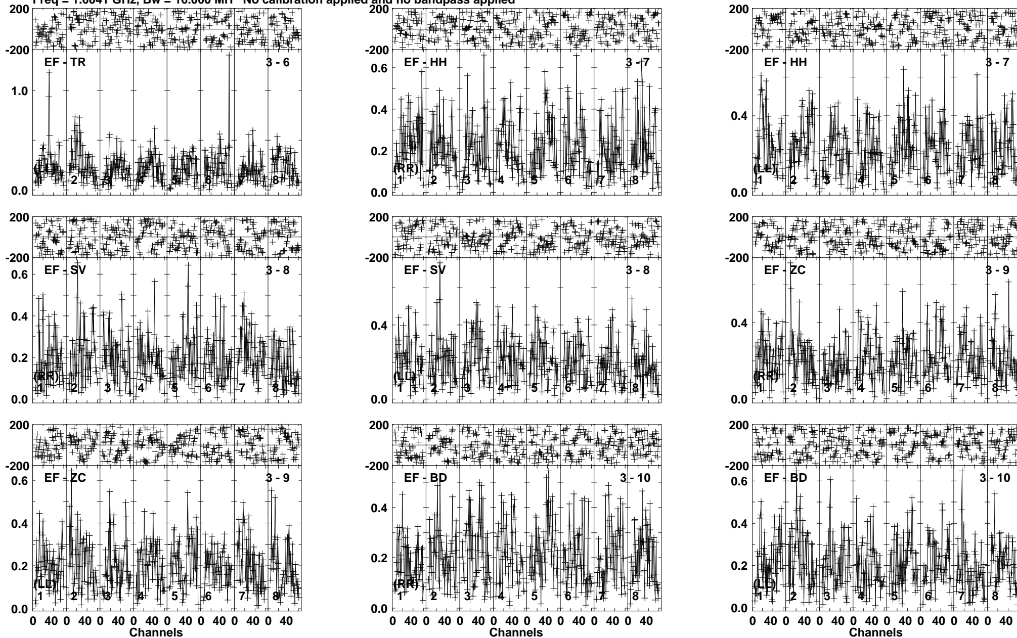
Lower frame: Milli Ampl Jy Top frame: Phas deg Vector averaged cross-power spectrum Baseline: EF (03) - TR (06) Timerange: 00/23:21:01 to 00/23:22:43
