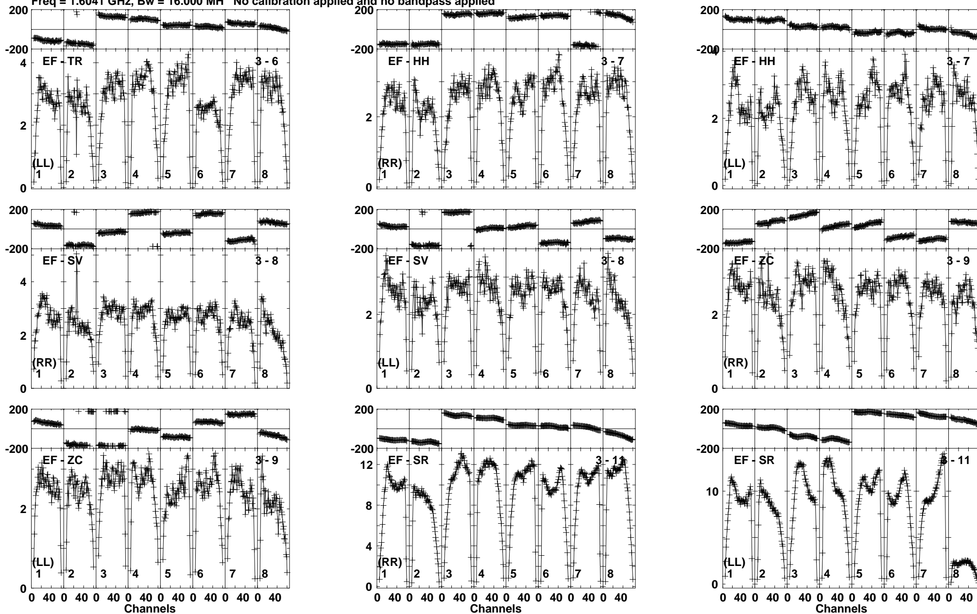
Lower frame: Milli Ampl Jy Top frame: Phas deg Vector averaged cross-power spectrum Baseline: EF (03) - TR (06) Timerange: 01/01:55:16 to 01/01:56:44
