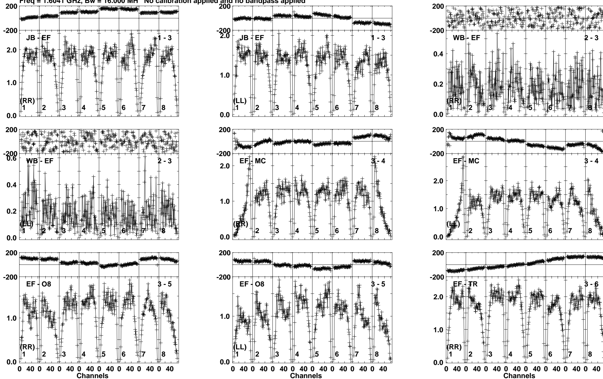
Lower frame: Milli Ampl Jy Top frame: Phas deg Vector averaged cross-power spectrum Baseline: JB (01) - EF (03) Timerange: 00:22:48:46 to 00:22:50:14
