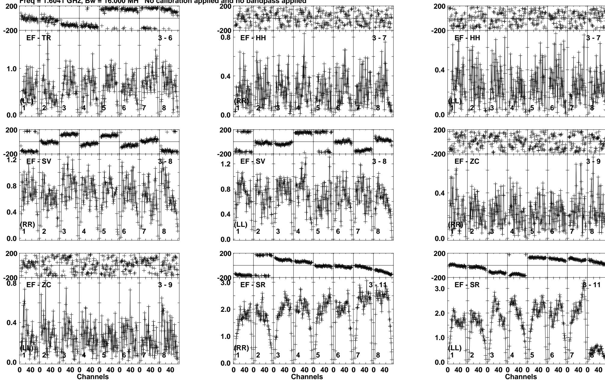
Lower frame: Milli Ampl Jy Top frame: Phas deg Vector averaged cross-power spectrum Baseline: EF (03) - TR (06) Timerange: 01/01:24:31 to 01/01:25:59
