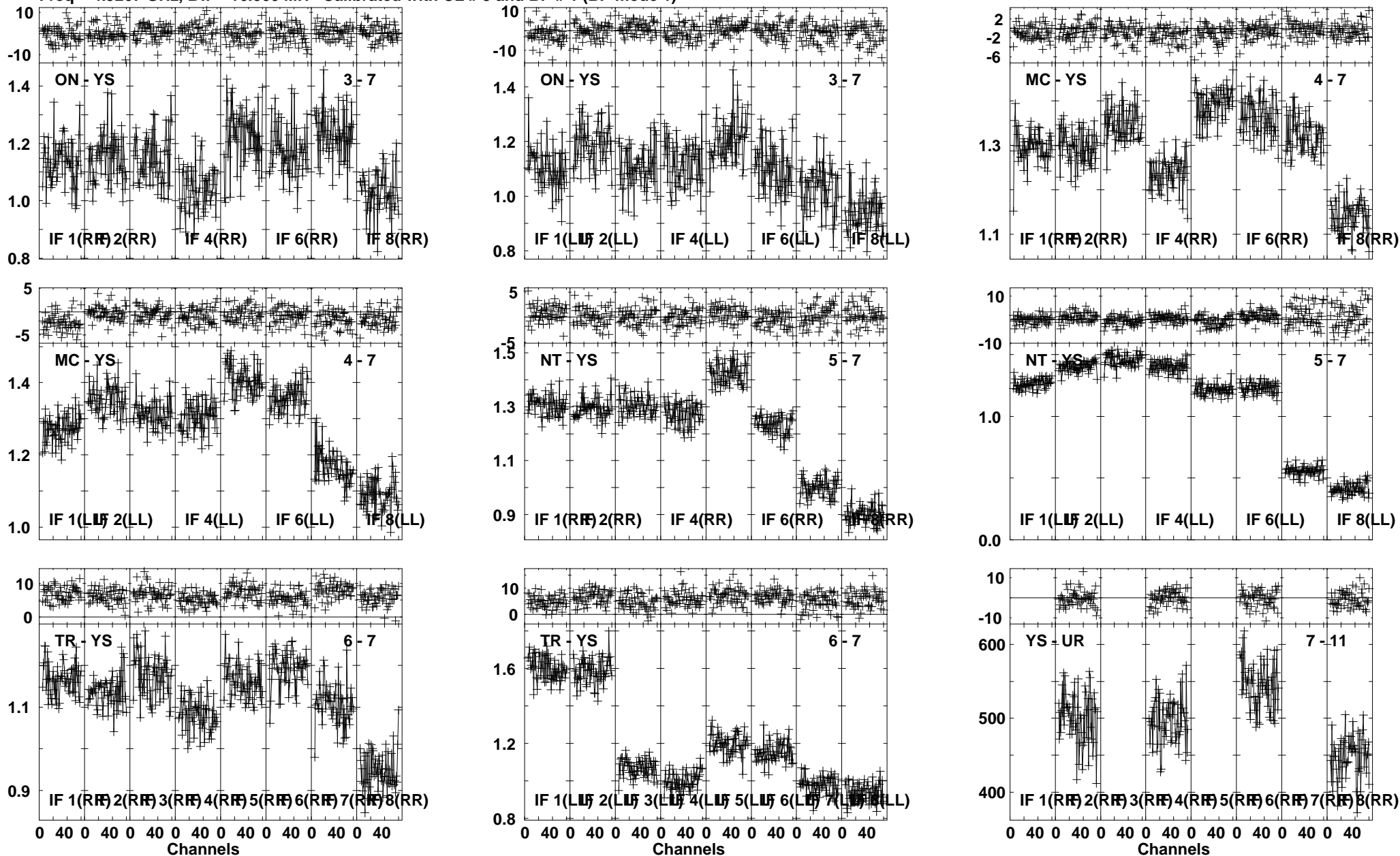
Lower frame: Ampl Jy Top frame: Phas deg Vector averaged cross-power spectrum Several baselines displayed Timerange: 00/03:52:40 to 00/03:53:40
