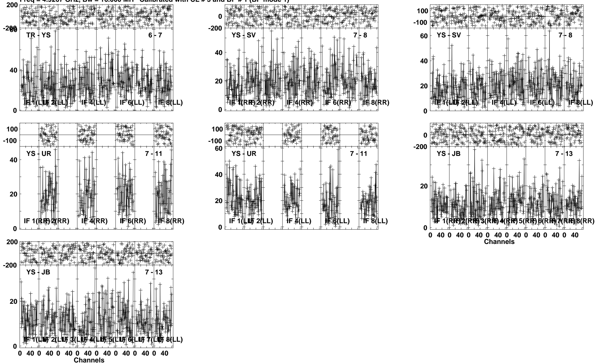
Lower frame: Milli Ampl Jy Top frame: Phas deg Vector averaged cross-power spectrum Several baselines displayed Timerange: 00/10/31:21 to 00/10/37:29
