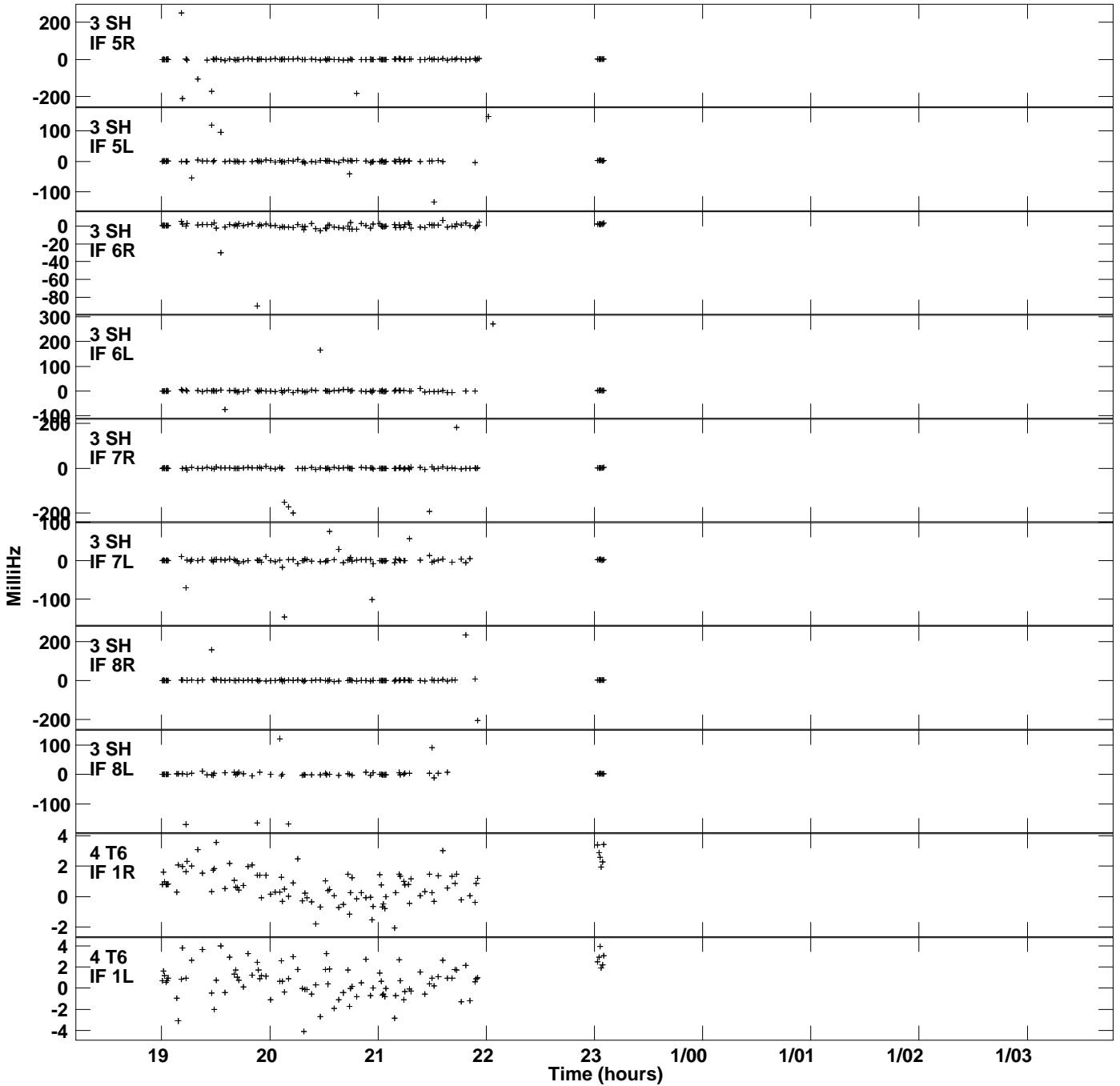
Plot file version 5 created 16-FEB-2016 14:15:38 Rate vs UTC time for EY023.UVDATA.1 SN 2 Rpol & Lpol IF 1 - 8
