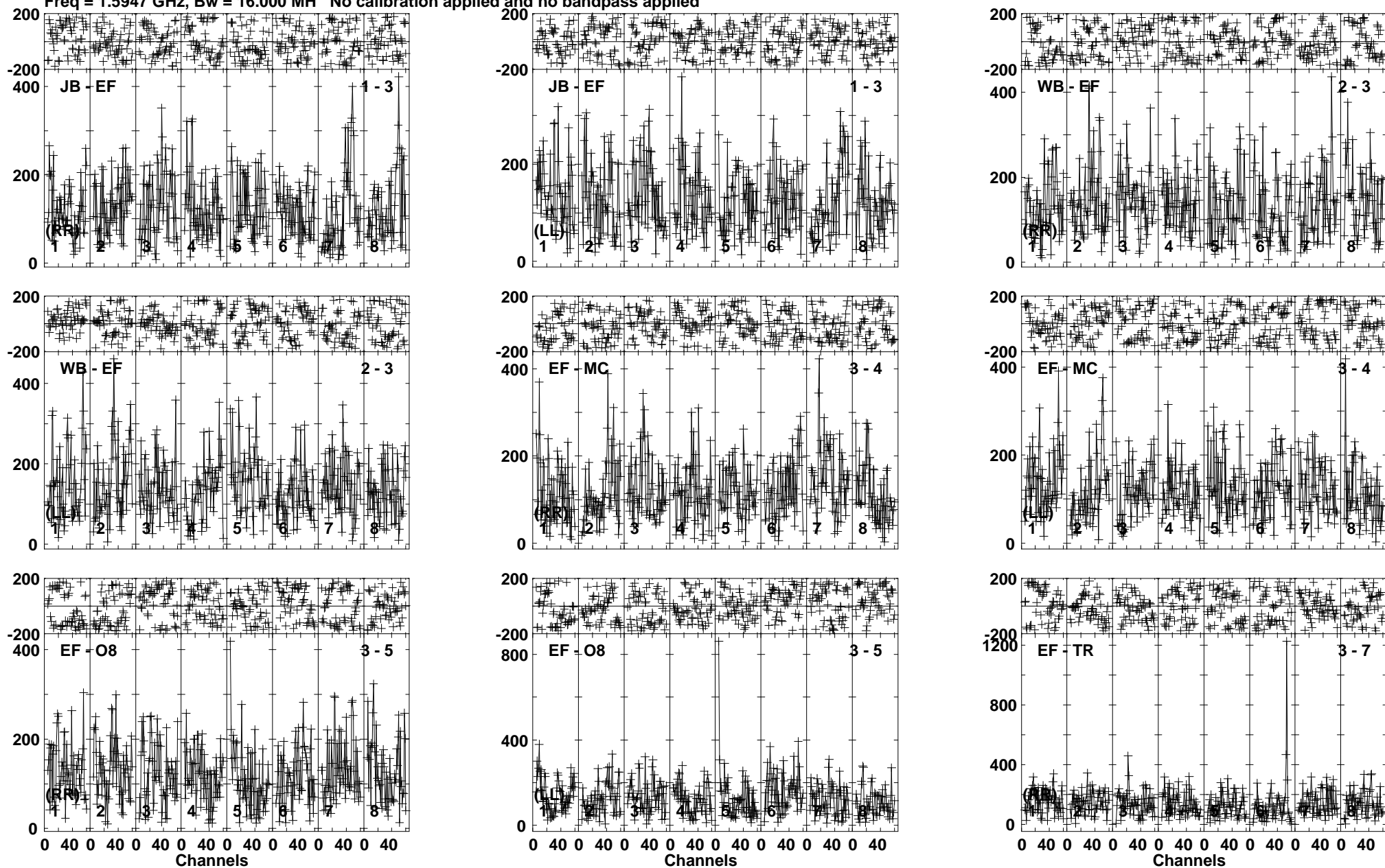
Lower frame: Micro Ampl Jy Top frame: Phas deg Vector averaged cross-power spectrum Baseline: JB (01) - EF (03) Timerange: 00/03:16:21 to 00/03:19:09
