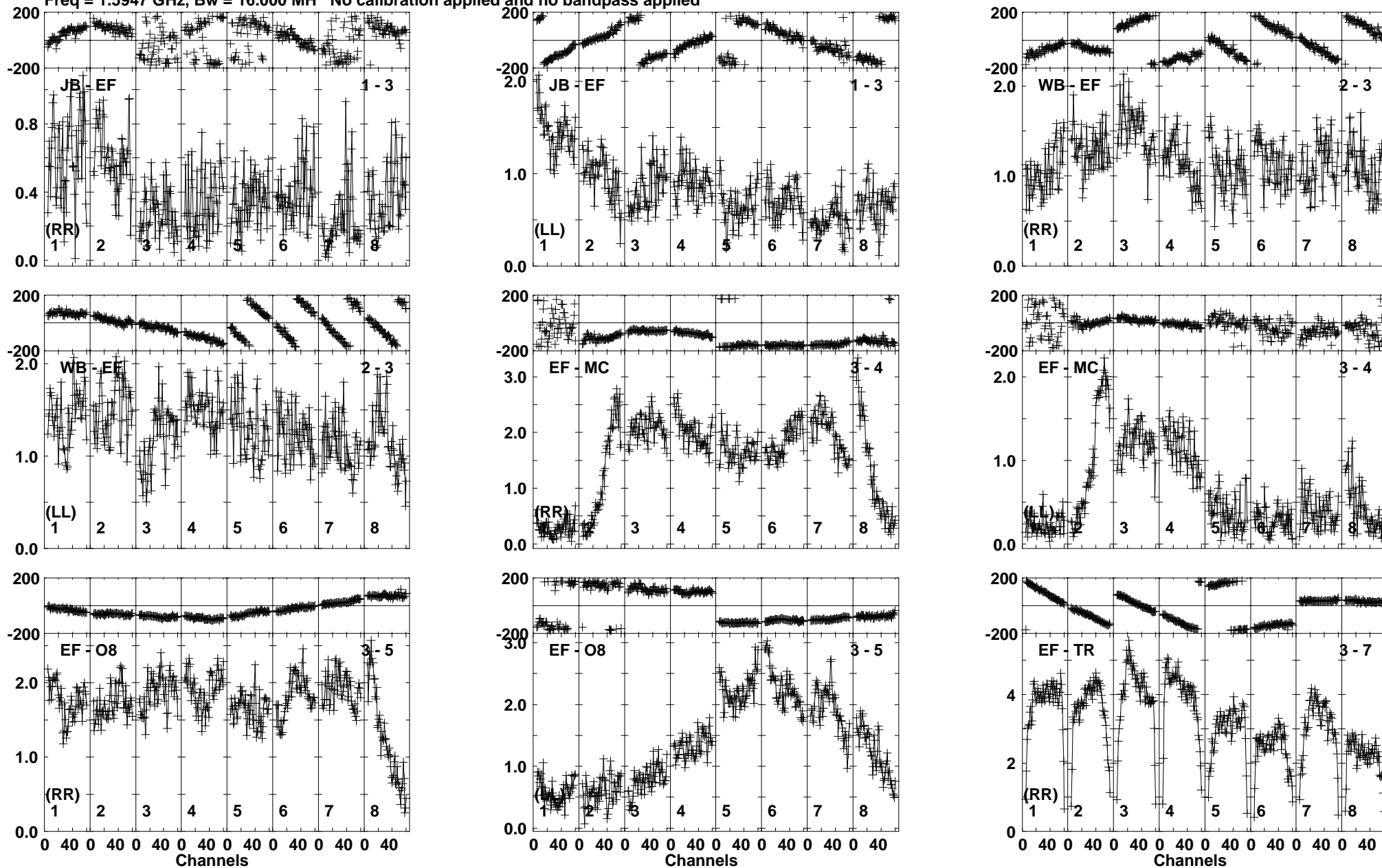
Lower frame: Milli Ampl Jy Top frame: Phas deg Vector averaged cross-power spectrum Baseline: JB (01) - EF (03) Timerange: 00/04:37:11 to 00/04:38:19
