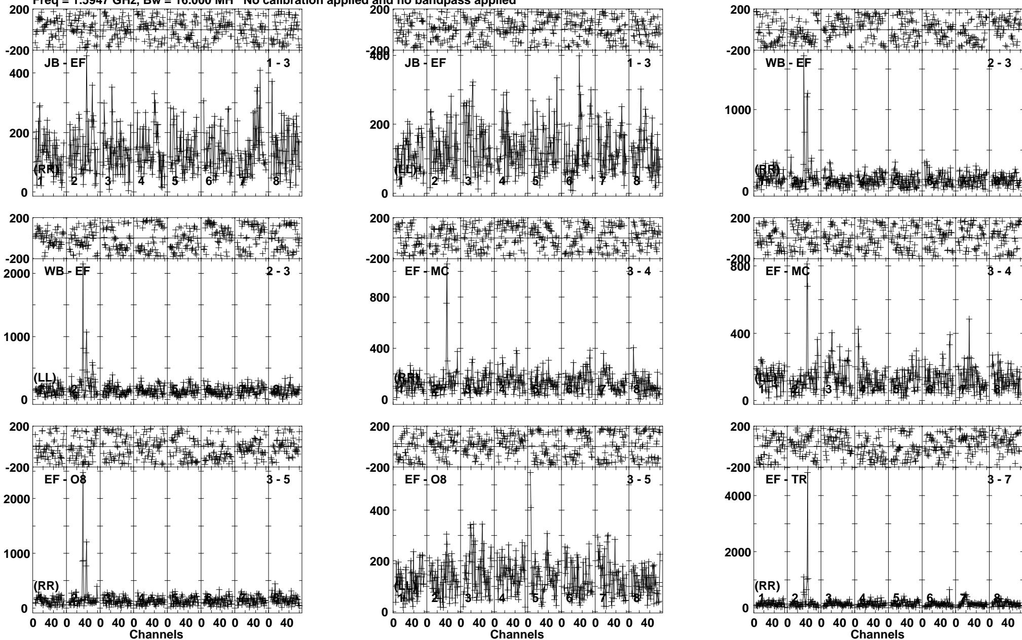
Lower frame: Micro Ampl Jy Top frame: Phas deg Vector averaged cross-power spectrum Baseline: JB (01) - EF (03) Timerange: 00/04:46:41 to 00/04:49:29
