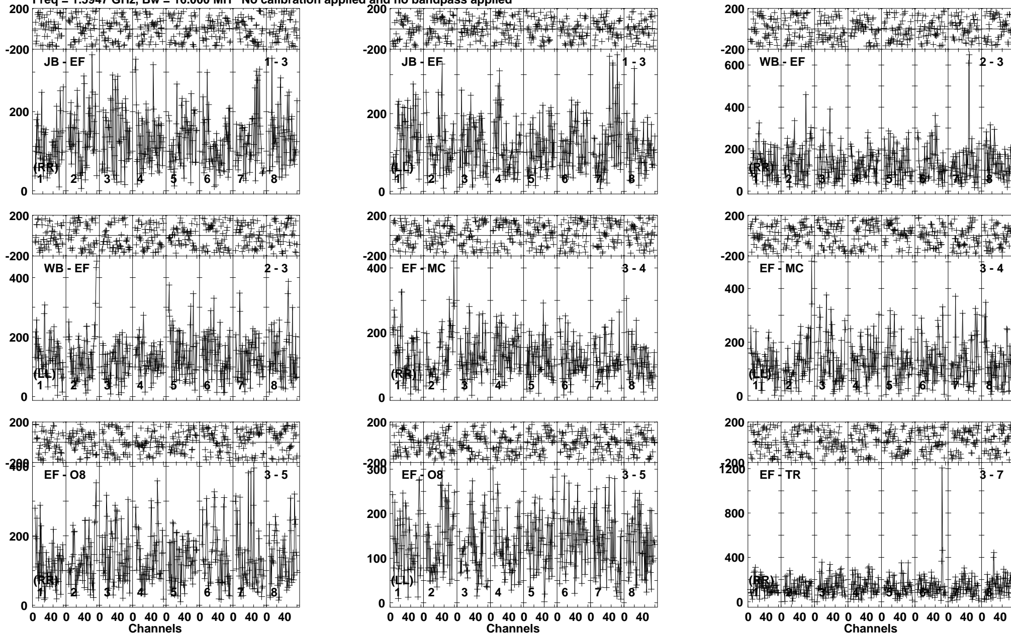
Lower frame: Micro Ampl Jy Top frame: Phas deg Vector averaged cross-power spectrum Baseline: JB (01) - EF (03) Timerange: 00/07:20:41 to 00/07:23:29
