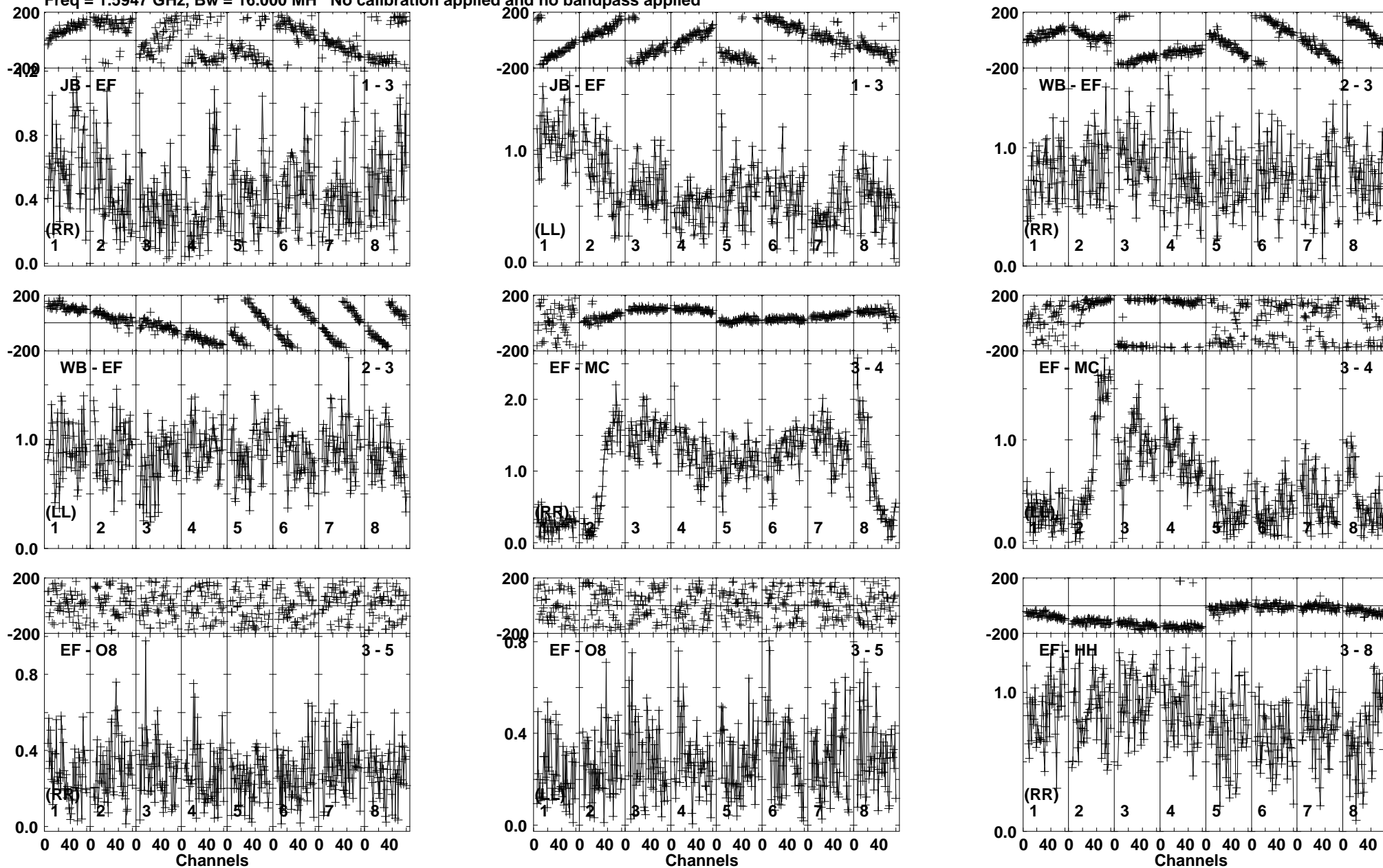
Lower frame: Milli Ampl Jy Top frame: Phas deg Vector averaged cross-power spectrum Baseline: JB (01) - EF (03) Timerange: 00/08:08:51 to 00/08:09:59
