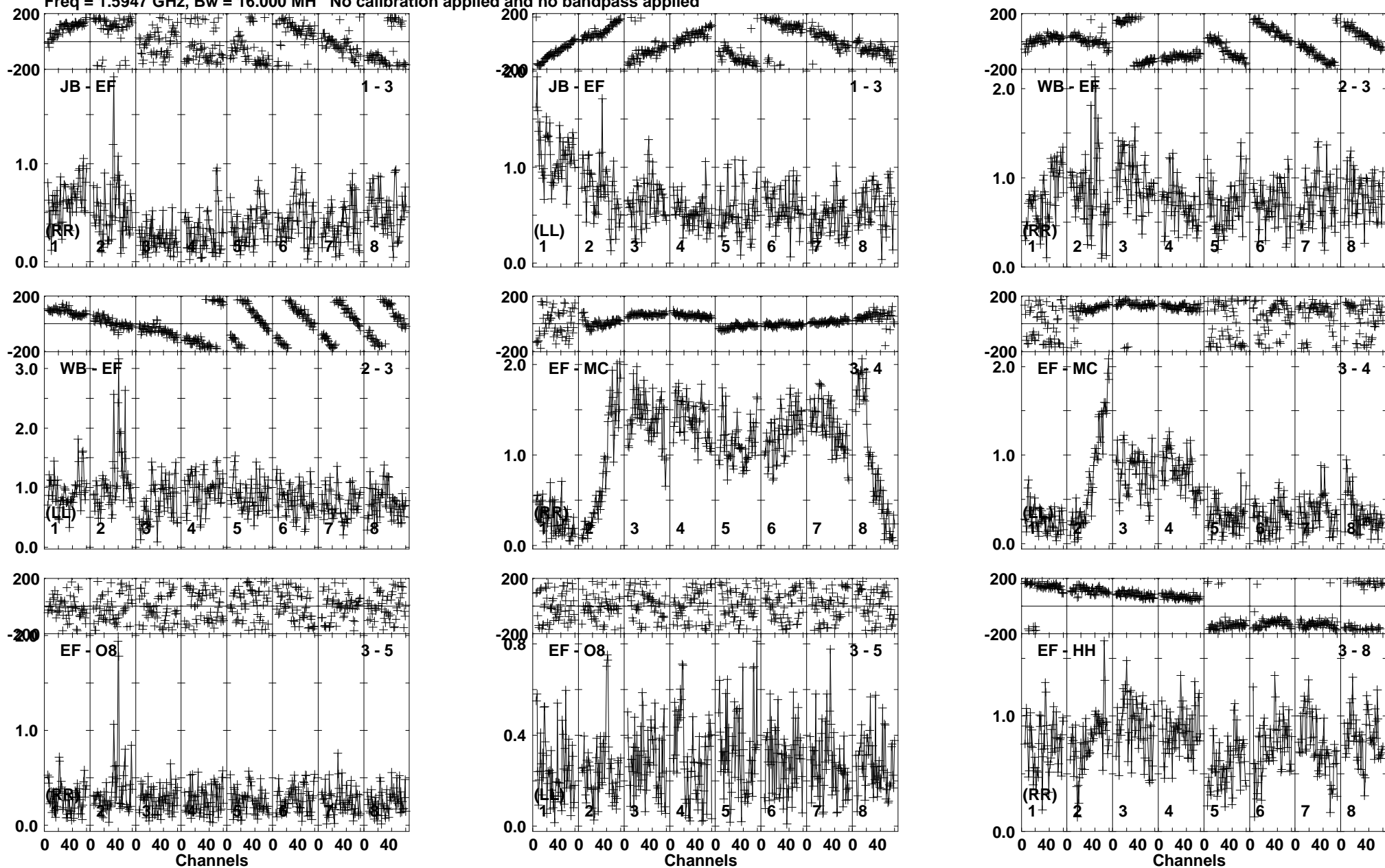
Lower frame: Milli Ampl Jy Top frame: Phas deg Vector averaged cross-power spectrum Baseline: JB (01) - EF (03) Timerange: 00/08:12:51 to 00/08:13:59
