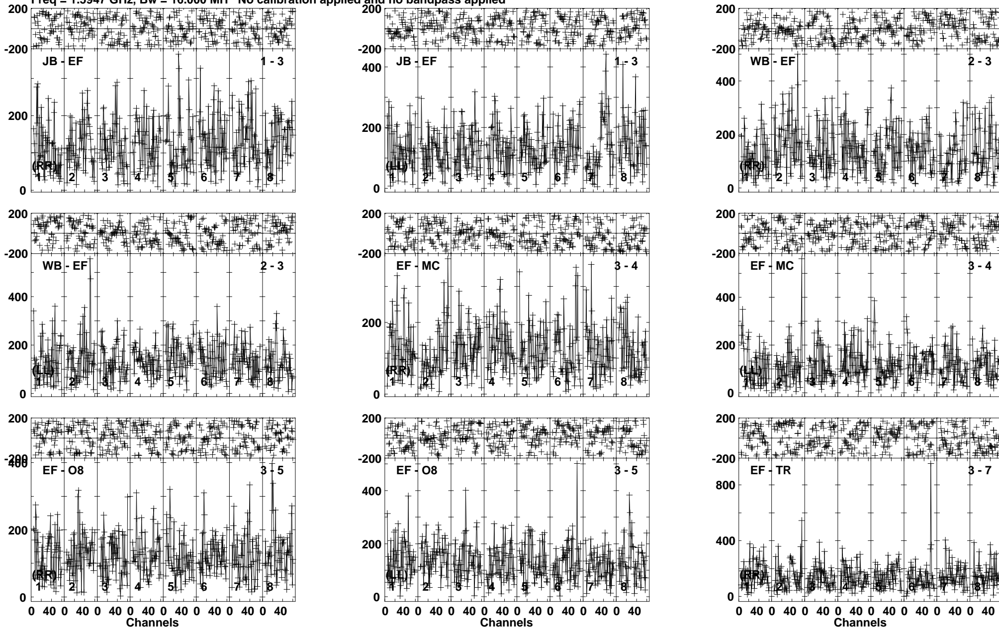
Lower frame: Micro Ampl Jy Top frame: Phas deg Vector averaged cross-power spectrum Baseline: JB (01) - EF (03) Timerange: 00/03:08:01 to 00/03:10:49
