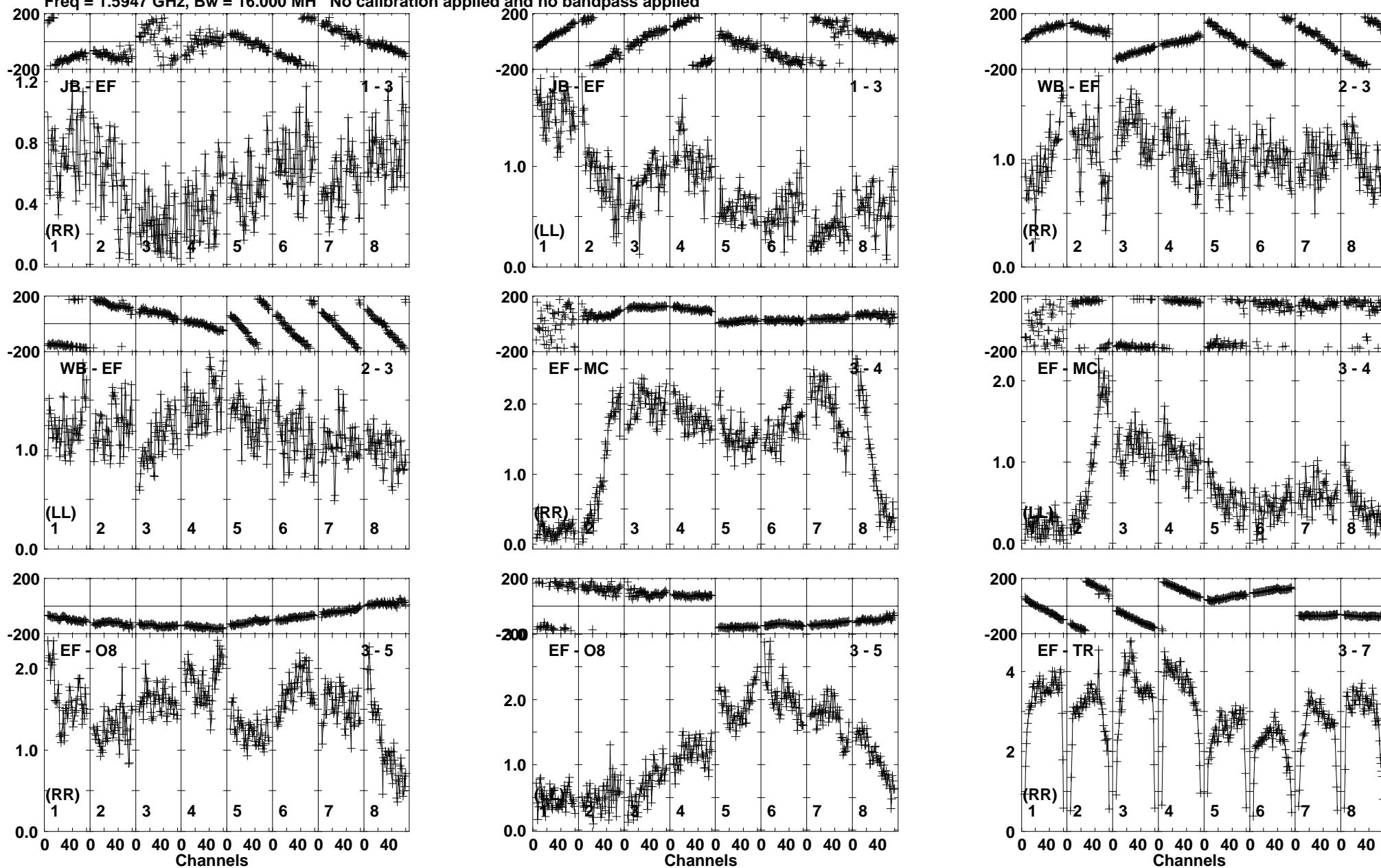
Lower frame: Milli Ampl Jy Top frame: Phas deg Vector averaged cross-power spectrum Baseline: JB (01) - EF (03) Timerange: 00/06:14:01 to 00/06:14:59
