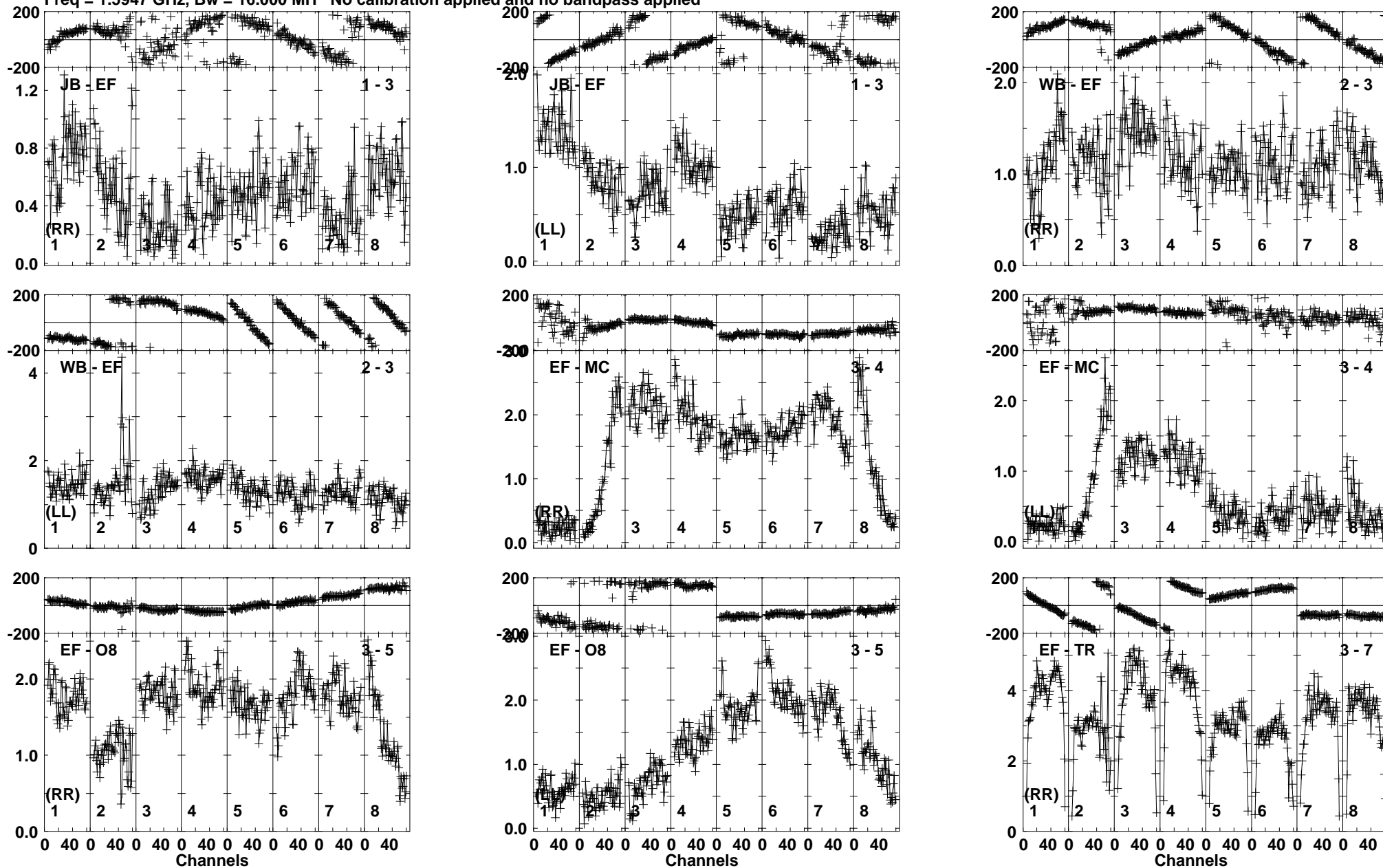
Lower frame: Milli Ampl Jy Top frame: Phas deg Vector averaged cross-power spectrum Baseline: JB (01) - EF (03) Timerange: 00/04:24:51 to 00/04:25:59
