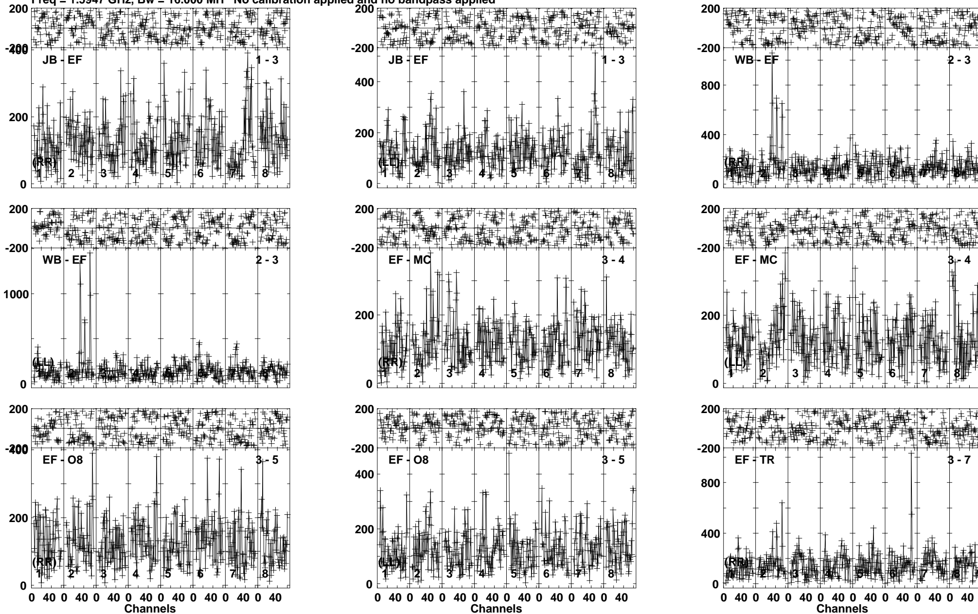
Lower frame: Micro Ampl Jy Top frame: Phas deg Vector averaged cross-power spectrum Baseline: JB (01) - EF (03) Timerange: 00/02:47:21 to 00/02:50:09
