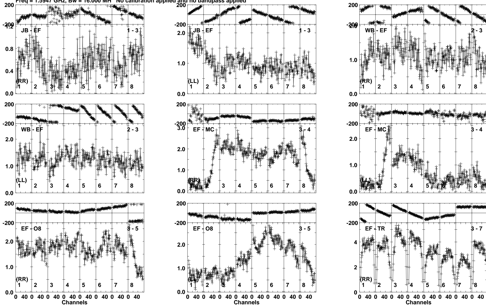
Lower frame: Milli Ampl Jy Top frame: Phas deg Vector averaged cross-power spectrum Baseline: JB (01) - EF (03) Timerange: 00/05:14:11 to 00/05:15:19
