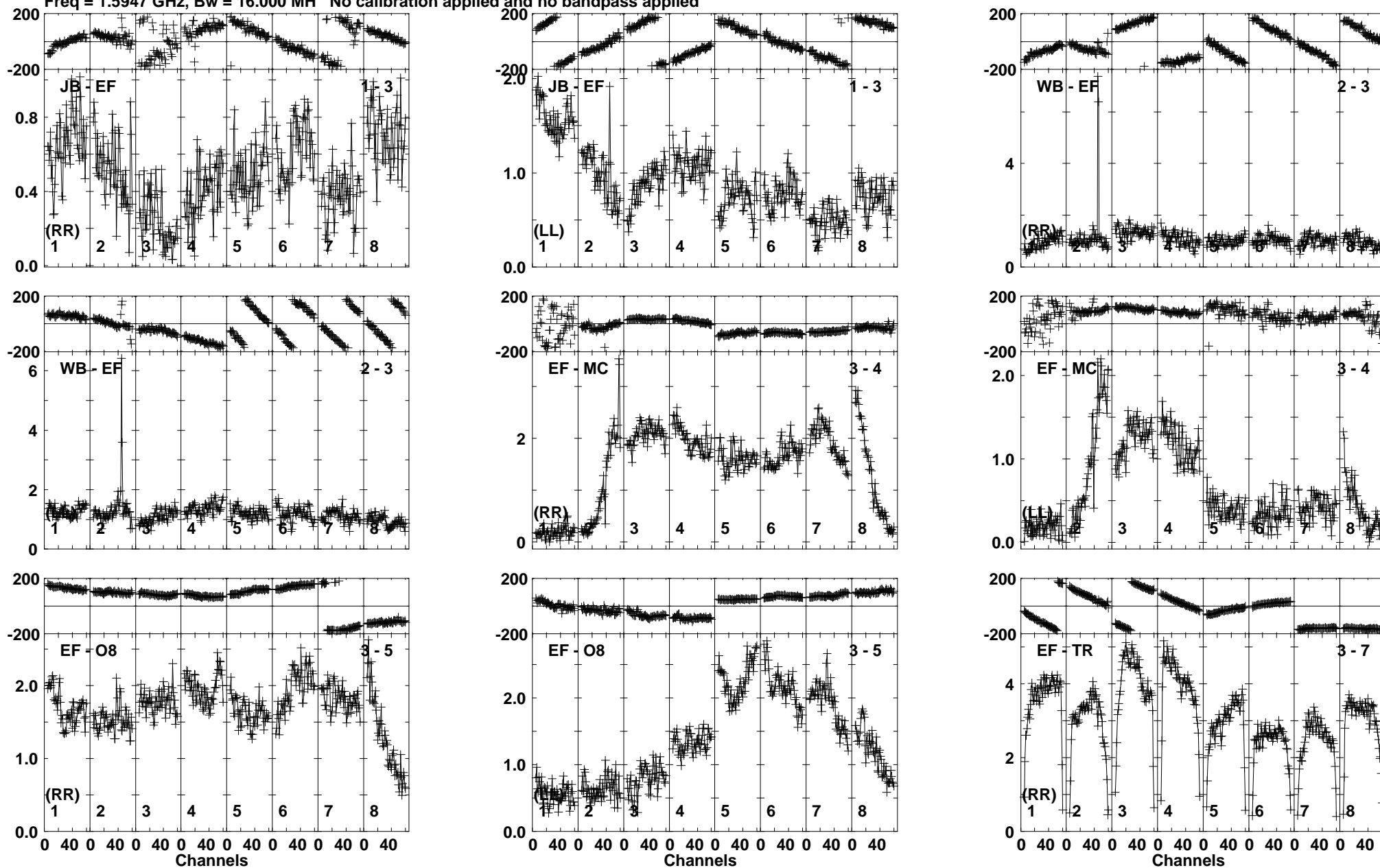
Lower frame: Milli Ampl Jy Top frame: Phas deg Vector averaged cross-power spectrum Baseline: JB (01) - EF (03) Timerange: 00/05:06:21 to 00/05:07:19
