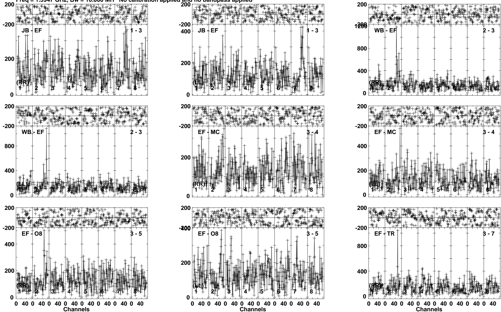
Lower frame: Micro Ampl Jy Top frame: Phas deg Vector averaged cross-power spectrum Baseline: JB (01) - EF (03) Timerange: 00/05:38:01 to 00/05:40:49
