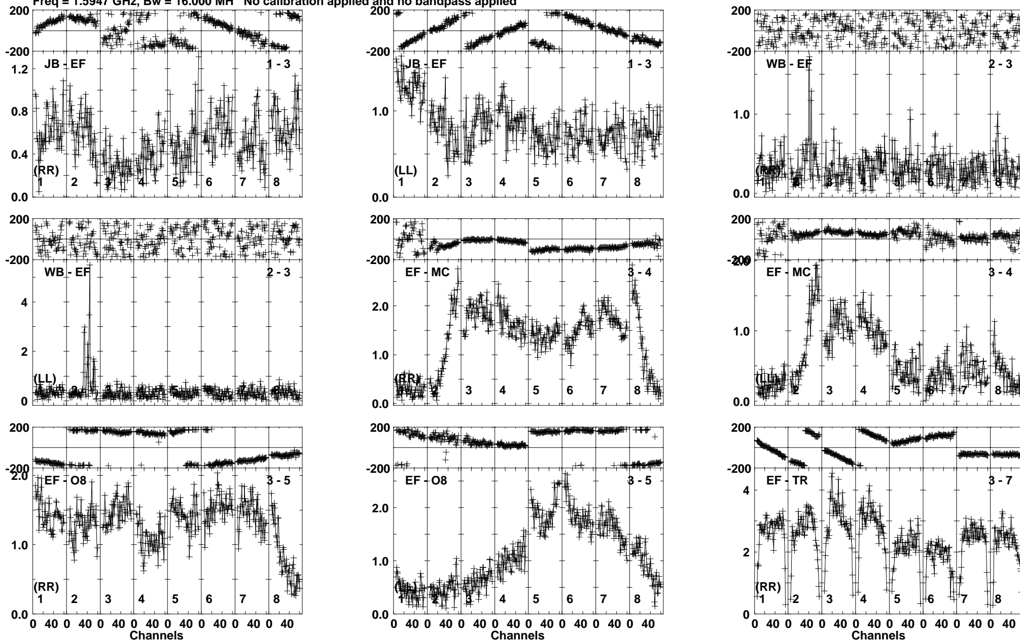
Lower frame: Milli Ampl Jy Top frame: Phas deg Vector averaged cross-power spectrum Baseline: JB (01) - EF (03) Timerange: 00/07:23:31 to 00/07:24:39
