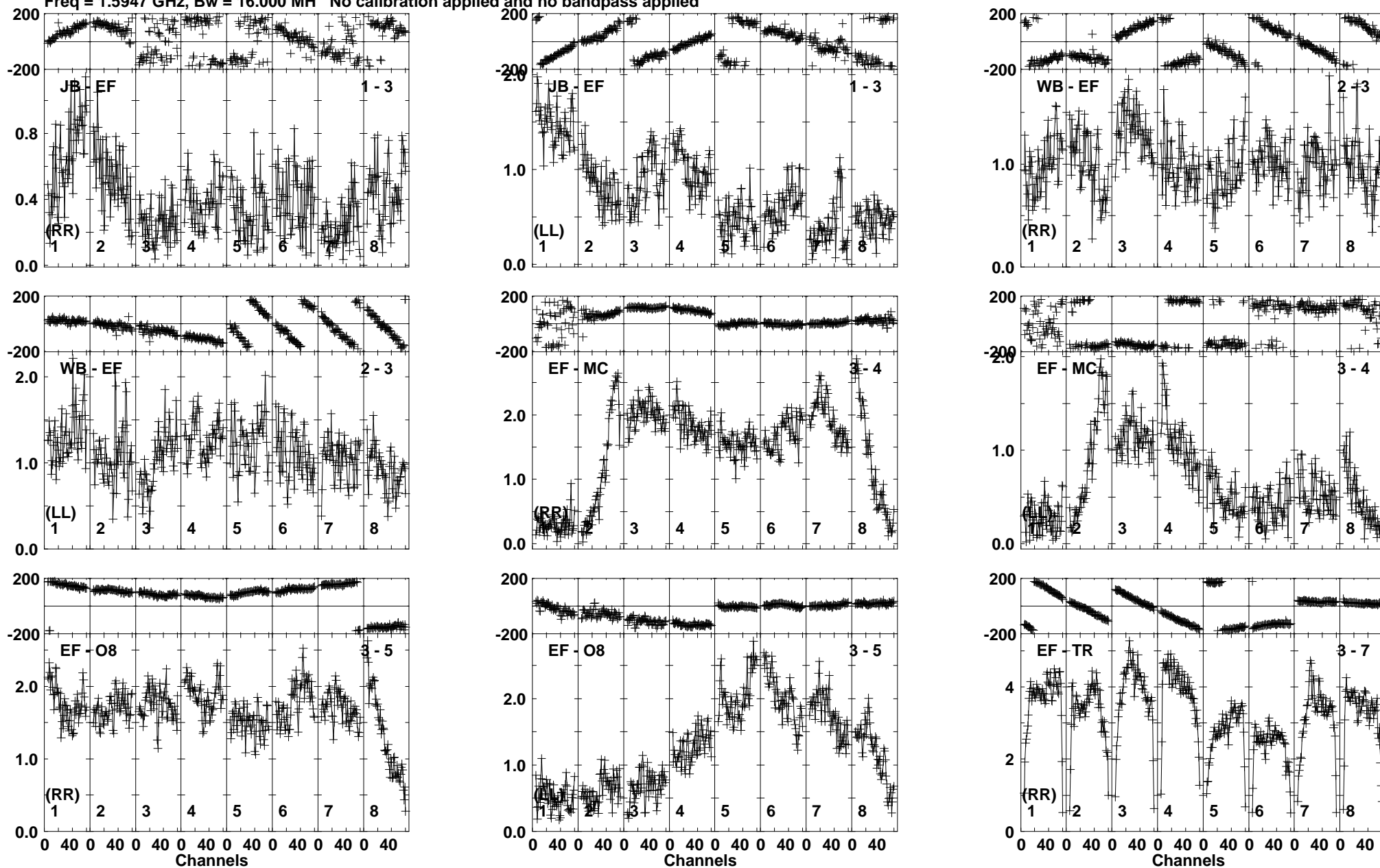
Lower frame: Milli Ampl Jy Top frame: Phas deg Vector averaged cross-power spectrum Baseline: JB (01) - EF (03) Timerange: 00/02:42:11 to 00/02:43:19
