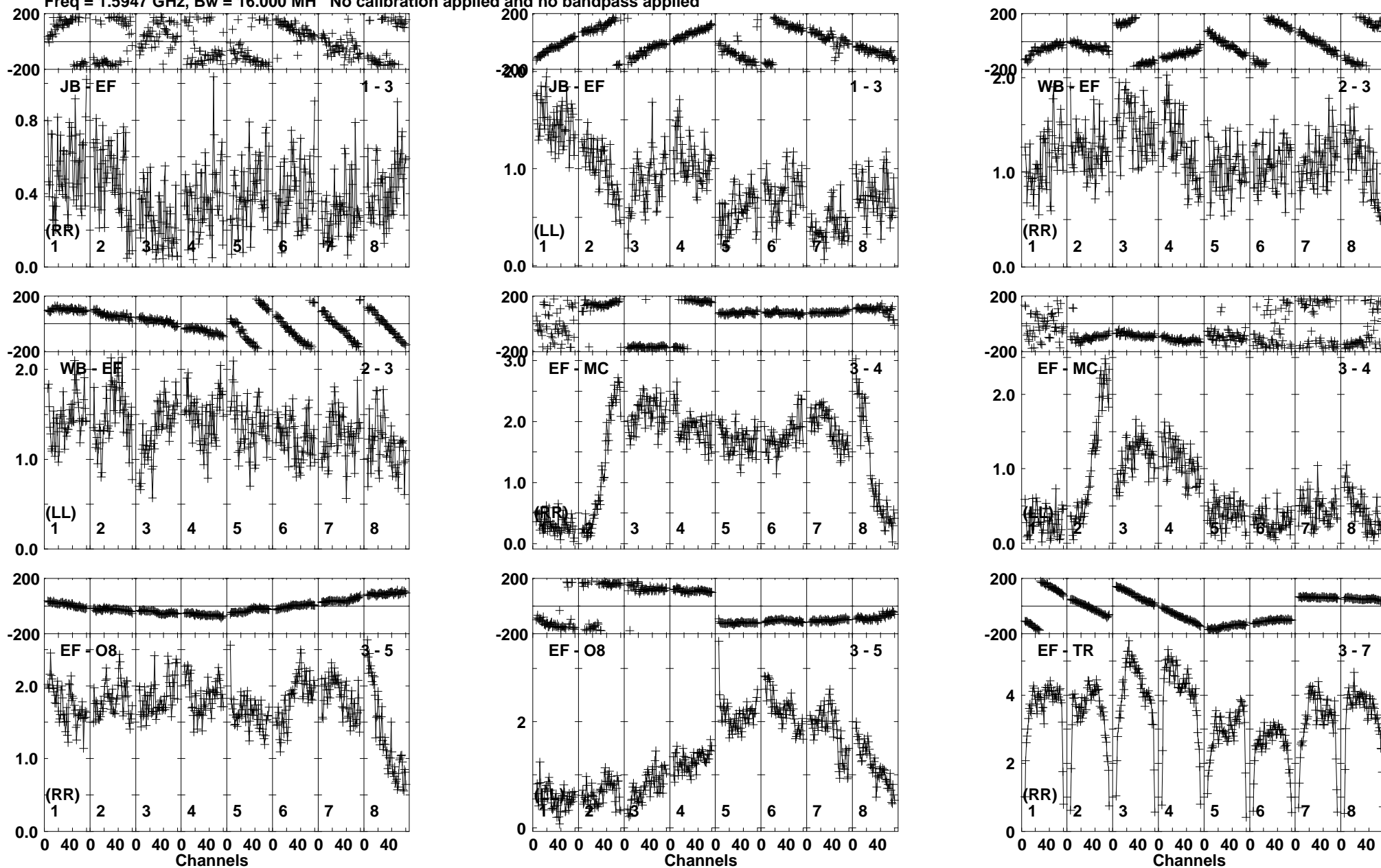
Lower frame: Milli Ampl Jy Top frame: Phas deg Vector averaged cross-power spectrum Baseline: JB (01) - EF (03) Timerange: 00/03:35:31 to 00/03:36:39
