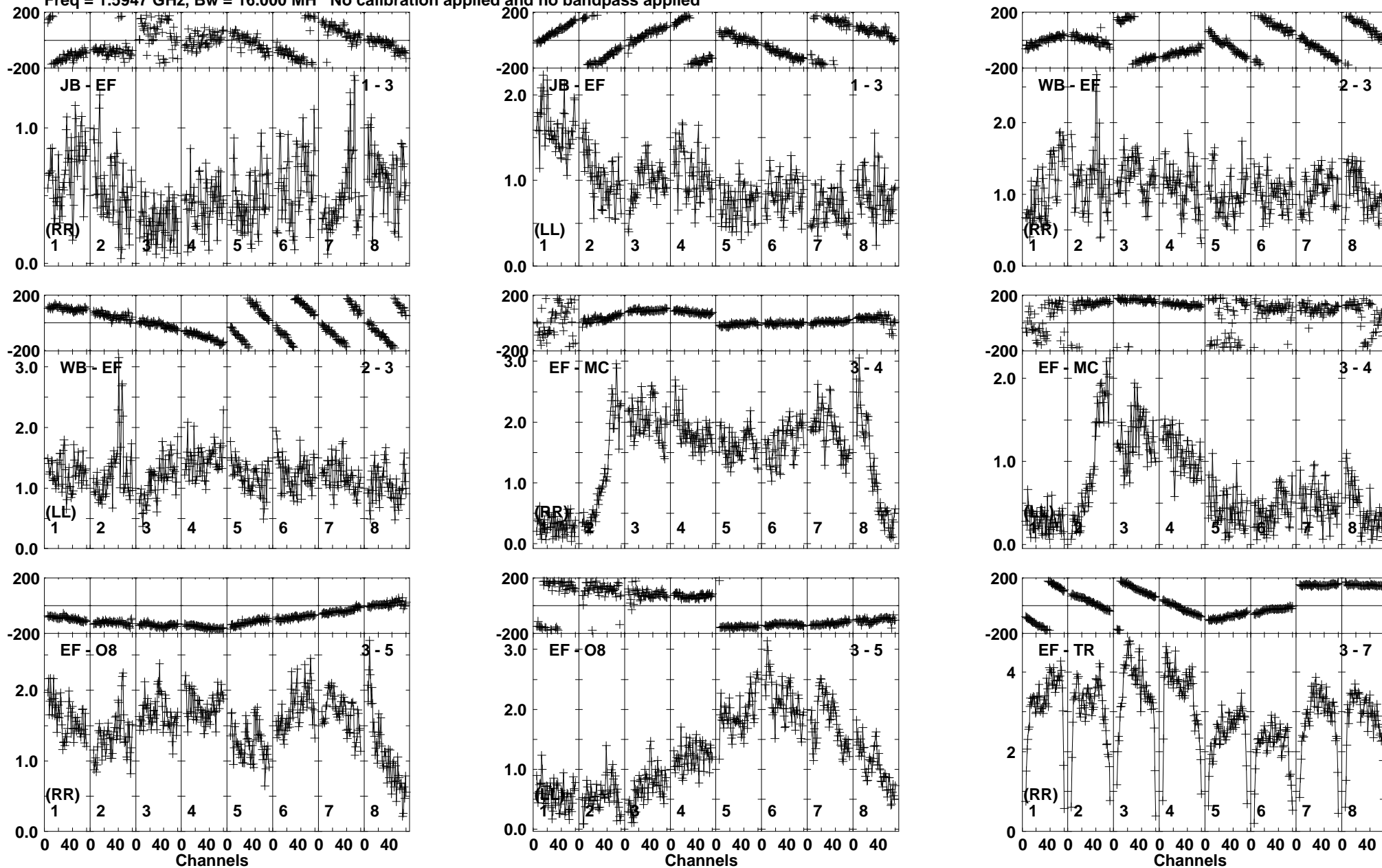
Lower frame: Milli Ampl Jy Top frame: Phas deg Vector averaged cross-power spectrum Baseline: JB (01) - EF (03) Timerange: 00/06:21:51 to 00/06:22:59
