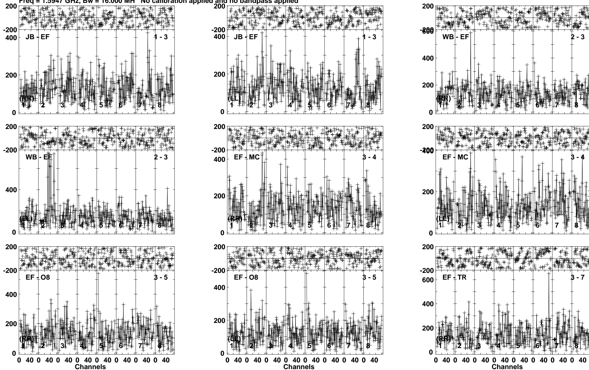
Lower frame: Micro Ampl Jy Top frame: Phas deg Vector averaged cross-power spectrum Baseline: JB (01) - EF (03) Timerange: 00/02:39:21 to 00/02:42:09
