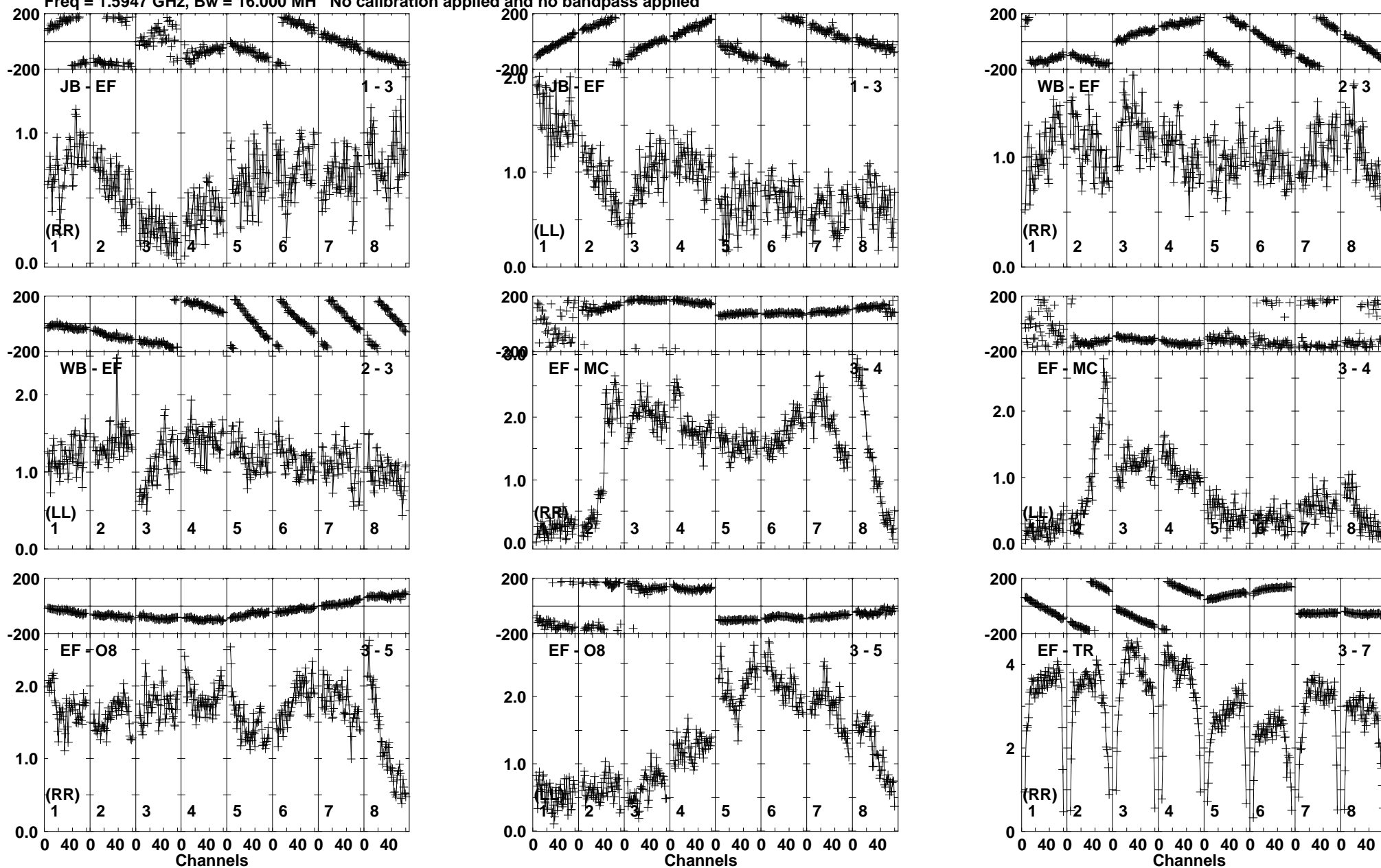
Lower frame: Milli Ampl Jy Top frame: Phas deg Vector averaged cross-power spectrum Baseline: JB (01) - EF (03) Timerange: 00/06:01:41 to 00/06:02:39
