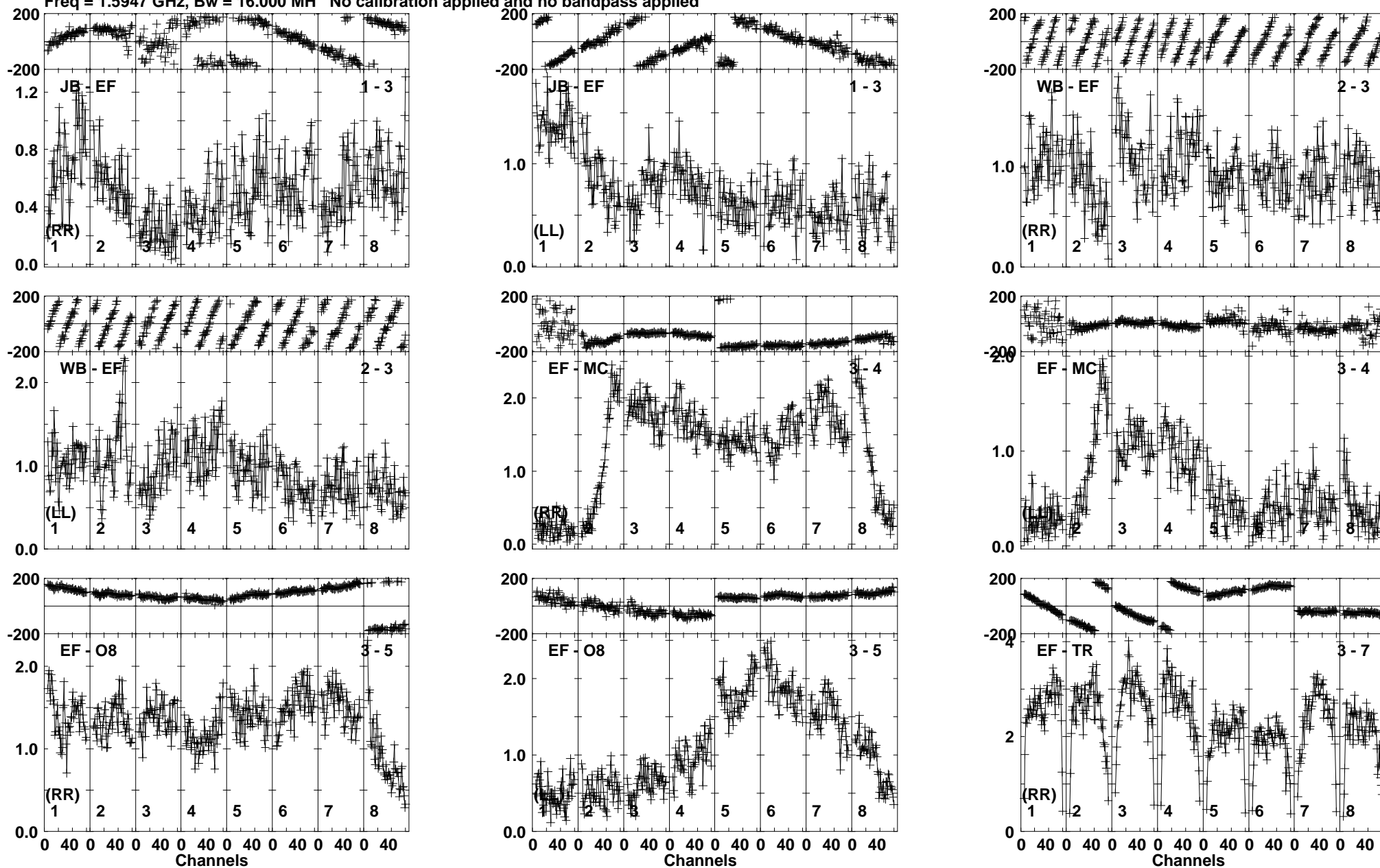
Lower frame: Milli Ampl Jy Top frame: Phas deg Vector averaged cross-power spectrum Baseline: JB (01) - EF (03) Timerange: 00/07:31:51 to 00/07:32:59
