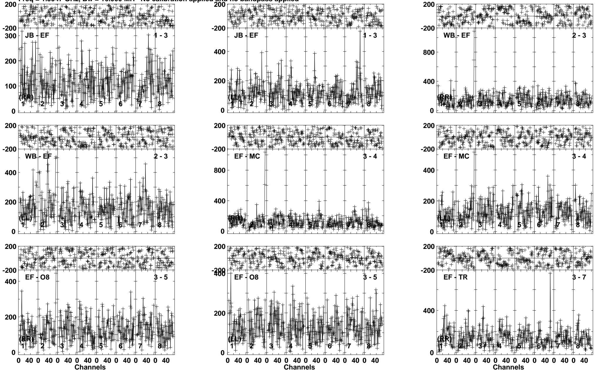
Lower frame: Micro Ampl Jy Top frame: Phas deg Vector averaged cross-power spectrum Baseline: JB (01) - EF (03) Timerange: 00/03:20:21 to 00/03:23:09
