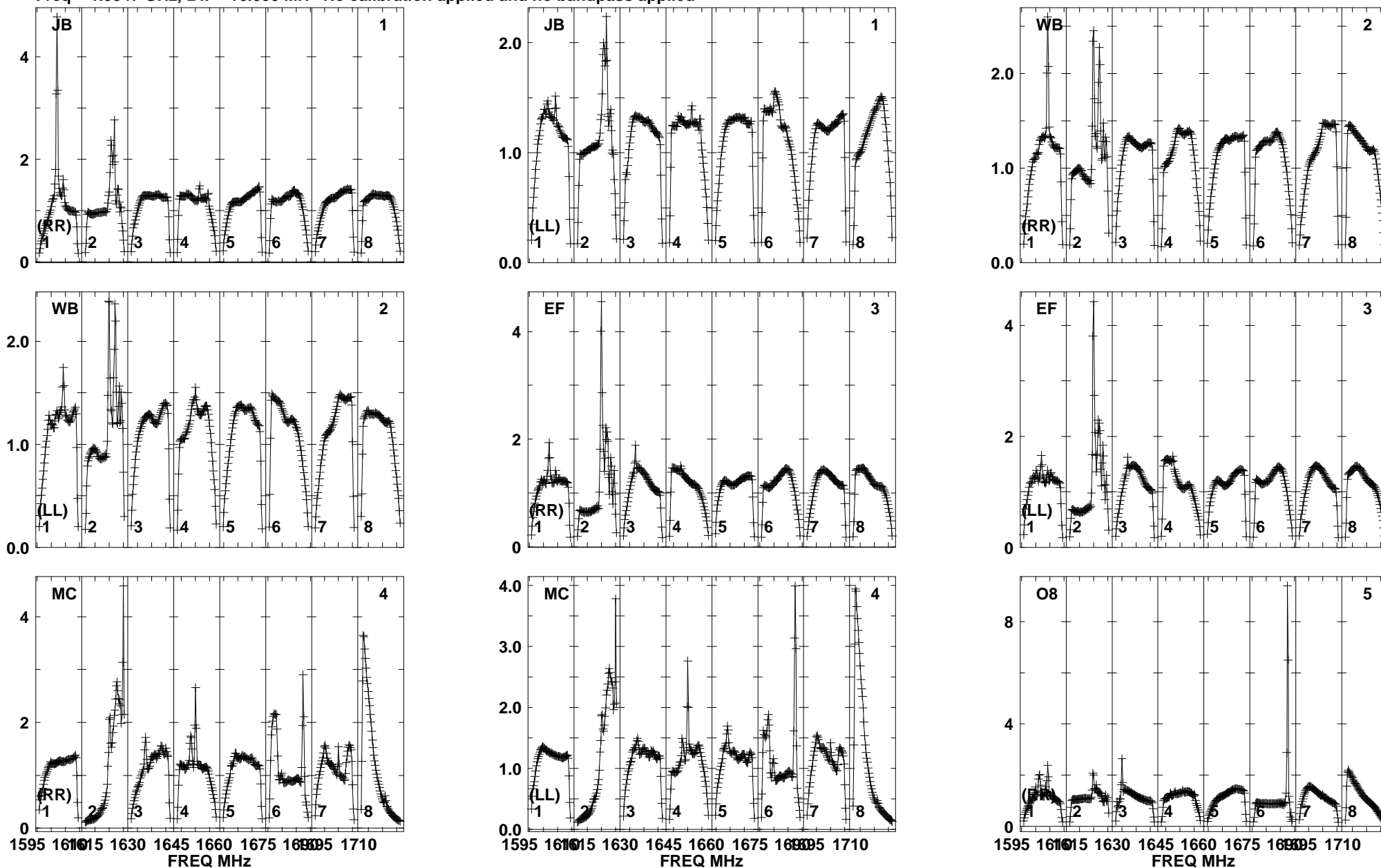
Lower frame: Real Jy Total-power spectrum Antenna: JB (01) Timerange: 01/09:15:20 to 01/09:18:20
