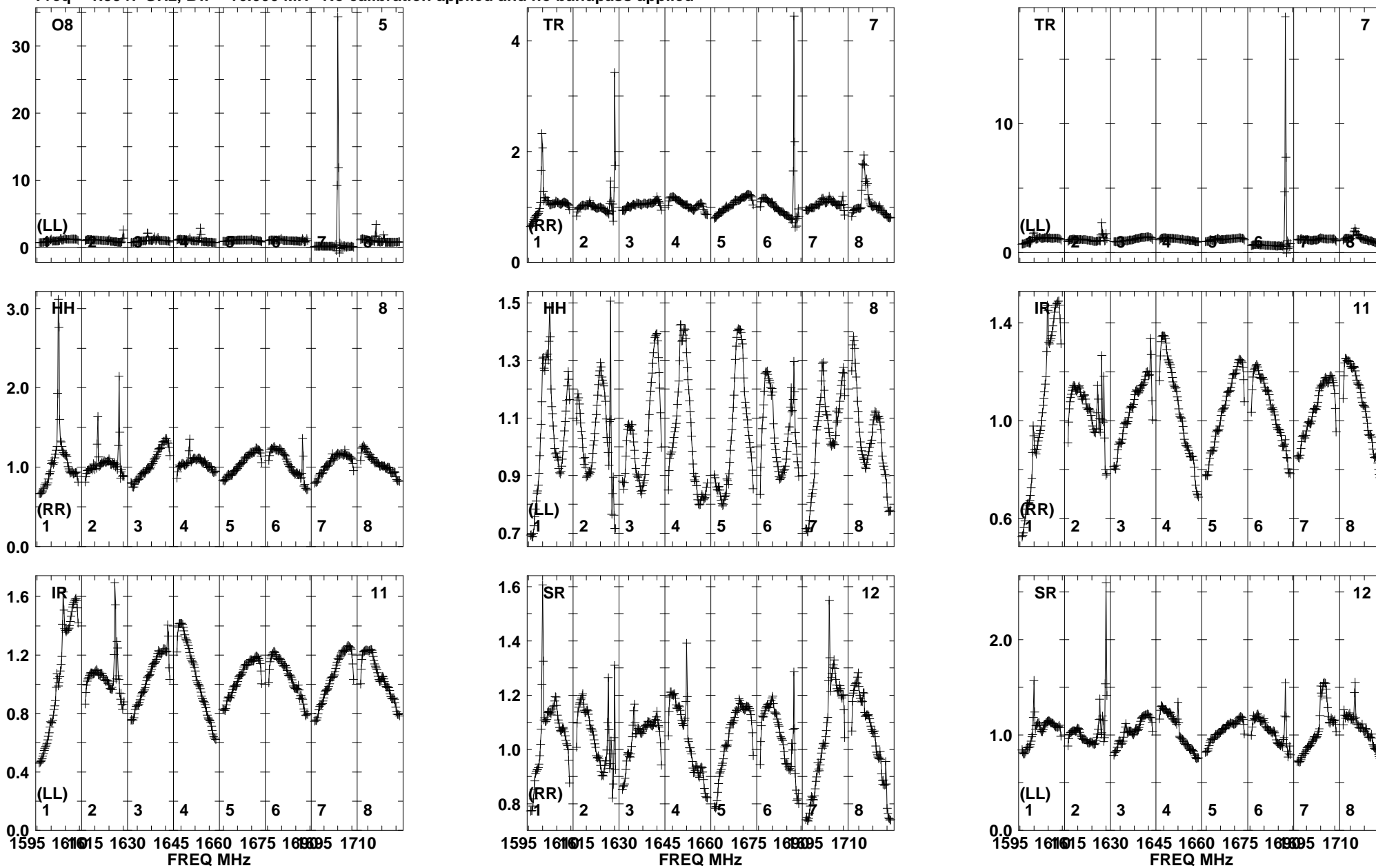
Lower frame: Real Jy Total-power spectrum Antenna: O8 (05) Timerange: 00/08:56:16 to 00/08:57:14
