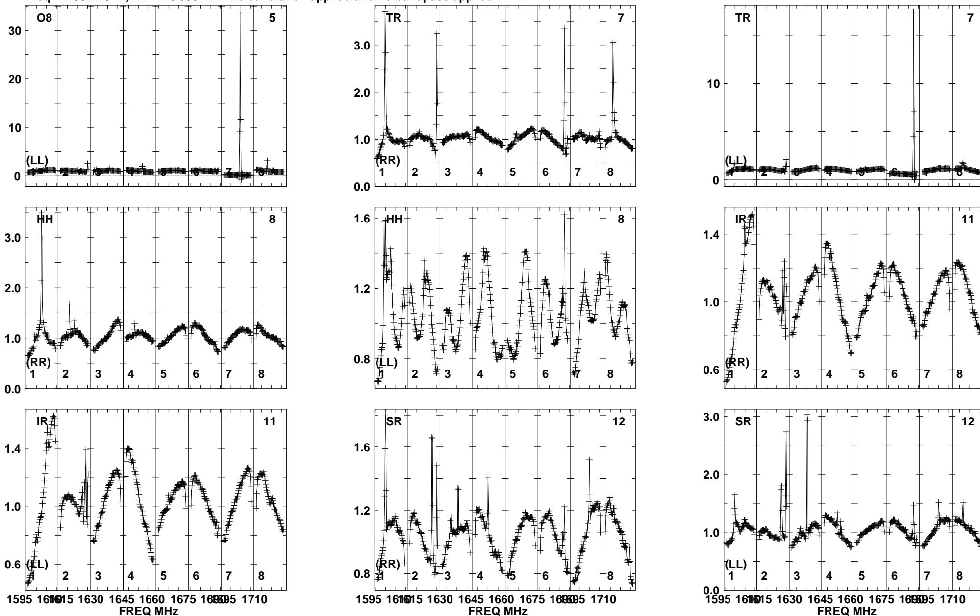
Lower frame: Real Jy Total-power spectrum Antenna: O8 (05) Timerange: 00/09:12:16 to 00/09:13:14
