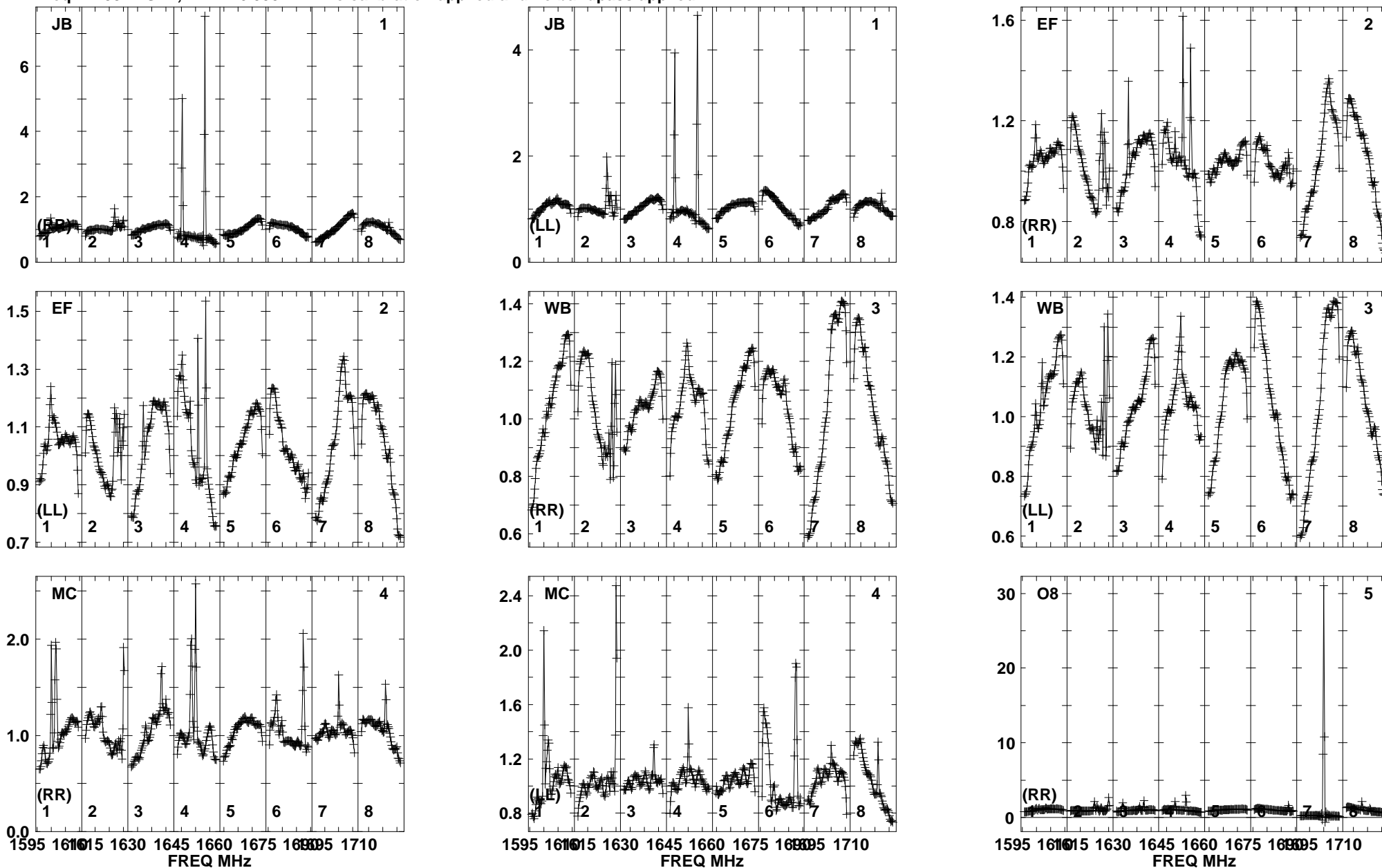
Lower frame: Real Jy Total-power spectrum Antenna: JB (01) Timerange: 00/08:57:16 to 00/08:59:54
