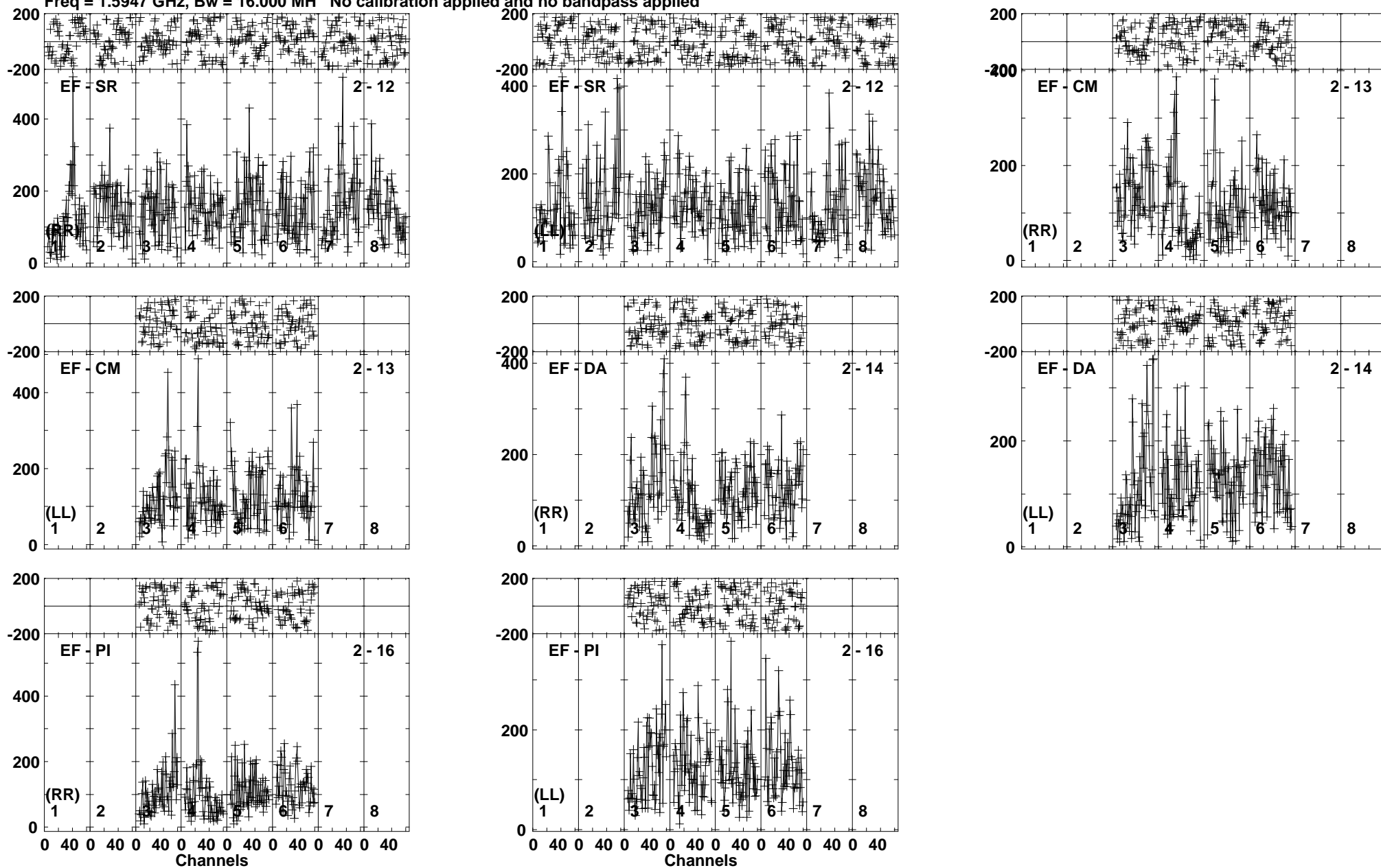
Lower frame: Micro Ampl Jy Top frame: Phas deg Vector averaged cross-power spectrum Baseline: EF (02) - SR (12) Timerange: 00/04:53:21 to 00/04:55:59
