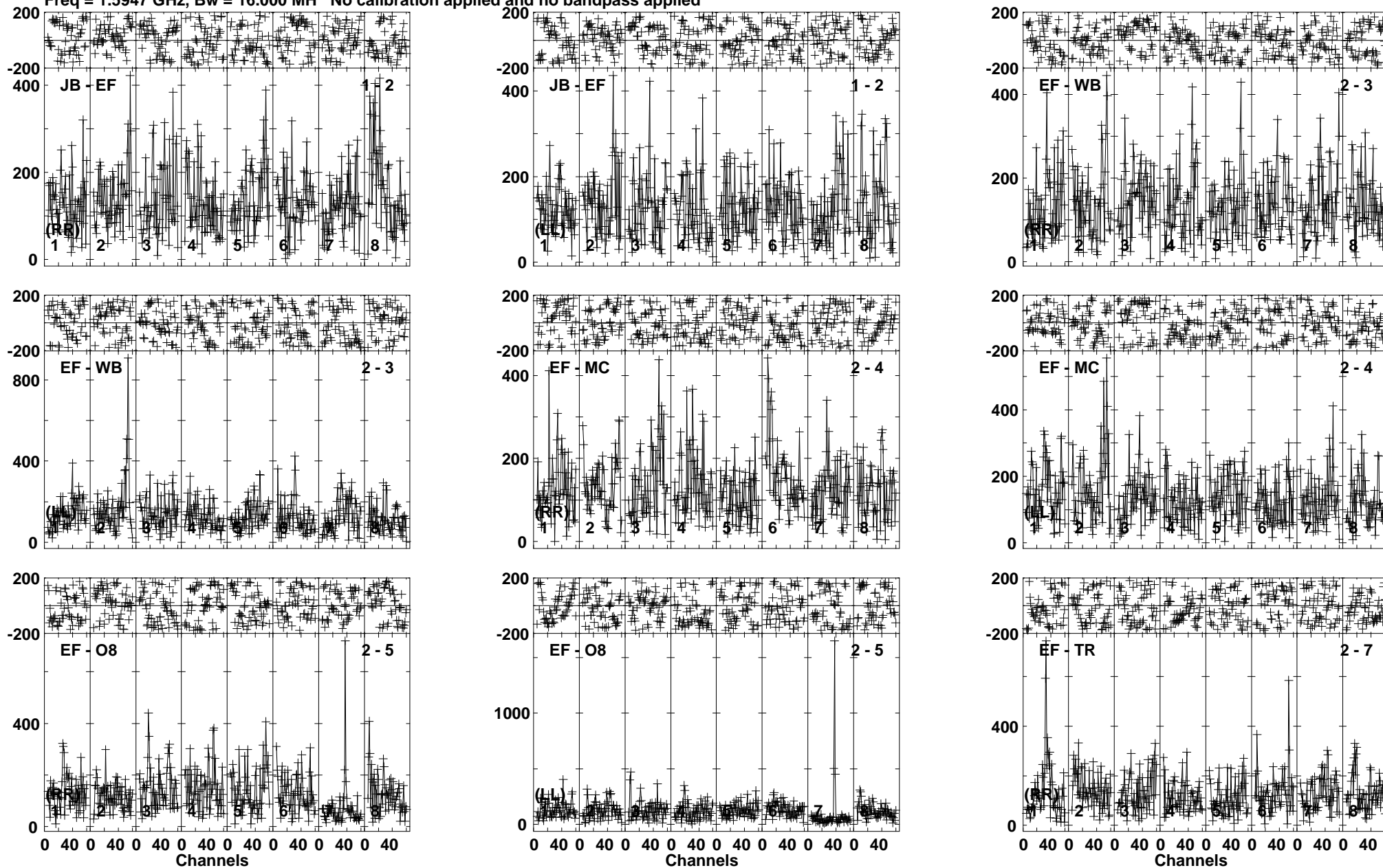
Lower frame: Micro Ampl Jy Top frame: Phas deg Vector averaged cross-power spectrum Baseline: JB (01) - EF (02) Timerange: 00/08:11:46 to 00/08:14:24
