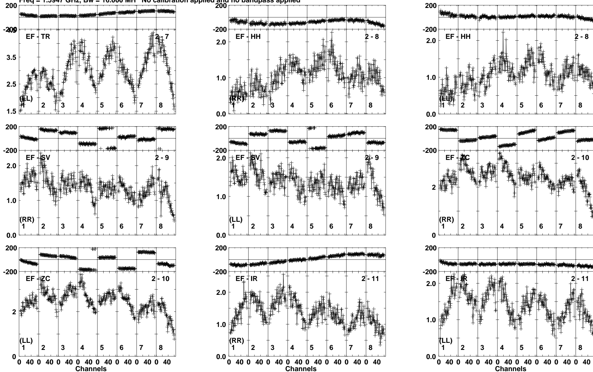
Lower frame: Milli Ampl Jy Top frame: Phas deg Vector averaged cross-power spectrum Baseline: EF (02) - TR (07) Timerange: 00/03:54:46 to 00/03:55:44
