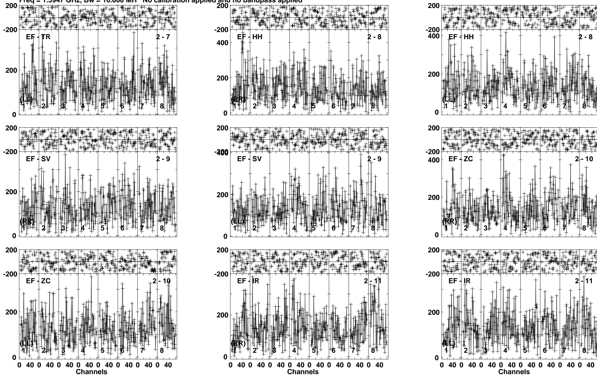
Lower frame: Micro Ampl Jy Top frame: Phas deg Vector averaged cross-power spectrum Baseline: EF (02) - TR (07) Timerange: 00/05:57:21 to 00/05:59:59
