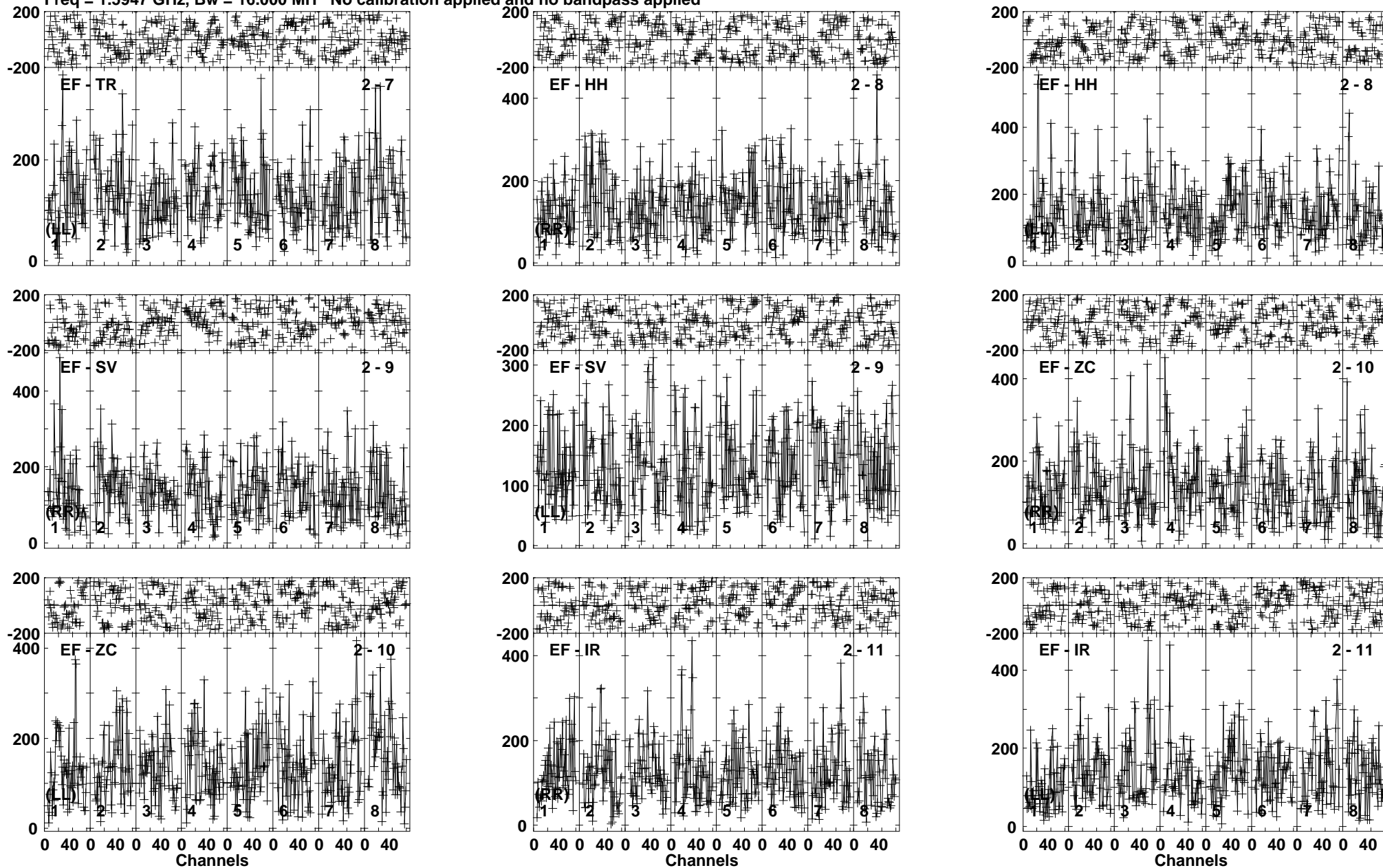
Lower frame: Micro Ampl Jy Top frame: Phas deg Vector averaged cross-power spectrum Baseline: EF (02) - TR (07) Timerange: 00/03:52:01 to 00/03:54:29
