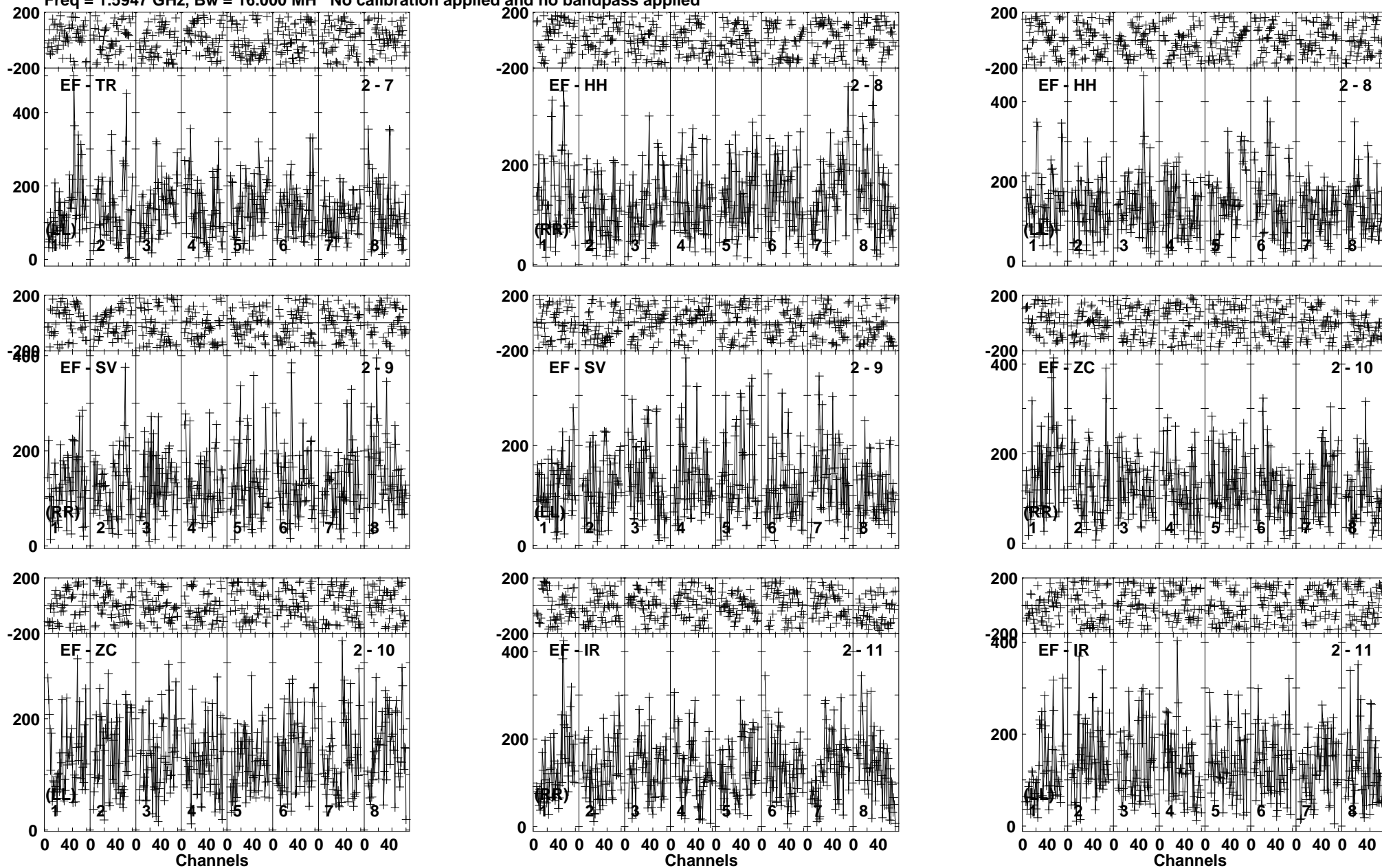
Lower frame: Micro Ampl Jy Top frame: Phas deg Vector averaged cross-power spectrum Baseline: EF (02) - TR (07) Timerange: 00/04:30:36 to 00/04:33:14
