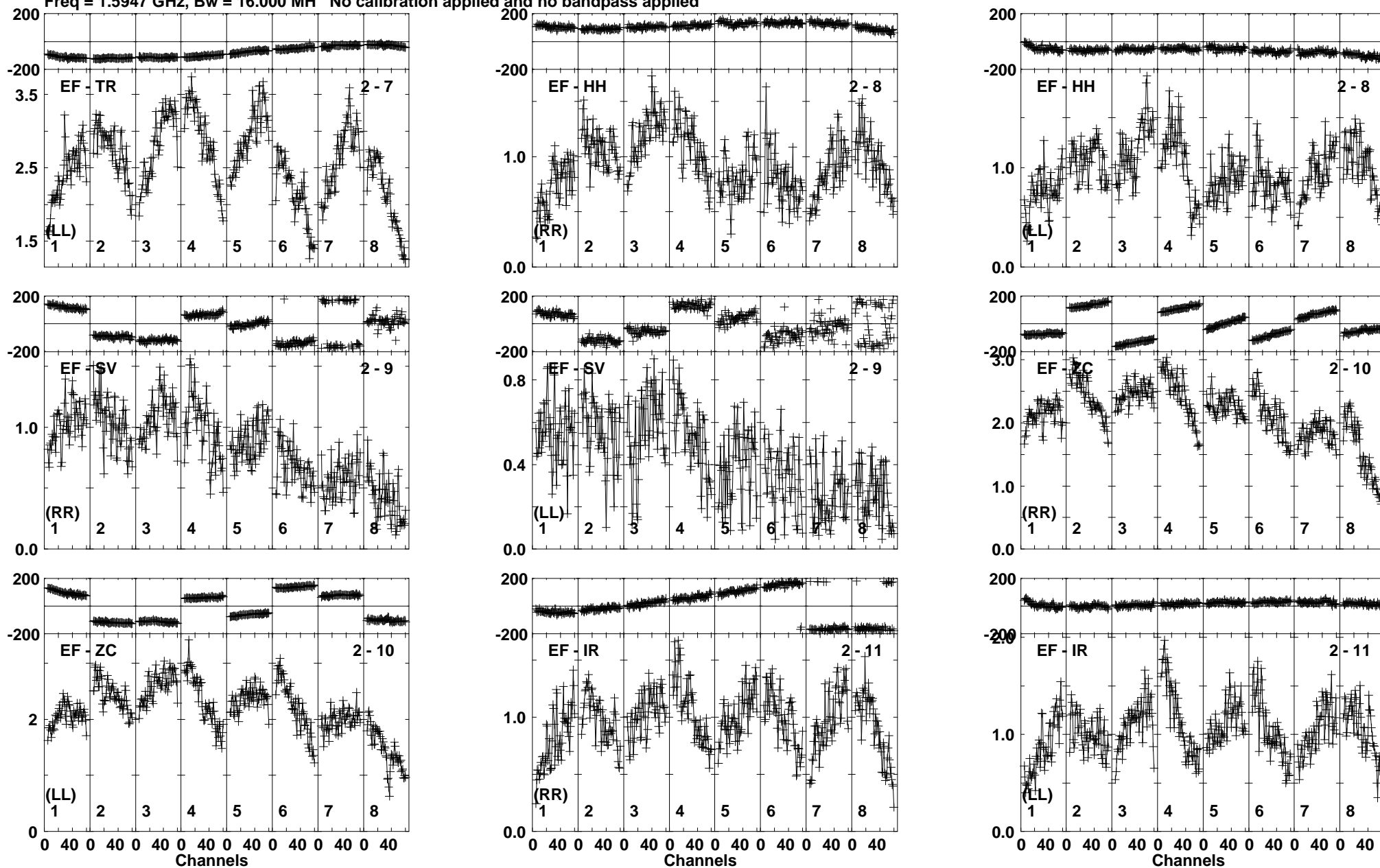
Lower frame: Milli Ampl Jy Top frame: Phas deg Vector averaged cross-power spectrum Baseline: EF (02) - TR (07) Timerange: 00/08:07:01 to 00/08:07:59
