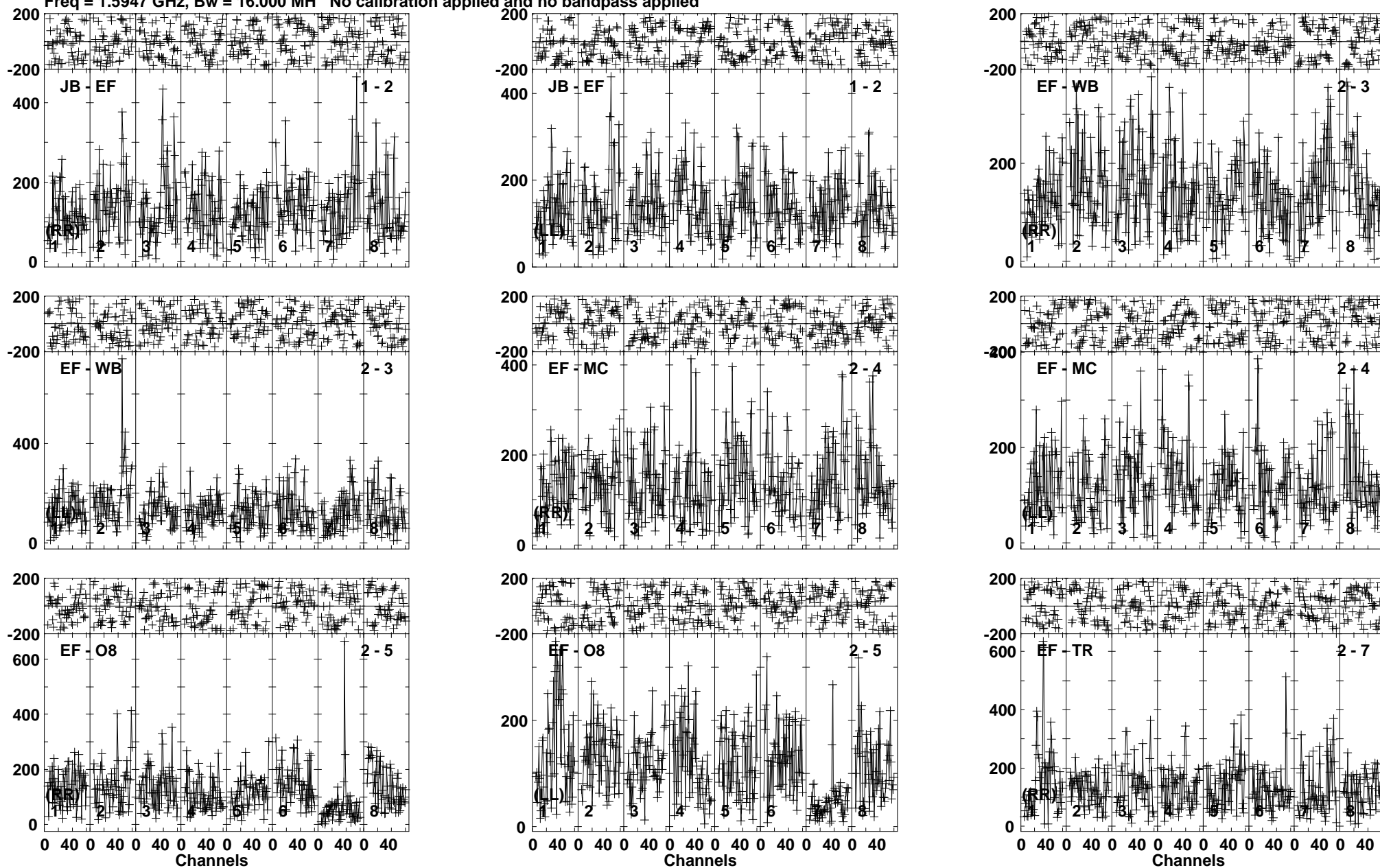
Lower frame: Micro Ampl Jy Top frame: Phas deg Vector averaged cross-power spectrum Baseline: JB (01) - EF (02) Timerange: 00/08:19:36 to 00/08:22:14
