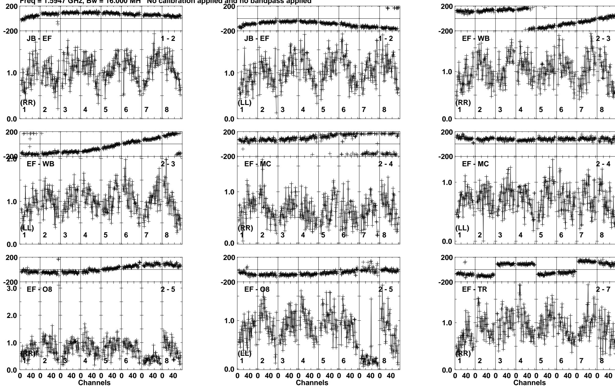
Lower frame: Milli Ampl Jy Top frame: Phas deg Vector averaged cross-power spectrum Baseline: JB (01) - EF (02) Timerange: 00/08:05:16 to 00/08:06:14
