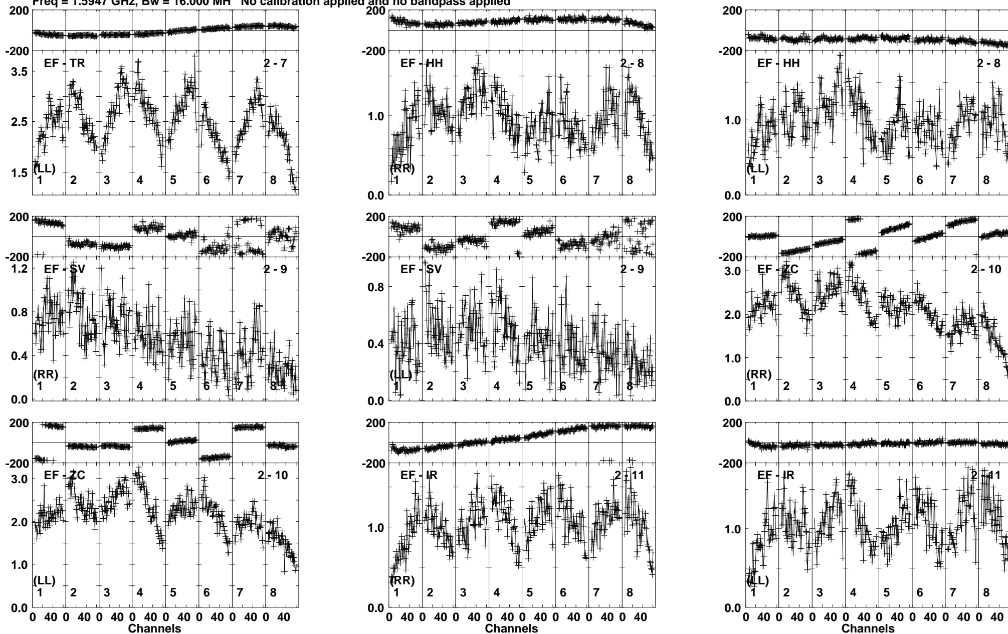
Lower frame: Milli Ampl Jy Top frame: Phas deg Vector averaged cross-power spectrum Baseline: EF (02) - TR (07) Timerange: 00/08:04:01 to 00/08:04:59
