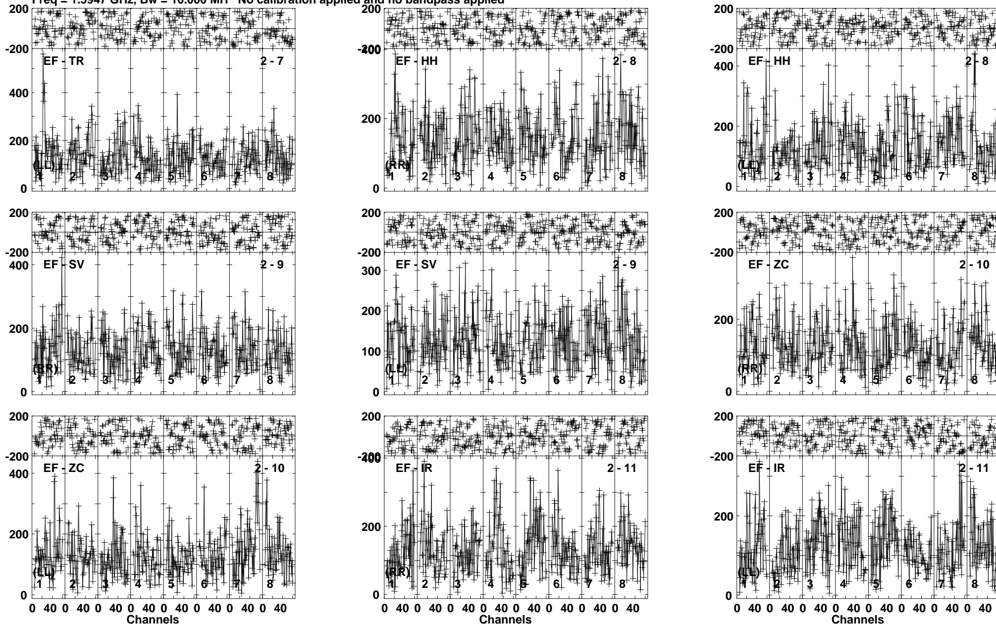
Lower frame: Micro Ampl Jy Top frame: Phas deg Vector averaged cross-power spectrum Baseline: EF (02) - TR (07) Timerange: 00/03:59:41 to 00/04:02:19
