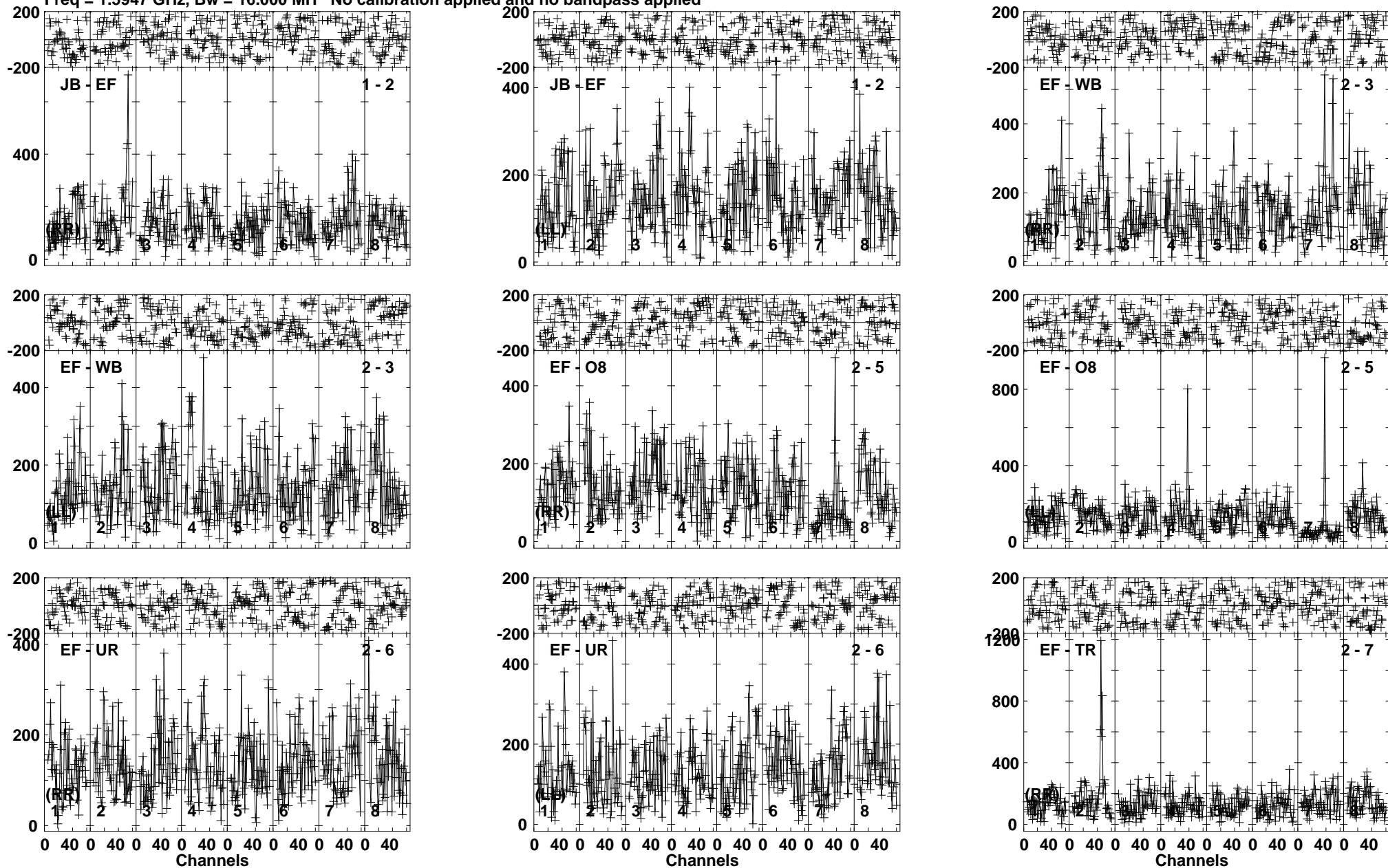
Lower frame: Micro Ampl Jy Top frame: Phas deg Vector averaged cross-power spectrum Baseline: JB (01) - EF (02) Timerange: 00/05:45:46 to 00/05:48:14
