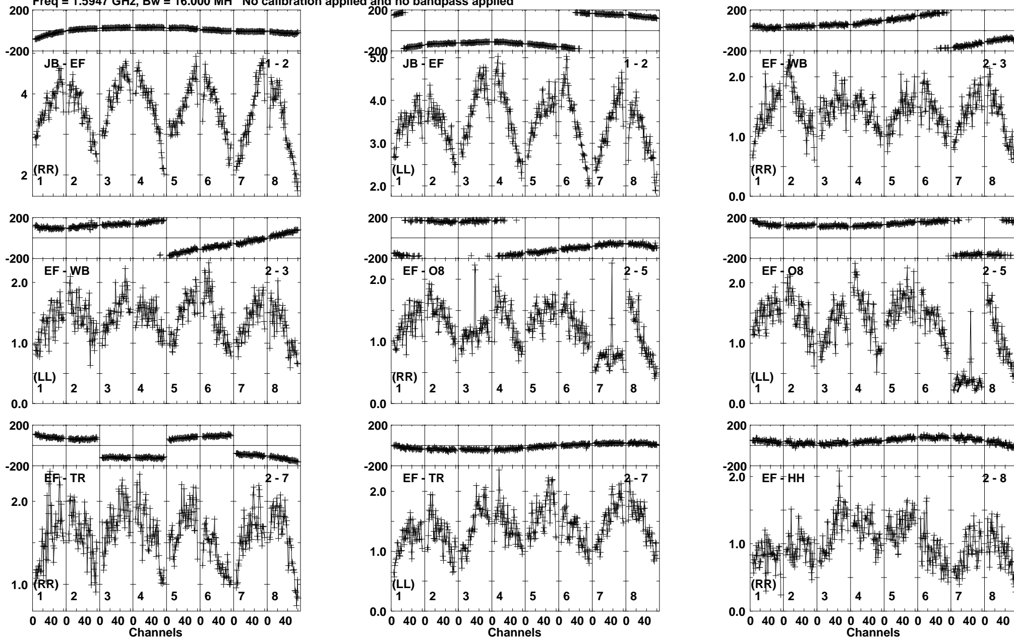
Lower frame: Milli Ampl Jy Top frame: Phas deg Vector averaged cross-power spectrum Baseline: JB (01) - EF (02) Timerange: 00/07:25:16 to 00/07:26:14
