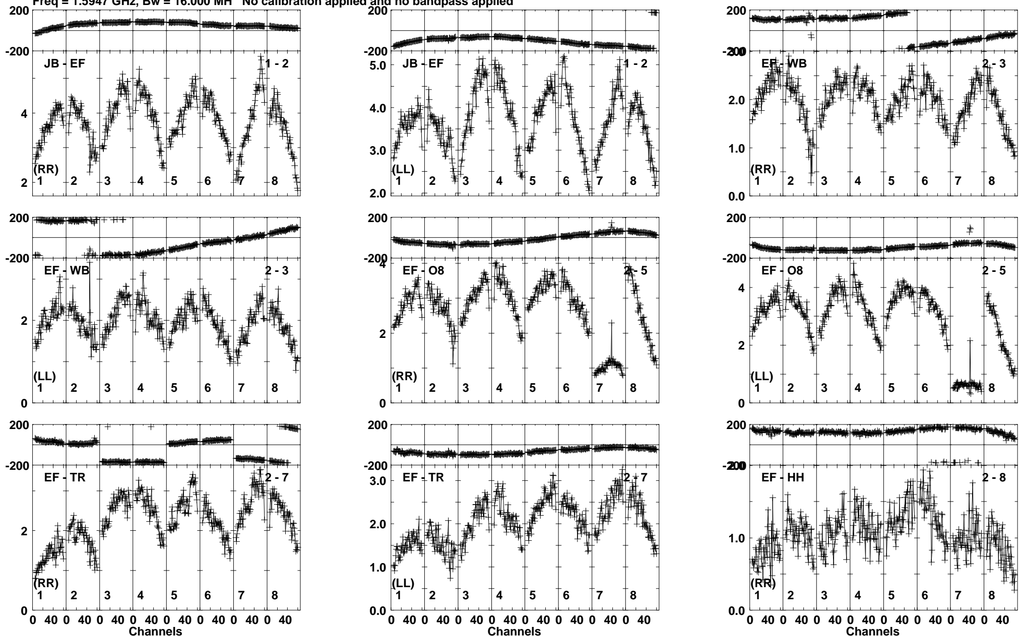
Lower frame: Milli Ampl Jy Top frame: Phas deg Vector averaged cross-power spectrum Baseline: JB (01) - EF (02) Timerange: 00/06:55:46 to 00/06:56:44
