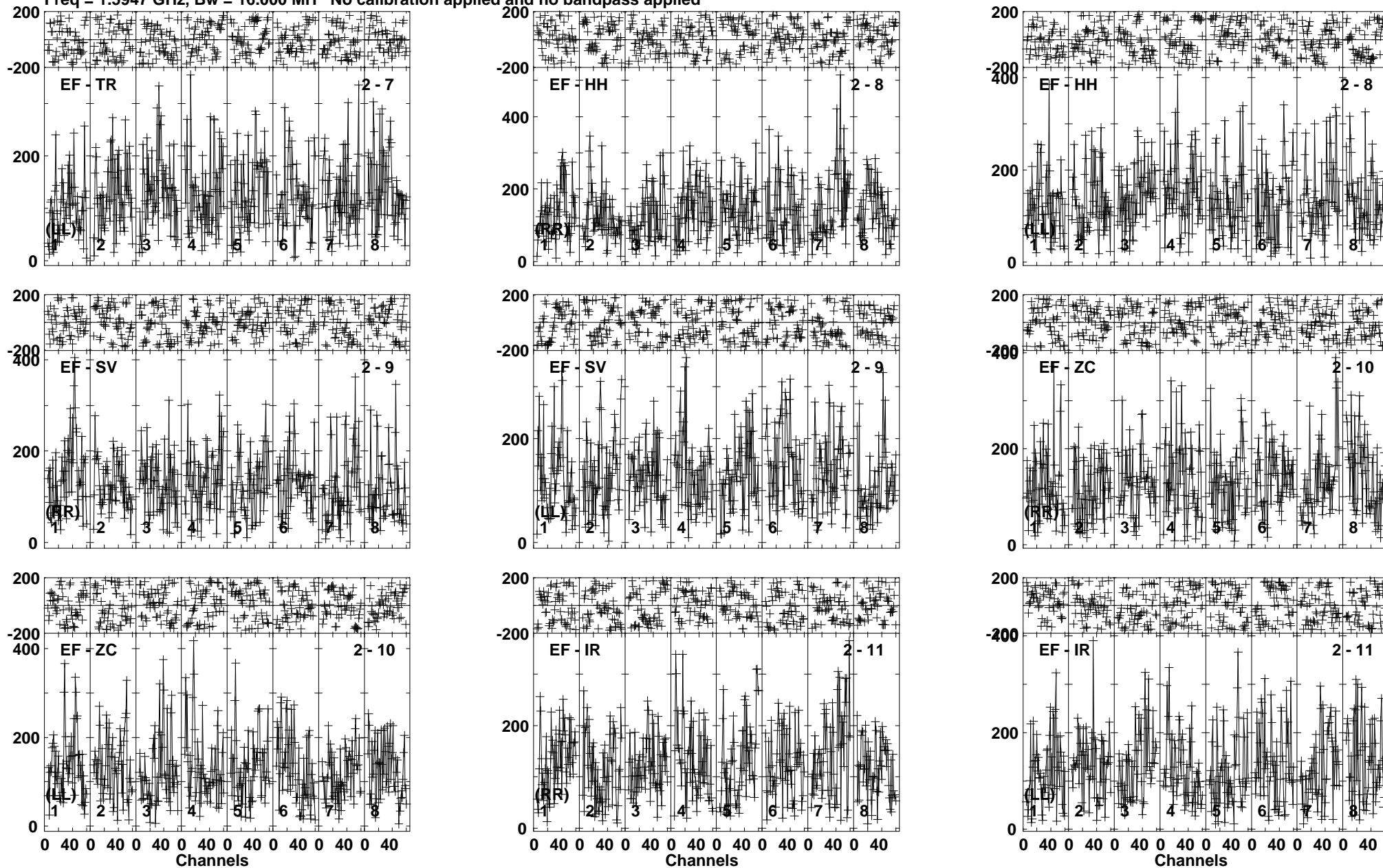
Lower frame: Micro Ampl Jy Top frame: Phas deg Vector averaged cross-power spectrum Baseline: EF (02) - TR (07) Timerange: 00/05:49:31 to 00/05:52:09
