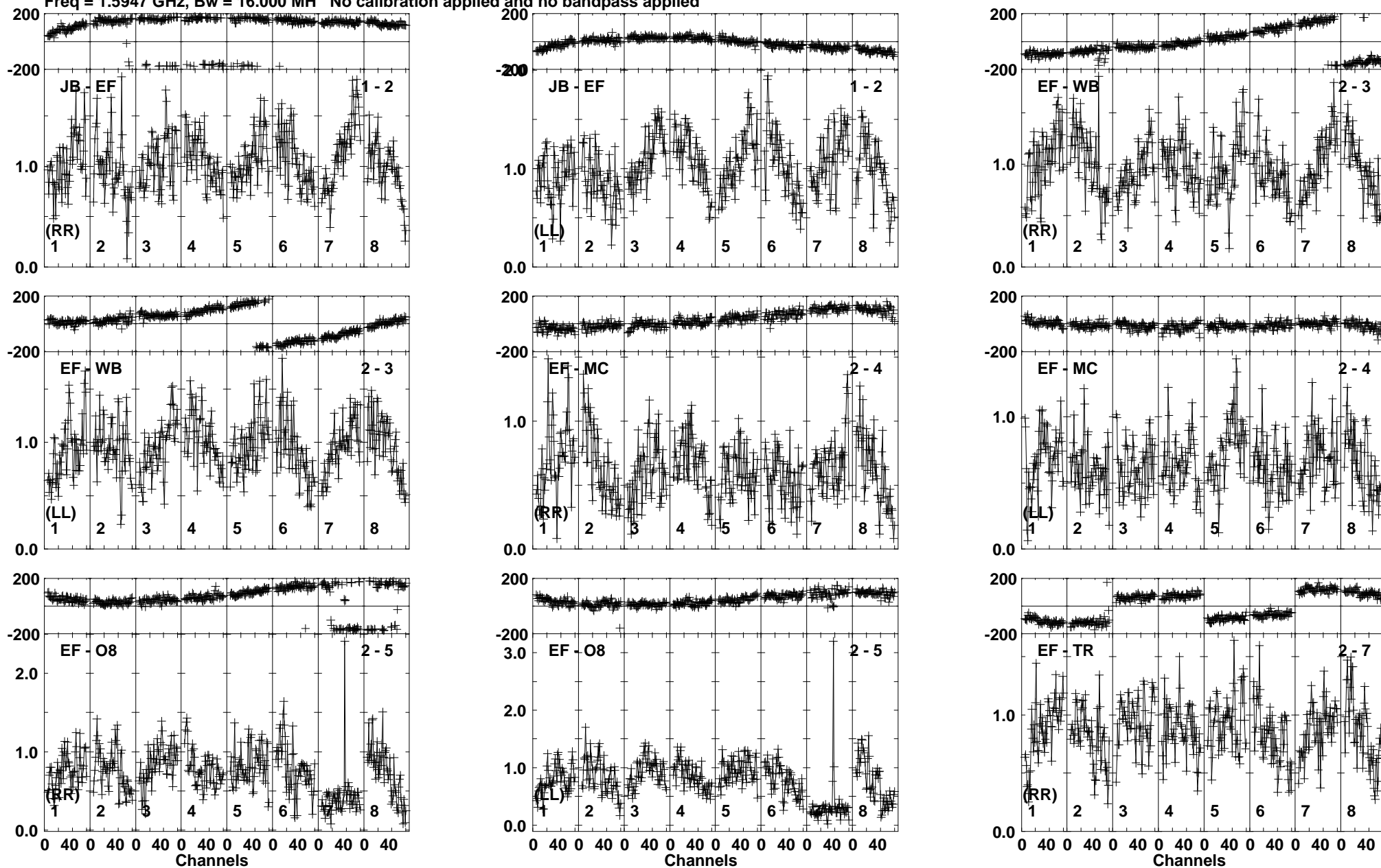
Lower frame: Milli Ampl Jy Top frame: Phas deg Vector averaged cross-power spectrum Baseline: JB (01) - EF (02) Timerange: 00/08:50:46 to 00/08:51:44
