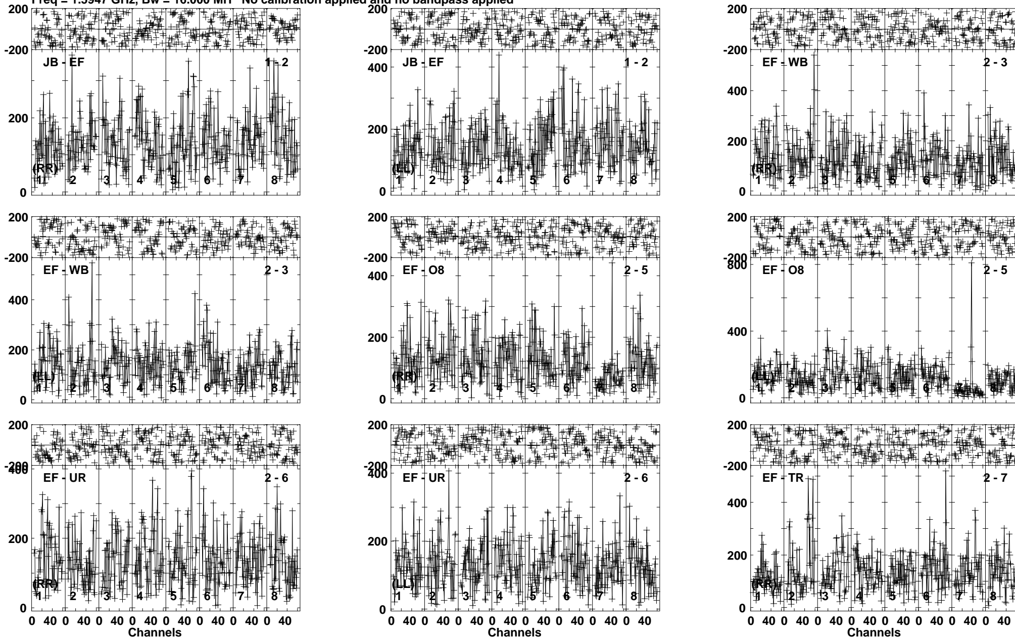
Lower frame: Micro Ampl Jy Top frame: Phas deg Vector averaged cross-power spectrum Baseline: JB (01) - EF (02) Timerange: 00/03:55:46 to 00/03:58:24
