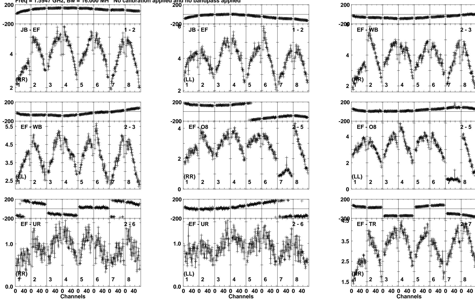
Lower frame: Milli Ampl Jy Top frame: Phas deg Vector averaged cross-power spectrum Baseline: JB (01) - EF (02) Timerange: 00/03:44:06 to 00/03:45:04
