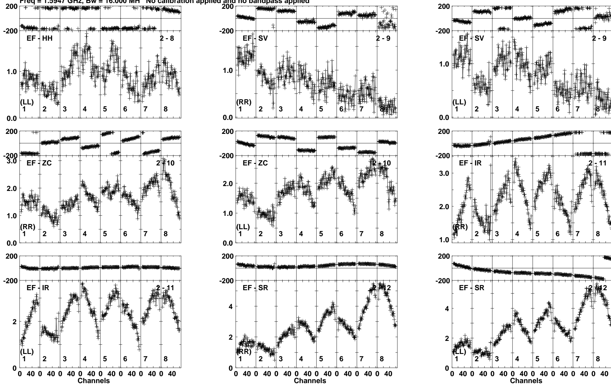
Lower frame: Milli Ampl Jy Top frame: Phas deg Vector averaged cross-power spectrum Baseline: EF (02) - HH (08) Timerange: 00/07:21:31 to 00/07:22:29
