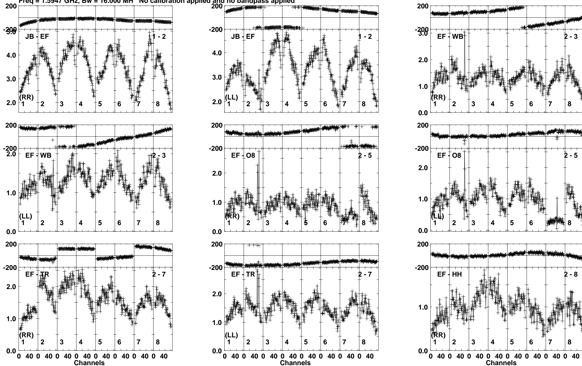
Lower frame: Milli Ampl Jy Top frame: Phas deg Vector averaged cross-power spectrum Baseline: JB (01) - EF (02) Timerange: 00/07:37:21 to 00/07:38:19
