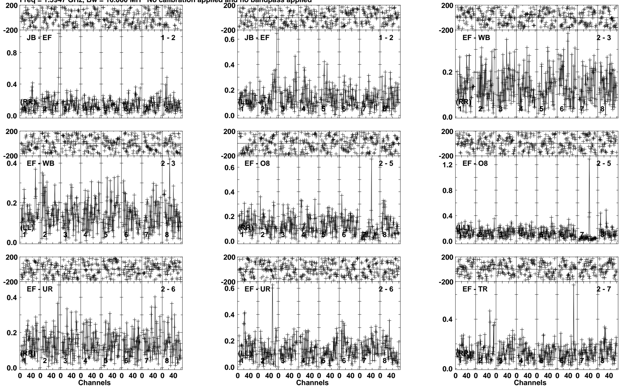
Lower frame: Milli Ampl Jy Top frame: Phas deg Vector averaged cross-power spectrum Baseline: JB (01) - EF (02) Timerange: 00/04:03:36 to 00/04:06:14
