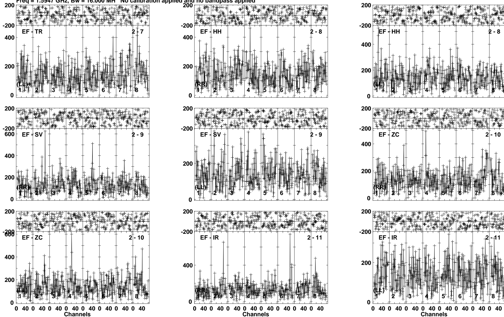
Lower frame: Micro Ampl Jy Top frame: Phas deg Vector averaged cross-power spectrum Baseline: EF (02) - TR (07) Timerange: 00/04:14:46 to 00/04:17:14
