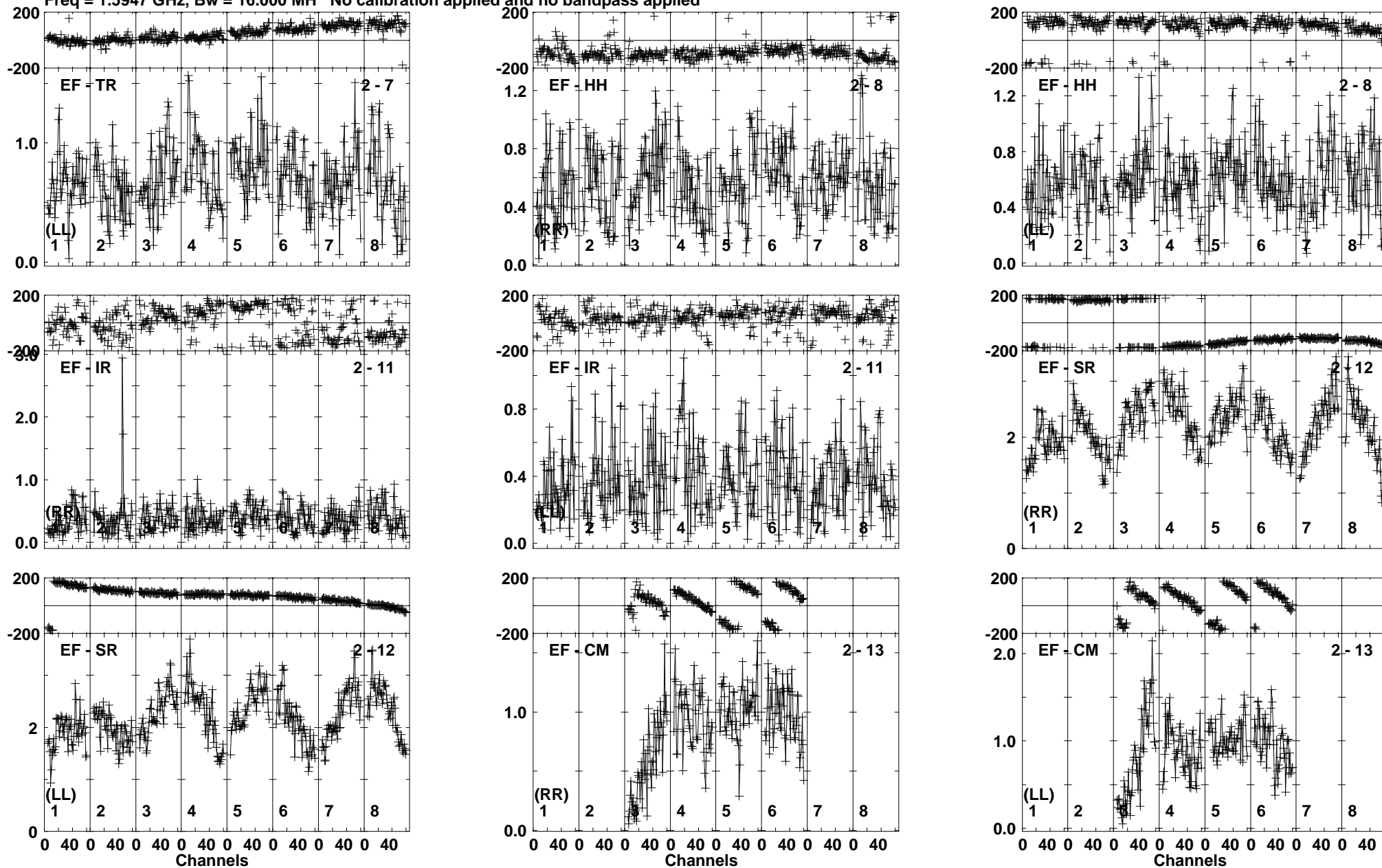
Lower frame: Milli Ampl Jy Top frame: Phas deg Vector averaged cross-power spectrum Baseline: EF (02) - TR (07) Timerange: 00/09:36:16 to 00/09:37:14
