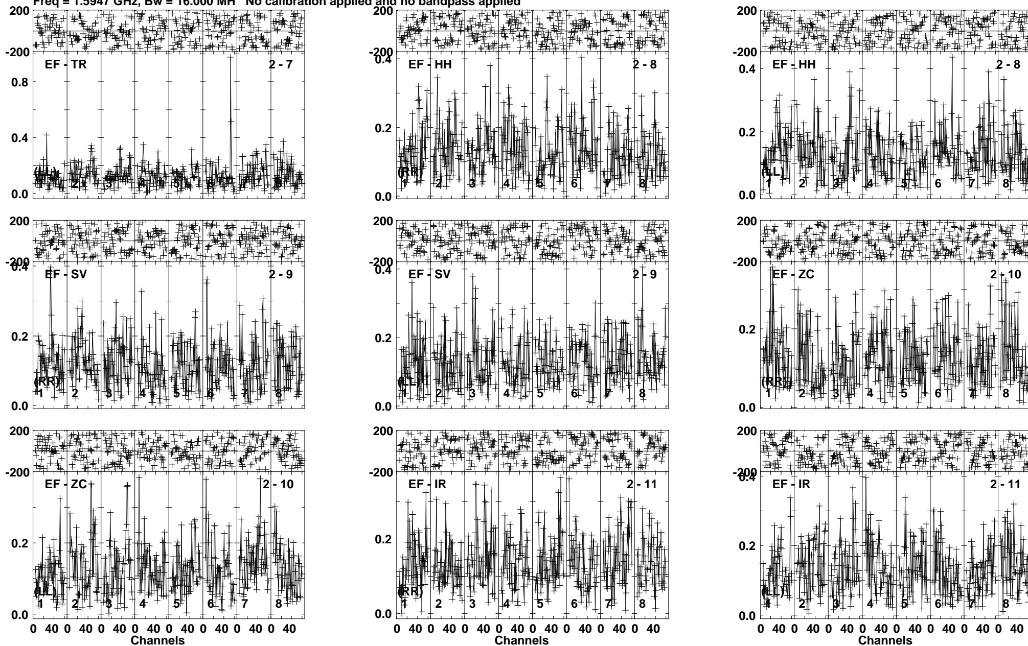
Lower frame: Milli Ampl Jy Top frame: Phas deg Vector averaged cross-power spectrum Baseline: EF (02) - TR (07) Timerange: 00/08:19:36 to 00/08:22:14
