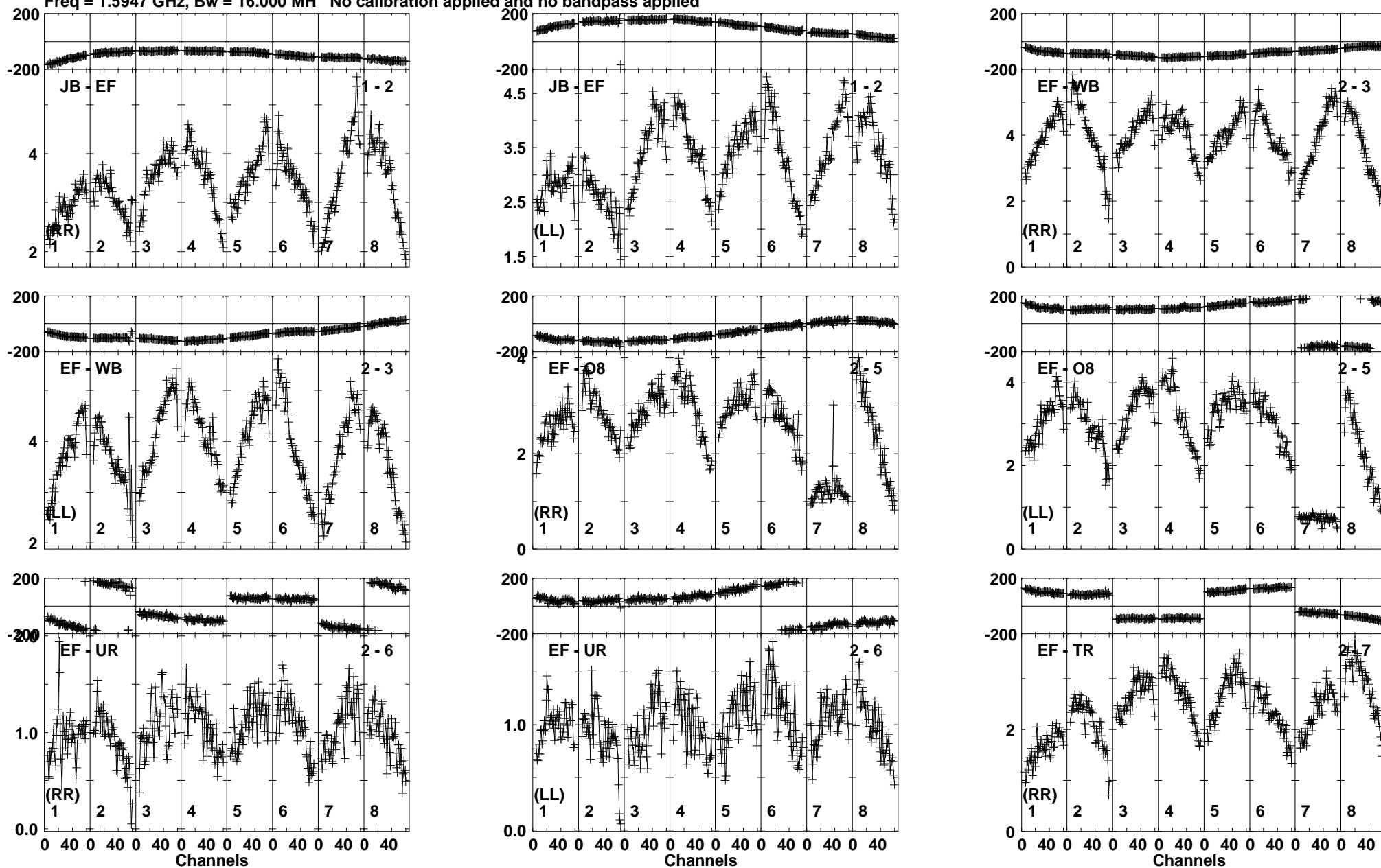
Lower frame: Milli Ampl Jy Top frame: Phas deg Vector averaged cross-power spectrum Baseline: JB (01) - EF (02) Timerange: 00/03:13:11 to 00/03:14:09
