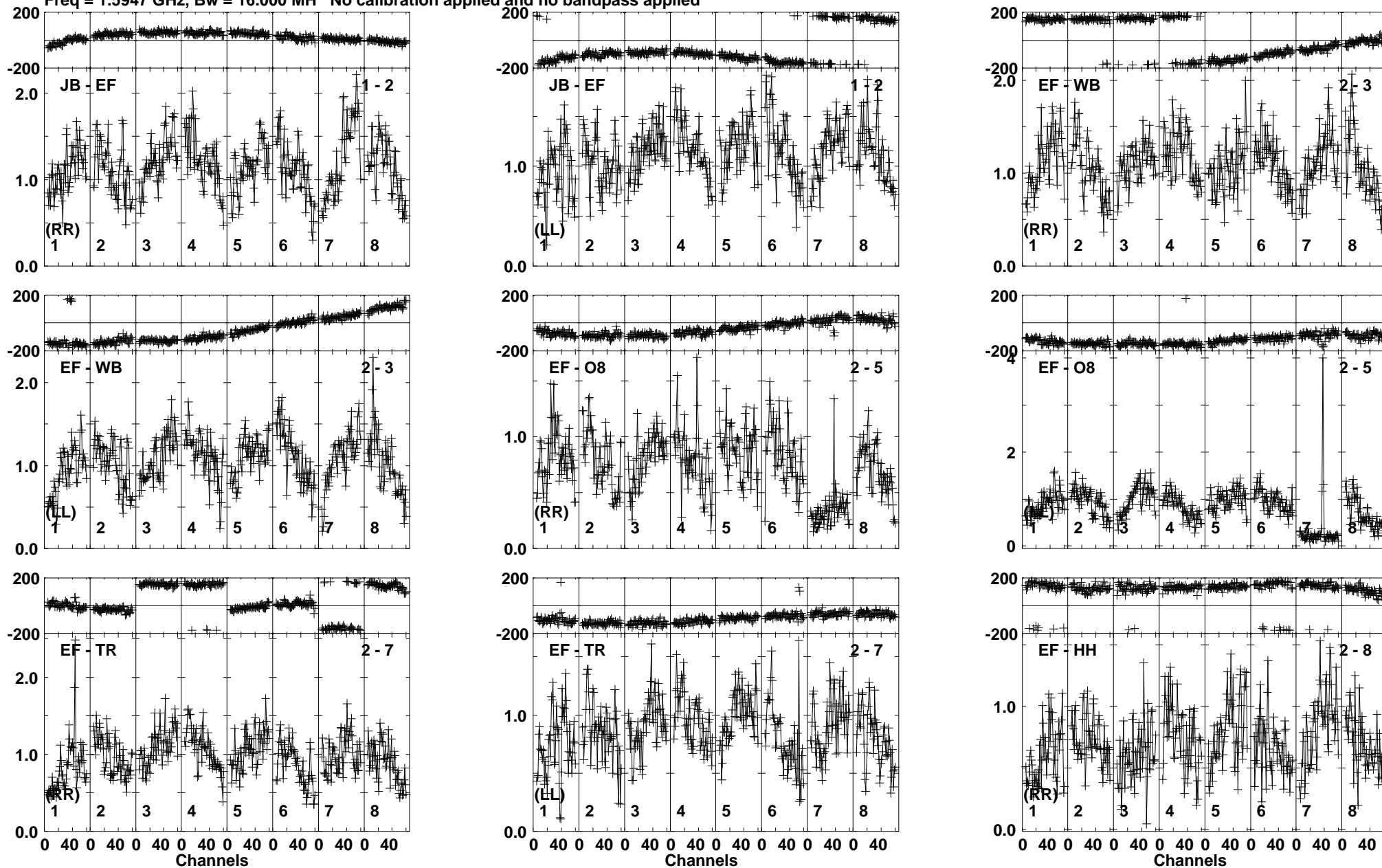
Lower frame: Milli Ampl Jy Top frame: Phas deg Vector averaged cross-power spectrum Baseline: JB (01) - EF (02) Timerange: 00/06:57:01 to 00/06:57:59
