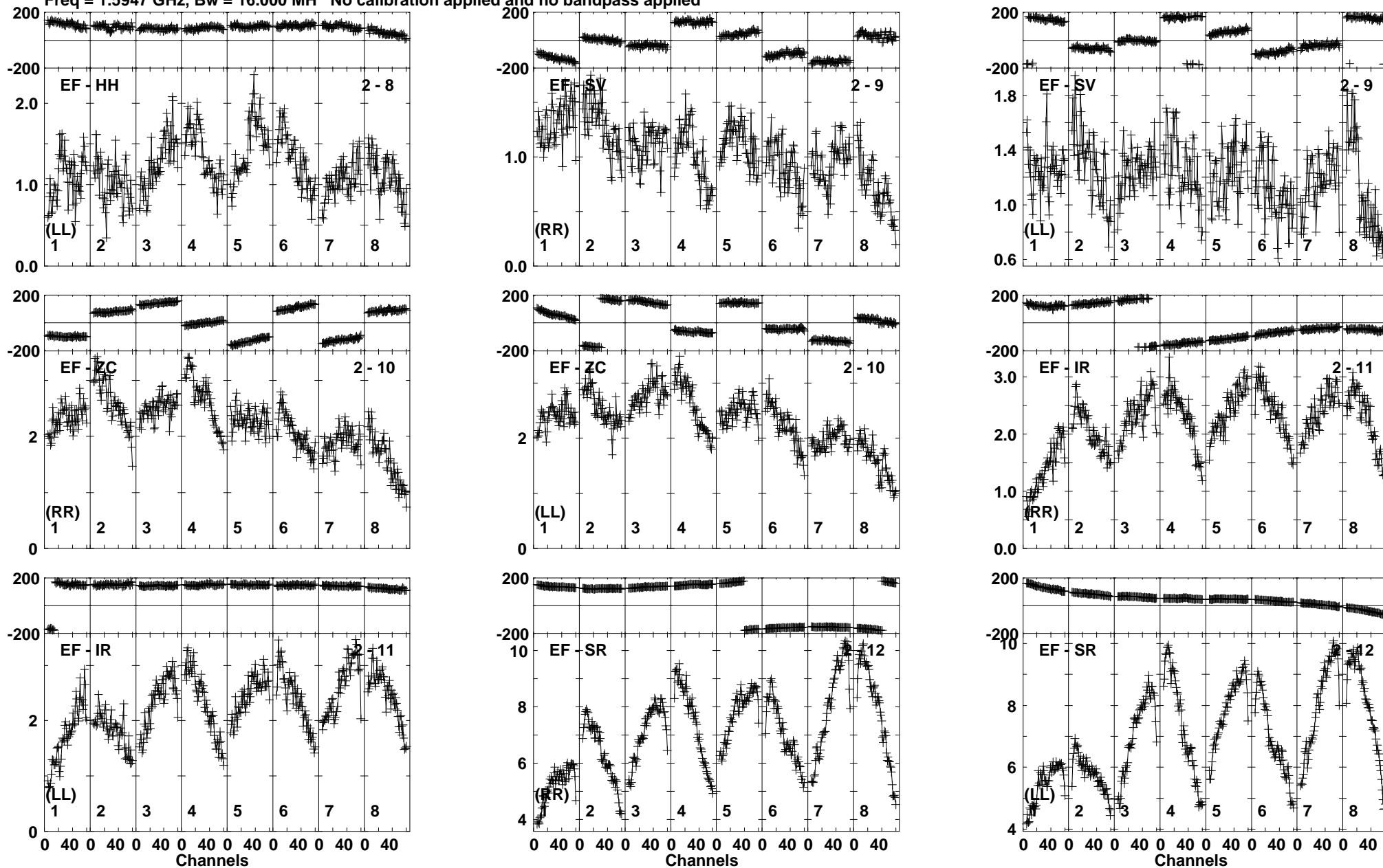
Lower frame: Milli Ampl Jy Top frame: Phas deg Vector averaged cross-power spectrum Baseline: EF (02) - HH (08) Timerange: 00/06:04:31 to 00/06:05:29
