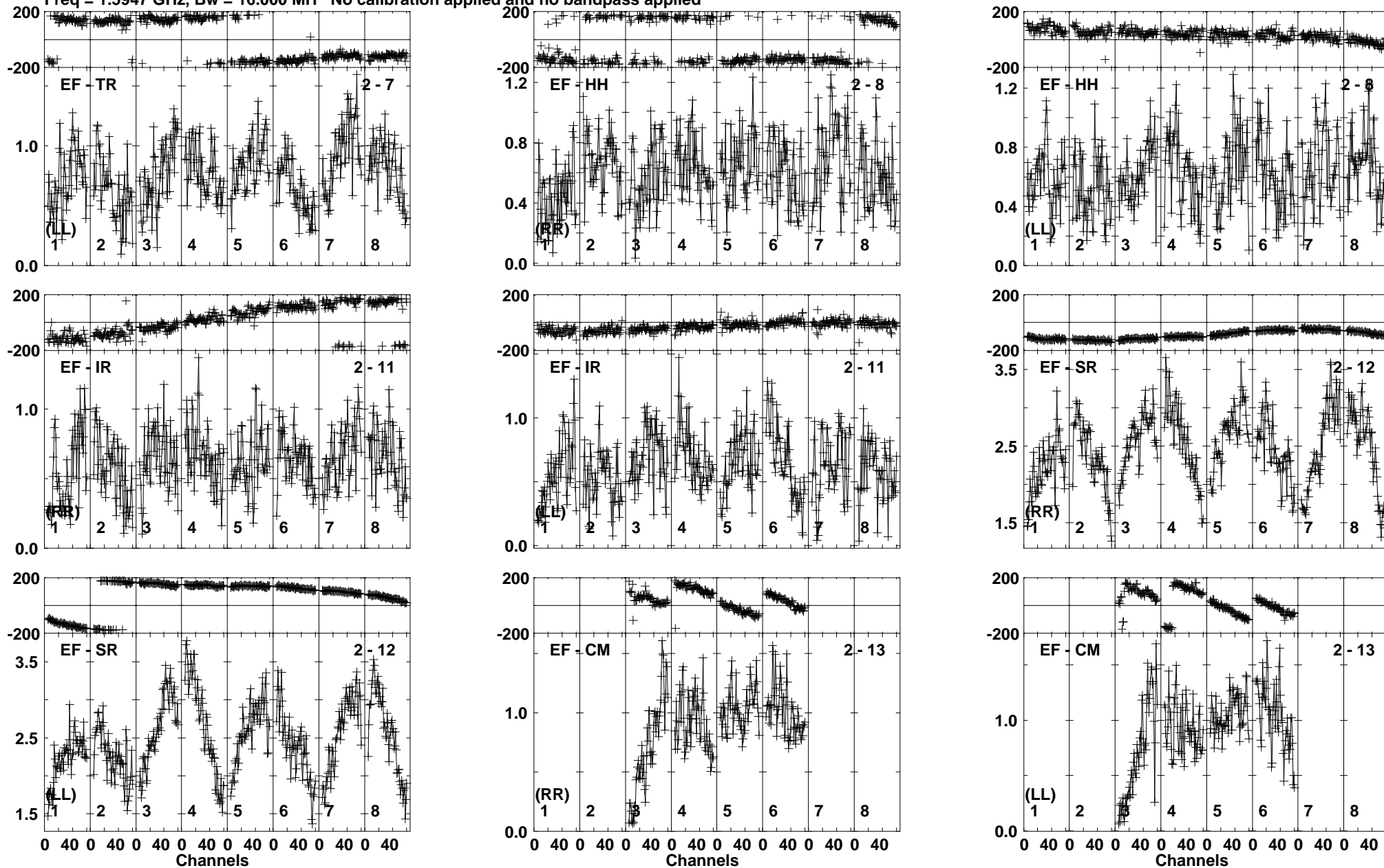
Lower frame: Milli Ampl Jy Top frame: Phas deg Vector averaged cross-power spectrum Baseline: EF (02) - TR (07) Timerange: 00/08:50:46 to 00/08:51:44
