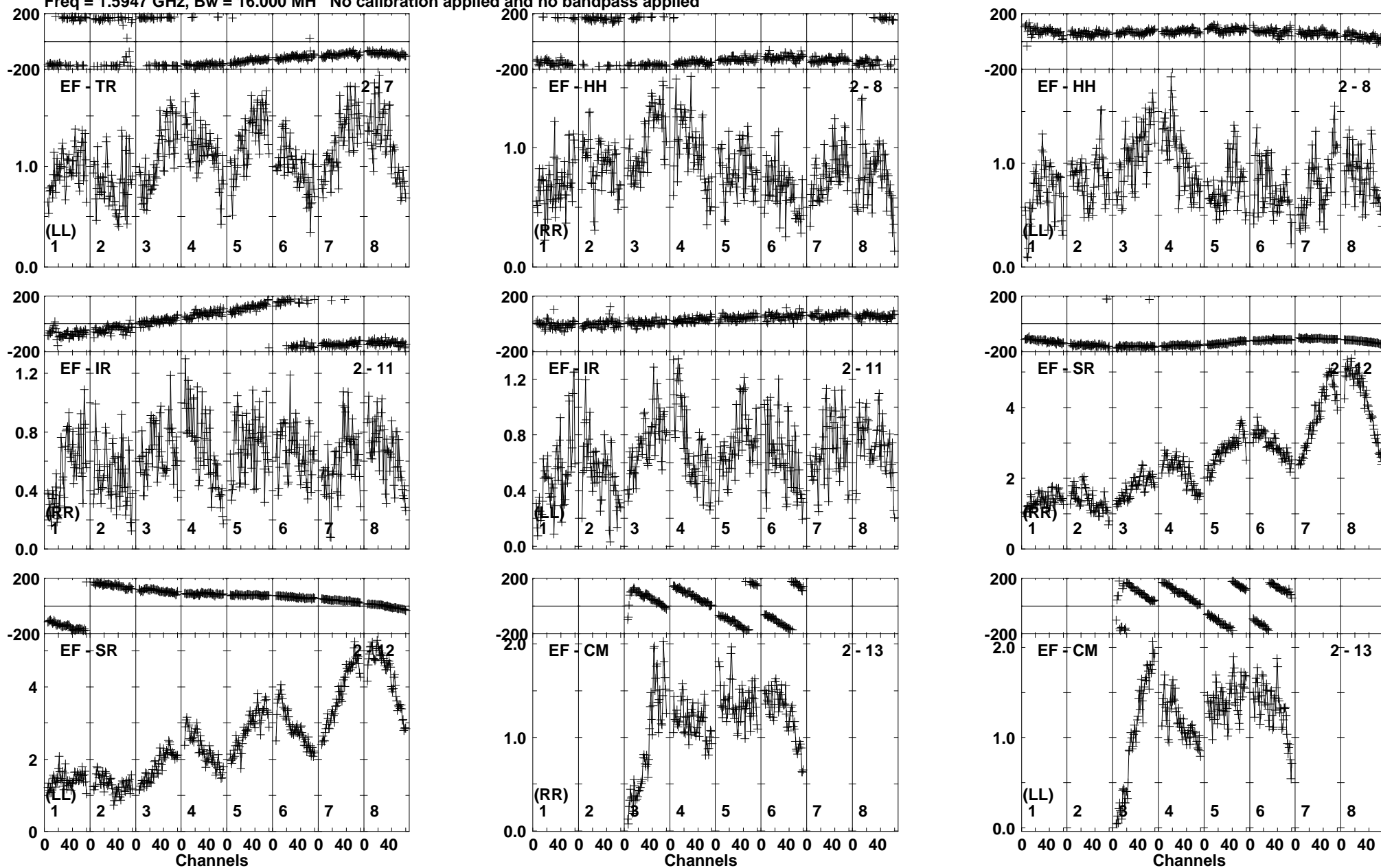
Lower frame: Milli Ampl Jy Top frame: Phas deg Vector averaged cross-power spectrum Baseline: EF (02) - TR (07) Timerange: 00/09:26:51 to 00/09:27:49
