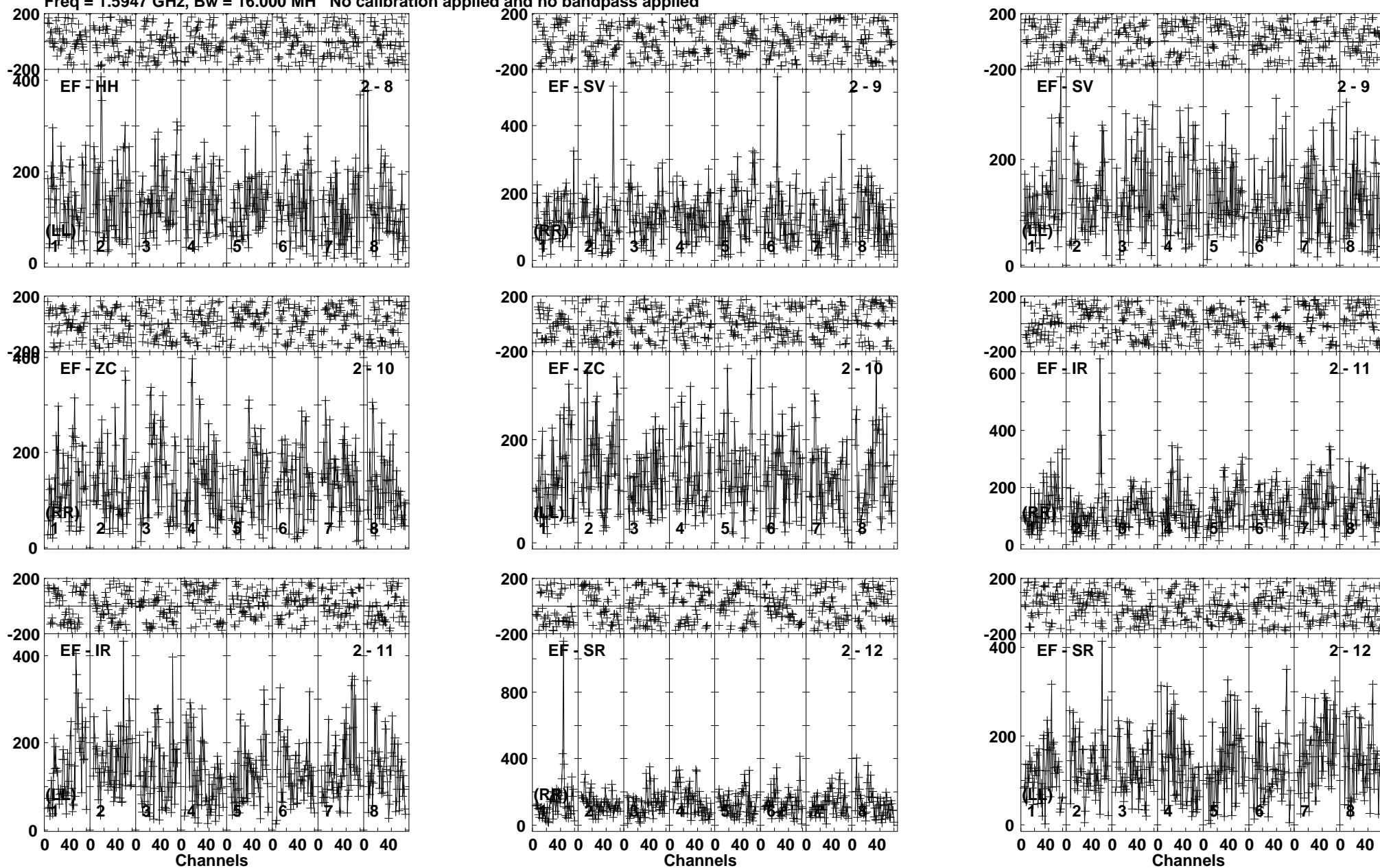
Lower frame: Micro Ampl Jy Top frame: Phas deg Vector averaged cross-power spectrum Baseline: EF (02) - HH (08) Timerange: 00/06:44:41 to 00/06:47:19
