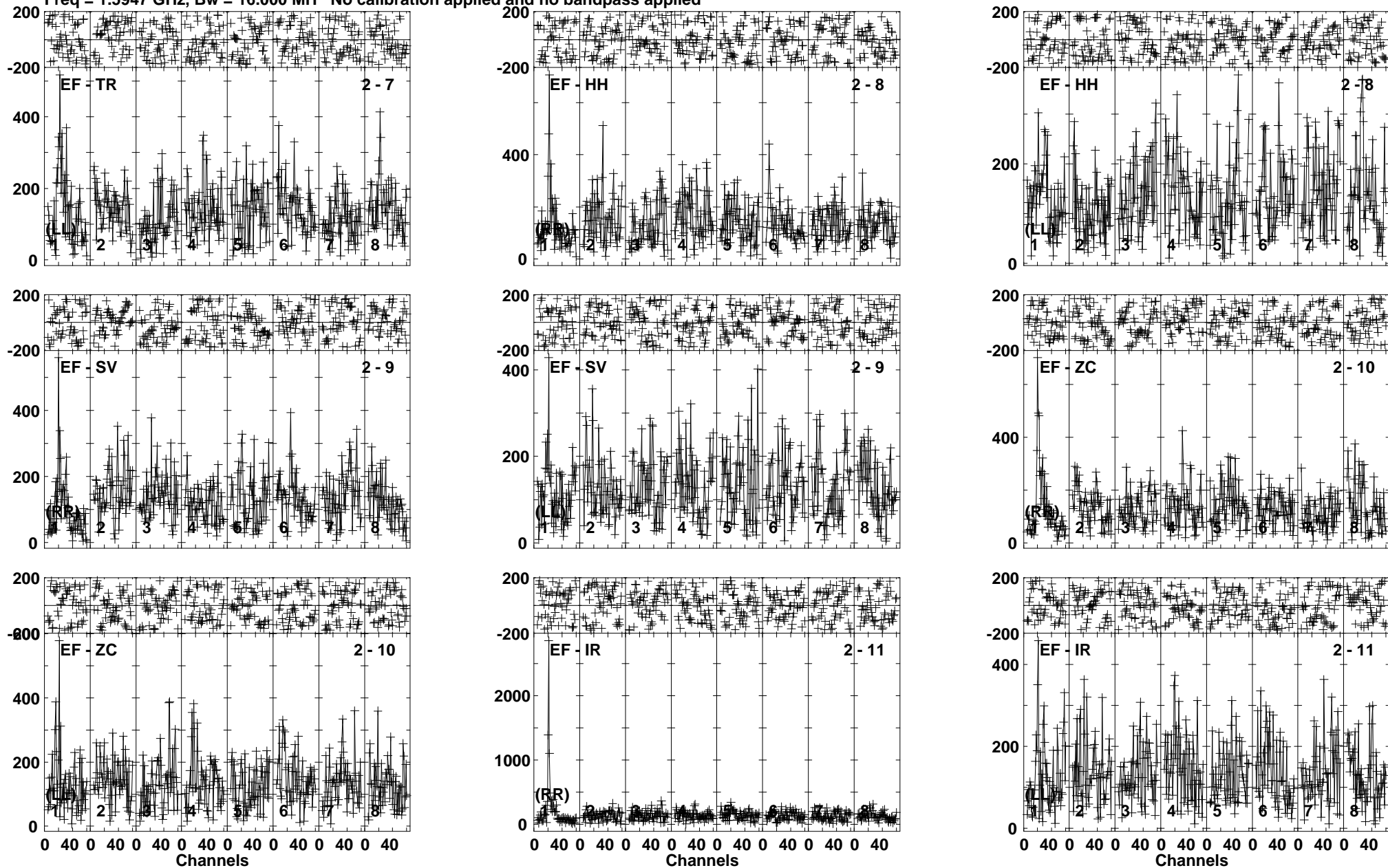
Lower frame: Micro Ampl Jy Top frame: Phas deg Vector averaged cross-power spectrum Baseline: EF (02) - TR (07) Timerange: 00/03:29:16 to 00/03:31:44
