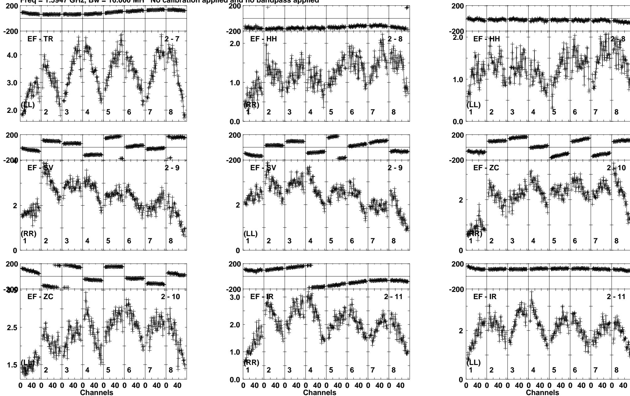
Lower frame: Milli Ampl Jy Top frame: Phas deg Vector averaged cross-power spectrum Baseline: EF (02) - TR (07) Timerange: 00/04:56:16 to 00/04:57:14
