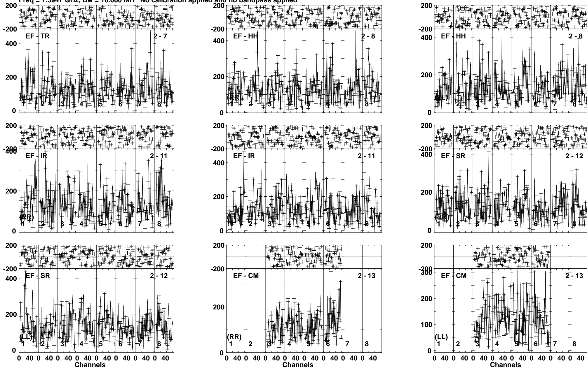
Lower frame: Micro Ampl Jy Top frame: Phas deg Vector averaged cross-power spectrum Baseline: EF (02) - TR (07) Timerange: 00/09:46:41 to 00/09:49:19
