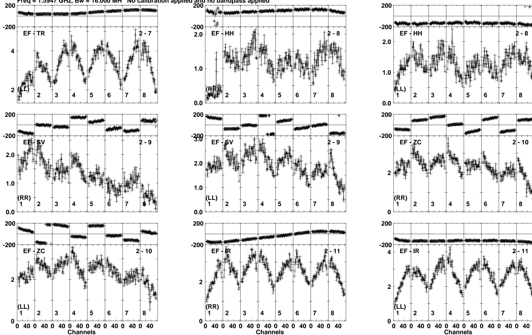
Lower frame: Milli Ampl Jy Top frame: Phas deg Vector averaged cross-power spectrum Baseline: EF (02) - TR (07) Timerange: 00/05:33:36 to 00/05:34:34
