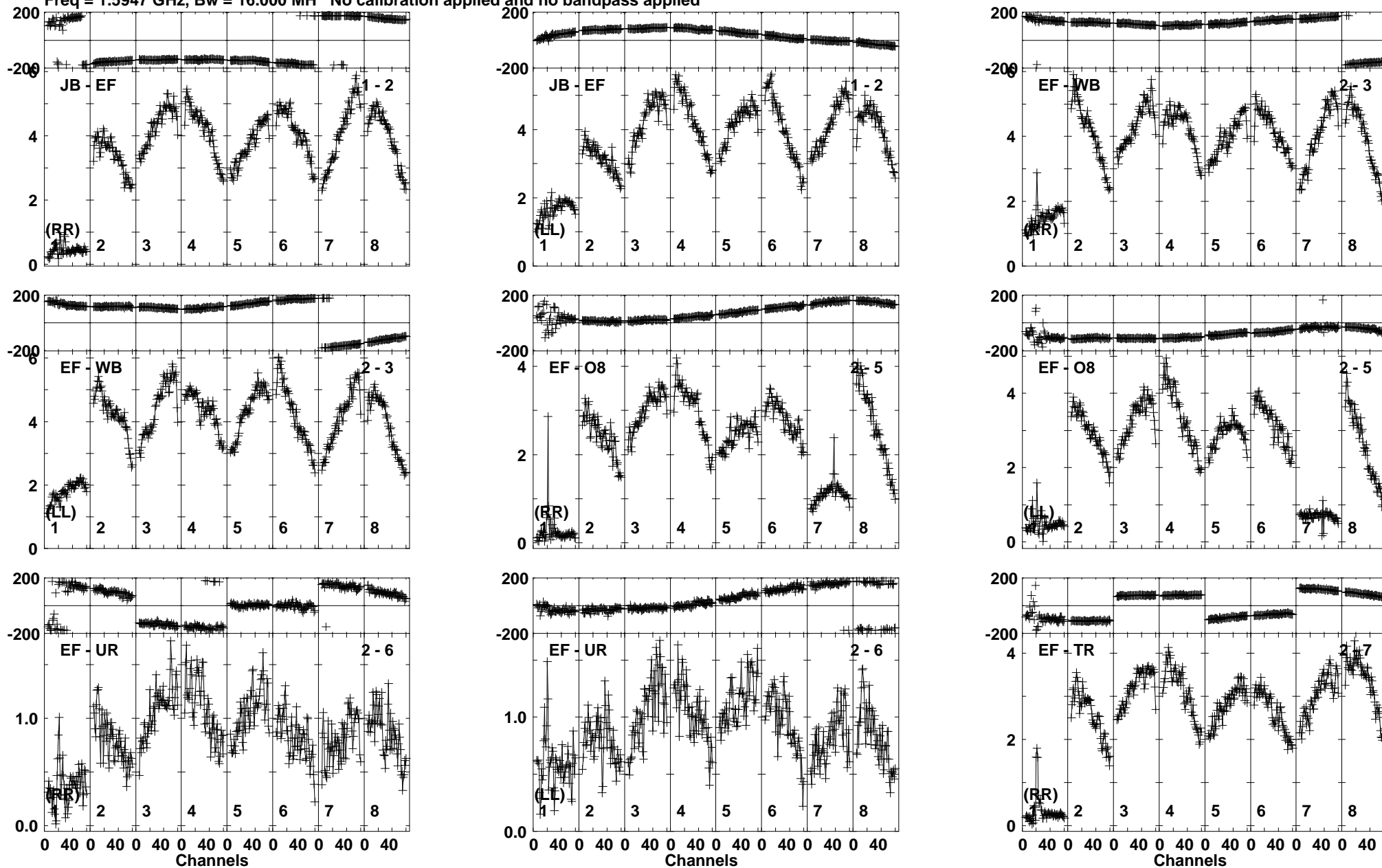
Lower frame: Milli Ampl Jy Top frame: Phas deg Vector averaged cross-power spectrum Baseline: JB (01) - EF (02) Timerange: 00/03:32:01 to 00/03:32:59
