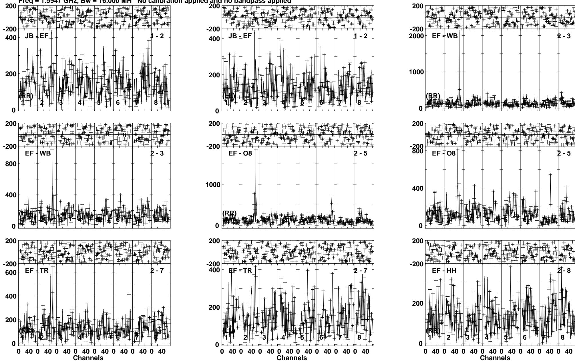
Lower frame: Micro Ampl Jy Top frame: Phas deg Vector averaged cross-power spectrum Baseline: JB (01) - EF (02) Timerange: 00/07:26:16 to 00/07:28:54
