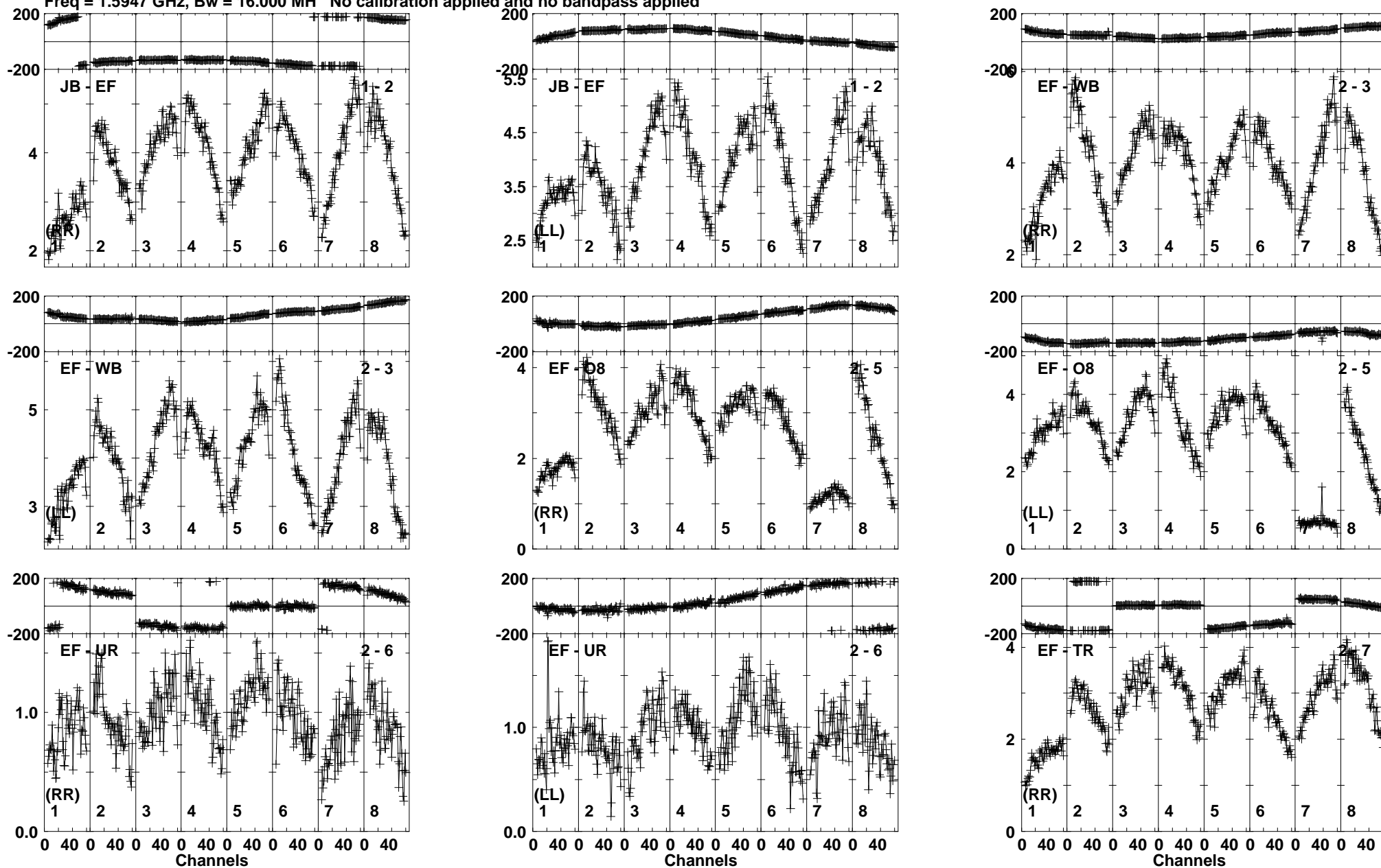
Lower frame: Milli Ampl Jy Top frame: Phas deg Vector averaged cross-power spectrum Baseline: JB (01) - EF (02) Timerange: 00/03:25:16 to 00/03:26:14
