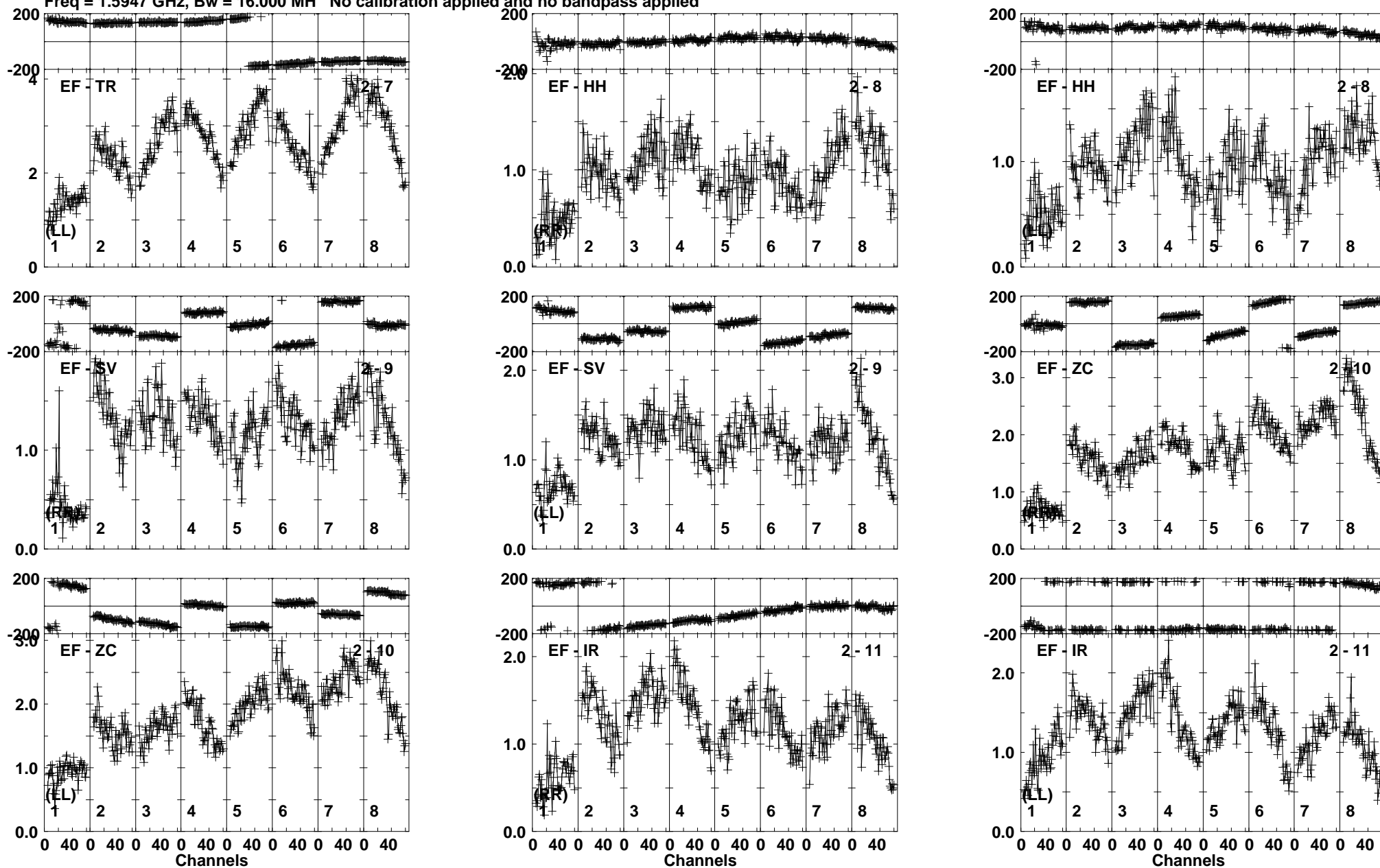
Lower frame: Milli Ampl Jy Top frame: Phas deg Vector averaged cross-power spectrum Baseline: EF (02) - TR (07) Timerange: 00/03:32:01 to 00/03:32:59
