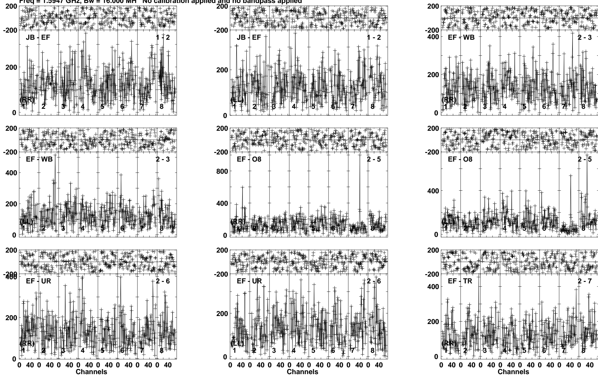
Lower frame: Micro Ampl Jy Top frame: Phas deg Vector averaged cross-power spectrum Baseline: JB (01) - EF (02) Timerange: 00/04:07:51 to 00/04:10:29
