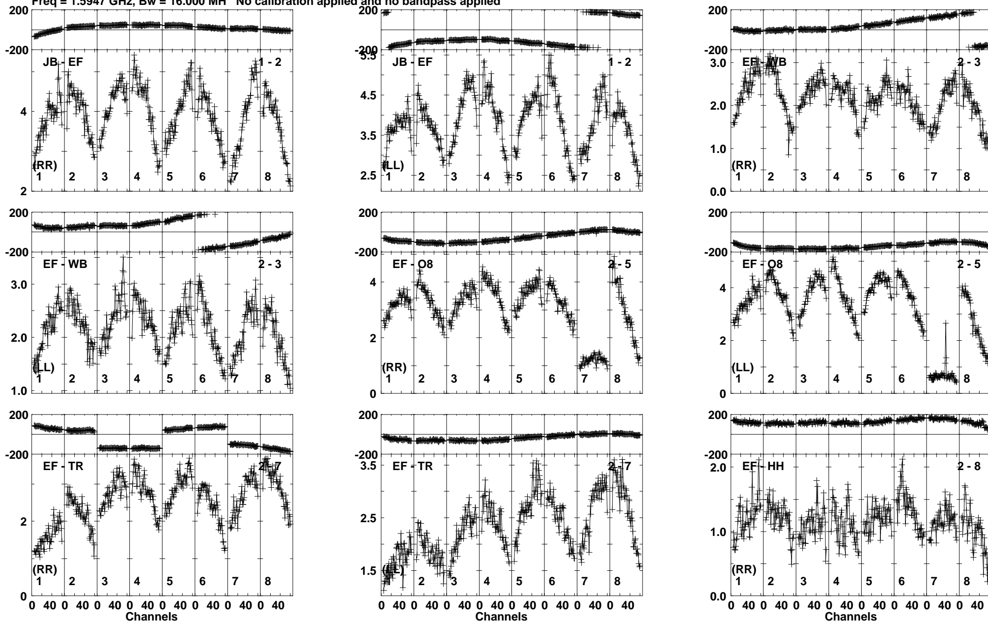
Lower frame: Milli Ampl Jy Top frame: Phas deg Vector averaged cross-power spectrum Baseline: JB (01) - EF (02) Timerange: 00:06:47:36 to 00:06:48:34
