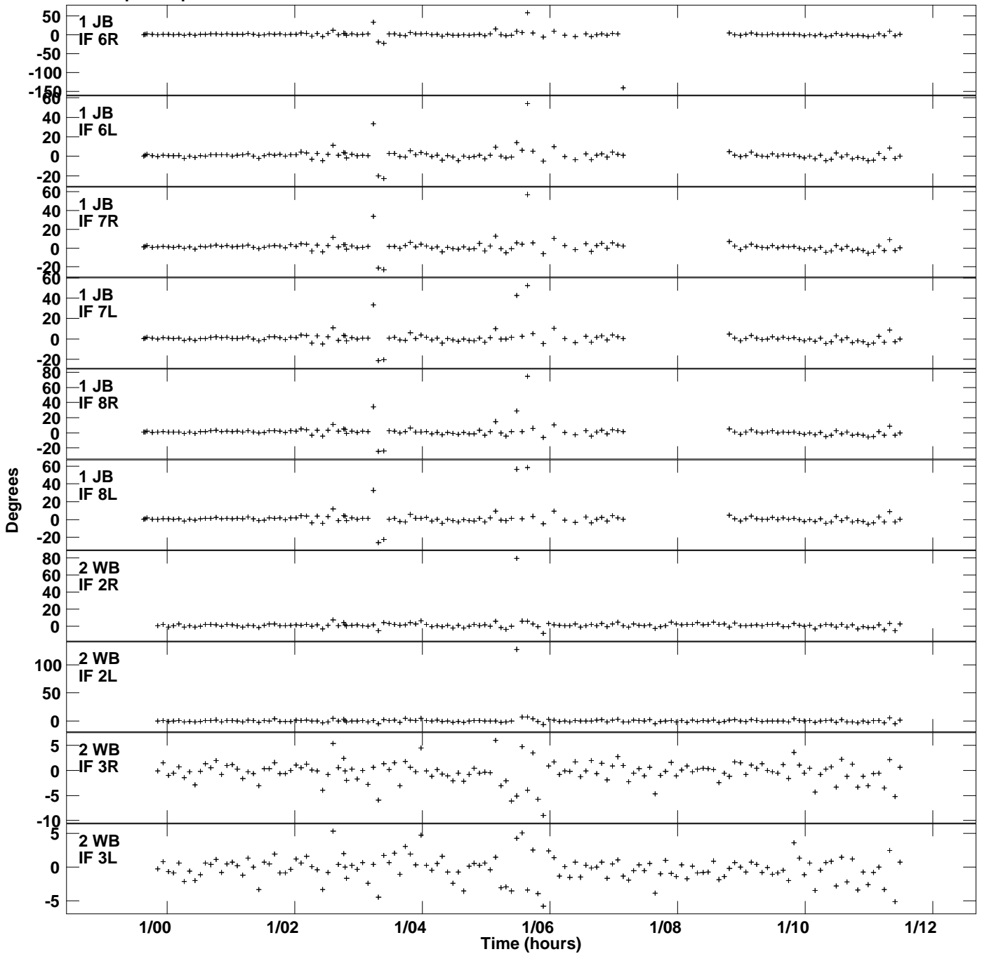
Plot file version 2 created 19-JUL-2021 16:26:58 Gain phs vs UTC time for J0854+5757.MULTI.1 SN 1 Rpol & Lpol IF 1 - 8
