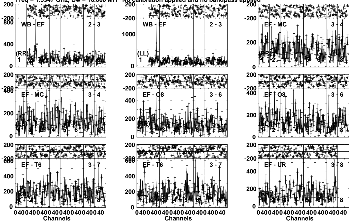
Lower frame: Micro Ampl Jy Top frame: Phas deg Vector averaged cross-power spectrum Several baselines displayed Timerange: 01/03:29:50 to 01/03:32:39
