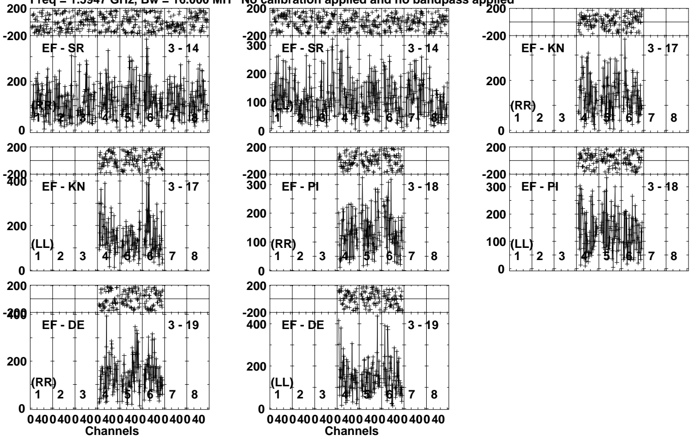
Lower frame: Micro Ampl Jy Top frame: Phas deg Vector averaged cross-power spectrum Several baselines displayed Timerange: 01/00:32:10 to 01/00:35:09
