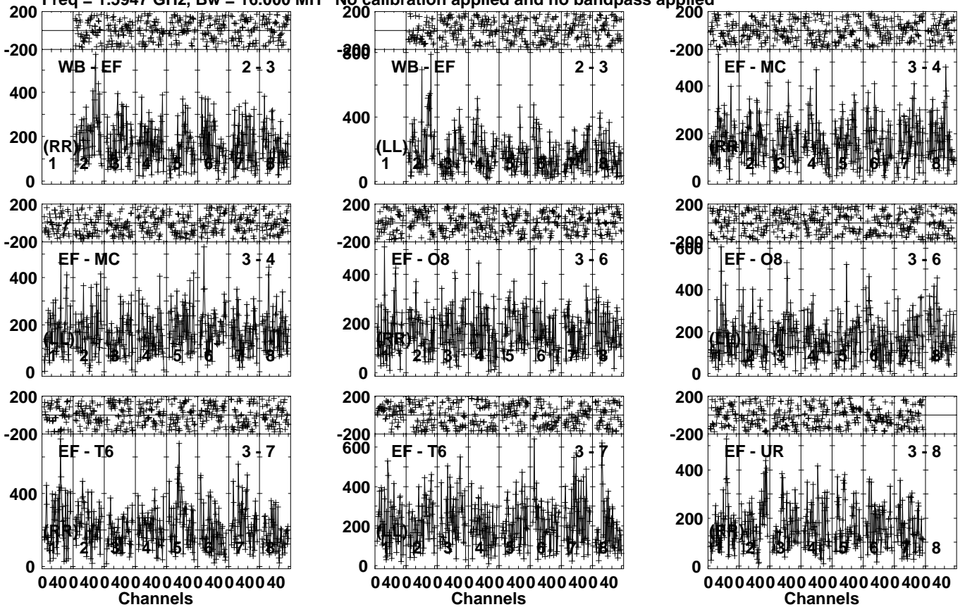
Lower frame: Micro Ampl Jy Top frame: Phas deg Vector averaged cross-power spectrum Several baselines displayed Timerange: 01/05:29:51 to 01/05:32:39
