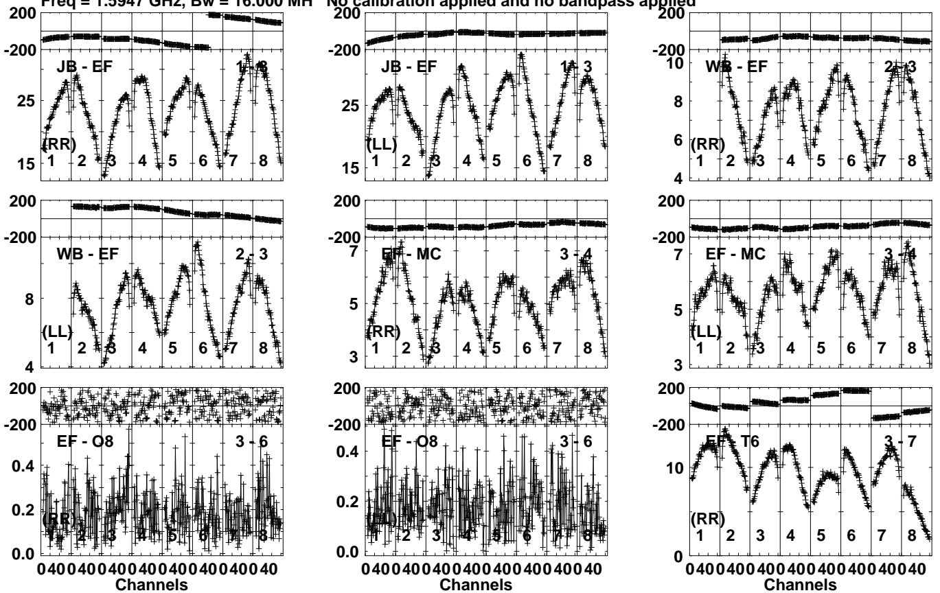
Lower frame: Milli Ampl Jy Top frame: Phas deg Vector averaged cross-power spectrum Several baselines displayed Timerange: 01/01:30:40 to 01/01:31:50
