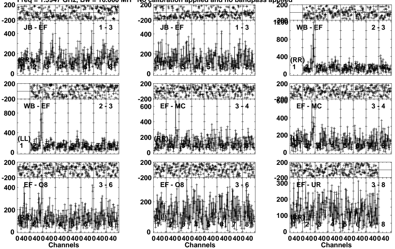
Lower frame: Micro Ampl Jy Top frame: Phas deg Vector averaged cross-power spectrum Several baselines displayed Timerange: 01/10:15:21 to 01/10:18:19
