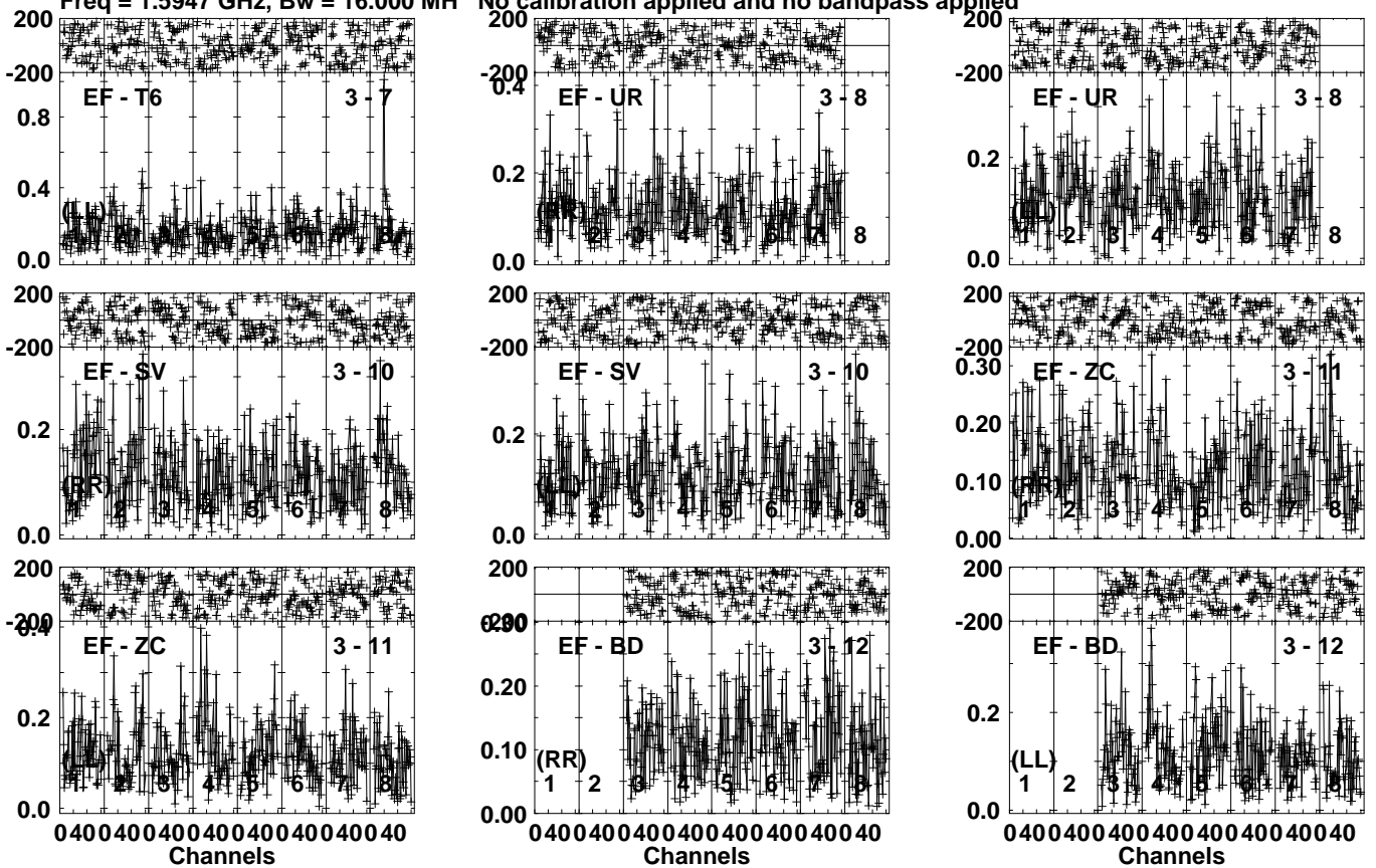
Lower frame: Milli Ampl Jy Top frame: Phas deg Vector averaged cross-power spectrum Several baselines displayed Timerange: 01/01:42:10 to 01/01:45:10
