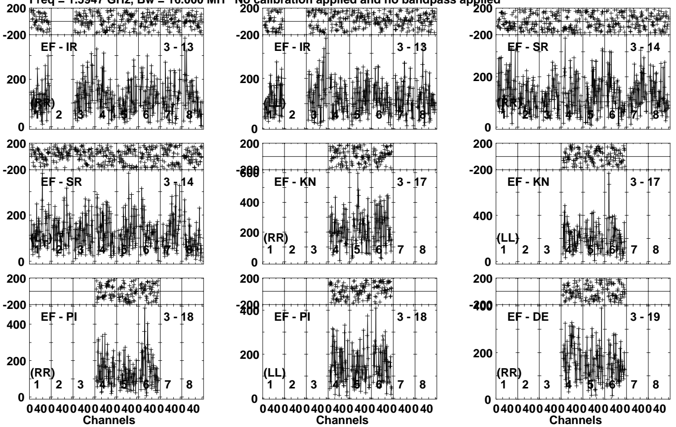
Lower frame: Micro Ampl Jy Top frame: Phas deg Vector averaged cross-power spectrum Several baselines displayed Timerange: 01/06:34:51 to 01/06:37:49
