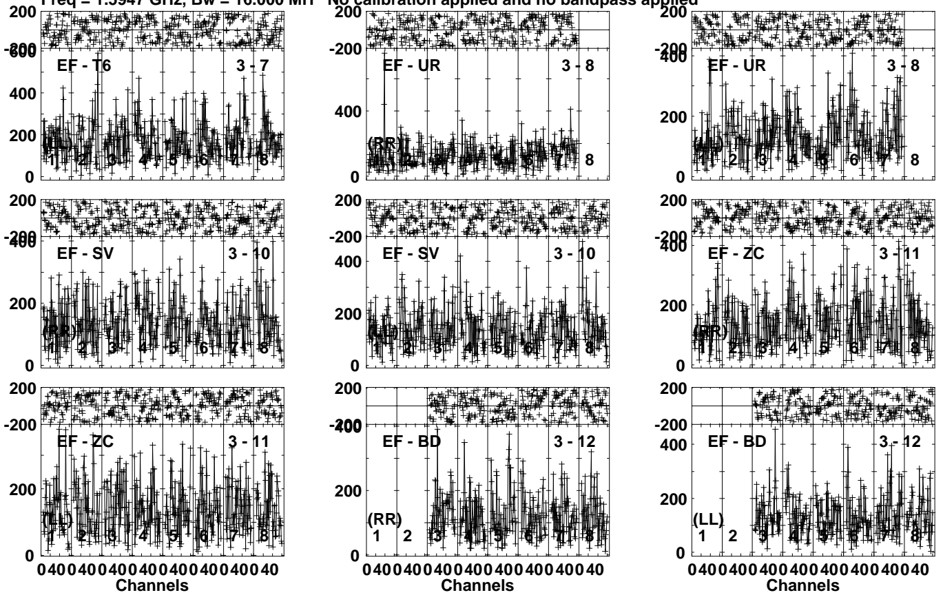
Lower frame: Micro Ampl Jy Top frame: Phas deg Vector averaged cross-power spectrum Several baselines displayed Timerange: 01/06:04:50 to 01/06:07:50
