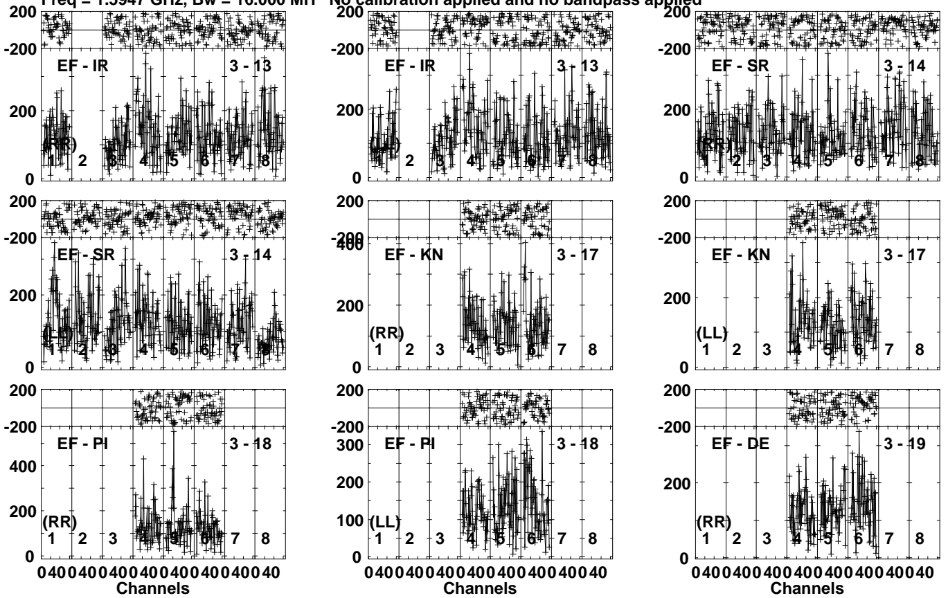
Lower frame: Micro Ampl Jy Top frame: Phas deg Vector averaged cross-power spectrum Several baselines displayed Timerange: 01/03:04:50 to 01/03:07:50
