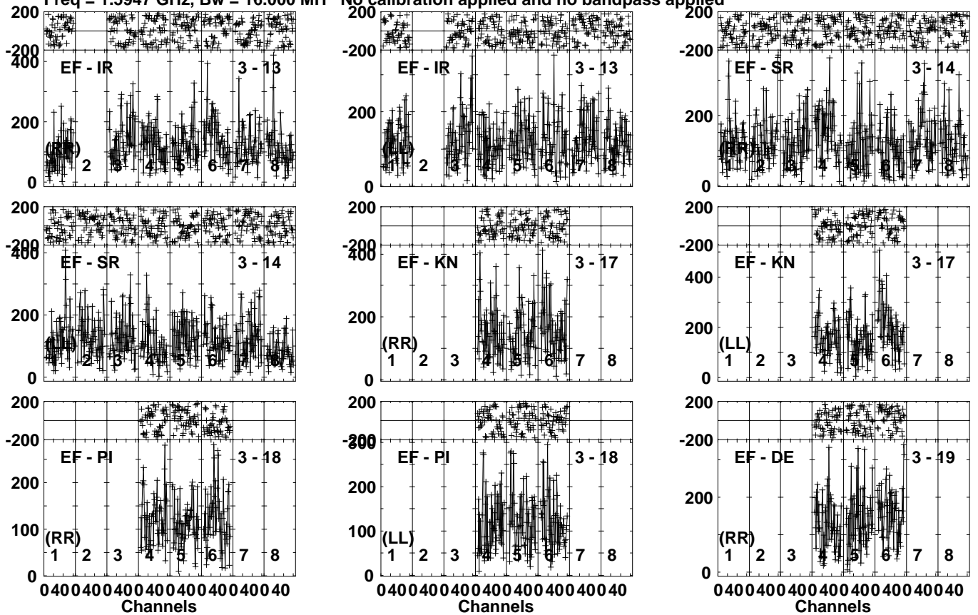
Lower frame: Micro Ampl Jy Top frame: Phas deg Vector averaged cross-power spectrum Several baselines displayed Timerange: 01/01:52:10 to 01/01:55:10
