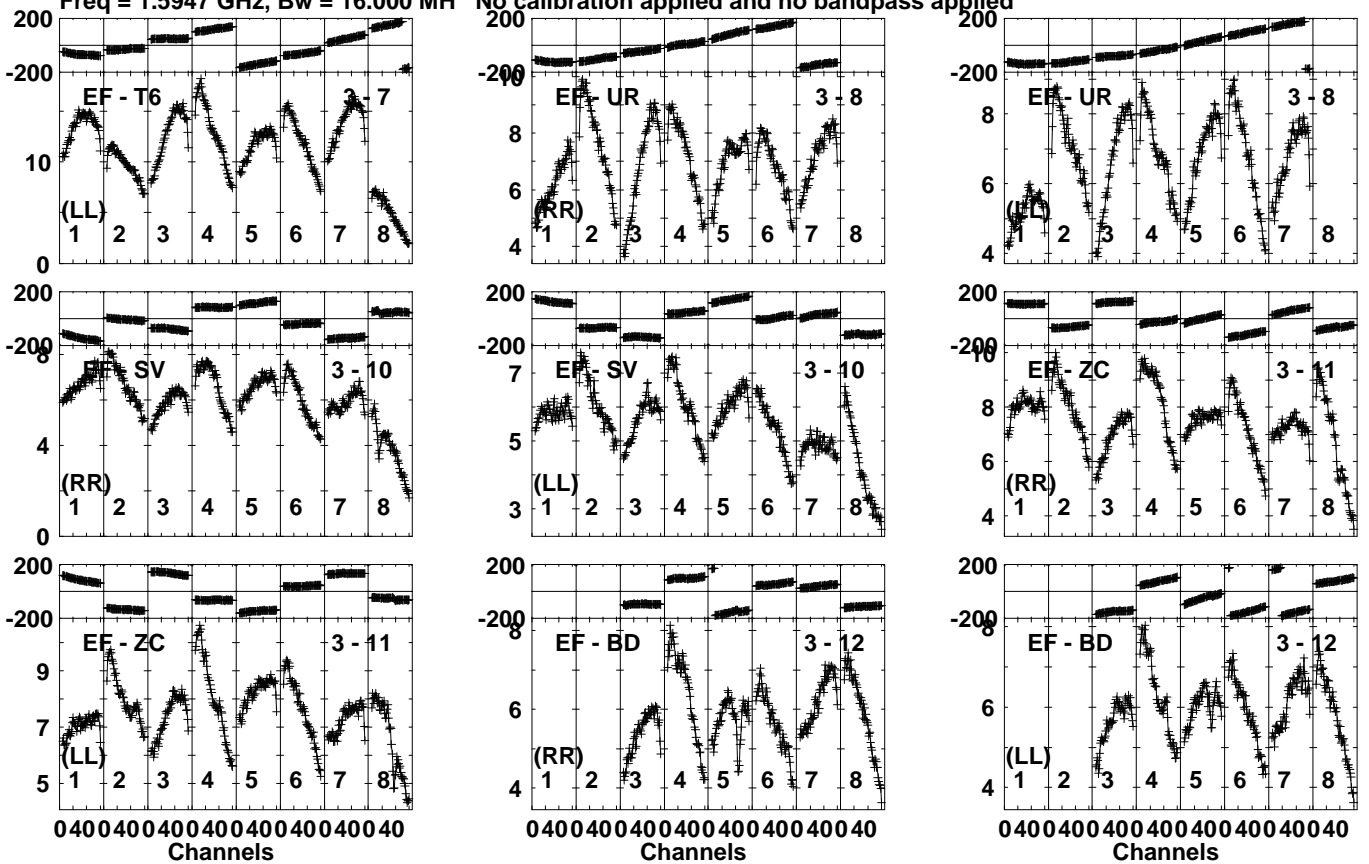
Lower frame: Milli Ampl Jy Top frame: Phas deg Vector averaged cross-power spectrum Several baselines displayed Timerange: 01/06:13:20 to 01/06:14:29
