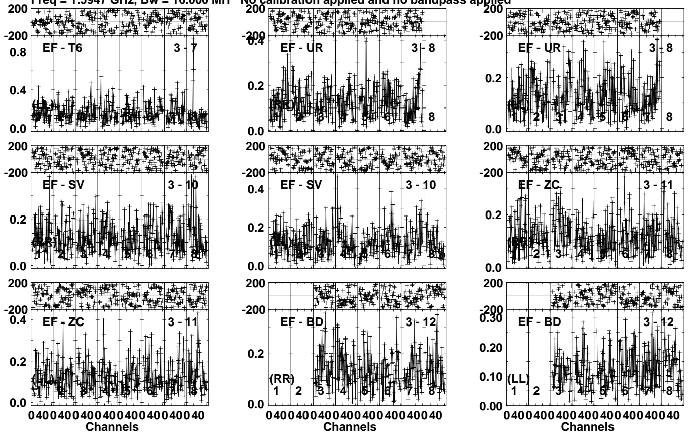
Lower frame: Milli Ampl Jy Top frame: Phas deg Vector averaged cross-power spectrum Several baselines displayed Timerange: 01/02:32:11 to 01/02:35:10
