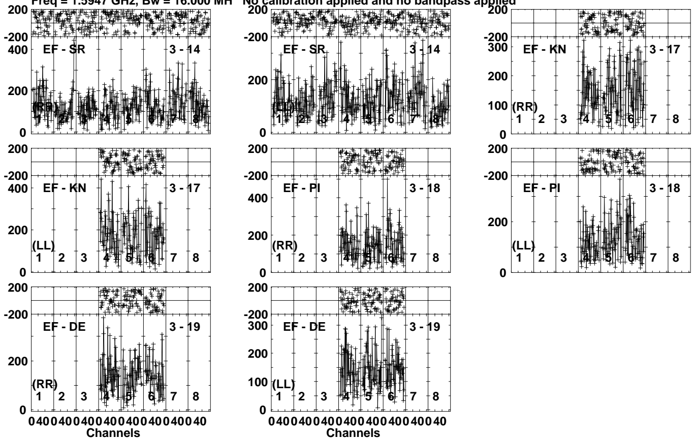
Lower frame: Micro Ampl Jy Top frame: Phas deg Vector averaged cross-power spectrum Several baselines displayed Timerange: 01/03:09:51 to 01/03:12:39
