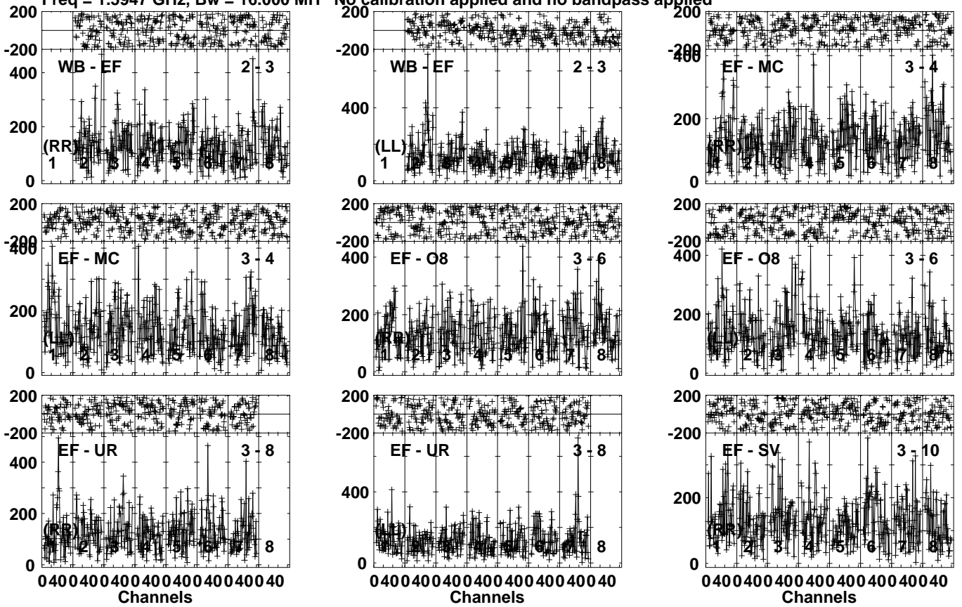
Lower frame: Micro Ampl Jy Top frame: Phas deg Vector averaged cross-power spectrum Several baselines displayed Timerange: 01/09:30:20 to 01/09:33:09
