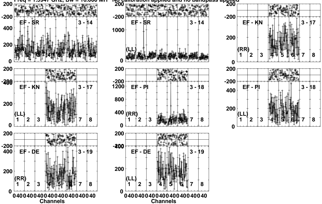
Lower frame: Micro Ampl Jy Top frame: Phas deg Vector averaged cross-power spectrum Several baselines displayed Timerange: 01/06:09:51 to 01/06:12:39
