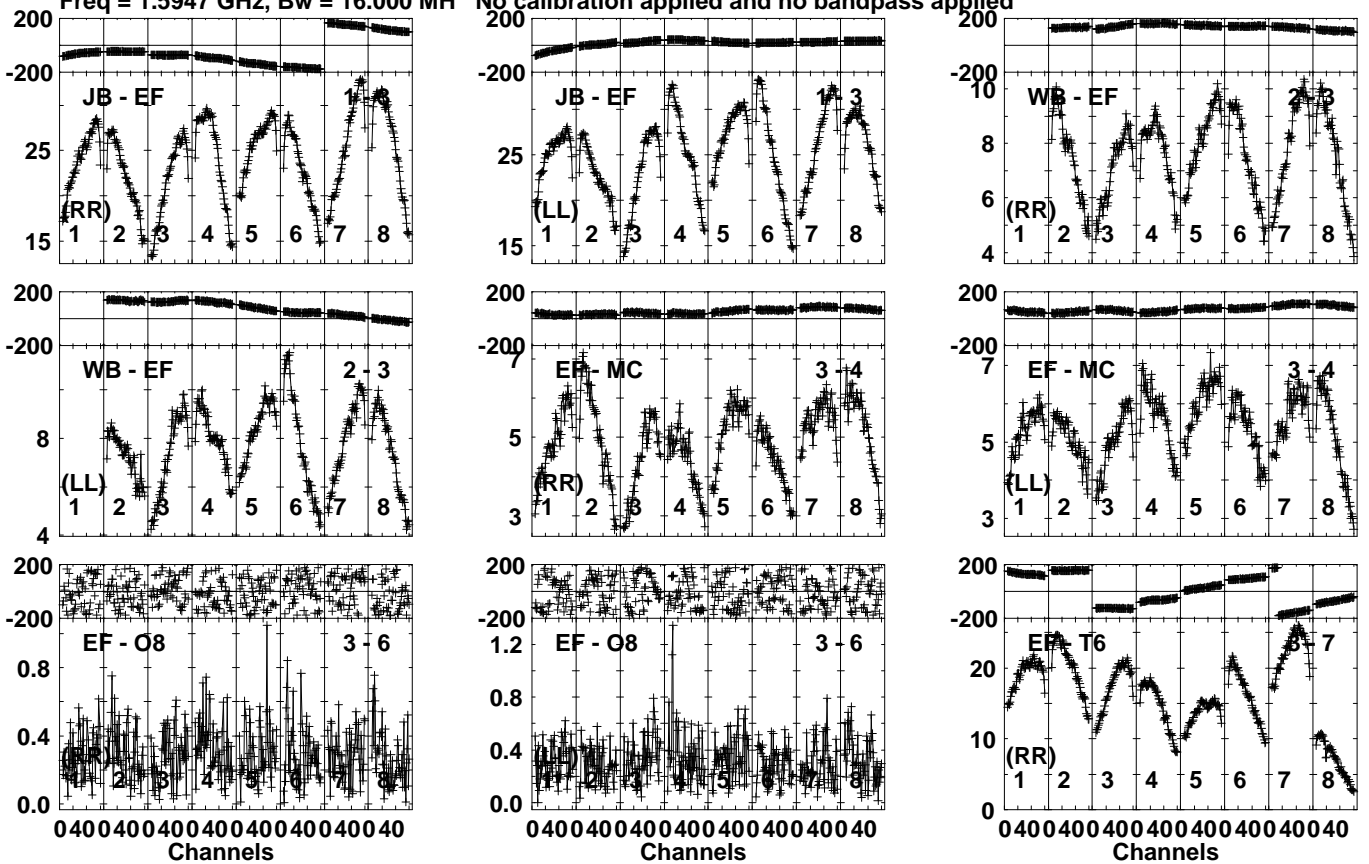
Lower frame: Milli Ampl Jy Top frame: Phas deg Vector averaged cross-power spectrum Several baselines displayed Timerange: 01/05:13:21 to 01/05:14:30
