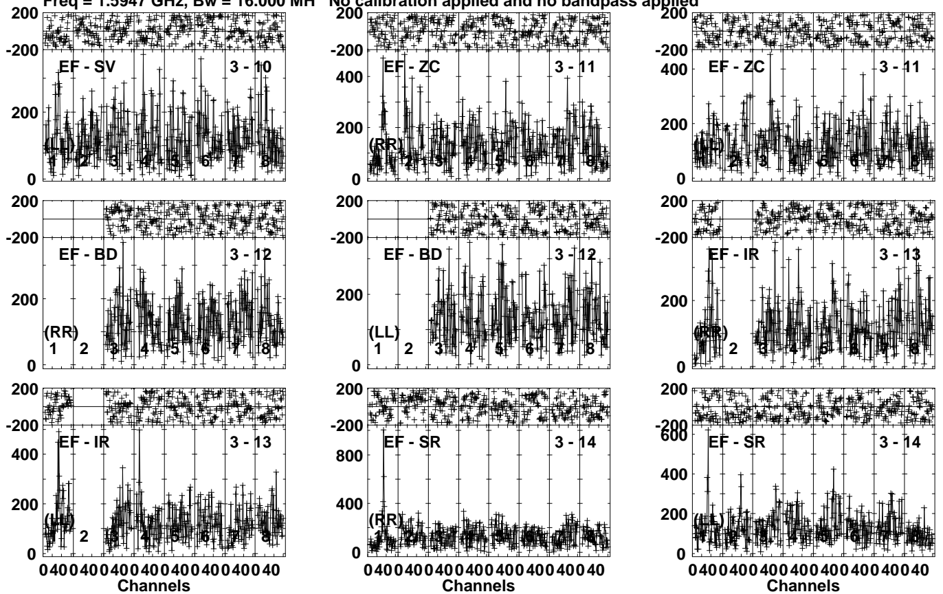
Lower frame: Micro Ampl Jy Top frame: Phas deg Vector averaged cross-power spectrum Several baselines displayed Timerange: 01/10:00:21 to 01/10:03:10
