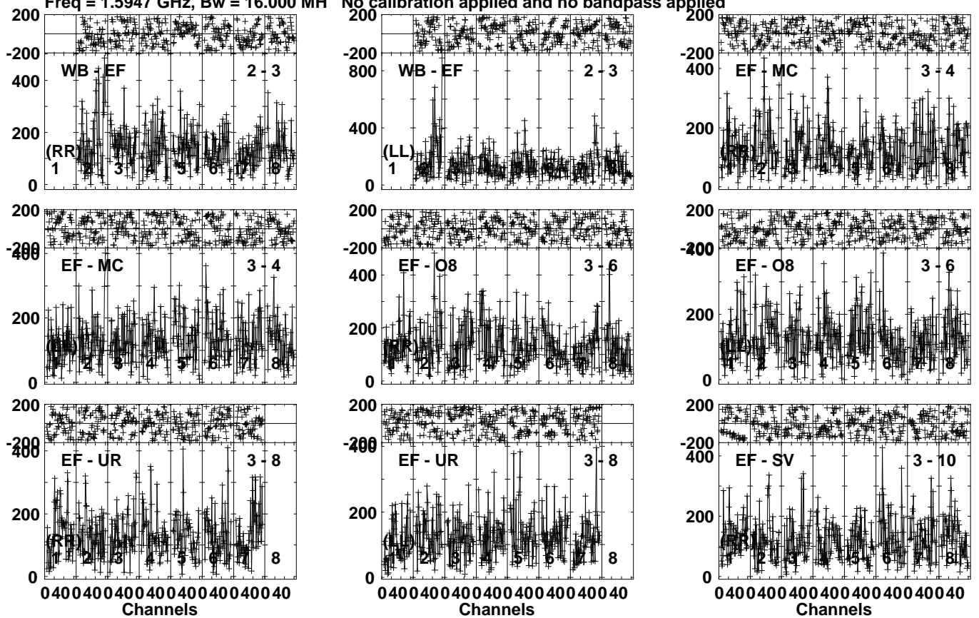
Lower frame: Micro Ampl Jy Top frame: Phas deg Vector averaged cross-power spectrum Several baselines displayed Timerange: 01/07:09:51 to 01/07:12:40
