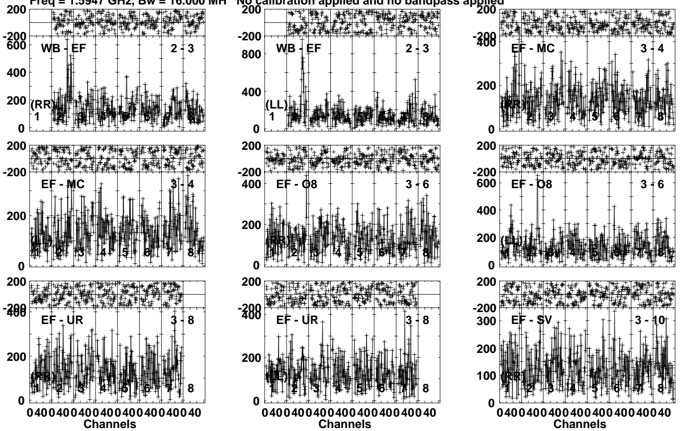
Lower frame: Micro Ampl Jy Top frame: Phas deg Vector averaged cross-power spectrum Several baselines displayed Timerange: 01/07:59:50 to 01/08:02:39
