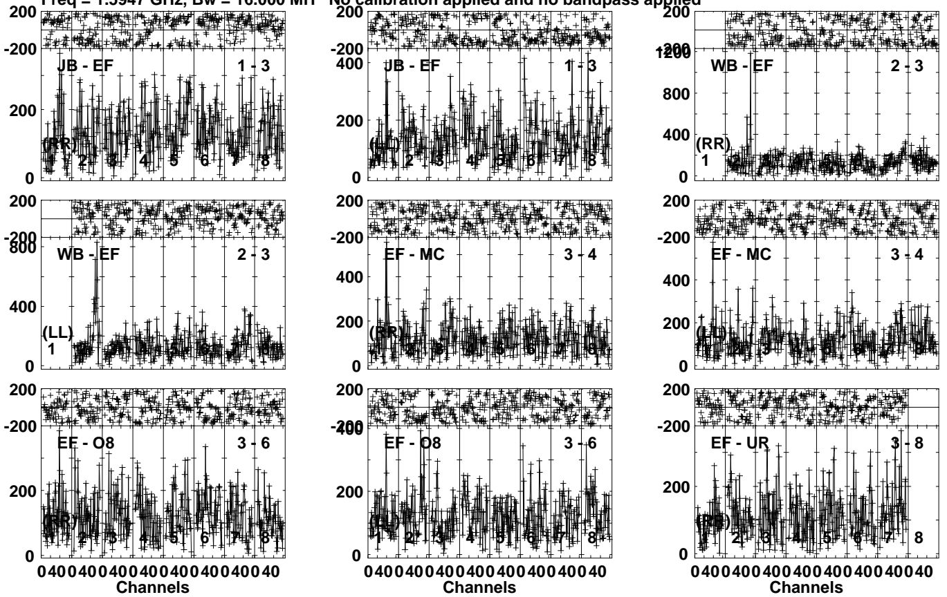
Lower frame: Micro Ampl Jy Top frame: Phas deg Vector averaged cross-power spectrum Several baselines displayed Timerange: 01/11:25:20 to 01/11:28:20
