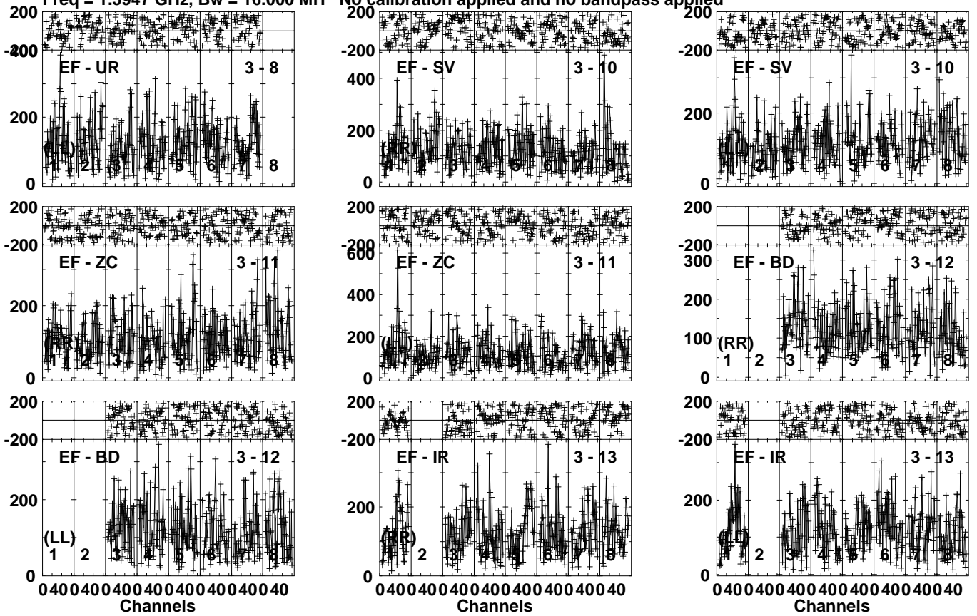
Lower frame: Micro Ampl Jy Top frame: Phas deg Vector averaged cross-power spectrum Several baselines displayed Timerange: 01/09:05:21 to 01/09:08:20
