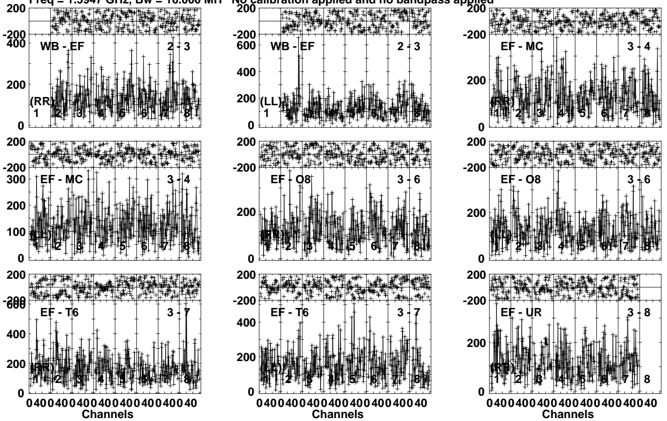
Lower frame: Micro Ampl Jy Top frame: Phas deg Vector averaged cross-power spectrum Several baselines displayed Timerange: 01/01:07:11 to 01/01:09:59
