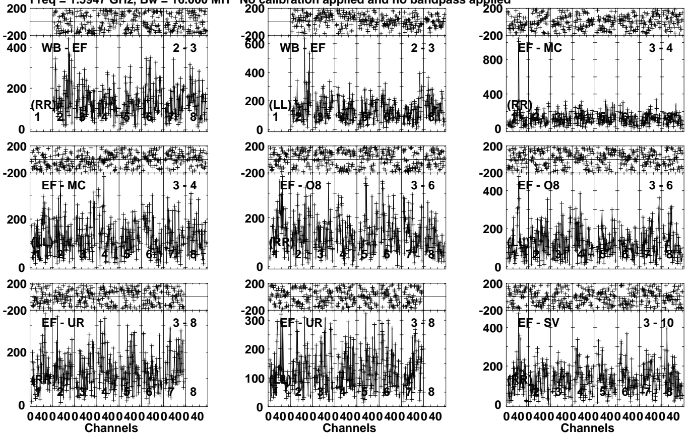
Lower frame: Micro Ampl Jy Top frame: Phas deg Vector averaged cross-power spectrum Several baselines displayed Timerange: 01/09:10:22 to 01/09:13:10
