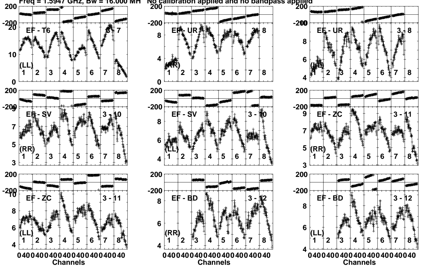
Lower frame: Milli Ampl Jy Top frame: Phas deg Vector averaged cross-power spectrum Several baselines displayed Timerange: 01/05:43:20 to 01/05:44:30
