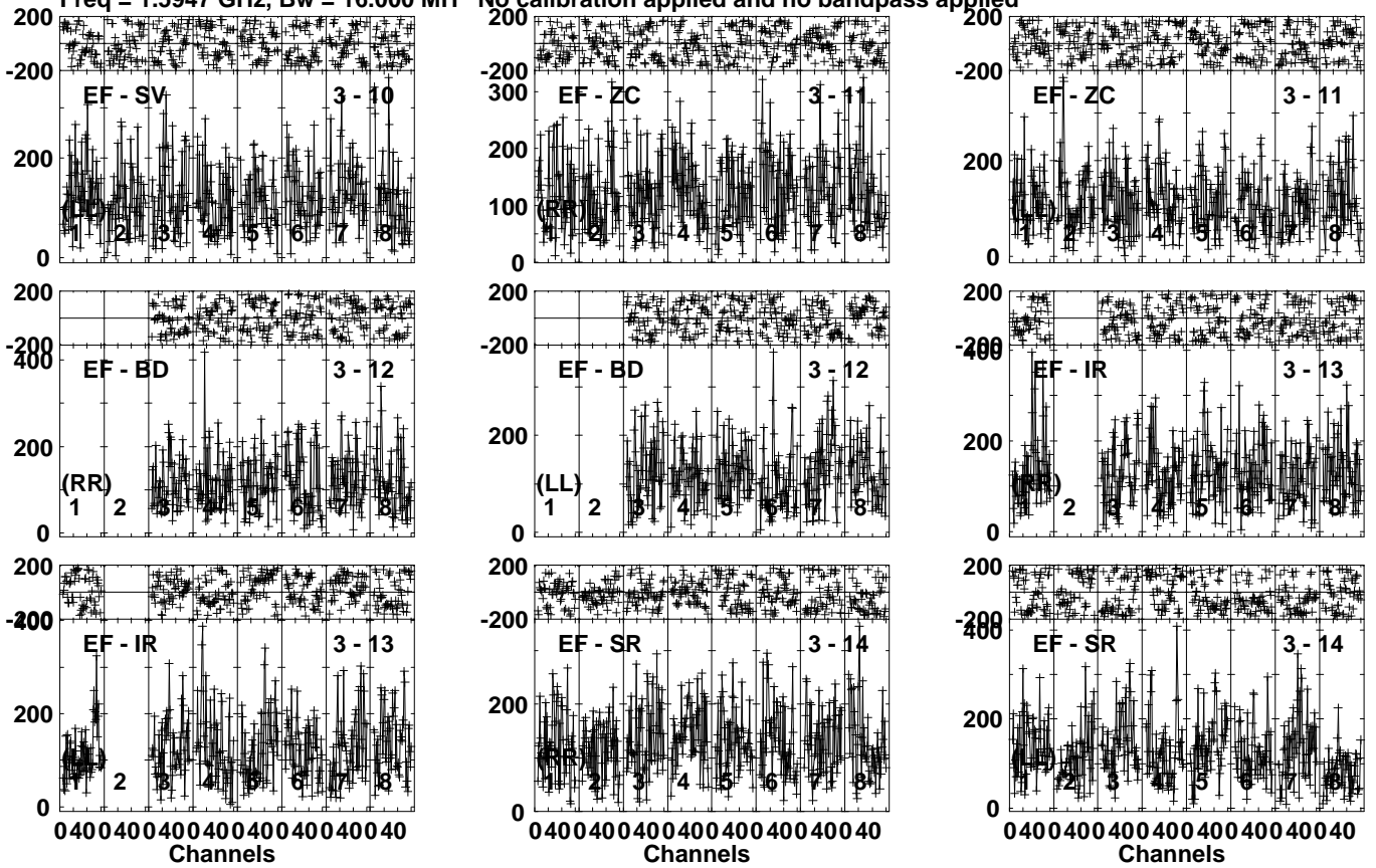
Lower frame: Micro Ampl Jy Top frame: Phas deg Vector averaged cross-power spectrum Several baselines displayed Timerange: 01/10:50:22 to 01/10:53:10
