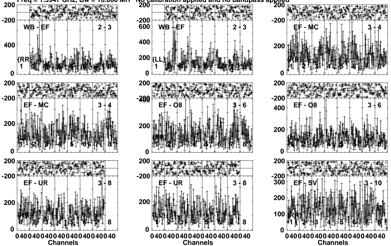
Lower frame: Micro Ampl Jy Top frame: Phas deg Vector averaged cross-power spectrum Several baselines displayed Timerange: 01/06:59:51 to 01/07:02:39
