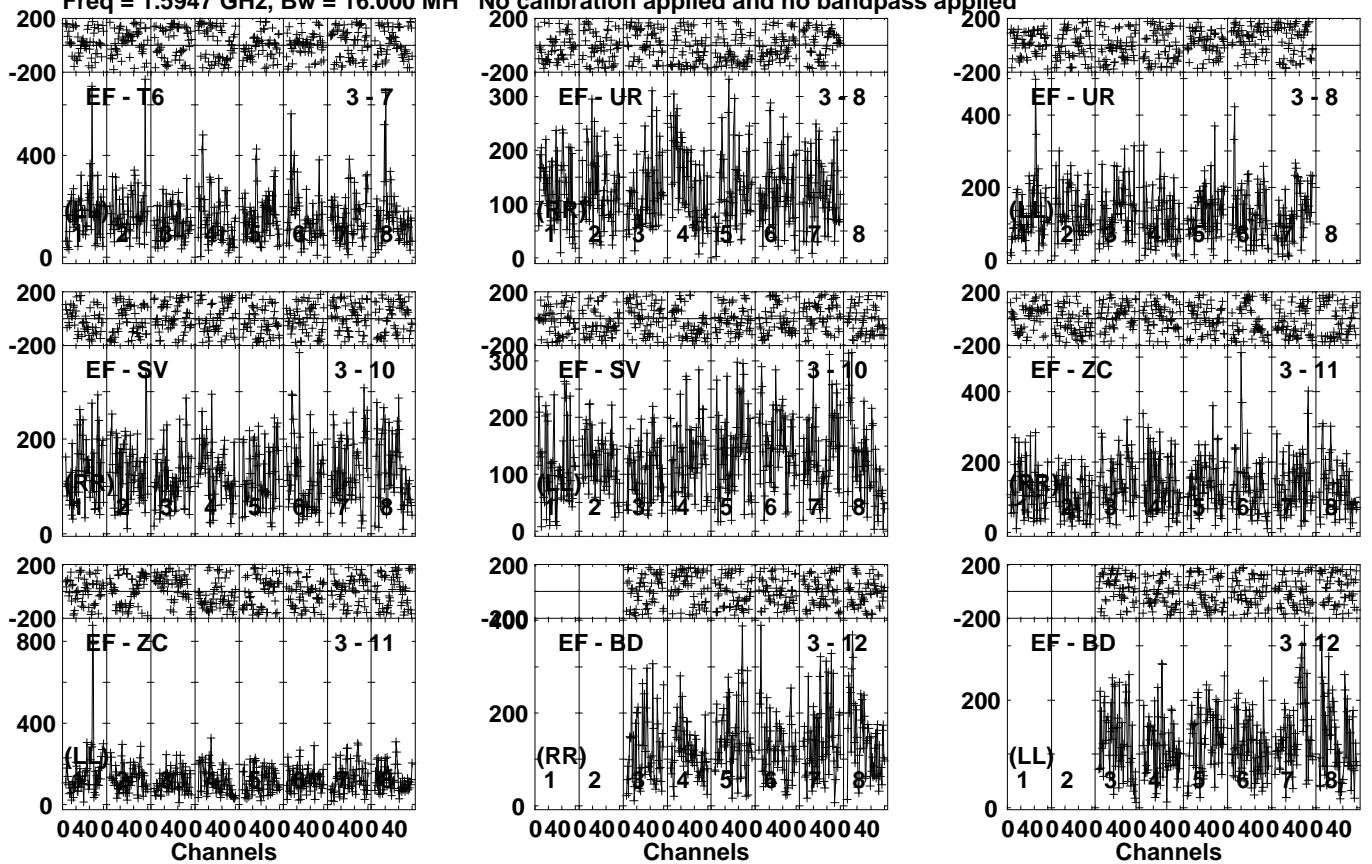
Lower frame: Micro Ampl Jy Top frame: Phas deg Vector averaged cross-power spectrum Several baselines displayed Timerange: 01/02:42:11 to 01/02:45:10
