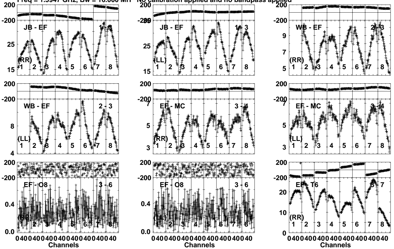
Lower frame: Milli Ampl Jy Top frame: Phas deg Vector averaged cross-power spectrum Several baselines displayed Timerange: 01/05:03:20 to 01/05:04:29
