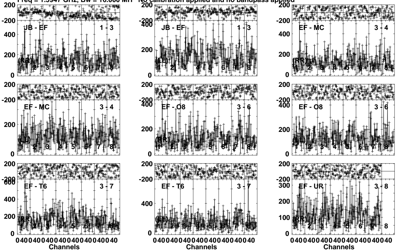
Lower frame: Micro Ampl Jy Top frame: Phas deg Vector averaged cross-power spectrum Several baselines displayed Timerange: 00/23:42:11 to 00/23:45:10
