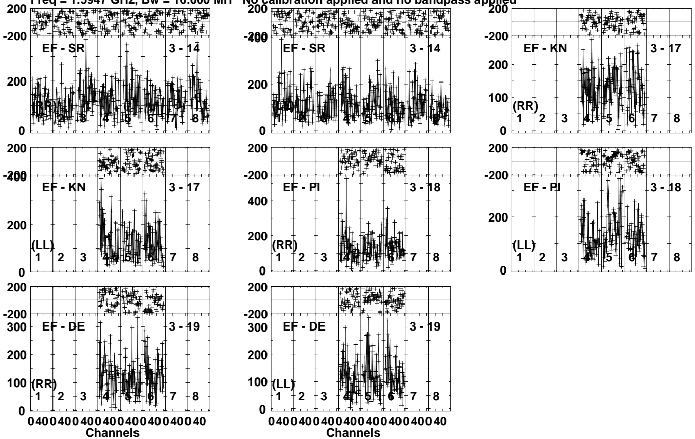
Lower frame: Micro Ampl Jy Top frame: Phas deg Vector averaged cross-power spectrum Several baselines displayed Timerange: 01/00:22:10 to 01/00:25:10
