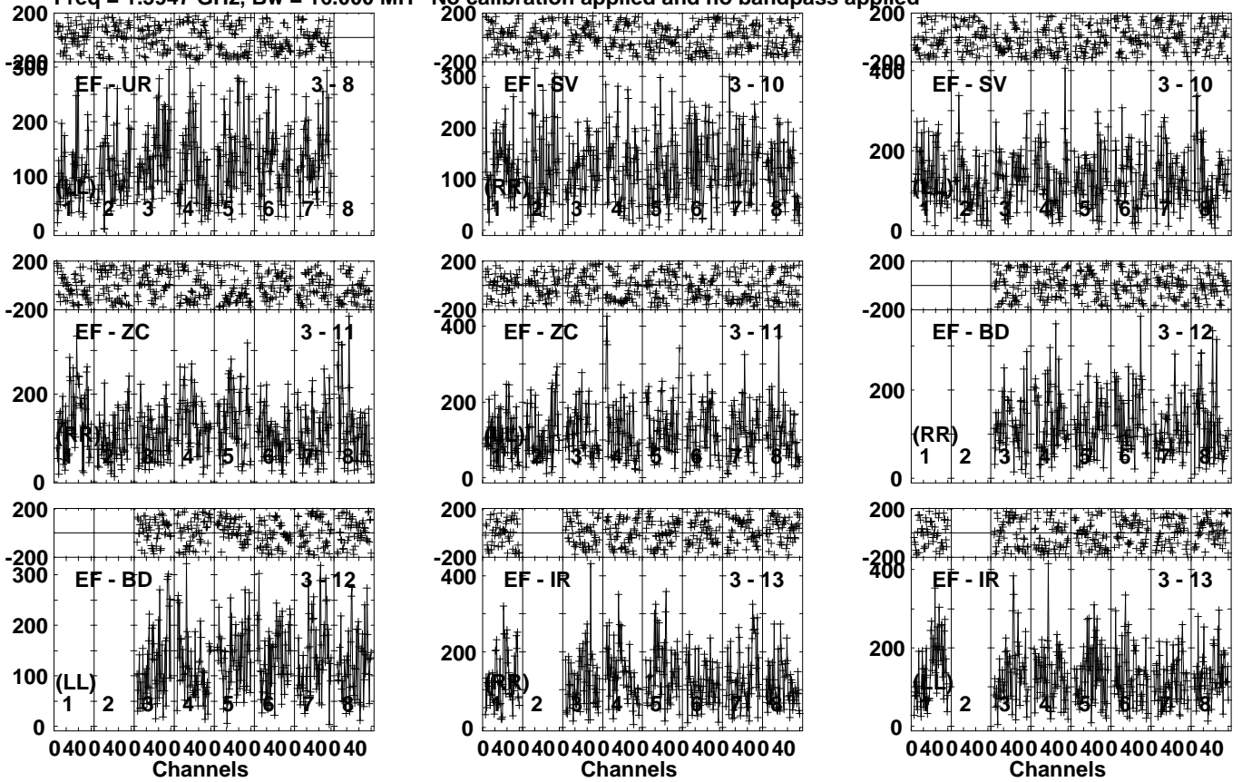
Lower frame: Micro Ampl Jy Top frame: Phas deg Vector averaged cross-power spectrum Several baselines displayed Timerange: 01/10:25:20 to 01/10:28:19
