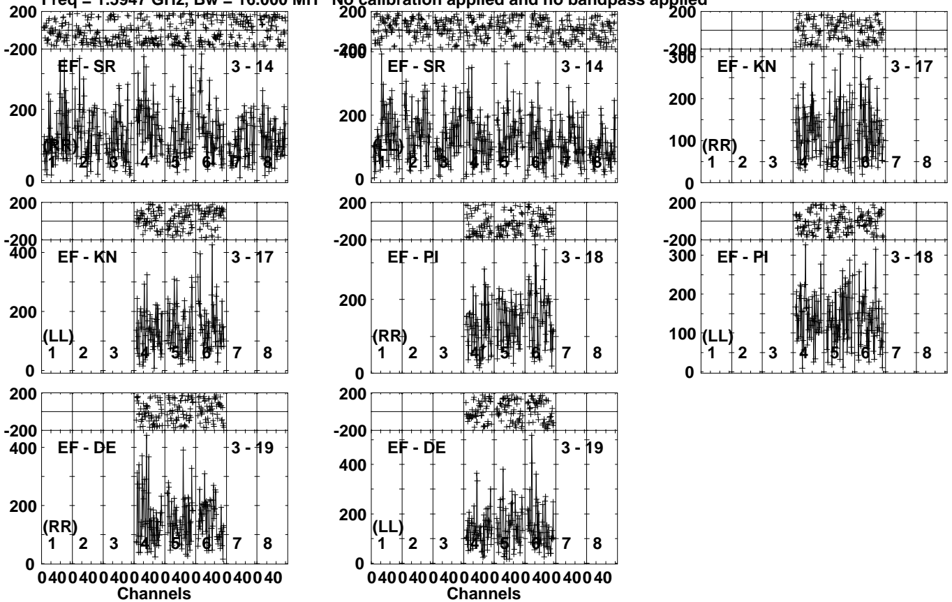
Lower frame: Micro Ampl Jy Top frame: Phas deg Vector averaged cross-power spectrum Several baselines displayed Timerange: 01/06:29:50 to 01/06:32:39
