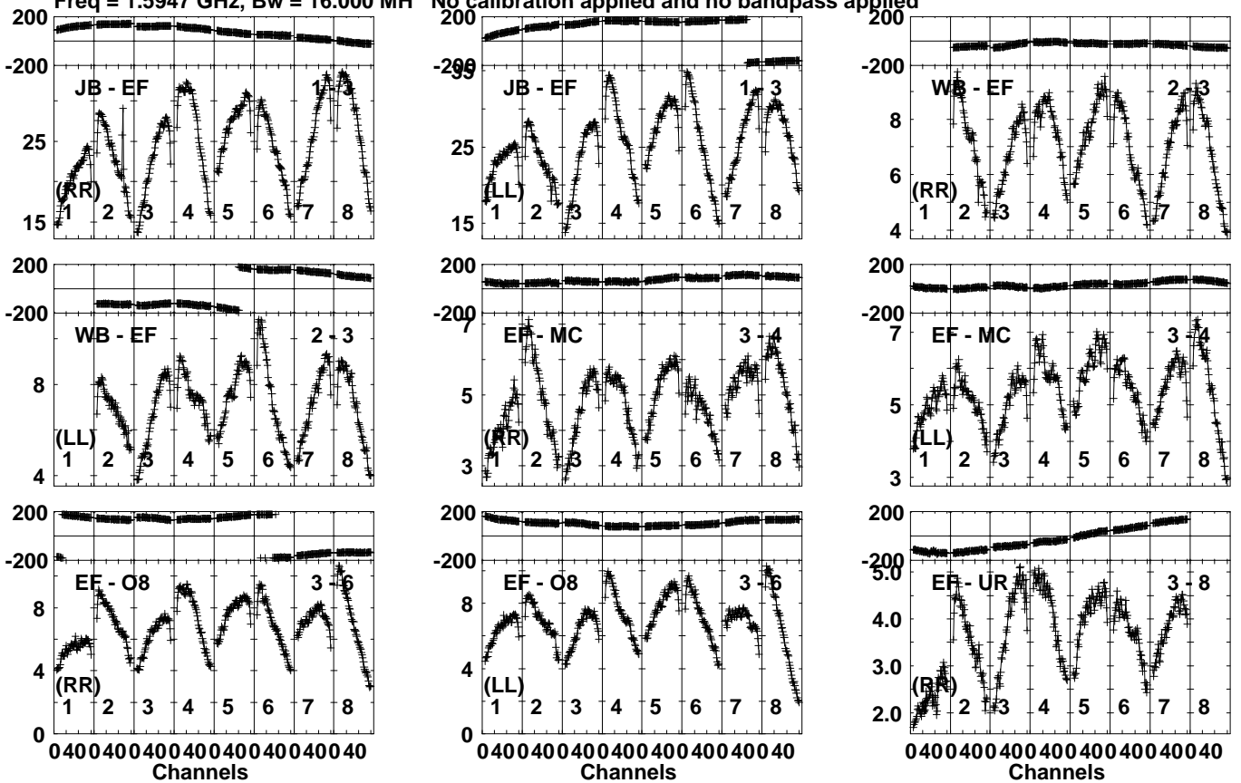
Lower frame: Milli Ampl Jy Top frame: Phas deg Vector averaged cross-power spectrum Several baselines displayed Timerange: 01/09:43:50 to 01/09:45:00
