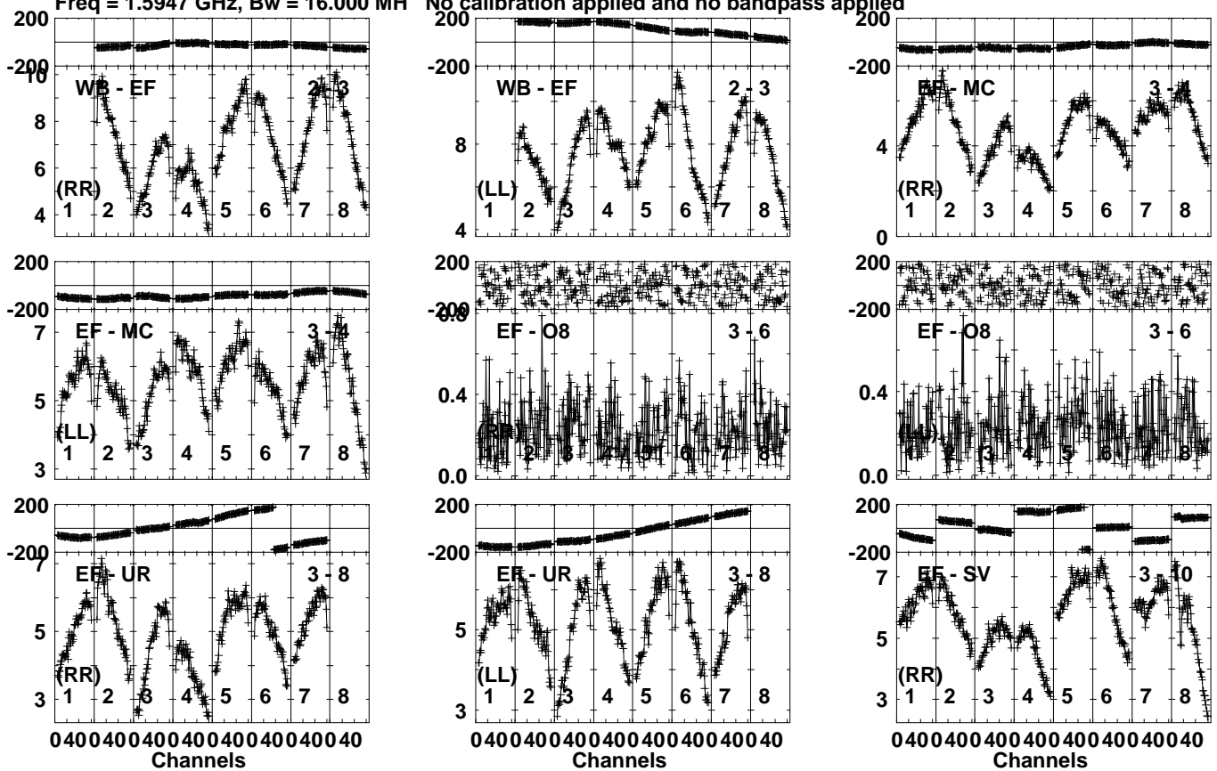
Lower frame: Milli Ampl Jy Top frame: Phas deg Vector averaged cross-power spectrum Several baselines displayed Timerange: 01/07:28:10 to 01/07:29:30
