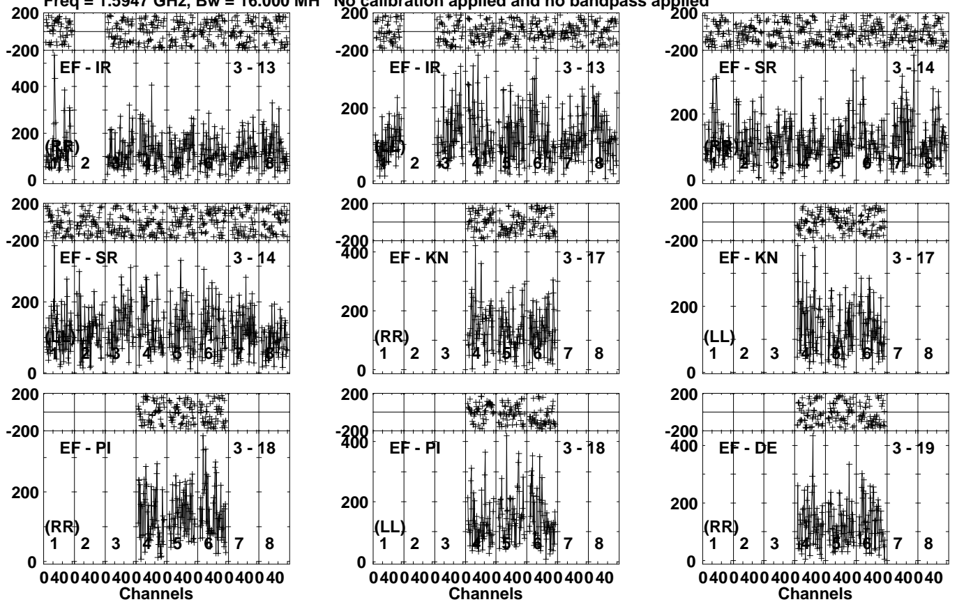
Lower frame: Micro Ampl Jy Top frame: Phas deg Vector averaged cross-power spectrum Several baselines displayed Timerange: 01/00:42:10 to 01/00:45:09
