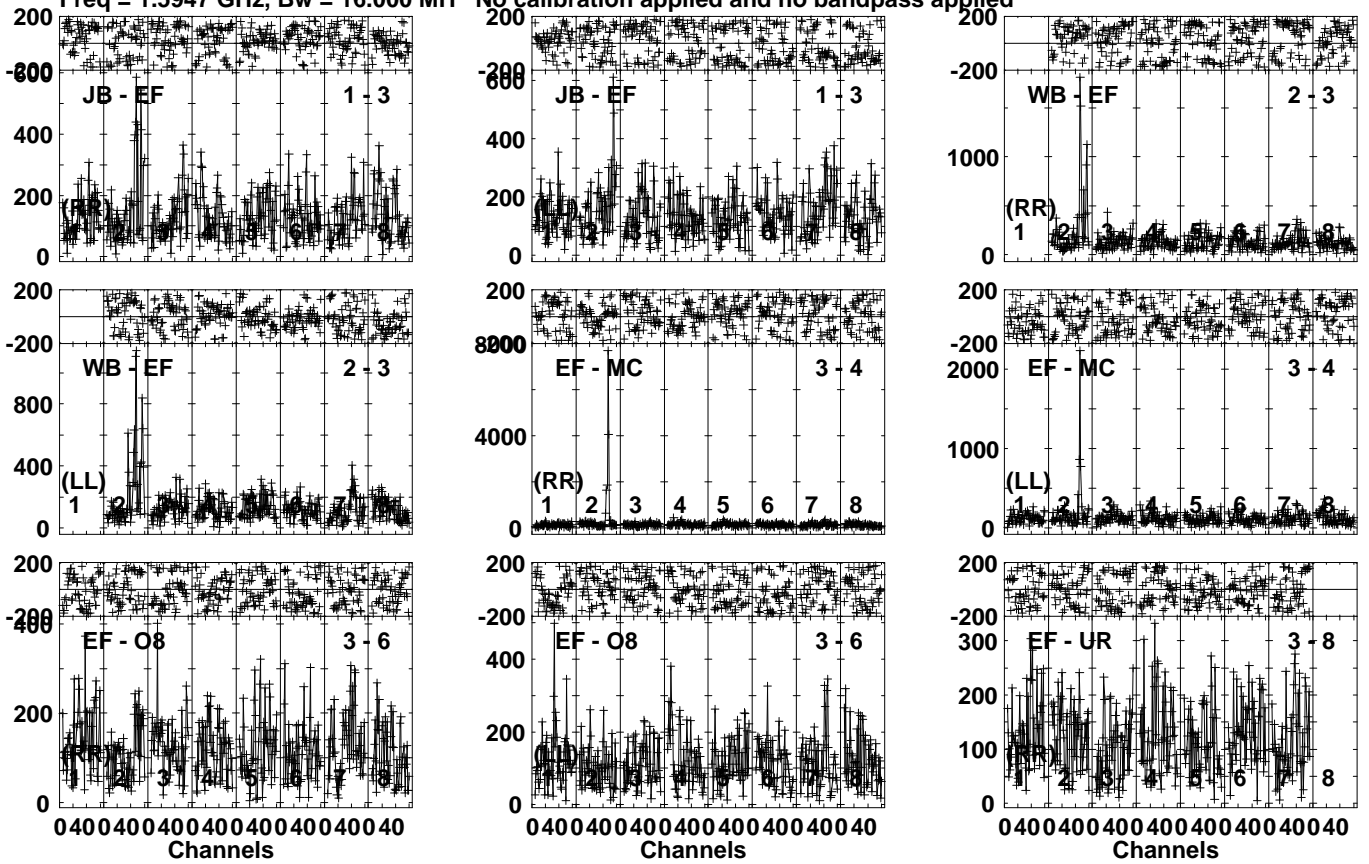
Lower frame: Micro Ampl Jy Top frame: Phas deg Vector averaged cross-power spectrum Several baselines displayed Timerange: 01/10:35:21 to 01/10:38:20
