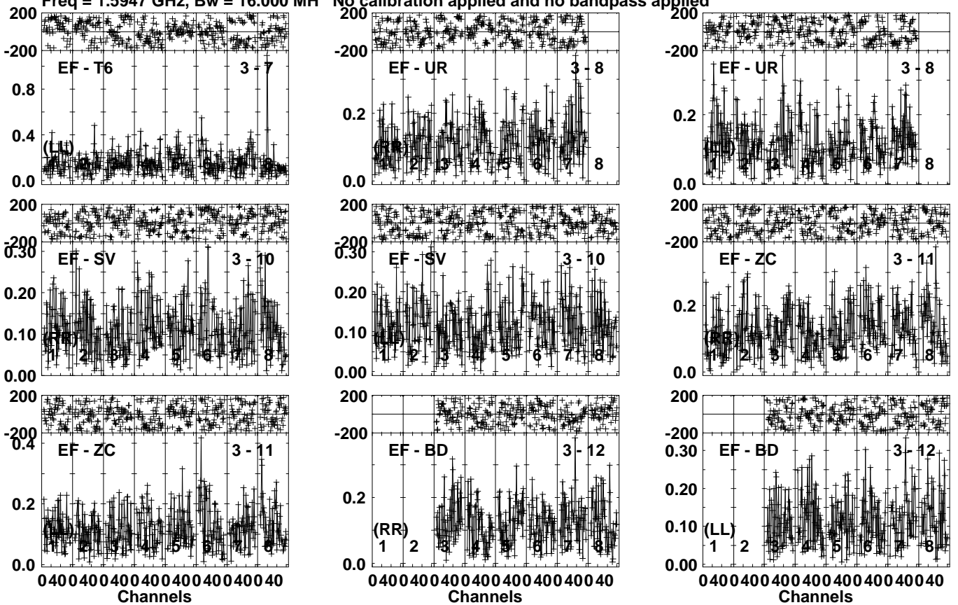
Lower frame: Milli Ampl Jy Top frame: Phas deg Vector averaged cross-power spectrum Several baselines displayed Timerange: 01/01:02:11 to 01/01:05:10
