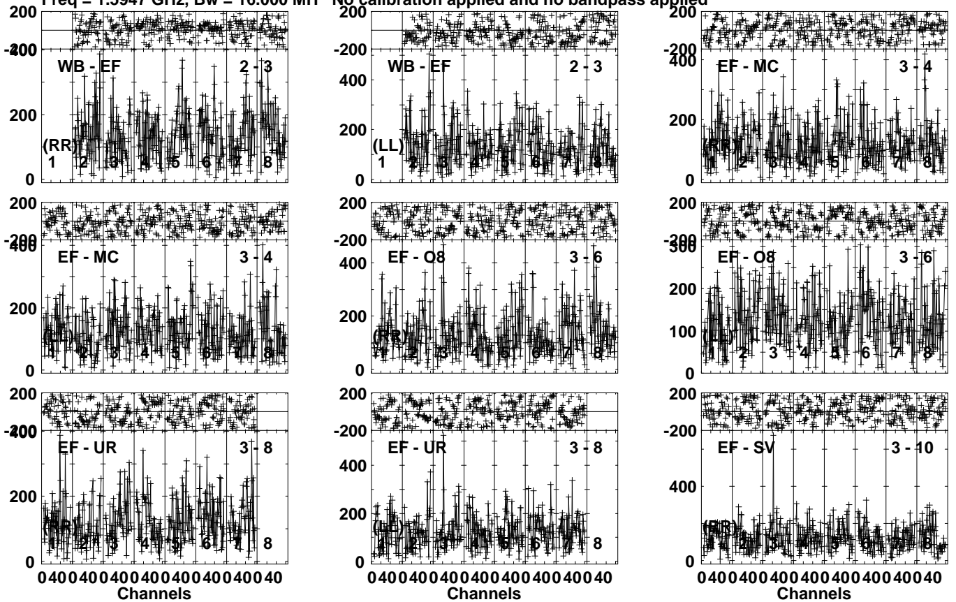
Lower frame: Micro Ampl Jy Top frame: Phas deg Vector averaged cross-power spectrum Several baselines displayed Timerange: 01/10:30:22 to 01/10:33:10
