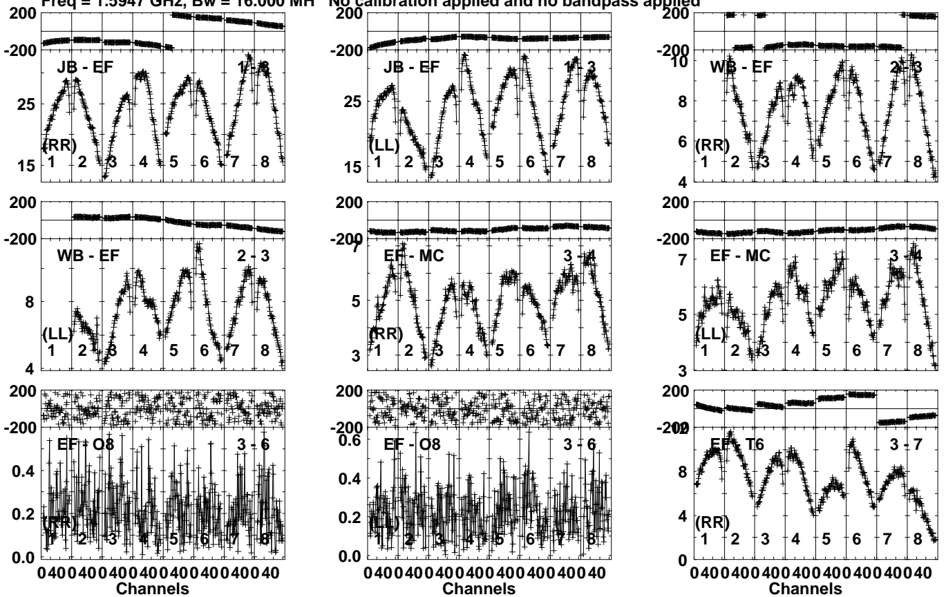
Lower frame: Milli Ampl Jy Top frame: Phas deg Vector averaged cross-power spectrum Several baselines displayed Timerange: 01/01:05:31 to 01/01:06:50
