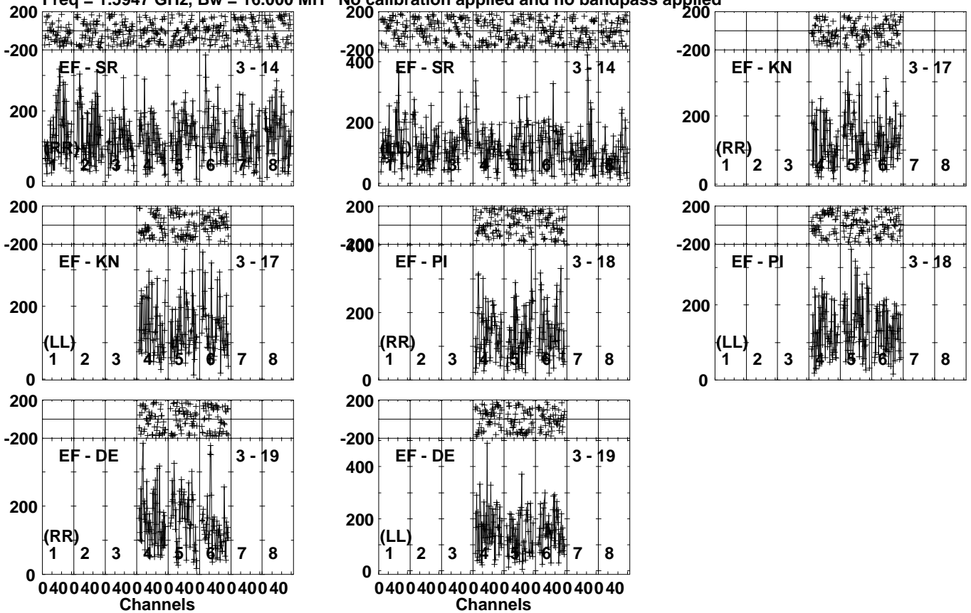
Lower frame: Micro Ampl Jy Top frame: Phas deg Vector averaged cross-power spectrum Several baselines displayed Timerange: 01/09:35:21 to 01/09:38:19
