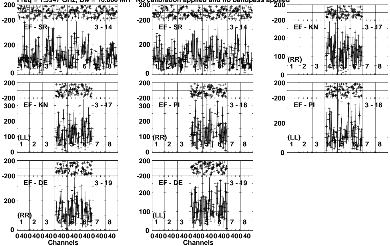
Lower frame: Micro Ampl Jy Top frame: Phas deg Vector averaged cross-power spectrum Several baselines displayed Timerange: 01/10:05:20 to 01/10:08:20
