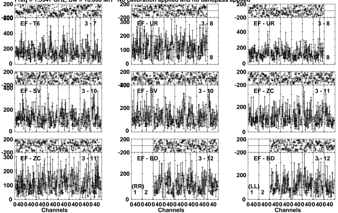
Lower frame: Micro Ampl Jy Top frame: Phas deg Vector averaged cross-power spectrum Several baselines displayed Timerange: 01/02:54:50 to 01/02:57:50
