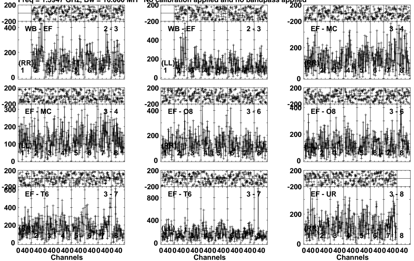
Lower frame: Micro Ampl Jy Top frame: Phas deg Vector averaged cross-power spectrum Several baselines displayed Timerange: 01/01:57:11 to 01/01:59:59
