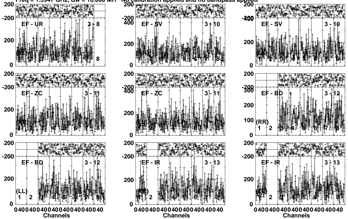
Lower frame: Micro Ampl Jy Top frame: Phas deg Vector averaged cross-power spectrum Several baselines displayed Timerange: 01/02:07:10 to 01/02:09:59
