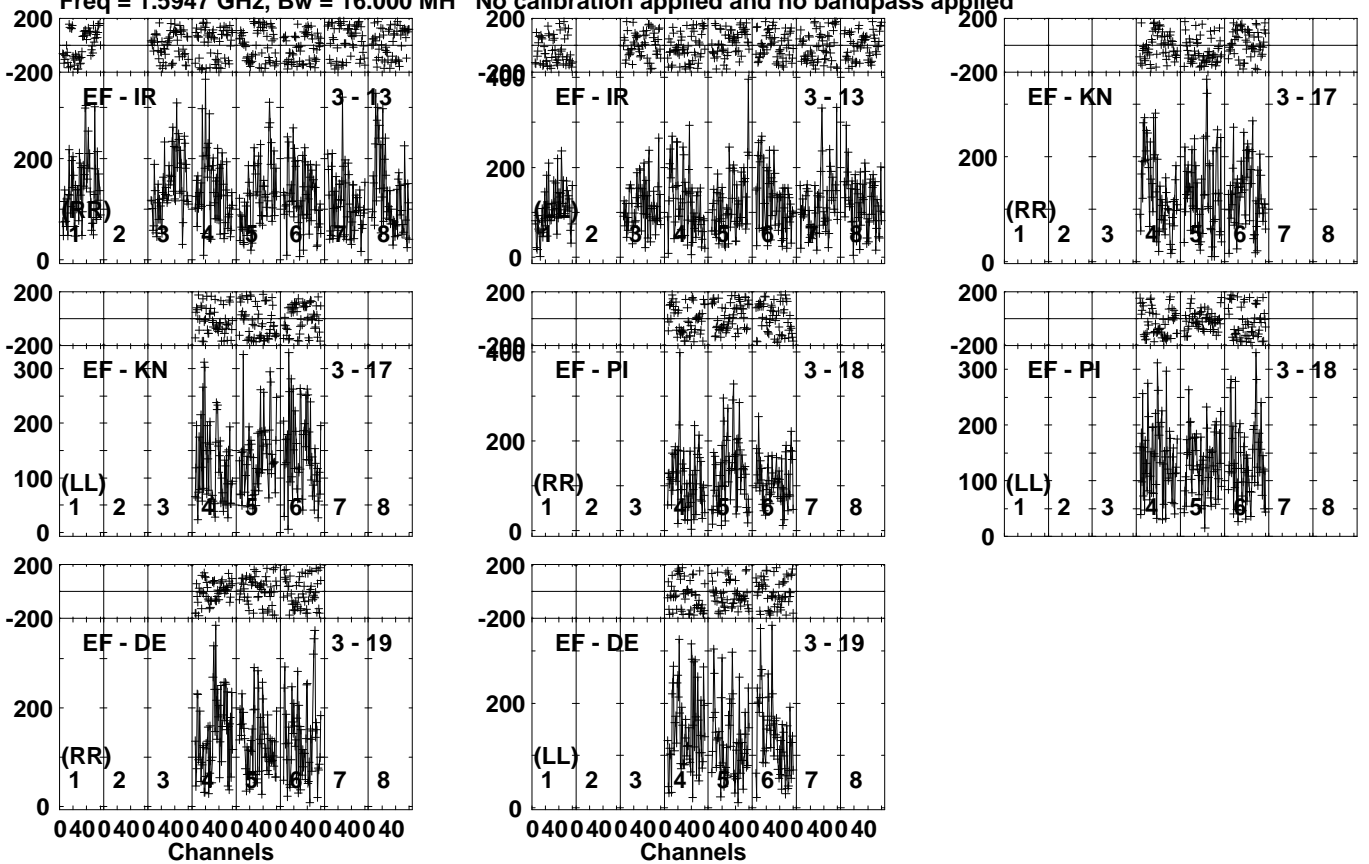
Lower frame: Micro Ampl Jy Top frame: Phas deg Vector averaged cross-power spectrum Several baselines displayed Timerange: 01/02:02:10 to 01/02:05:09
