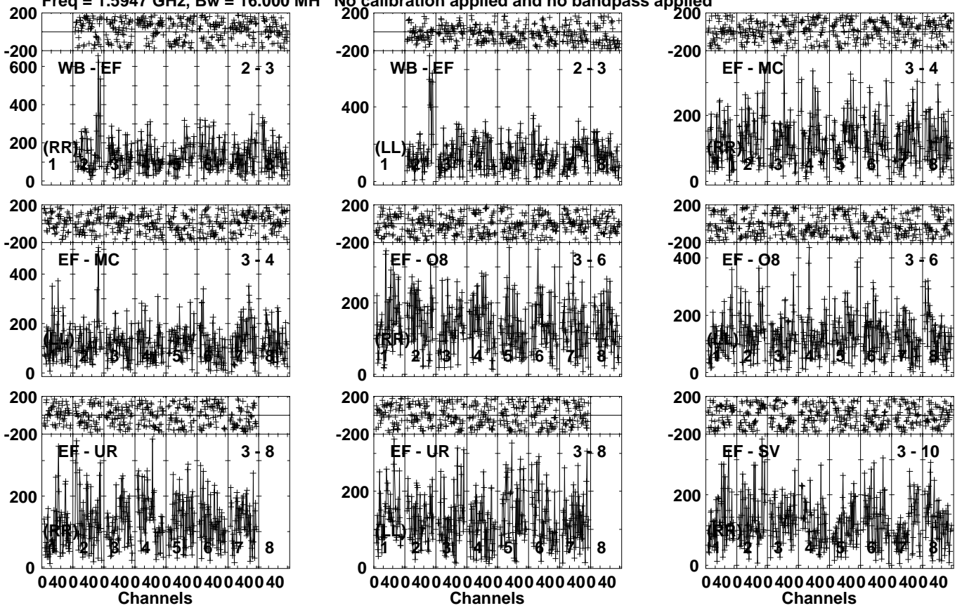
Lower frame: Micro Ampl Jy Top frame: Phas deg Vector averaged cross-power spectrum Several baselines displayed Timerange: 01/09:40:21 to 01/09:43:10
