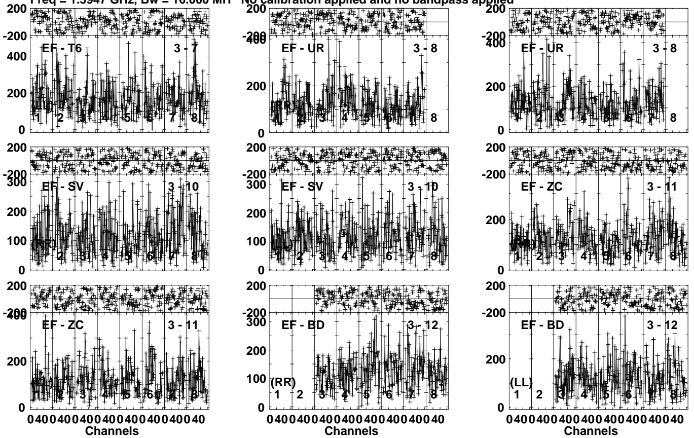
Lower frame: Micro Ampl Jy Top frame: Phas deg Vector averaged cross-power spectrum Several baselines displayed Timerange: 01/03:14:50 to 01/03:17:49
