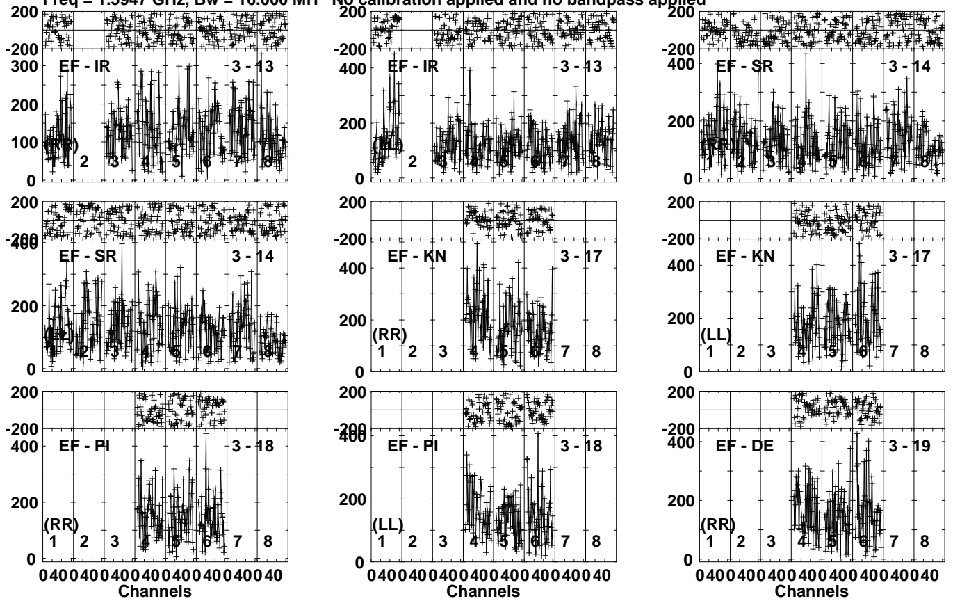
Lower frame: Micro Ampl Jy Top frame: Phas deg Vector averaged cross-power spectrum Several baselines displayed Timerange: 01/06:14:50 to 01/06:17:49
