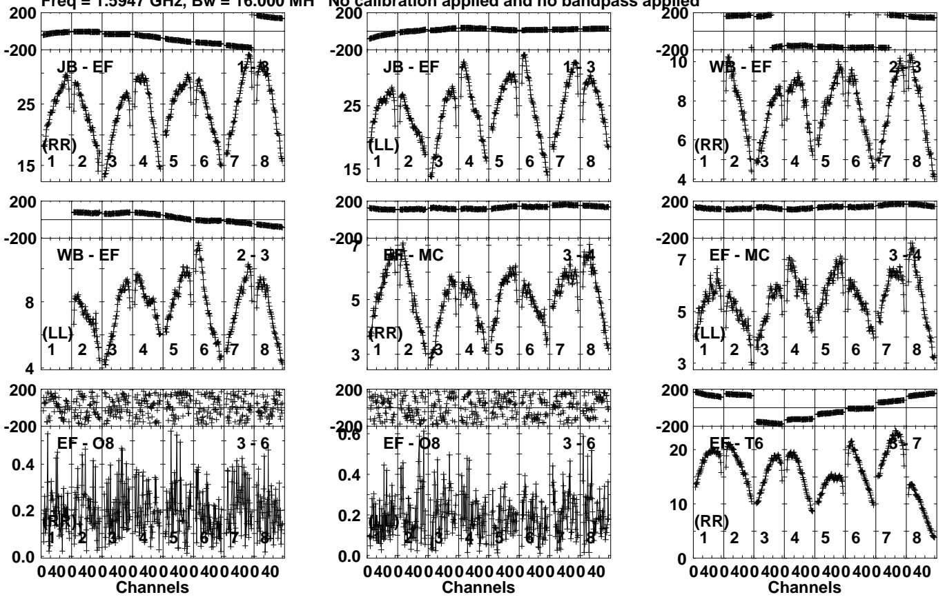
Lower frame: Milli Ampl Jy Top frame: Phas deg Vector averaged cross-power spectrum Several baselines displayed Timerange: 01/03:33:20 to 01/03:34:29
