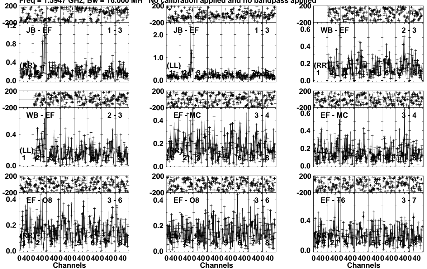
Lower frame: Milli Ampl Jy Top frame: Phas deg Vector averaged cross-power spectrum Several baselines displayed Timerange: 01/05:34:50 to 01/05:37:50
