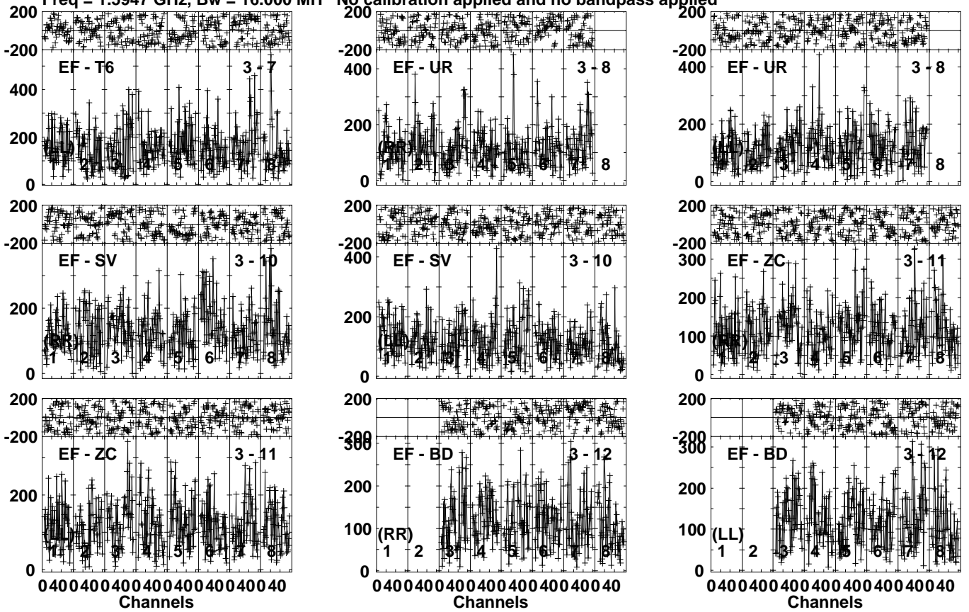
Lower frame: Micro Ampl Jy Top frame: Phas deg Vector averaged cross-power spectrum Several baselines displayed Timerange: 01/01:22:10 to 01/01:25:10
