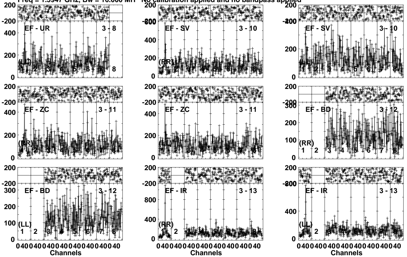
Lower frame: Micro Ampl Jy Top frame: Phas deg Vector averaged cross-power spectrum Several baselines displayed Timerange: 01/09:55:20 to 01/09:58:20
