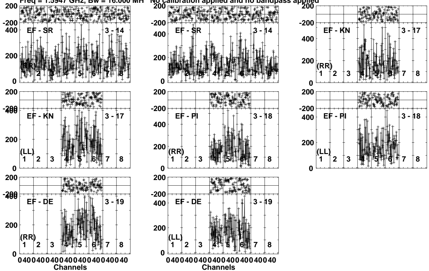
Lower frame: Micro Ampl Jy Top frame: Phas deg Vector averaged cross-power spectrum Several baselines displayed Timerange: 01/05:49:51 to 01/05:52:40
