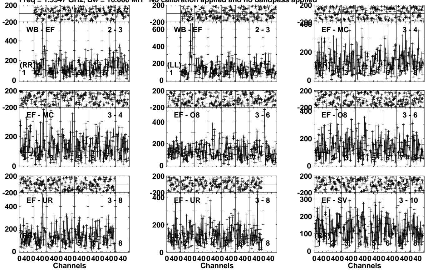
Lower frame: Micro Ampl Jy Top frame: Phas deg Vector averaged cross-power spectrum Several baselines displayed Timerange: 01/08:09:50 to 01/08:12:39
