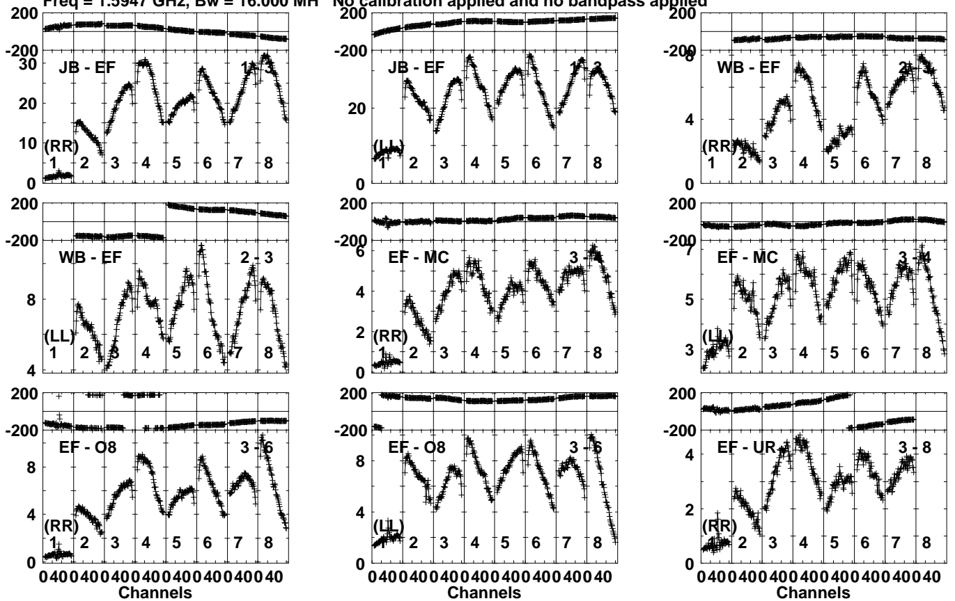
Lower frame: Milli Ampl Jy Top frame: Phas deg Vector averaged cross-power spectrum Several baselines displayed Timerange: 01/09:53:50 to 01/09:55:00
