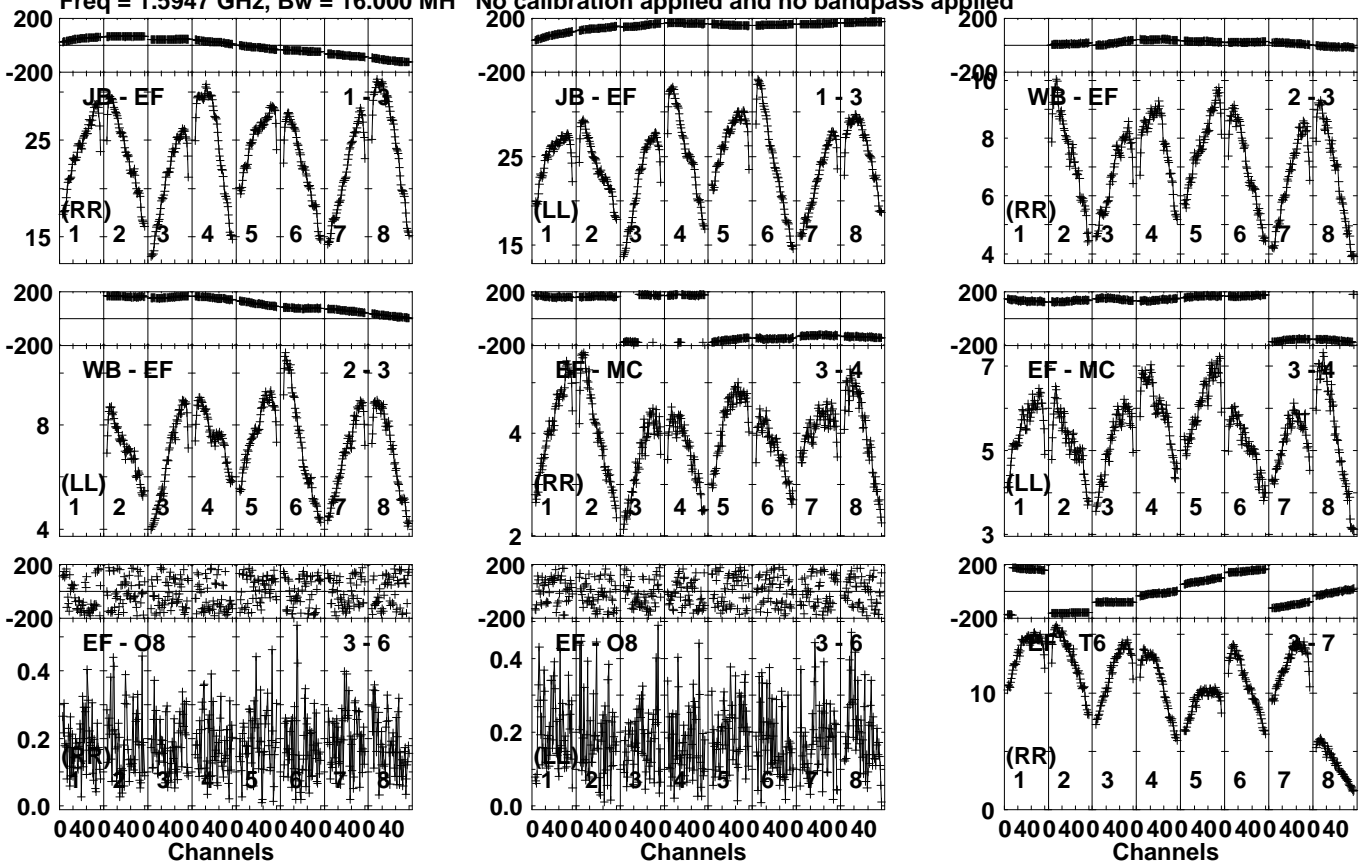
Lower frame: Milli Ampl Jy Top frame: Phas deg Vector averaged cross-power spectrum Several baselines displayed Timerange: 01/06:23:20 to 01/06:24:29
