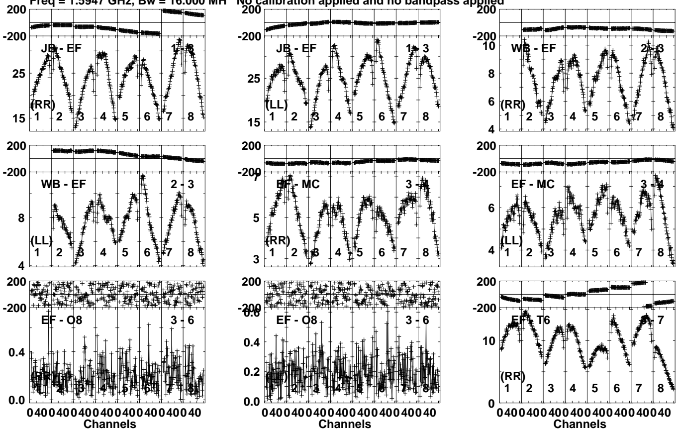
Lower frame: Milli Ampl Jy Top frame: Phas deg Vector averaged cross-power spectrum Several baselines displayed Timerange: 01/01:35:30 to 01/01:36:49
