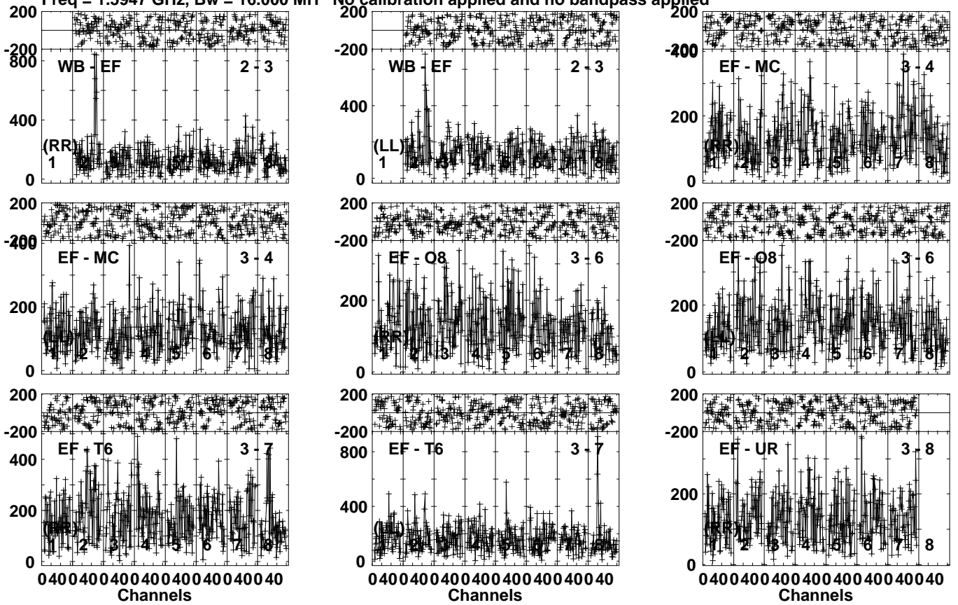
Lower frame: Micro Ampl Jy Top frame: Phas deg Vector averaged cross-power spectrum Several baselines displayed Timerange: 01/04:09:51 to 01/04:12:40
