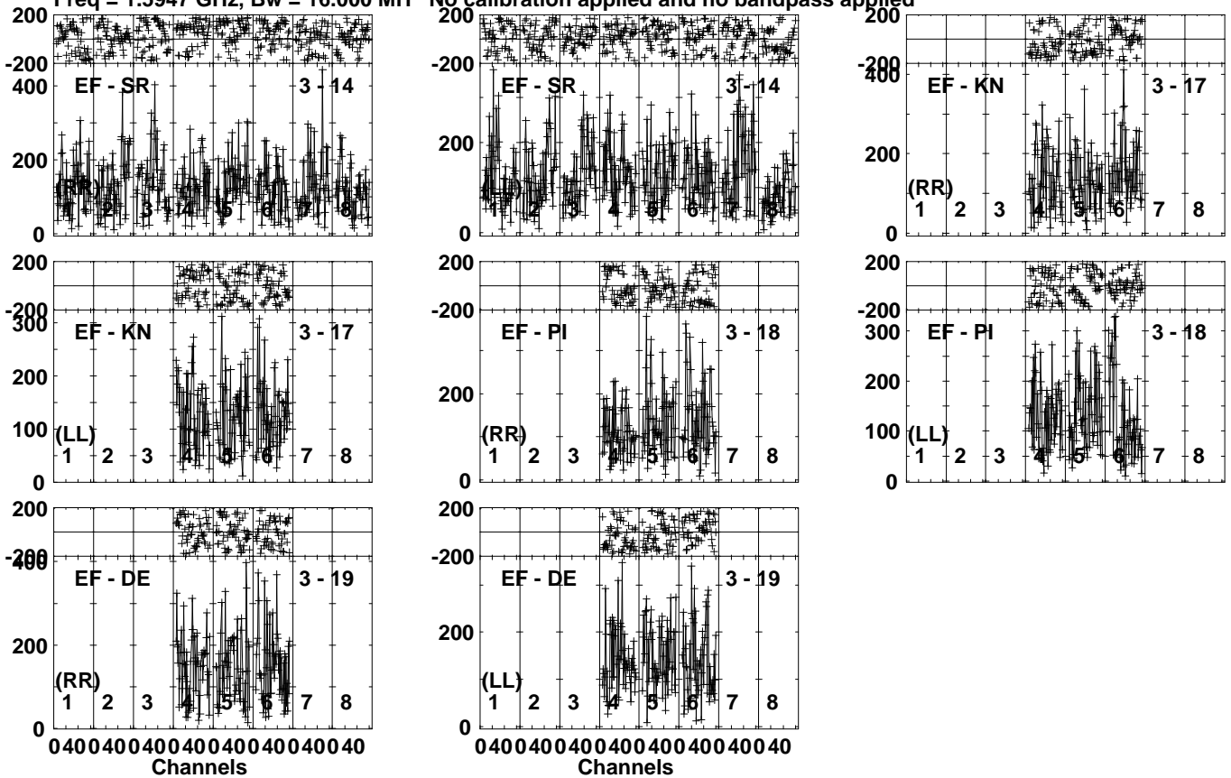
Lower frame: Micro Ampl Jy Top frame: Phas deg Vector averaged cross-power spectrum Several baselines displayed Timerange: 01/03:24:50 to 01/03:27:49
