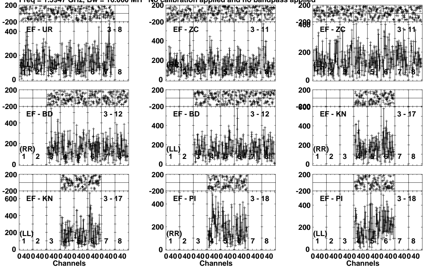
Lower frame: Micro Ampl Jy Top frame: Phas deg Vector averaged cross-power spectrum Several baselines displayed Timerange: 01/05:09:50 to 01/05:12:39
