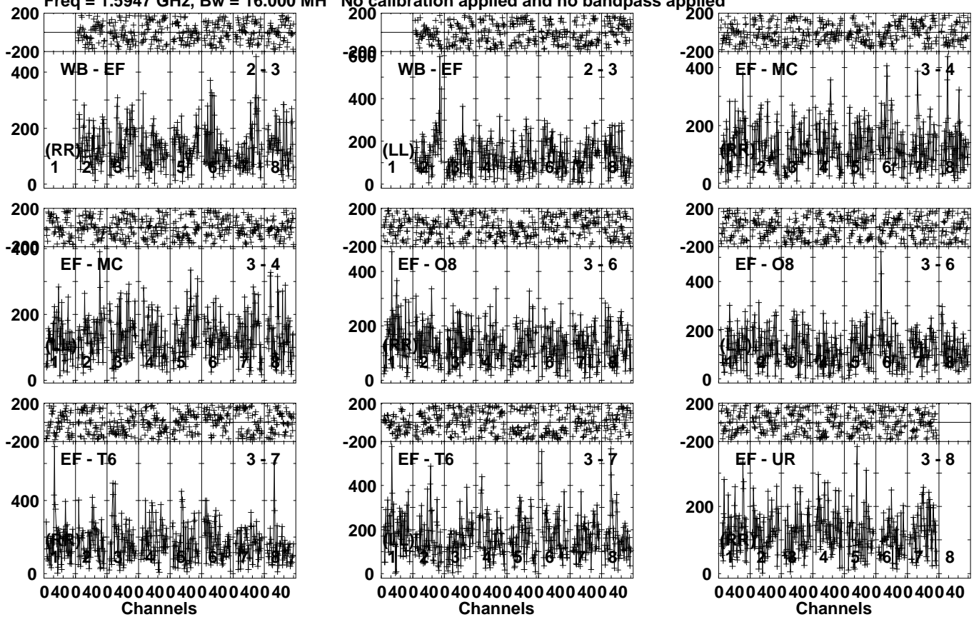
Lower frame: Micro Ampl Jy Top frame: Phas deg Vector averaged cross-power spectrum Several baselines displayed Timerange: 01/00:47:10 to 01/00:49:59
