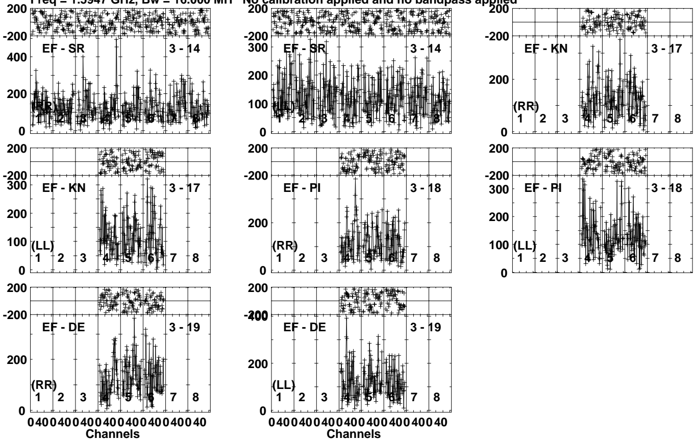
Lower frame: Micro Ampl Jy Top frame: Phas deg Vector averaged cross-power spectrum Several baselines displayed Timerange: 01/01:27:10 to 01/01:29:59
