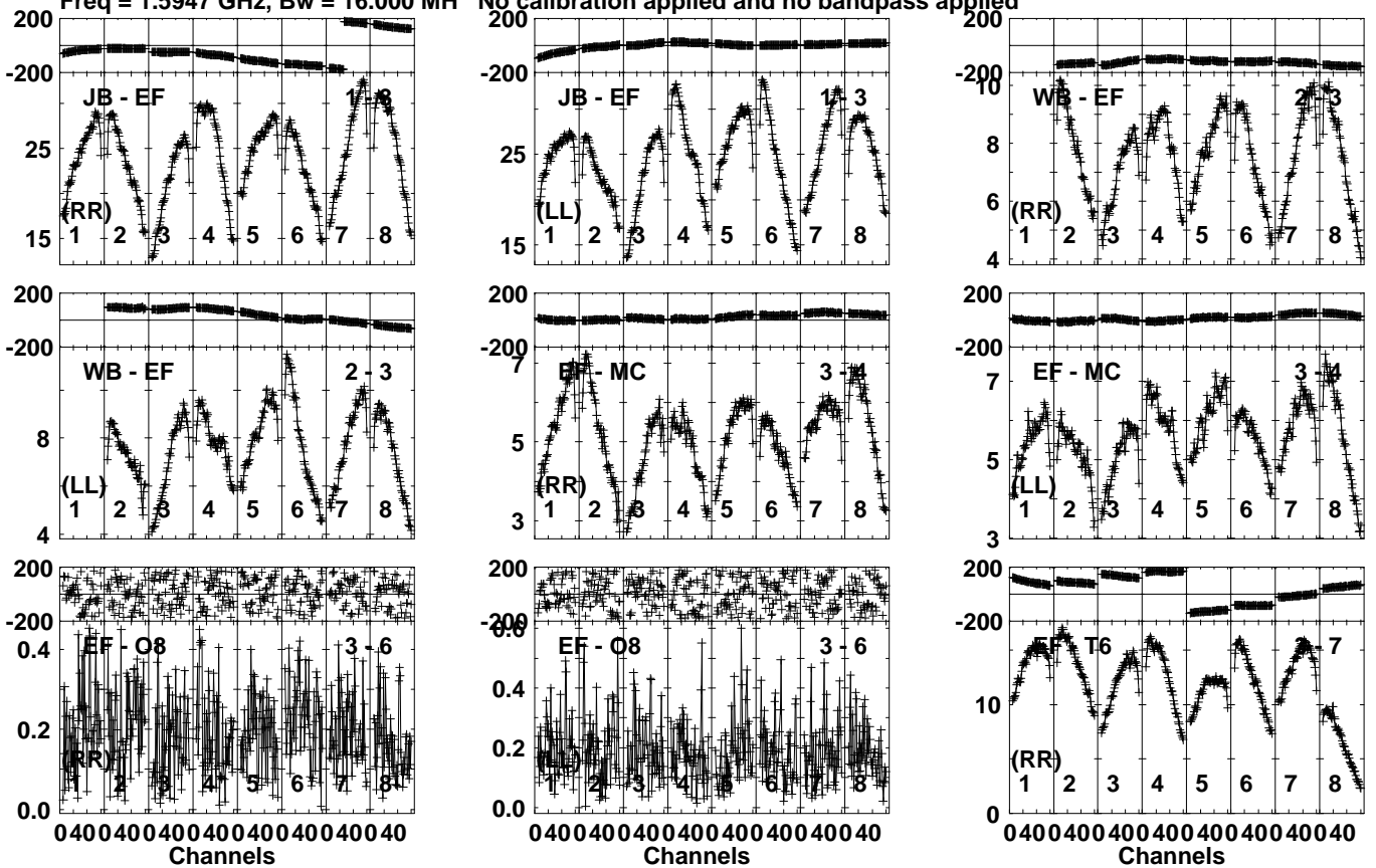
Lower frame: Milli Ampl Jy Top frame: Phas deg Vector averaged cross-power spectrum Several baselines displayed Timerange: 01/01:55:31 to 01/01:56:50
