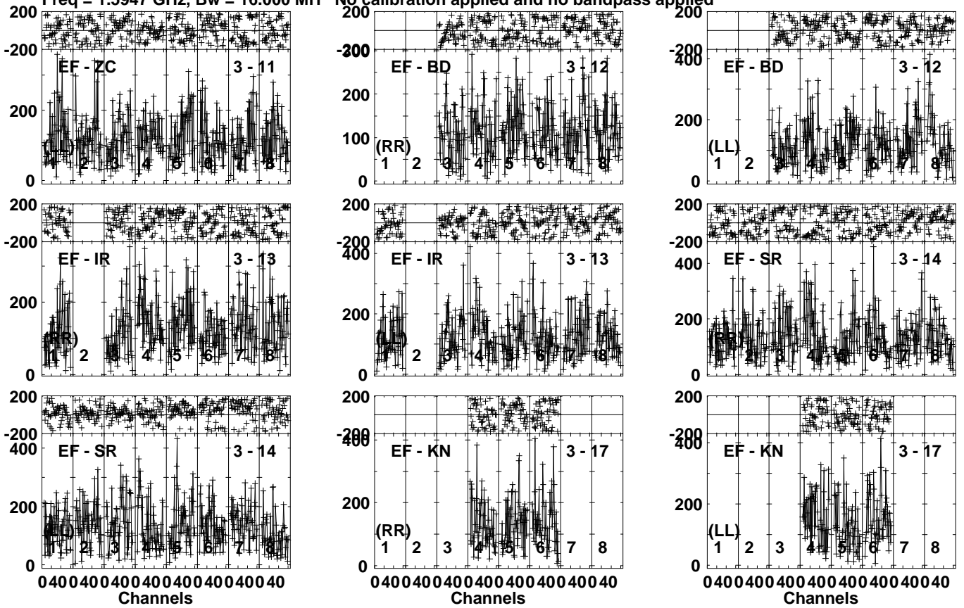
Lower frame: Micro Ampl Jy Top frame: Phas deg Vector averaged cross-power spectrum Several baselines displayed Timerange: 01/07:54:51 to 01/07:57:49
