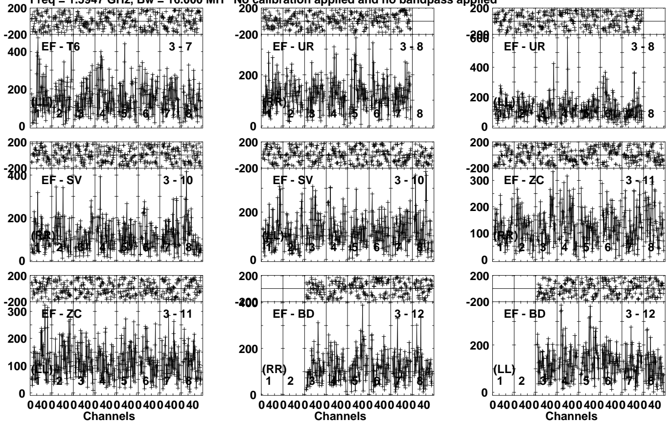
Lower frame: Micro Ampl Jy Top frame: Phas deg Vector averaged cross-power spectrum Several baselines displayed Timerange: 01/01:12:11 to 01/01:15:10
