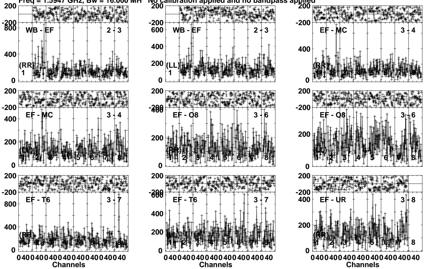
Lower frame: Micro Ampl Jy Top frame: Phas deg Vector averaged cross-power spectrum Several baselines displayed Timerange: 01/06:19:50 to 01/06:22:39
