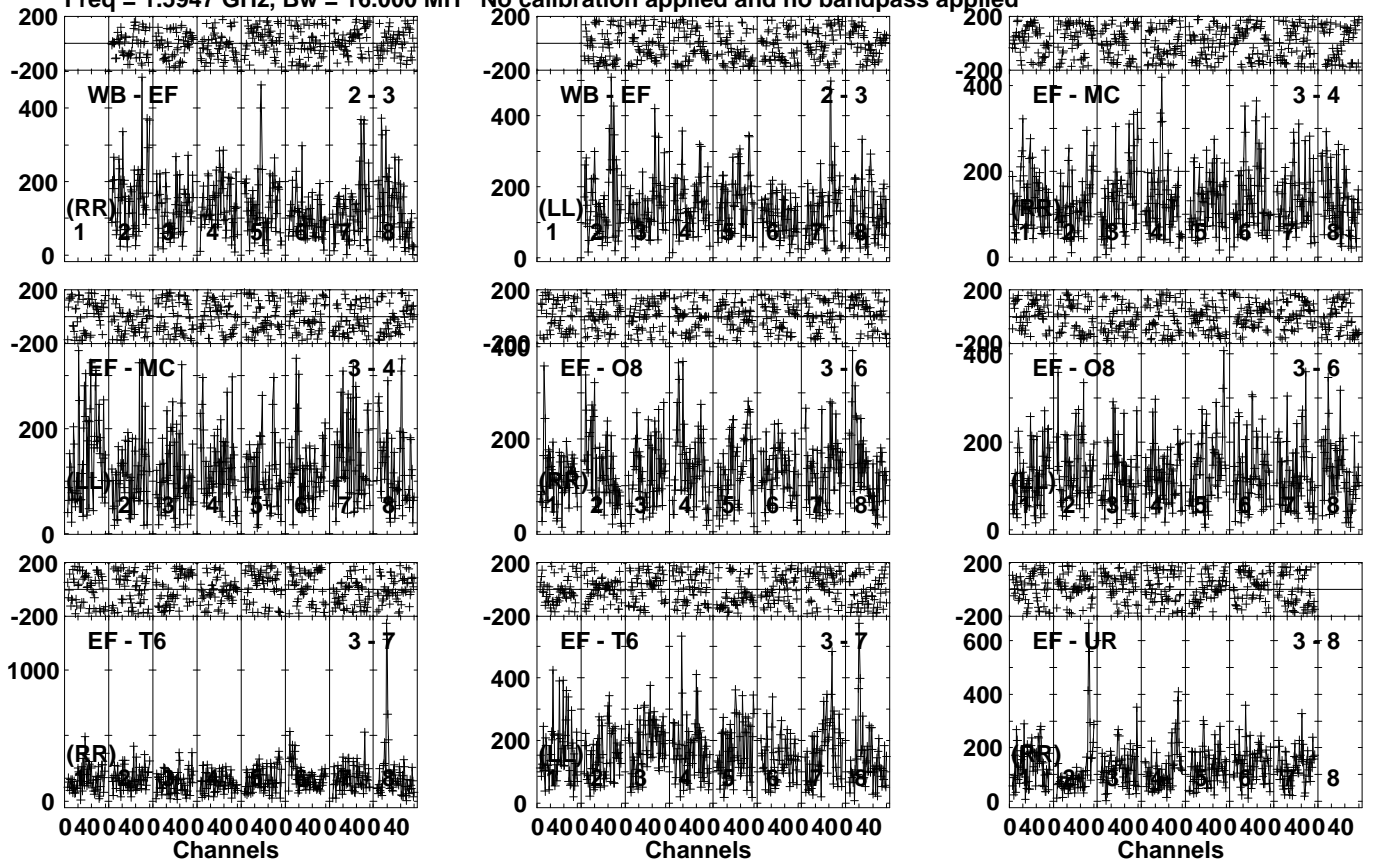
Lower frame: Micro Ampl Jy Top frame: Phas deg Vector averaged cross-power spectrum Several baselines displayed Timerange: 01/03:49:51 to 01/03:52:39
