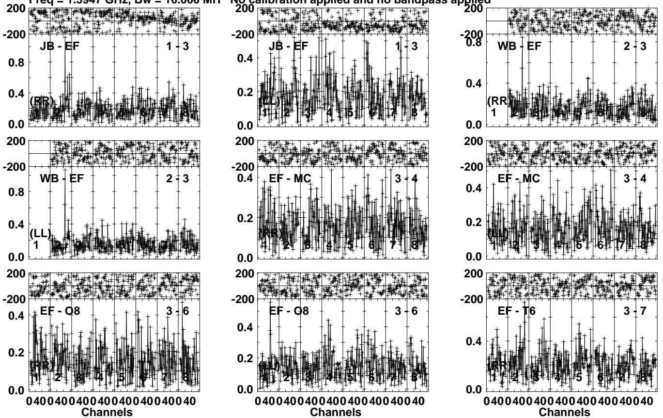
Lower frame: Milli Ampl Jy Top frame: Phas deg Vector averaged cross-power spectrum Several baselines displayed Timerange: 01/05:24:51 to 01/05:27:50
