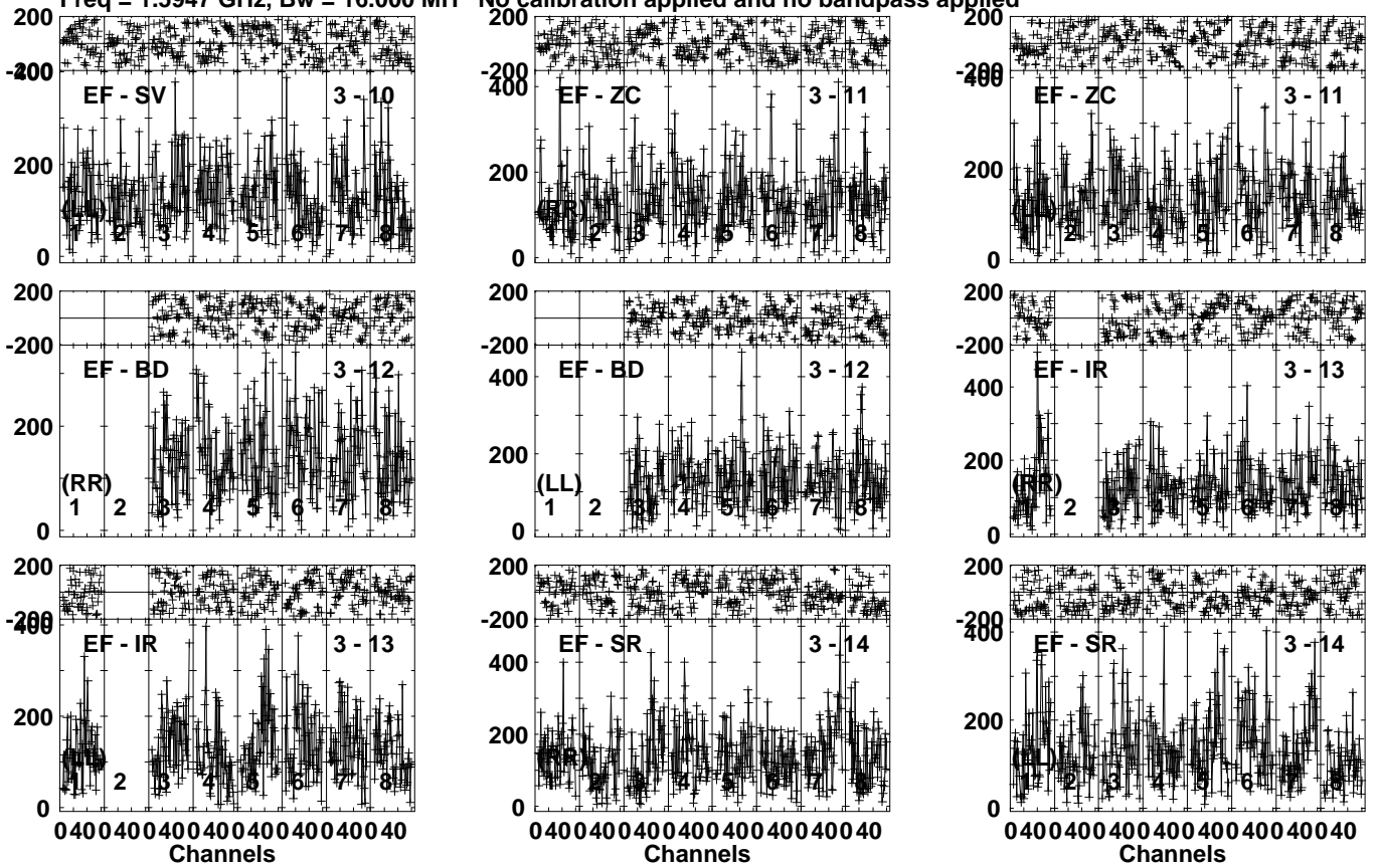
Lower frame: Micro Ampl Jy Top frame: Phas deg Vector averaged cross-power spectrum Several baselines displayed Timerange: 01/08:19:51 to 01/08:22:39
