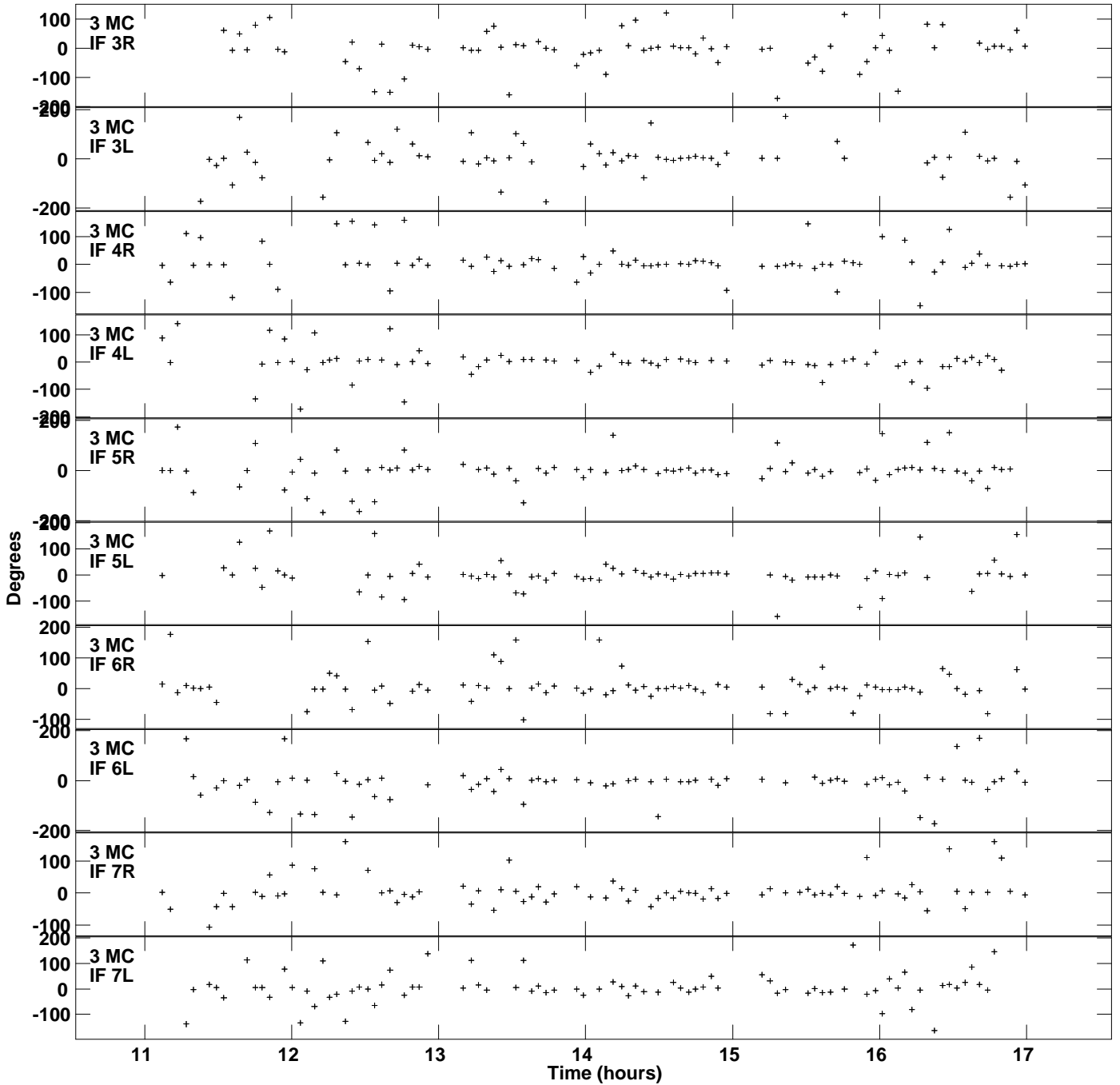
Plot file version 3 created 18-MAY-2021 13:58:37 Gain phs vs UTC time for J0243+0121.MULTI.1 SN 1 Rpol & Lpol IF 1 - 8
