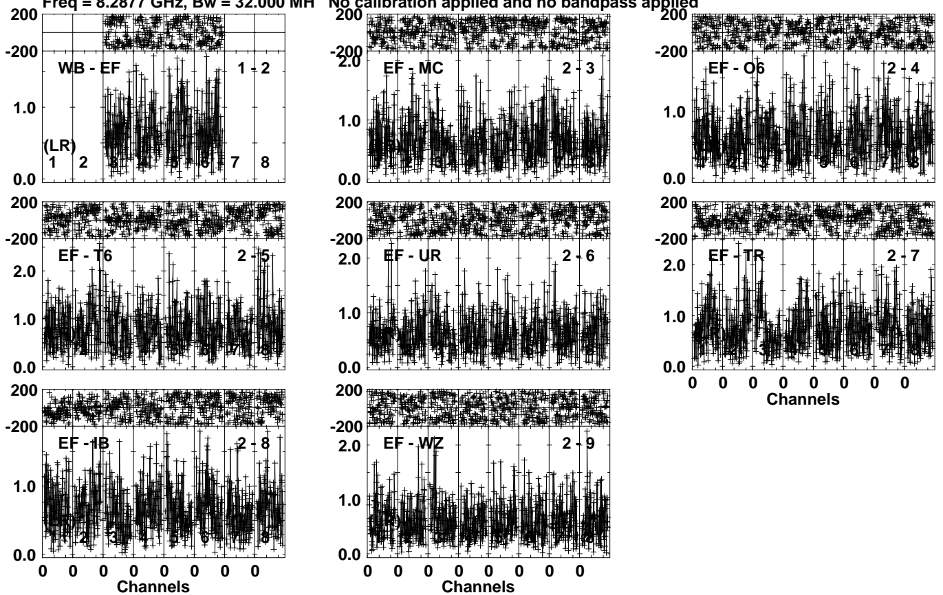
Lower frame: Milli Ampl Jy Top frame: Phas deg Vector averaged cross-power spectrum Several baselines displayed Timerange: 00/17:34:03 to 00/17:34:59
