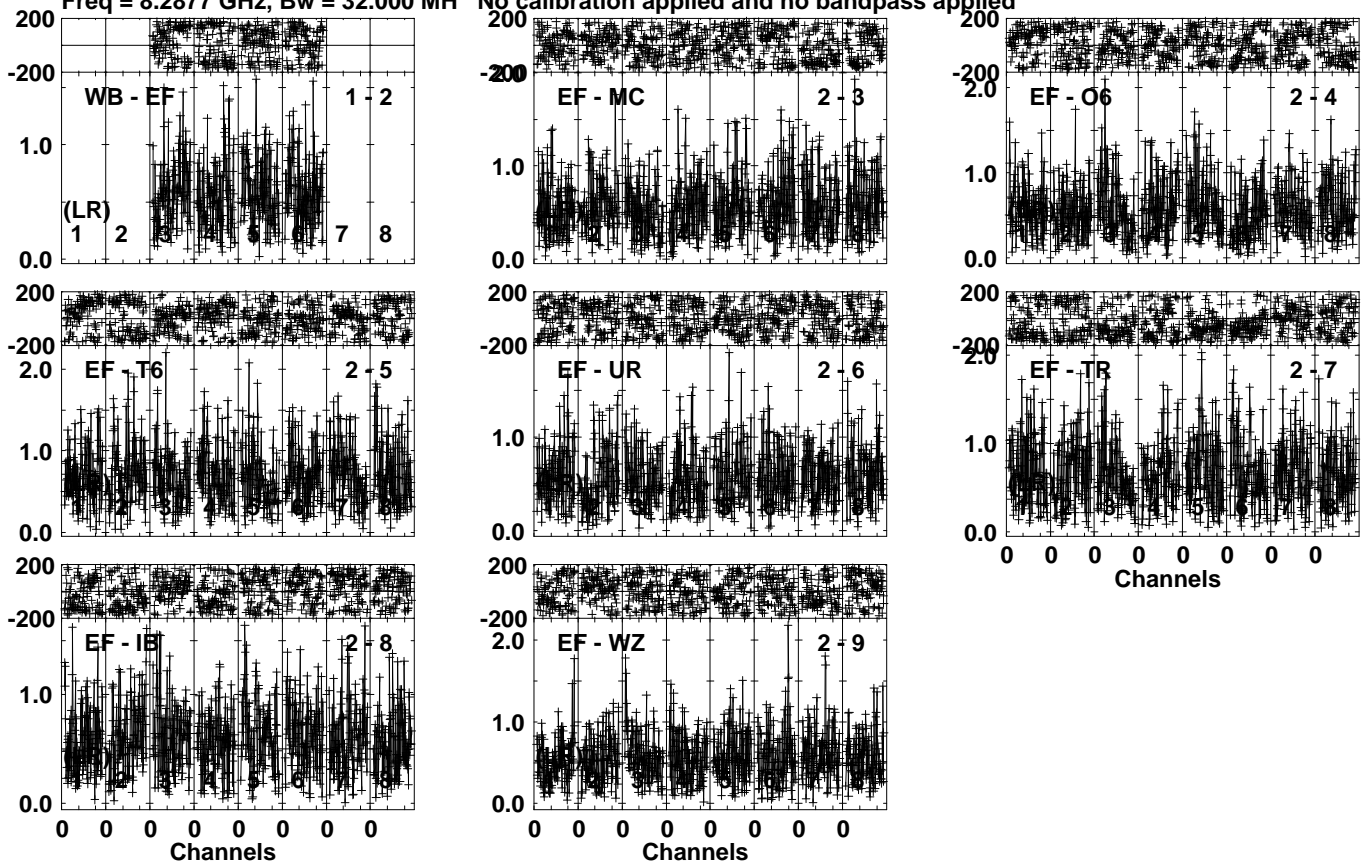
Lower frame: Milli Ampl Jy Top frame: Phas deg Vector averaged cross-power spectrum Several baselines displayed Timerange: 00/16:23:03 to 00/16:23:59
