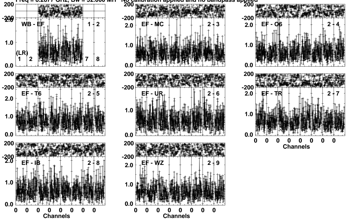
Lower frame: Milli Ampl Jy Top frame: Phas deg Vector averaged cross-power spectrum Several baselines displayed Timerange: 00/16:46:43 to 00/16:47:39
