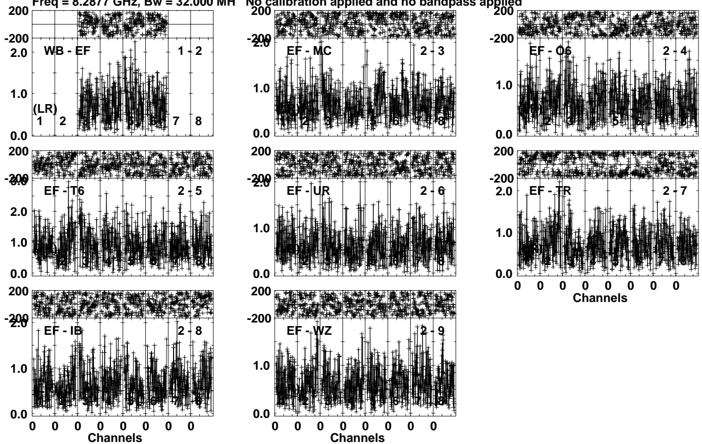
Lower frame: Milli Ampl Jy Top frame: Phas deg Vector averaged cross-power spectrum Several baselines displayed Timerange: 00/15:31:43 to 00/15:32:39
