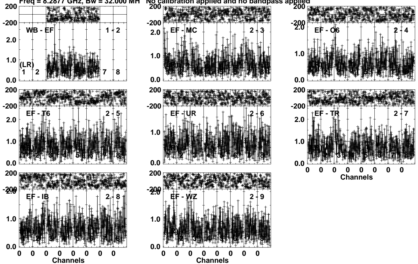
Lower frame: Milli Ampl Jy Top frame: Phas deg Vector averaged cross-power spectrum Several baselines displayed Timerange: 00/17:37:51 to 00/17:38:49
