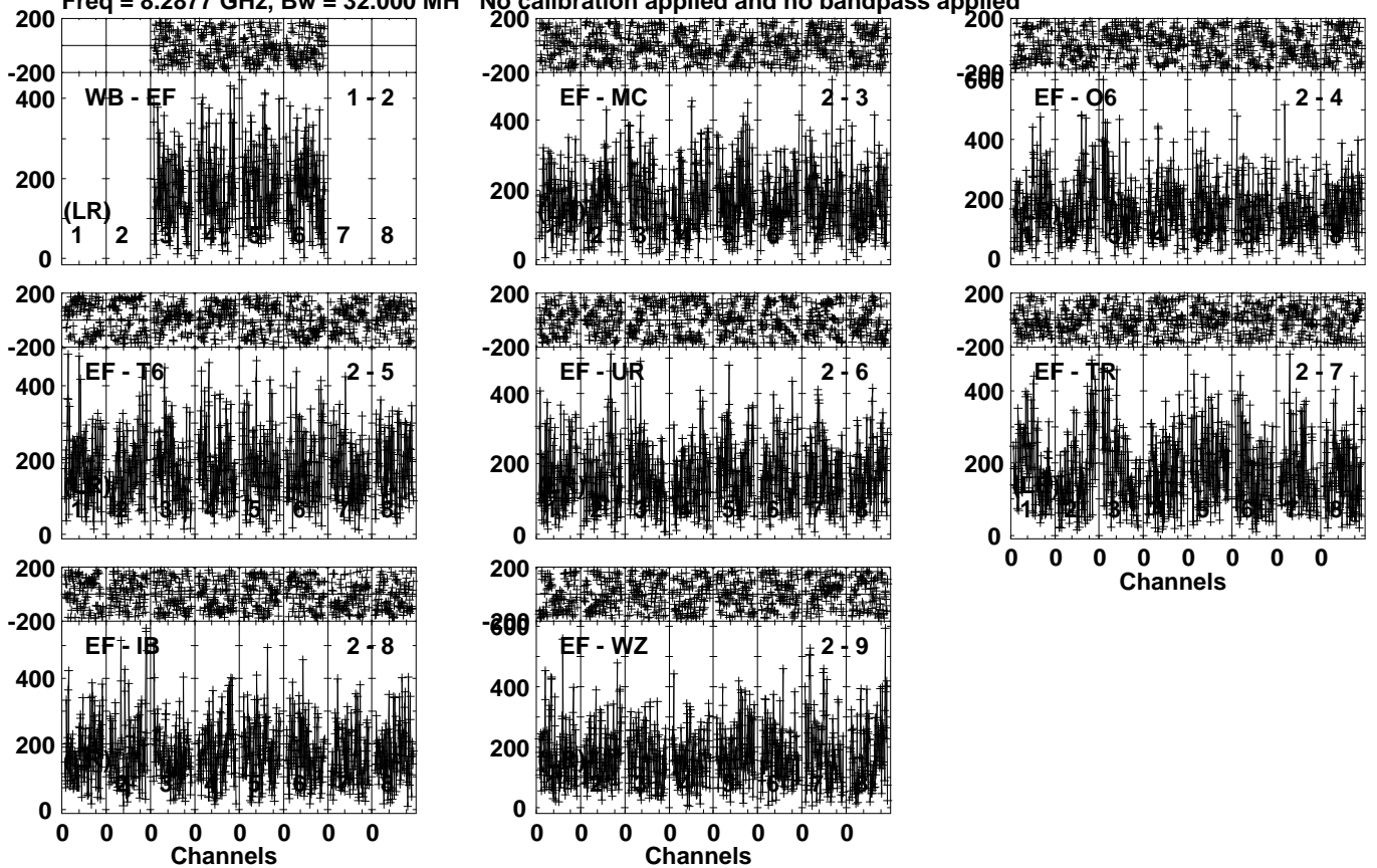
Lower frame: Micro Ampl Jy Top frame: Phas deg Vector averaged cross-power spectrum Several baselines displayed Timerange: 00/16:00:21 to 00/16:03:09
