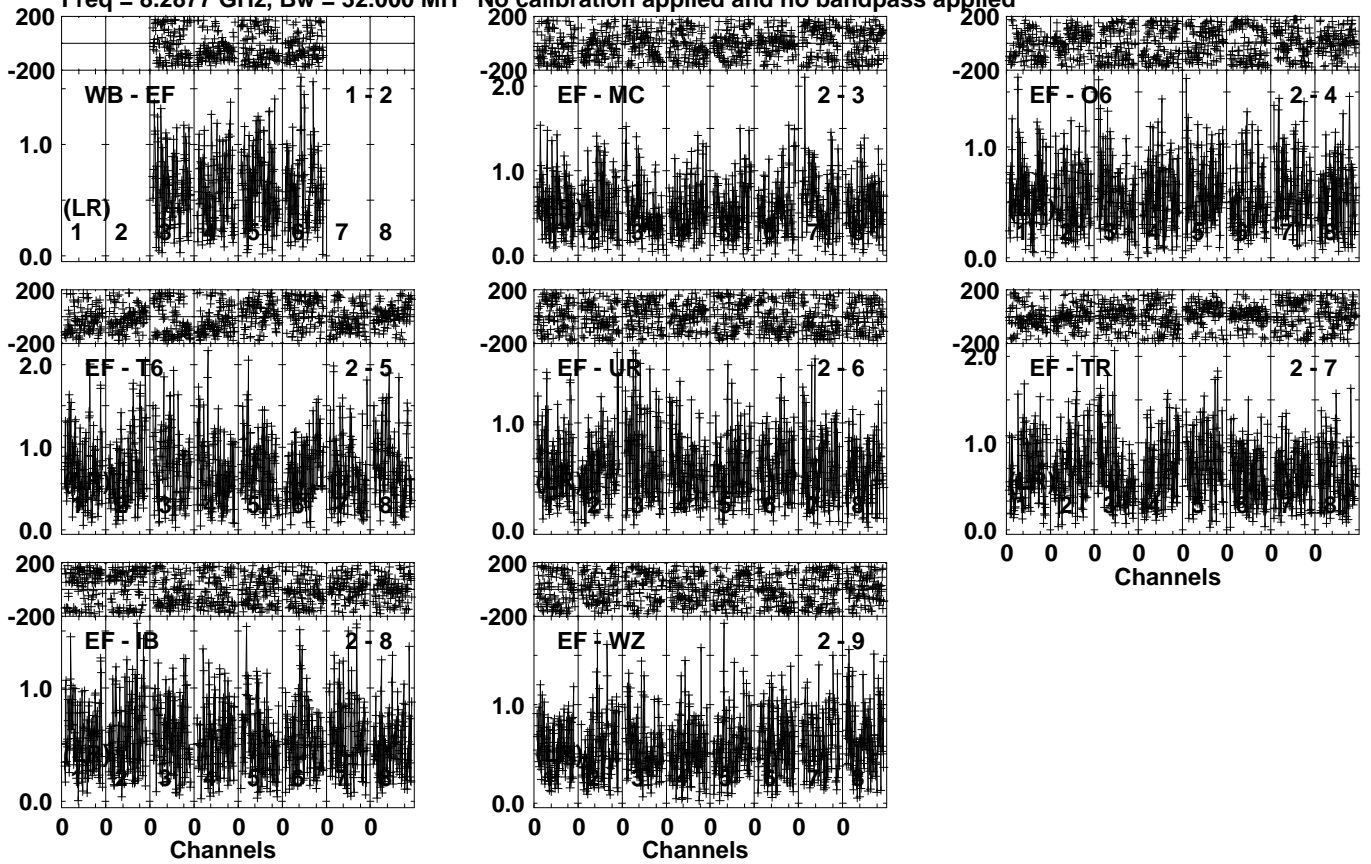
Lower frame: Milli Ampl Jy Top frame: Phas deg Vector averaged cross-power spectrum Several baselines displayed Timerange: 00/16:38:41 to 00/16:39:39
