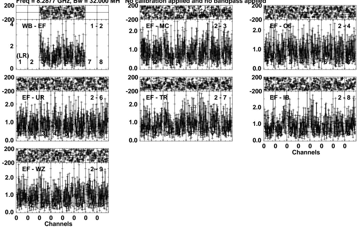
Lower frame: Milli Ampl Jy Top frame: Phas deg Vector averaged cross-power spectrum Several baselines displayed Timerange: 00/18:29:23 to 00/18:30:19
