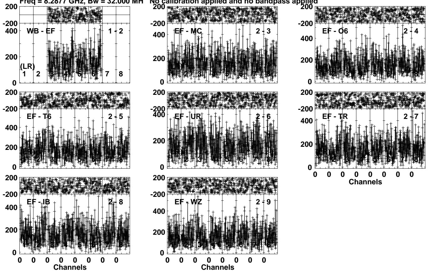
Lower frame: Micro Ampl Jy Top frame: Phas deg Vector averaged cross-power spectrum Several baselines displayed Timerange: 00/18:26:21 to 00/18:29:19
