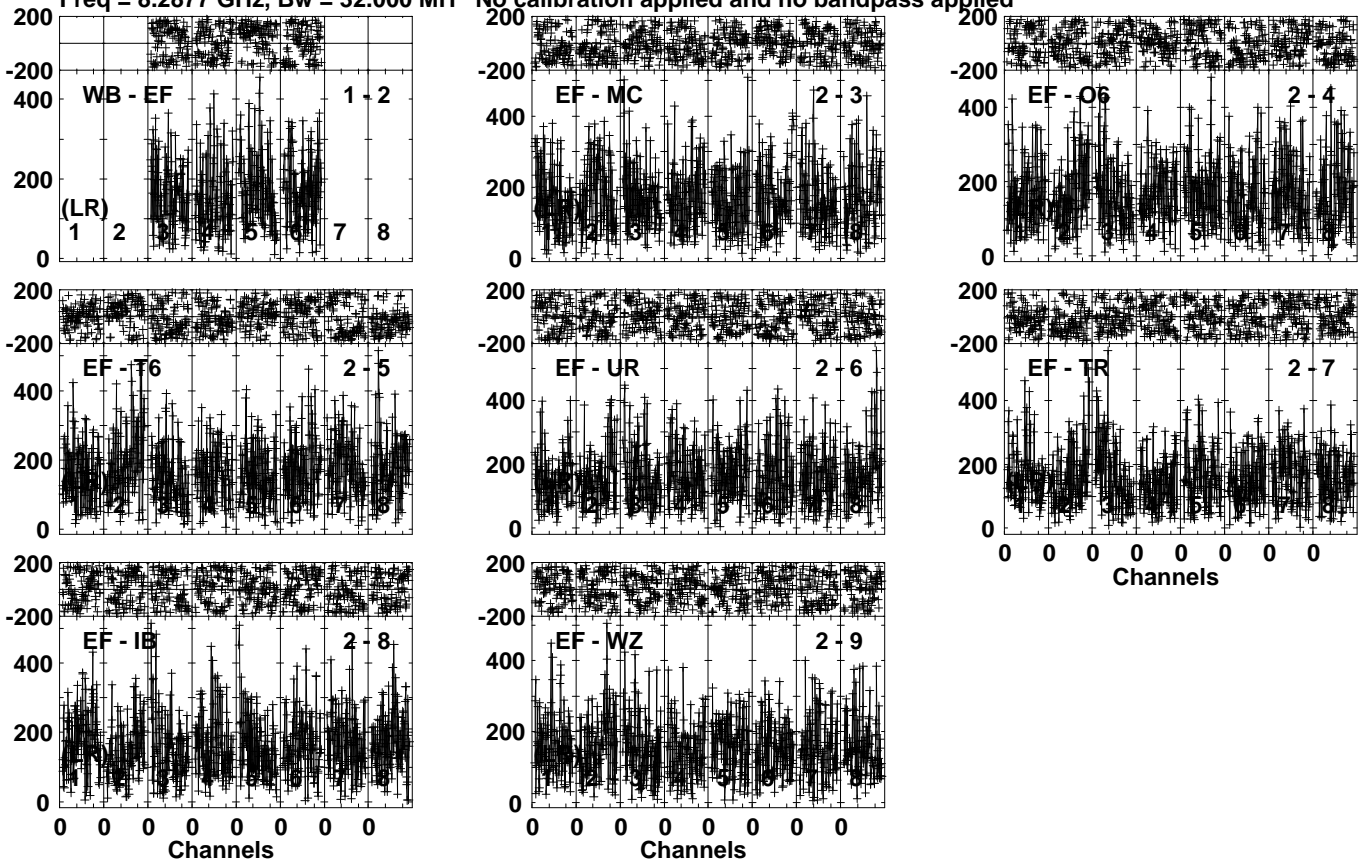
Lower frame: Micro Ampl Jy Top frame: Phas deg Vector averaged cross-power spectrum Several baselines displayed Timerange: 00/18:42:41 to 00/18:45:09
