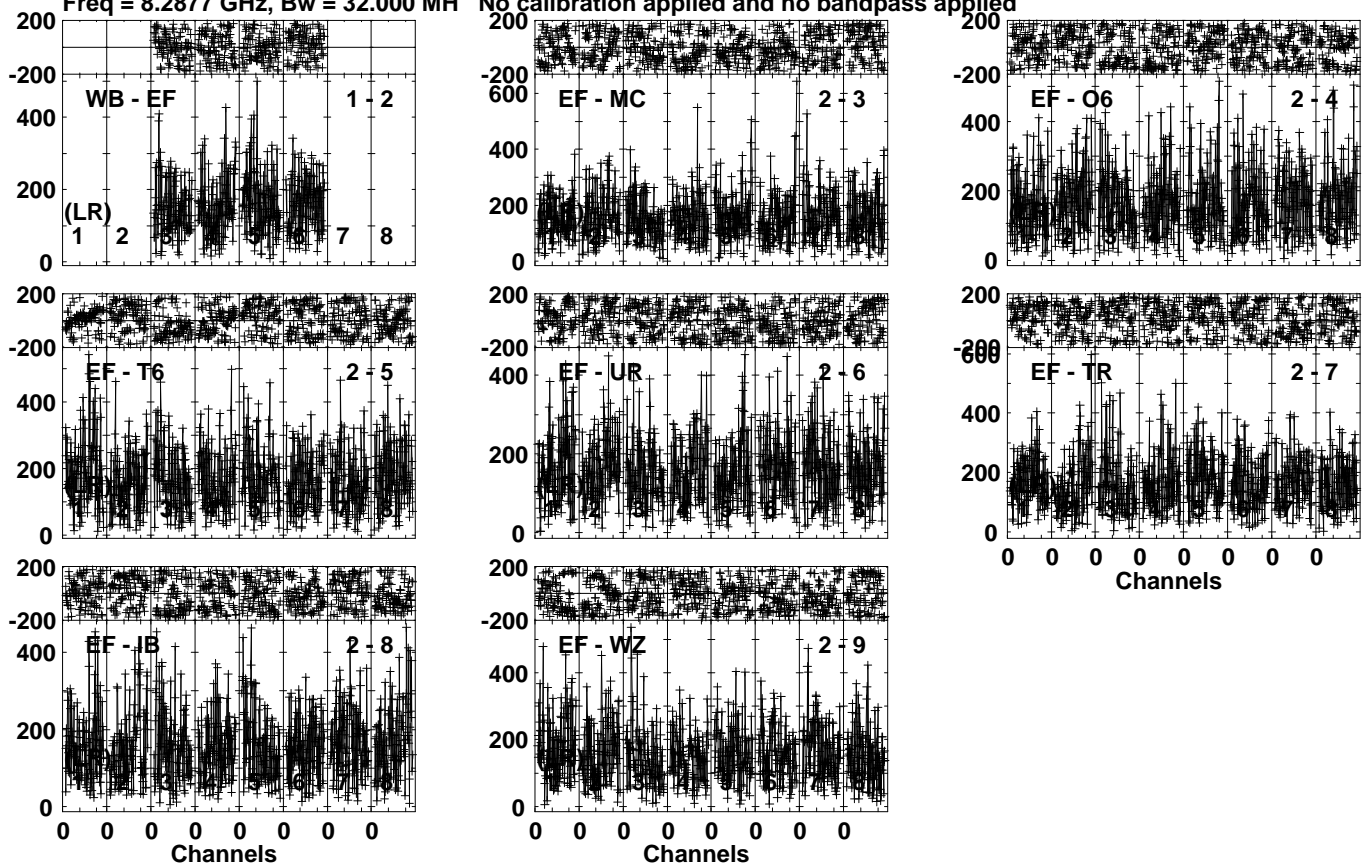
Lower frame: Micro Ampl Jy Top frame: Phas deg Vector averaged cross-power spectrum Several baselines displayed Timerange: 00/16:12:11 to 00/16:14:59
