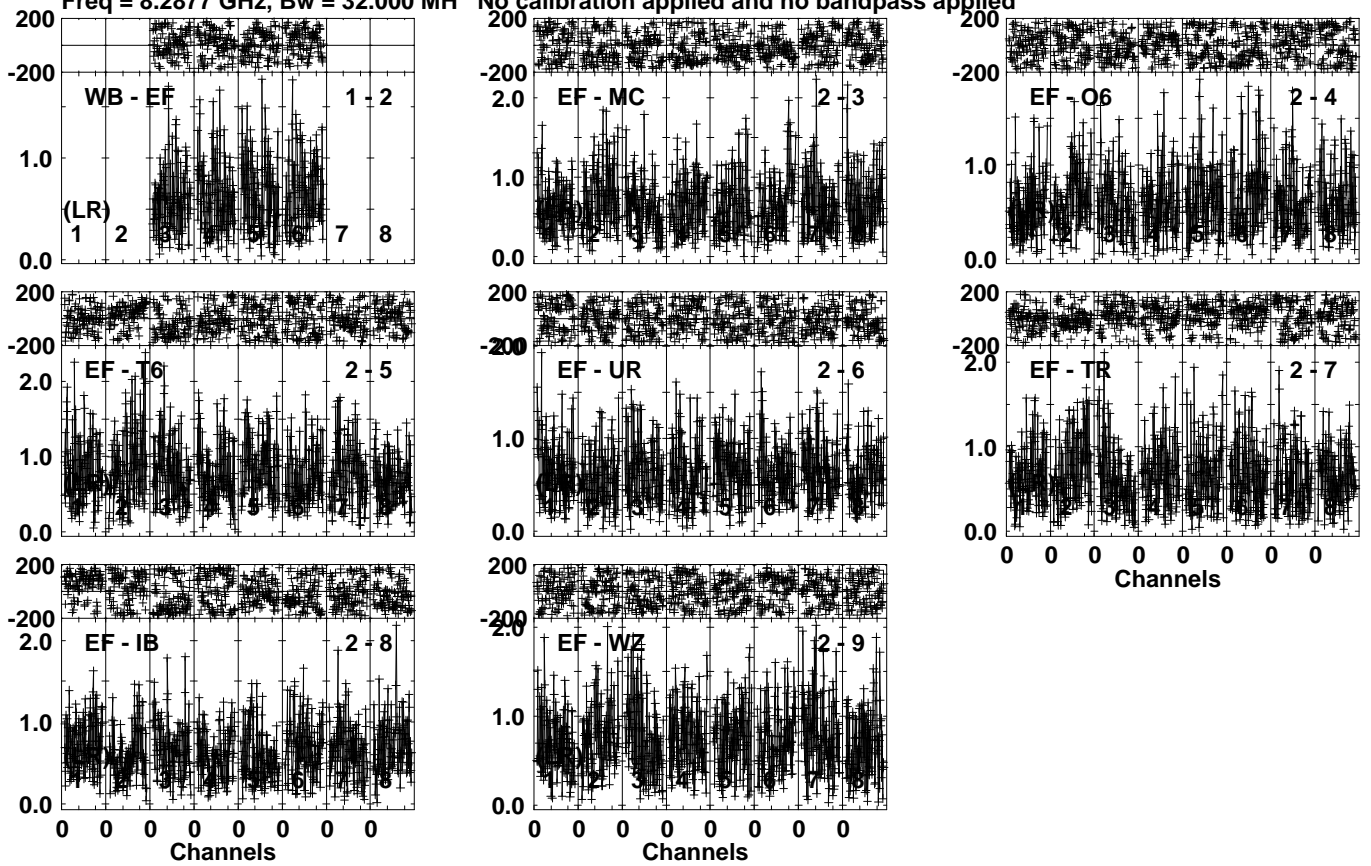
Lower frame: Milli Ampl Jy Top frame: Phas deg Vector averaged cross-power spectrum Several baselines displayed Timerange: 00/16:58:33 to 00/16:59:29
