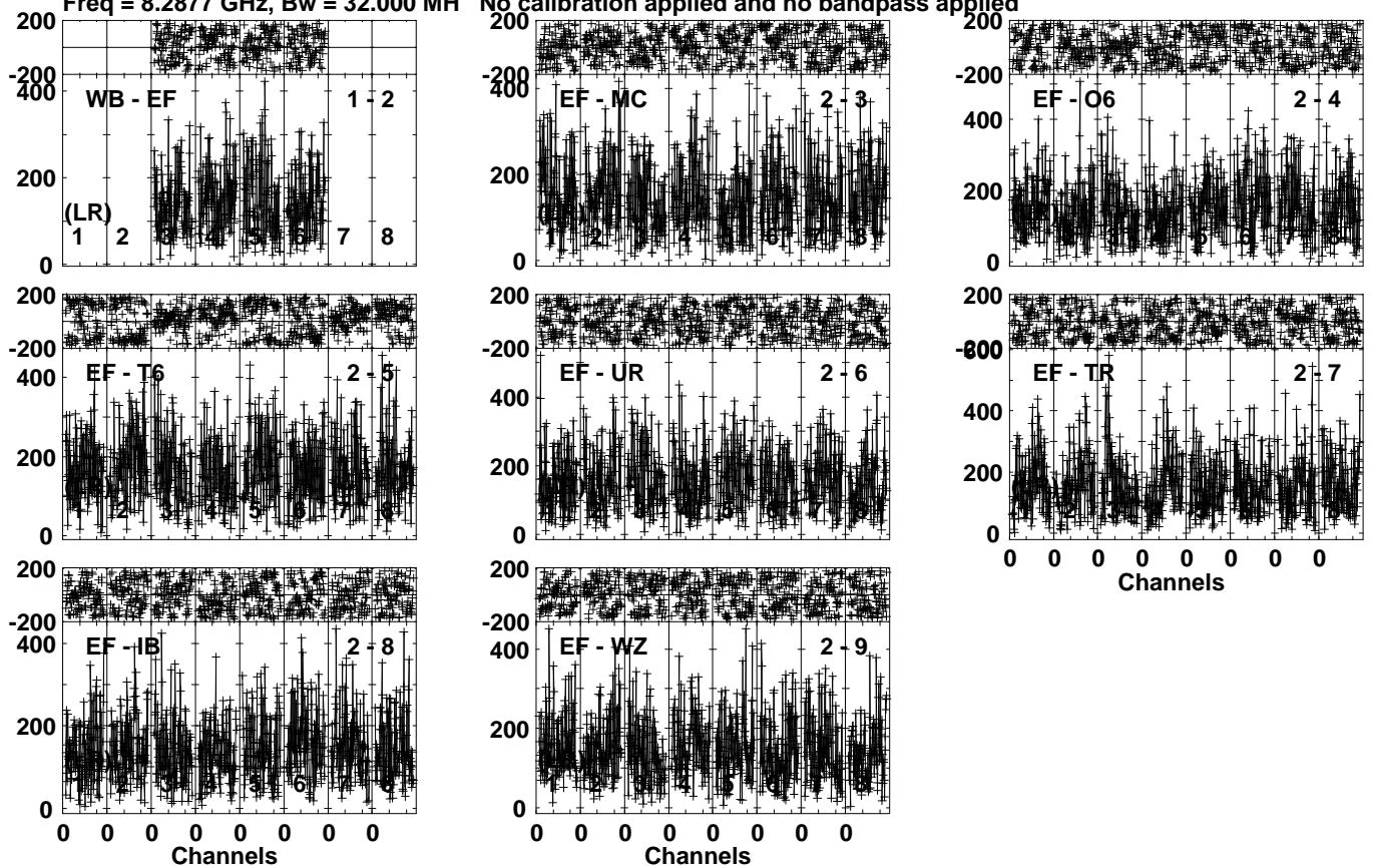
Lower frame: Micro Ampl Jy Top frame: Phas deg Vector averaged cross-power spectrum Several baselines displayed Timerange: 00/19:18:11 to 00/19:20:39
