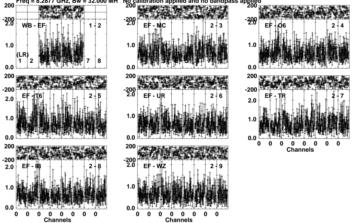
Lower frame: Milli Ampl Jy Top frame: Phas deg Vector averaged cross-power spectrum Several baselines displayed Timerange: 00/17:22:13 to 00/17:23:09
