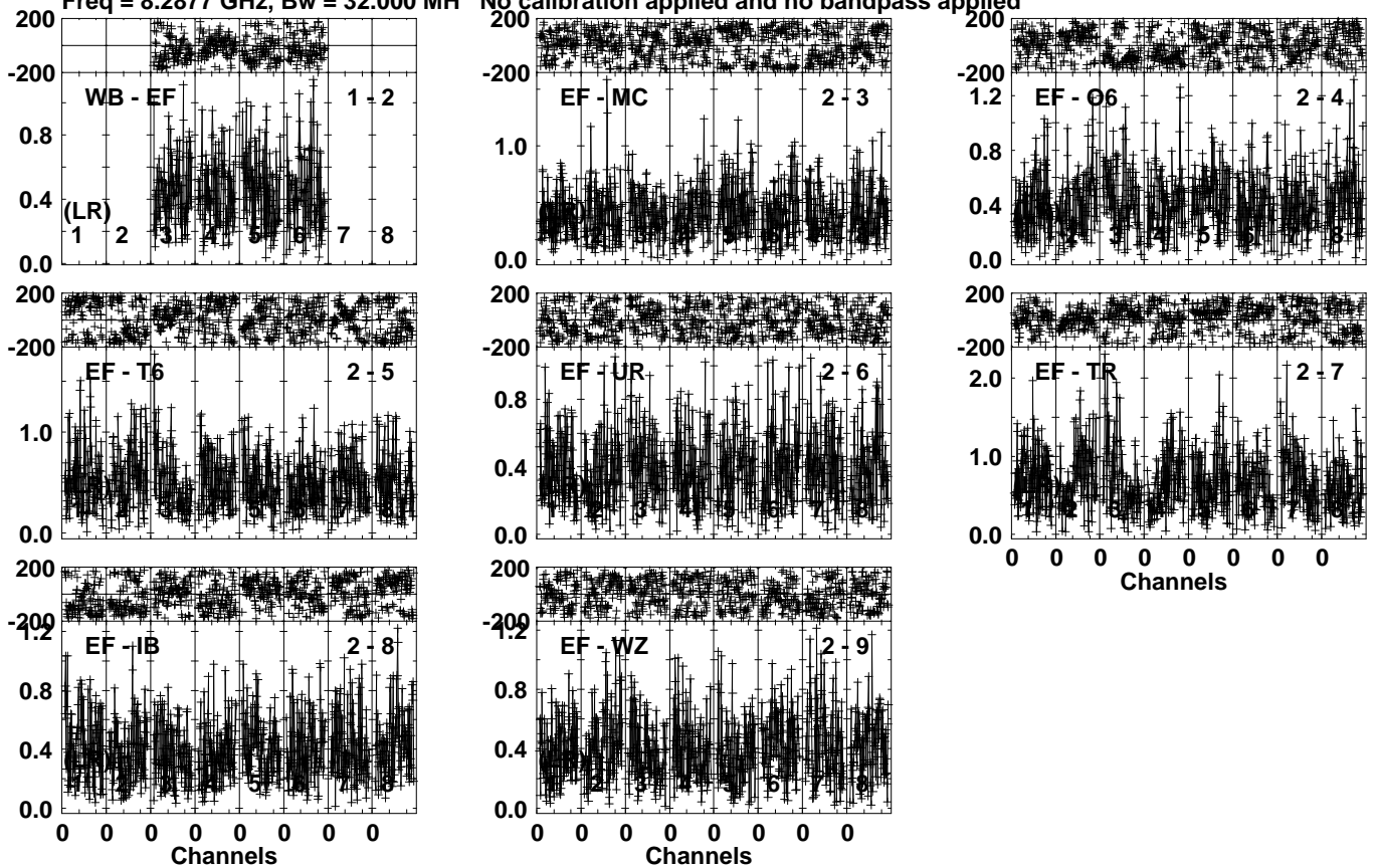
Lower frame: Milli Ampl Jy Top frame: Phas deg Vector averaged cross-power spectrum Several baselines displayed Timerange: 00/15:19:53 to 00/15:20:49
