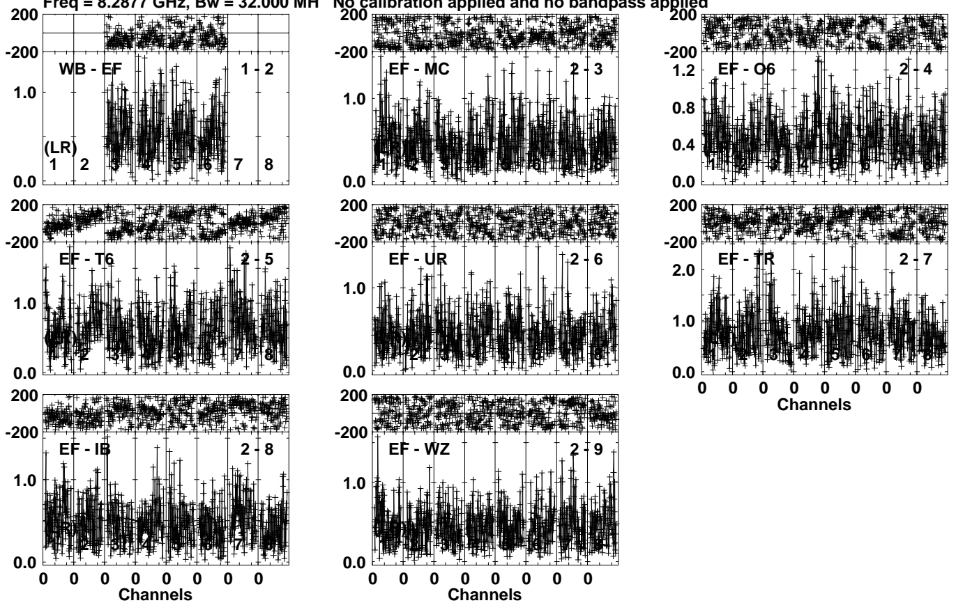
Lower frame: Milli Ampl Jy Top frame: Phas deg Vector averaged cross-power spectrum Several baselines displayed Timerange: 00/18:17:33 to 00/18:18:29
