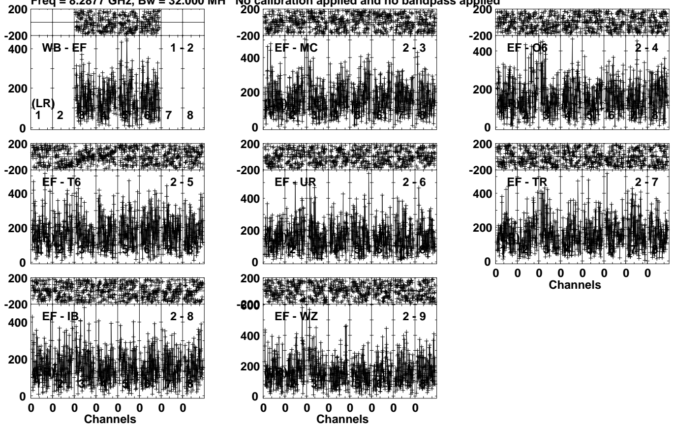
Lower frame: Micro Ampl Jy Top frame: Phas deg Vector averaged cross-power spectrum Several baselines displayed Timerange: 00/16:44:11 to 00/16:46:39
