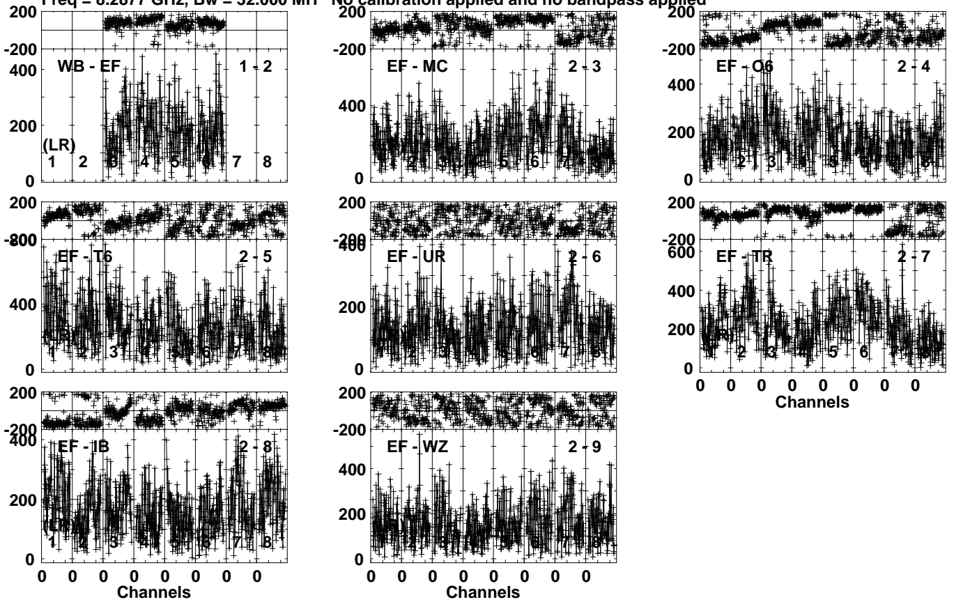
Lower frame: Micro Ampl Jy Top frame: Phas deg Vector averaged cross-power spectrum Several baselines displayed Timerange: 00/15:00:01 to 00/15:04:59
