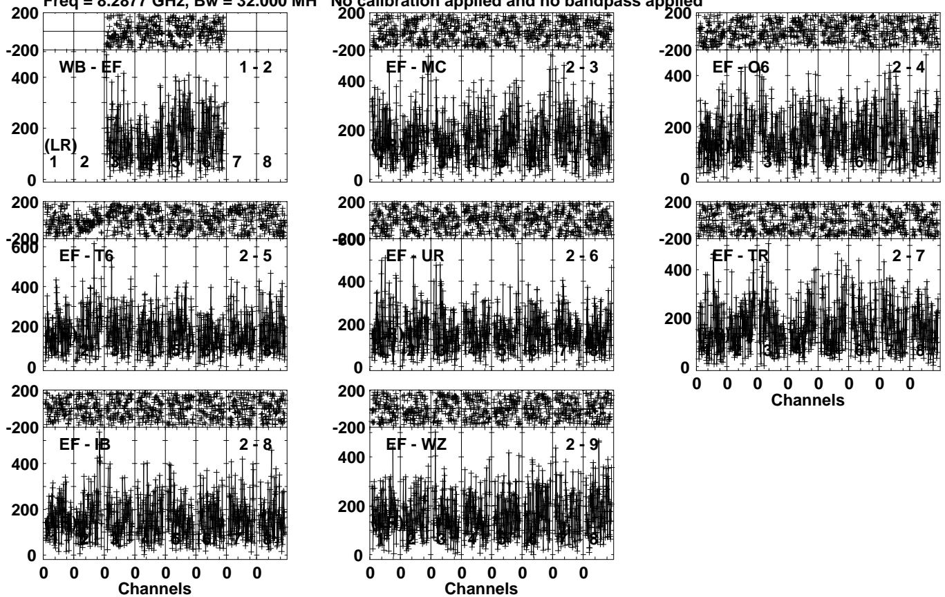
Lower frame: Micro Ampl Jy Top frame: Phas deg Vector averaged cross-power spectrum Several baselines displayed Timerange: 00/17:46:51 to 00/17:49:39
