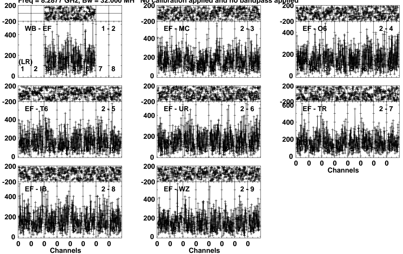
Lower frame: Micro Ampl Jy Top frame: Phas deg Vector averaged cross-power spectrum Several baselines displayed Timerange: 00/16:04:11 to 00/16:07:09
