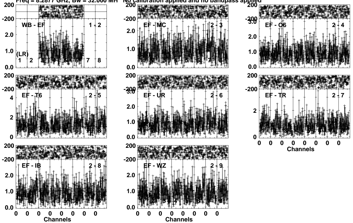
Lower frame: Milli Ampl Jy Top frame: Phas deg Vector averaged cross-power spectrum Several baselines displayed Timerange: 00/18:45:13 to 00/18:46:09
