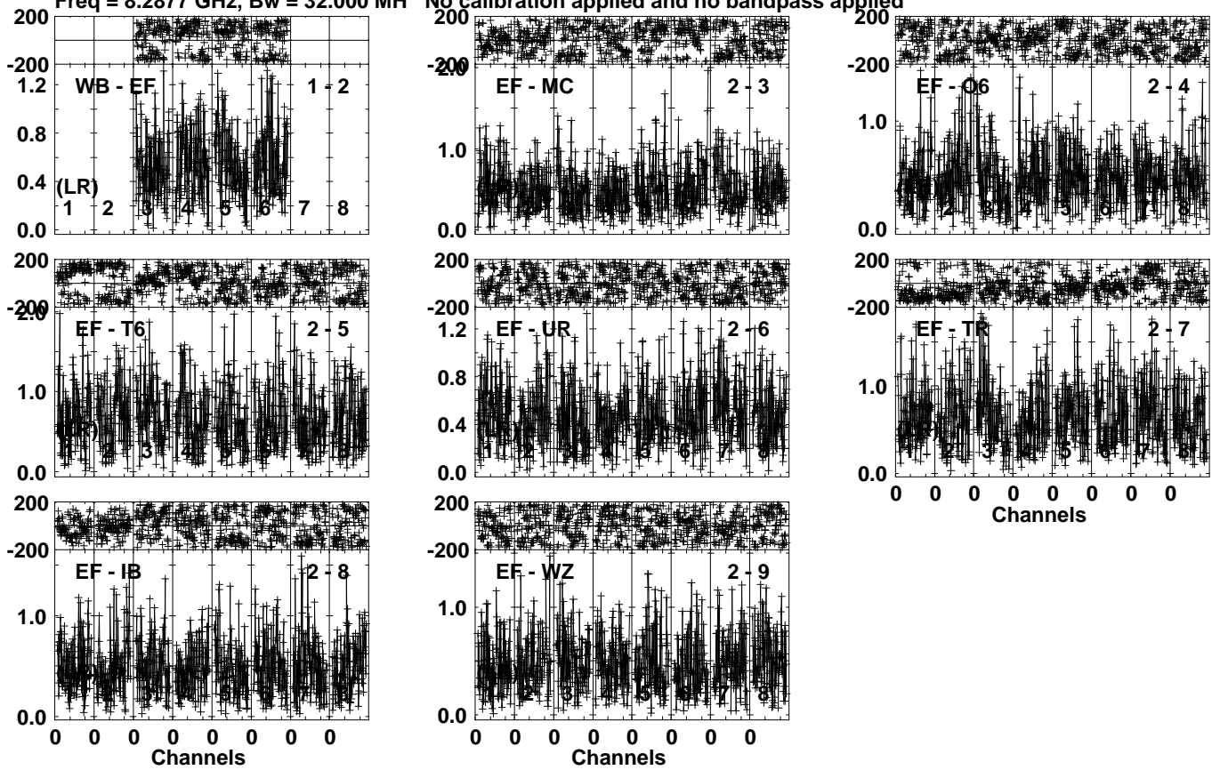
Lower frame: Milli Ampl Jy Top frame: Phas deg Vector averaged cross-power spectrum Several baselines displayed Timerange: 00/16:19:03 to 00/16:19:59
