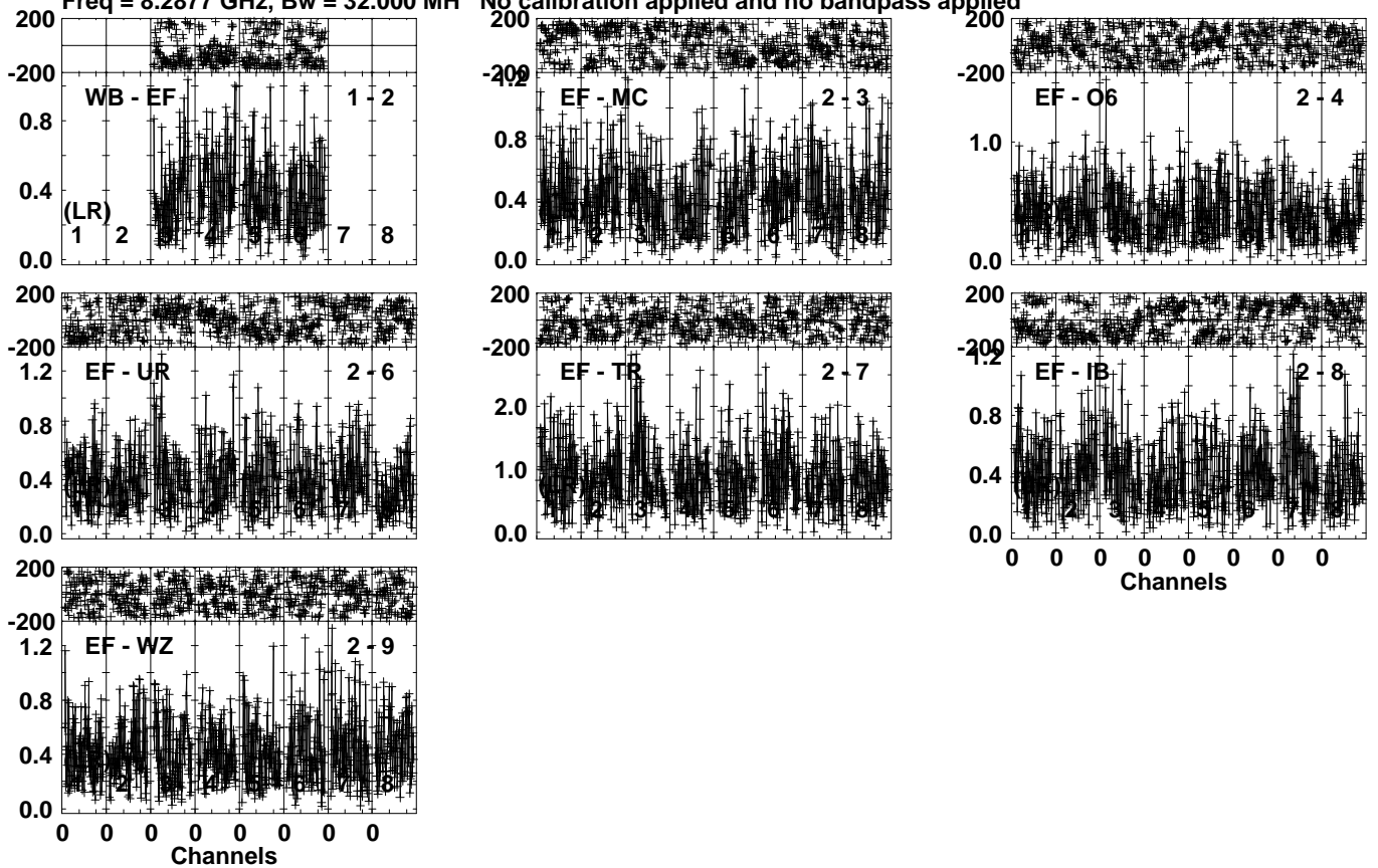
Lower frame: Milli Ampl Jy Top frame: Phas deg Vector averaged cross-power spectrum Several baselines displayed Timerange: 00/20:47:21 to 00/20:48:19
