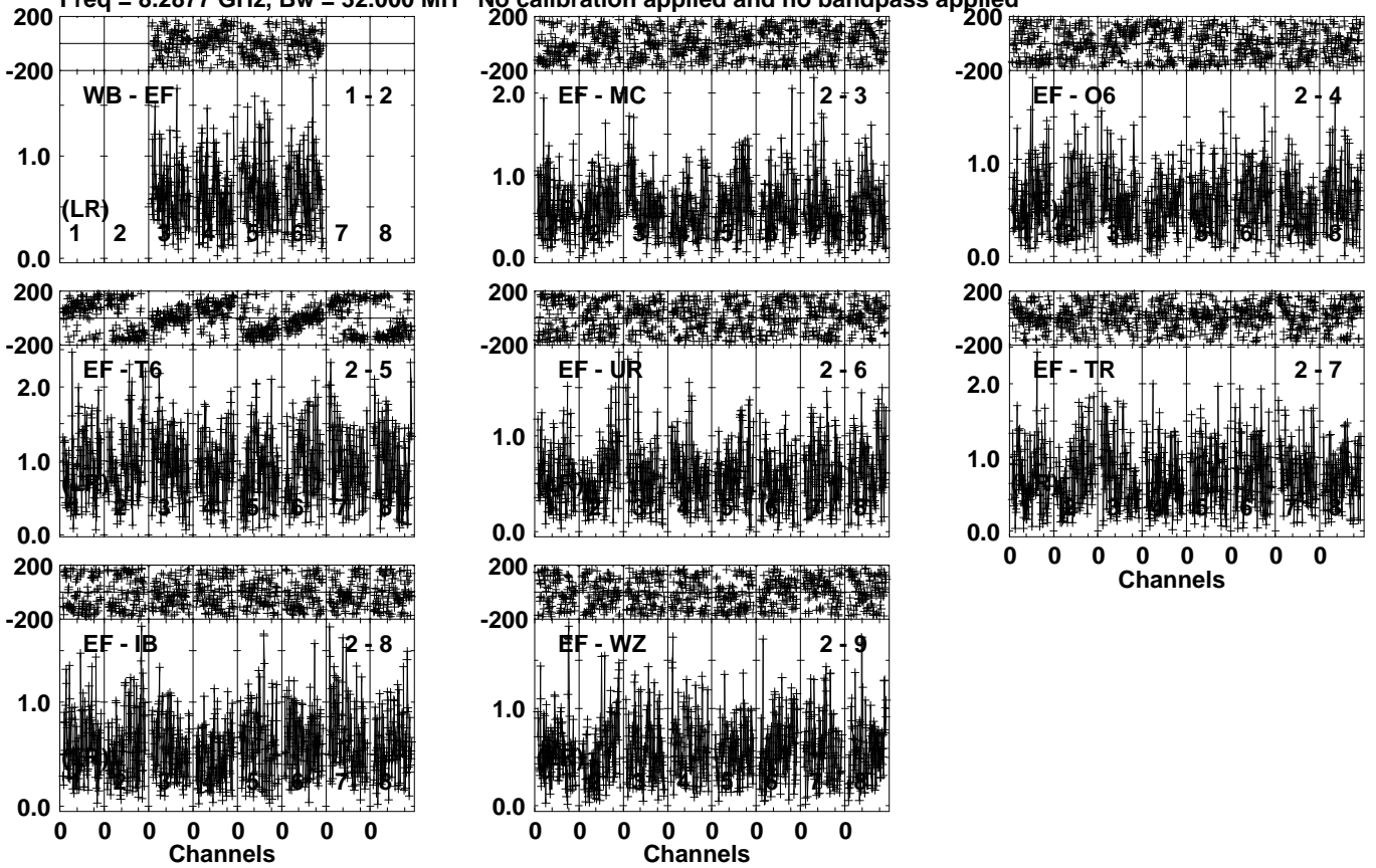
Lower frame: Milli Ampl Jy Top frame: Phas deg Vector averaged cross-power spectrum Several baselines displayed Timerange: 00/19:04:51 to 00/19:05:49
