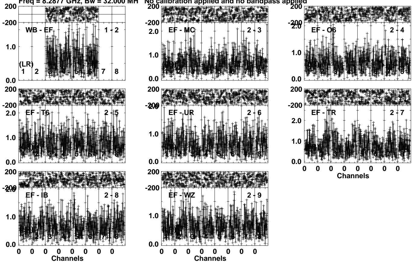
Lower frame: Milli Ampl Jy Top frame: Phas deg Vector averaged cross-power spectrum Several baselines displayed Timerange: 00/17:14:11 to 00/17:15:09
