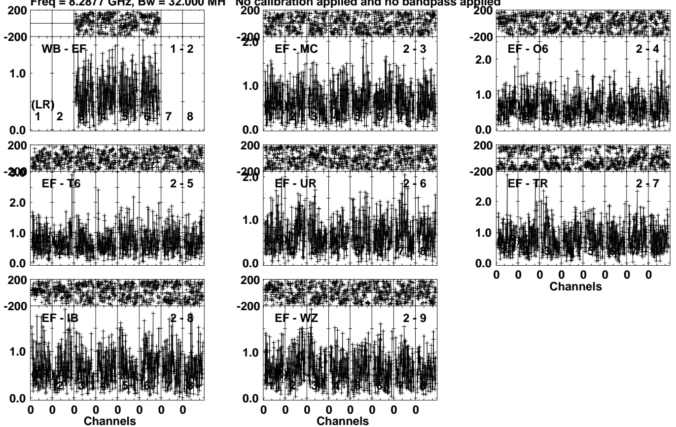
Lower frame: Milli Ampl Jy Top frame: Phas deg Vector averaged cross-power spectrum Several baselines displayed Timerange: 00/17:10:23 to 00/17:11:19
