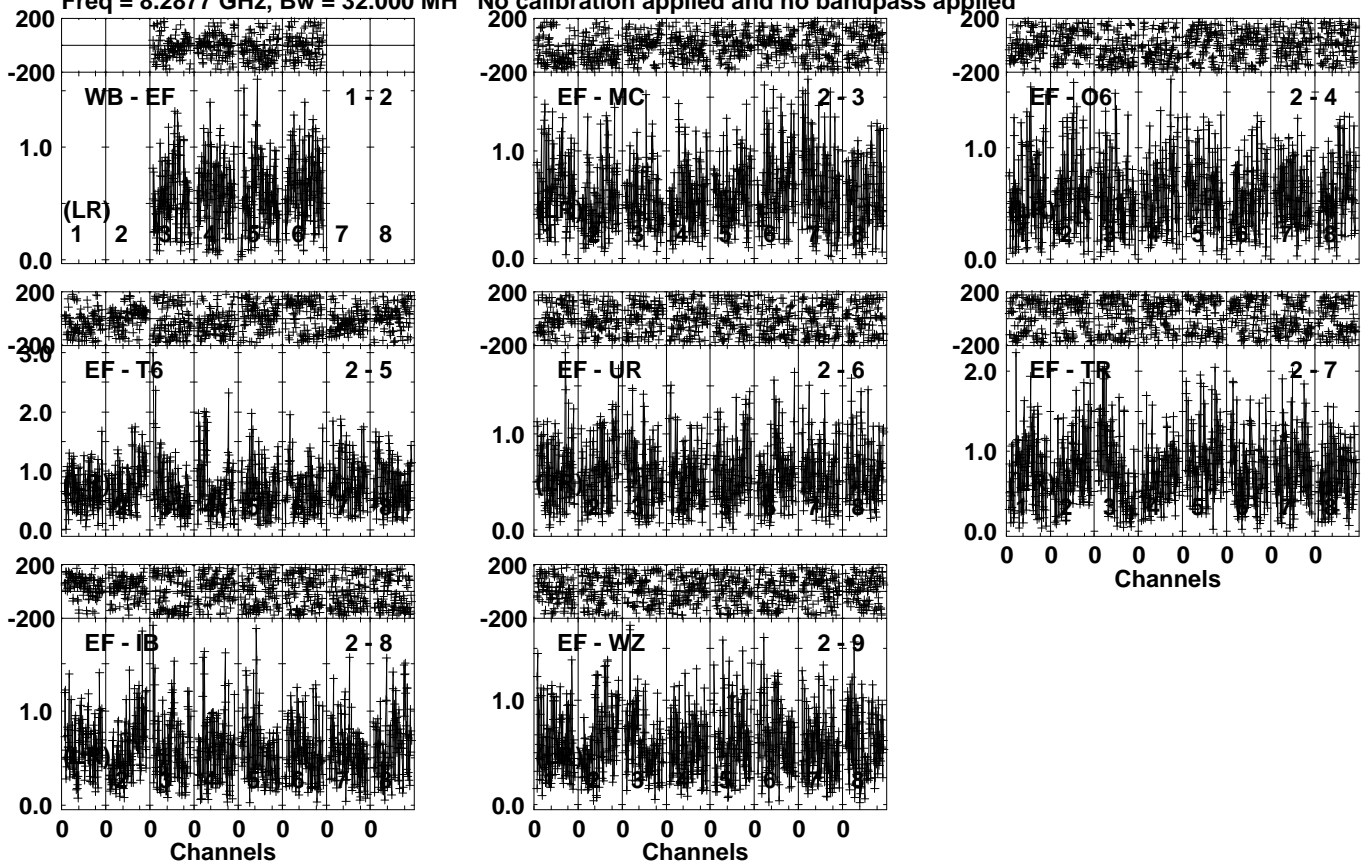
Lower frame: Milli Ampl Jy Top frame: Phas deg Vector averaged cross-power spectrum Several baselines displayed Timerange: 00/17:45:51 to 00/17:46:49
