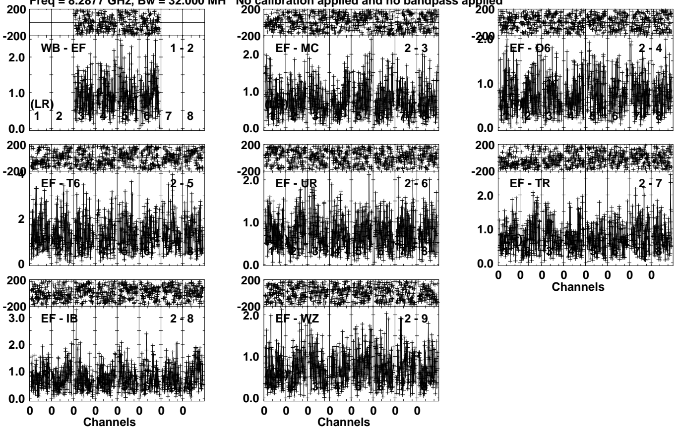
Lower frame: Milli Ampl Jy Top frame: Phas deg Vector averaged cross-power spectrum Several baselines displayed Timerange: 00/18:53:01 to 00/18:53:59
