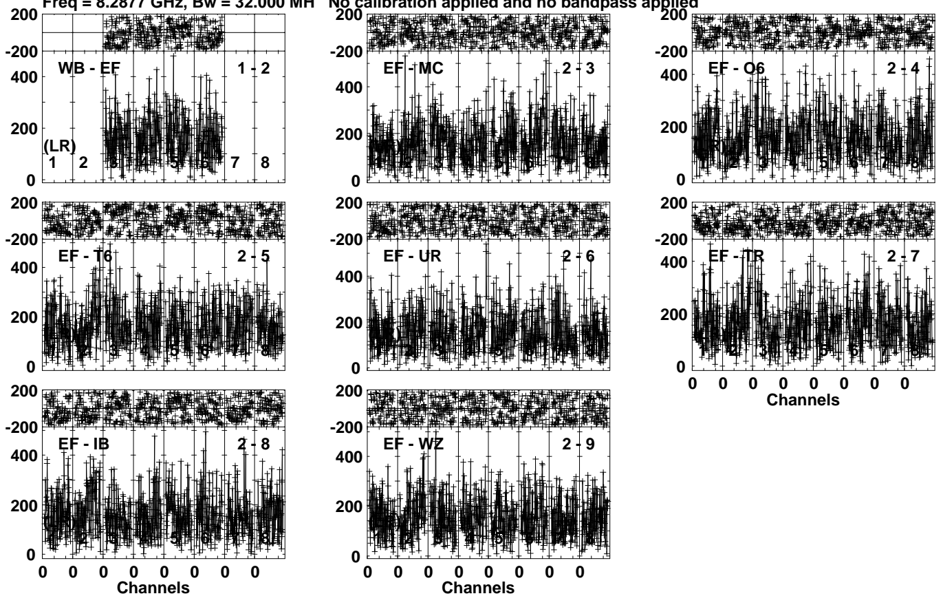
Lower frame: Micro Ampl Jy Top frame: Phas deg Vector averaged cross-power spectrum Several baselines displayed Timerange: 00/15:21:21 to 00/15:23:49
