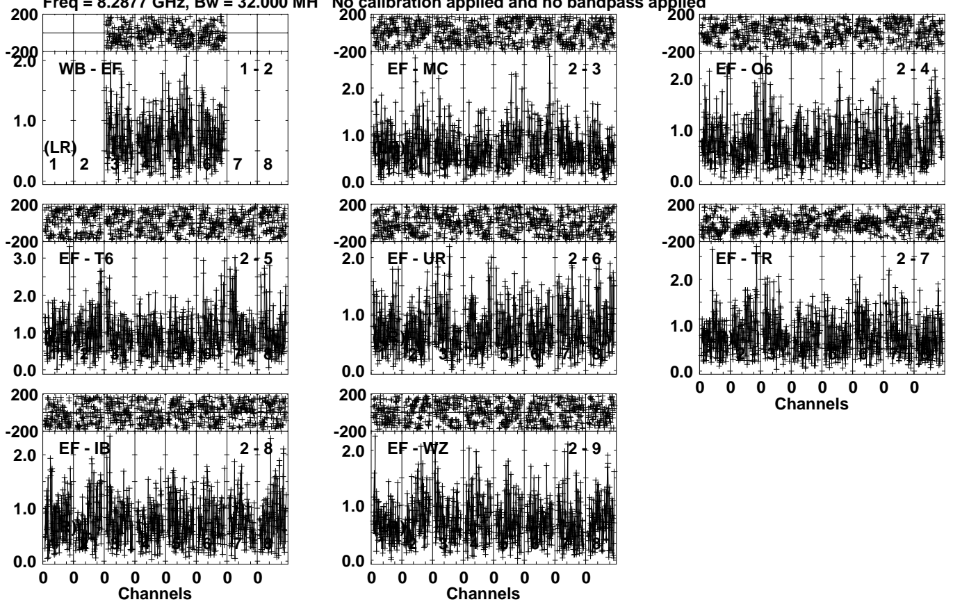
Lower frame: Milli Ampl Jy Top frame: Phas deg Vector averaged cross-power spectrum Several baselines displayed Timerange: 00/15:23:53 to 00/15:24:49
