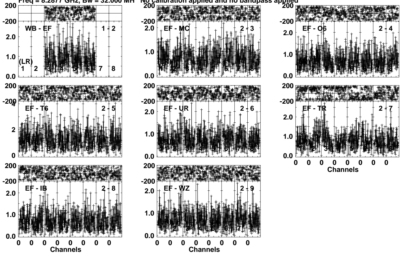
Lower frame: Milli Ampl Jy Top frame: Phas deg Vector averaged cross-power spectrum Several baselines displayed Timerange: 00/15:43:33 to 00/15:44:29
