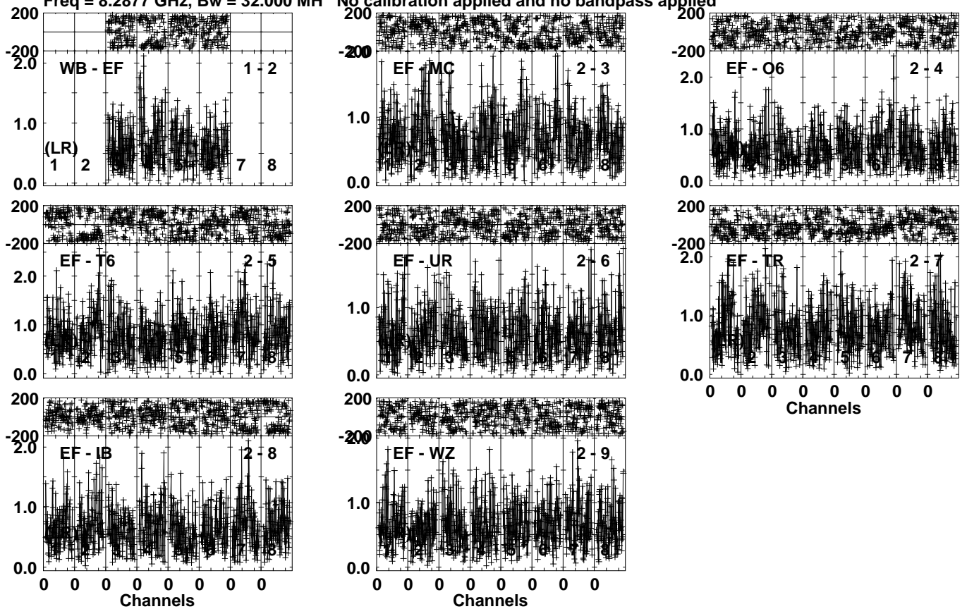
Lower frame: Milli Ampl Jy Top frame: Phas deg Vector averaged cross-power spectrum Several baselines displayed Timerange: 00/17:26:01 to 00/17:26:59
