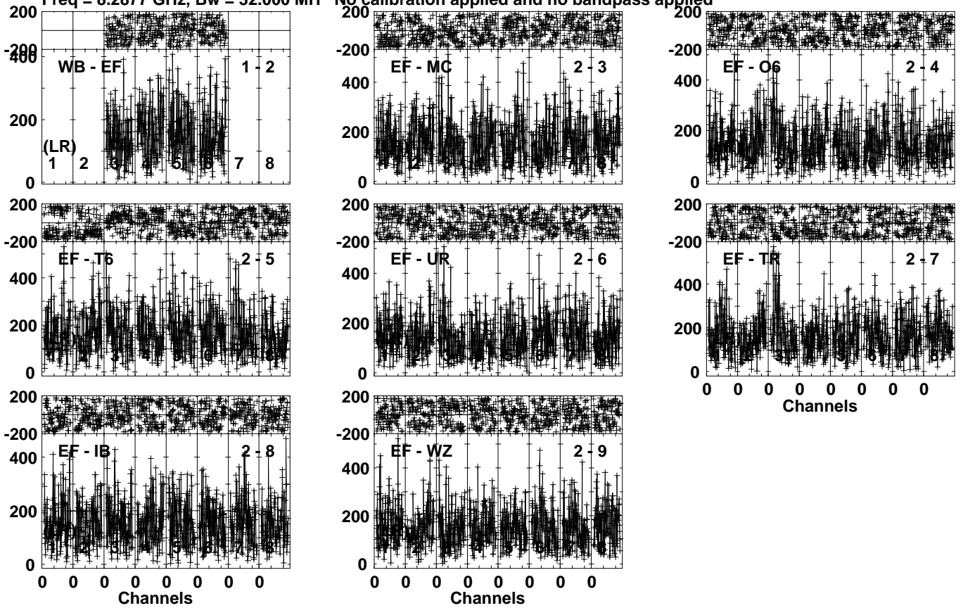
Lower frame: Micro Ampl Jy Top frame: Phas deg Vector averaged cross-power spectrum Several baselines displayed Timerange: 00/16:08:41 to 00/16:11:09
