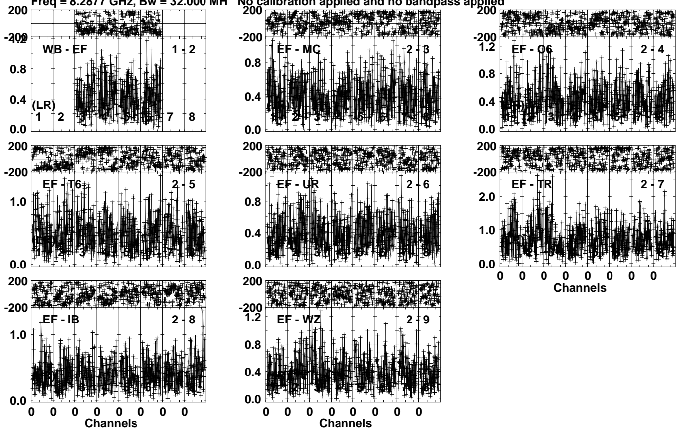
Lower frame: Milli Ampl Jy Top frame: Phas deg Vector averaged cross-power spectrum Several baselines displayed Timerange: 00/15:15:51 to 00/15:16:49
