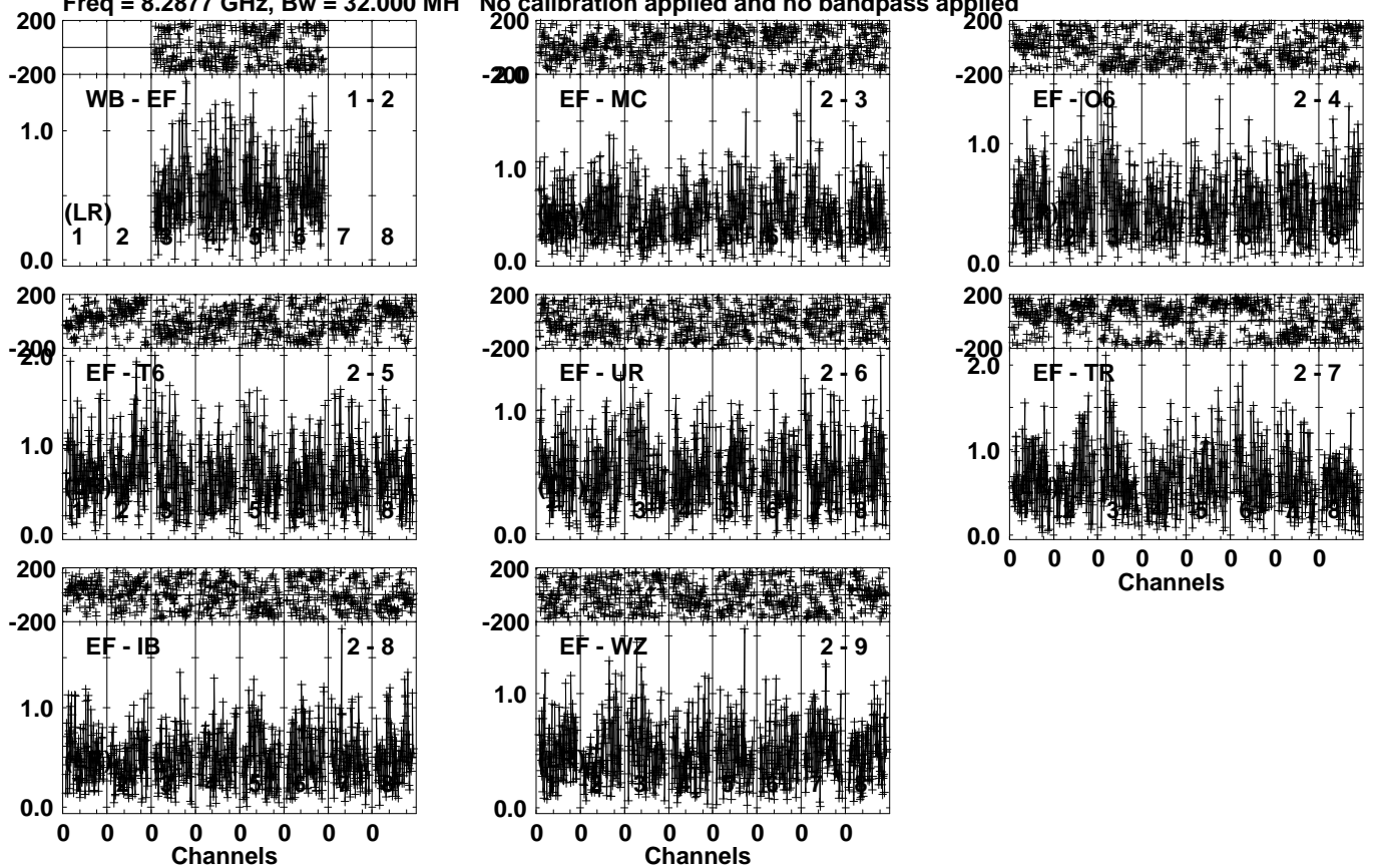
Lower frame: Milli Ampl Jy Top frame: Phas deg Vector averaged cross-power spectrum Several baselines displayed Timerange: 00/16:30:53 to 00/16:31:49
