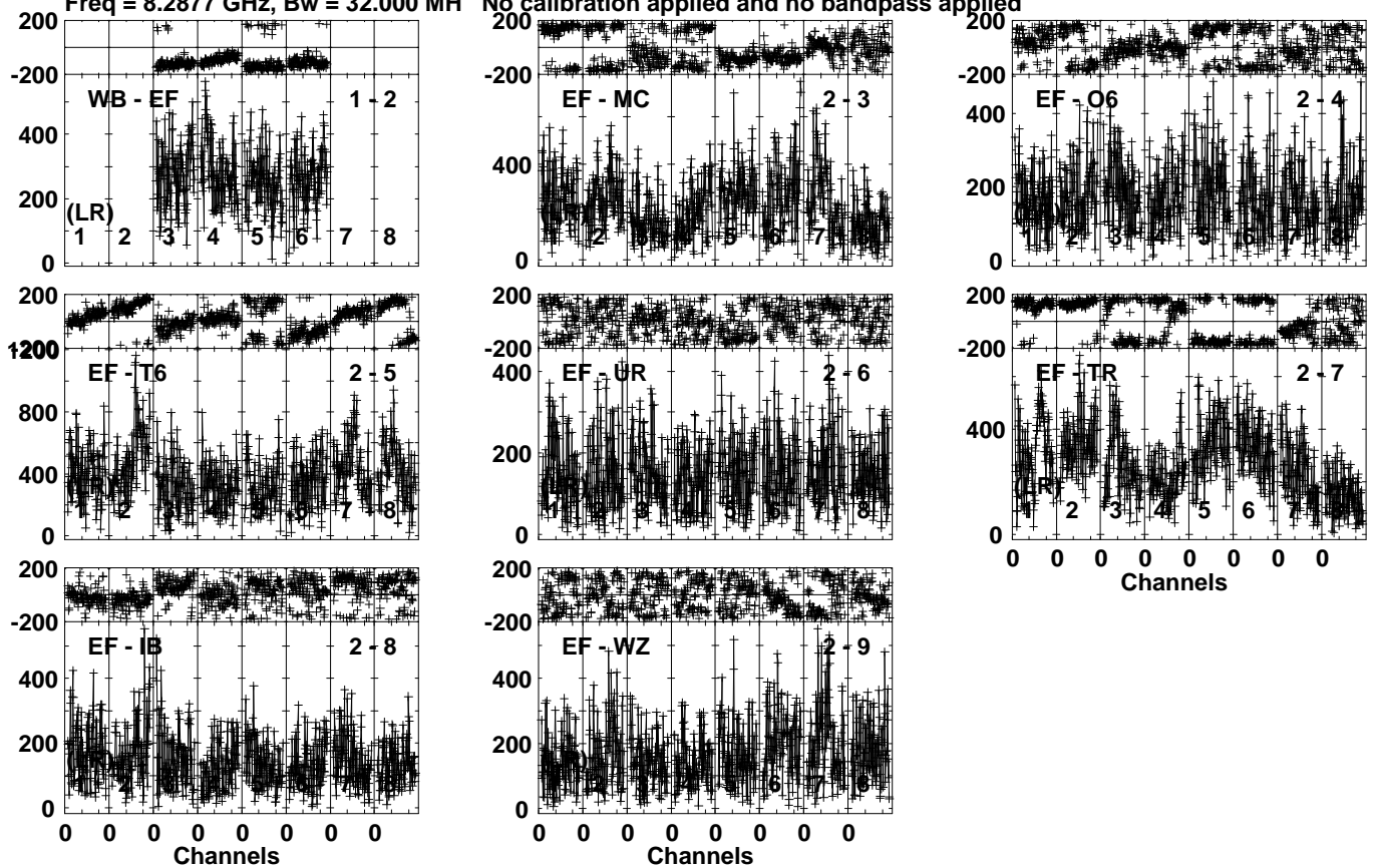
Lower frame: Micro Ampl Jy Top frame: Phas deg Vector averaged cross-power spectrum Several baselines displayed Timerange: 00/18:09:33 to 00/18:14:29
