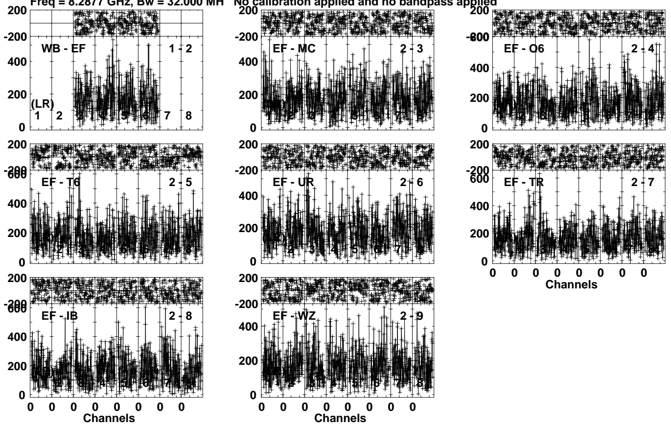
Lower frame: Micro Ampl Jy Top frame: Phas deg Vector averaged cross-power spectrum Several baselines displayed Timerange: 00/18:22:31 to 00/18:25:19
