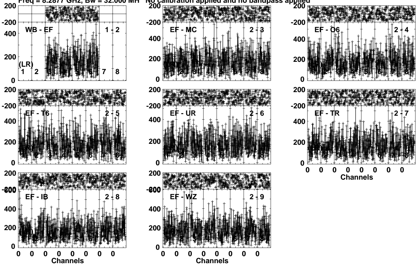
Lower frame: Micro Ampl Jy Top frame: Phas deg Vector averaged cross-power spectrum Several baselines displayed Timerange: 00/18:34:21 to 00/18:37:09
