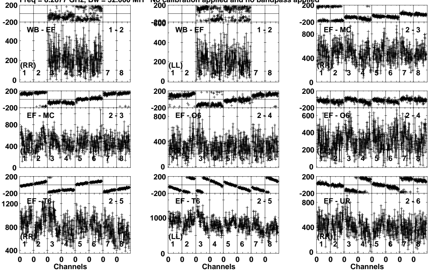
Lower frame: Micro Ampl Jy Top frame: Phas deg Vector averaged cross-power spectrum Several baselines displayed Timerange: 00/17:58:43 to 00/18:01:29
