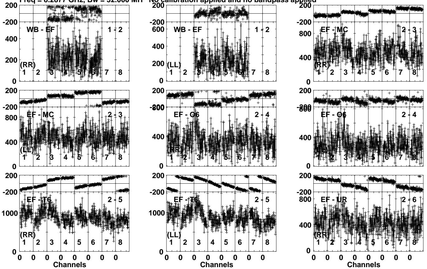
Lower frame: Micro Ampl Jy Top frame: Phas deg Vector averaged cross-power spectrum Several baselines displayed Timerange: 00/16:59:31 to 00/17:02:19
