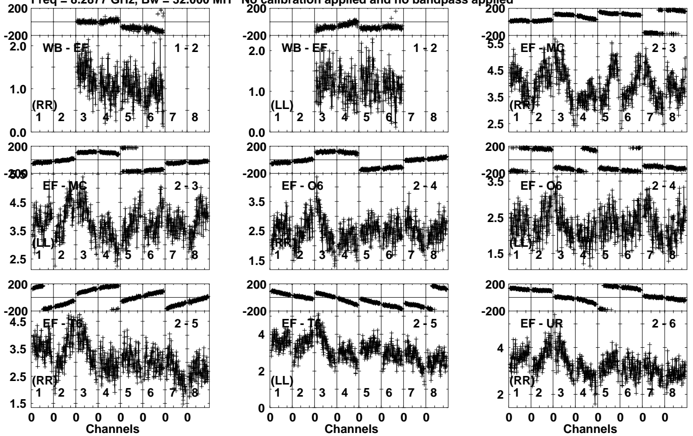
Lower frame: Milli Ampl Jy Top frame: Phas deg Vector averaged cross-power spectrum Several baselines displayed Timerange: 00/19:20:43 to 00/19:21:39
