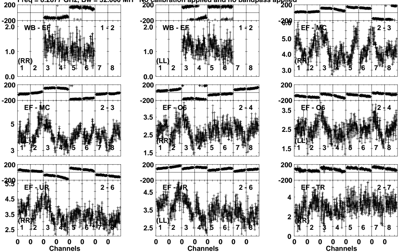
Lower frame: Milli Ampl Jy Top frame: Phas deg Vector averaged cross-power spectrum Several baselines displayed Timerange: 00/19:44:23 to 00/19:45:19
