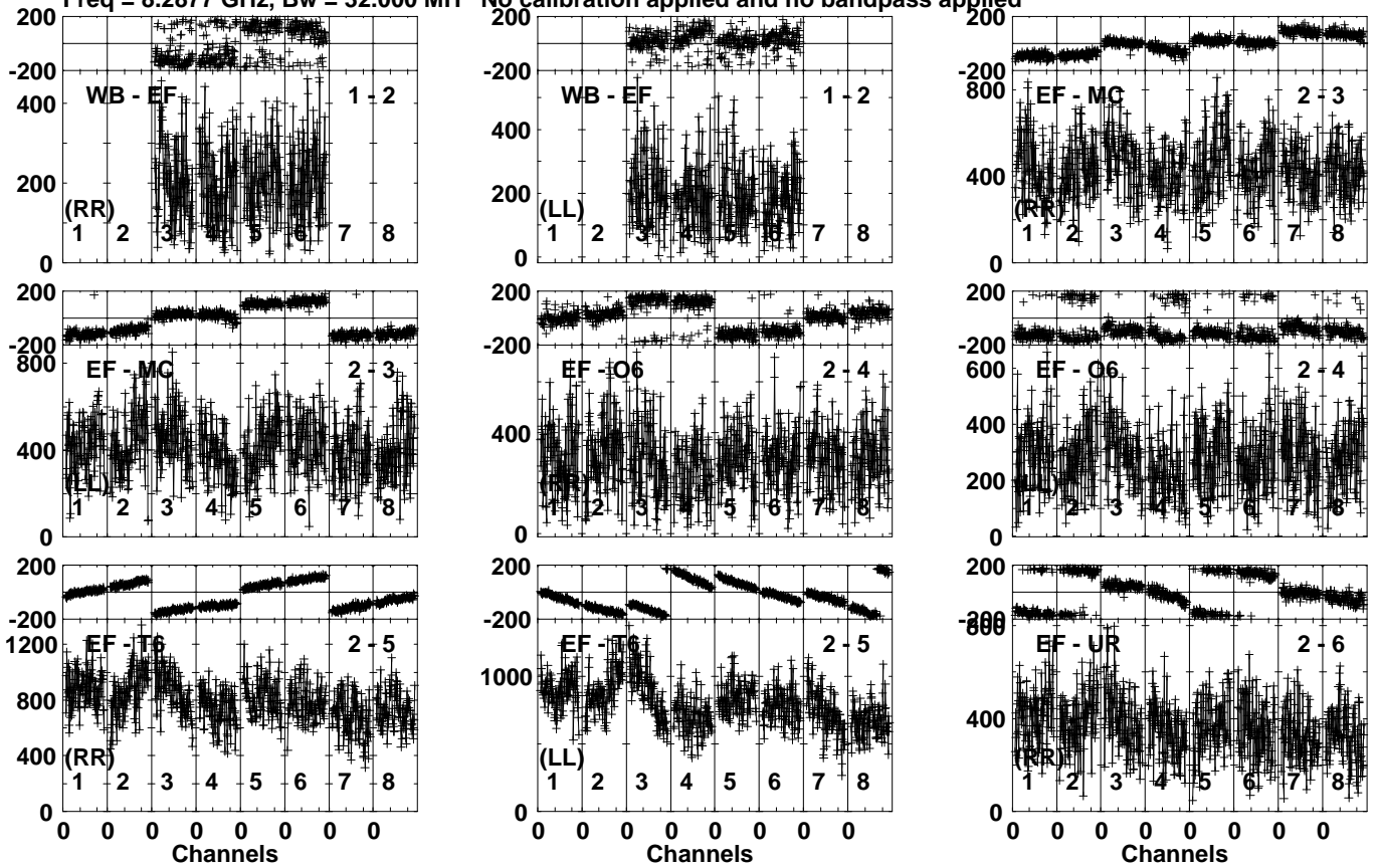
Lower frame: Micro Ampl Jy Top frame: Phas deg Vector averaged cross-power spectrum Several baselines displayed Timerange: 00/17:07:51 to 00/17:10:19
