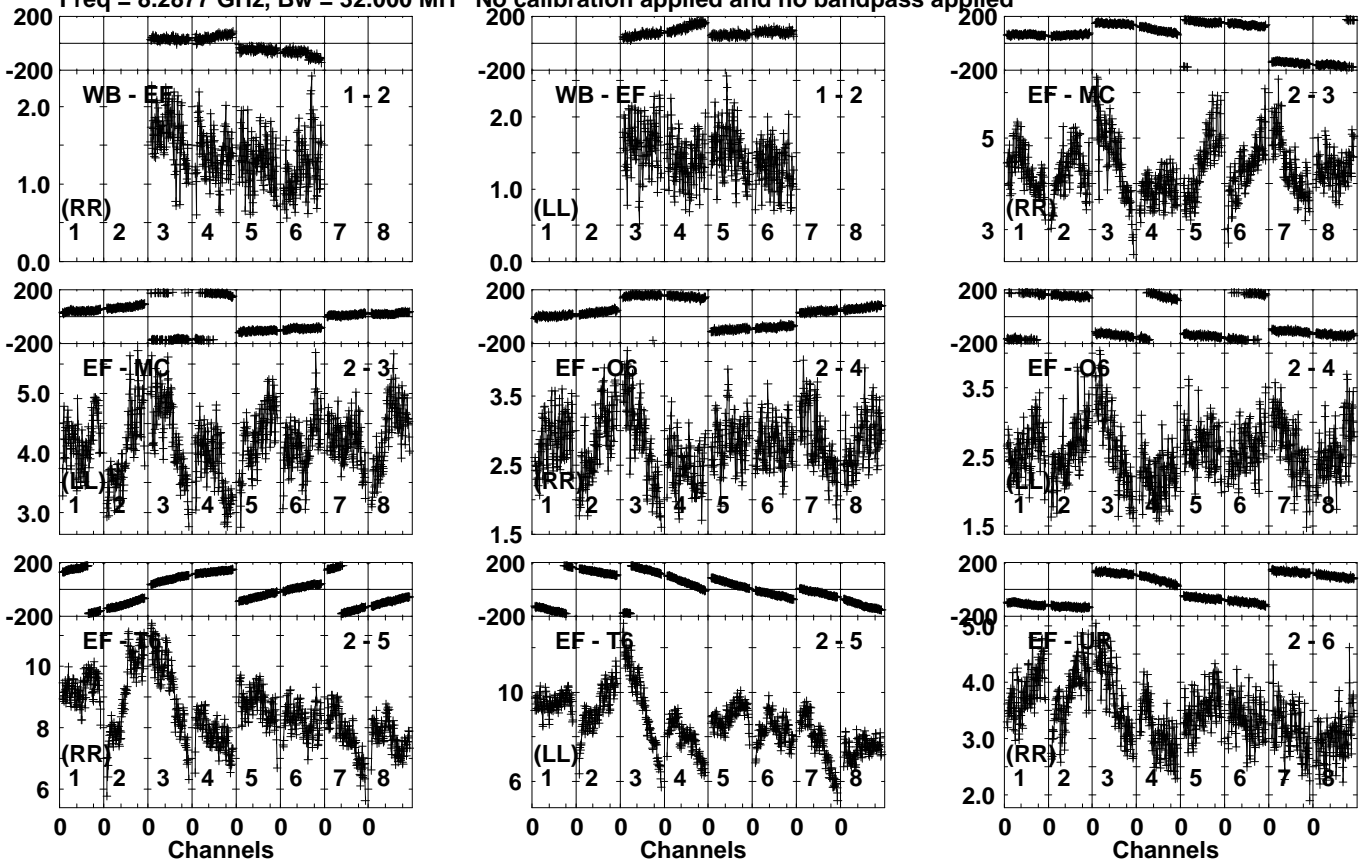
Lower frame: Milli Ampl Jy Top frame: Phas deg Vector averaged cross-power spectrum Several baselines displayed Timerange: 00/15:12:03 to 00/15:12:59
