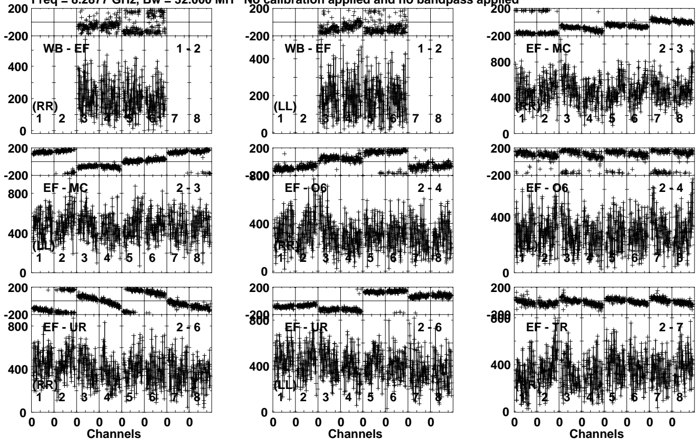
Lower frame: Micro Ampl Jy Top frame: Phas deg Vector averaged cross-power spectrum Several baselines displayed Timerange: 00/20:12:51 to 00/20:15:49
