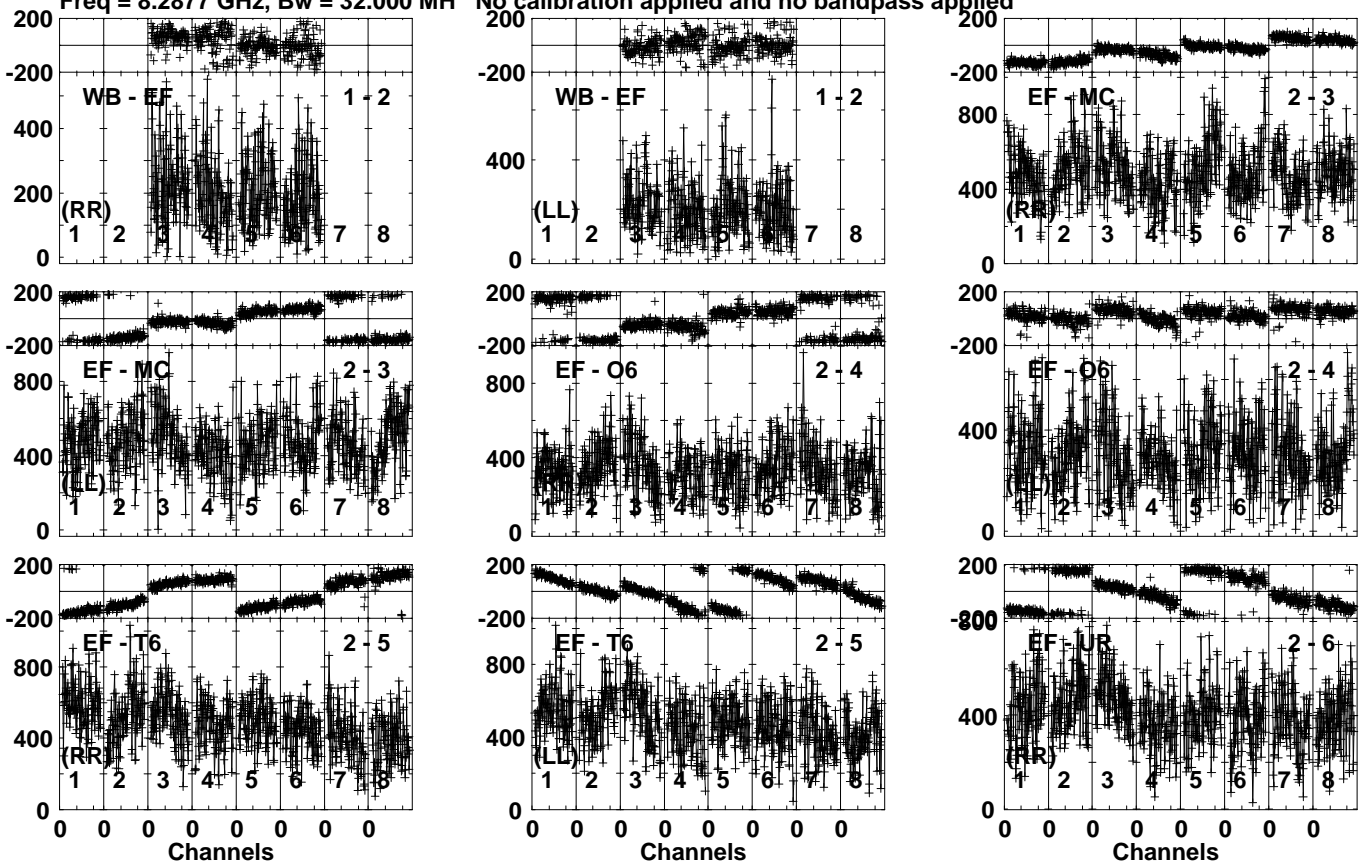
Lower frame: Micro Ampl Jy Top frame: Phas deg Vector averaged cross-power spectrum Several baselines displayed Timerange: 00/18:58:01 to 00/19:00:49
