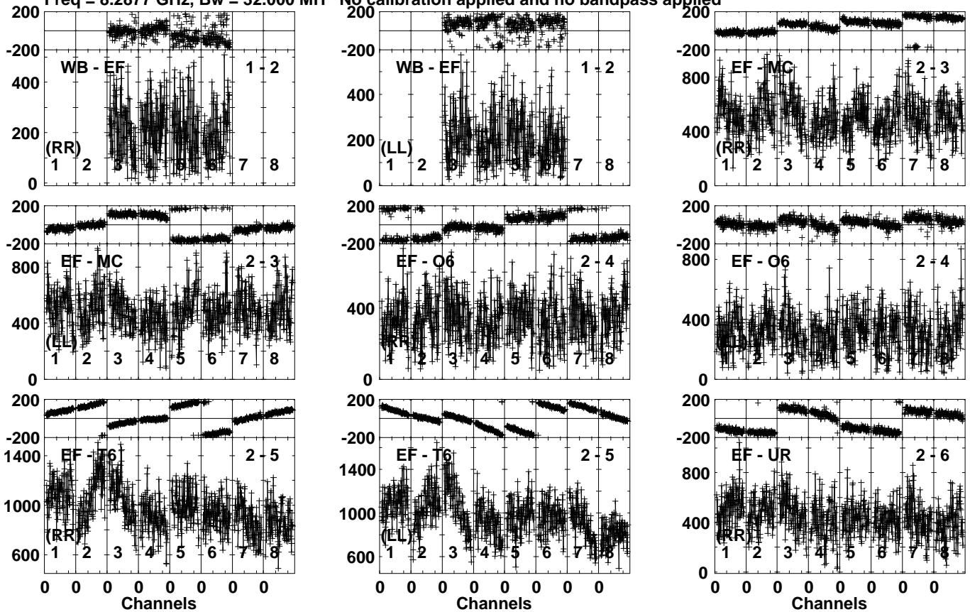
Lower frame: Micro Ampl Jy Top frame: Phas deg Vector averaged cross-power spectrum Several baselines displayed Timerange: 00/15:52:21 to 00/15:55:19
