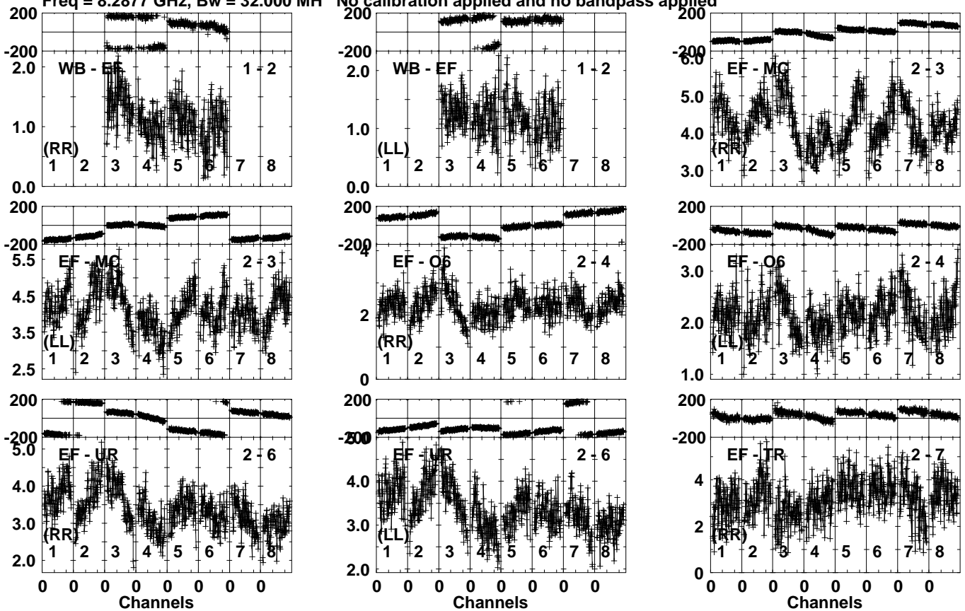
Lower frame: Milli Ampl Jy Top frame: Phas deg Vector averaged cross-power spectrum Several baselines displayed Timerange: 00/20:23:41 to 00/20:24:39
