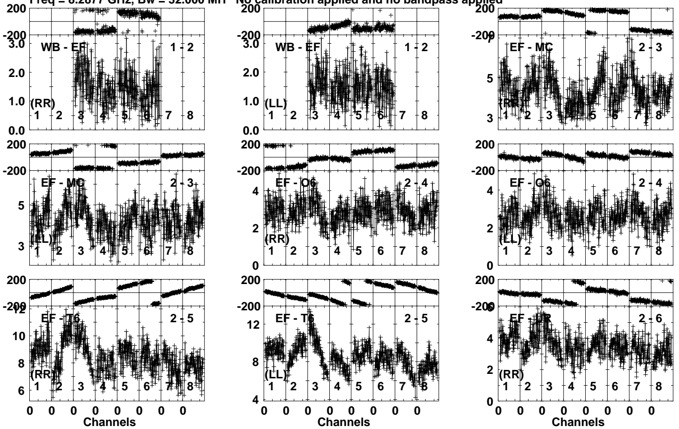
Lower frame: Milli Ampl Jy Top frame: Phas deg Vector averaged cross-power spectrum Several baselines displayed Timerange: 00/15:27:41 to 00/15:28:39
