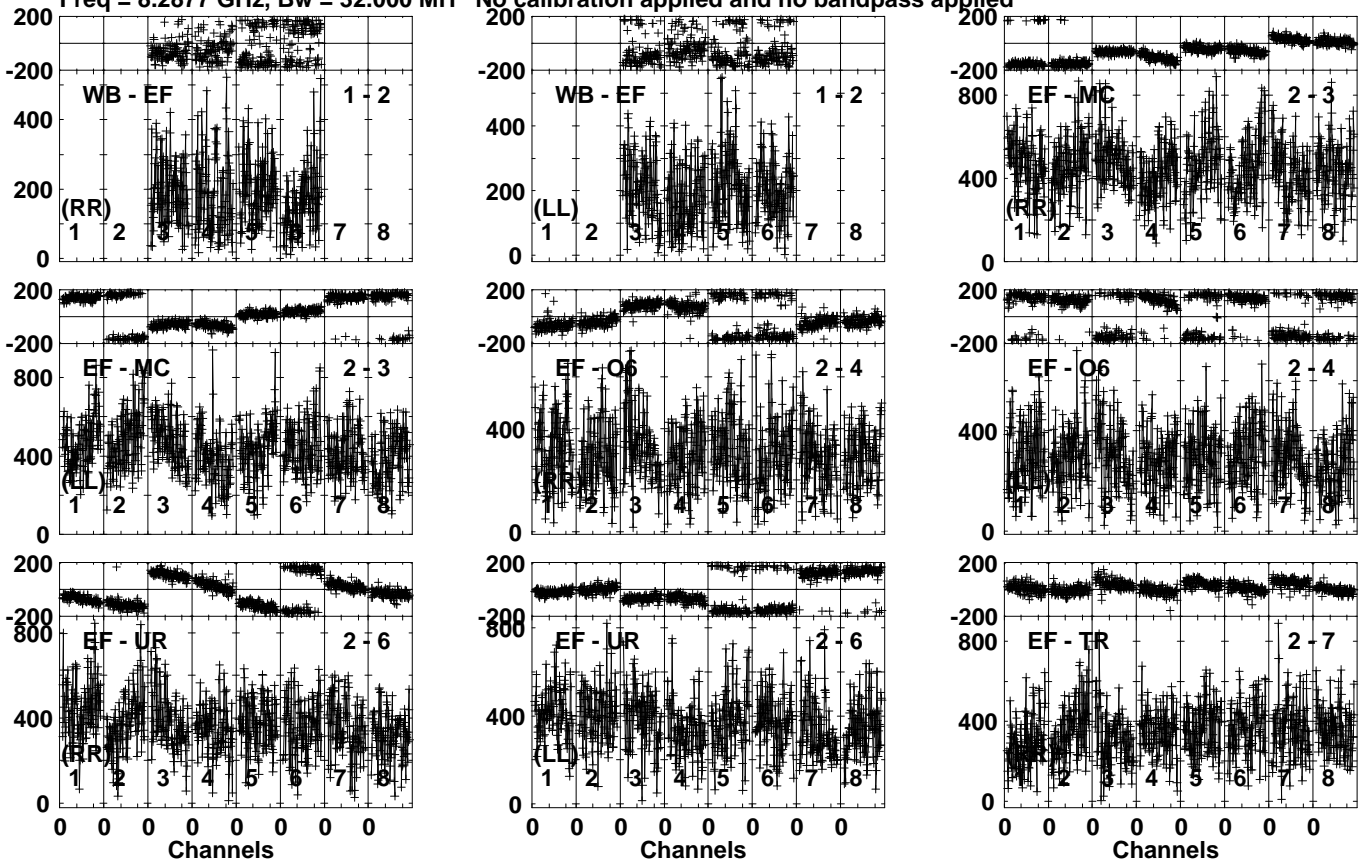
Lower frame: Micro Ampl Jy Top frame: Phas deg Vector averaged cross-power spectrum Several baselines displayed Timerange: 00/20:09:01 to 00/20:11:49
