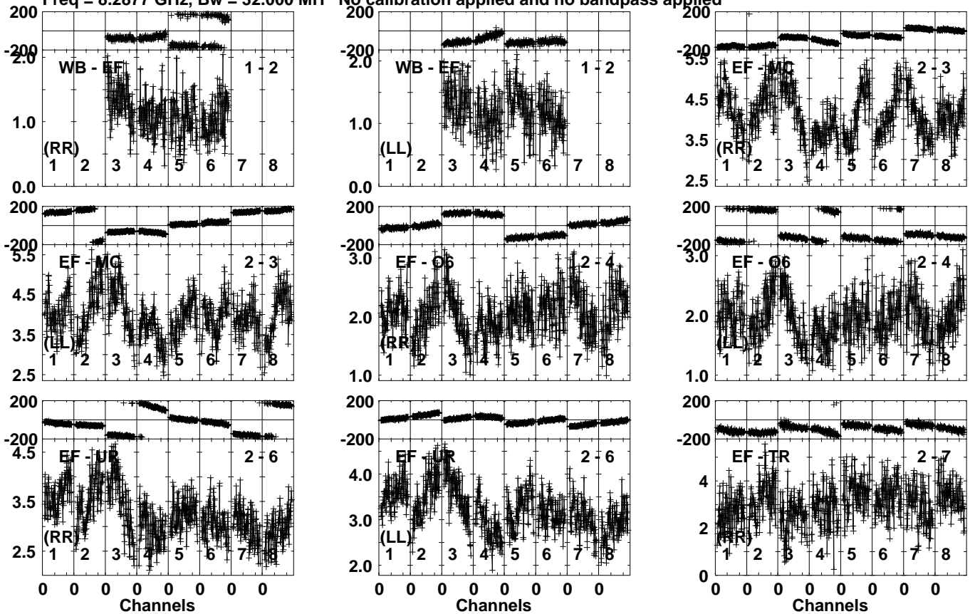
Lower frame: Milli Ampl Jy Top frame: Phas deg Vector averaged cross-power spectrum Several baselines displayed Timerange: 00/20:35:31 to 00/20:36:29
