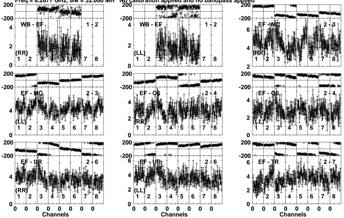
Lower frame: Milli Ampl Jy Top frame: Phas deg Vector averaged cross-power spectrum Several baselines displayed Timerange: 00/15:55:23 to 00/15:56:19
