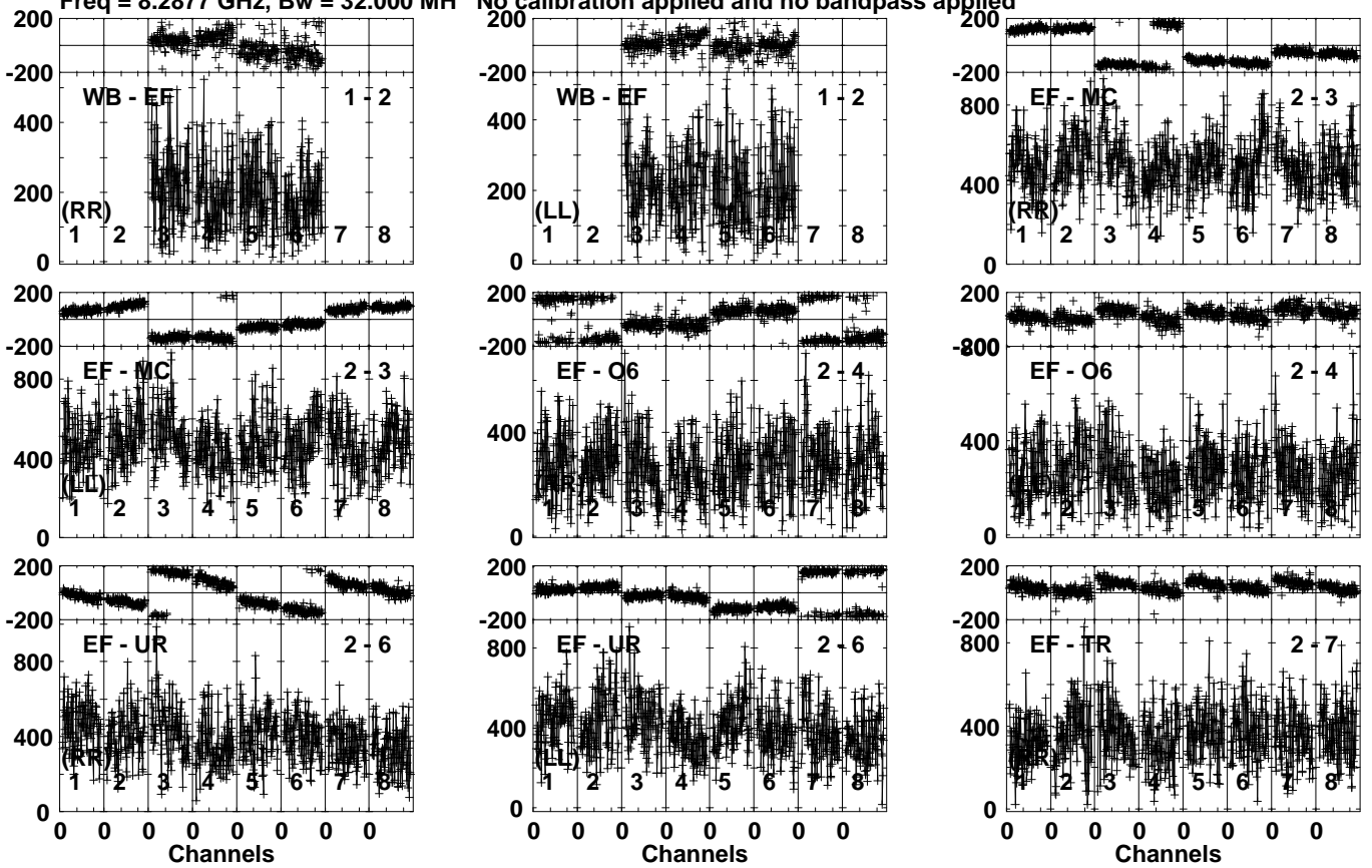
Lower frame: Micro Ampl Jy Top frame: Phas deg Vector averaged cross-power spectrum Several baselines displayed Timerange: 00/20:24:41 to 00/20:27:39
