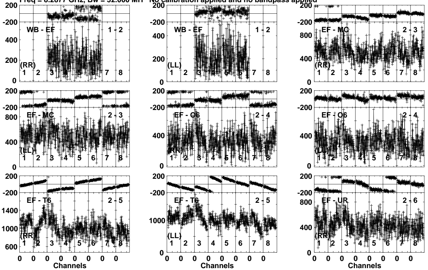
Lower frame: Micro Ampl Jy Top frame: Phas deg Vector averaged cross-power spectrum Several baselines displayed Timerange: 00/16:20:31 to 00/16:22:59
