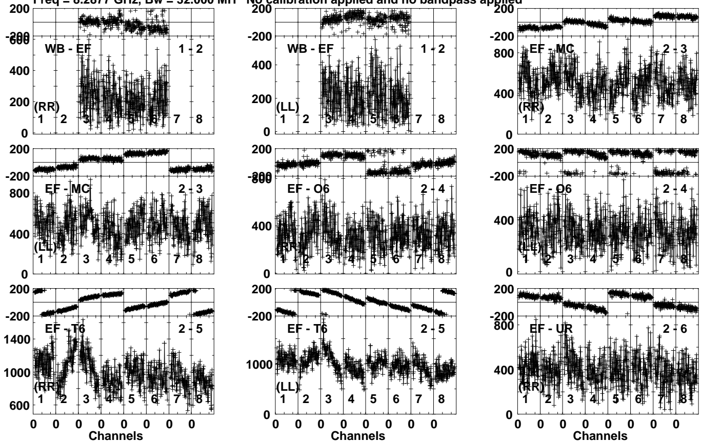
Lower frame: Micro Ampl Jy Top frame: Phas deg Vector averaged cross-power spectrum Several baselines displayed Timerange: 00/15:13:01 to 00/15:15:49
