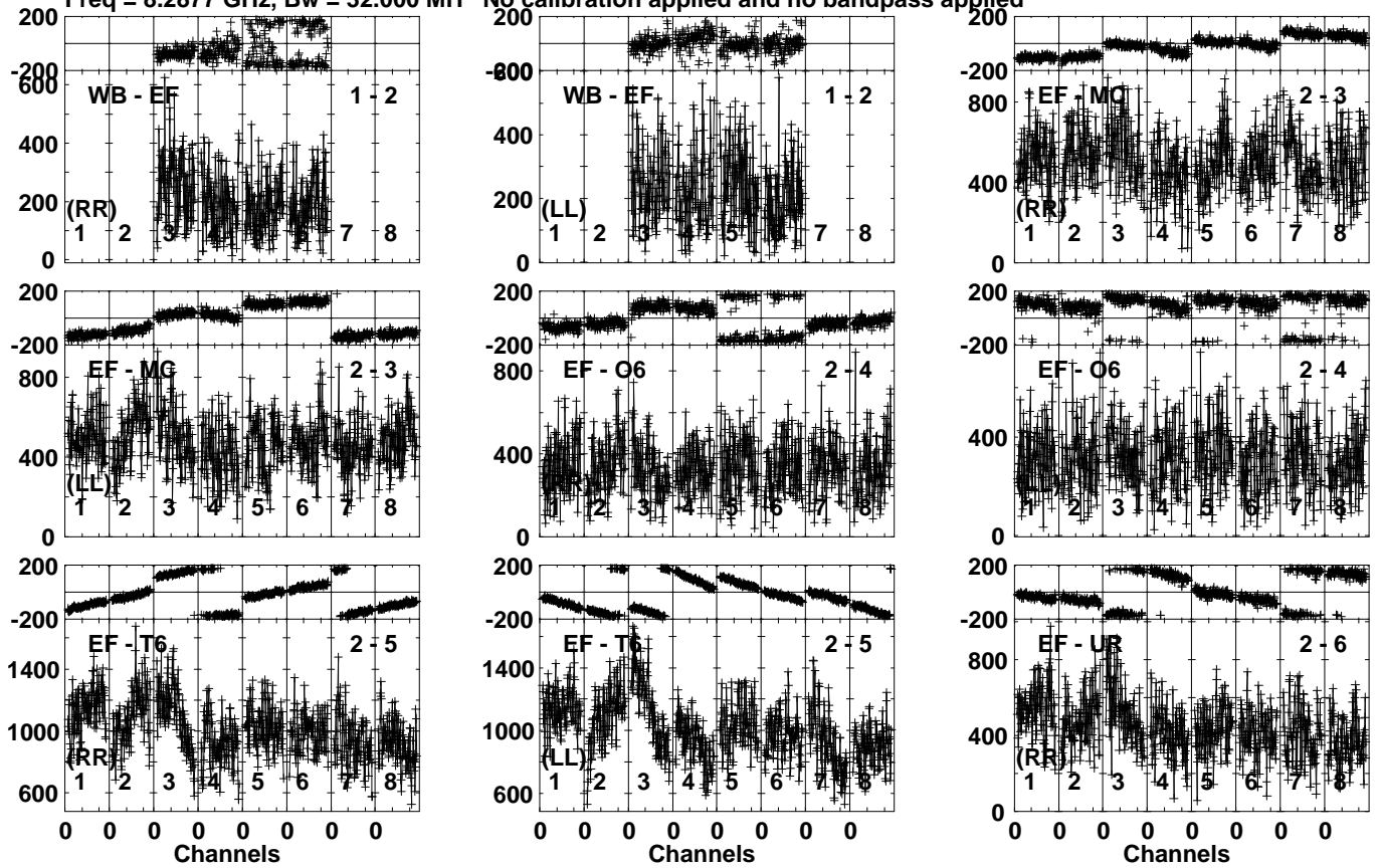
Lower frame: Micro Ampl Jy Top frame: Phas deg Vector averaged cross-power spectrum Several baselines displayed Timerange: 00/15:40:31 to 00/15:43:29
