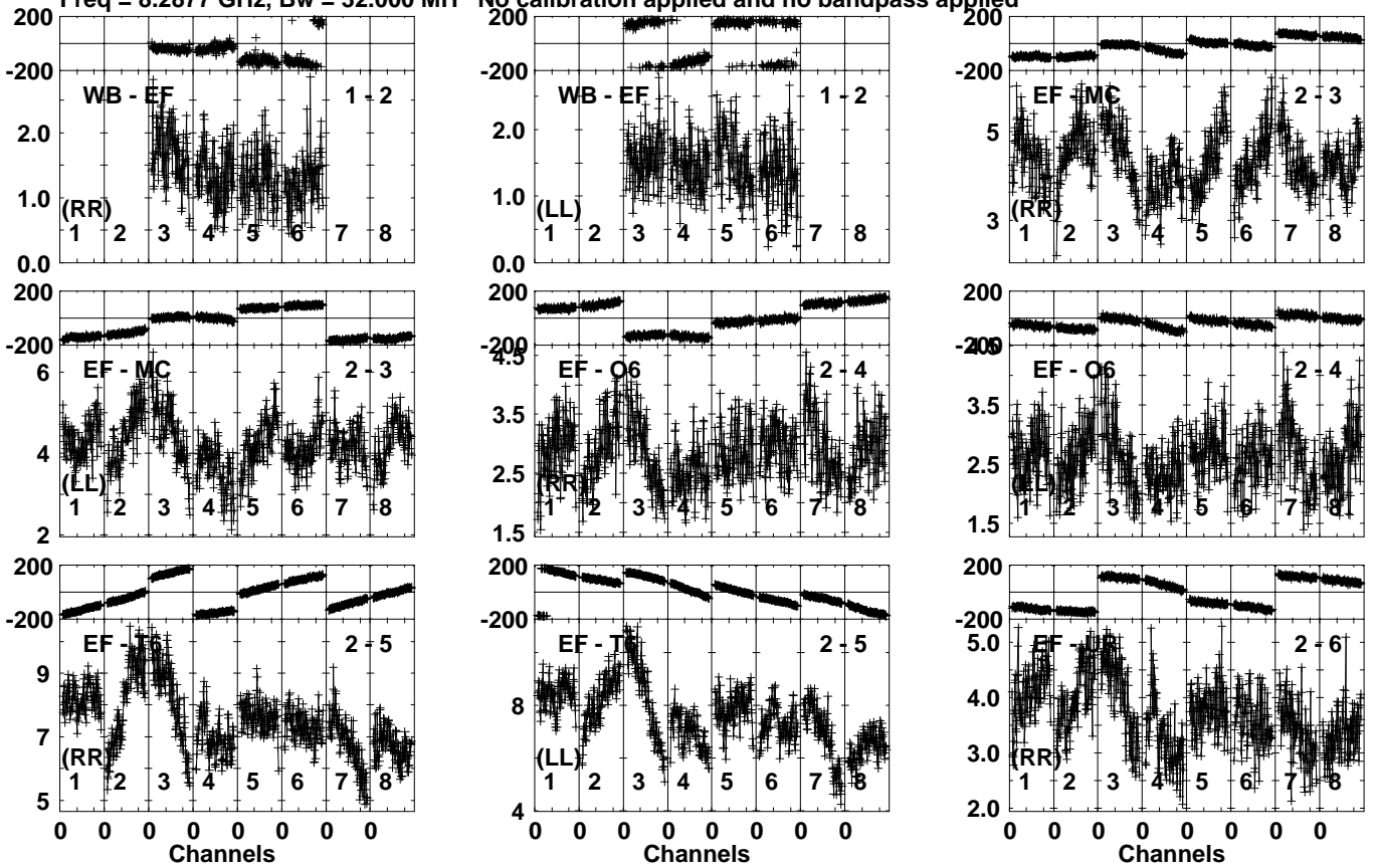
Lower frame: Milli Ampl Jy Top frame: Phas deg Vector averaged cross-power spectrum Several baselines displayed Timerange: 00/17:57:43 to 00/17:58:39
