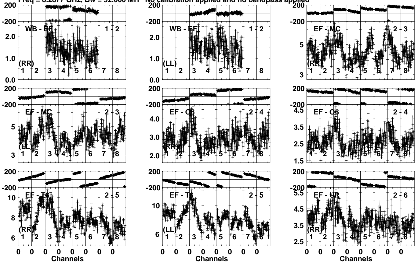
Lower frame: Milli Ampl Jy Top frame: Phas deg Vector averaged cross-power spectrum Several baselines displayed Timerange: 00/17:41:53 to 00/17:42:49
