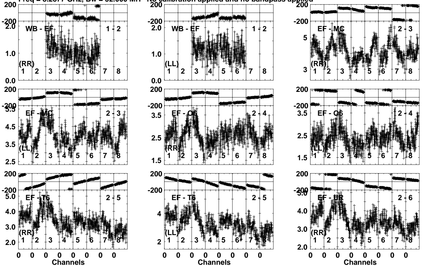
Lower frame: Milli Ampl Jy Top frame: Phas deg Vector averaged cross-power spectrum Several baselines displayed Timerange: 00/19:16:43 to 00/19:17:39
