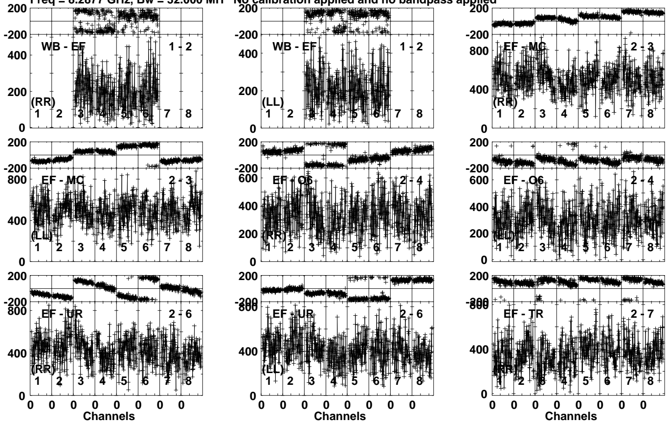
Lower frame: Micro Ampl Jy Top frame: Phas deg Vector averaged cross-power spectrum Several baselines displayed Timerange: 00/19:49:11 to 00/19:52:09
