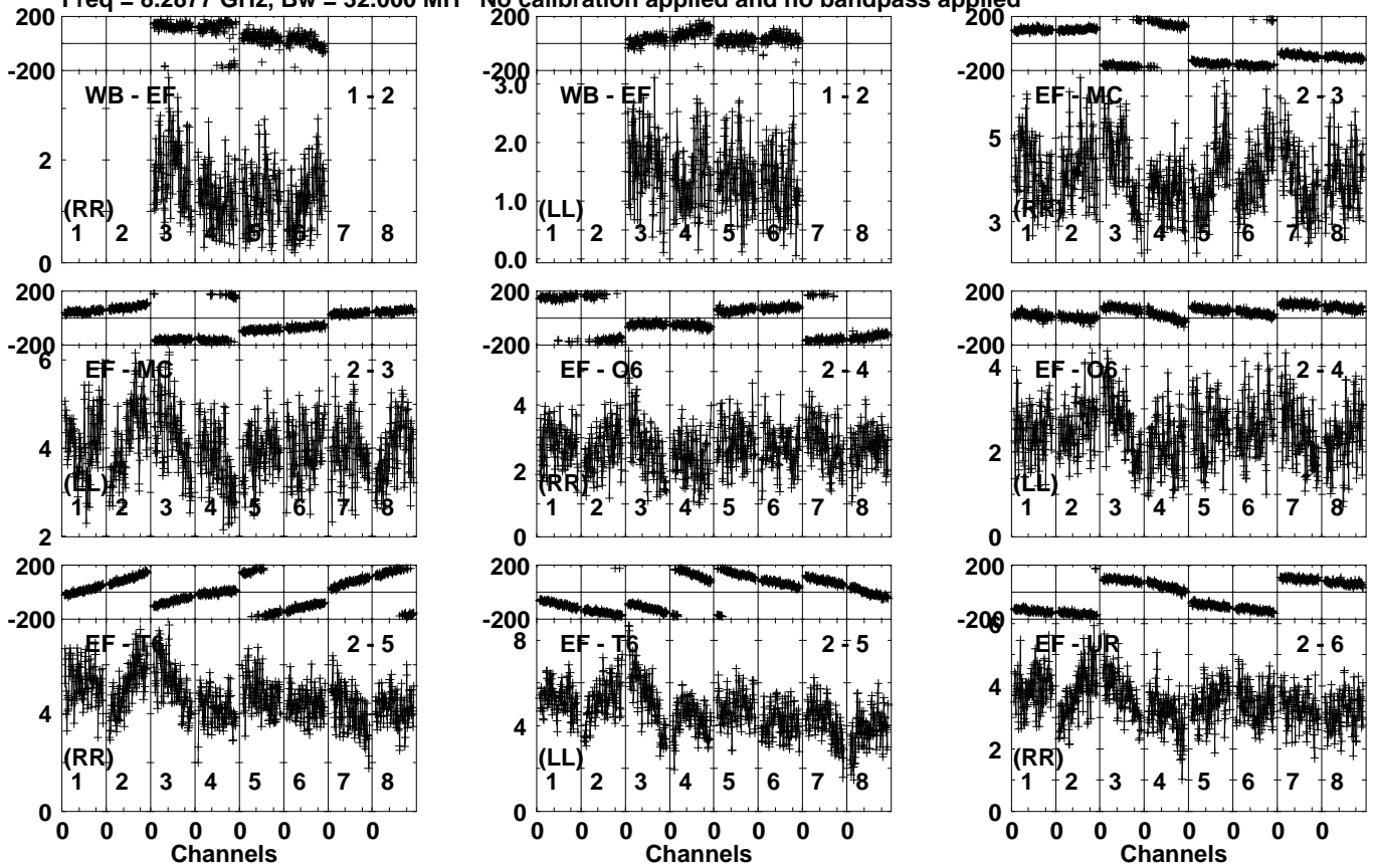
Lower frame: Milli Ampl Jy Top frame: Phas deg Vector averaged cross-power spectrum Several baselines displayed Timerange: 00/18:57:03 to 00/18:57:59
