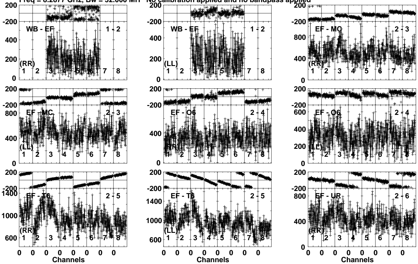
Lower frame: Micro Ampl Jy Top frame: Phas deg Vector averaged cross-power spectrum Several baselines displayed Timerange: 00/16:16:01 to 00/16:18:59
