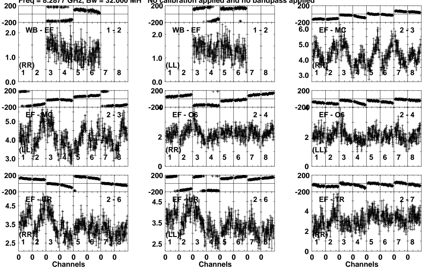
Lower frame: Milli Ampl Jy Top frame: Phas deg Vector averaged cross-power spectrum Several baselines displayed Timerange: 00/20:27:43 to 00/20:28:39
