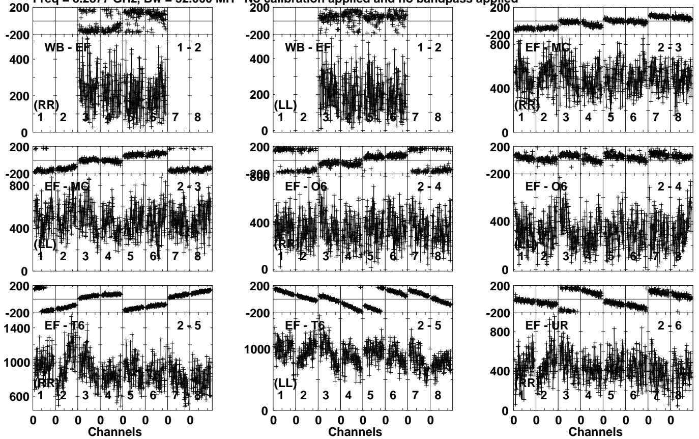
Lower frame: Micro Ampl Jy Top frame: Phas deg Vector averaged cross-power spectrum Several baselines displayed Timerange: 00/17:50:41 to 00/17:53:39
