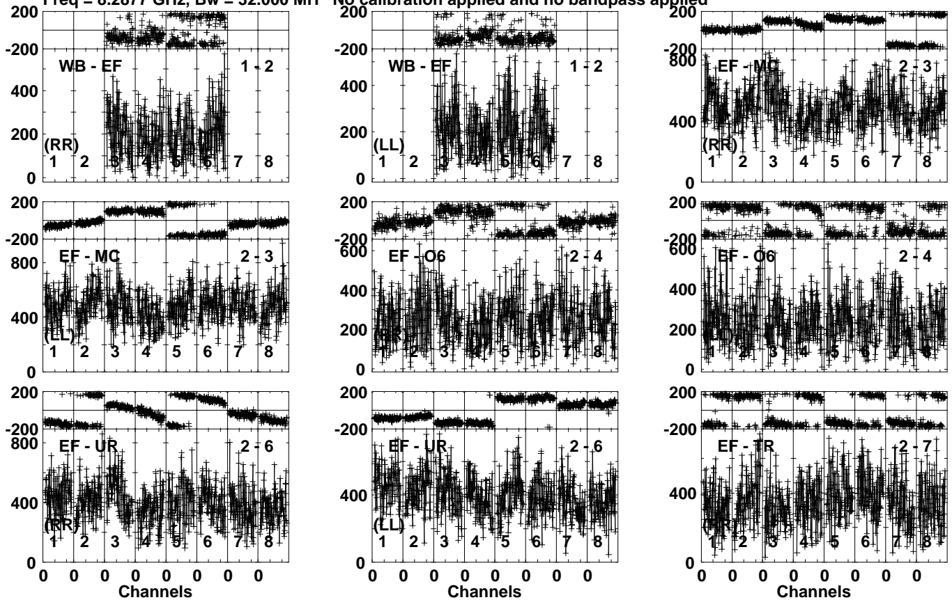
Lower frame: Micro Ampl Jy Top frame: Phas deg Vector averaged cross-power spectrum Several baselines displayed Timerange: 00/20:48:21 to 00/20:51:19
