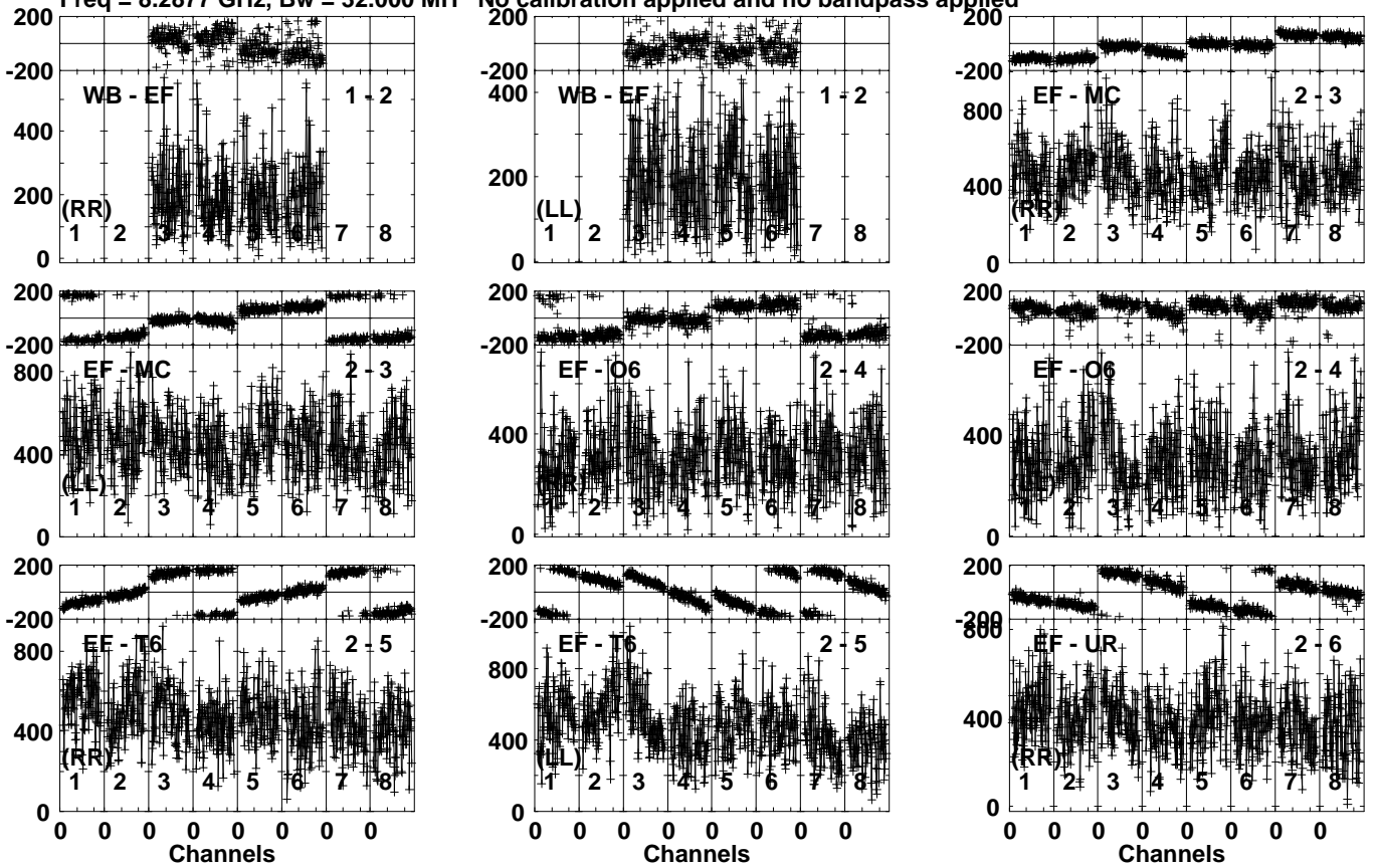
Lower frame: Micro Ampl Jy Top frame: Phas deg Vector averaged cross-power spectrum Several baselines displayed Timerange: 00/18:54:31 to 00/18:56:59
