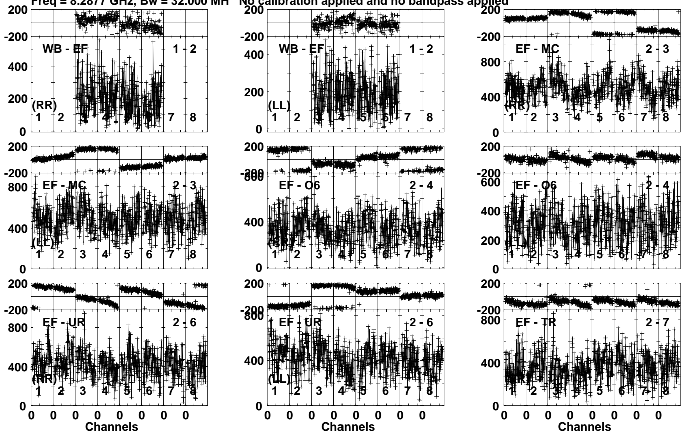
Lower frame: Micro Ampl Jy Top frame: Phas deg Vector averaged cross-power spectrum Several baselines displayed Timerange: 00/19:37:21 to 00/19:40:19
