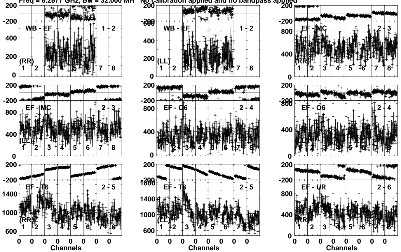
Lower frame: Micro Ampl Jy Top frame: Phas deg Vector averaged cross-power spectrum Several baselines displayed Timerange: 00/16:24:01 to 00/16:26:49
