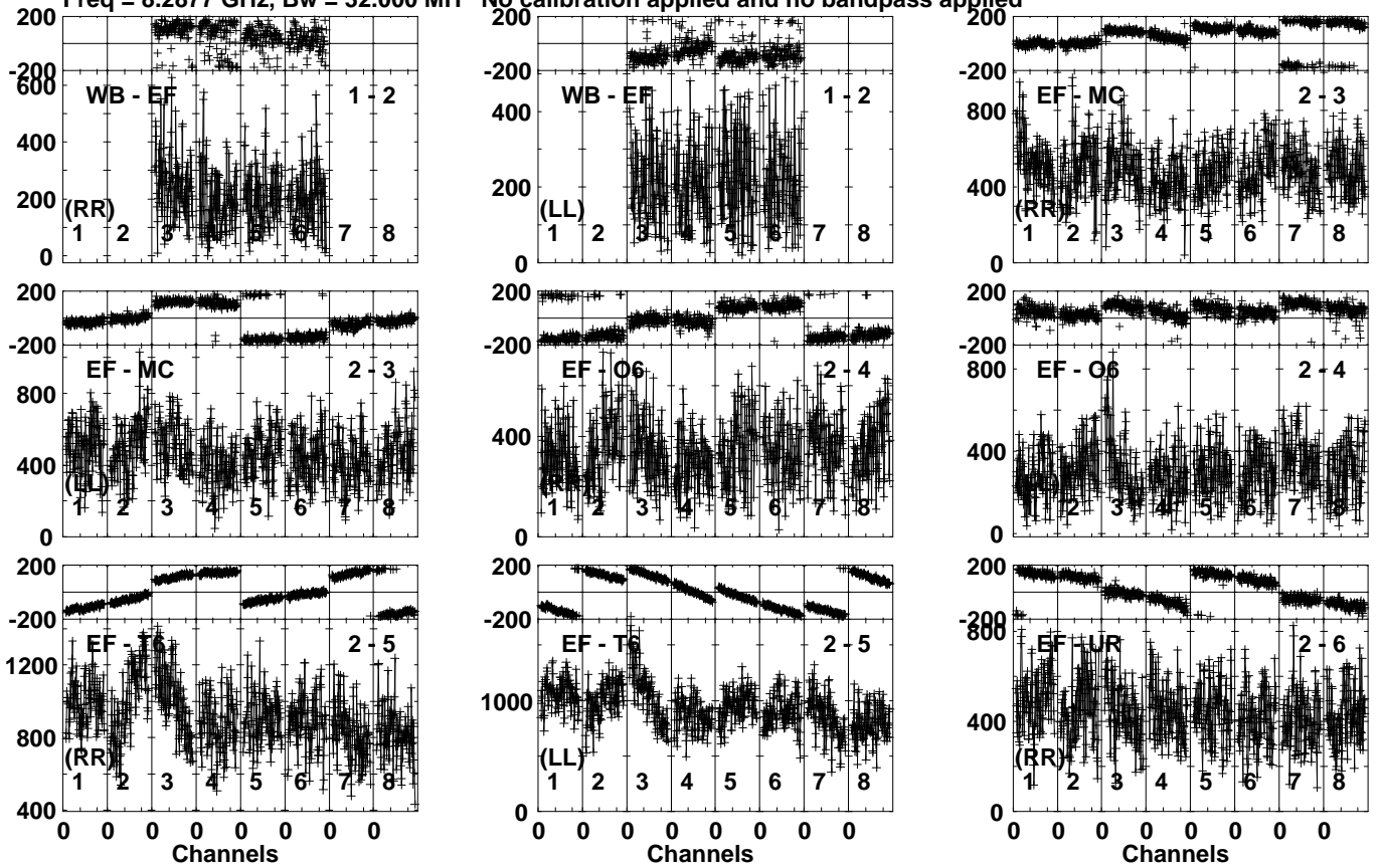
Lower frame: Micro Ampl Jy Top frame: Phas deg Vector averaged cross-power spectrum Several baselines displayed Timerange: 00/16:47:41 to 00/16:50:29
