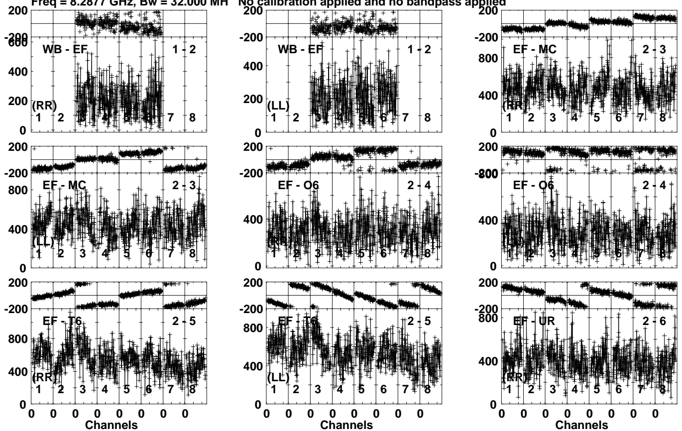
Lower frame: Micro Ampl Jy Top frame: Phas deg Vector averaged cross-power spectrum Several baselines displayed Timerange: 00/18:50:01 to 00/18:52:59
