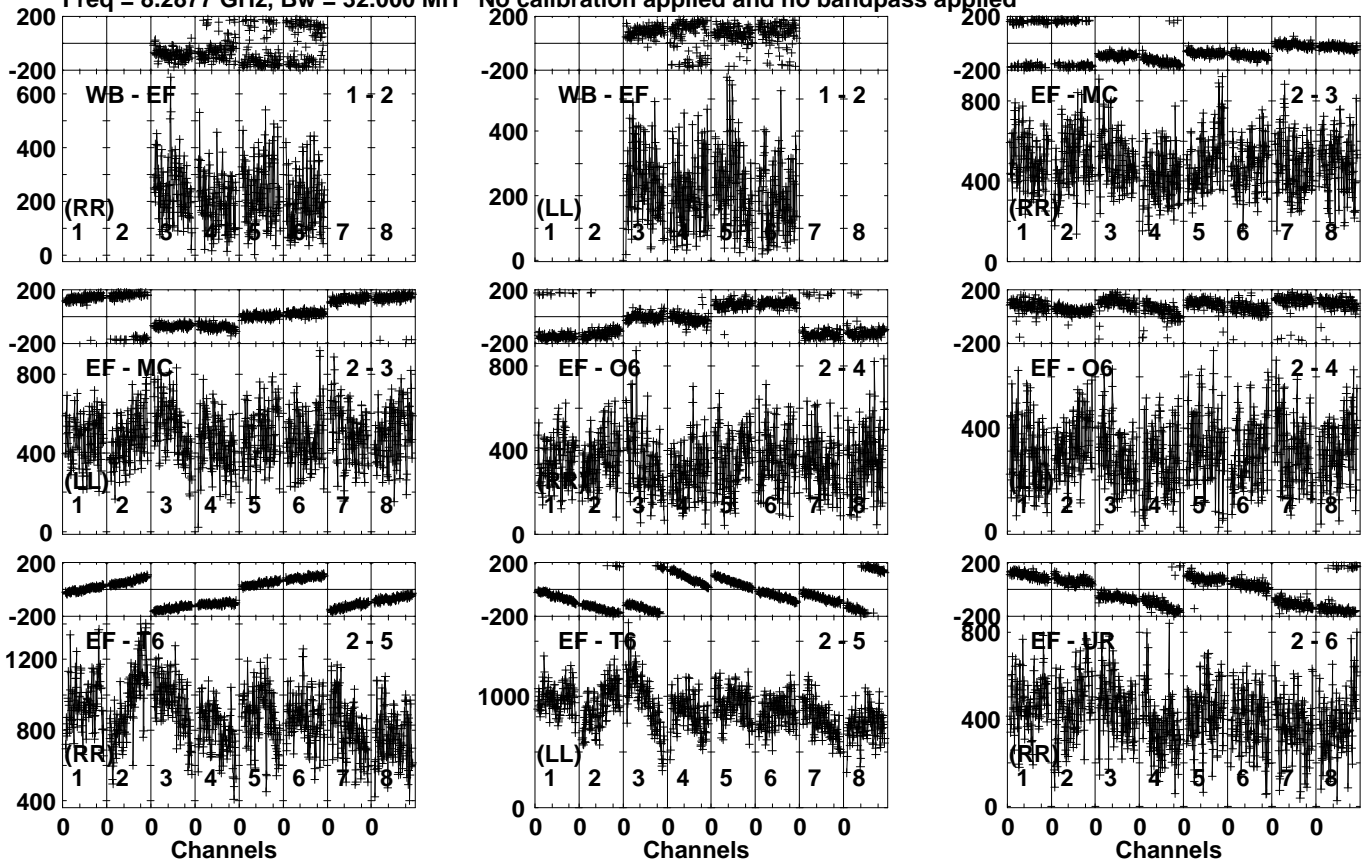
Lower frame: Micro Ampl Jy Top frame: Phas deg Vector averaged cross-power spectrum Several baselines displayed Timerange: 00/17:19:41 to 00/17:22:09
