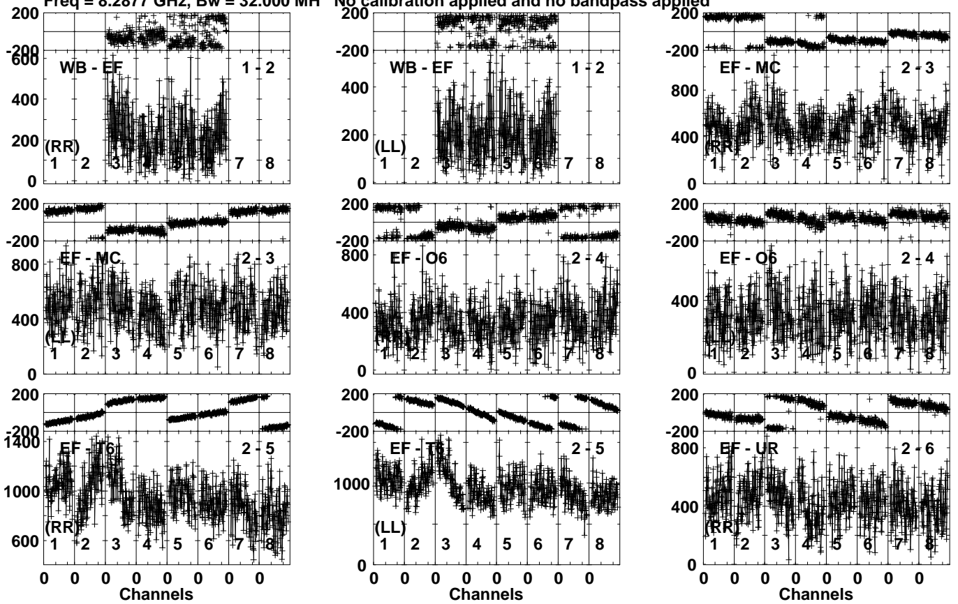
Lower frame: Micro Ampl Jy Top frame: Phas deg Vector averaged cross-power spectrum Several baselines displayed Timerange: 00/17:23:11 to 00/17:25:59
