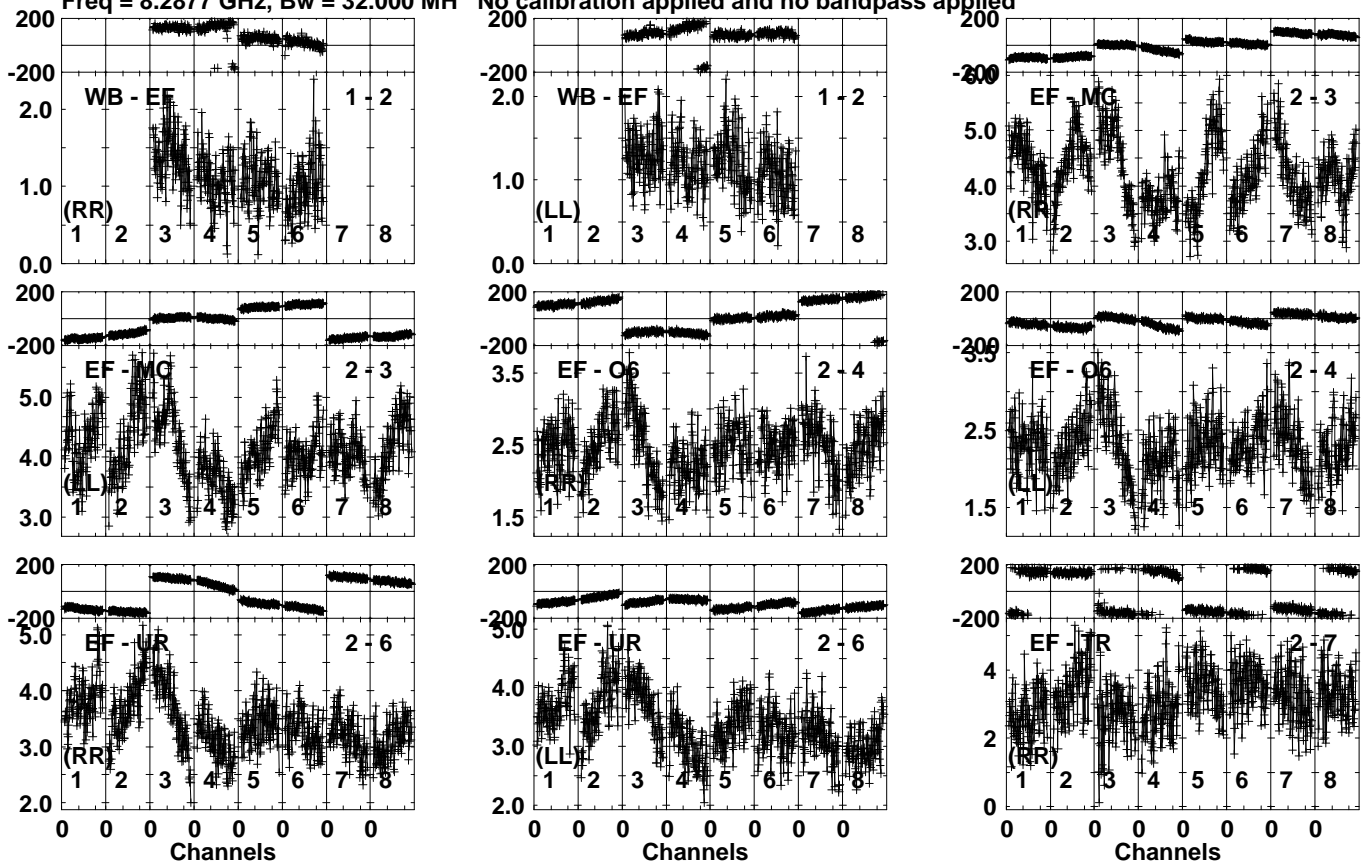
Lower frame: Milli Ampl Jy Top frame: Phas deg Vector averaged cross-power spectrum Several baselines displayed Timerange: 00/20:19:53 to 00/20:20:49
