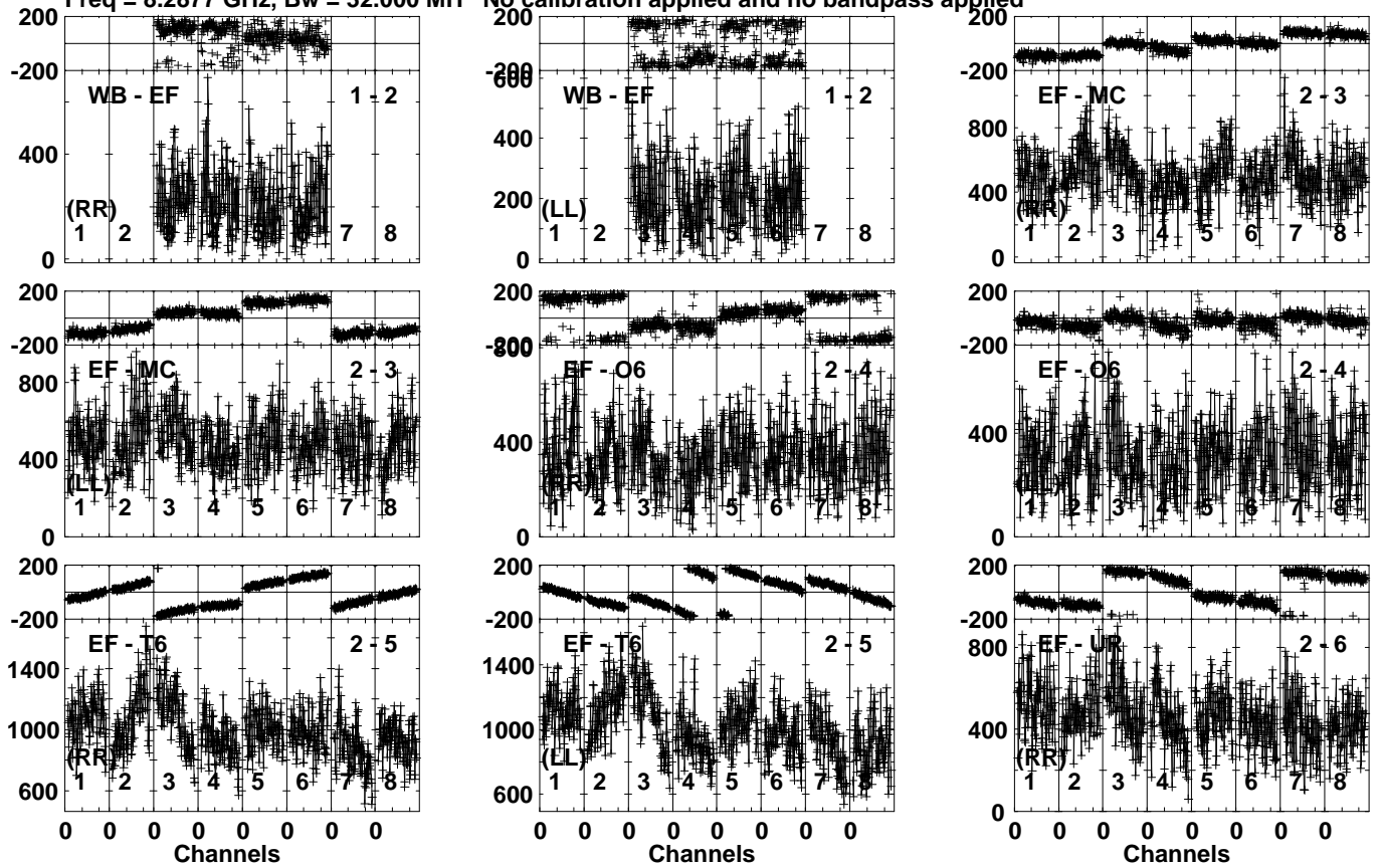
Lower frame: Micro Ampl Jy Top frame: Phas deg Vector averaged cross-power spectrum Several baselines displayed Timerange: 00/15:24:51 to 00/15:27:39
