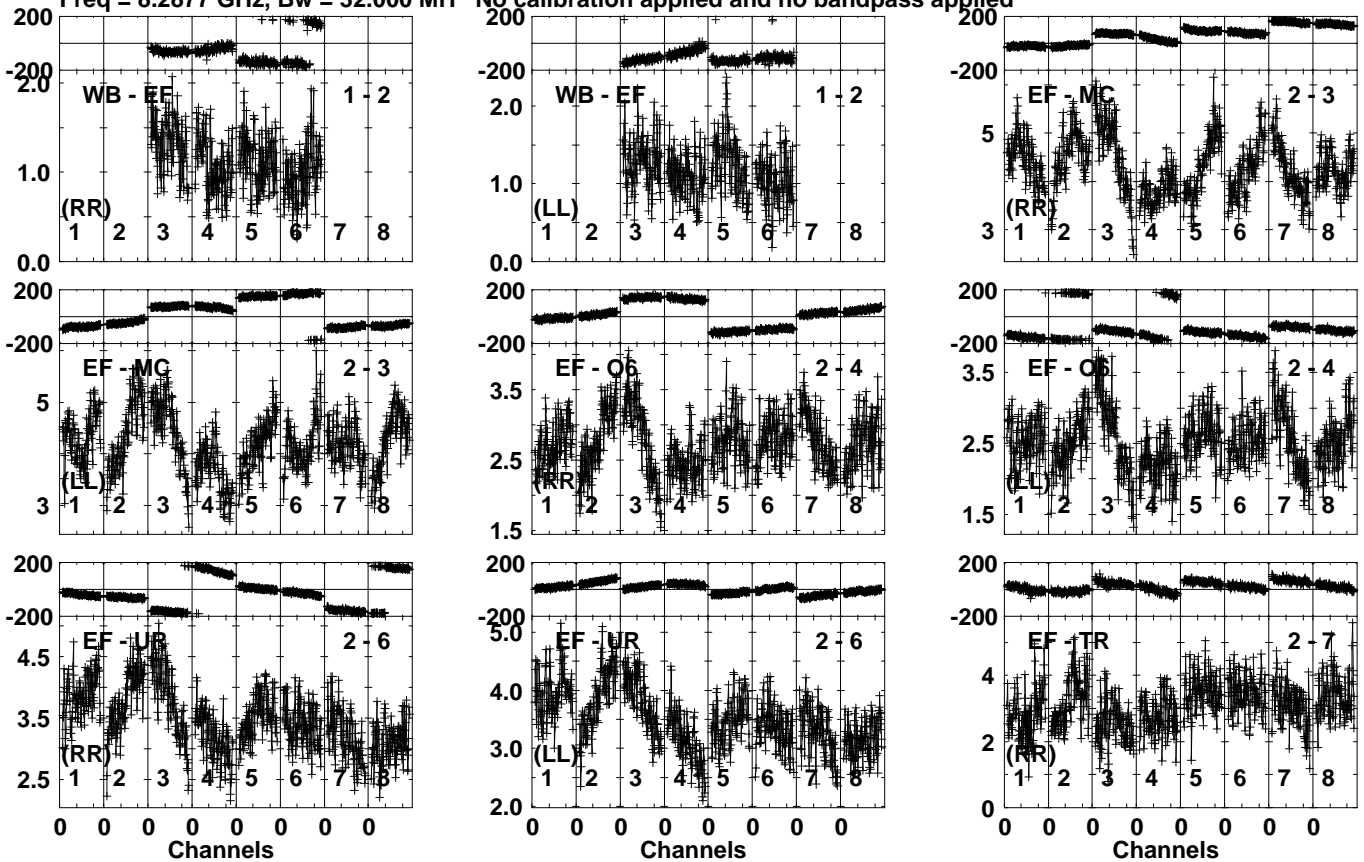
Lower frame: Milli Ampl Jy Top frame: Phas deg Vector averaged cross-power spectrum Several baselines displayed Timerange: 00/19:52:13 to 00/19:53:09
