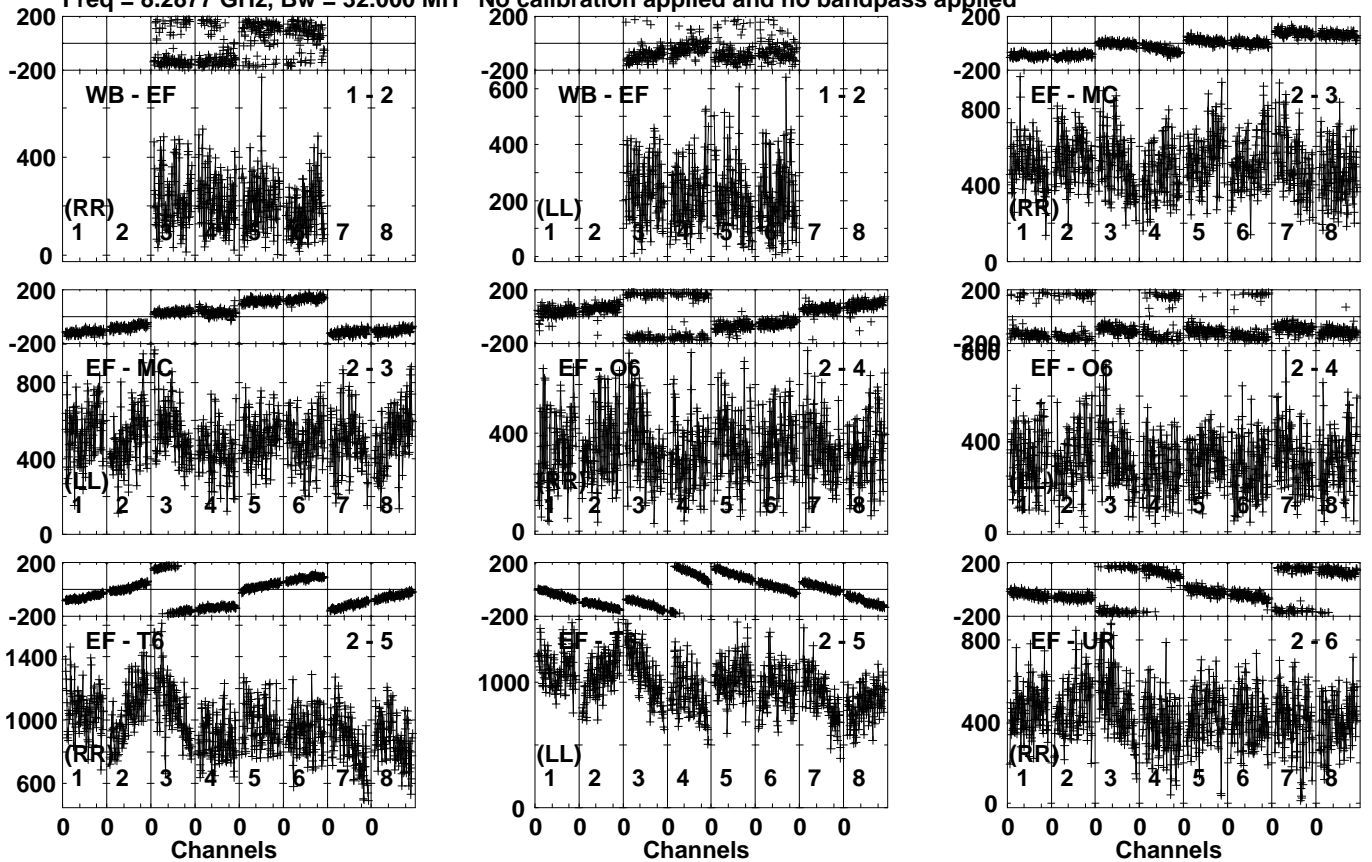
Lower frame: Micro Ampl Jy Top frame: Phas deg Vector averaged cross-power spectrum Several baselines displayed Timerange: 00/15:33:11 to 00/15:35:39
