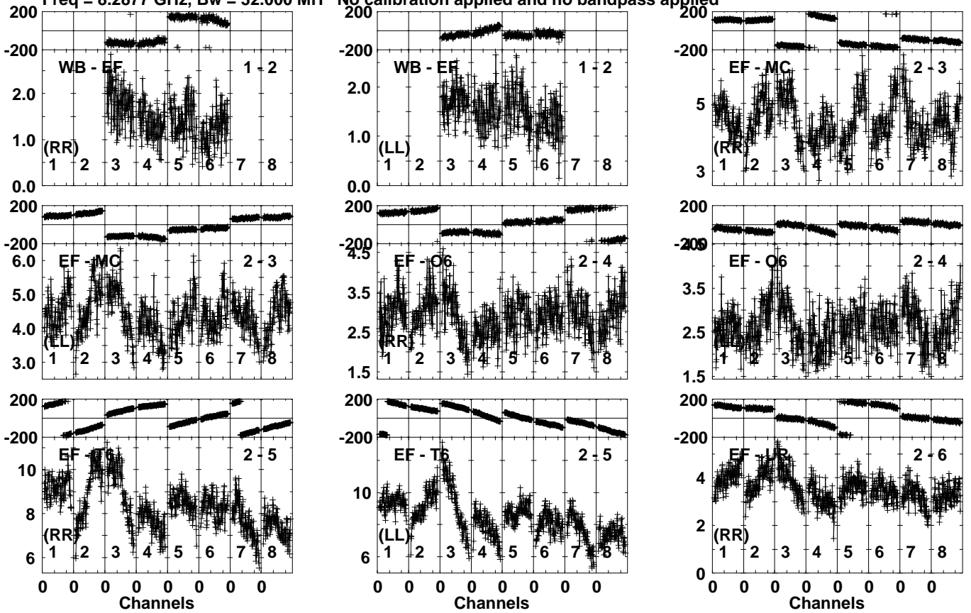
Lower frame: Milli Ampl Jy Top frame: Phas deg Vector averaged cross-power spectrum Several baselines displayed Timerange: 00/16:11:13 to 00/16:12:09
