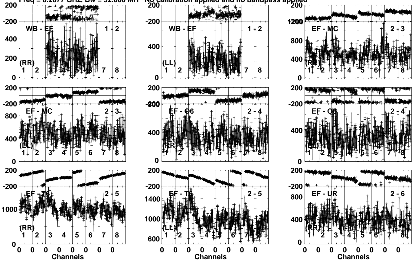
Lower frame: Micro Ampl Jy Top frame: Phas deg Vector averaged cross-power spectrum Several baselines displayed Timerange: 00/15:36:41 to 00/15:39:29
