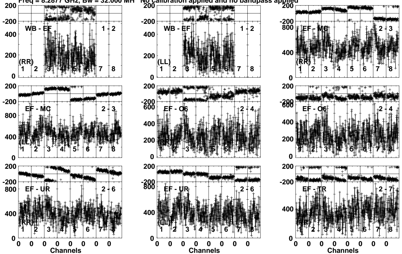
Lower frame: Micro Ampl Jy Top frame: Phas deg Vector averaged cross-power spectrum Several baselines displayed Timerange: 00/20:41:01 to 00/20:43:29
