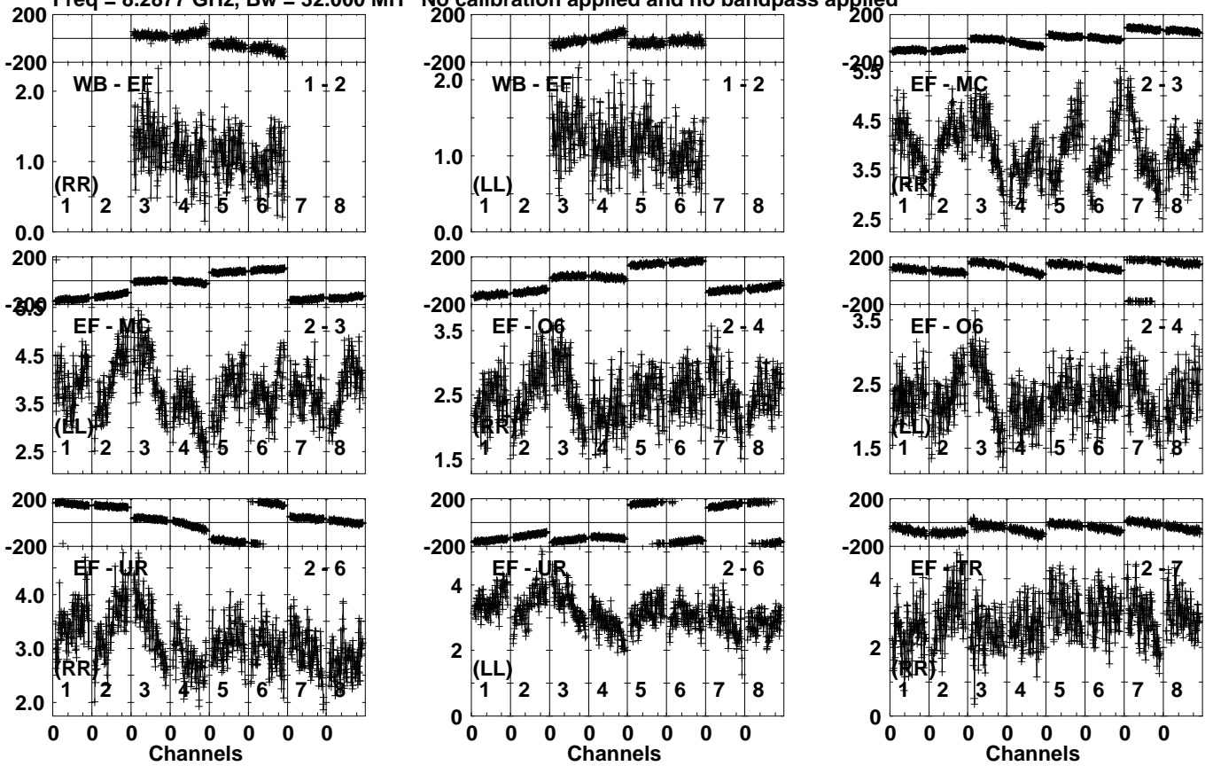
Lower frame: Milli Ampl Jy Top frame: Phas deg Vector averaged cross-power spectrum Several baselines displayed Timerange: 00/20:04:03 to 00/20:04:59
