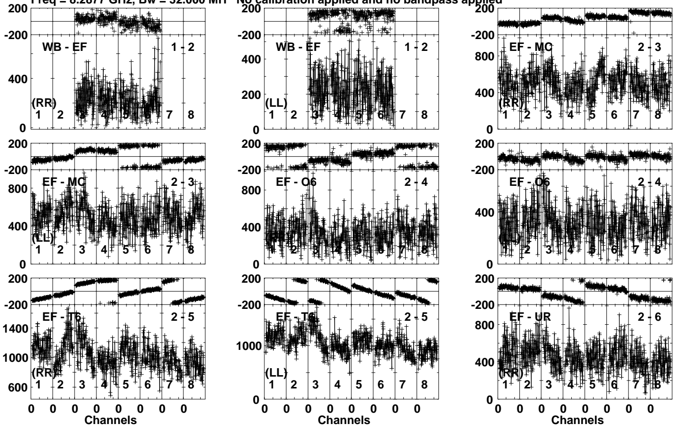
Lower frame: Micro Ampl Jy Top frame: Phas deg Vector averaged cross-power spectrum Several baselines displayed Timerange: 00/15:56:51 to 00/15:59:19
