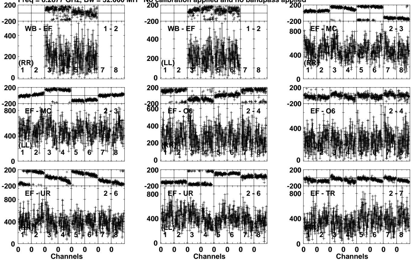
Lower frame: Micro Ampl Jy Top frame: Phas deg Vector averaged cross-power spectrum Several baselines displayed Timerange: 00/20:32:41 to 00/20:35:29
