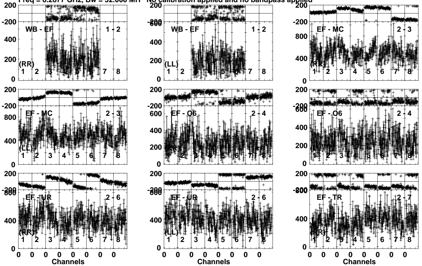
Lower frame: Micro Ampl Jy Top frame: Phas deg Vector averaged cross-power spectrum Several baselines displayed Timerange: 00/20:44:31 to 00/20:47:19
