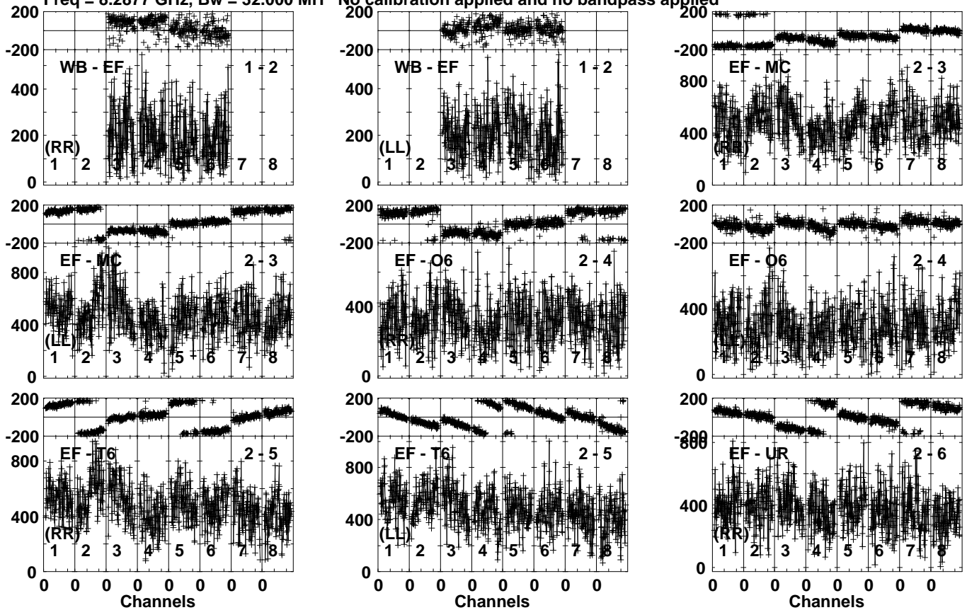
Lower frame: Micro Ampl Jy Top frame: Phas deg Vector averaged cross-power spectrum Several baselines displayed Timerange: 00/19:01:51 to 00/19:04:49
