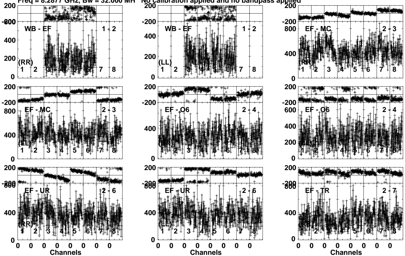
Lower frame: Micro Ampl Jy Top frame: Phas deg Vector averaged cross-power spectrum Several baselines displayed Timerange: 00/19:57:11 to 00/19:59:59
