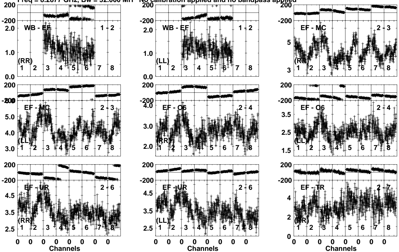
Lower frame: Milli Ampl Jy Top frame: Phas deg Vector averaged cross-power spectrum Several baselines displayed Timerange: 00/19:48:11 to 00/19:49:09
