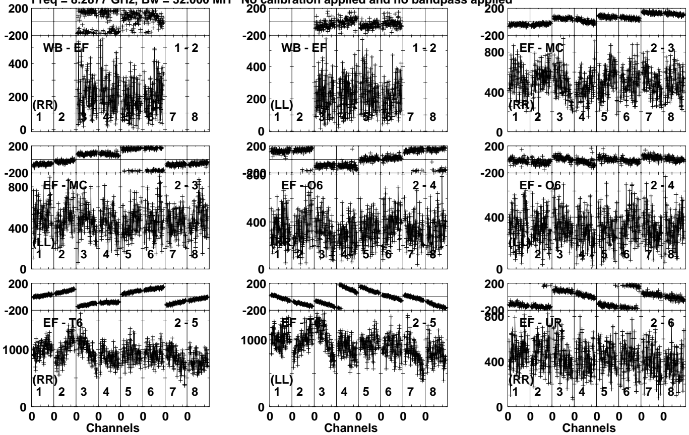
Lower frame: Micro Ampl Jy Top frame: Phas deg Vector averaged cross-power spectrum Several baselines displayed Timerange: 00/16:56:01 to 00/16:58:29
