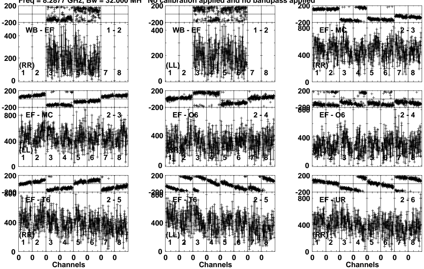
Lower frame: Micro Ampl Jy Top frame: Phas deg Vector averaged cross-power spectrum Several baselines displayed Timerange: 00/19:13:41 to 00/19:16:39
