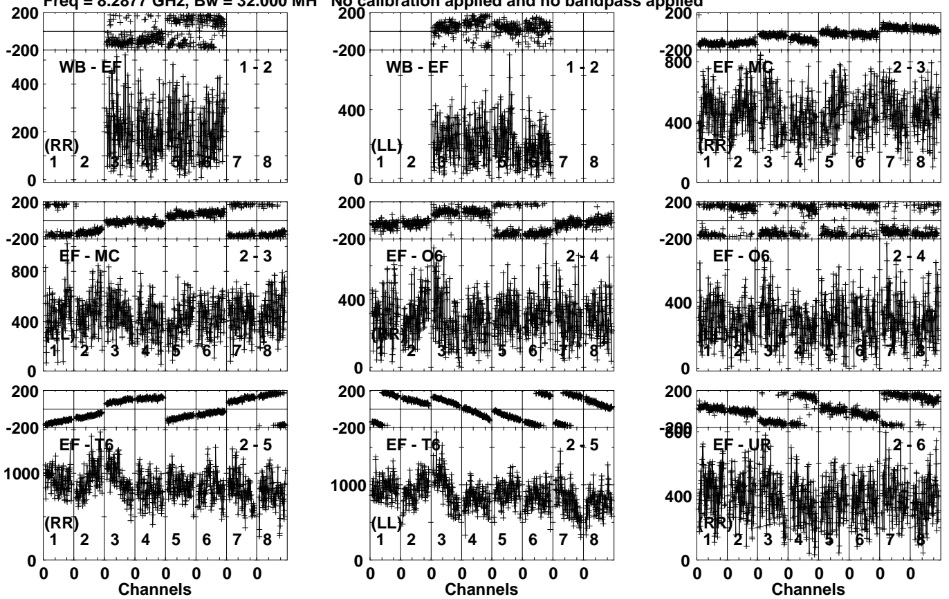
Lower frame: Micro Ampl Jy Top frame: Phas deg Vector averaged cross-power spectrum Several baselines displayed Timerange: 00/17:11:21 to 00/17:14:09
