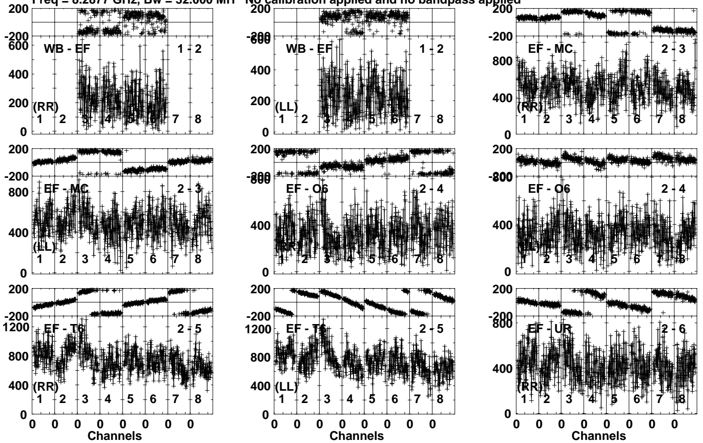
Lower frame: Micro Ampl Jy Top frame: Phas deg Vector averaged cross-power spectrum Several baselines displayed Timerange: 00/18:30:51 to 00/18:33:19
