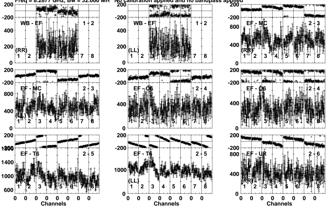
Lower frame: Micro Ampl Jy Top frame: Phas deg Vector averaged cross-power spectrum Several baselines displayed Timerange: 00/16:39:41 to 00/16:42:39
