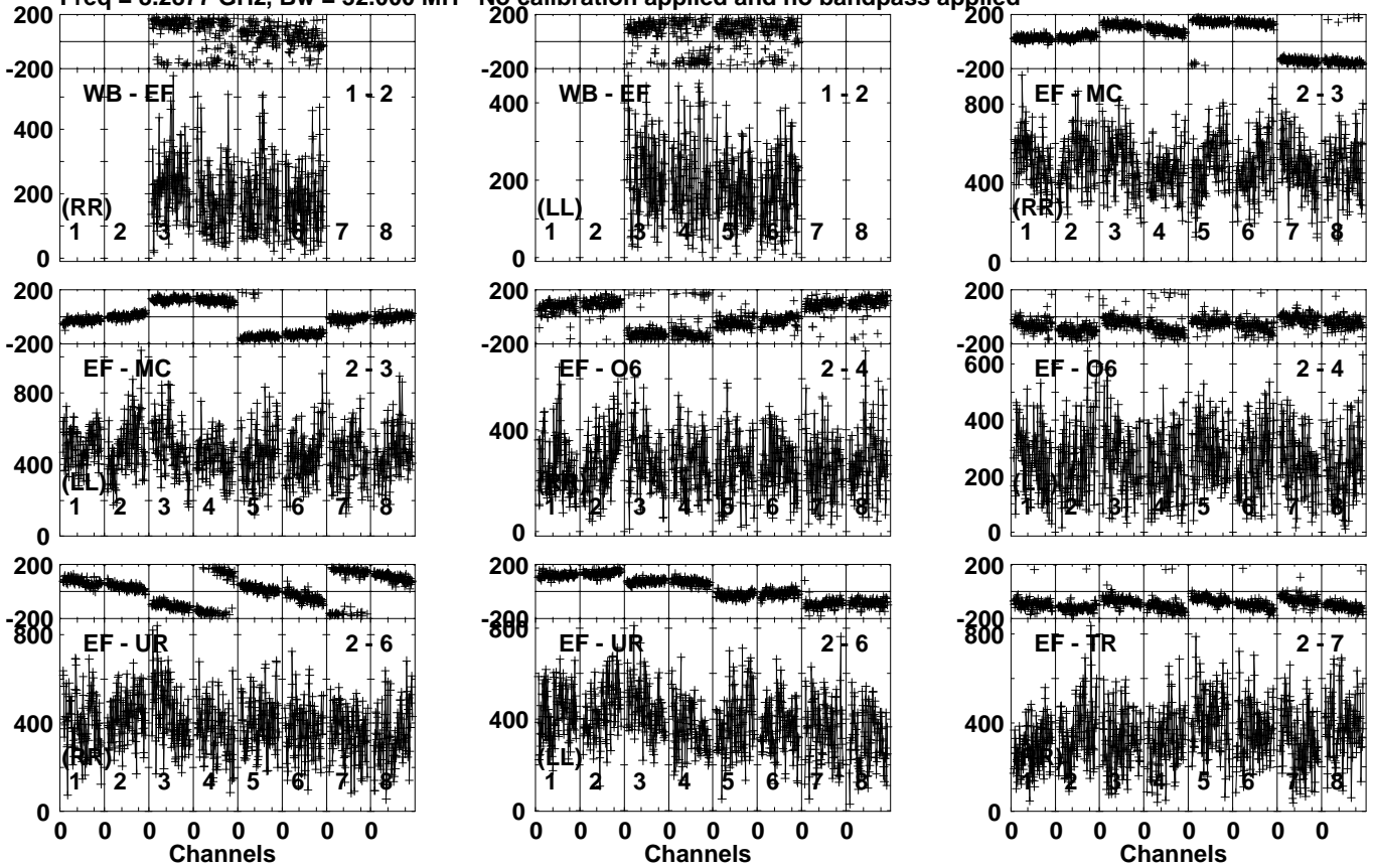
Lower frame: Micro Ampl Jy Top frame: Phas deg Vector averaged cross-power spectrum Several baselines displayed Timerange: 00/20:36:31 to 00/20:39:29
