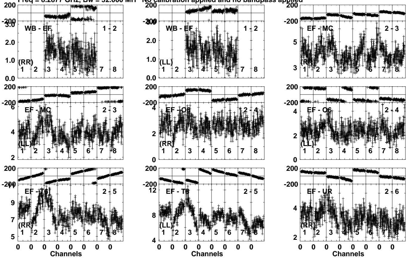
Lower frame: Milli Ampl Jy Top frame: Phas deg Vector averaged cross-power spectrum Several baselines displayed Timerange: 00/17:02:21 to 00/17:03:19
