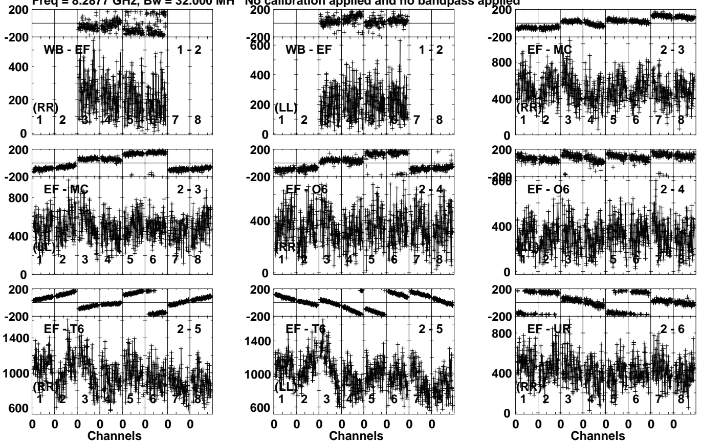
Lower frame: Micro Ampl Jy Top frame: Phas deg Vector averaged cross-power spectrum Several baselines displayed Timerange: 00/15:45:01 to 00/15:47:29
