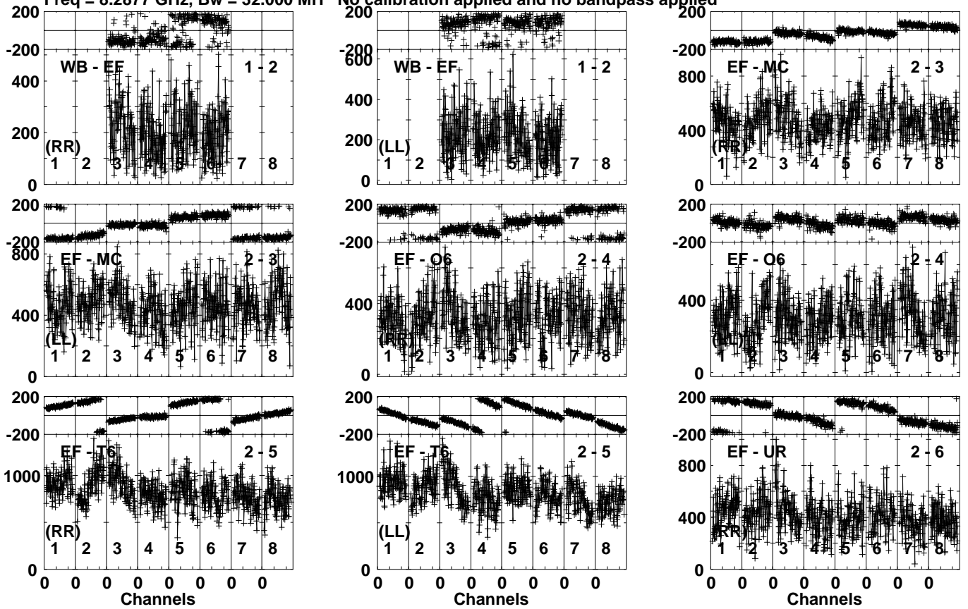
Lower frame: Micro Ampl Jy Top frame: Phas deg Vector averaged cross-power spectrum Several baselines displayed Timerange: 00/17:55:11 to 00/17:57:39
