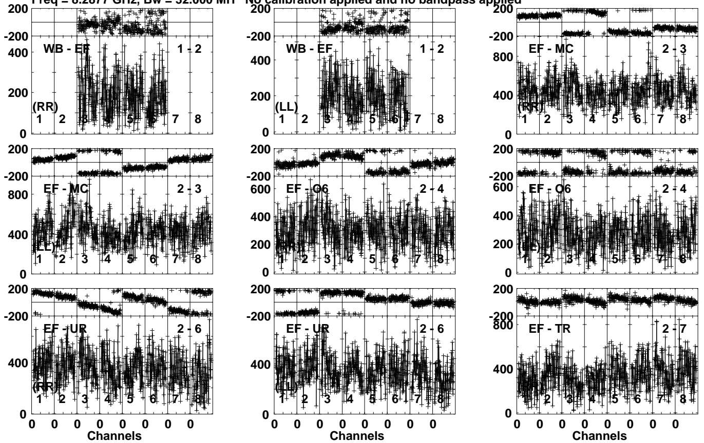
Lower frame: Micro Ampl Jy Top frame: Phas deg Vector averaged cross-power spectrum Several baselines displayed Timerange: 00/19:25:31 to 00/19:28:29
