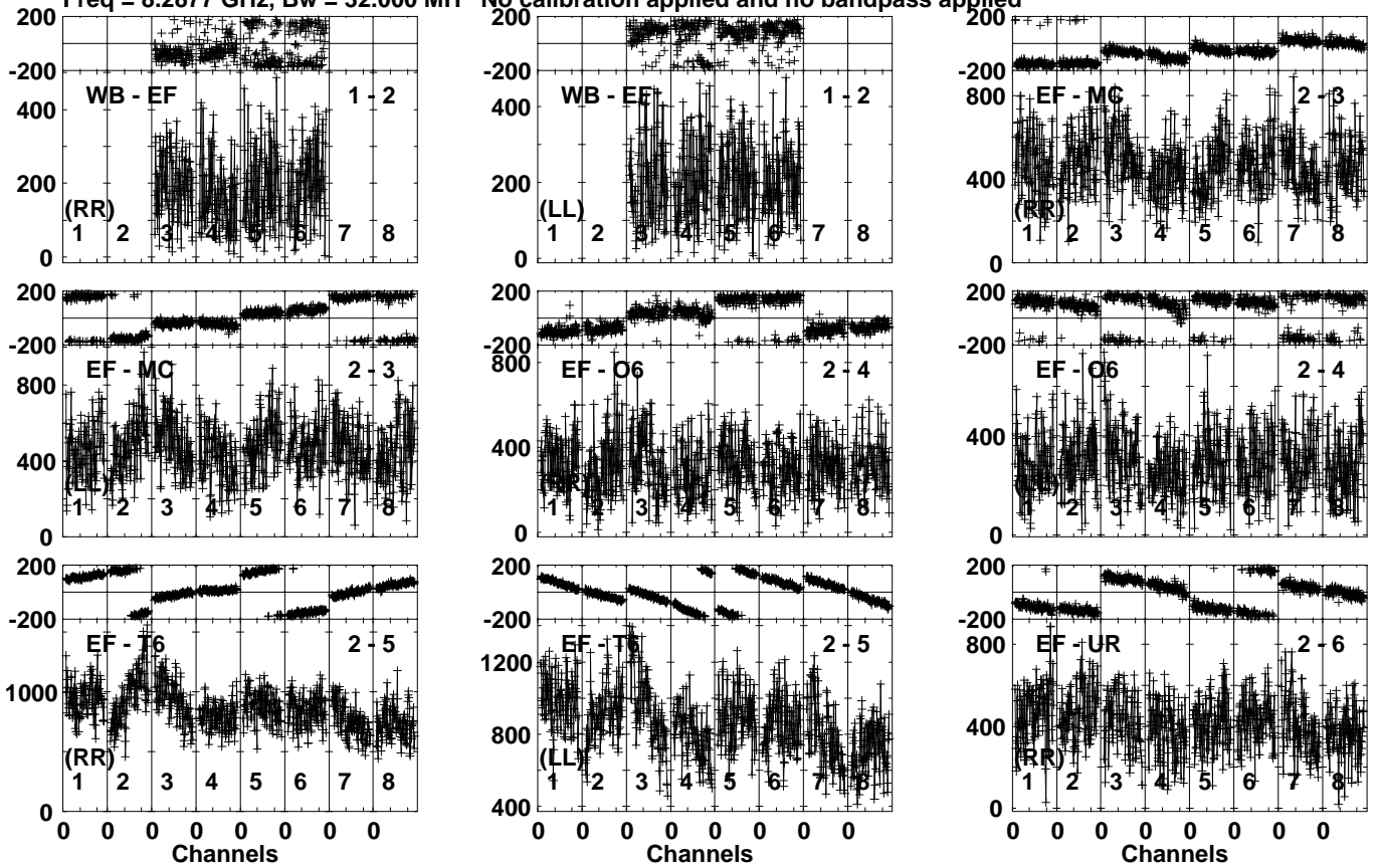
Lower frame: Micro Ampl Jy Top frame: Phas deg Vector averaged cross-power spectrum Several baselines displayed Timerange: 00/17:15:11 to 00/17:18:09
