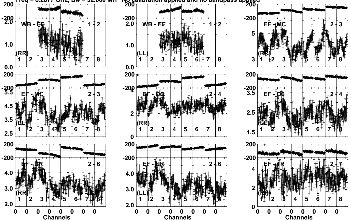
Lower frame: Milli Ampl Jy Top frame: Phas deg Vector averaged cross-power spectrum Several baselines displayed Timerange: 00/20:11:51 to 00/20:12:49
