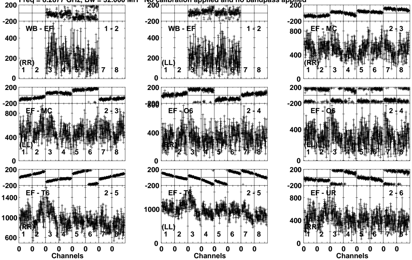
Lower frame: Micro Ampl Jy Top frame: Phas deg Vector averaged cross-power spectrum Several baselines displayed Timerange: 00/15:09:31 to 00/15:11:59
