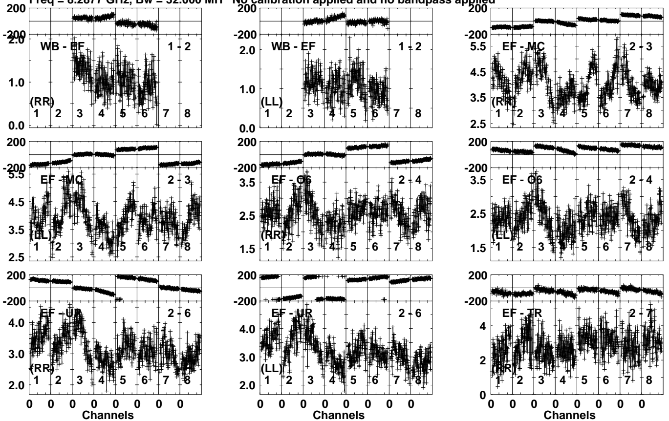
Lower frame: Milli Ampl Jy Top frame: Phas deg Vector averaged cross-power spectrum Several baselines displayed Timerange: 00/20:08:03 to 00/20:08:59
