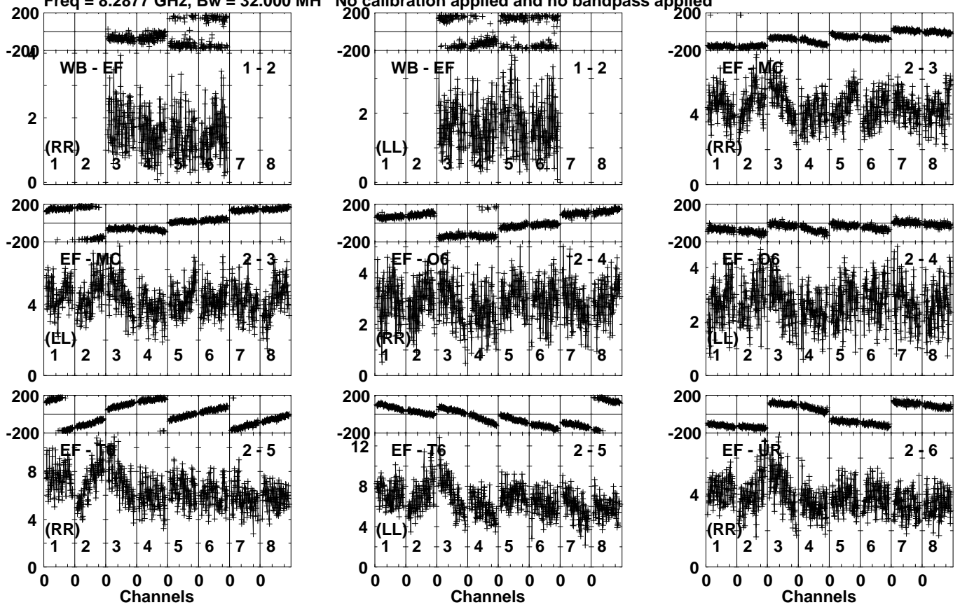
Lower frame: Milli Ampl Jy Top frame: Phas deg Vector averaged cross-power spectrum Several baselines displayed Timerange: 00/18:37:11 to 00/18:38:09
