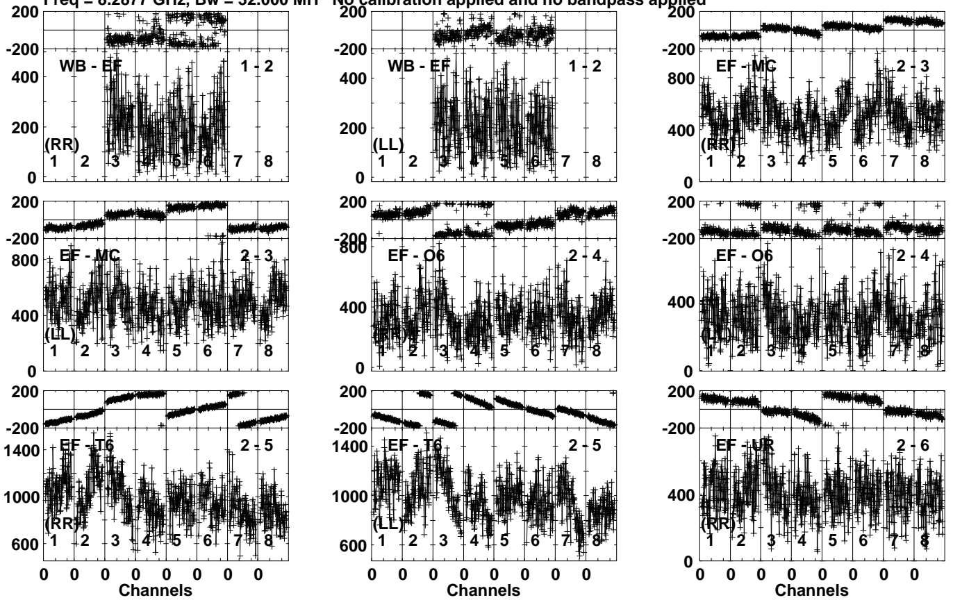
Lower frame: Micro Ampl Jy Top frame: Phas deg Vector averaged cross-power spectrum Several baselines displayed Timerange: 00/15:05:01 to 00/15:07:59
