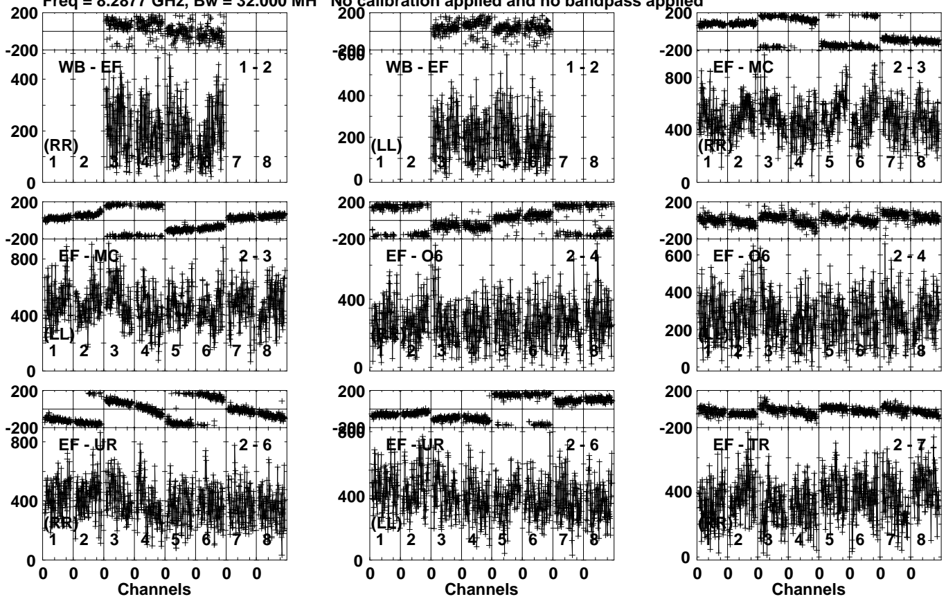
Lower frame: Micro Ampl Jy Top frame: Phas deg Vector averaged cross-power spectrum Several baselines displayed Timerange: 00/20:29:11 to 00/20:31:39
