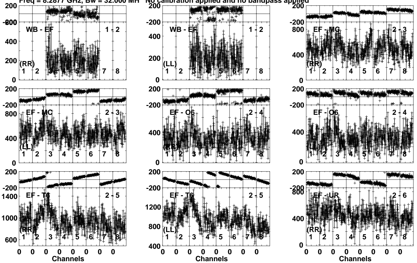
Lower frame: Micro Ampl Jy Top frame: Phas deg Vector averaged cross-power spectrum Several baselines displayed Timerange: 00/15:16:51 to 00/15:19:49
