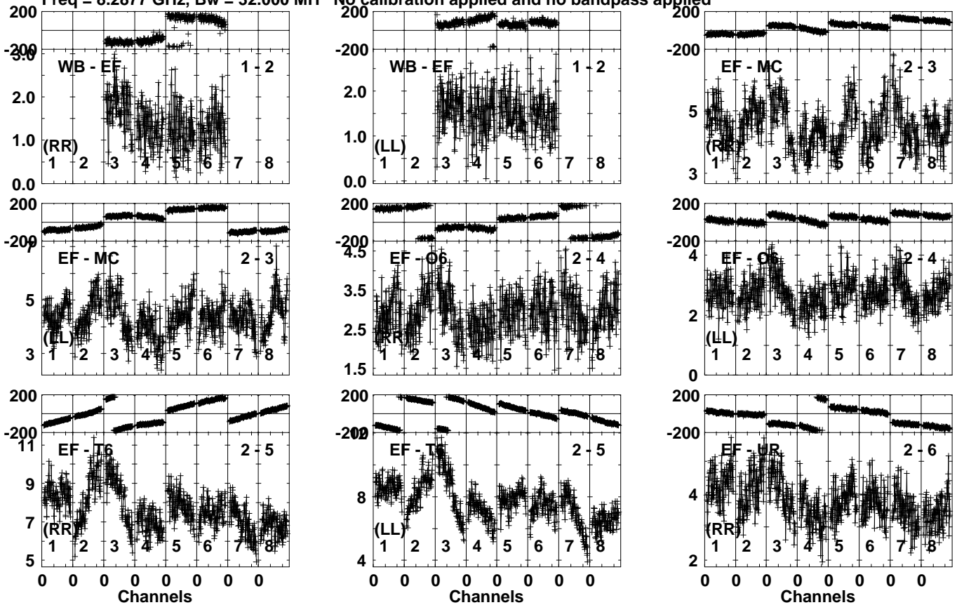
Lower frame: Milli Ampl Jy Top frame: Phas deg Vector averaged cross-power spectrum Several baselines displayed Timerange: 00/17:49:41 to 00/17:50:39
