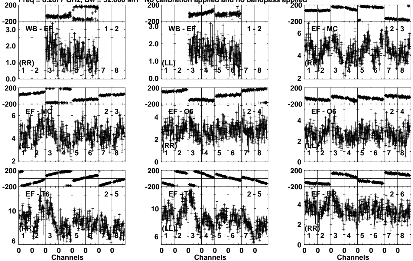
Lower frame: Milli Ampl Jy Top frame: Phas deg Vector averaged cross-power spectrum Several baselines displayed Timerange: 00/15:35:43 to 00/15:36:39
