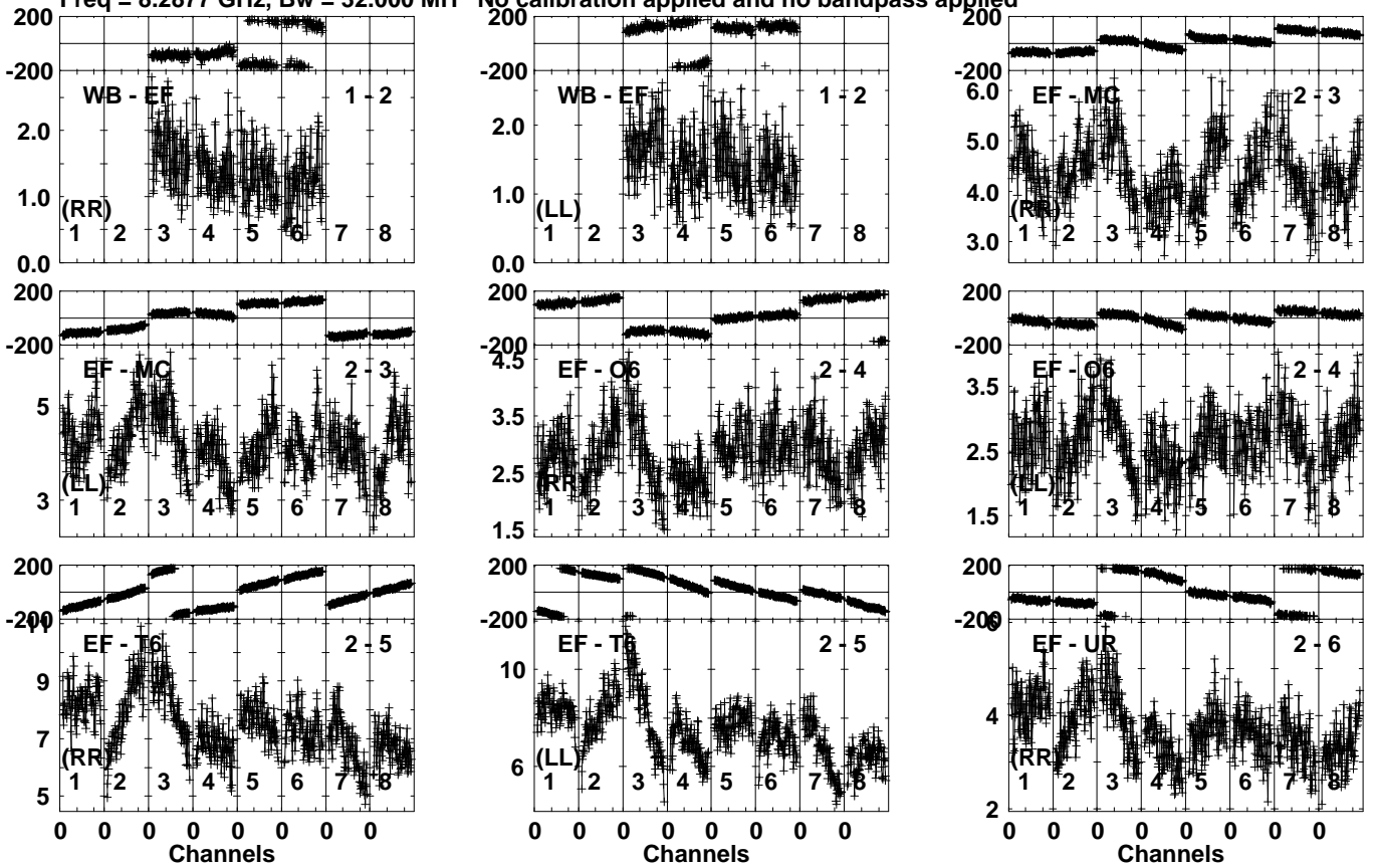
Lower frame: Milli Ampl Jy Top frame: Phas deg Vector averaged cross-power spectrum Several baselines displayed Timerange: 00/17:53:43 to 00/17:54:39
