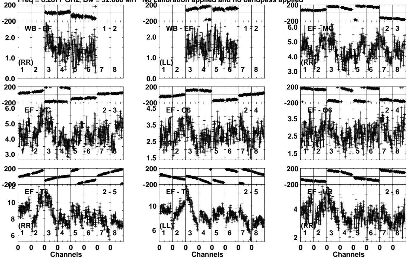
Lower frame: Milli Ampl Jy Top frame: Phas deg Vector averaged cross-power spectrum Several baselines displayed Timerange: 00/16:26:51 to 00/16:27:49
