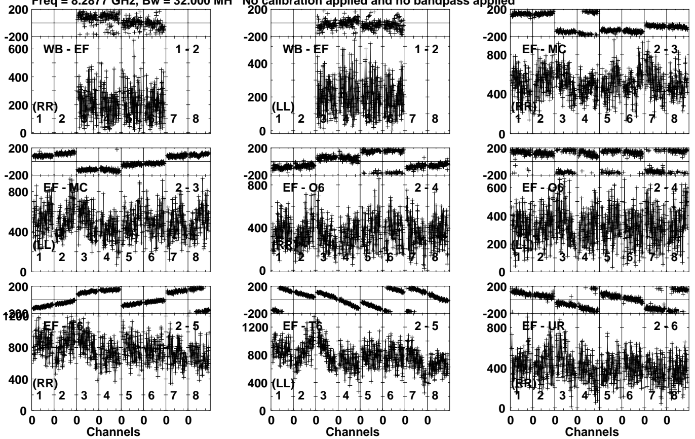
Lower frame: Micro Ampl Jy Top frame: Phas deg Vector averaged cross-power spectrum Several baselines displayed Timerange: 00/18:19:01 to 00/18:21:29
