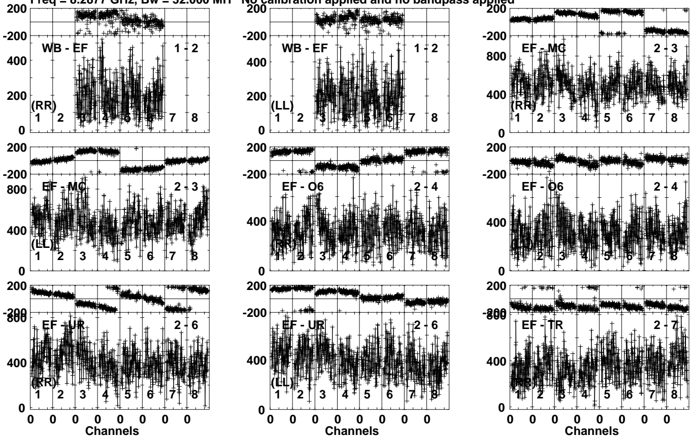
Lower frame: Micro Ampl Jy Top frame: Phas deg Vector averaged cross-power spectrum Several baselines displayed Timerange: 00/19:41:51 to 00/19:44:19
