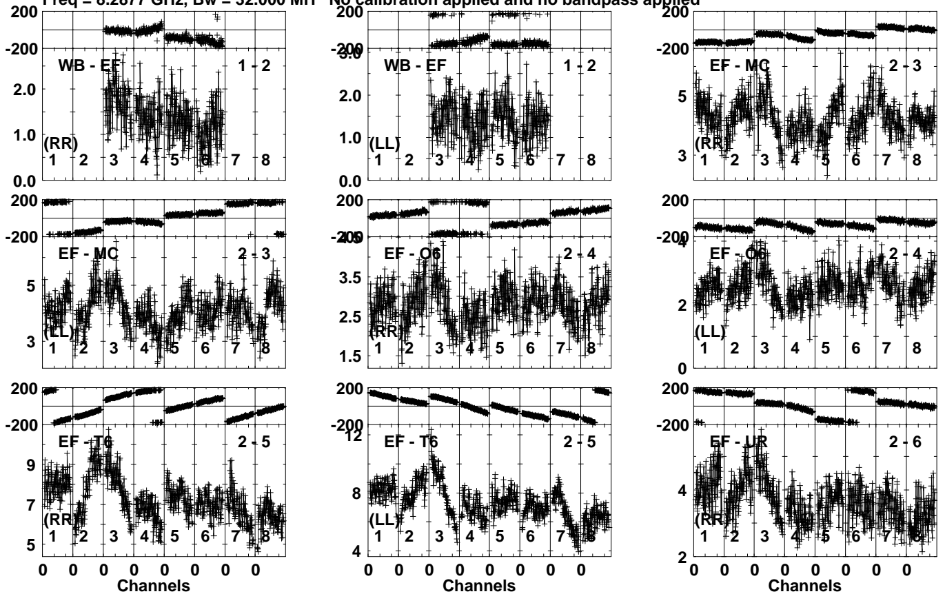
Lower frame: Milli Ampl Jy Top frame: Phas deg Vector averaged cross-power spectrum Several baselines displayed Timerange: 00/18:01:31 to 00/18:02:29
