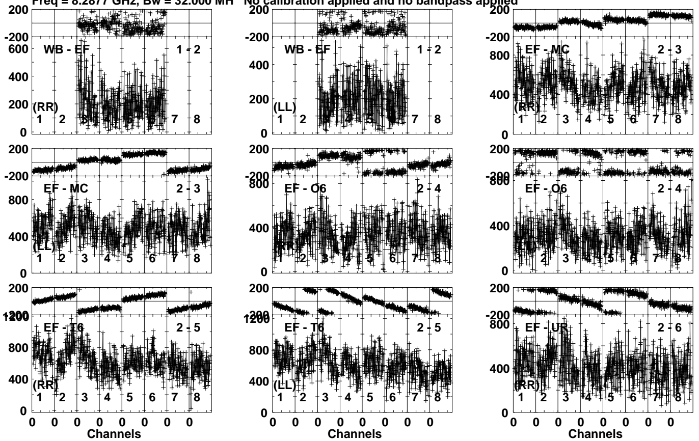
Lower frame: Micro Ampl Jy Top frame: Phas deg Vector averaged cross-power spectrum Several baselines displayed Timerange: 00/18:46:11 to 00/18:48:59
