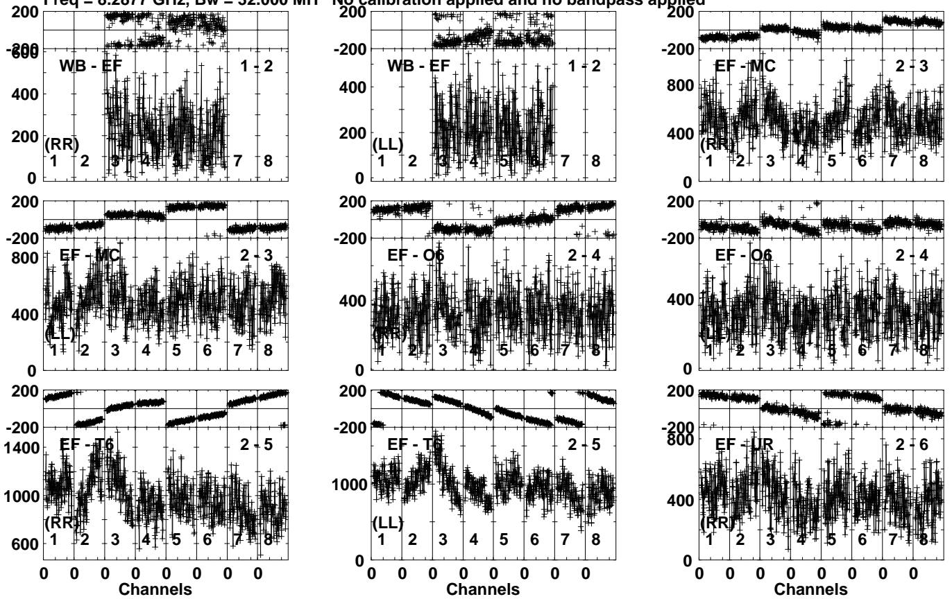
Lower frame: Micro Ampl Jy Top frame: Phas deg Vector averaged cross-power spectrum Several baselines displayed Timerange: 00/15:28:41 to 00/15:31:39
