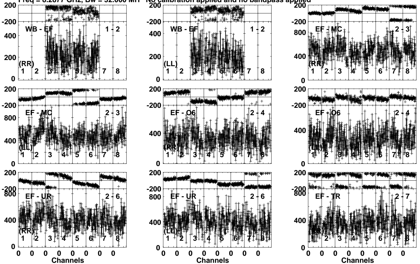
Lower frame: Micro Ampl Jy Top frame: Phas deg Vector averaged cross-power spectrum Several baselines displayed Timerange: 00/19:45:21 to 00/19:48:09
