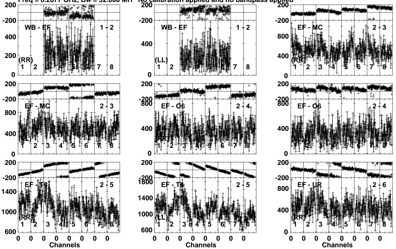
Lower frame: Micro Ampl Jy Top frame: Phas deg Vector averaged cross-power spectrum Several baselines displayed Timerange: 00/15:48:31 to 00/15:51:19
