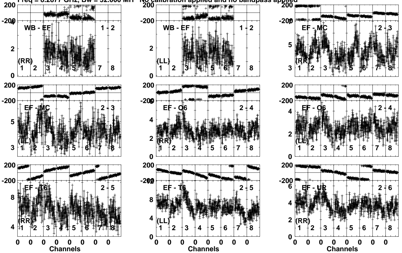
Lower frame: Milli Ampl Jy Top frame: Phas deg Vector averaged cross-power spectrum Several baselines displayed Timerange: 00/18:41:11 to 00/18:42:09
