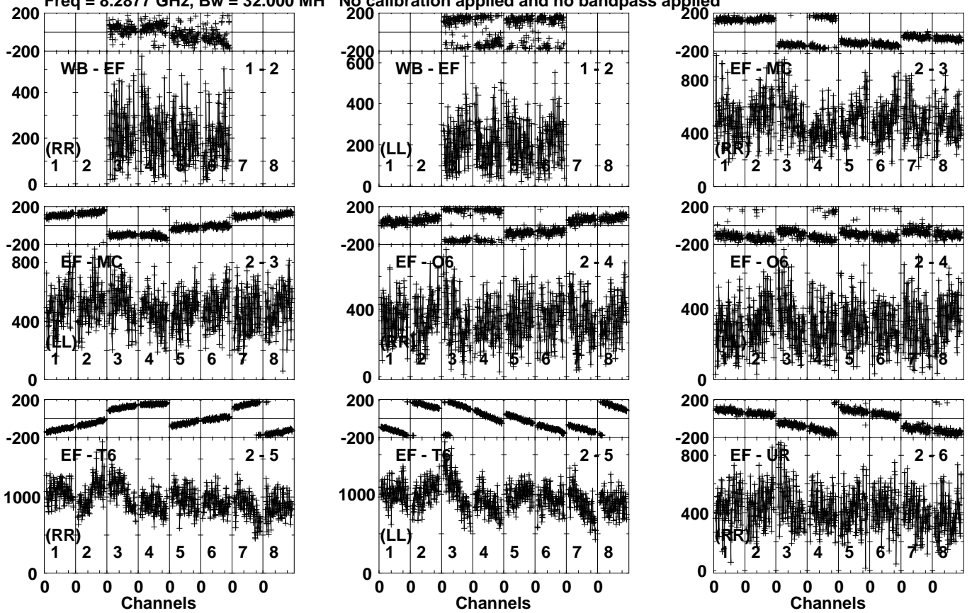
Lower frame: Micro Ampl Jy Top frame: Phas deg Vector averaged cross-power spectrum Several baselines displayed Timerange: 00/16:32:21 to 00/16:34:49
