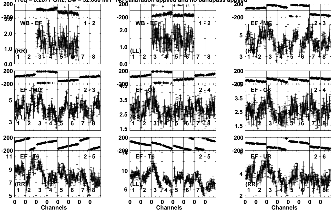
Lower frame: Milli Ampl Jy Top frame: Phas deg Vector averaged cross-power spectrum Several baselines displayed Timerange: 00/17:30:03 to 00/17:30:59
