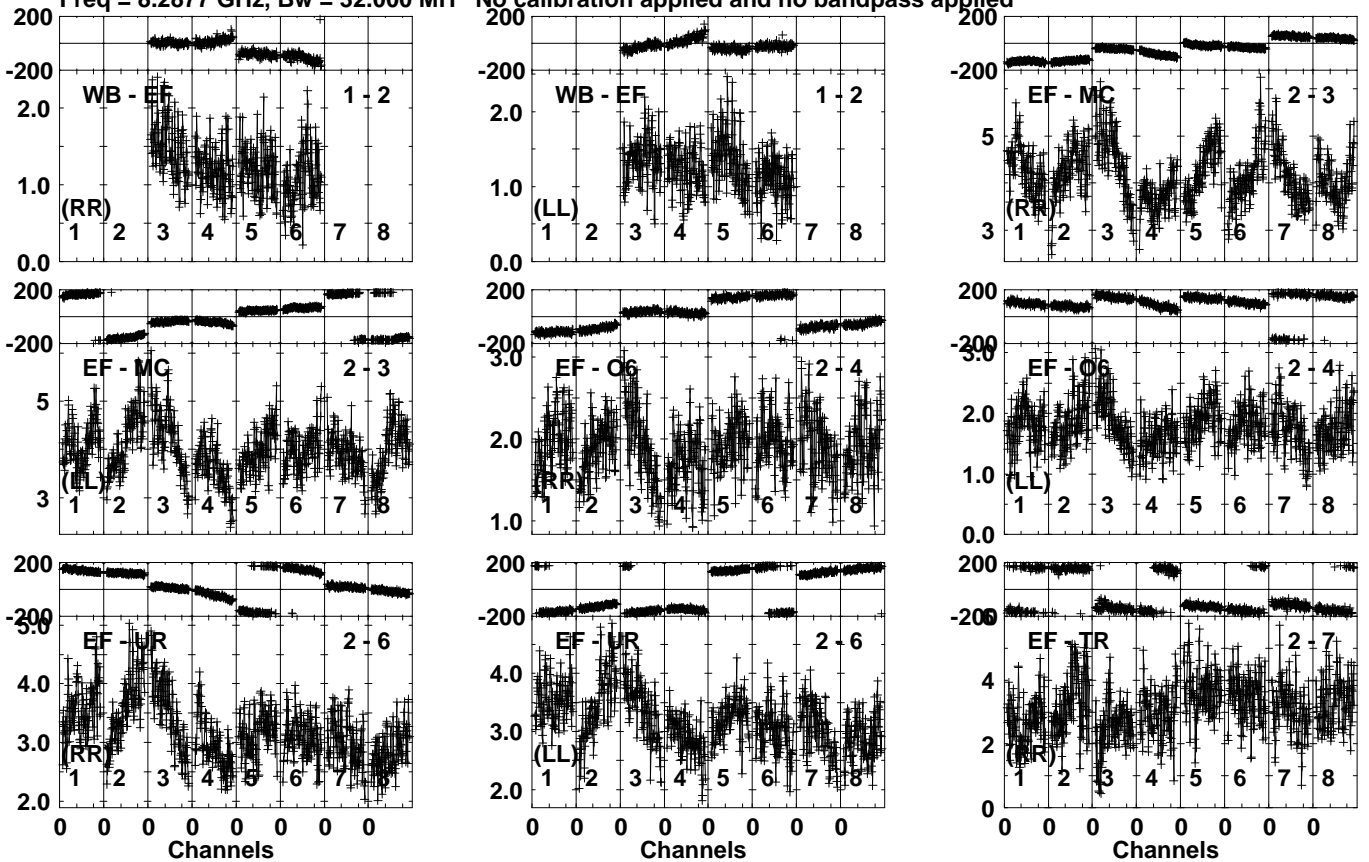
Lower frame: Milli Ampl Jy Top frame: Phas deg Vector averaged cross-power spectrum Several baselines displayed Timerange: 00/20:43:33 to 00/20:44:29
