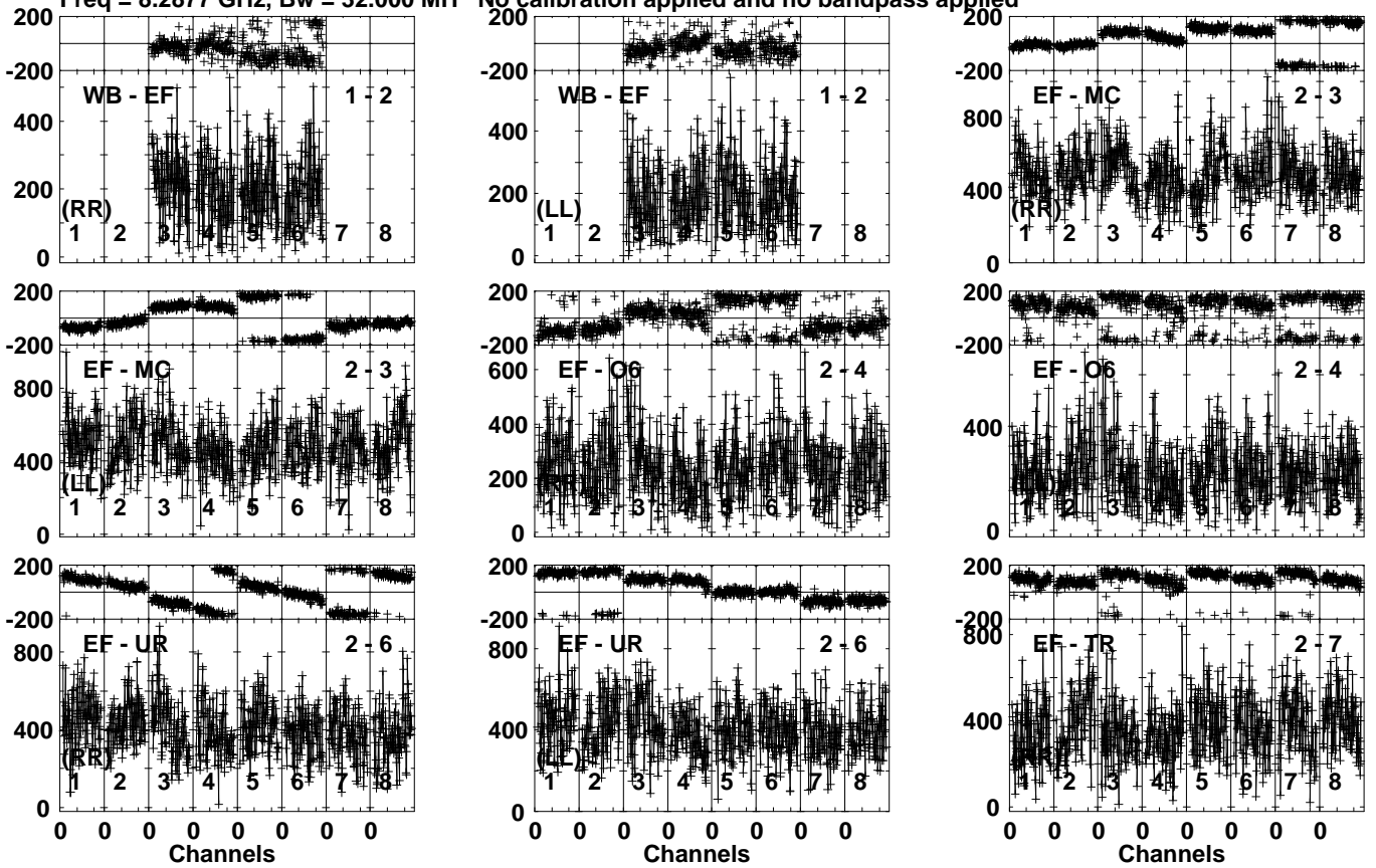
Lower frame: Micro Ampl Jy Top frame: Phas deg Vector averaged cross-power spectrum Several baselines displayed Timerange: 00/20:56:21 to 00/20:59:09
