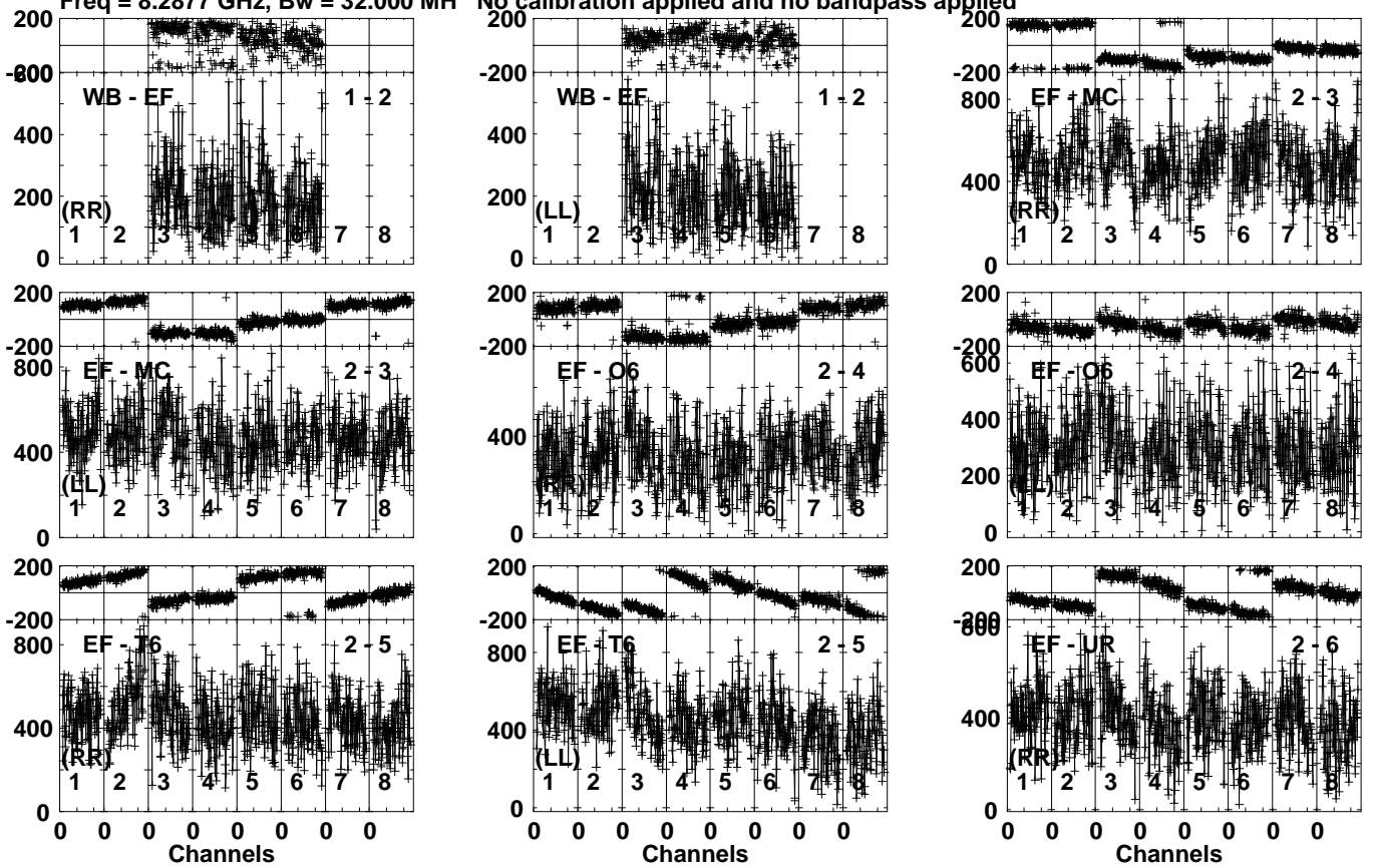
Lower frame: Micro Ampl Jy Top frame: Phas deg Vector averaged cross-power spectrum Several baselines displayed Timerange: 00/19:06:21 to 00/19:08:49
