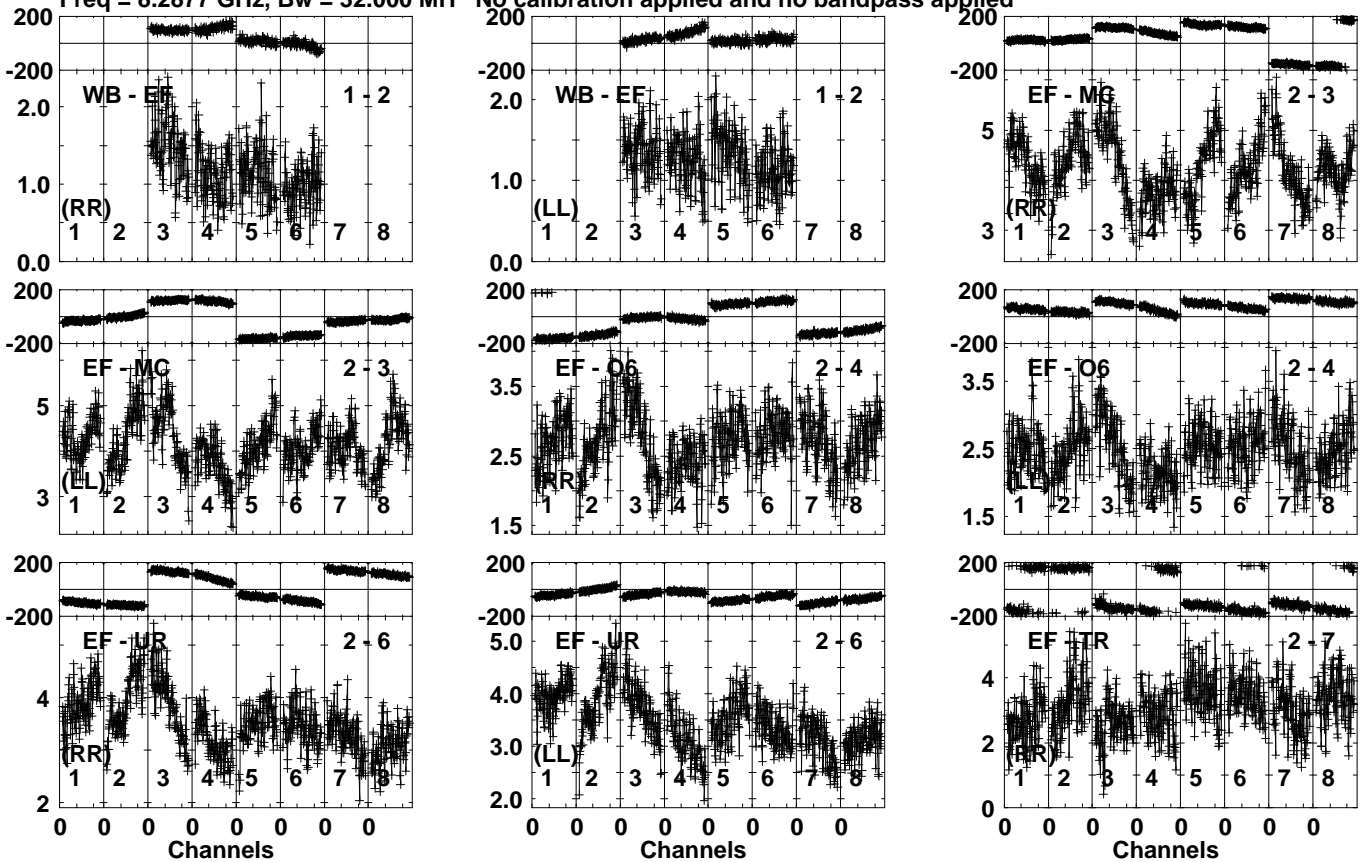
Lower frame: Milli Ampl Jy Top frame: Phas deg Vector averaged cross-power spectrum Several baselines displayed Timerange: 00/19:32:33 to 00/19:33:29
