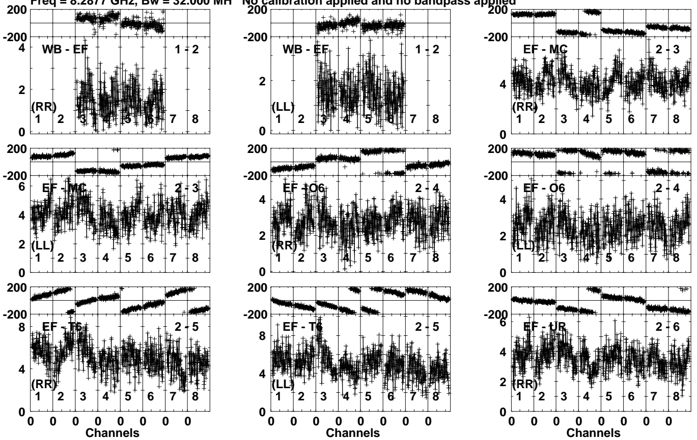
Lower frame: Milli Ampl Jy Top frame: Phas deg Vector averaged cross-power spectrum Several baselines displayed Timerange: 00/18:49:01 to 00/18:49:59
