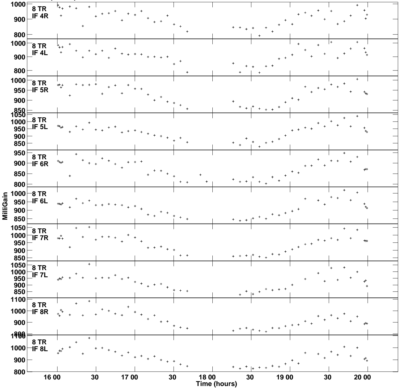
Plot file version 12 created 17-MAY-2024 11:15:24 Gain amp vs UTC time for 1933+655.MULTI.1 SN 2 Rpol & Lpol IF 1 - 8
