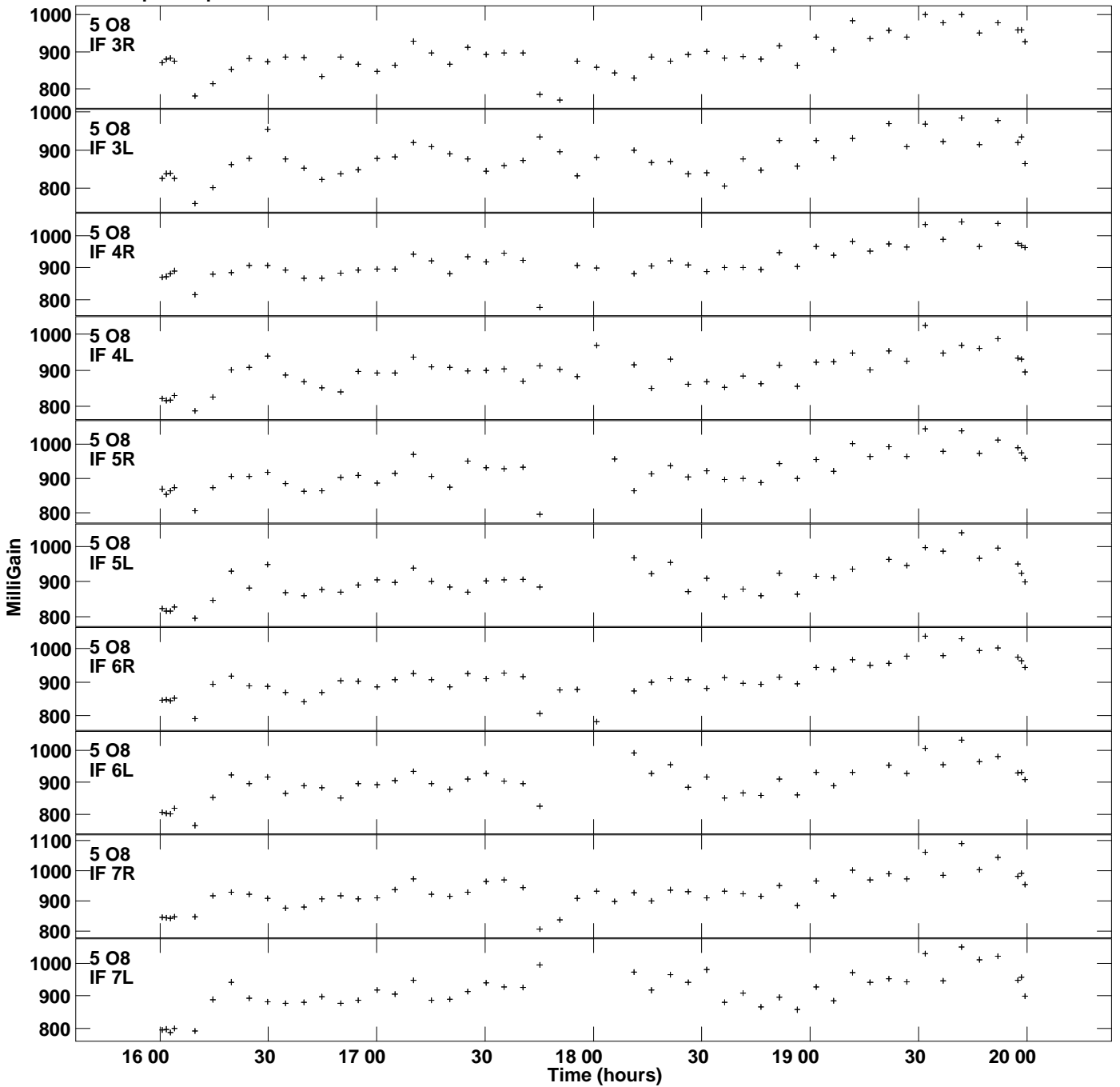
Plot file version 7 created 17-MAY-2024 11:15:24 Gain amp vs UTC time for 1933+655.MULTI.1 SN 2 Rpol & Lpol IF 1 - 8
