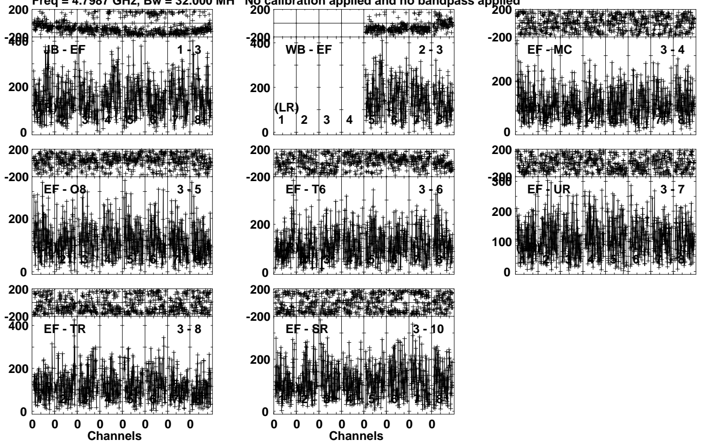
Lower frame: Micro Ampl Jy Top frame: Phas deg Vector averaged cross-power spectrum Several baselines displayed Timerange: 00/16:10:11 to 00/16:14:03
