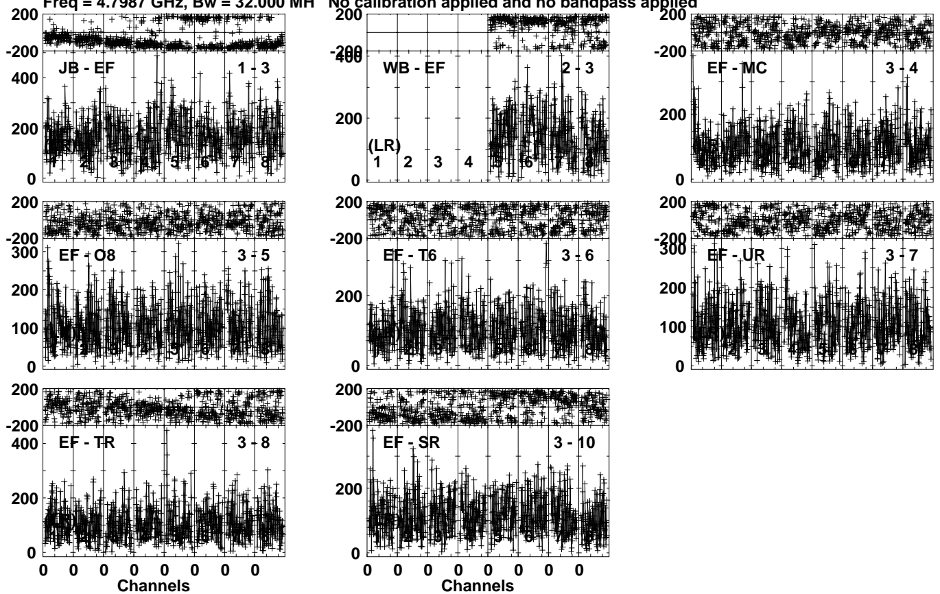
Lower frame: Micro Ampl Jy Top frame: Phas deg Vector averaged cross-power spectrum Several baselines displayed Timerange: 00/18:57:26 to 00/19:01:04
