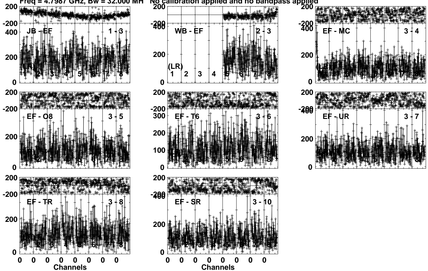
Lower frame: Micro Ampl Jy Top frame: Phas deg Vector averaged cross-power spectrum Several baselines displayed Timerange: 00/17:36:16 to 00/17:39:54
