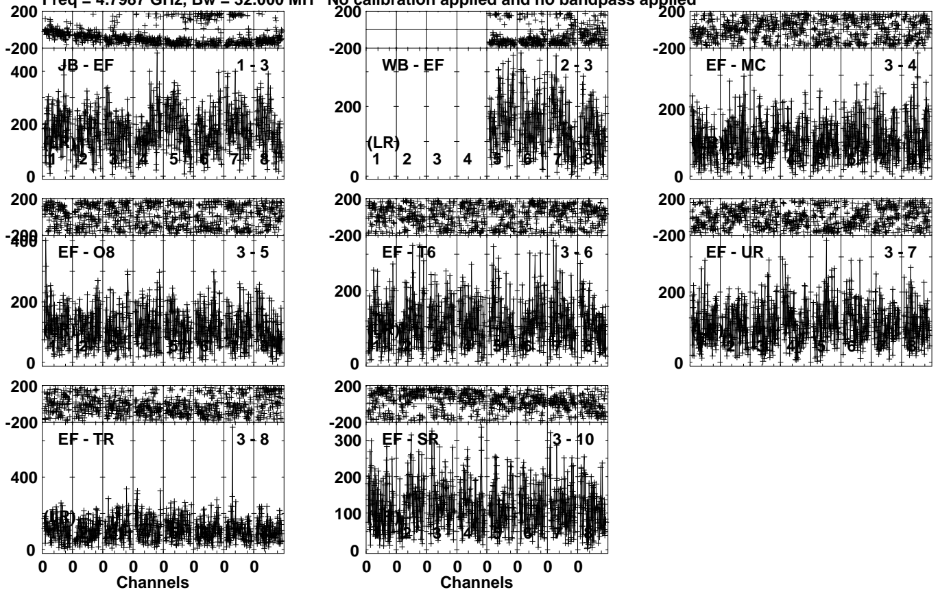
Lower frame: Micro Ampl Jy Top frame: Phas deg Vector averaged cross-power spectrum Several baselines displayed Timerange: 00/17:56:31 to 00/18:00:19
