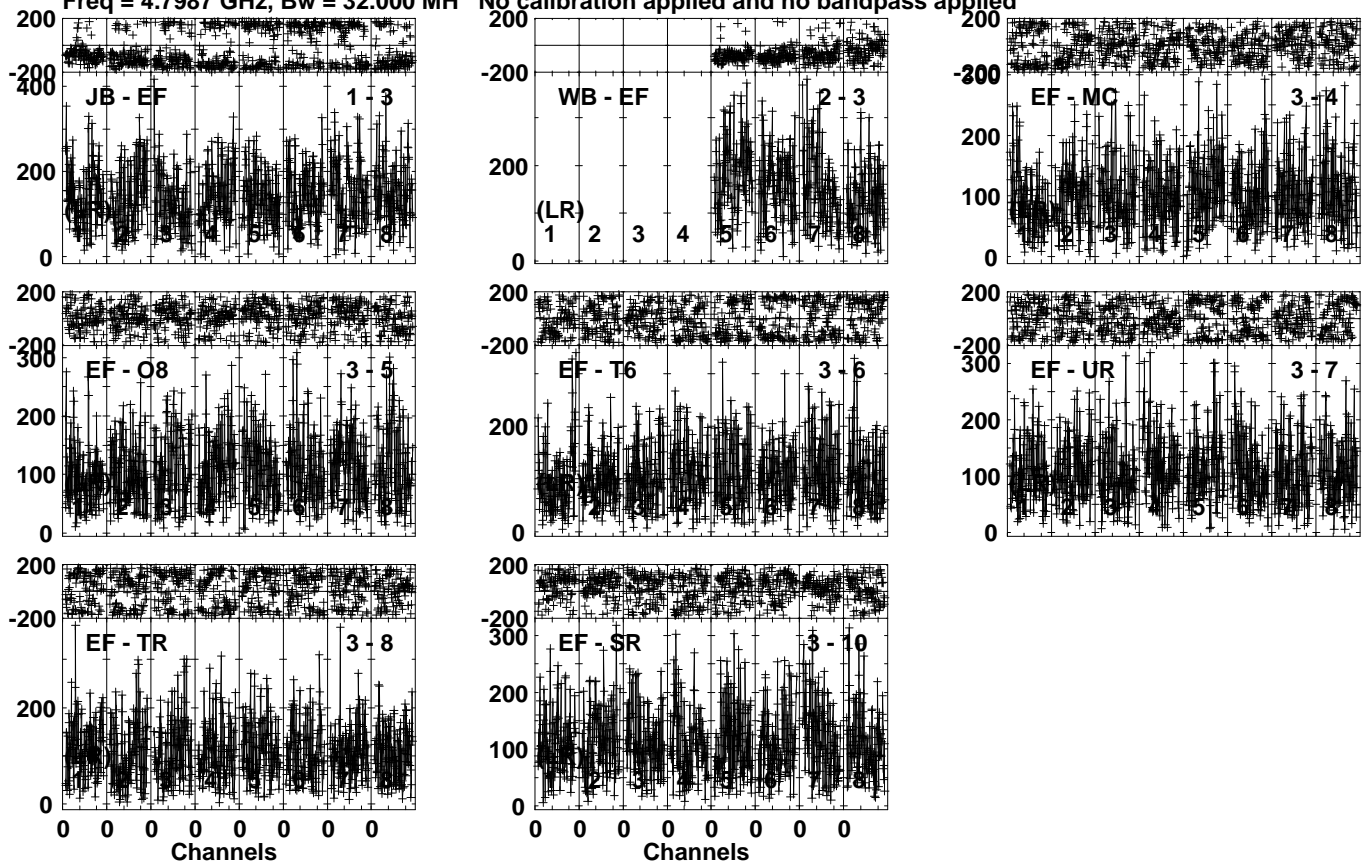
Lower frame: Micro Ampl Jy Top frame: Phas deg Vector averaged cross-power spectrum Several baselines displayed Timerange: 00/16:15:36 to 00/16:19:14
