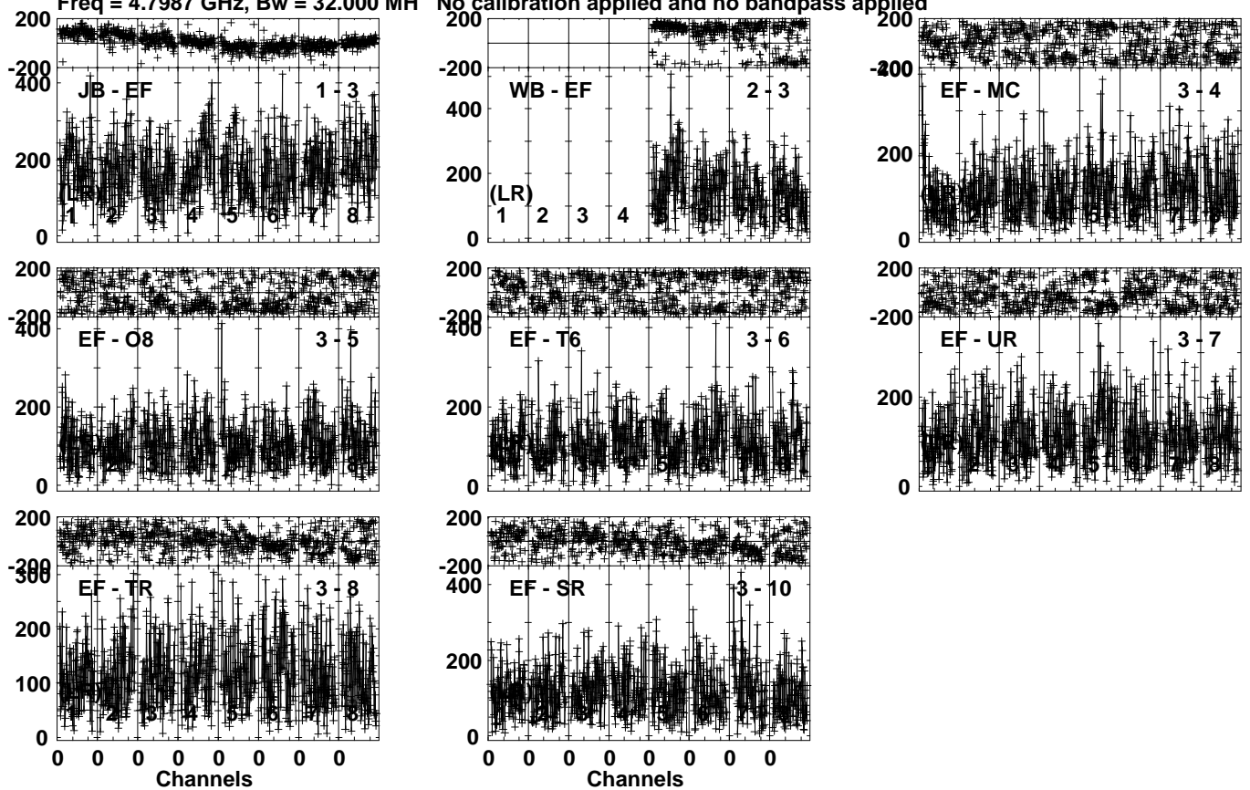
Lower frame: Micro Ampl Jy Top frame: Phas deg Vector averaged cross-power spectrum Several baselines displayed Timerange: 00/18:17:06 to 00/18:20:44
