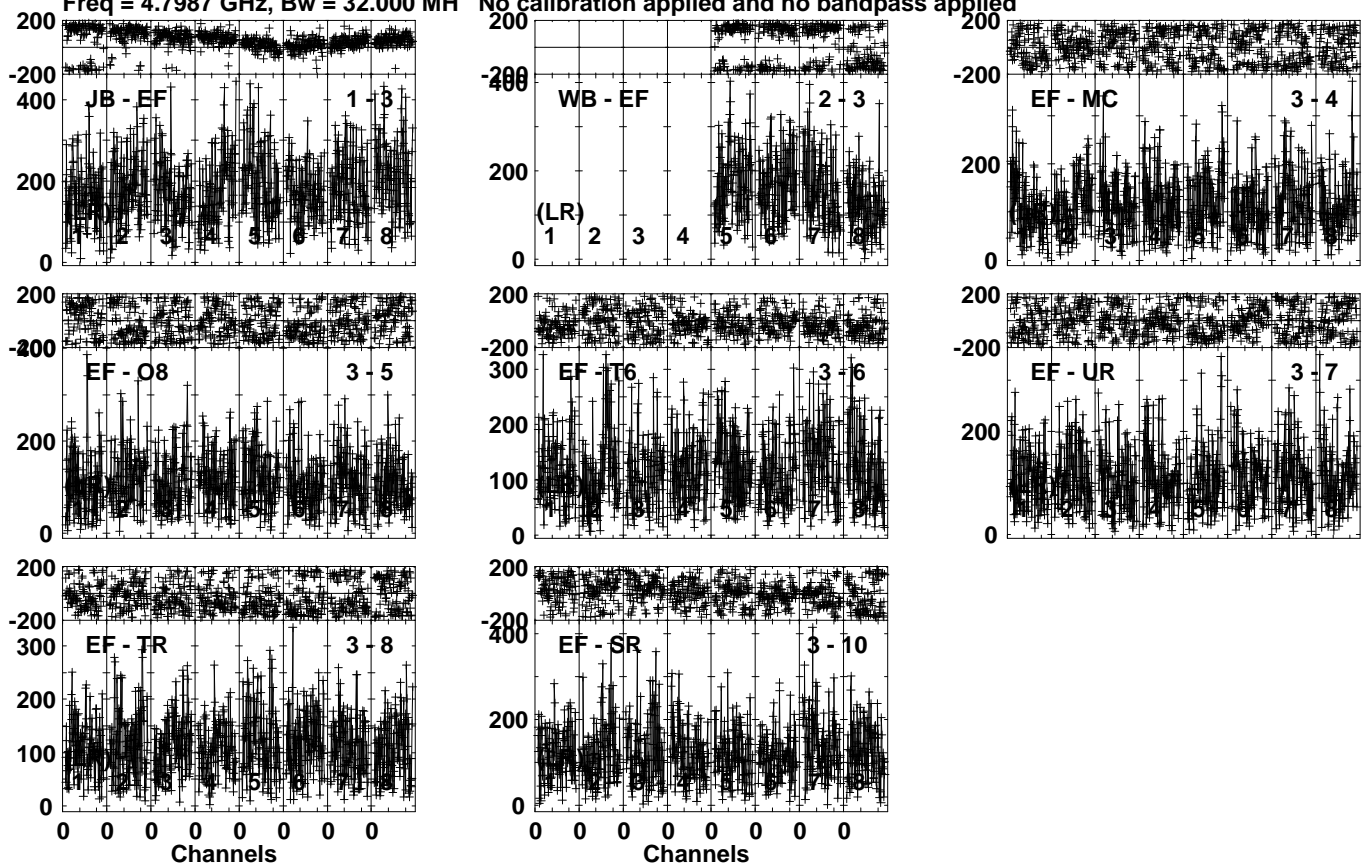
Lower frame: Micro Ampl Jy Top frame: Phas deg Vector averaged cross-power spectrum Several baselines displayed Timerange: 00/18:01:21 to 00/18:05:19
