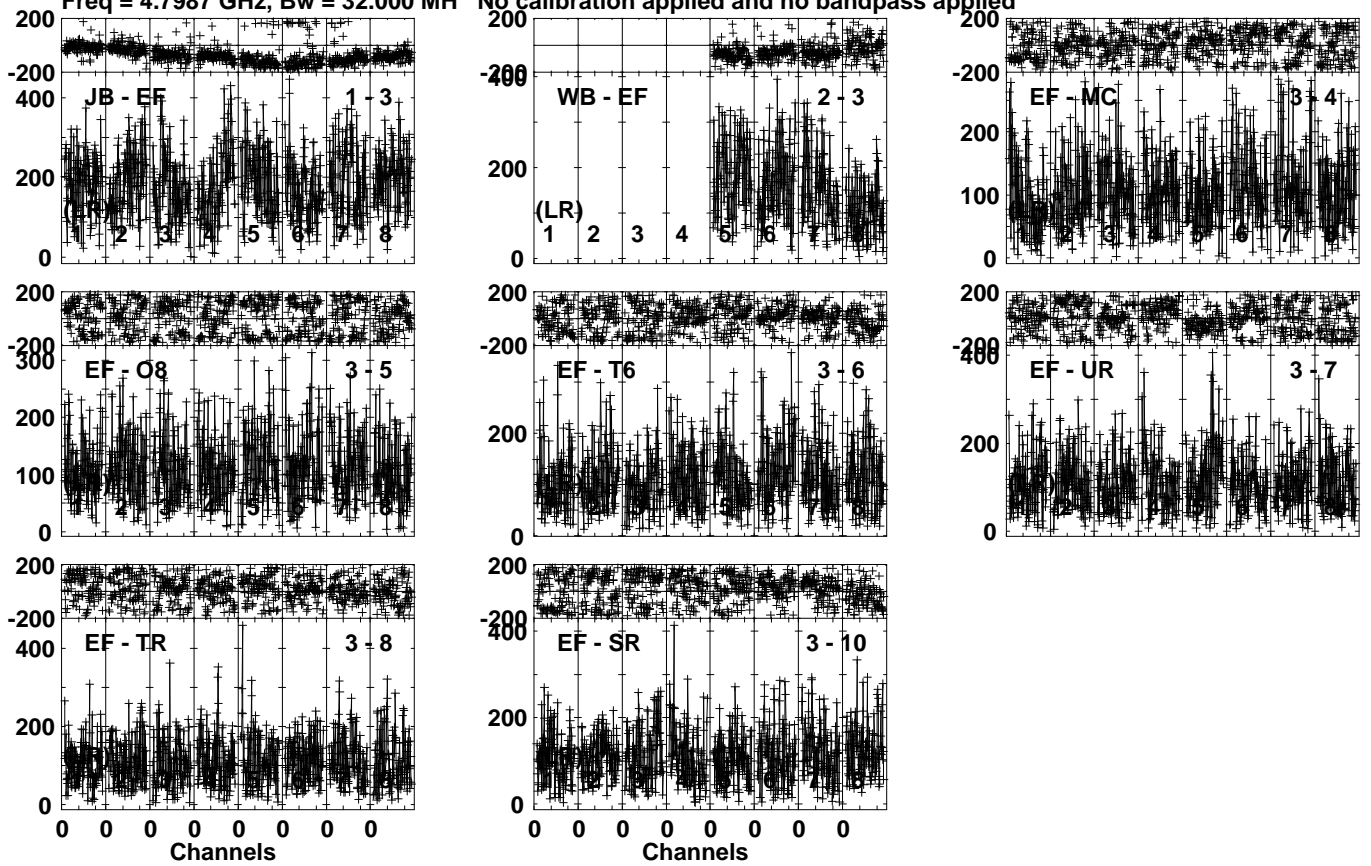
Lower frame: Micro Ampl Jy Top frame: Phas deg Vector averaged cross-power spectrum Several baselines displayed Timerange: 00/17:40:56 to 00/17:44:48
