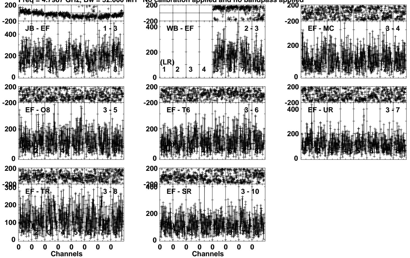
Lower frame: Micro Ampl Jy Top frame: Phas deg Vector averaged cross-power spectrum Several baselines displayed Timerange: 00/18:21:46 to 00/18:25:38
