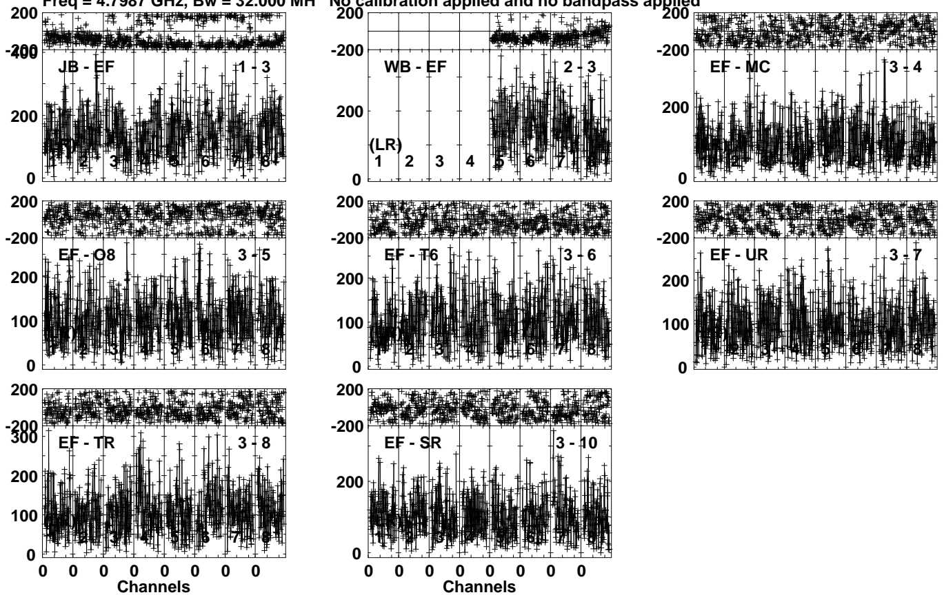
Lower frame: Micro Ampl Jy Top frame: Phas deg Vector averaged cross-power spectrum Several baselines displayed Timerange: 00/16:05:11 to 00/16:09:09
