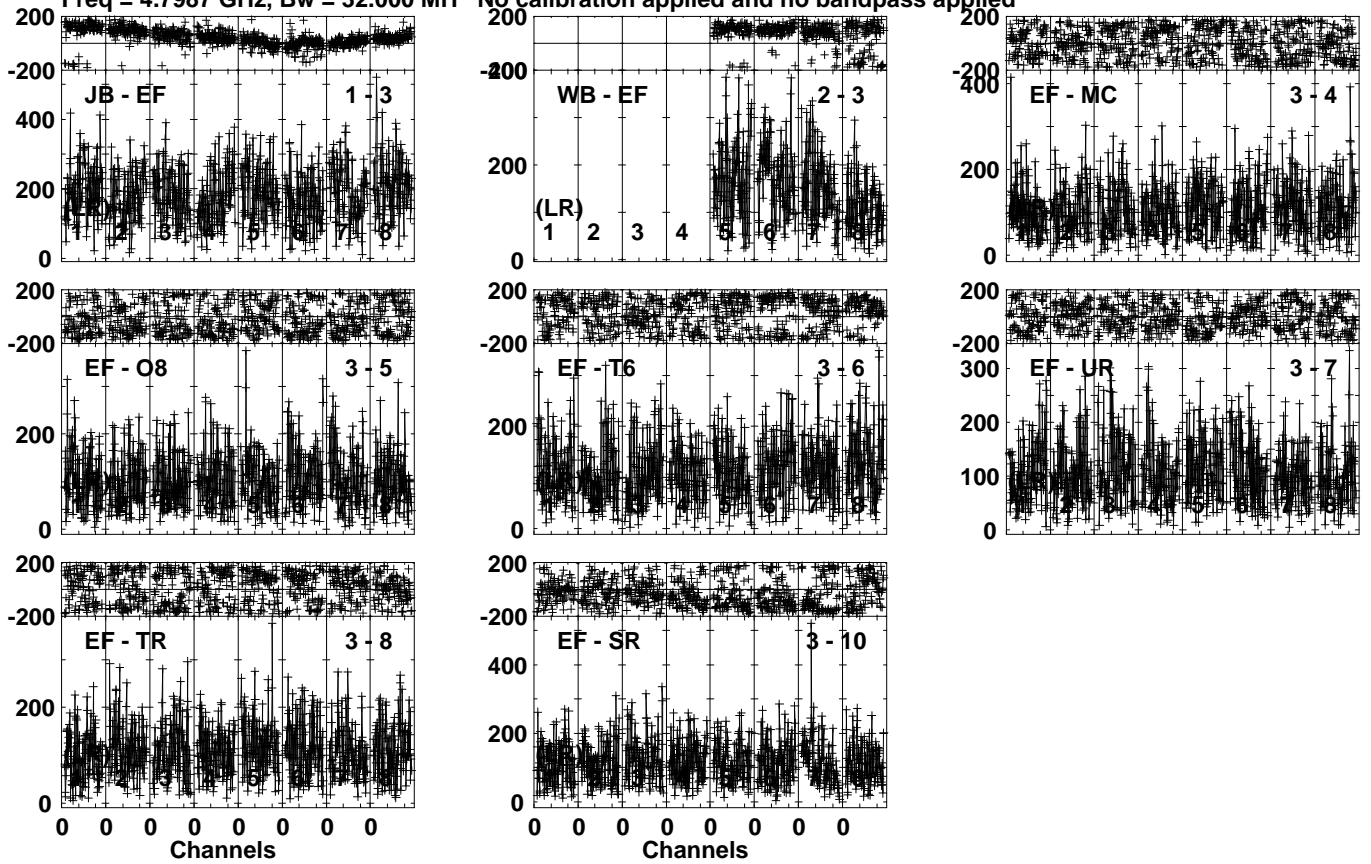
Lower frame: Micro Ampl Jy Top frame: Phas deg Vector averaged cross-power spectrum Several baselines displayed Timerange: 00/18:06:51 to 00/18:10:39
