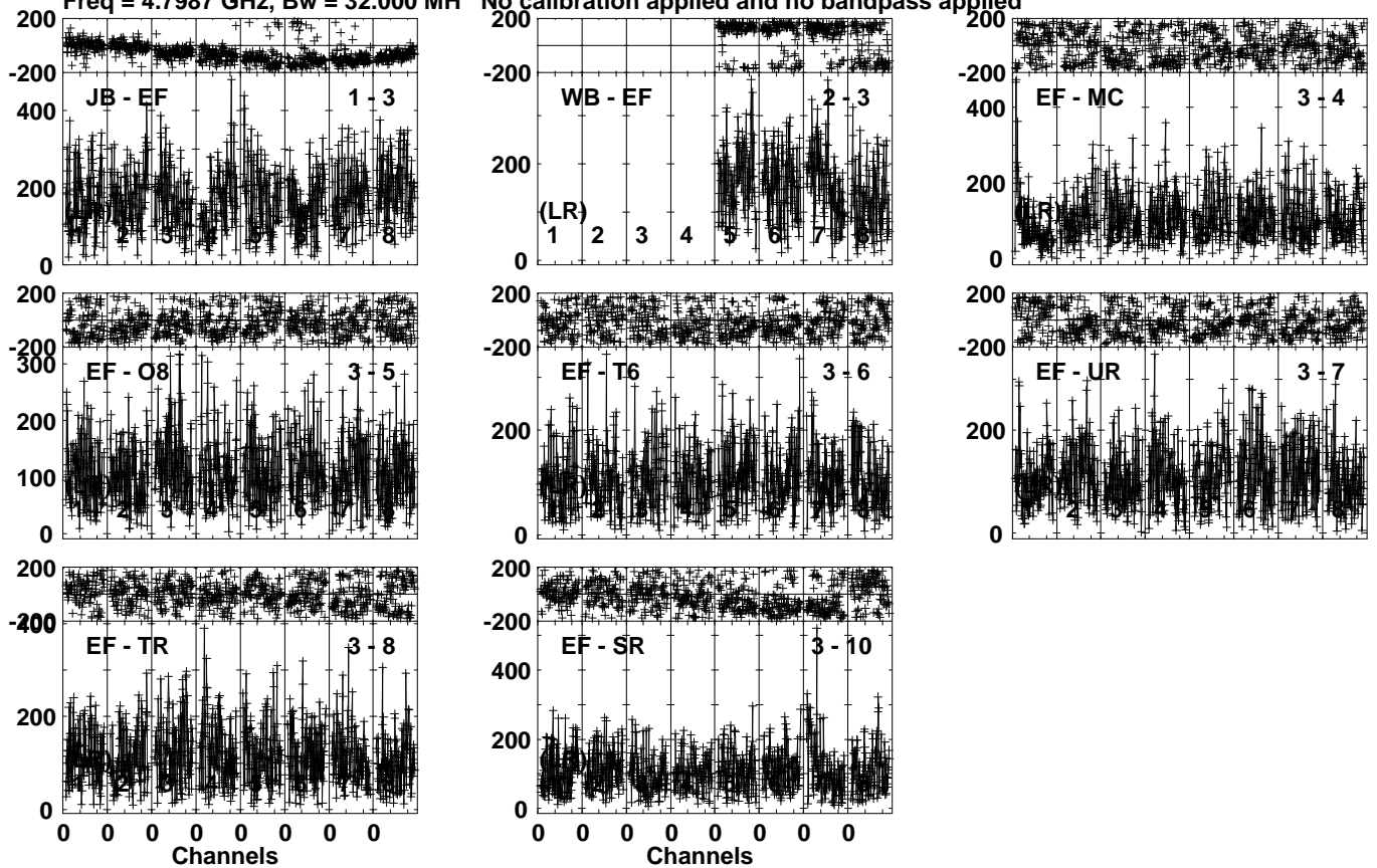
Lower frame: Micro Ampl Jy Top frame: Phas deg Vector averaged cross-power spectrum Several baselines displayed Timerange: 00/18:52:01 to 00/18:55:53
