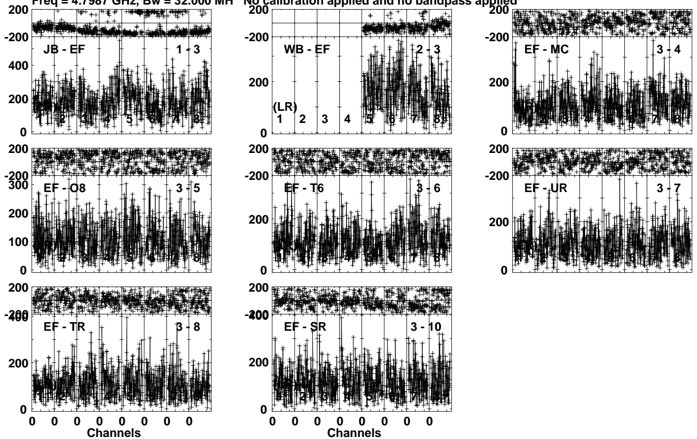
Lower frame: Micro Ampl Jy Top frame: Phas deg Vector averaged cross-power spectrum Several baselines displayed Timerange: 00/17:46:21 to 00/17:49:59
