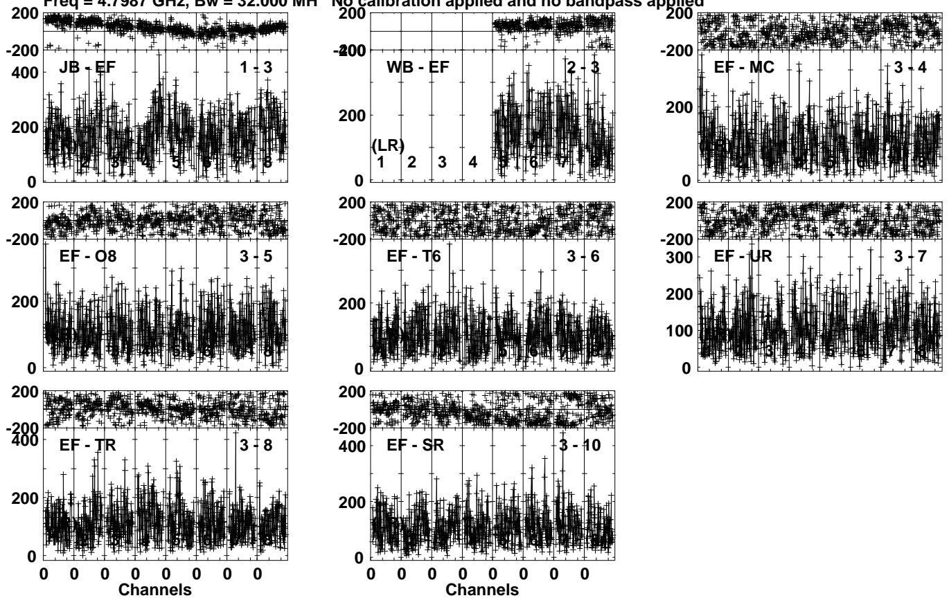
Lower frame: Micro Ampl Jy Top frame: Phas deg Vector averaged cross-power spectrum Several baselines displayed Timerange: 00/19:27:41 to 00/19:31:19
