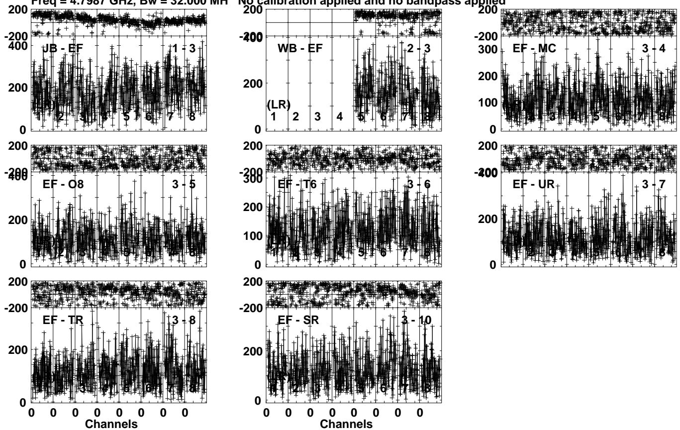
Lower frame: Micro Ampl Jy Top frame: Phas deg Vector averaged cross-power spectrum Several baselines displayed Timerange: 00/18:11:41 to 00/18:15:33
