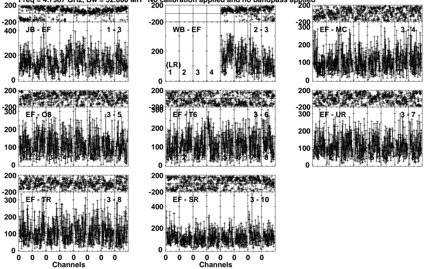
Lower frame: Micro Ampl Jy Top frame: Phas deg Vector averaged cross-power spectrum Several baselines displayed Timerange: 00/17:06:01 to 00/17:09:39
