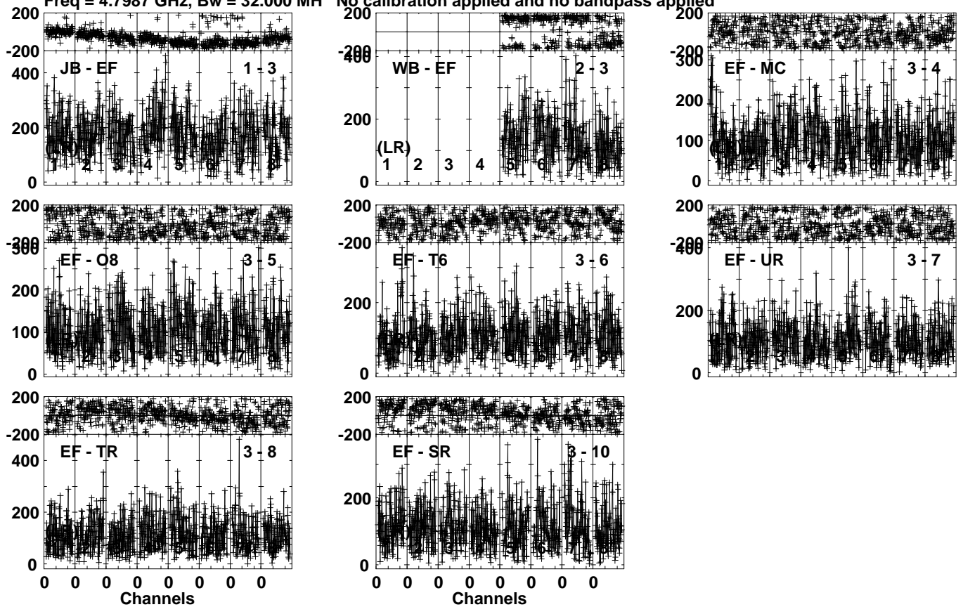
Lower frame: Micro Ampl Jy Top frame: Phas deg Vector averaged cross-power spectrum Several baselines displayed Timerange: 00/18:47:21 to 00/18:50:59
