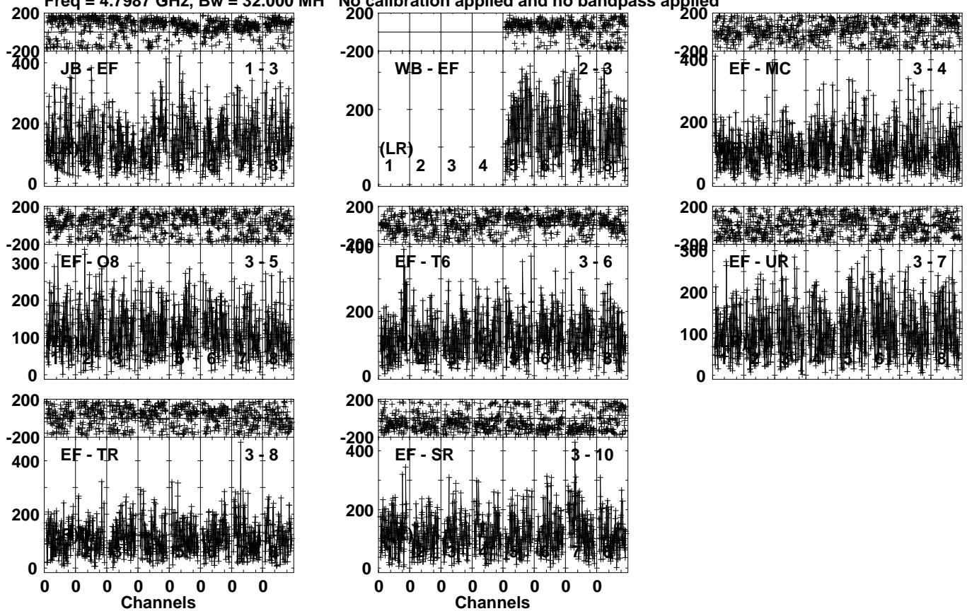
Lower frame: Micro Ampl Jy Top frame: Phas deg Vector averaged cross-power spectrum Several baselines displayed Timerange: 00/17:00:36 to 00/17:04:28
