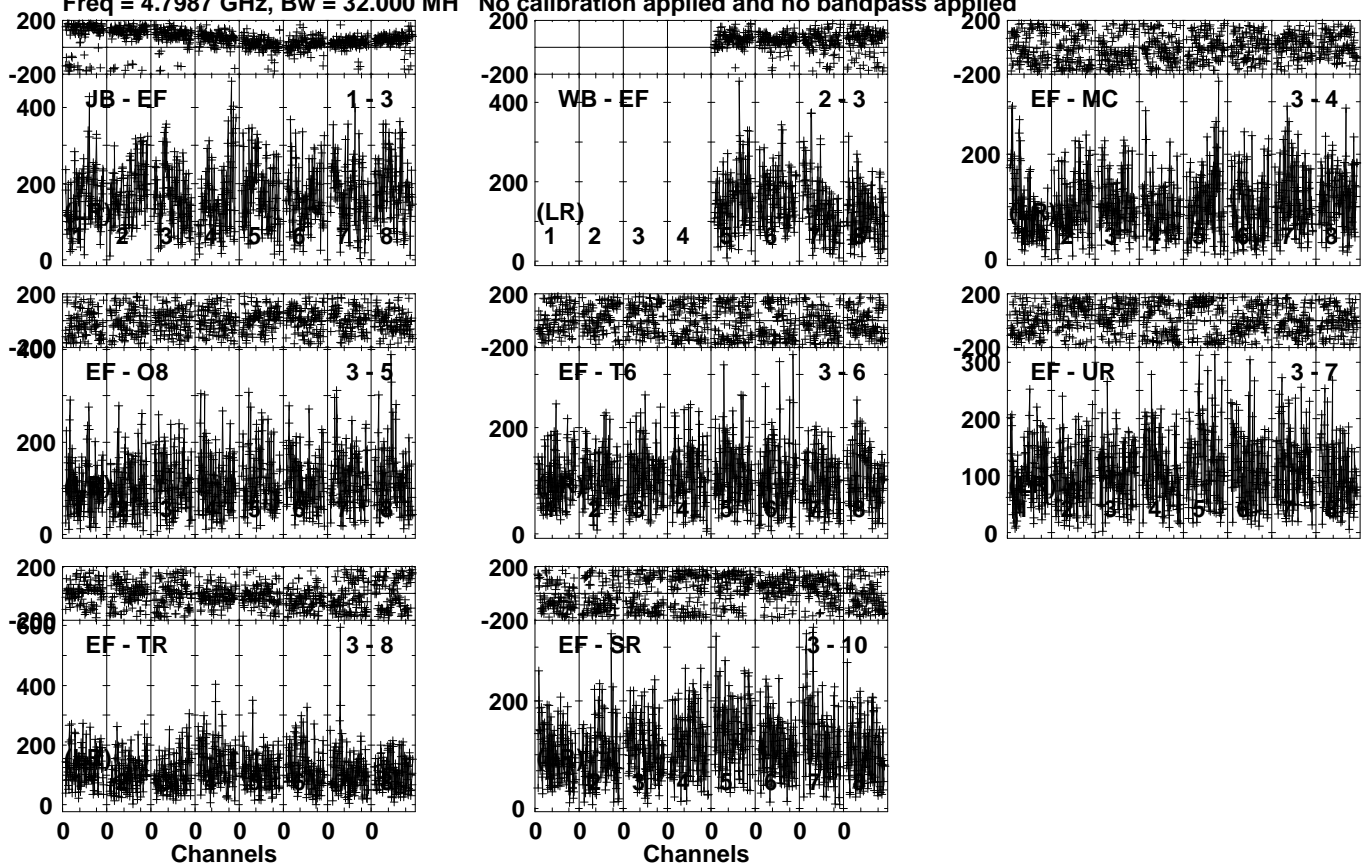
Lower frame: Micro Ampl Jy Top frame: Phas deg Vector averaged cross-power spectrum Several baselines displayed Timerange: 00/19:32:21 to 00/19:36:13
