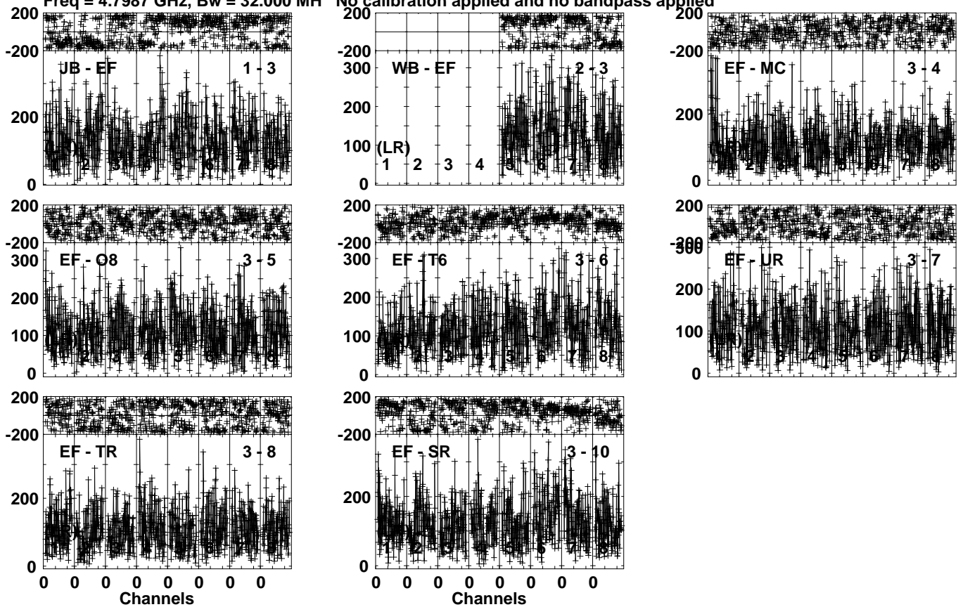
Lower frame: Micro Ampl Jy Top frame: Phas deg Vector averaged cross-power spectrum Several baselines displayed Timerange: 00/16:50:31 to 00/16:54:23
