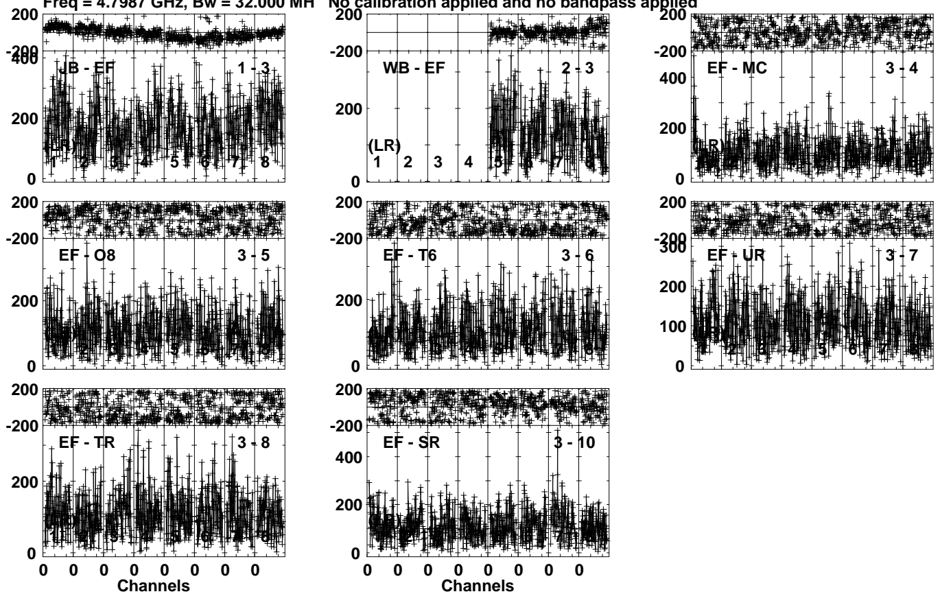
Lower frame: Micro Ampl Jy Top frame: Phas deg Vector averaged cross-power spectrum Several baselines displayed Timerange: 00/17:26:11 to 00/17:29:49
