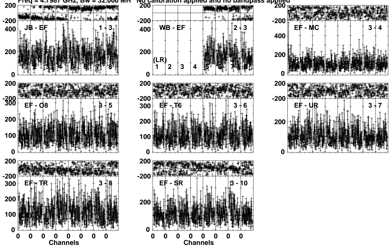
Lower frame: Micro Ampl Jy Top frame: Phas deg Vector averaged cross-power spectrum Several baselines displayed Timerange: 00/19:02:06 to 00/19:05:58
