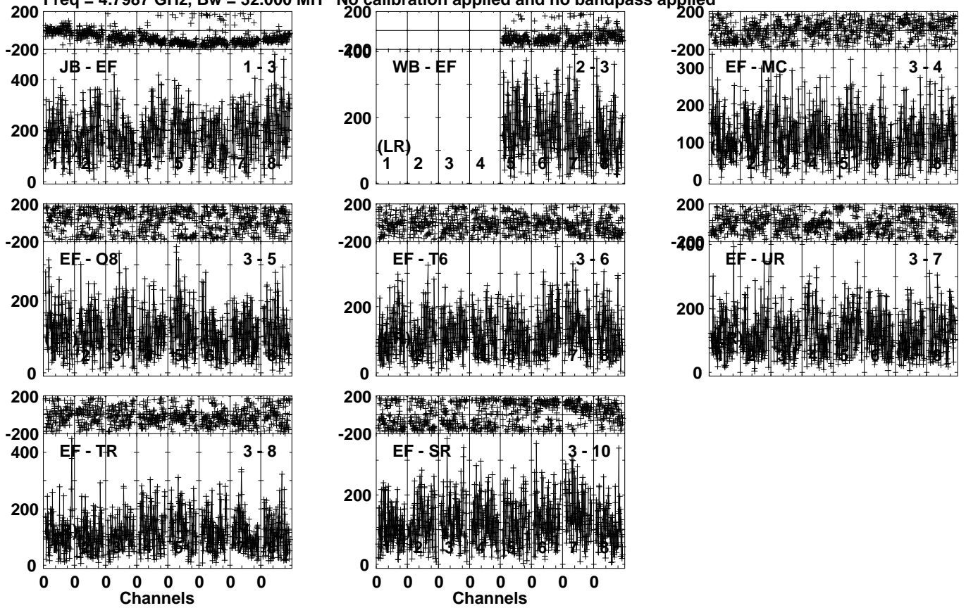
Lower frame: Micro Ampl Jy Top frame: Phas deg Vector averaged cross-power spectrum Several baselines displayed Timerange: 00/17:51:01 to 00/17:54:59
