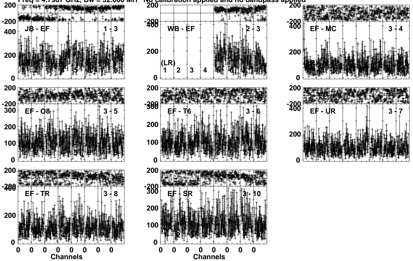
Lower frame: Micro Ampl Jy Top frame: Phas deg Vector averaged cross-power spectrum Several baselines displayed Timerange: 00/19:17:36 to 00/19:21:14
