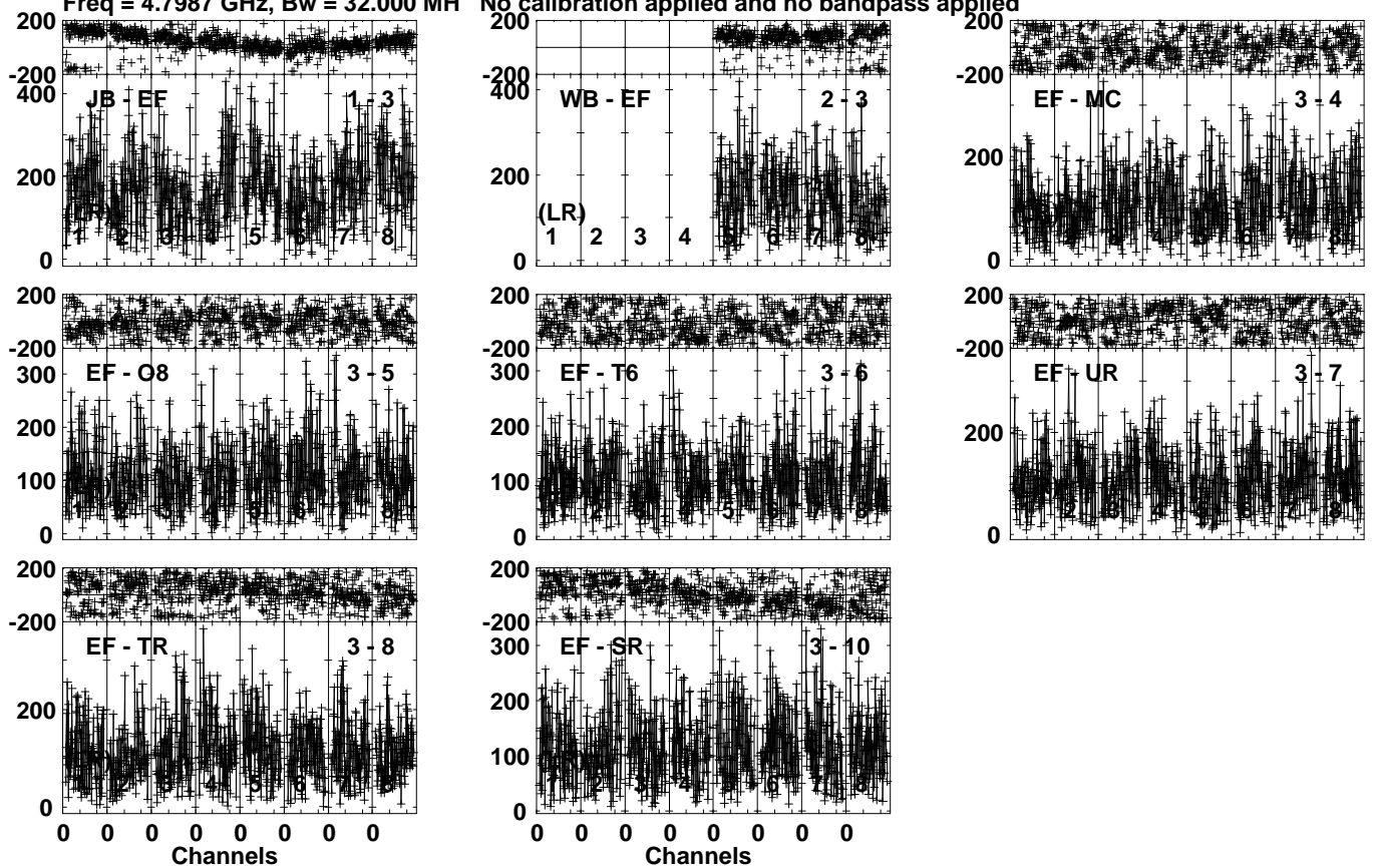
Lower frame: Micro Ampl Jy Top frame: Phas deg Vector averaged cross-power spectrum Several baselines displayed Timerange: 00/19:22:16 to 00/19:26:08
