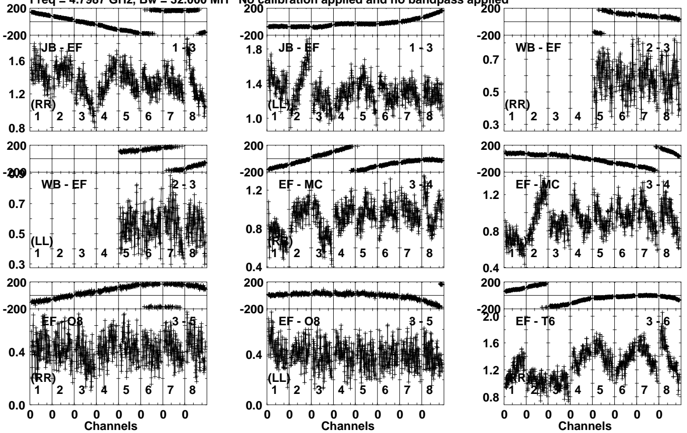
Lower frame: Milli Ampl Jy Top frame: Phas deg Vector averaged cross-power spectrum Several baselines displayed Timerange: 00/18:11:41 to 00/18:15:33
