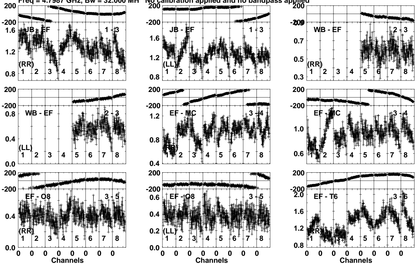
Lower frame: Milli Ampl Jy Top frame: Phas deg Vector averaged cross-power spectrum Several baselines displayed Timerange: 00/17:46:21 to 00/17:49:59
