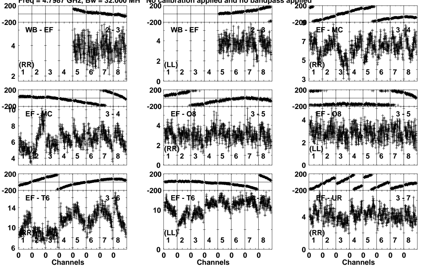
Lower frame: Milli Ampl Jy Top frame: Phas deg Vector averaged cross-power spectrum Several baselines displayed Timerange: 00/18:00:21 to 00/18:01:19
