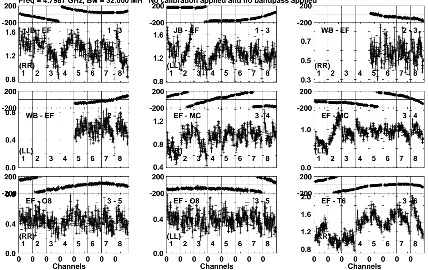
Lower frame: Milli Ampl Jy Top frame: Phas deg Vector averaged cross-power spectrum Several baselines displayed Timerange: 00/17:40:56 to 00/17:44:48
