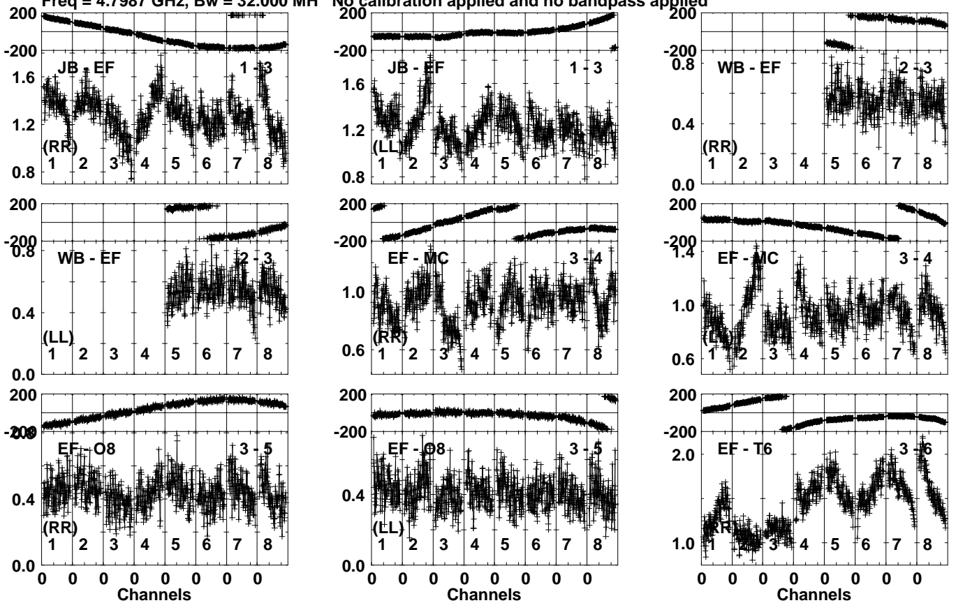
Lower frame: Milli Ampl Jy Top frame: Phas deg Vector averaged cross-power spectrum Several baselines displayed Timerange: 00/18:01:21 to 00/18:05:19
