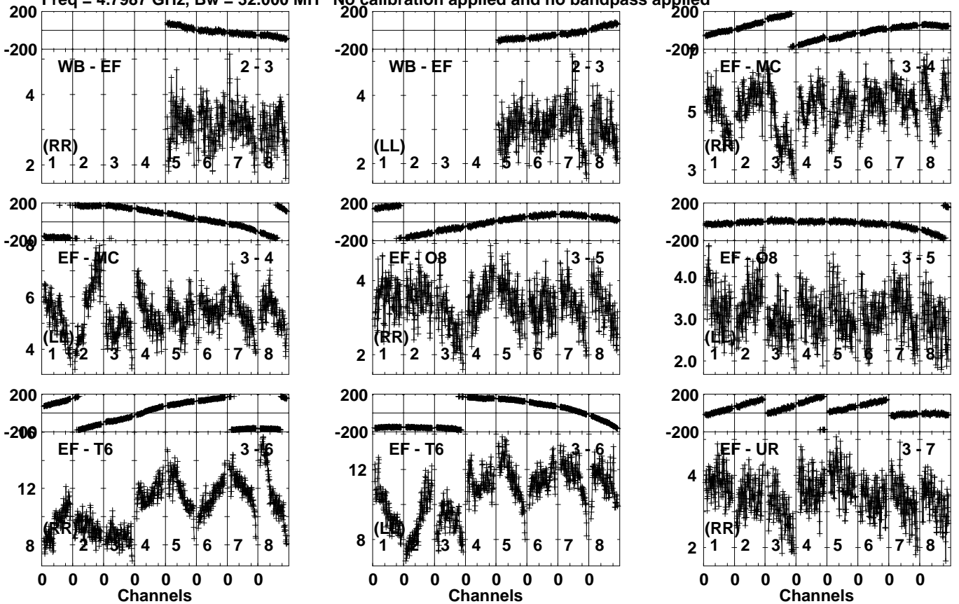
Lower frame: Milli Ampl Jy Top frame: Phas deg Vector averaged cross-power spectrum Several baselines displayed Timerange: 00/16:49:31 to 00/16:50:29
