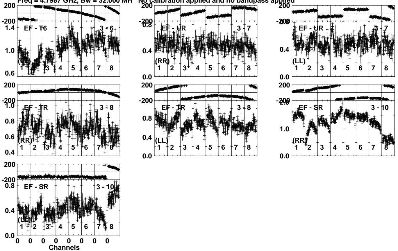
Lower frame: Milli Ampl Jy Top frame: Phas deg Vector averaged cross-power spectrum Several baselines displayed Timerange: 00/16:25:41 to 00/16:29:19
