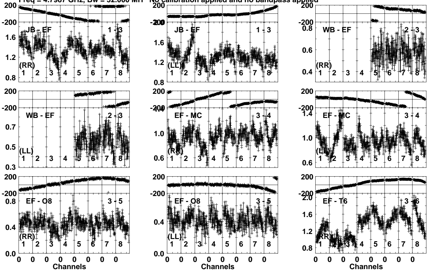
Lower frame: Milli Ampl Jy Top frame: Phas deg Vector averaged cross-power spectrum Several baselines displayed Timerange: 00/18:06:51 to 00/18:10:39
