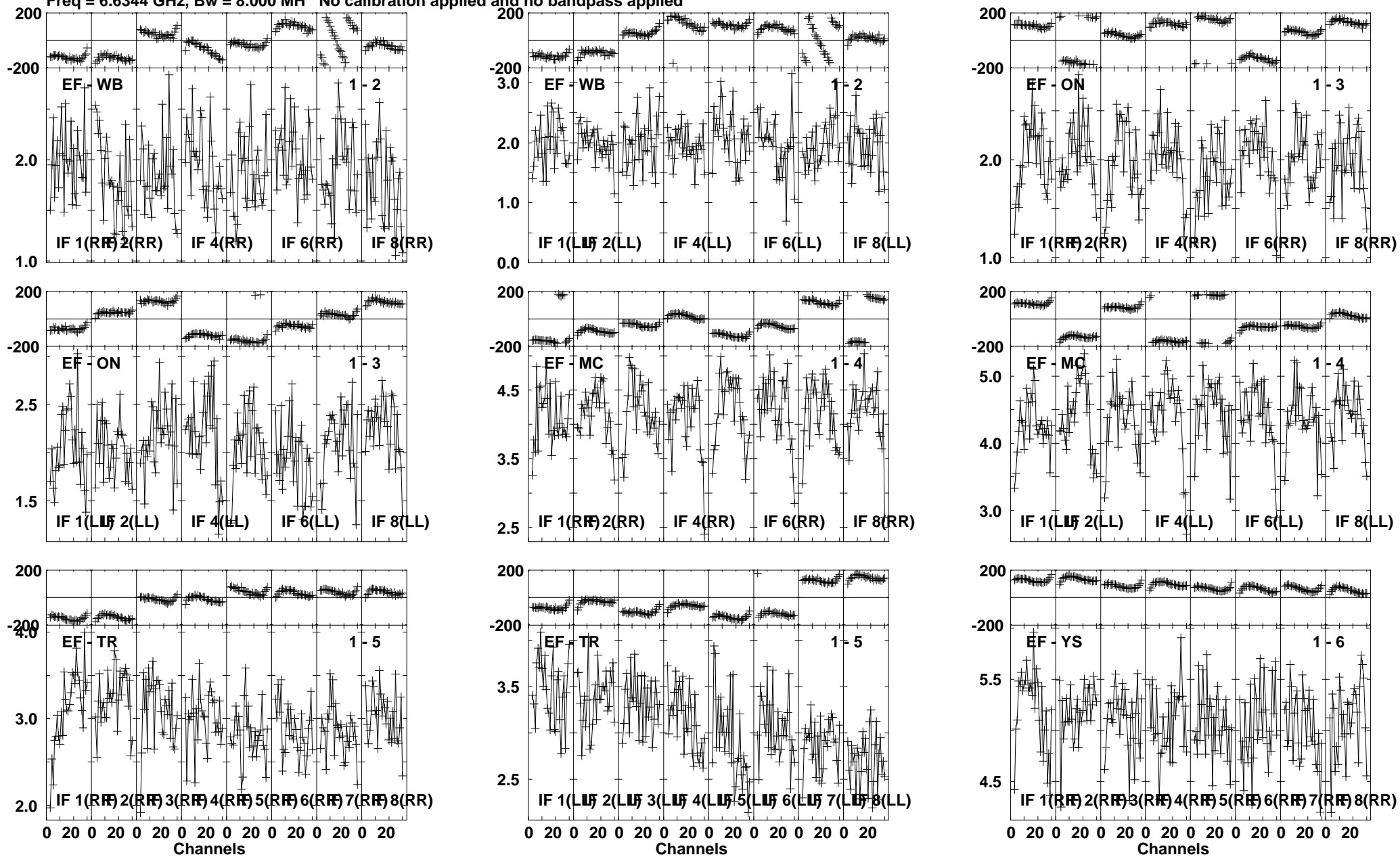
Lower frame: Milli Ampl Jy Top frame: Phas deg Vector averaged cross-power spectrum Several baselines displayed Timerange: 01/02:45:33 to 01/02:47:01
