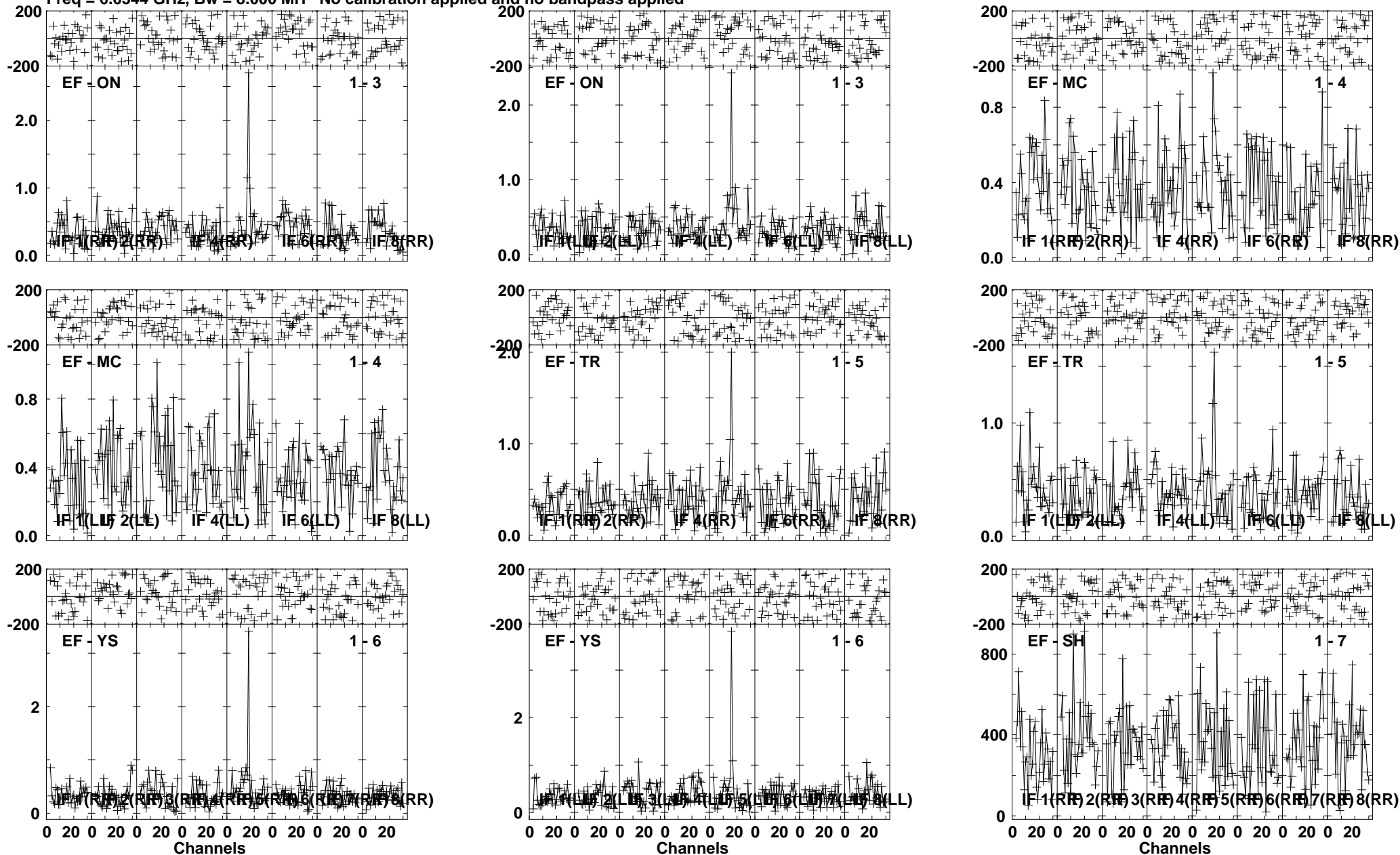
Lower frame: Milli Ampl Jy Top frame: Phas deg Vector averaged cross-power spectrum Several baselines displayed Timerange: 01/00:19:42 to 01/00:20:41
