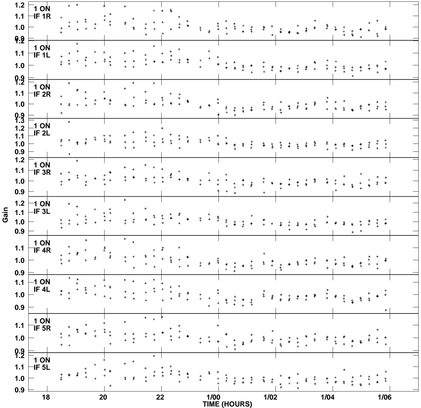
Plot file version 1 created 26-JUL-2013 10:38:48 Gain amp vs UTC time for J1125+2610.MULTI.1 SN 4 Rpol & Lpol IF 1 - 8
