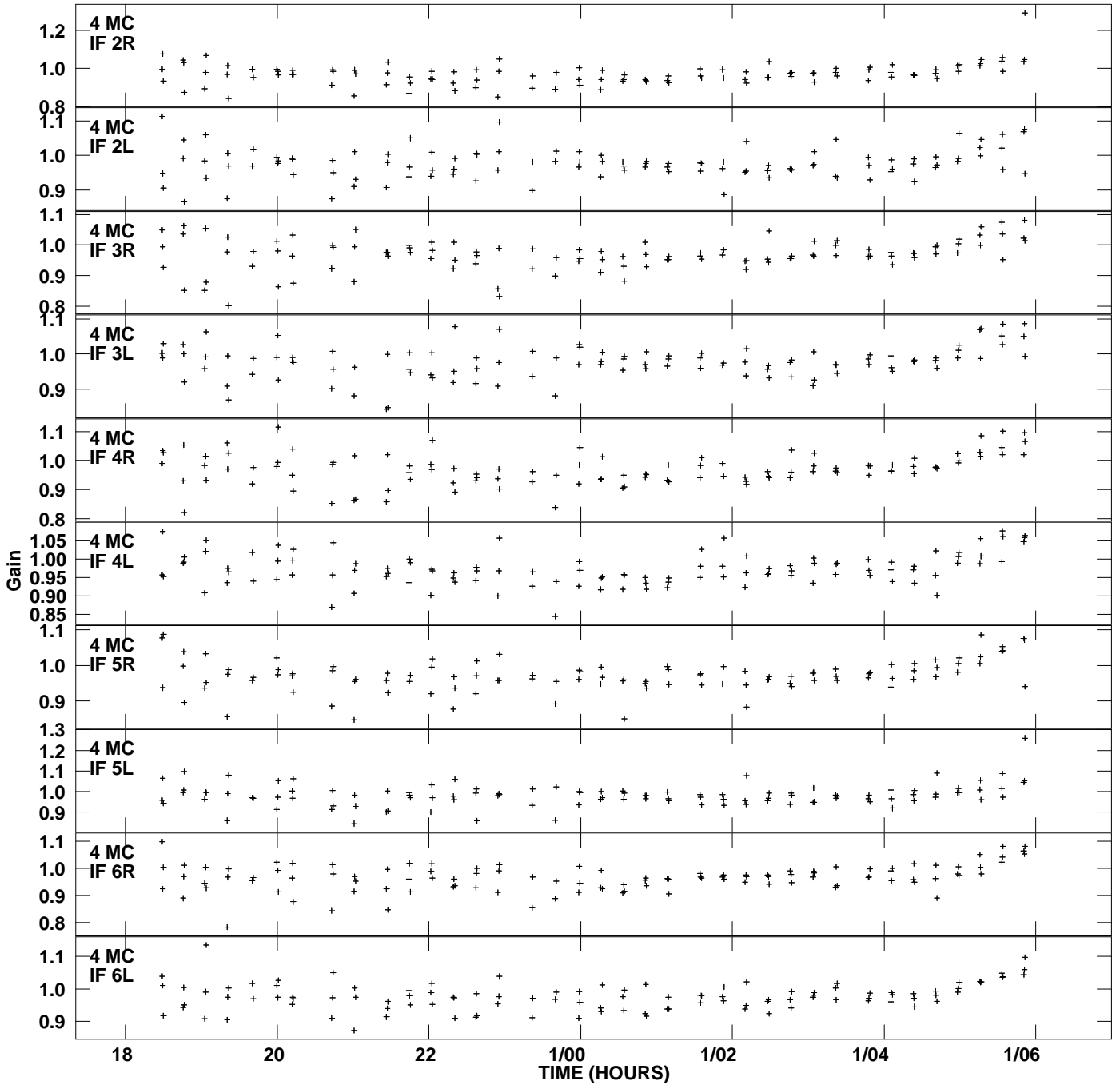
Plot file version 6 created 26-JUL-2013 10:38:48 Gain amp vs UTC time for J1125+2610.MULTI.1 SN 4 Rpol & Lpol IF 1 - 8
