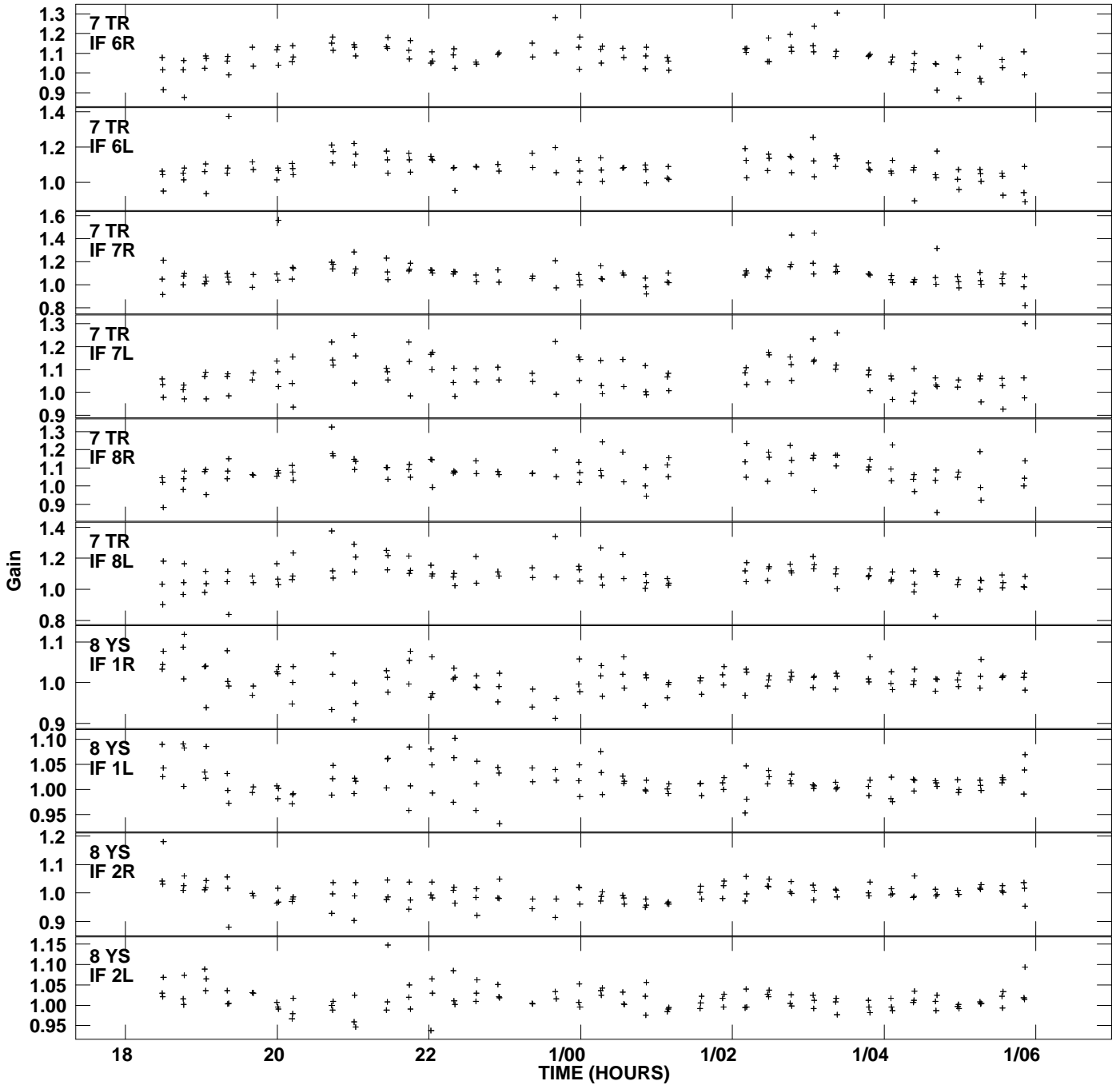
Plot file version 10 created 26-JUL-2013 10:38:48 Gain amp vs UTC time for J1125+2610.MULTI.1 SN 4 Rpol & Lpol IF 1 - 8
