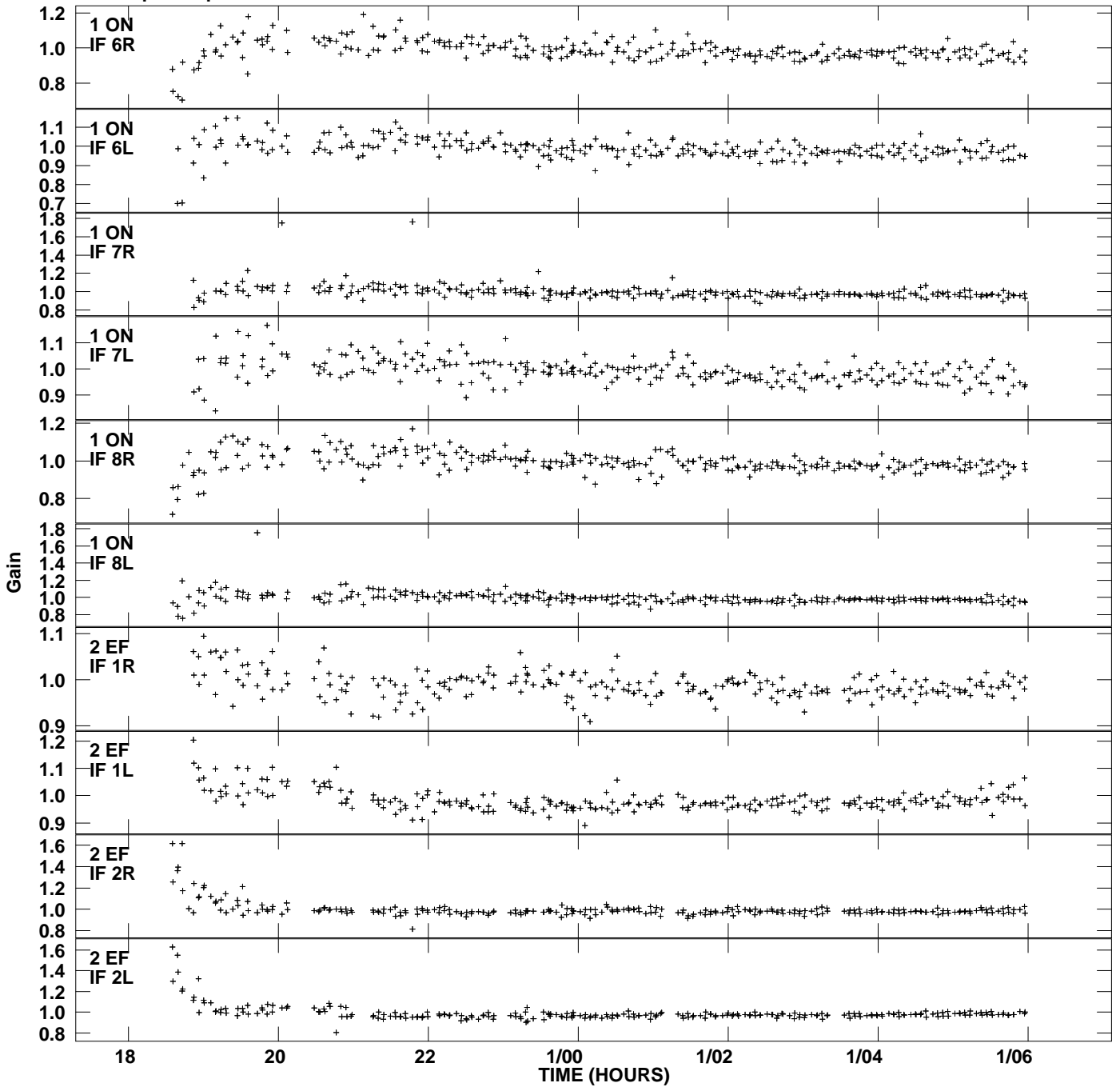
Plot file version 2 created 26-JUL-2013 10:37:47 Gain amp vs UTC time for J1157.MULTI.1 SN 4 Rpol & Lpol IF 1 - 8
