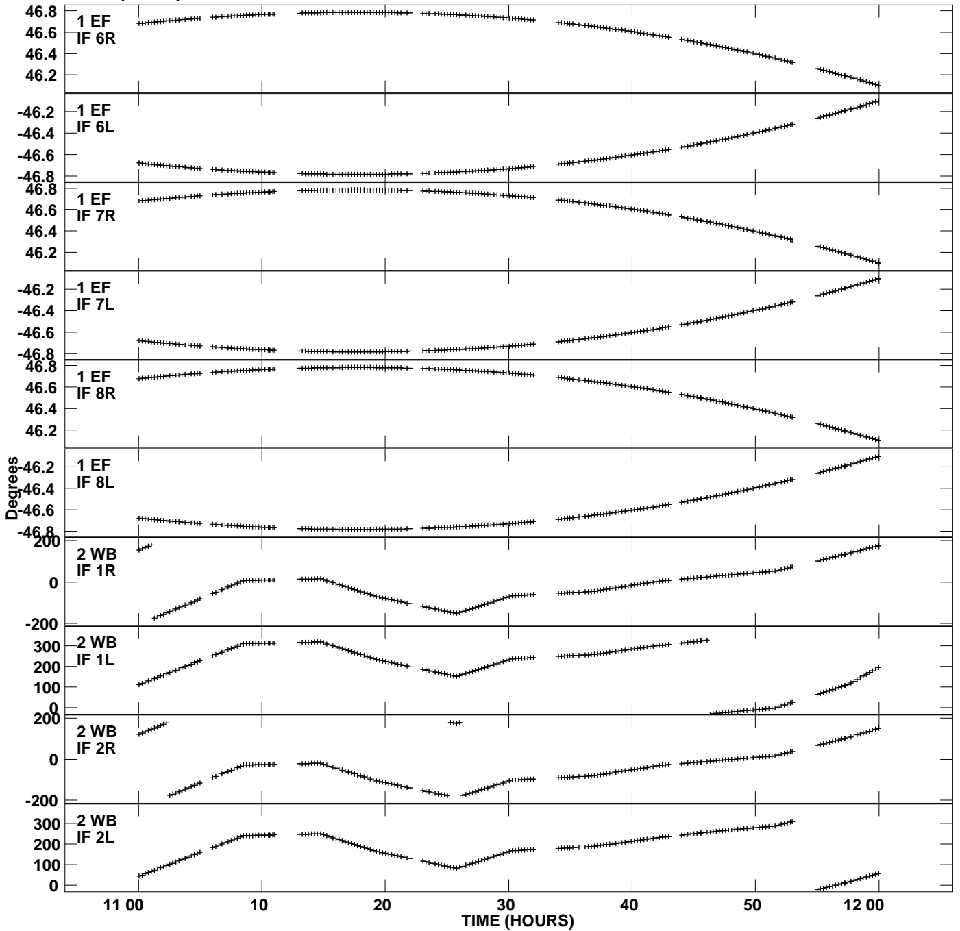
Plot file version 2 created 25-MAY-2012 00:44:04 Gain phs vs UTC time for F12L1.UVDATA.1 CL 3 Rpol & Lpol IF 1 - 8
