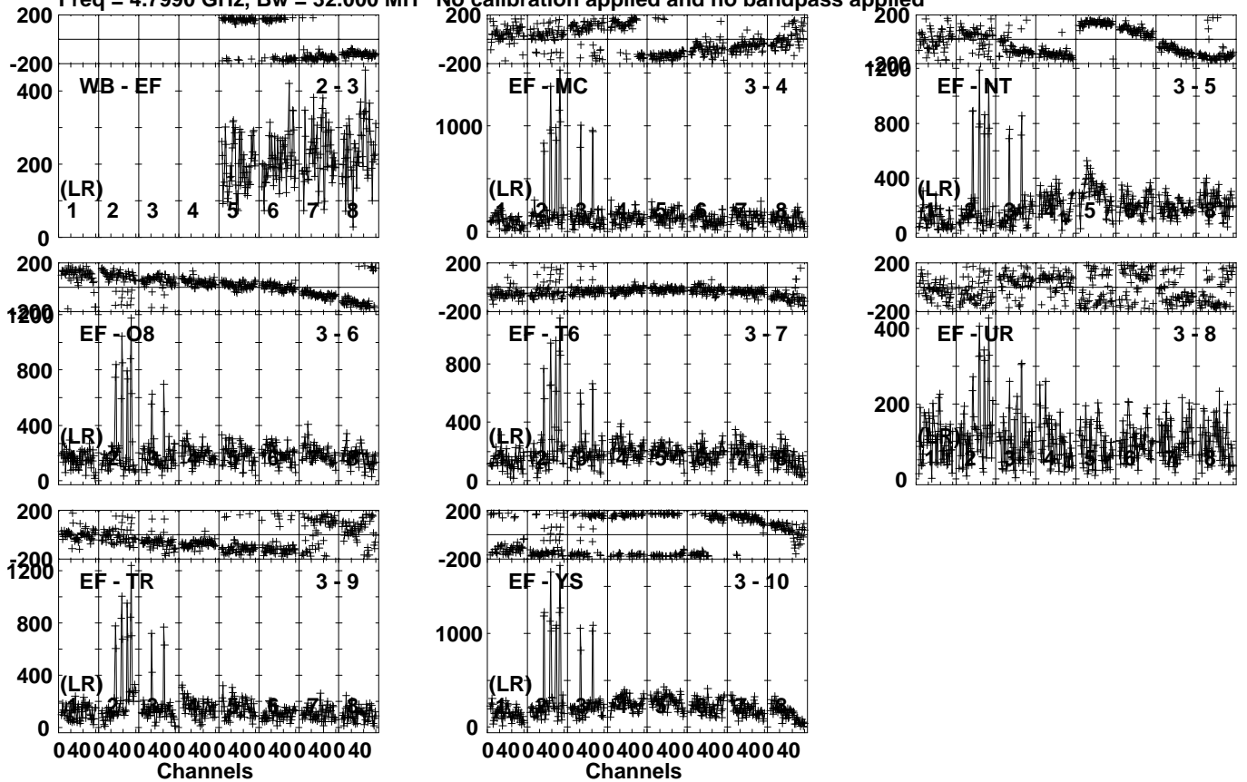
Lower frame: Micro Ampl Jy Top frame: Phas deg Vector averaged cross-power spectrum Several baselines displayed Timerange: 00/08:12:01 to 00/08:15:29
