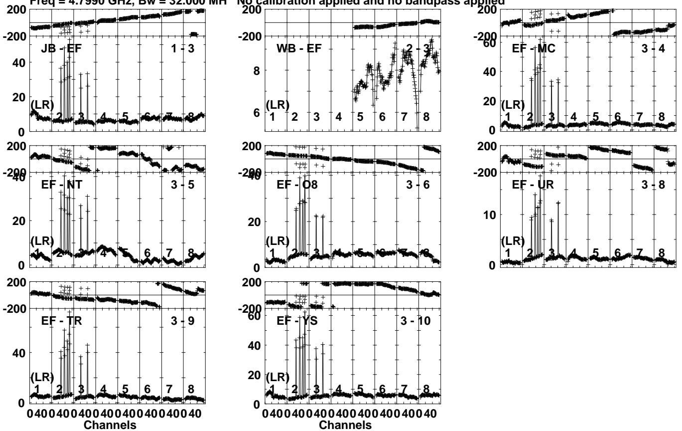
Lower frame: Milli Ampl Jy Top frame: Phas deg Vector averaged cross-power spectrum Several baselines displayed Timerange: 00/10:55:31 to 00/10:59:59
