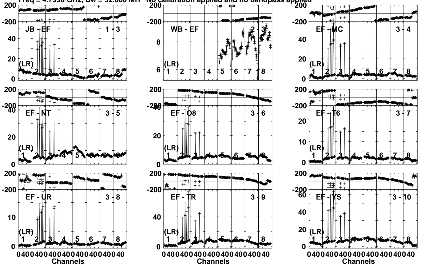
Lower frame: Milli Ampl Jy Top frame: Phas deg Vector averaged cross-power spectrum Several baselines displayed Timerange: 00/09:05:31 to 00/09:07:29
