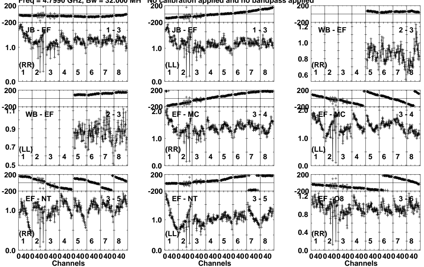
Lower frame: Milli Ampl Jy Top frame: Phas deg Vector averaged cross-power spectrum Several baselines displayed Timerange: 00/09:18:31 to 00/09:21:59
