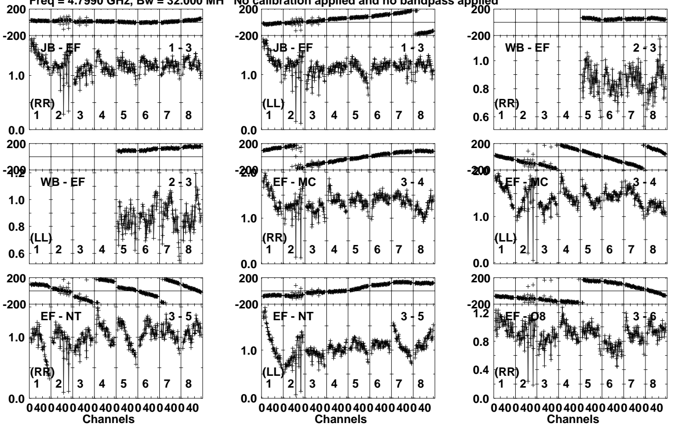
Lower frame: Milli Ampl Jy Top frame: Phas deg Vector averaged cross-power spectrum Several baselines displayed Timerange: 00/09:24:01 to 00/09:27:29
