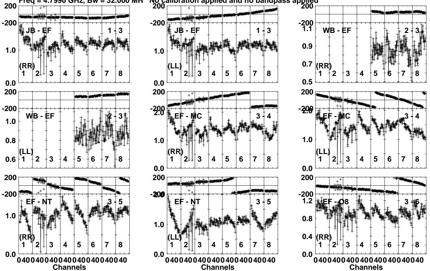
Lower frame: Milli Ampl Jy Top frame: Phas deg Vector averaged cross-power spectrum Several baselines displayed Timerange: 00/09:13:01 to 00/09:16:29
