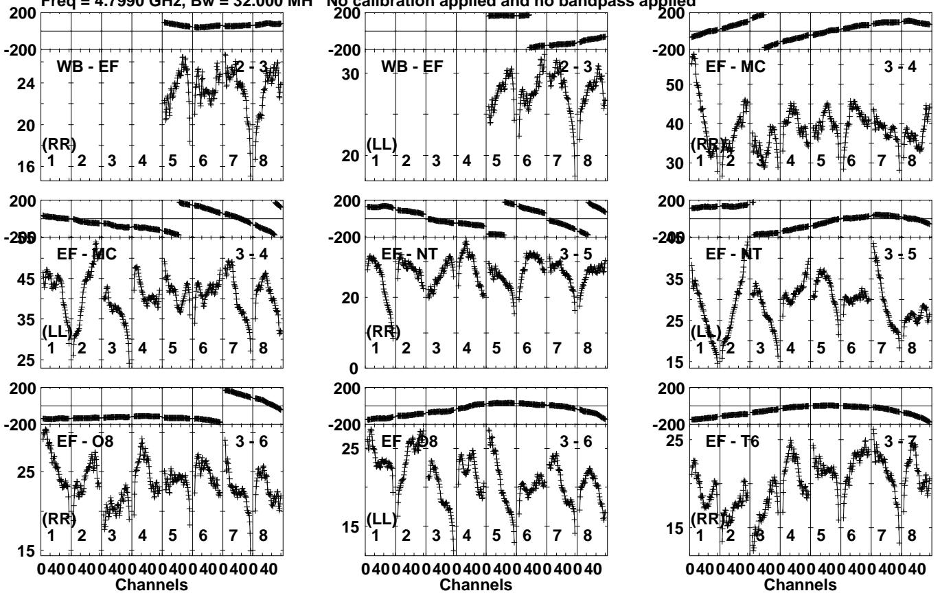
Lower frame: Milli Ampl Jy Top frame: Phas deg Vector averaged cross-power spectrum Several baselines displayed Timerange: 00/06:42:01 to 00/06:45:17
