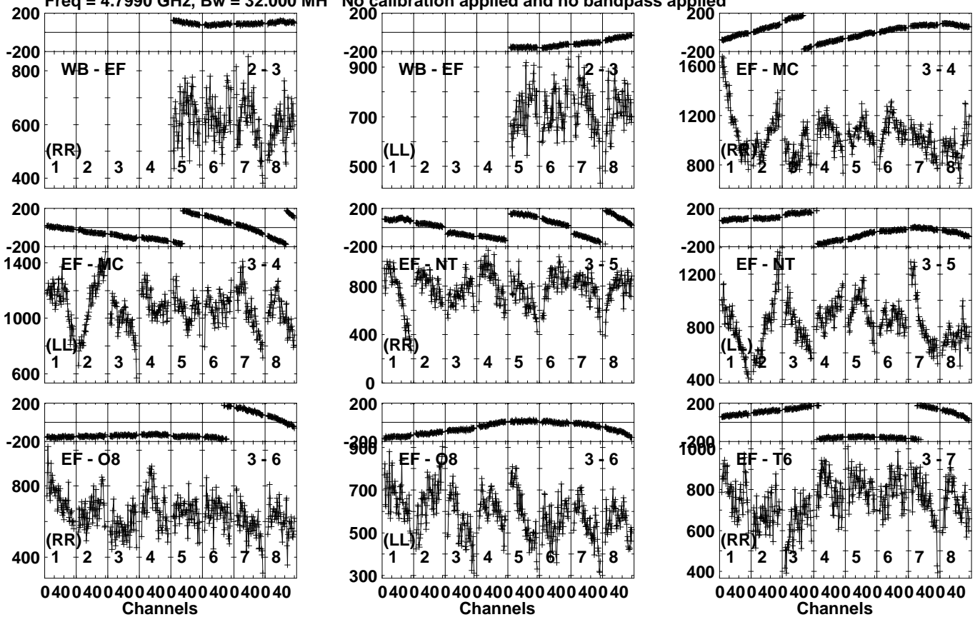
Lower frame: Micro Ampl Jy Top frame: Phas deg Vector averaged cross-power spectrum Several baselines displayed Timerange: 00/06:38:01 to 00/06:41:29
