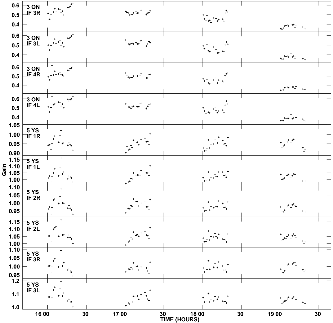
Plot file version 3 created 22-NOV-2011 14:59:57 Gain amp vs UTC time for 3C345.MULTI.1 SN 2 Rpol & Lpol IF 1 - 4
