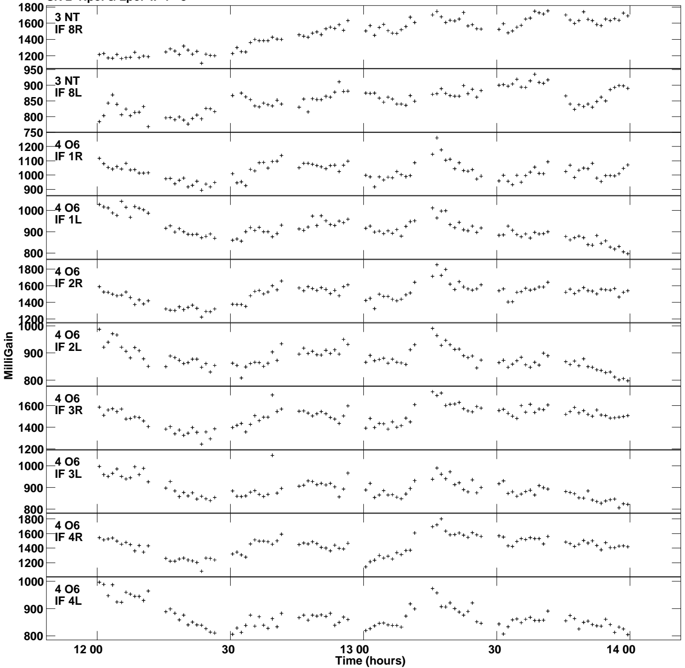
Plot file version 4 created 21-MAY-2021 14:27:24 Gain amp vs UTC time for 0528+134.MULTI.1 SN 2 Rpol & Lpol IF 1 - 8
