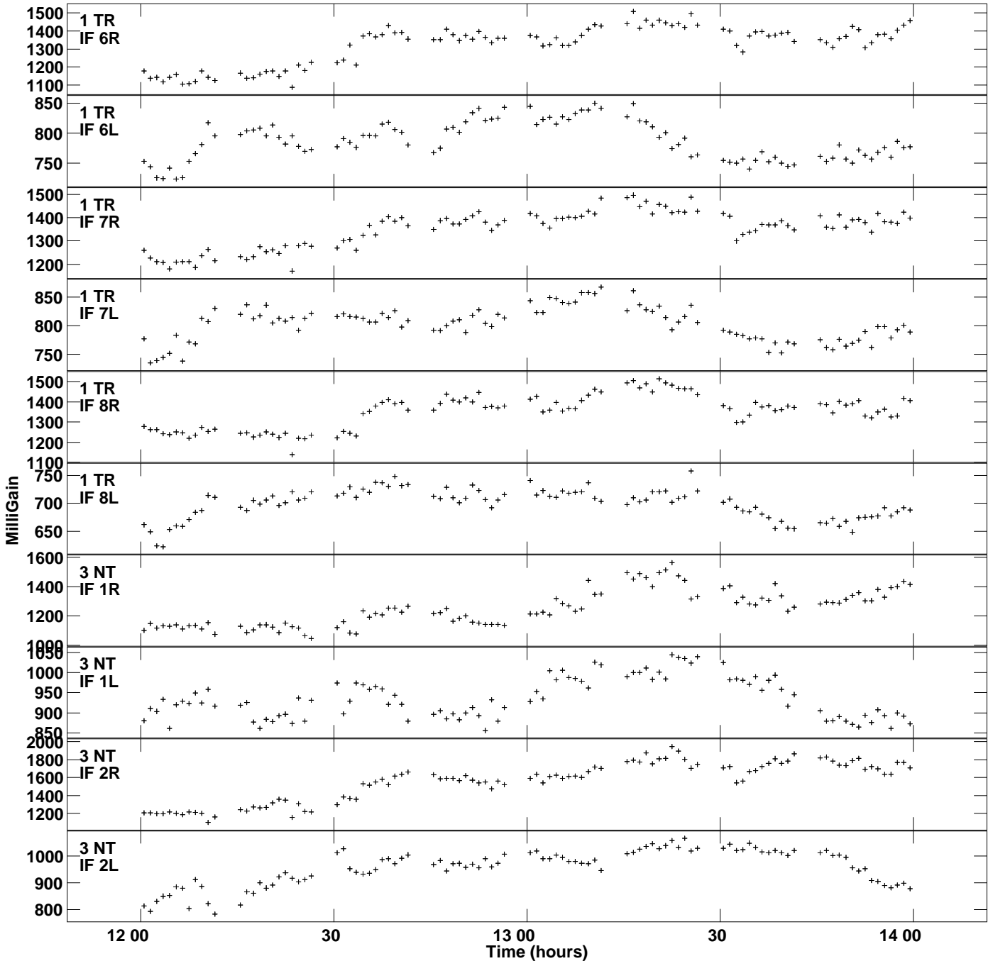
Plot file version 2 created 21-MAY-2021 14:27:24 Gain amp vs UTC time for 0528+134.MULTI.1 SN 2 Rpol & Lpol IF 1 - 8
