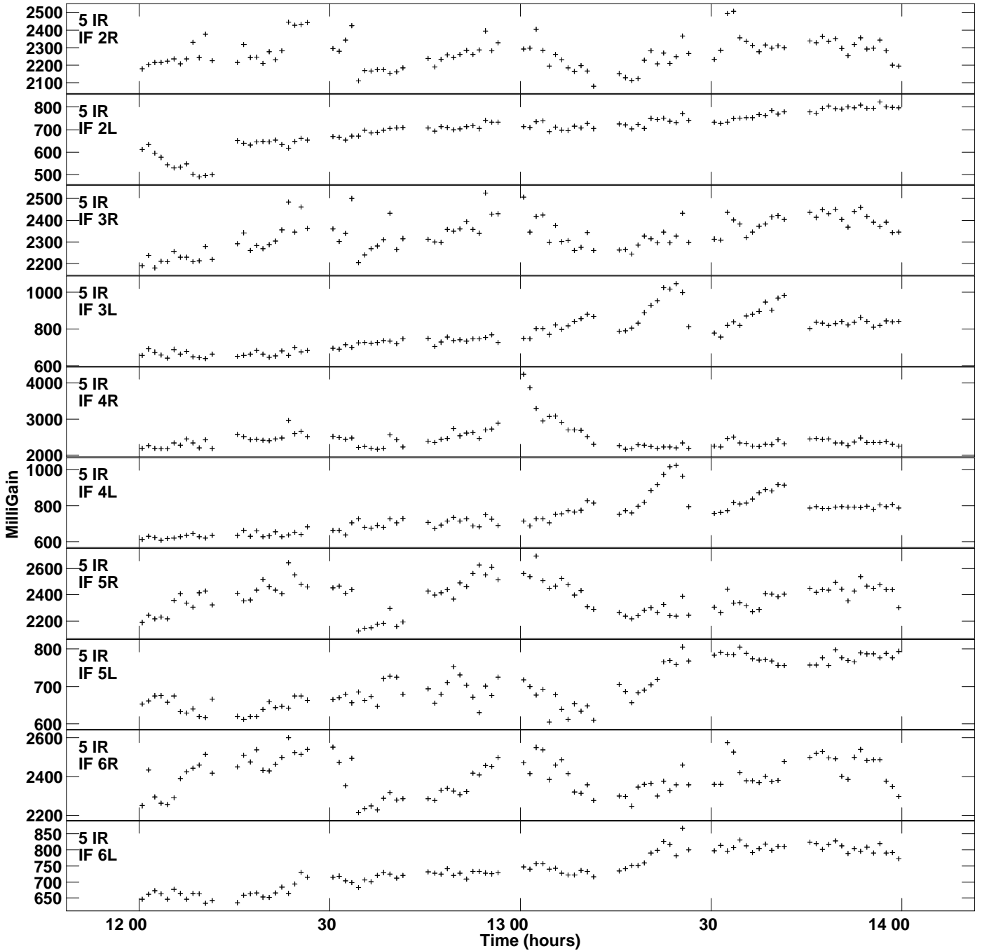
Plot file version 6 created 21-MAY-2021 14:27:24 Gain amp vs UTC time for 0528+134.MULTI.1 SN 2 Rpol & Lpol IF 1 - 8
