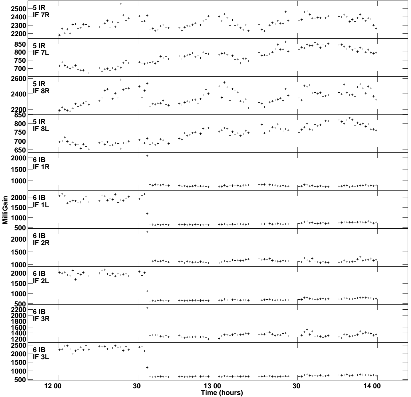
Plot file version 7 created 21-MAY-2021 14:27:24 Gain amp vs UTC time for 0528+134.MULTI.1 SN 2 Rpol & Lpol IF 1 - 8
