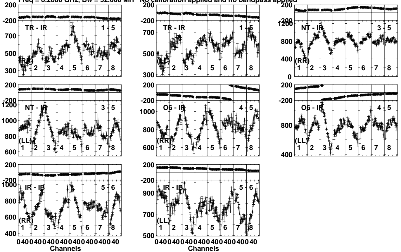
Lower frame: Micro Ampl Jy Top frame: Phas deg Vector averaged cross-power spectrum Several baselines displayed Timerange: 00/12:45:01 to 00/12:56:59
