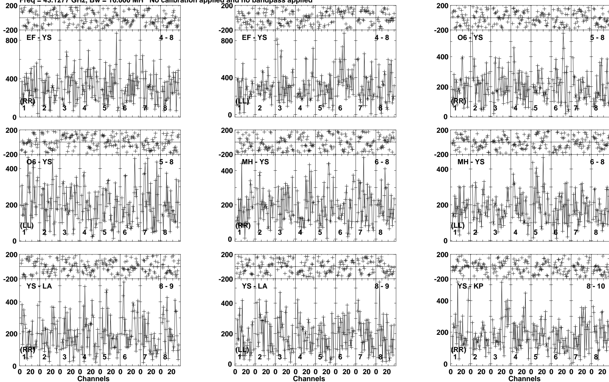
Lower frame: Micro Ampl Jy Top frame: Phas deg Vector averaged cross-power spectrum Baseline: EF (04) - YS (08) Timerange: 00/16:47:54 to 00/16:48:34
