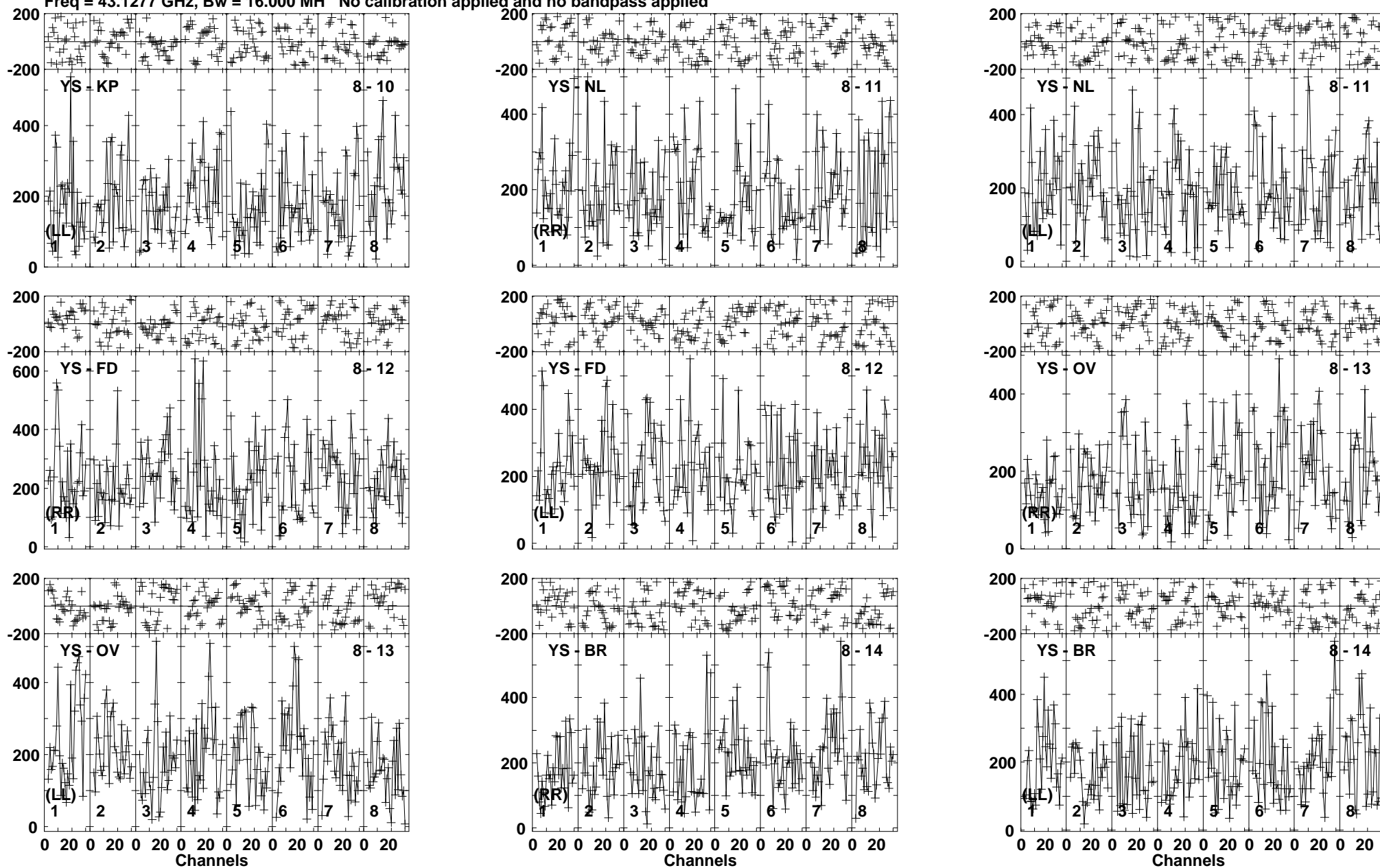
Lower frame: Micro Ampl Jy Top frame: Phas deg Vector averaged cross-power spectrum Baseline: YS (08) - KP (10) Timerange: 00/17:25:20 to 00/17:26:00
