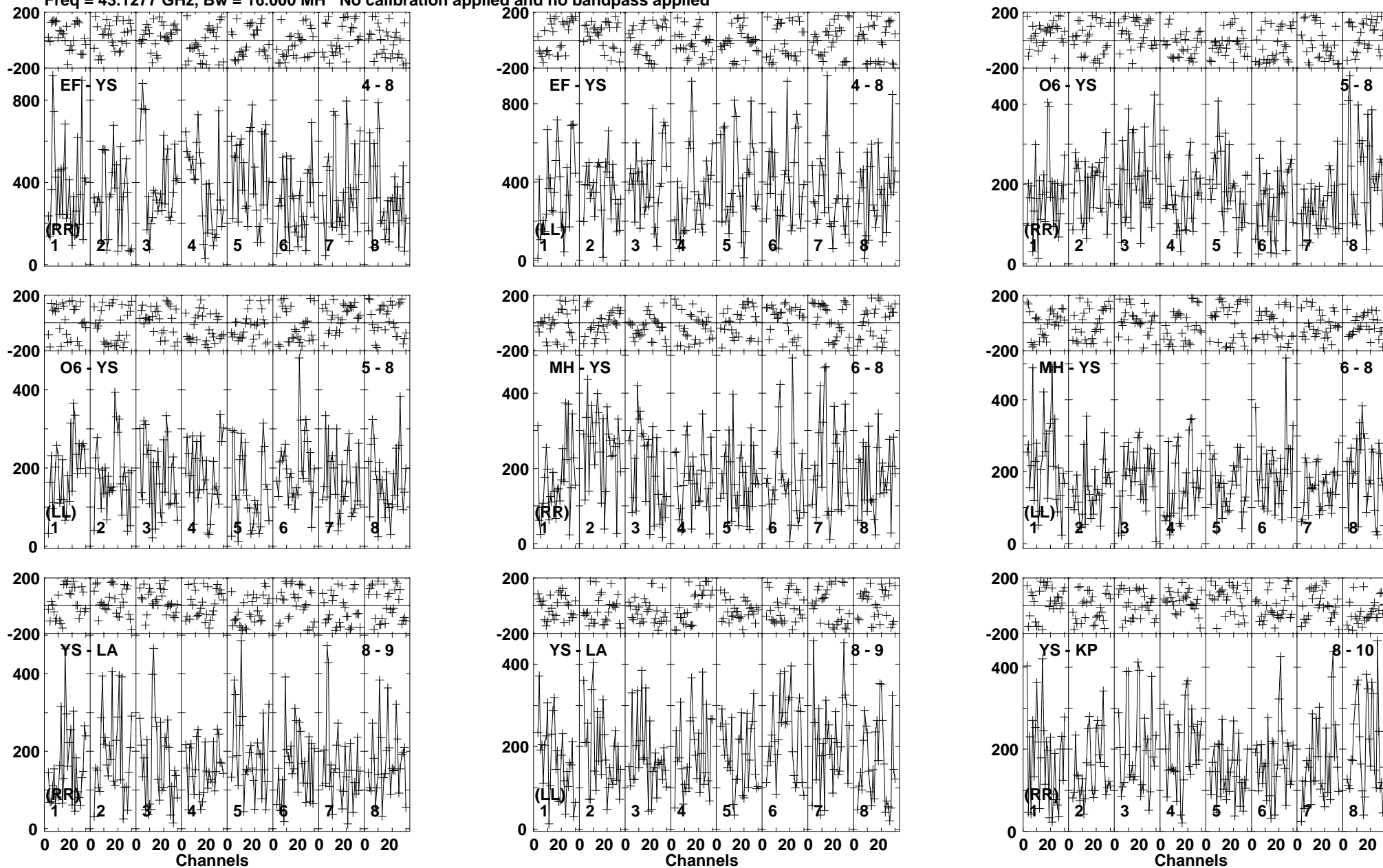
Lower frame: Micro Ampl Jy Top frame: Phas deg Vector averaged cross-power spectrum Baseline: EF (04) - YS (08) Timerange: 00/17:15:02 to 00/17:15:45
