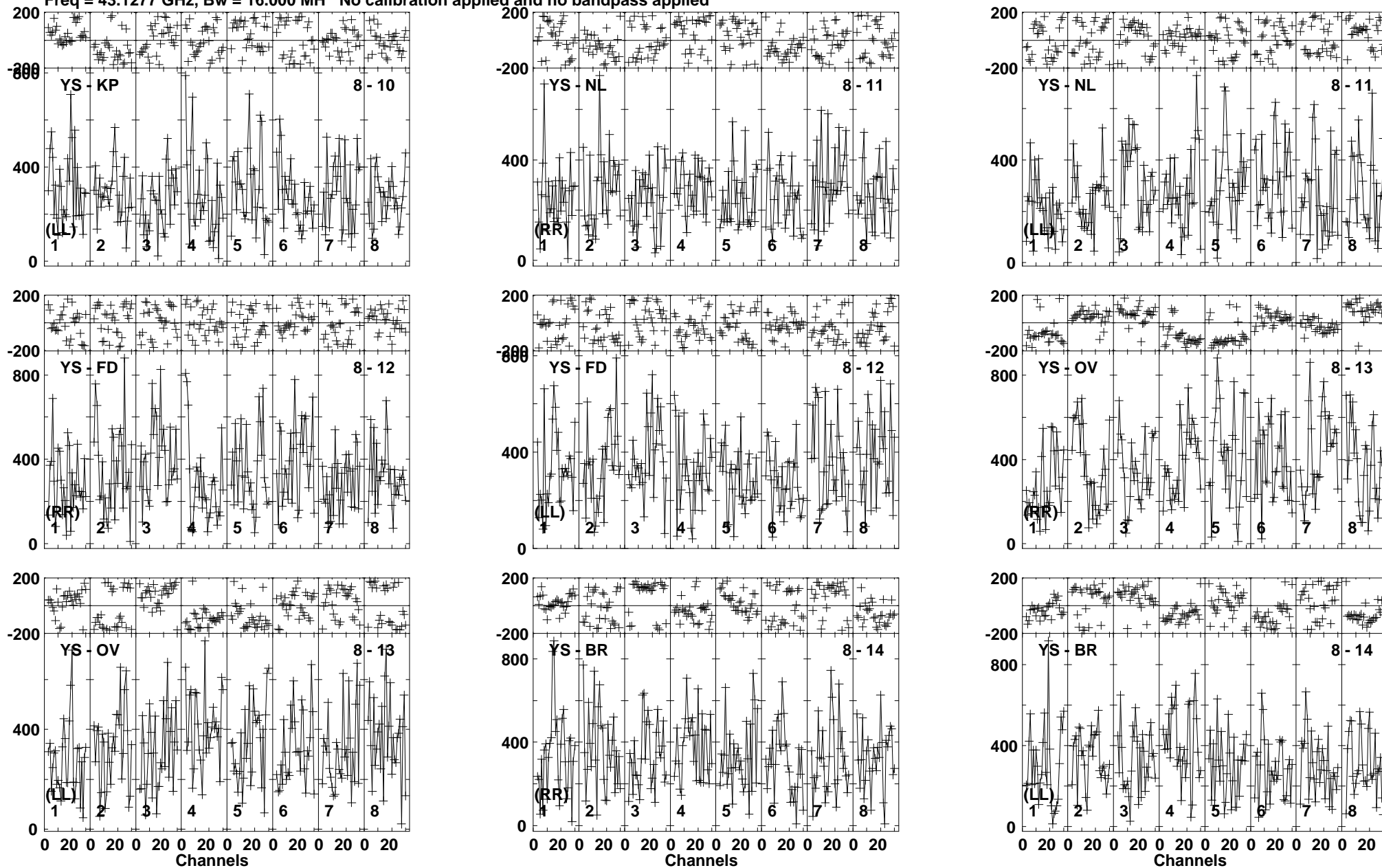
Lower frame: Micro Ampl Jy Top frame: Phas deg Vector averaged cross-power spectrum Baseline: YS (08) - KP (10) Timerange: 00/19:55:05 to 00/19:55:35
