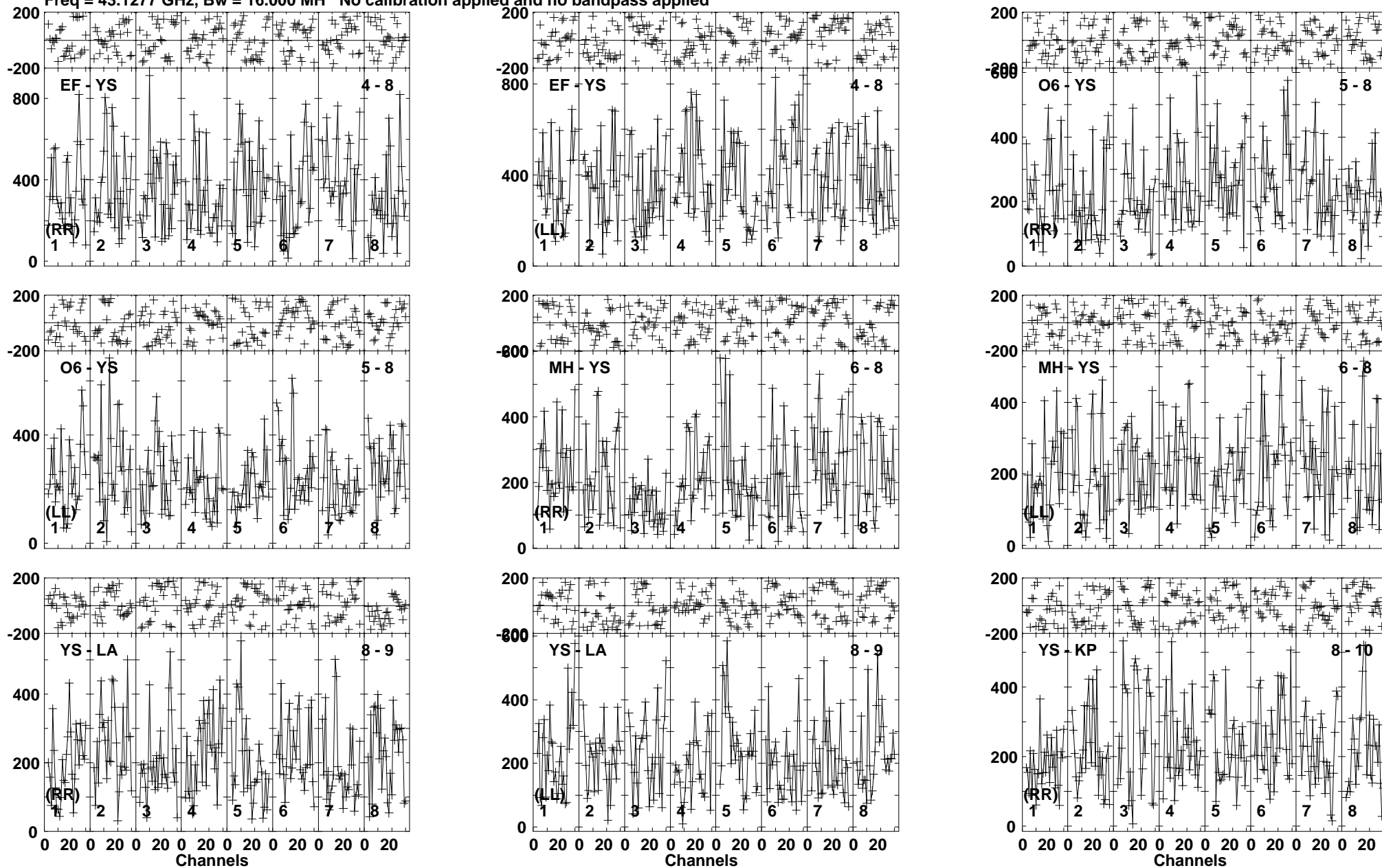
Lower frame: Micro Ampl Jy Top frame: Phas deg Vector averaged cross-power spectrum Baseline: EF (04) - YS (08) Timerange: 00/19:07:25 to 00/19:08:02
