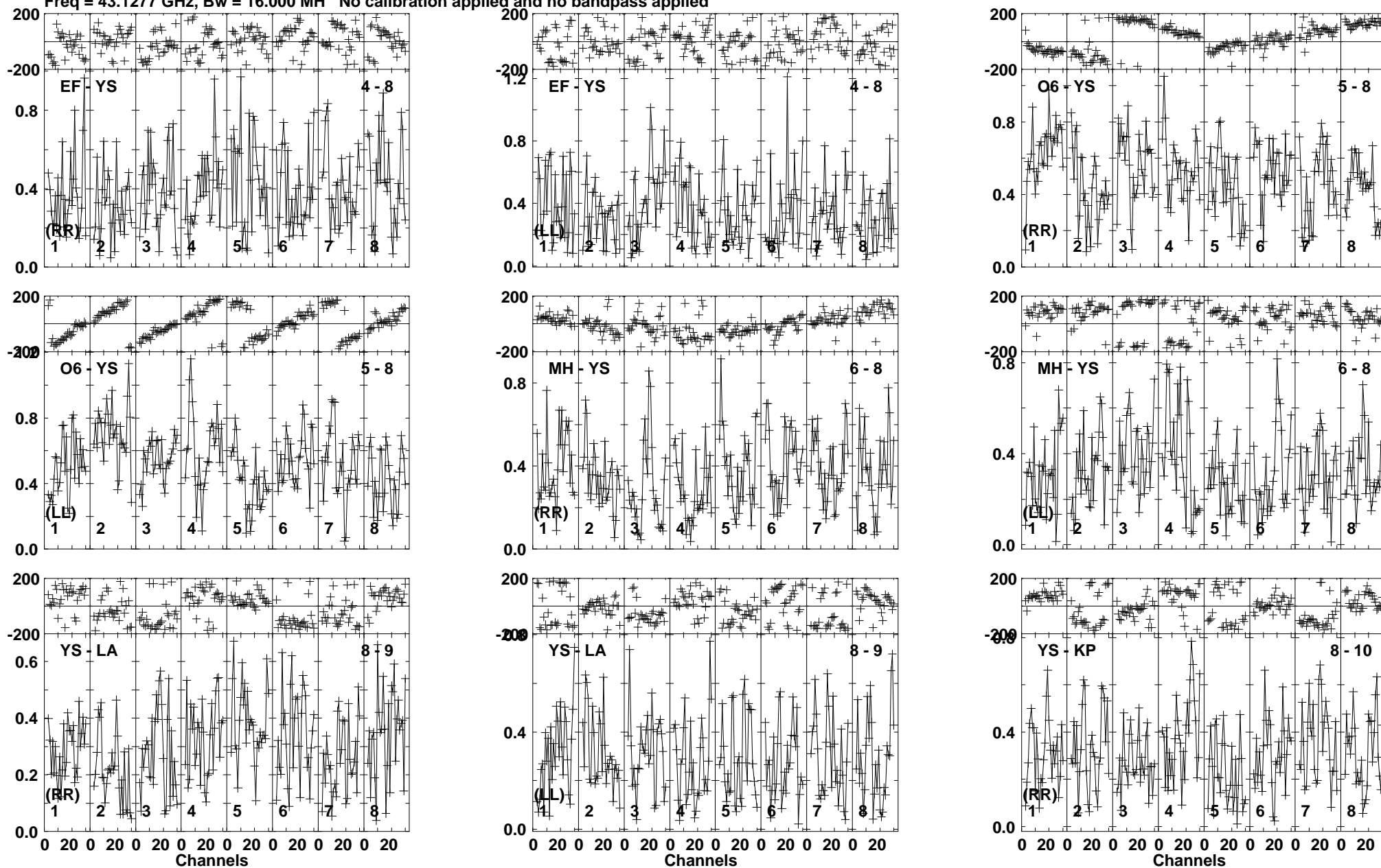
Lower frame: Milli Ampl Jy Top frame: Phas deg Vector averaged cross-power spectrum Baseline: EF (04) - YS (08) Timerange: 00/21:00:09 to 00/21:00:39
