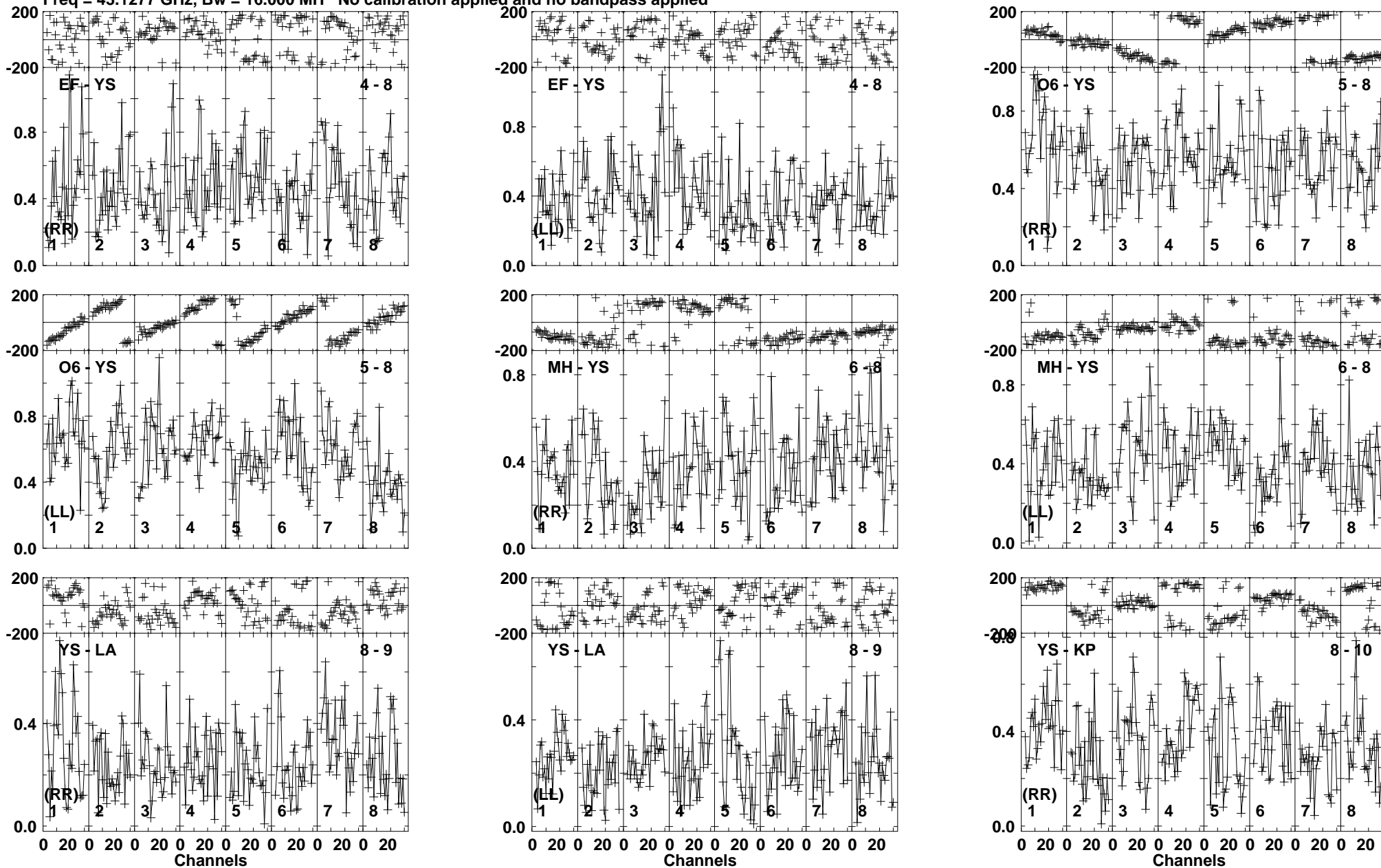
Lower frame: Milli Ampl Jy Top frame: Phas deg Vector averaged cross-power spectrum Baseline: EF (04) - YS (08) Timerange: 00/17:10:44 to 00/17:11:17
