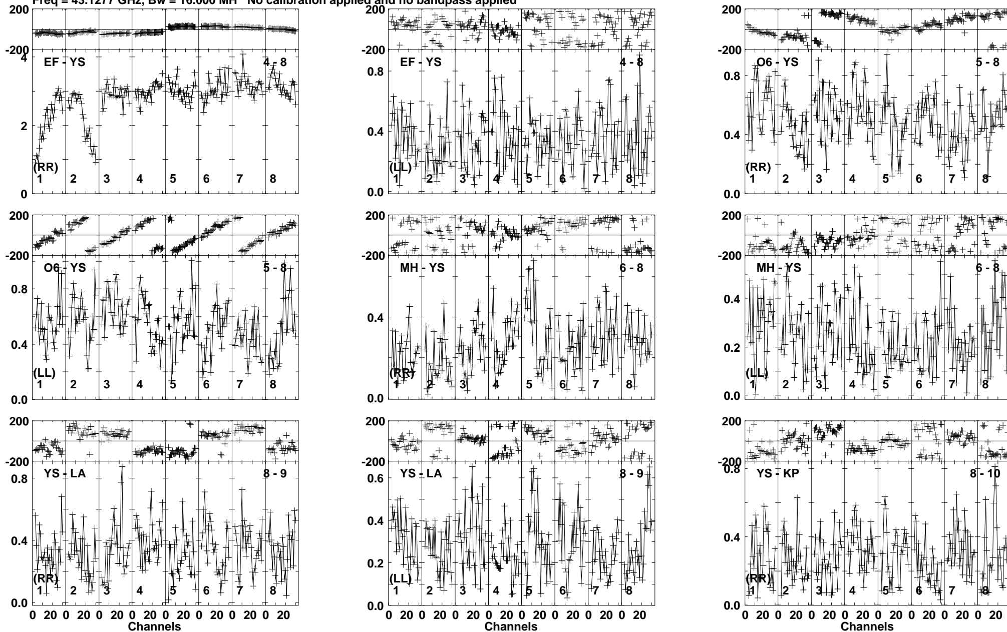
Lower frame: Milli Ampl Jy Top frame: Phas deg Vector averaged cross-power spectrum Baseline: EF (04) - YS (08) Timerange: 00/18:56:02 to 00/18:56:31
