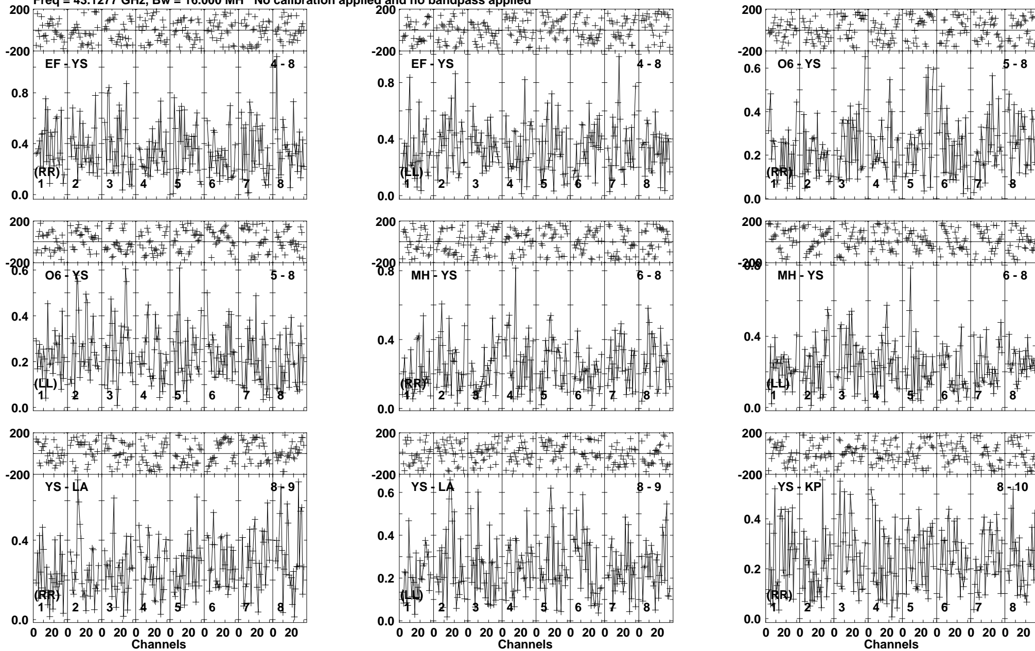
Lower frame: Milli Ampl Jy Top frame: Phas deg Vector averaged cross-power spectrum Baseline: EF (04) - YS (08) Timerange: 00/19:15:13 to 00/19:15:46
