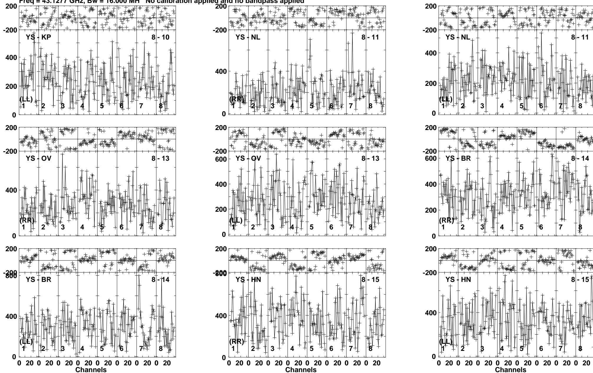
Lower frame: Micro Ampl Jy Top frame: Phas deg Vector averaged cross-power spectrum Baseline: YS (08) - KP (10) Timerange: 00/20:08:51 to 00/20:09:20
