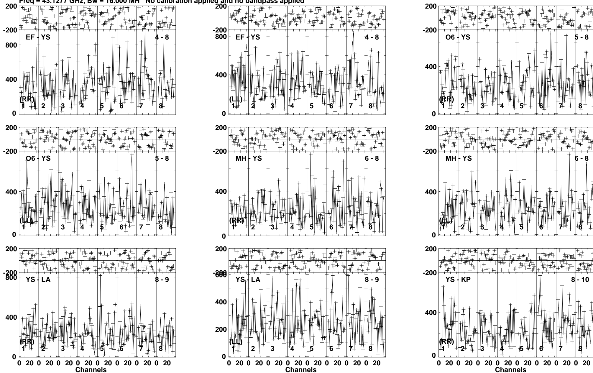
Lower frame: Micro Ampl Jy Top frame: Phas deg Vector averaged cross-power spectrum Baseline: EF (04) - YS (08) Timerange: 00/19:21:20 to 00/19:21:53
