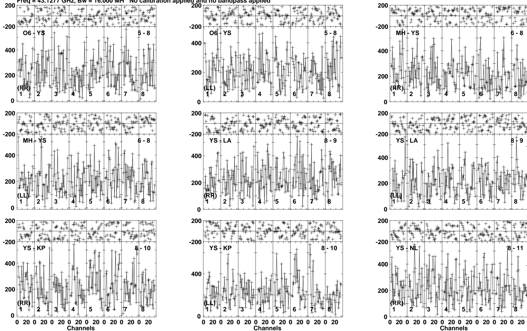
Lower frame: Micro Ampl Jy Top frame: Phas deg Vector averaged cross-power spectrum Baseline: O6 (05) - YS (08) Timerange: 00/17:52:06 to 00/17:52:41
