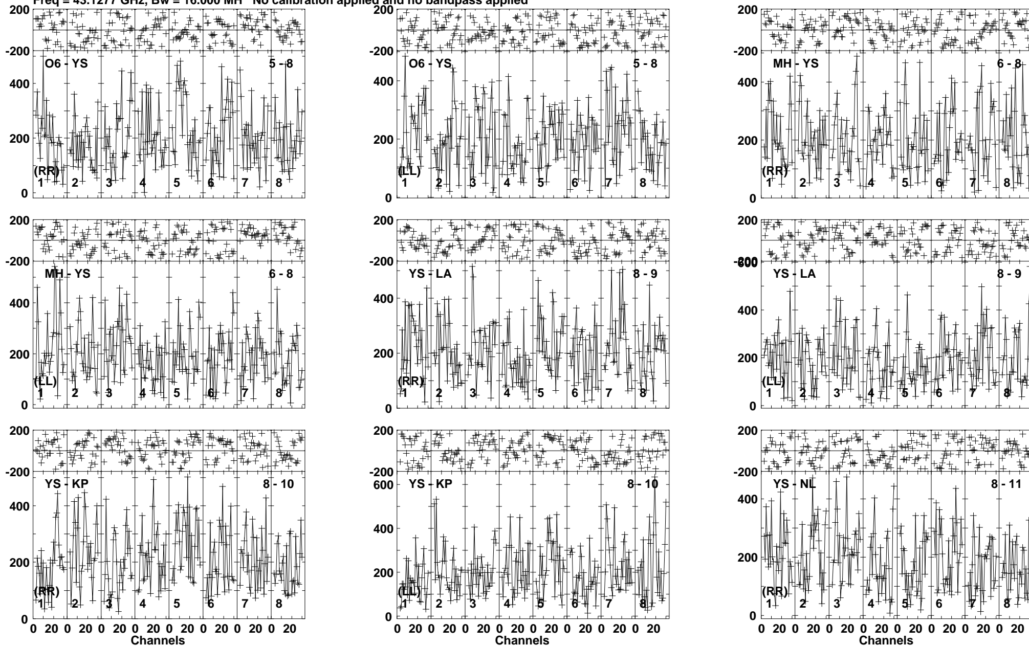
Lower frame: Micro Ampl Jy Top frame: Phas deg Vector averaged cross-power spectrum Baseline: O6 (05) - YS (08) Timerange: 00/17:50:23 to 00/17:51:02
