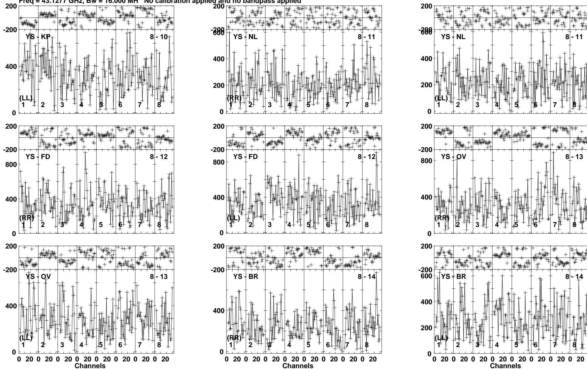
Lower frame: Micro Ampl Jy Top frame: Phas deg Vector averaged cross-power spectrum Baseline: YS (08) - KP (10) Timerange: 00/17:29:43 to 00/17:30:12
