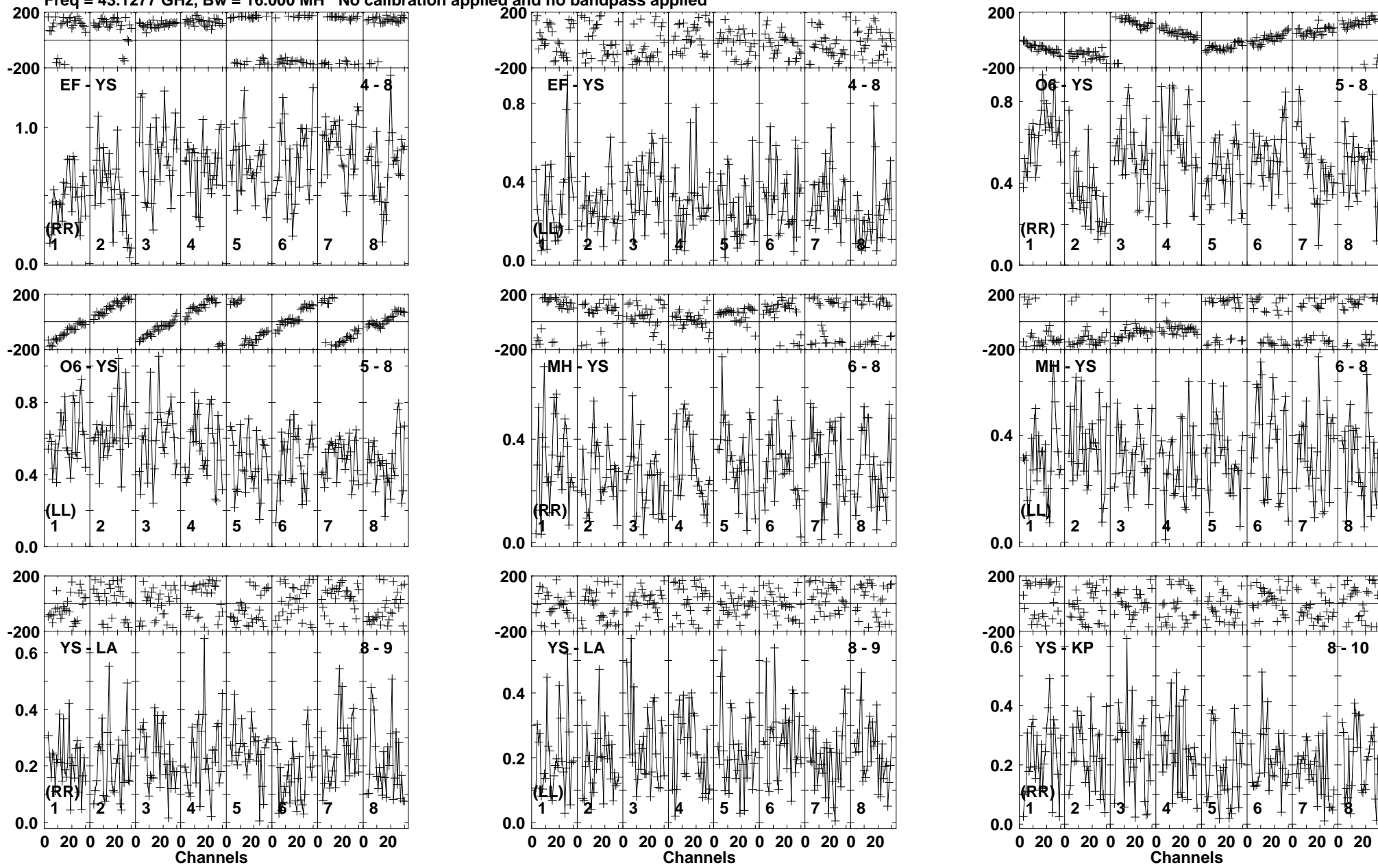
Lower frame: Milli Ampl Jy Top frame: Phas deg Vector averaged cross-power spectrum Baseline: EF (04) - YS (08) Timerange: 00/19:59:45 to 00/20:00:14
