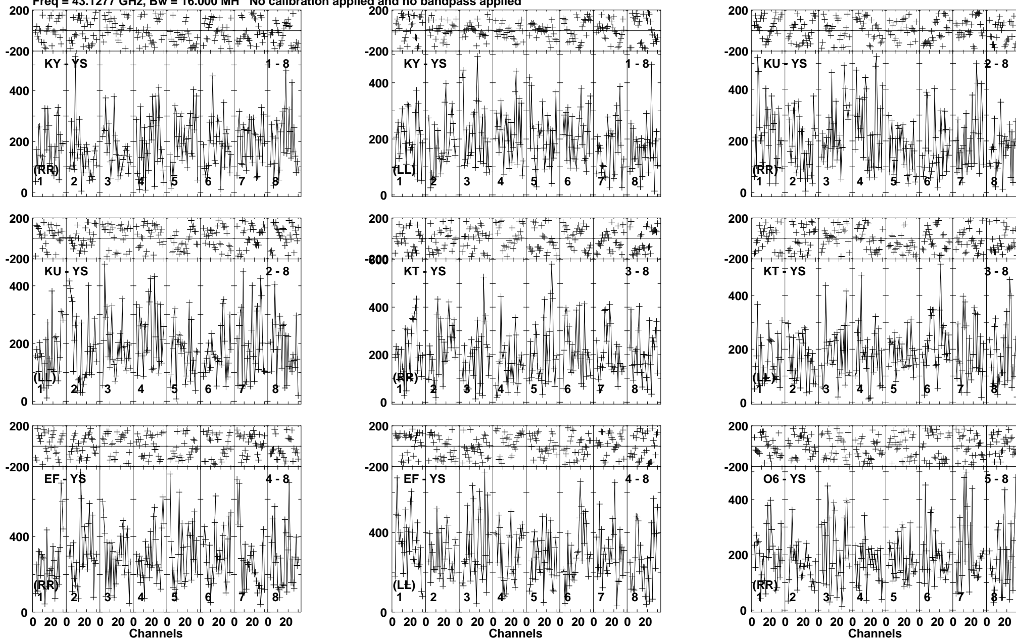
Lower frame: Micro Ampl Jy Top frame: Phas deg Vector averaged cross-power spectrum Baseline: KY (01) - YS (08) Timerange: 00/15:07:50 to 00/15:08:27
