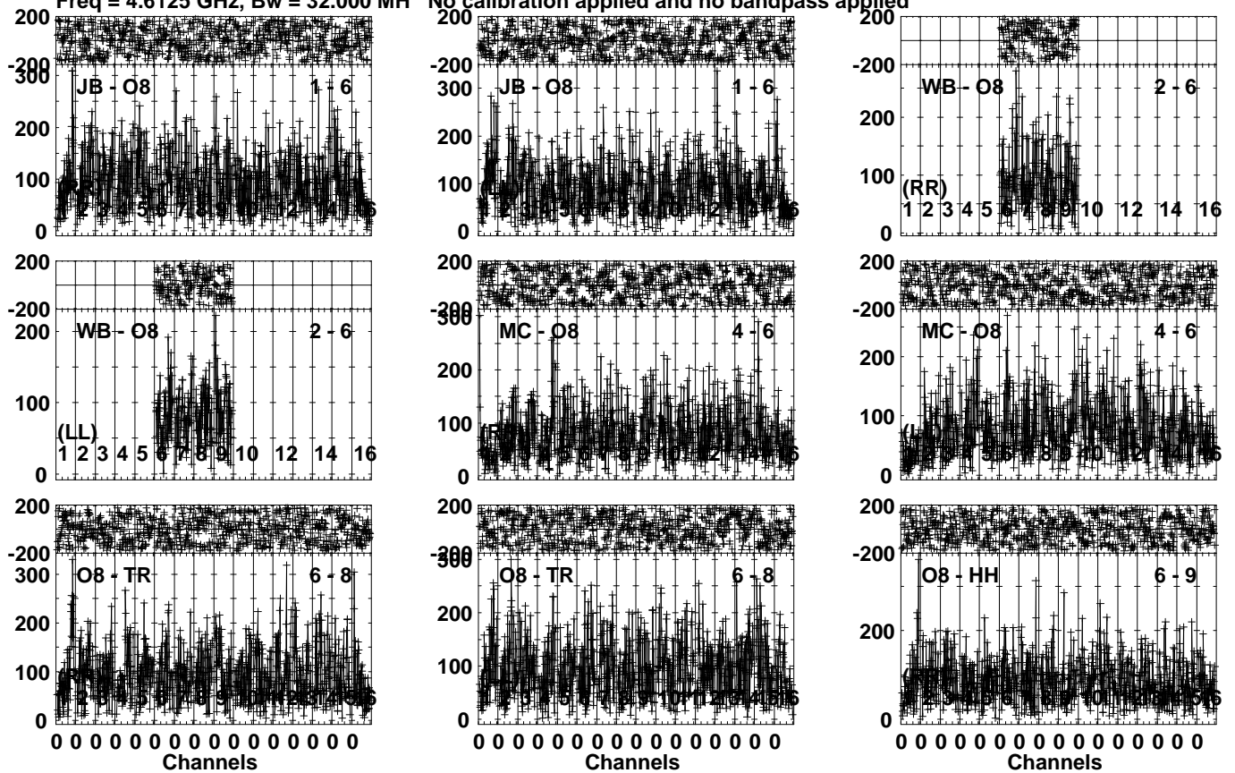
Lower frame: Micro Ampl Jy Top frame: Phas deg Vector averaged cross-power spectrum Several baselines displayed Timerange: 00/17:36:31 to 00/17:40:29
