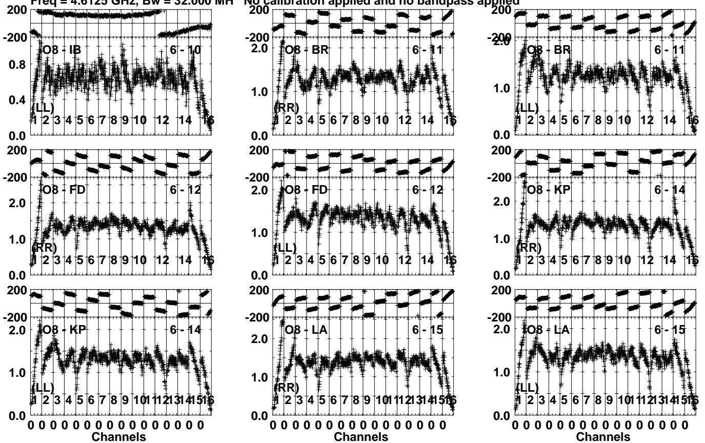
Lower frame: Milli Ampl Jy Top frame: Phas deg Vector averaged cross-power spectrum Several baselines displayed Timerange: 00/20:48:53 to 00/20:50:49
