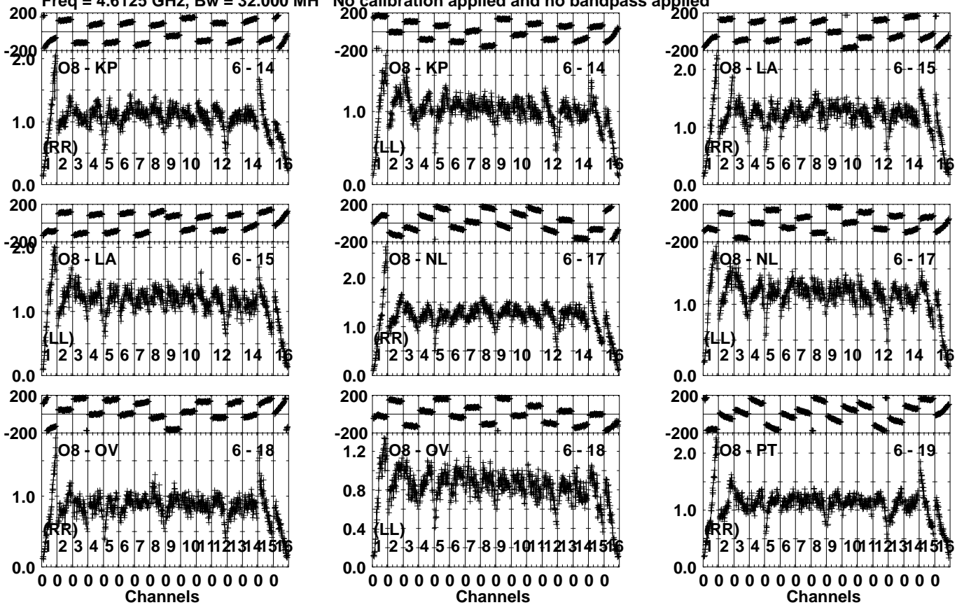
Lower frame: Milli Ampl Jy Top frame: Phas deg Vector averaged cross-power spectrum Several baselines displayed Timerange: 00/17:34:33 to 00/17:36:29
