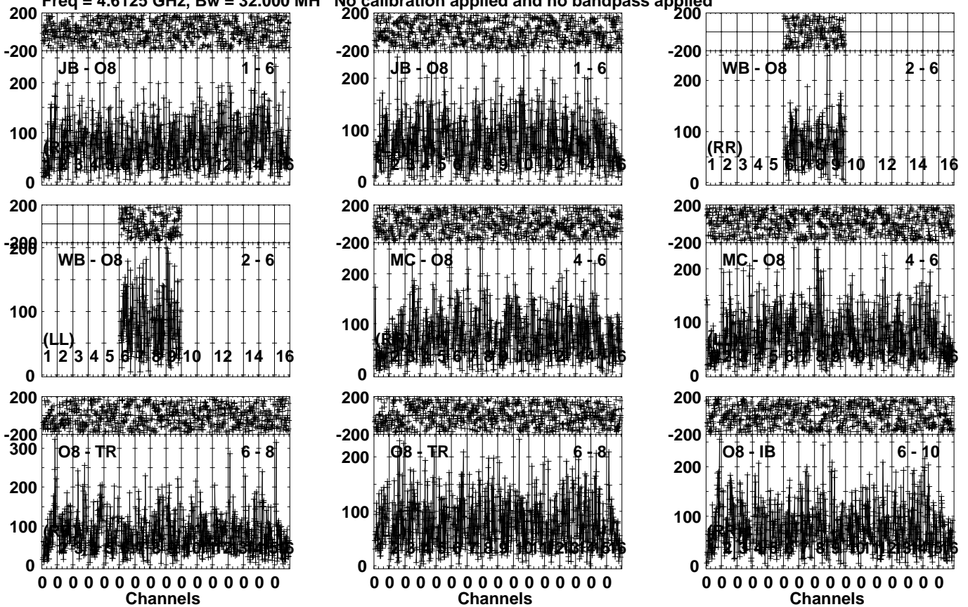
Lower frame: Micro Ampl Jy Top frame: Phas deg Vector averaged cross-power spectrum Several baselines displayed Timerange: 00/20:19:53 to 00/20:23:49
