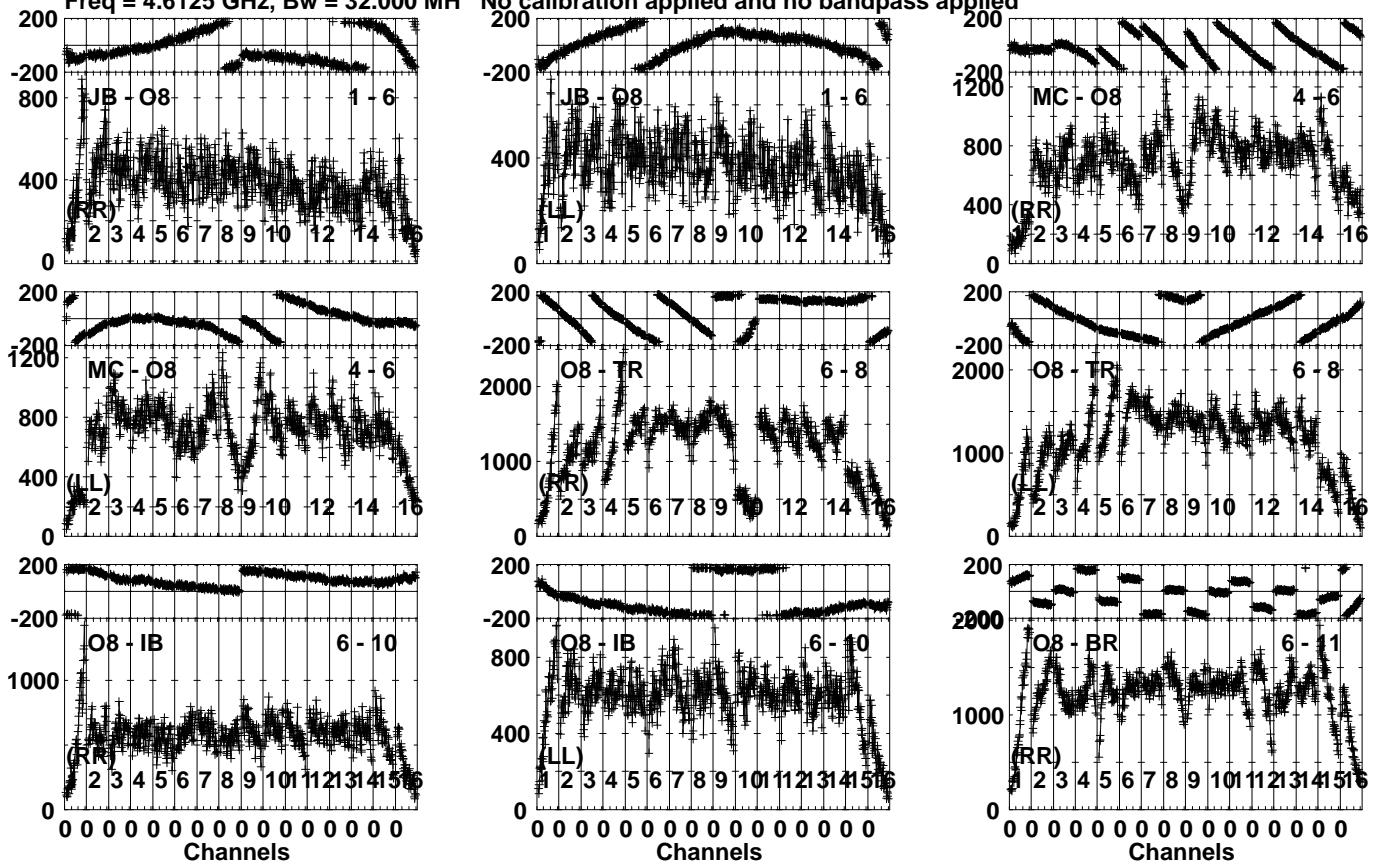
Lower frame: Micro Ampl Jy Top frame: Phas deg Vector averaged cross-power spectrum Several baselines displayed Timerange: 00/21:38:13 to 00/21:40:09
