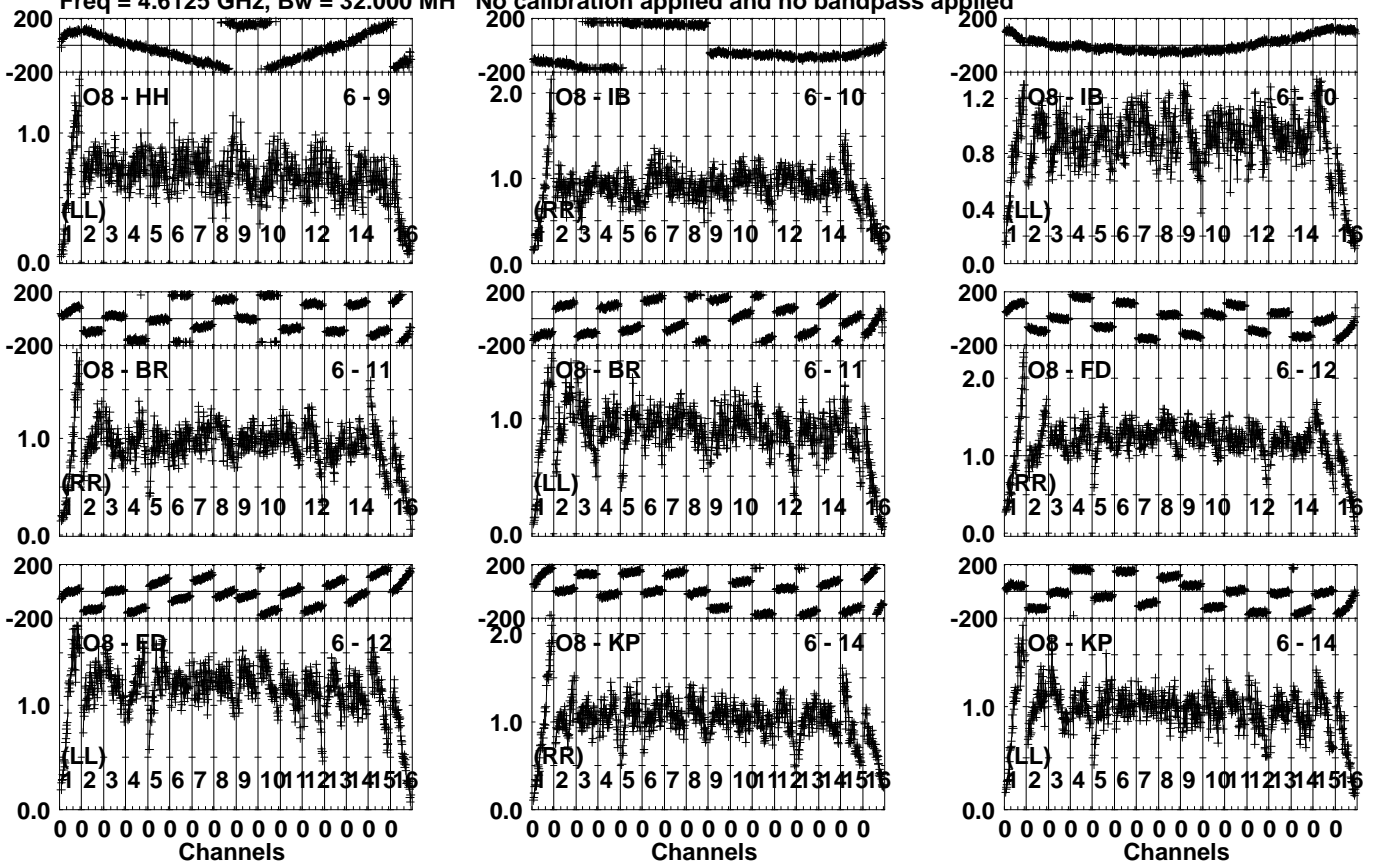
Lower frame: Milli Ampl Jy Top frame: Phas deg Vector averaged cross-power spectrum Several baselines displayed Timerange: 00/17:04:23 to 00/17:06:19
