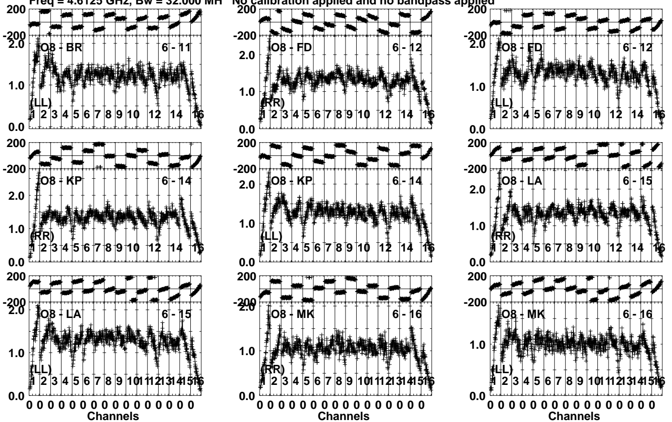
Lower frame: Milli Ampl Jy Top frame: Phas deg Vector averaged cross-power spectrum Several baselines displayed Timerange: 00/21:07:13 to 00/21:09:09
