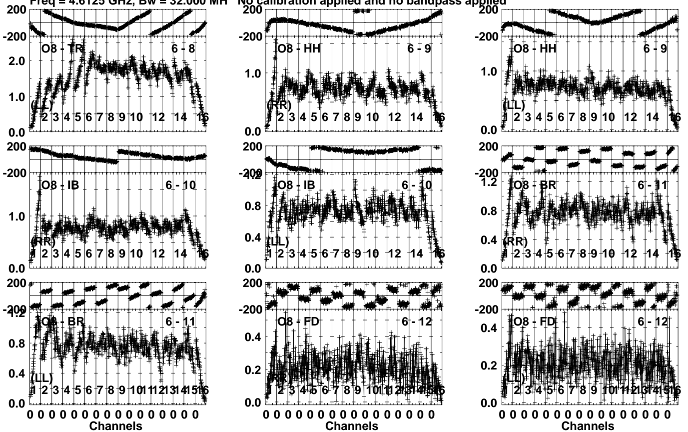
Lower frame: Milli Ampl Jy Top frame: Phas deg Vector averaged cross-power spectrum Several baselines displayed Timerange: 00/16:23:23 to 00/16:25:19
