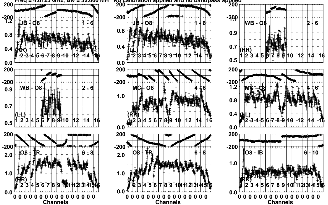
Lower frame: Milli Ampl Jy Top frame: Phas deg Vector averaged cross-power spectrum Several baselines displayed Timerange: 00/20:36:33 to 00/20:38:29
