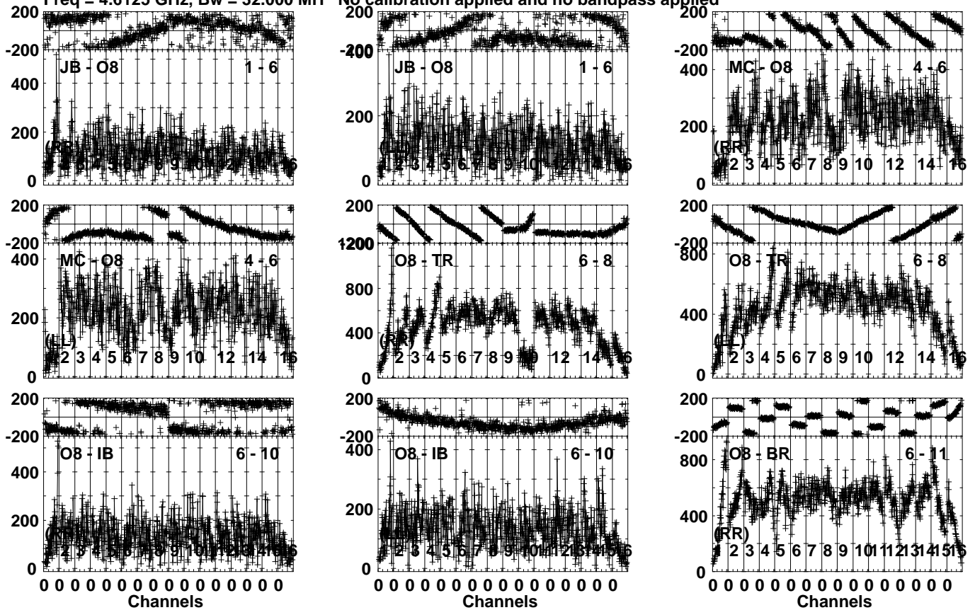
Lower frame: Micro Ampl Jy Top frame: Phas deg Vector averaged cross-power spectrum Several baselines displayed Timerange: 00/21:56:03 to 00/21:59:59
