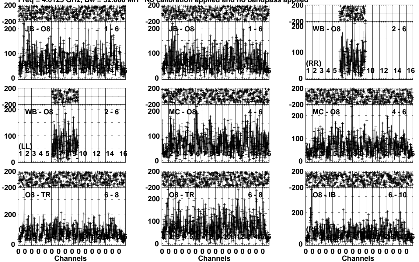
Lower frame: Micro Ampl Jy Top frame: Phas deg Vector averaged cross-power spectrum Several baselines displayed Timerange: 00/19:42:51 to 00/19:46:49
