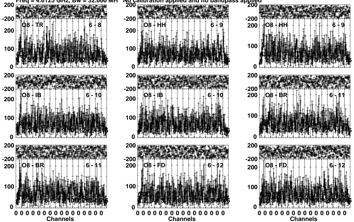
Lower frame: Micro Ampl Jy Top frame: Phas deg Vector averaged cross-power spectrum Several baselines displayed Timerange: 00/16:43:41 to 00/16:47:39
