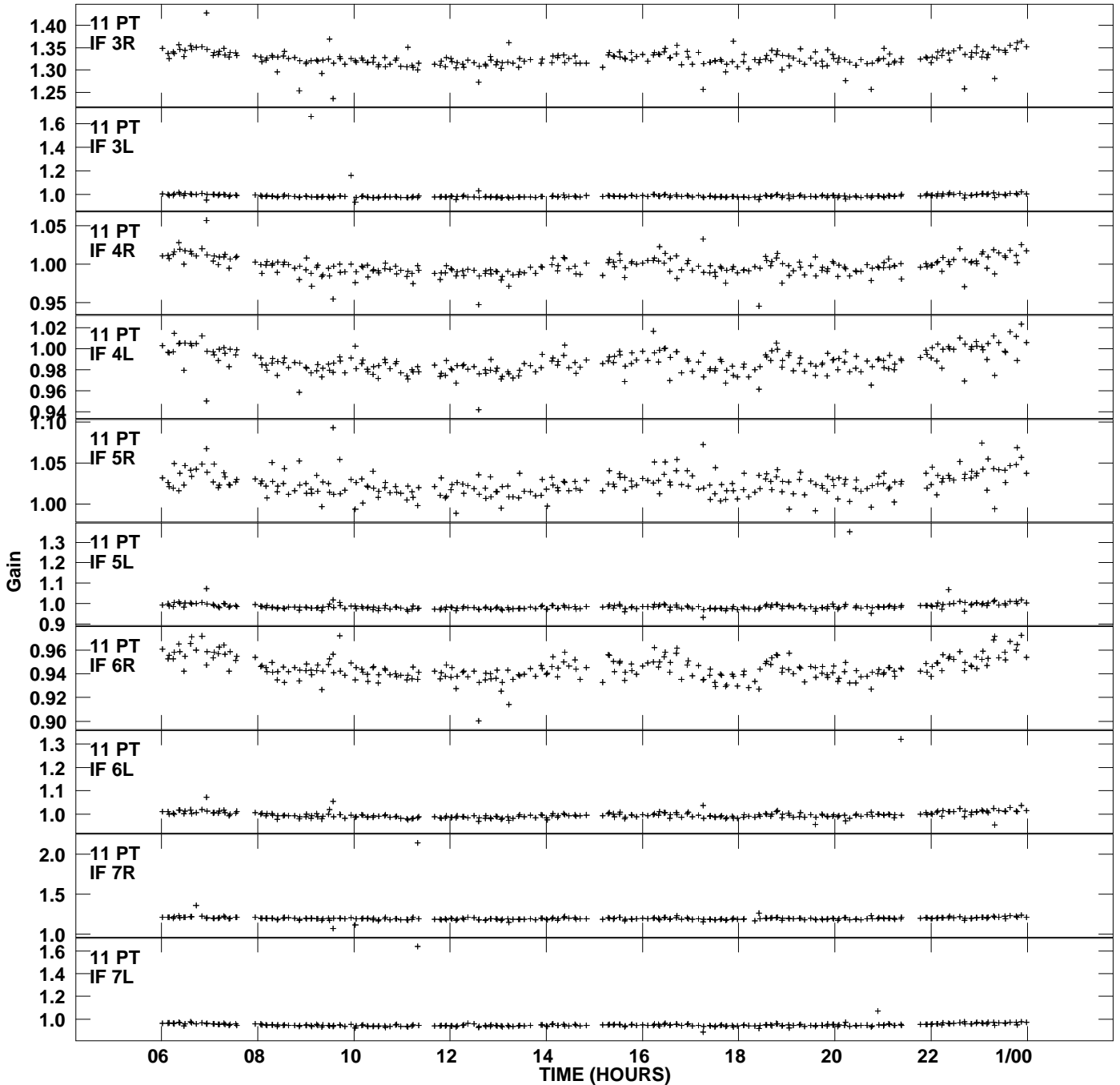
Plot file version 16 created 27-FEB-2010 09:38:06 Gain amp vs UTC time for J0958+65.MULTI.1 SN 2 Rpol & Lpol IF 1 - 8
