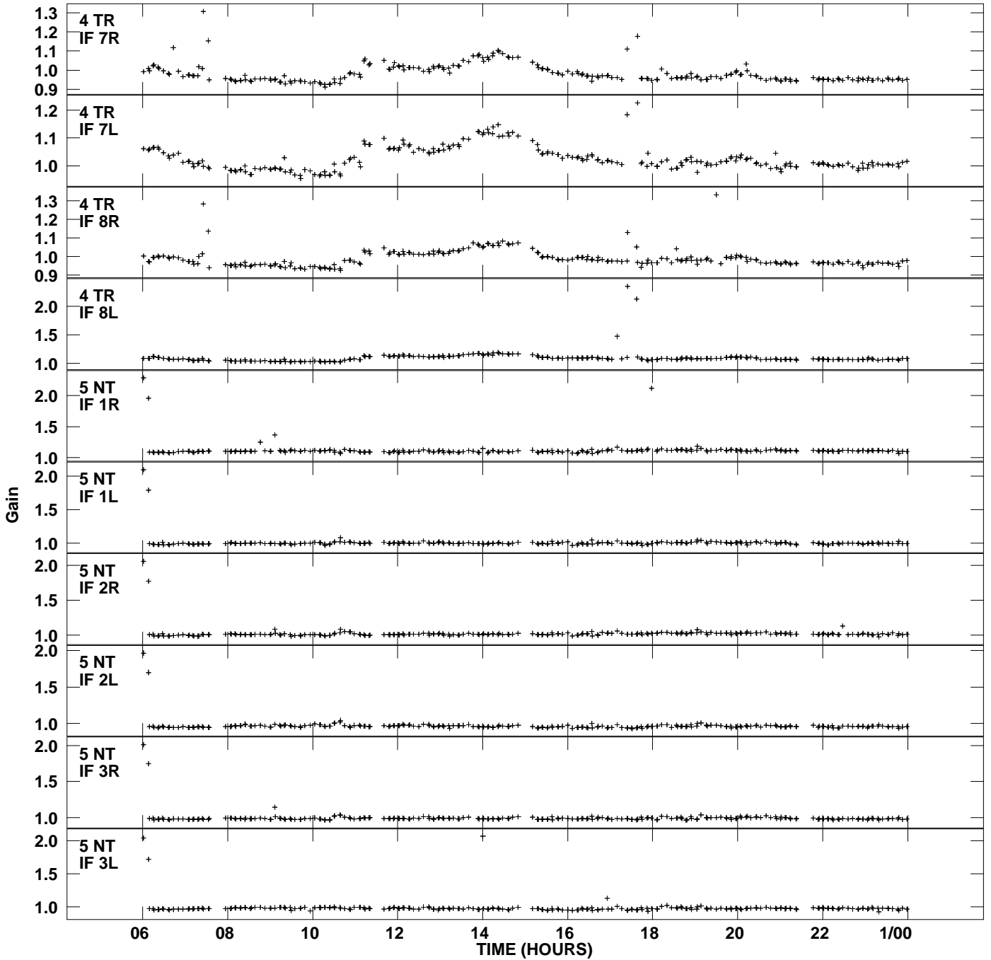
Plot file version 7 created 27-FEB-2010 09:38:06 Gain amp vs UTC time for J0958+65.MULTI.1 SN 2 Rpol & Lpol IF 1 - 8
