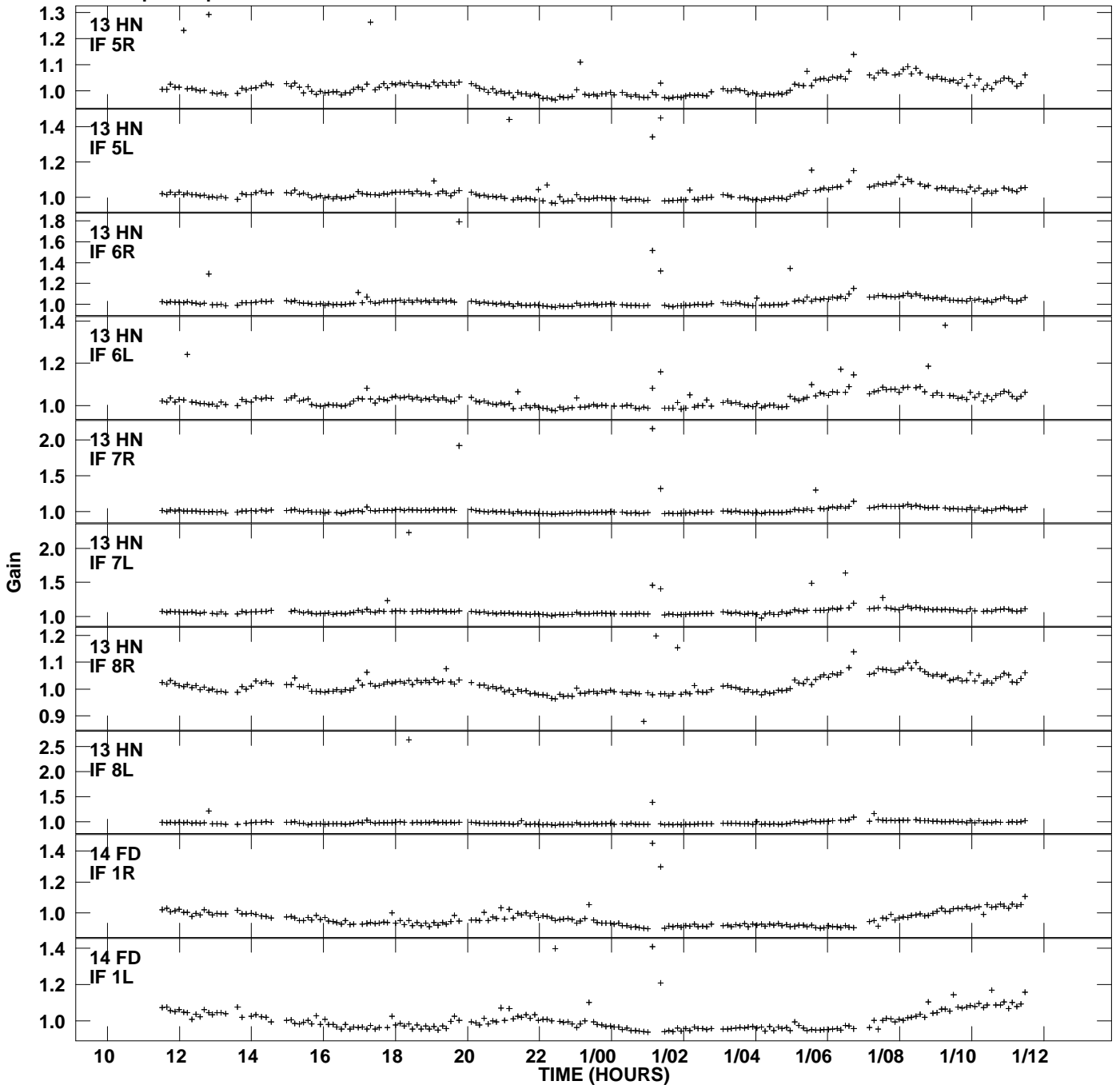
Plot file version 21 created 19-SEP-2012 15:17:43 Gain amp vs UTC time for J0958+65.MULTI.1 SN 2 Rpol & Lpol IF 1 - 8
