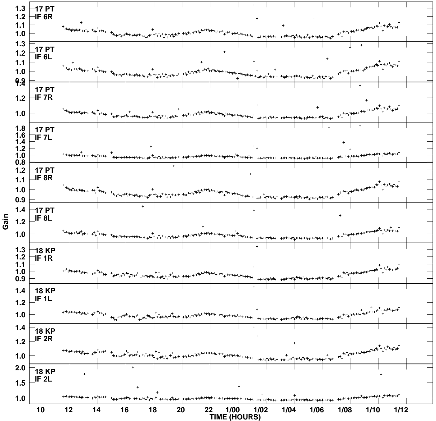
Plot file version 26 created 19-SEP-2012 15:17:43 Gain amp vs UTC time for J0958+65.MULTI.1 SN 2 Rpol & Lpol IF 1 - 8
