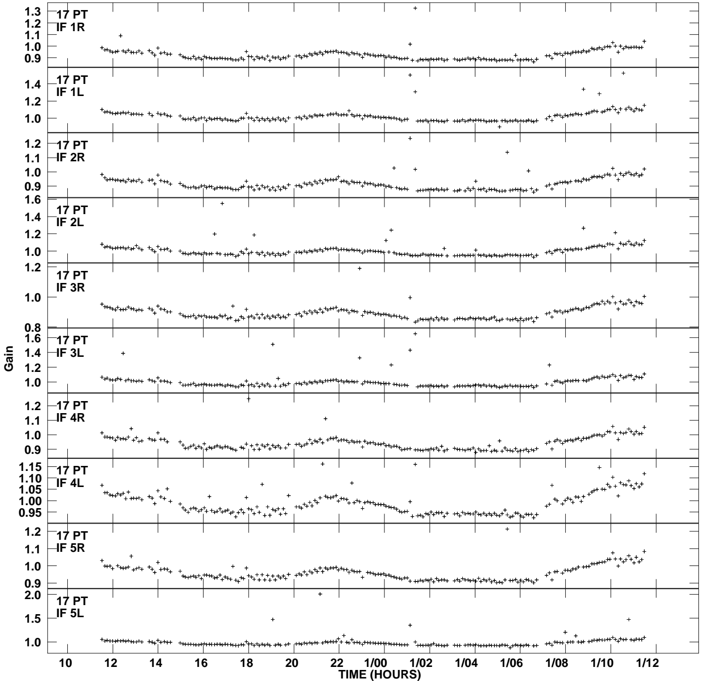
Plot file version 25 created 19-SEP-2012 15:17:43 Gain amp vs UTC time for J0958+65.MULTI.1 SN 2 Rpol & Lpol IF 1 - 8
