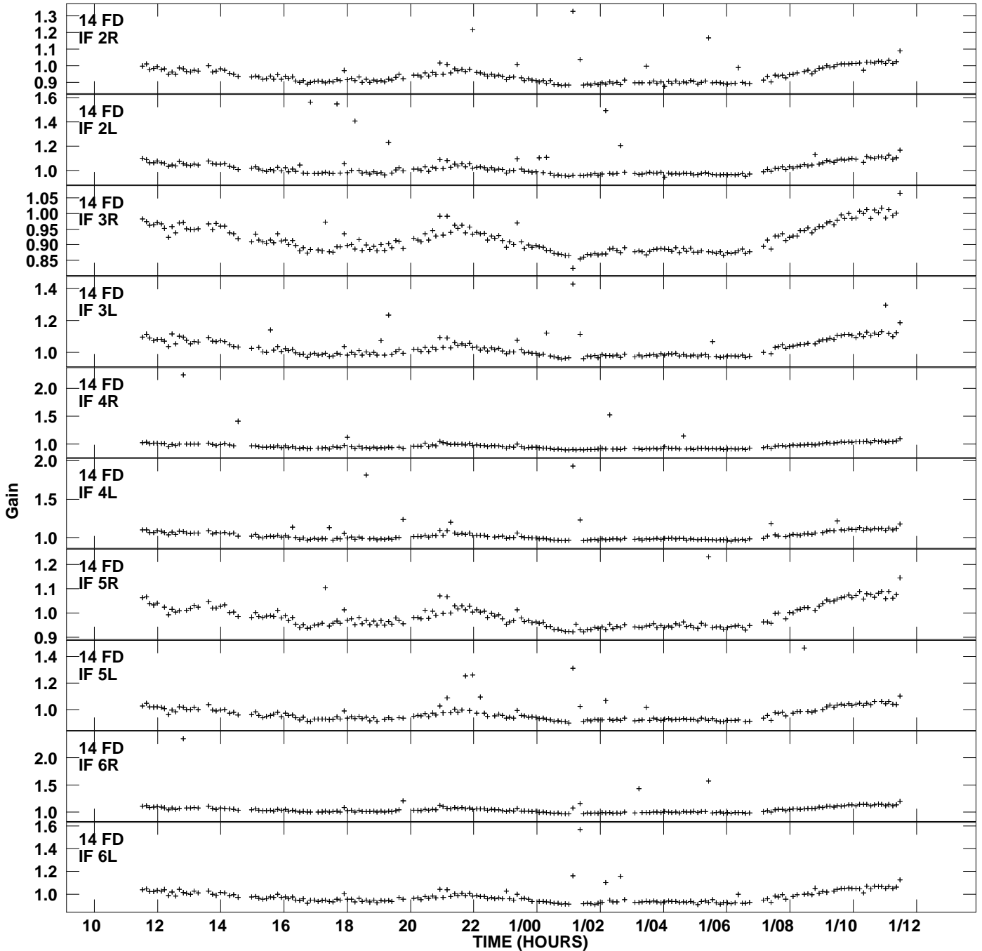
Plot file version 22 created 19-SEP-2012 15:17:43 Gain amp vs UTC time for J0958+65.MULTI.1 SN 2 Rpol & Lpol IF 1 - 8
