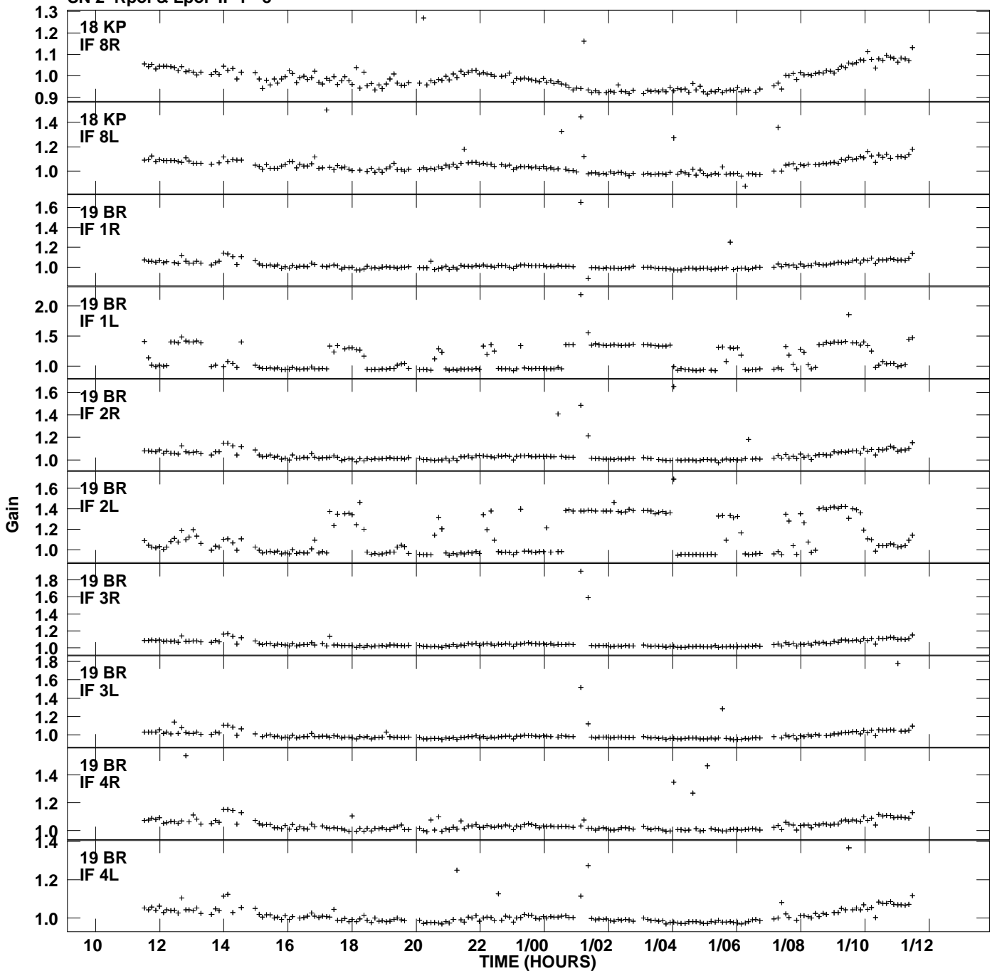
Plot file version 28 created 19-SEP-2012 15:17:43 Gain amp vs UTC time for J0958+65.MULTI.1 SN 2 Rpol & Lpol IF 1 - 8
