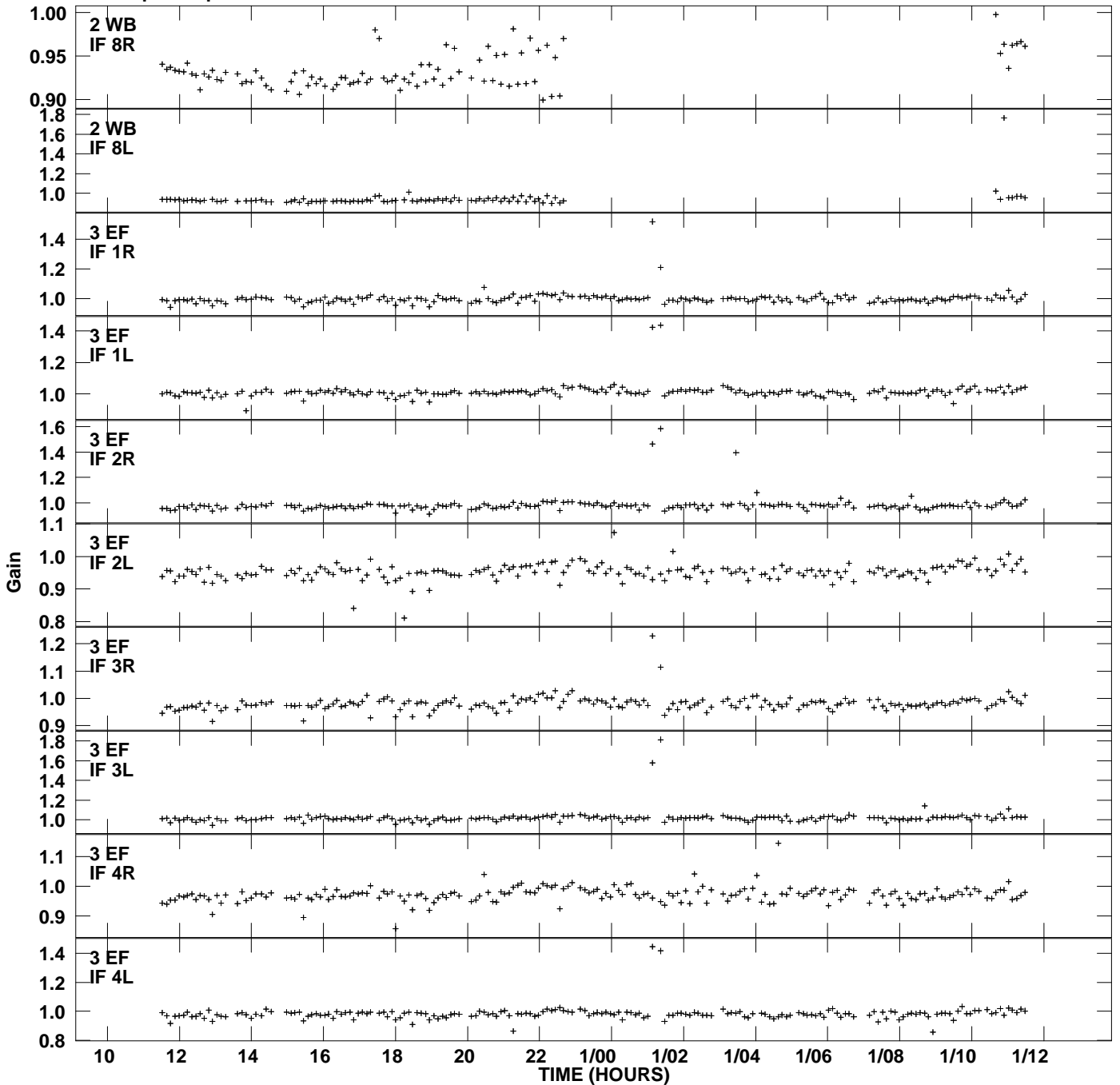
Plot file version 4 created 19-SEP-2012 15:17:42 Gain amp vs UTC time for J0958+65.MULTI.1 SN 2 Rpol & Lpol IF 1 - 8
