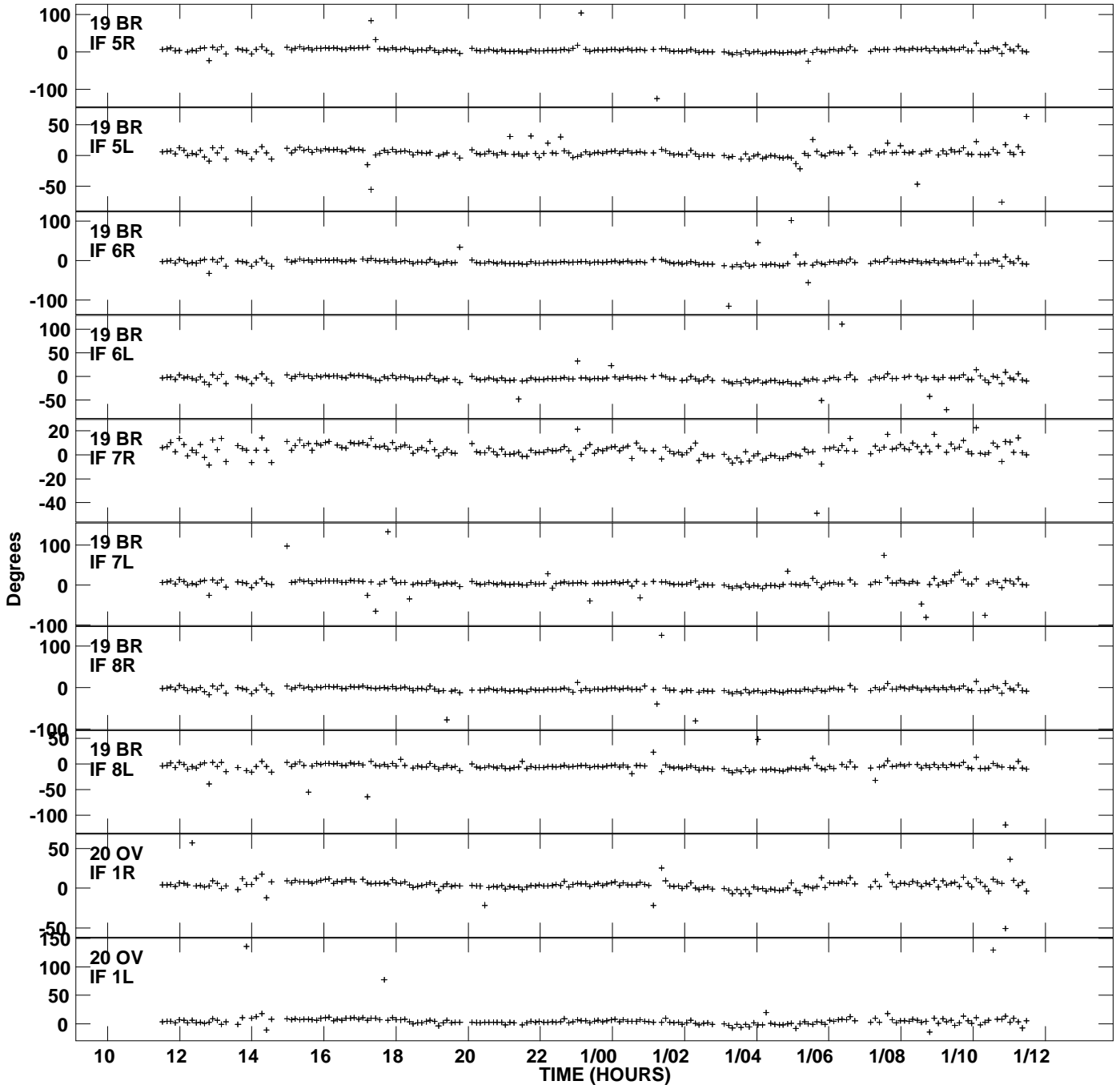
Plot file version 29 created 19-SEP-2012 15:15:34 Gain phs vs UTC time for J0958+65.MULTI.1 SN 1 Rpol & Lpol IF 1 - 8
