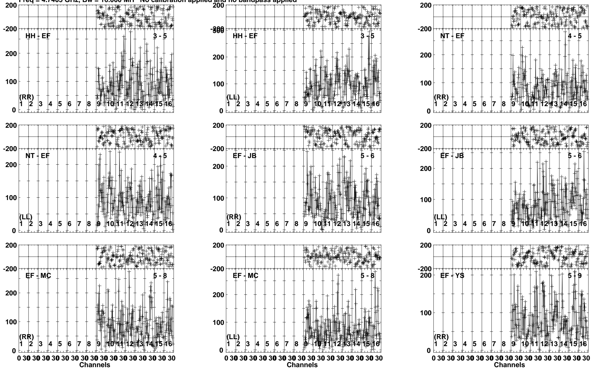
Lower frame: Micro Ampl Jy Top frame: Phas deg Vector averaged cross-power spectrum Baseline: HH (03) - EF (05) Timerange: 00/21:35:55 to 00/21:38:19
