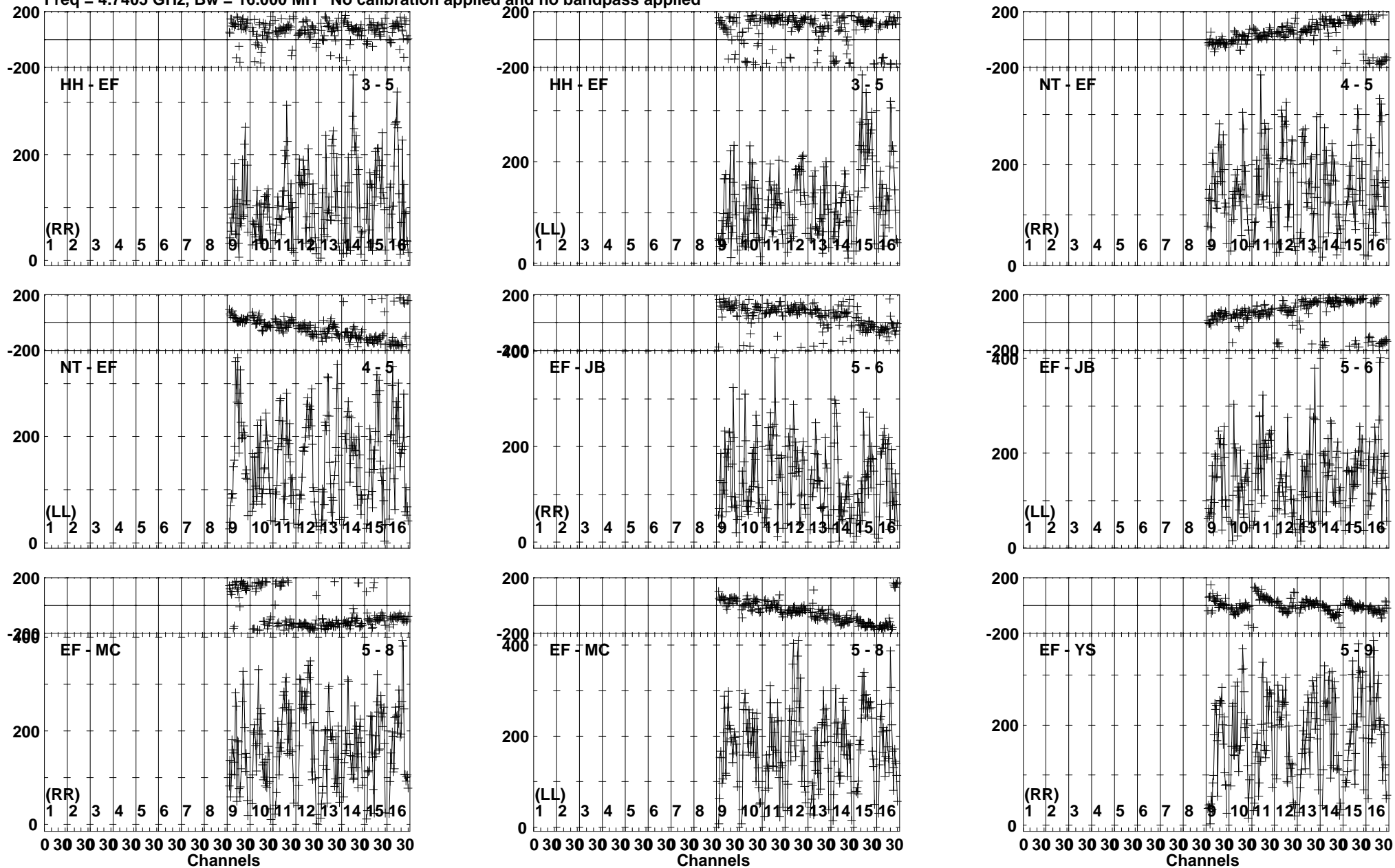
Lower frame: Micro Ampl Jy Top frame: Phas deg Vector averaged cross-power spectrum Baseline: HH (03) - EF (05) Timerange: 00/22:08:04 to 00/22:10:29
