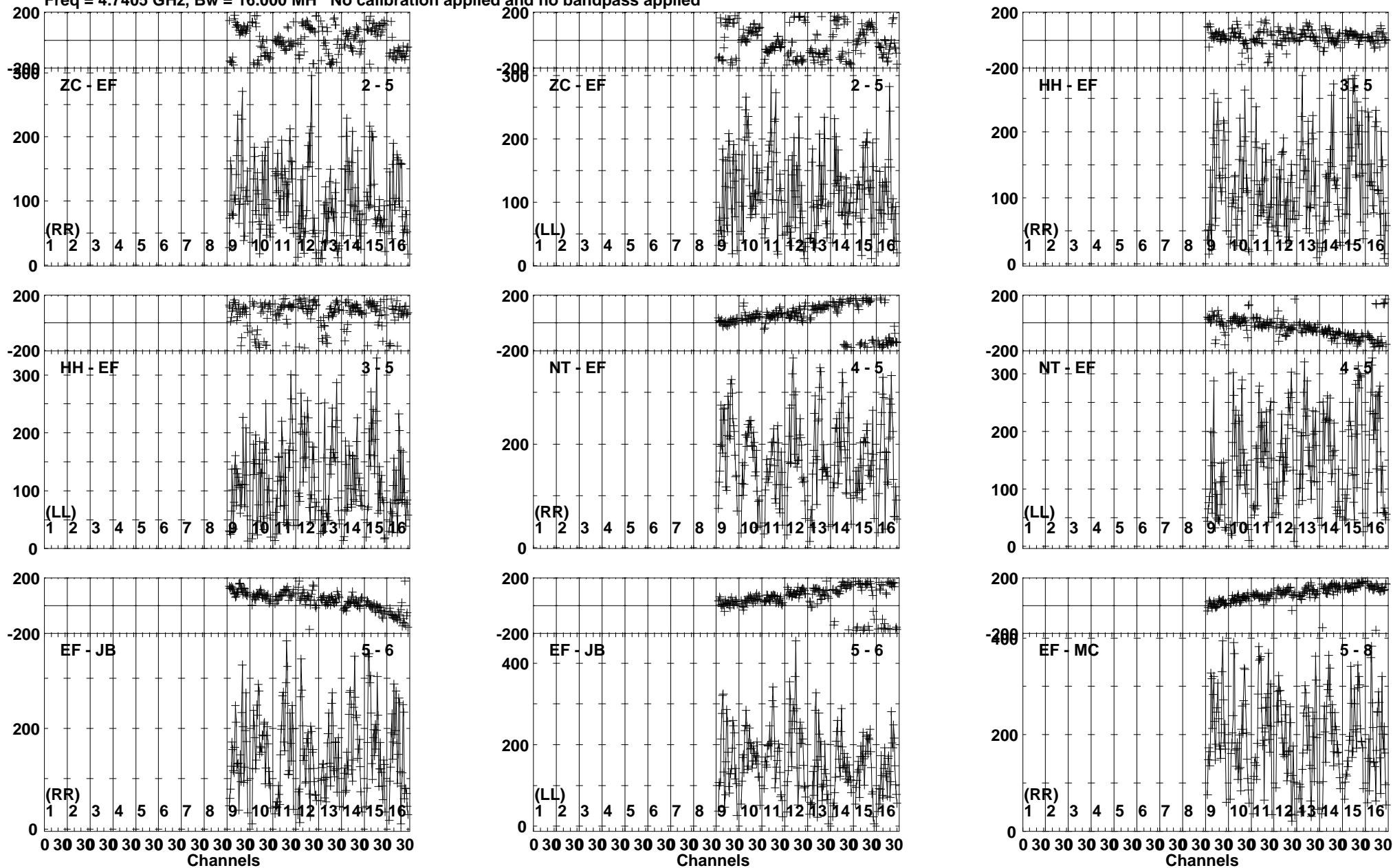
Lower frame: Micro Ampl Jy Top frame: Phas deg Vector averaged cross-power spectrum Baseline: ZC (02) - EF (05) Timerange: 00/20:11:43 to 00/20:14:10
