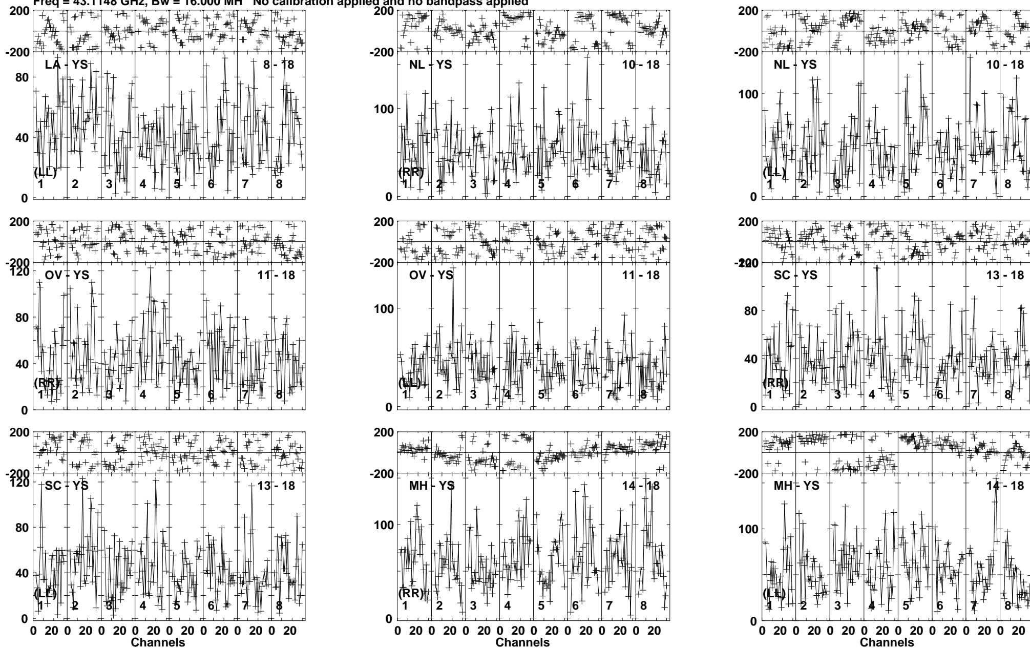
Lower frame: Micro Ampl Jy Top frame: Phas deg Vector averaged cross-power spectrum Baseline: LA (08) - YS (18) Timerange: 01/06:20:20 to 01/06:29:59
