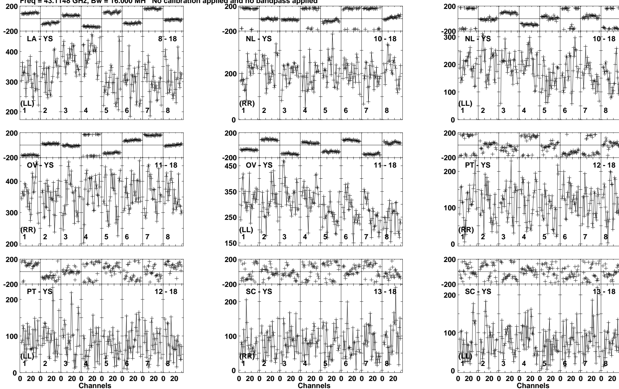
Lower frame: Micro Ampl Jy Top frame: Phas deg Vector averaged cross-power spectrum Baseline: LA (08) - YS (18) Timerange: 01/08:02:32 to 01/08:08:00
