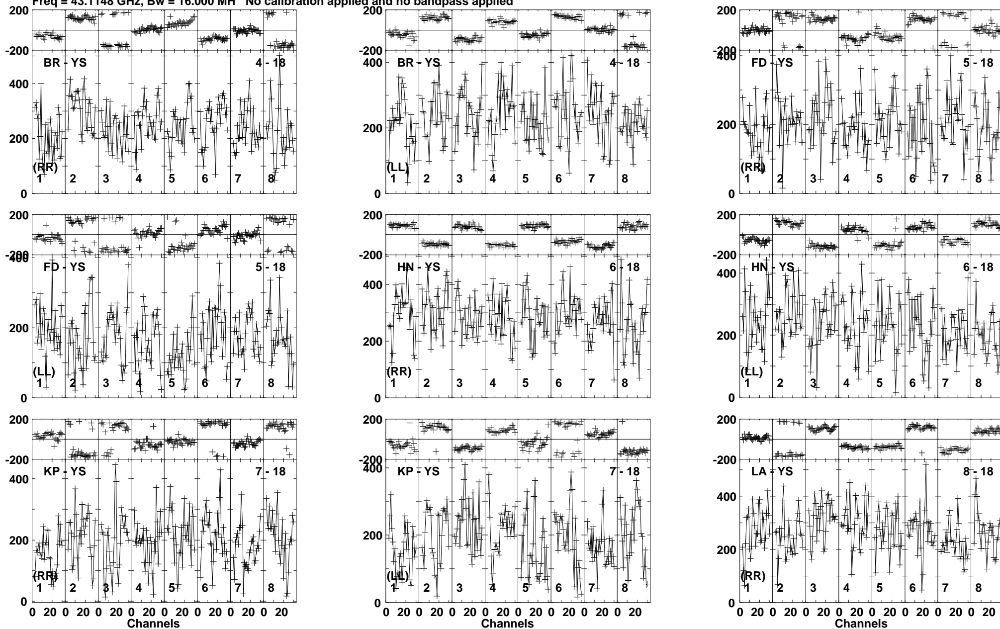
Lower frame: Micro Ampl Jy Top frame: Phas deg Vector averaged cross-power spectrum Baseline: BR (04) - YS (18) Timerange: 01/10:26:09 to 01/10:27:59
