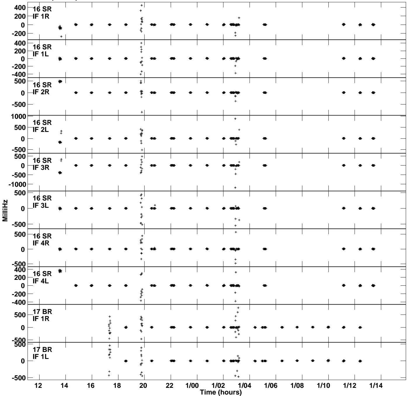
Plot file version 13 created 20-MAY-2021 12:41:10 Rate vs UTC time for GM077_1.UVDATA.1 SN 3 Rpol & Lpol IF 1 - 4
