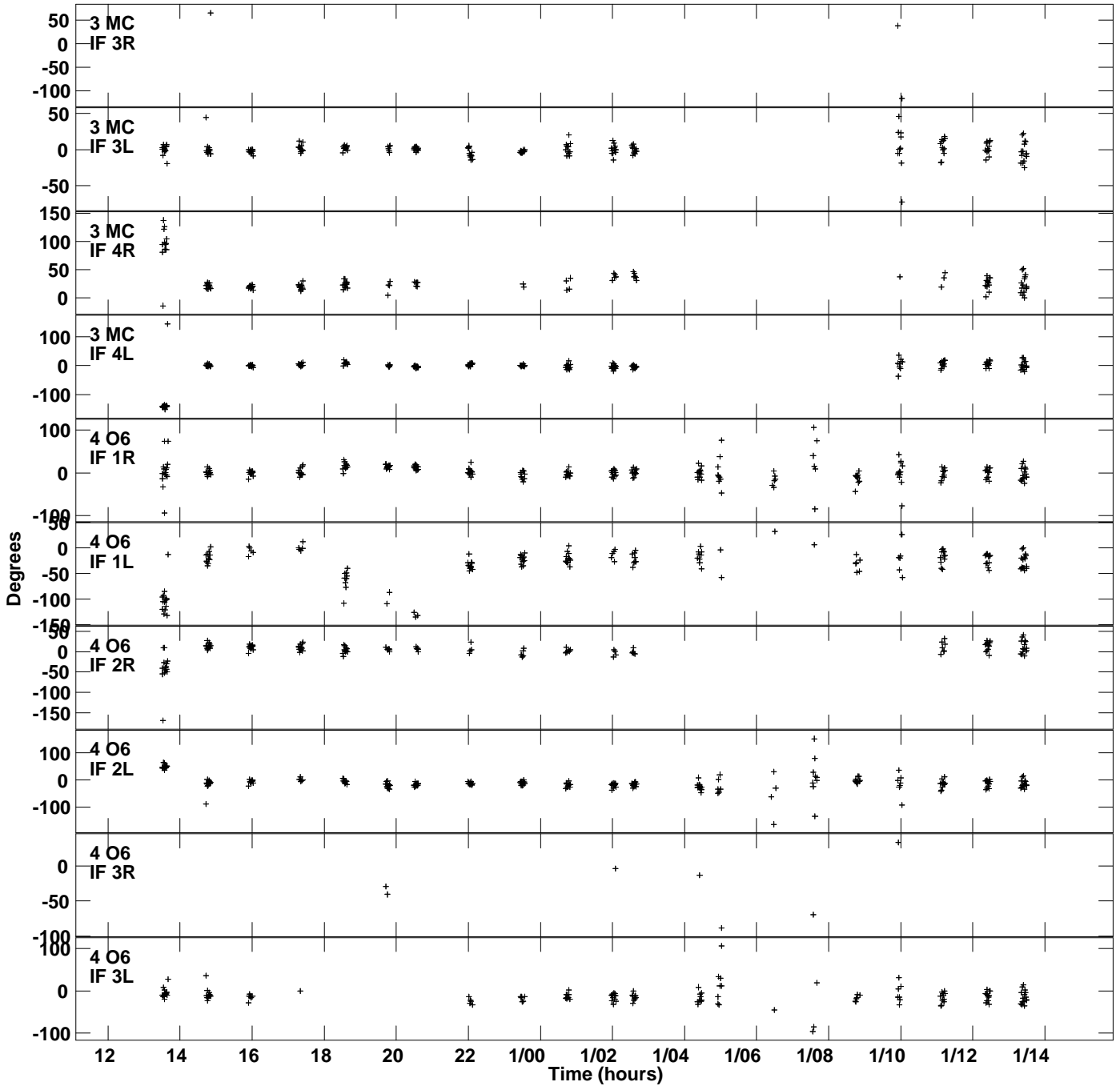
Plot file version 3 created 19-MAR-2021 20:12:18 Gain phs vs UTC time for J2202+4216.MULTI.1 SN 1 Rpol & Lpol IF 1 - 4
