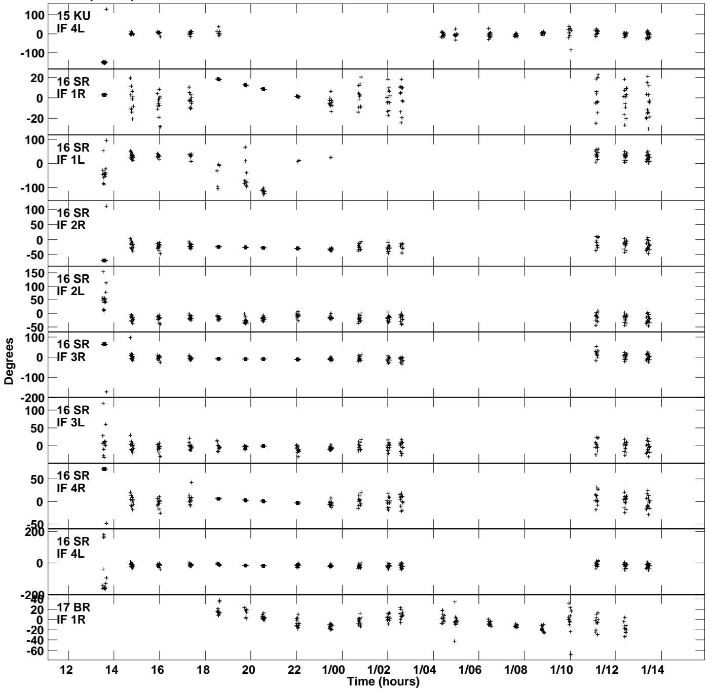
Plot file version 12 created 19-MAR-2021 20:12:18 Gain phs vs UTC time for J2202+4216.MULTI.1 SN 1 Rpol & Lpol IF 1 - 4
