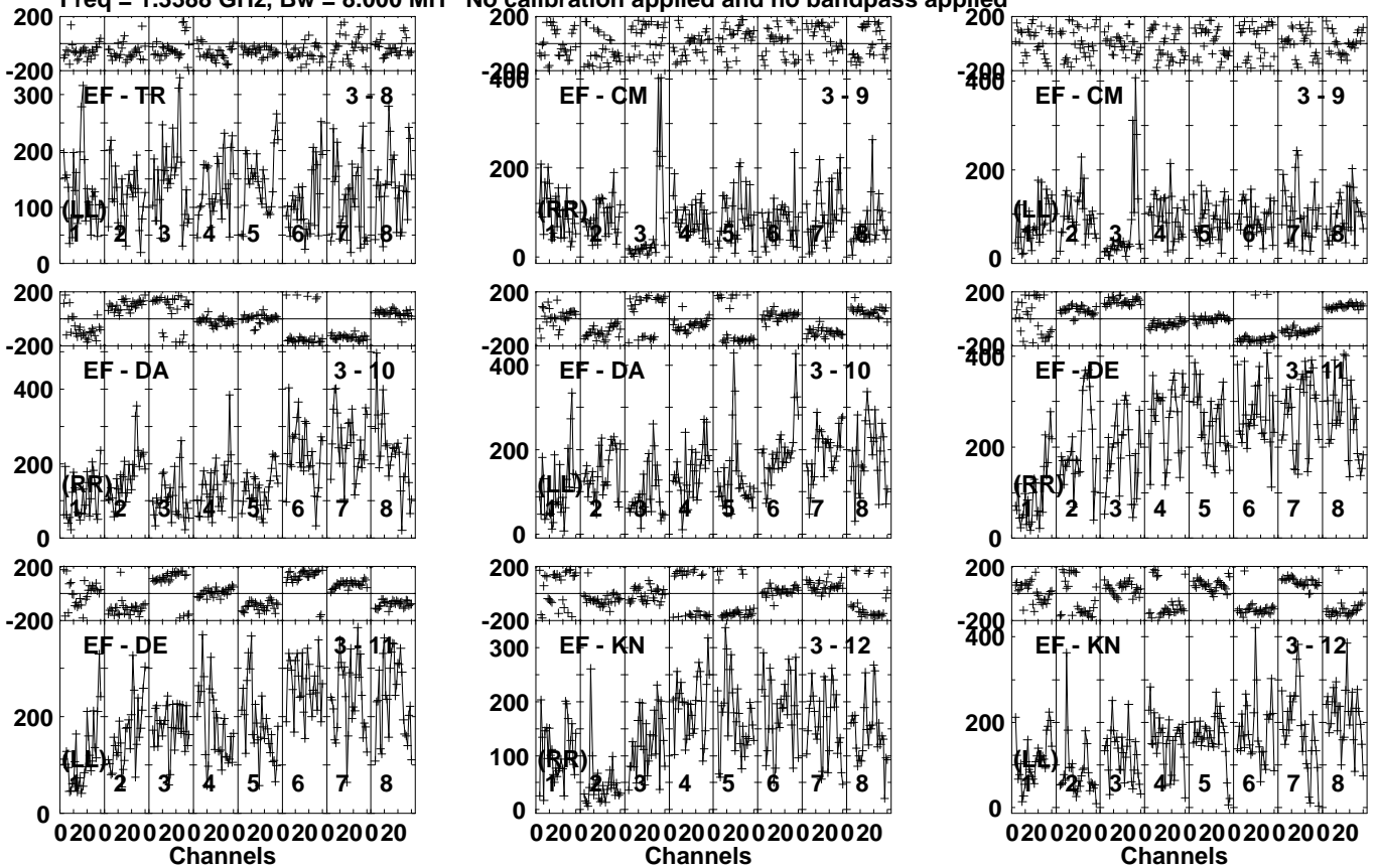
Lower frame: Micro Ampl Jy Top frame: Phas deg Vector averaged cross-power spectrum Several baselines displayed Timerange: 00/22:25:01 to 00/22:29:59
