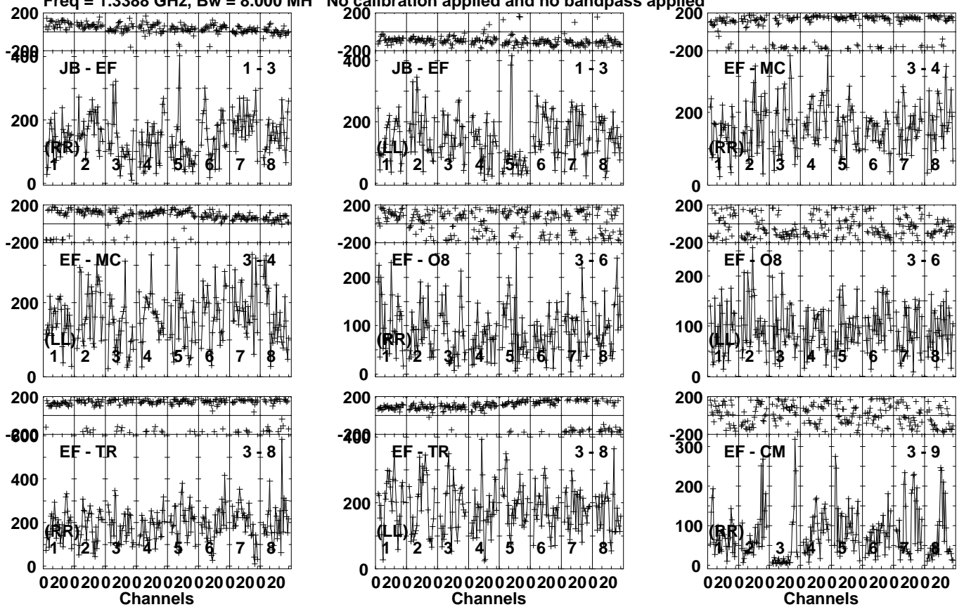
Lower frame: Micro Ampl Jy Top frame: Phas deg Vector averaged cross-power spectrum Several baselines displayed Timerange: 01/02:26:01 to 01/02:30:59
