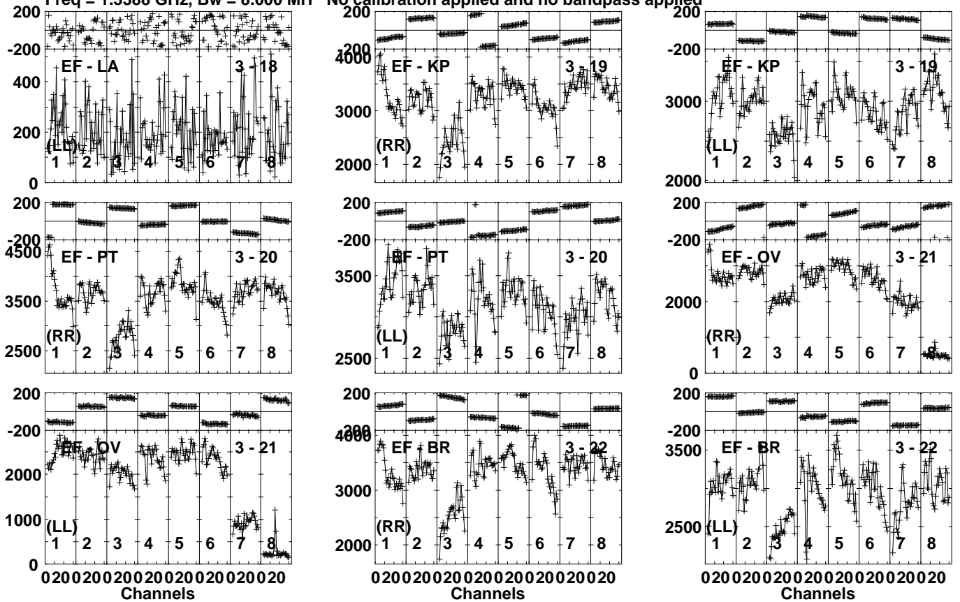
Lower frame: Micro Ampl Jy Top frame: Phas deg Vector averaged cross-power spectrum Several baselines displayed Timerange: 00/17:19:31 to 00/17:20:59
