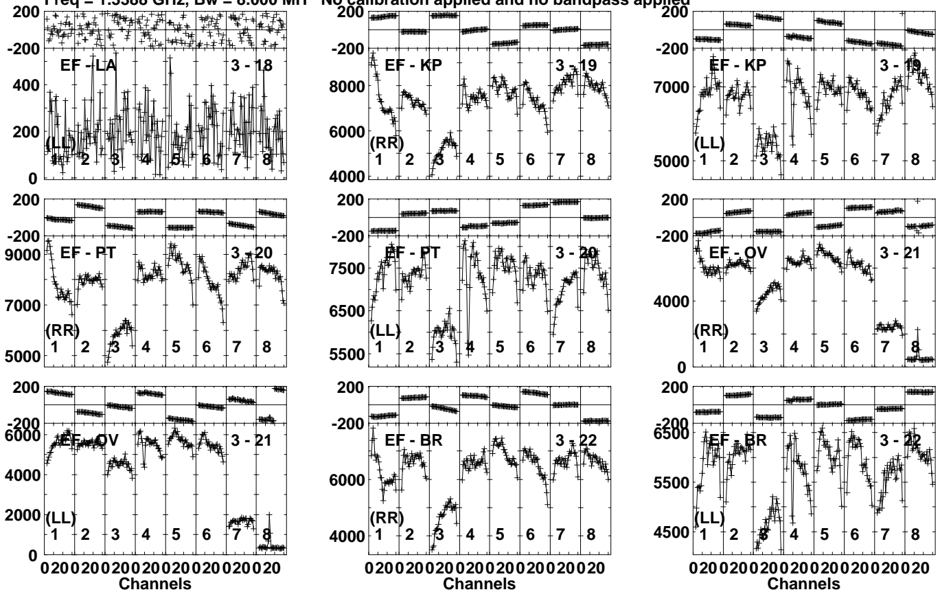
Lower frame: Micro Ampl Jy Top frame: Phas deg Vector averaged cross-power spectrum Several baselines displayed Timerange: 00/19:44:31 to 00/19:45:59
