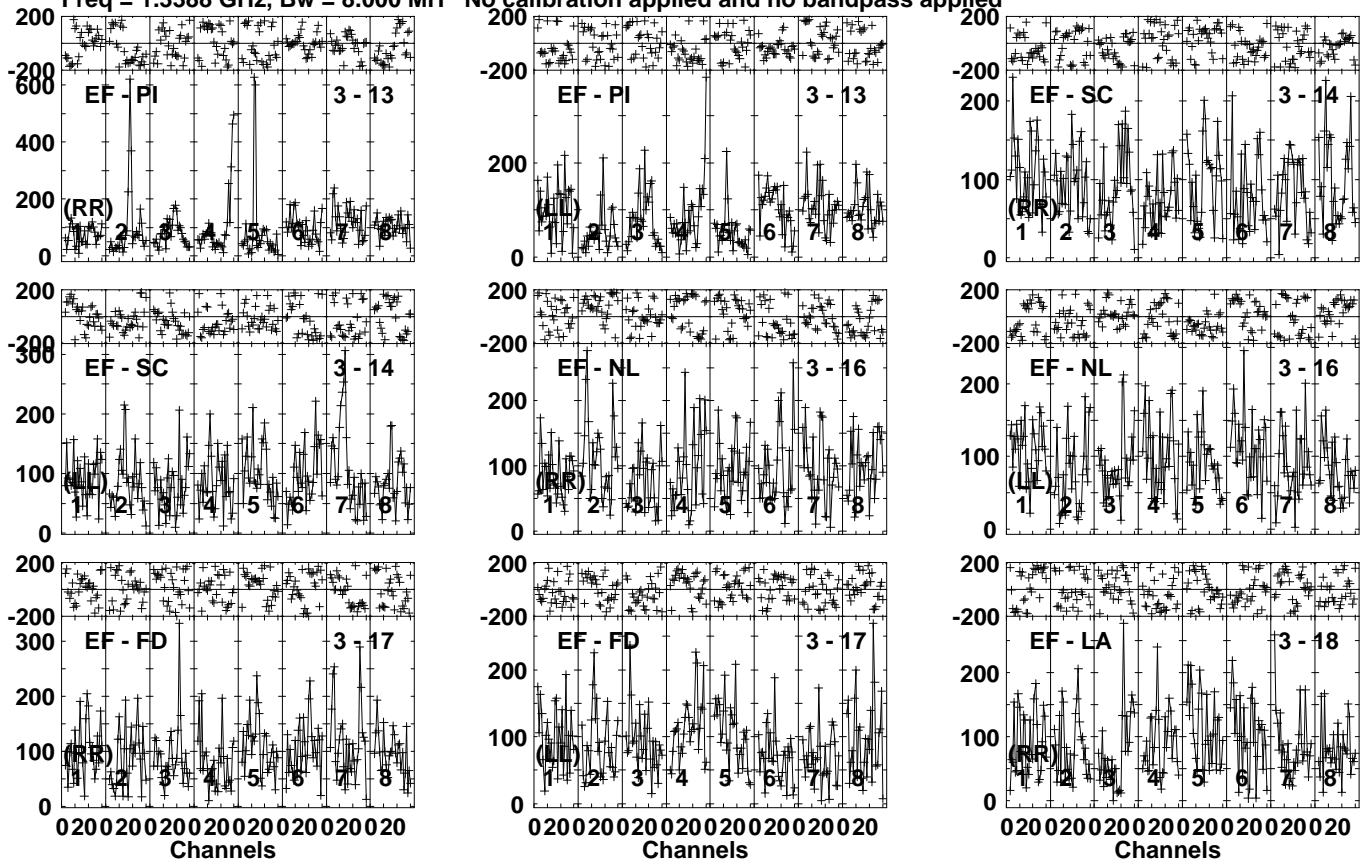
Lower frame: Micro Ampl Jy Top frame: Phas deg Vector averaged cross-power spectrum Several baselines displayed Timerange: 00/20:14:01 to 00/20:18:59
