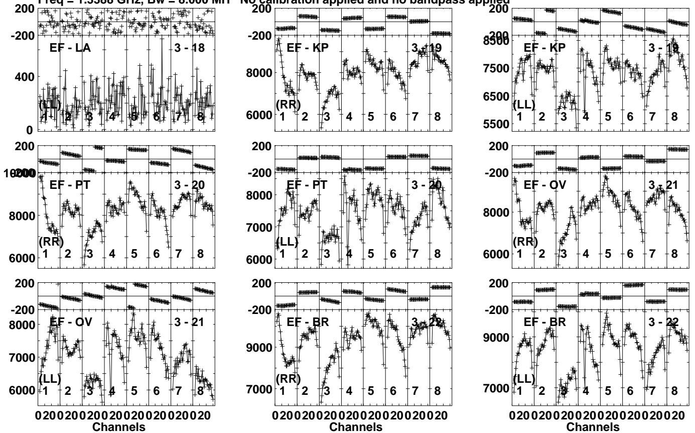
Lower frame: Micro Ampl Jy Top frame: Phas deg Vector averaged cross-power spectrum Several baselines displayed Timerange: 00/22:09:31 to 00/22:10:59
