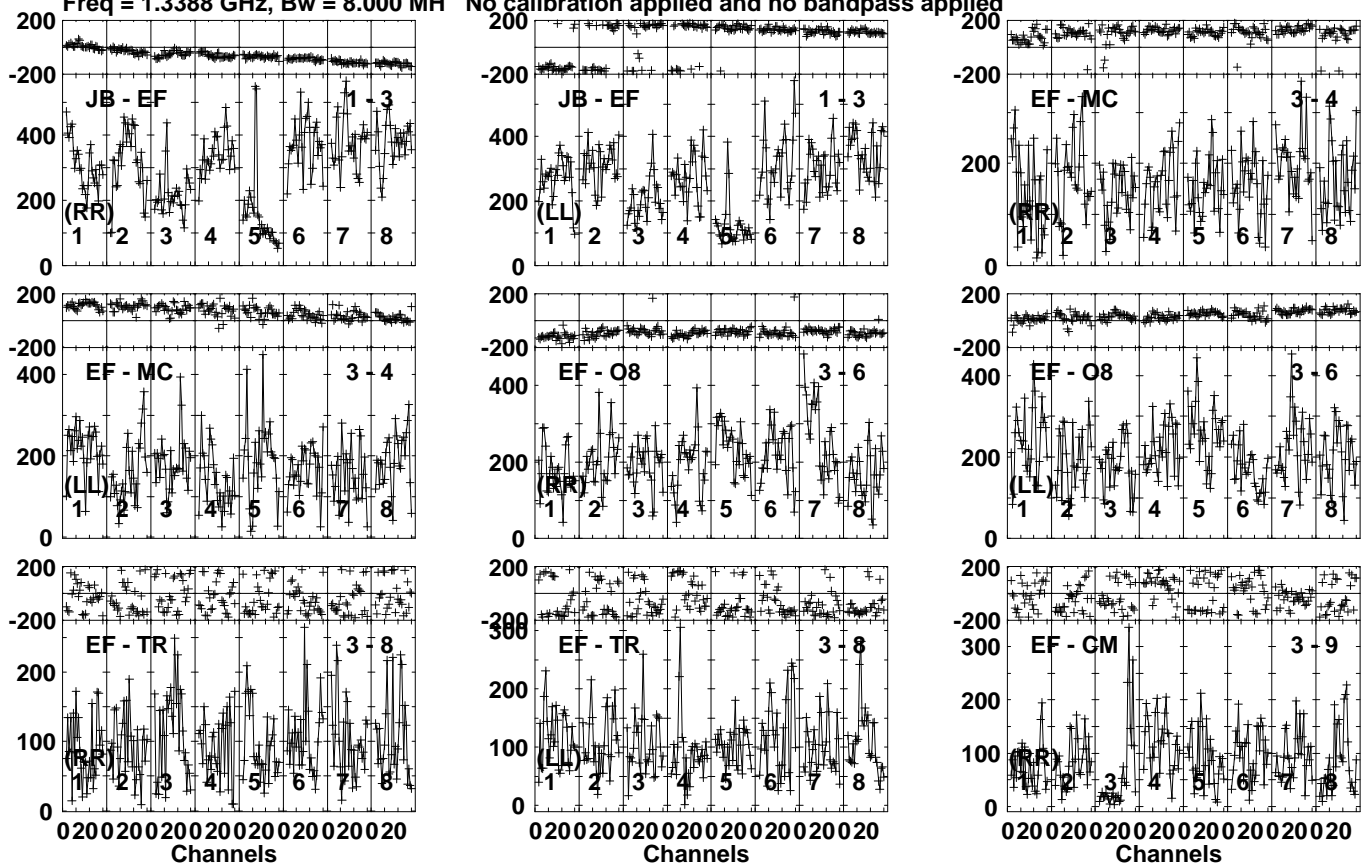
Lower frame: Micro Ampl Jy Top frame: Phas deg Vector averaged cross-power spectrum Several baselines displayed Timerange: 00/23:21:01 to 00/23:25:59
