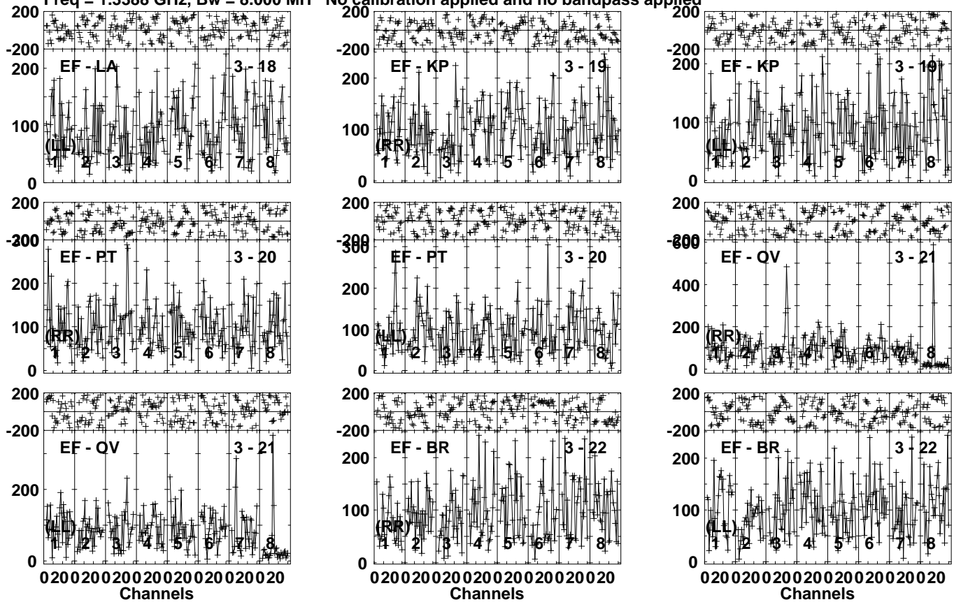
Lower frame: Micro Ampl Jy Top frame: Phas deg Vector averaged cross-power spectrum Several baselines displayed Timerange: 00/19:25:01 to 00/19:29:59
