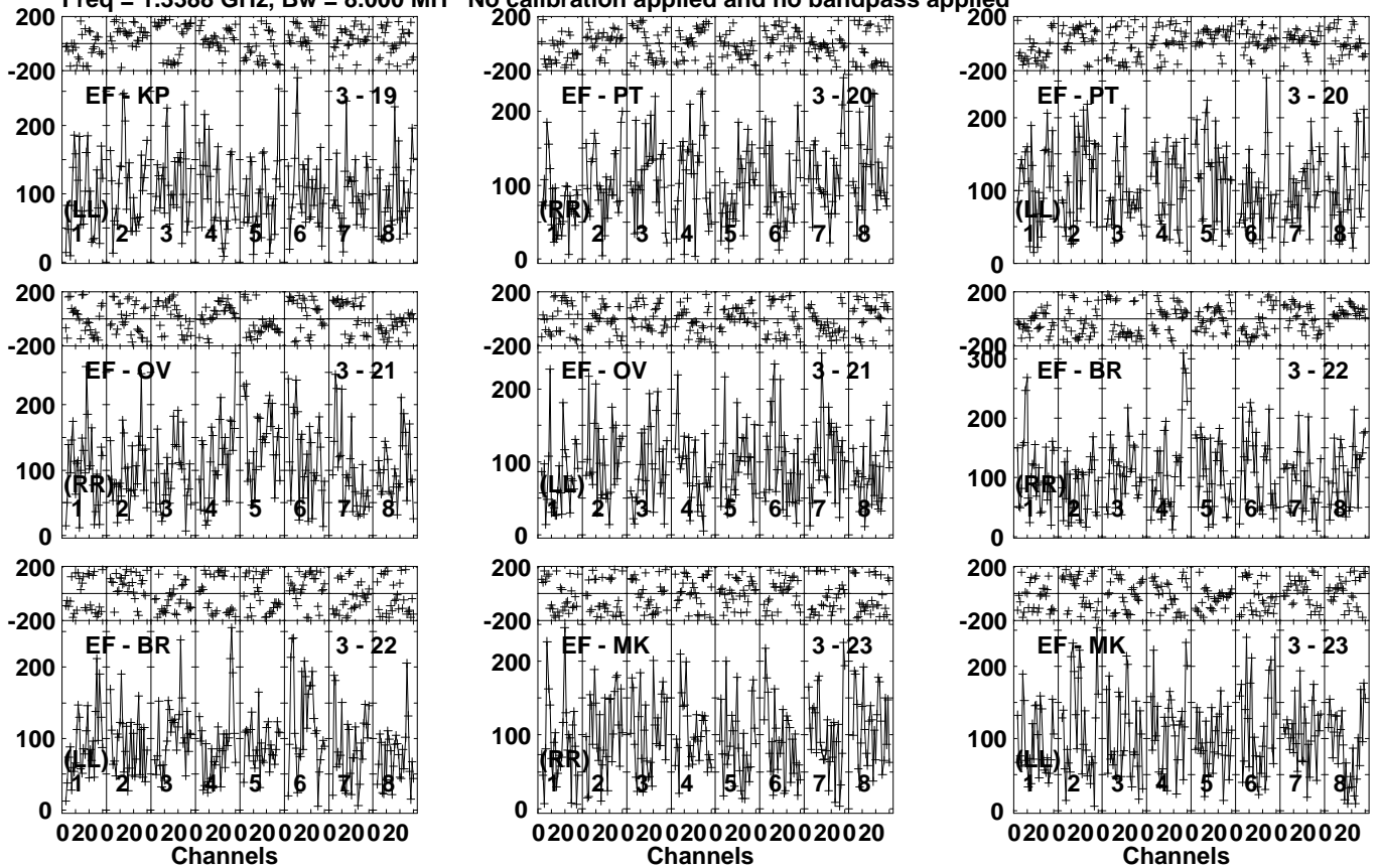
Lower frame: Micro Ampl Jy Top frame: Phas deg Vector averaged cross-power spectrum Several baselines displayed Timerange: 01/03:36:01 to 01/03:40:59
