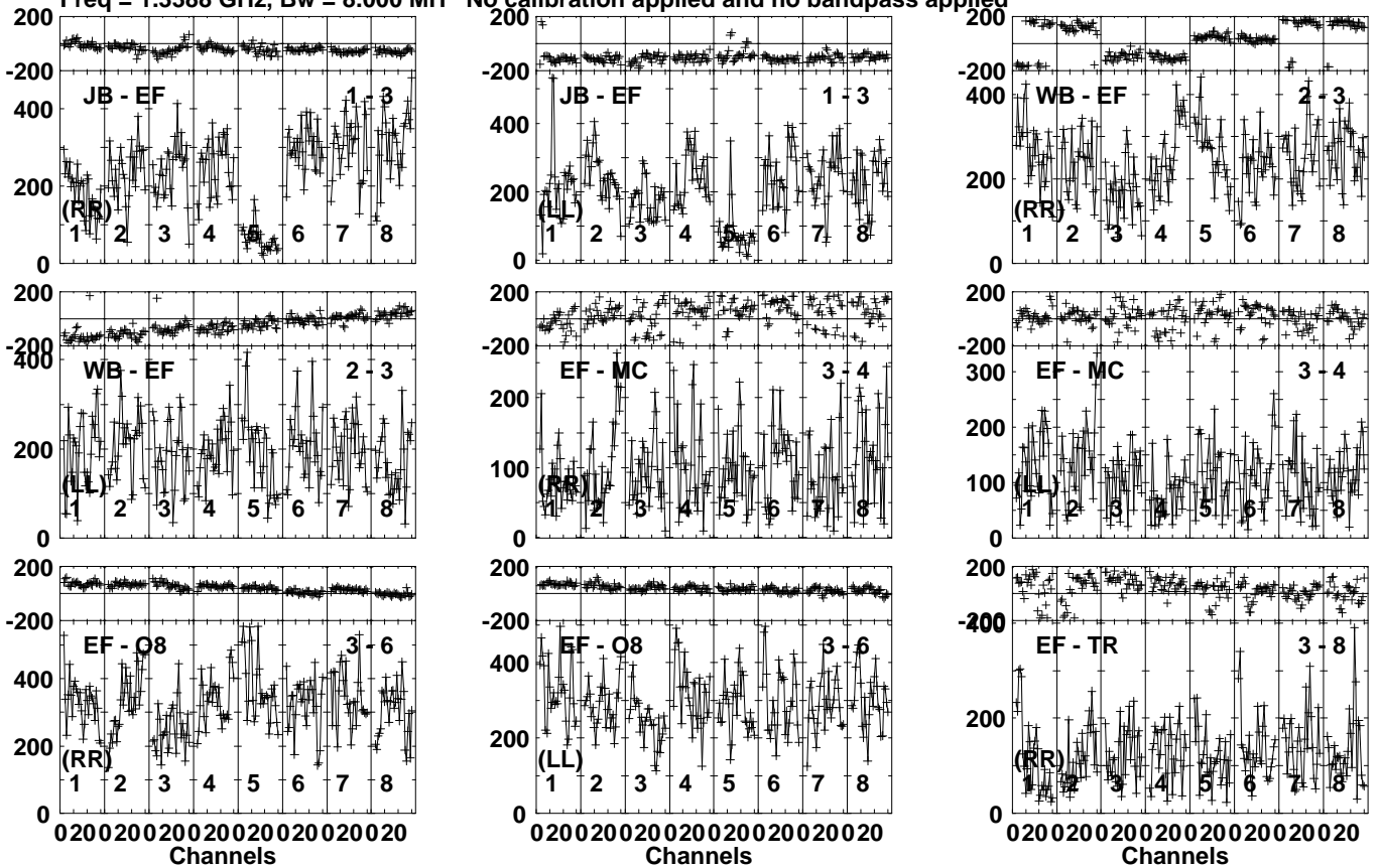
Lower frame: Micro Ampl Jy Top frame: Phas deg Vector averaged cross-power spectrum Several baselines displayed Timerange: 00:17:00:01 to 00:17:04:59
