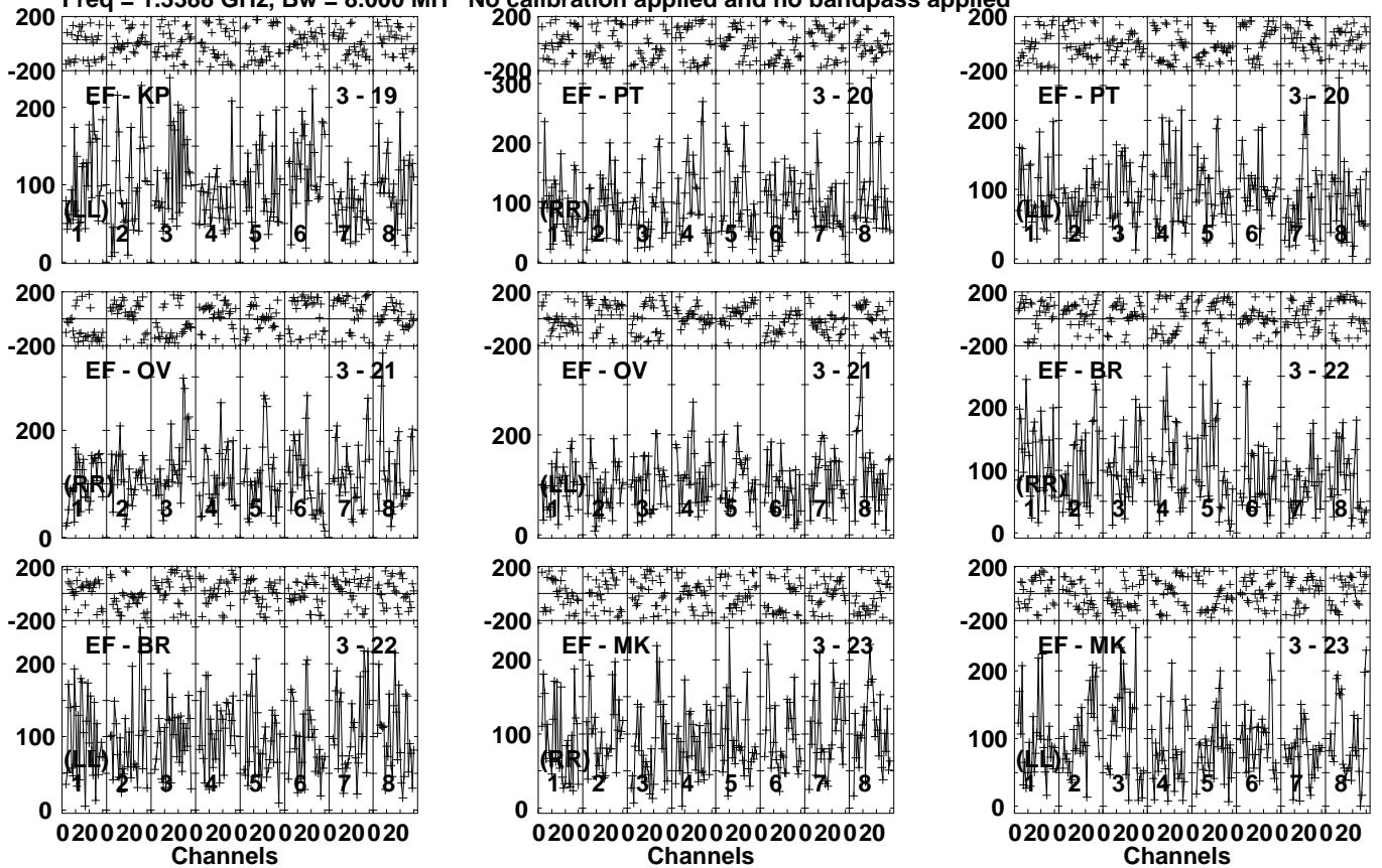
Lower frame: Micro Ampl Jy Top frame: Phas deg Vector averaged cross-power spectrum Several baselines displayed Timerange: 01/03:50:01 to 01/03:54:59
