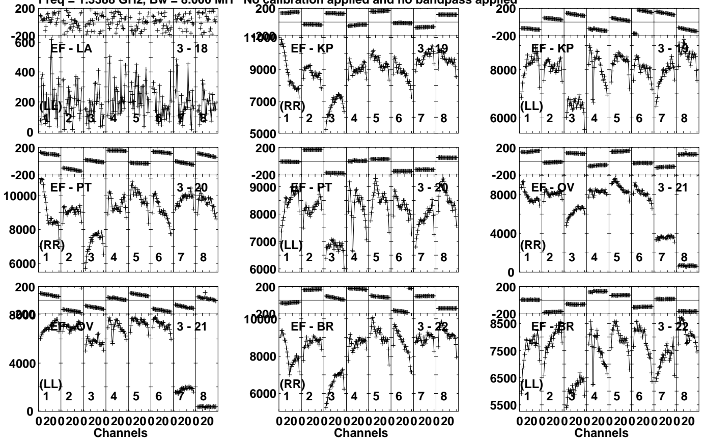
Lower frame: Micro Ampl Jy Top frame: Phas deg Vector averaged cross-power spectrum Several baselines displayed Timerange: 00/21:01:31 to 00/21:02:59
