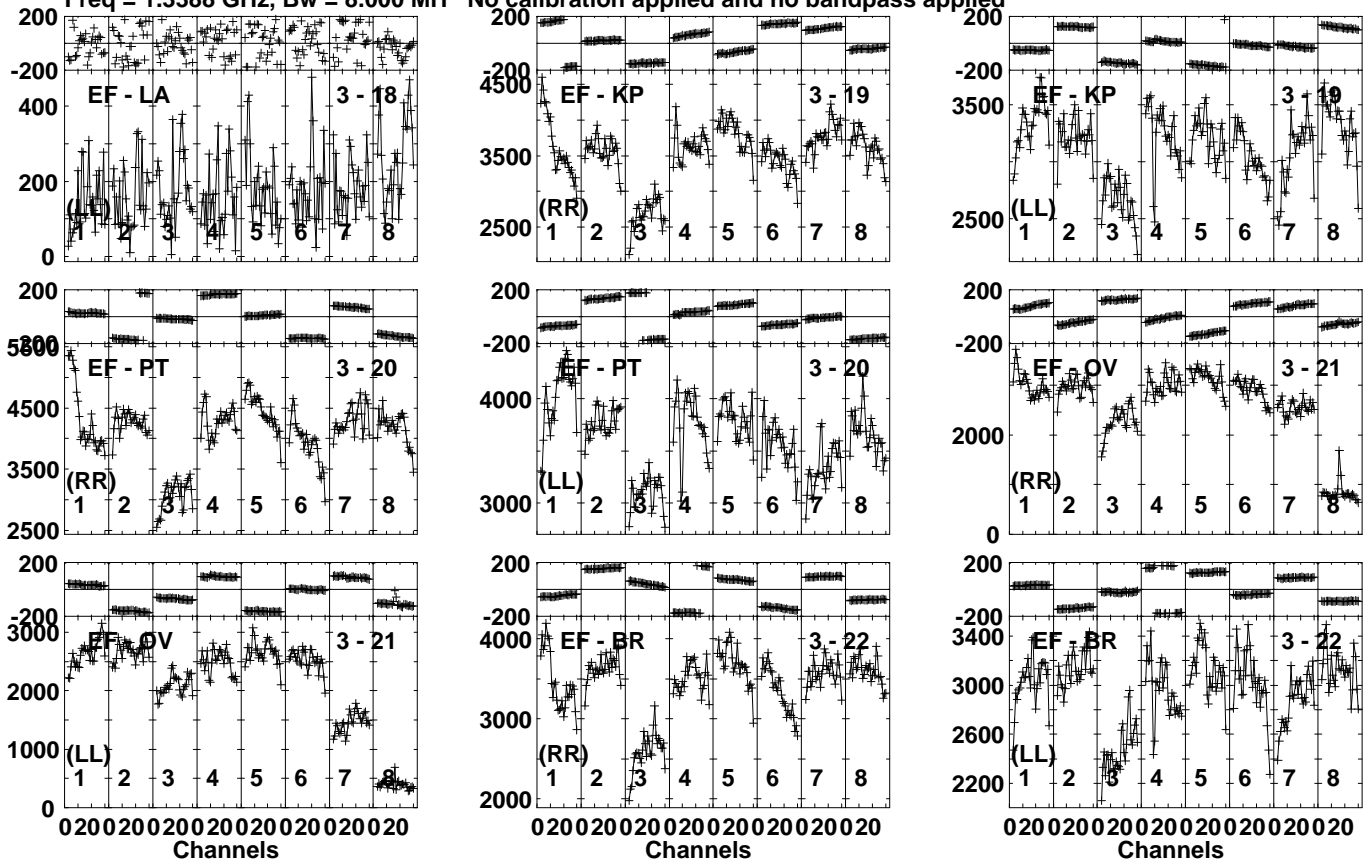
Lower frame: Micro Ampl Jy Top frame: Phas deg Vector averaged cross-power spectrum Several baselines displayed Timerange: 00/17:40:31 to 00/17:41:59
