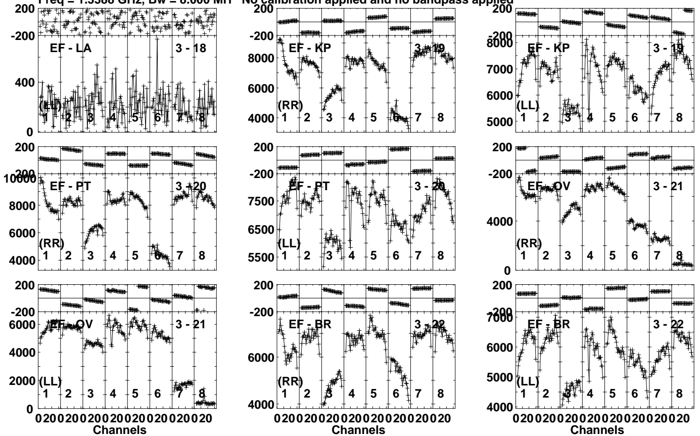
Lower frame: Micro Ampl Jy Top frame: Phas deg Vector averaged cross-power spectrum Several baselines displayed Timerange: 00/19:51:31 to 00/19:52:59
