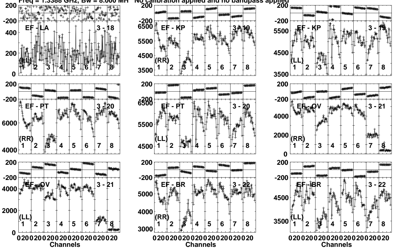
Lower frame: Micro Ampl Jy Top frame: Phas deg Vector averaged cross-power spectrum Several baselines displayed Timerange: 00/18:57:31 to 00/18:58:59
