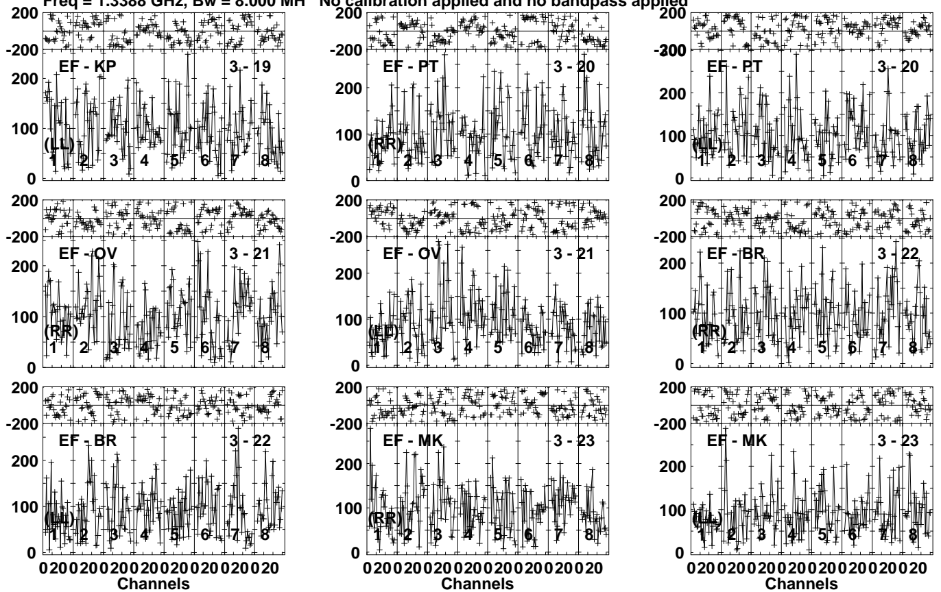
Lower frame: Micro Ampl Jy Top frame: Phas deg Vector averaged cross-power spectrum Several baselines displayed Timerange: 01/03:22:01 to 01/03:26:59
