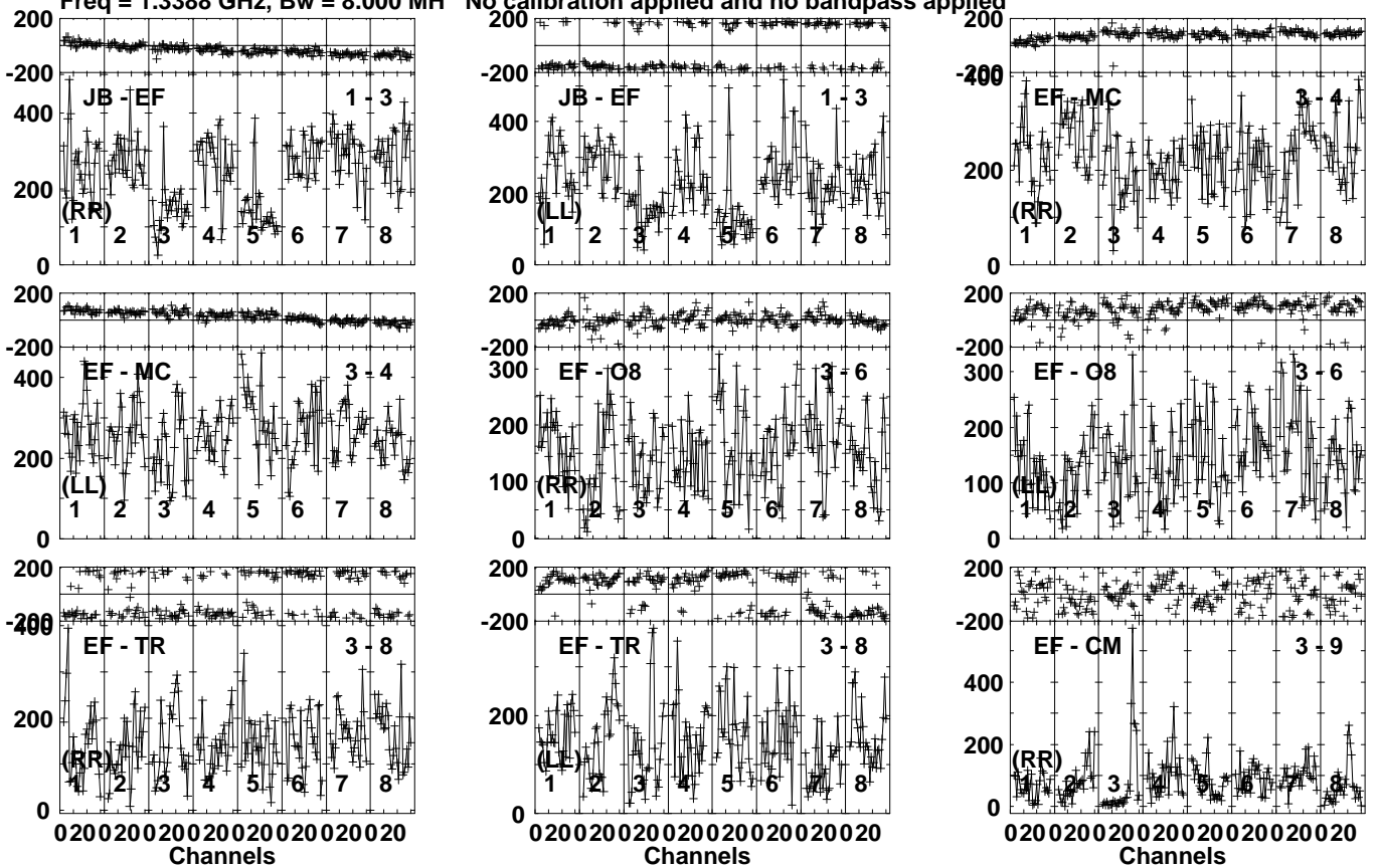
Lower frame: Micro Ampl Jy Top frame: Phas deg Vector averaged cross-power spectrum Several baselines displayed Timerange: 01/01:32:01 to 01/01:36:59
