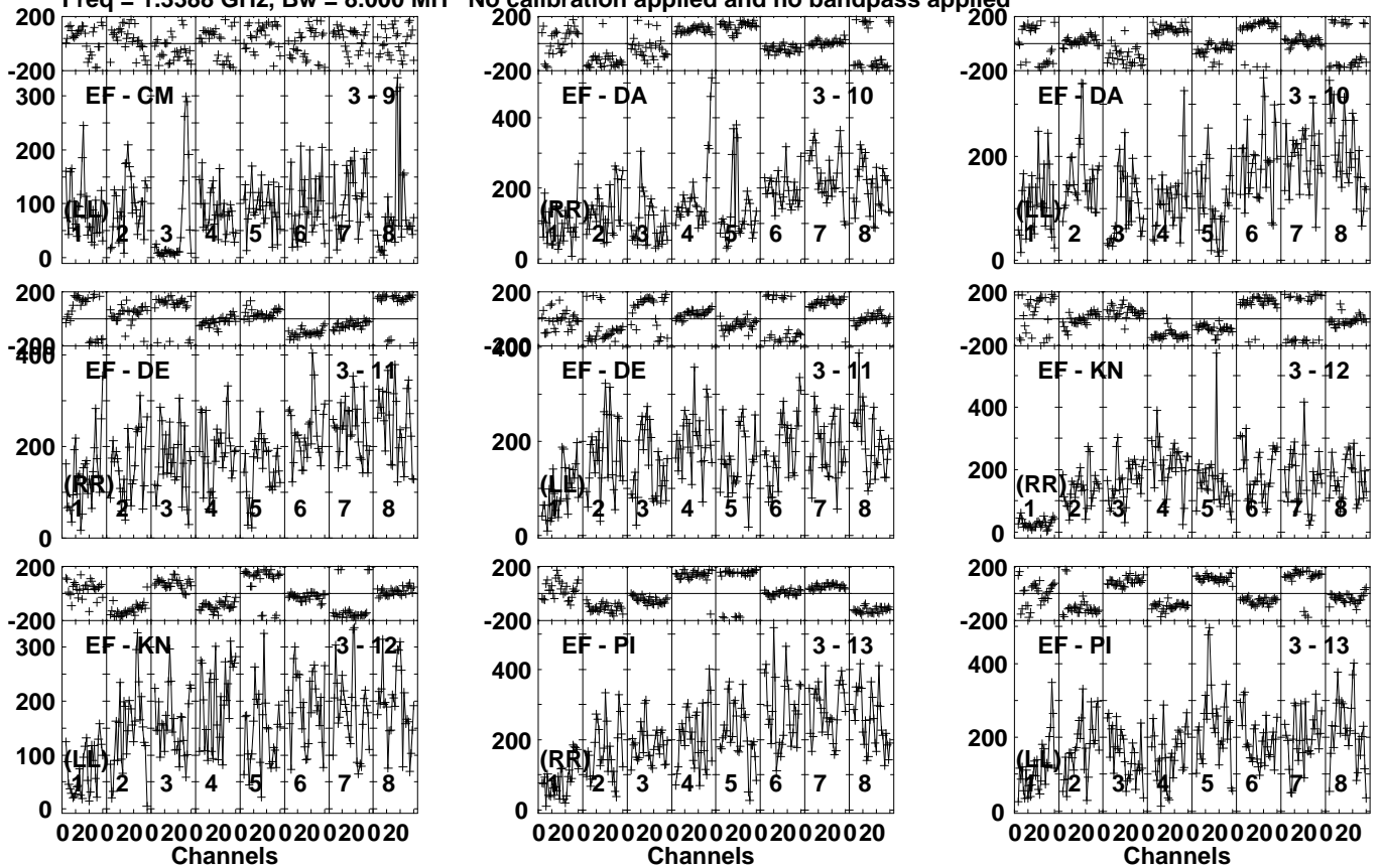
Lower frame: Micro Ampl Jy Top frame: Phas deg Vector averaged cross-power spectrum Several baselines displayed Timerange: 01/00:50:01 to 01/00:54:59
