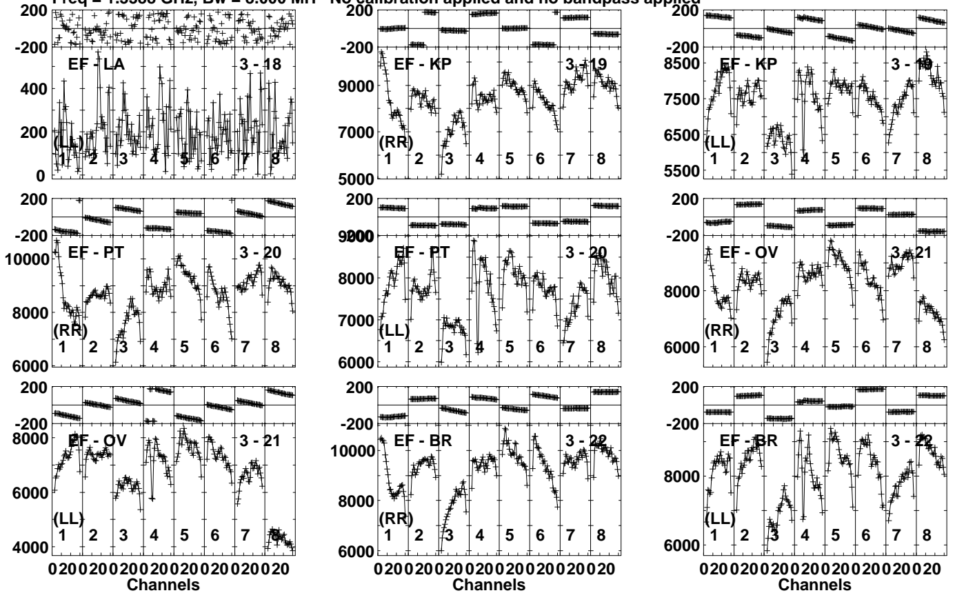
Lower frame: Micro Ampl Jy Top frame: Phas deg Vector averaged cross-power spectrum Several baselines displayed Timerange: 00/21:48:31 to 00/21:49:59
