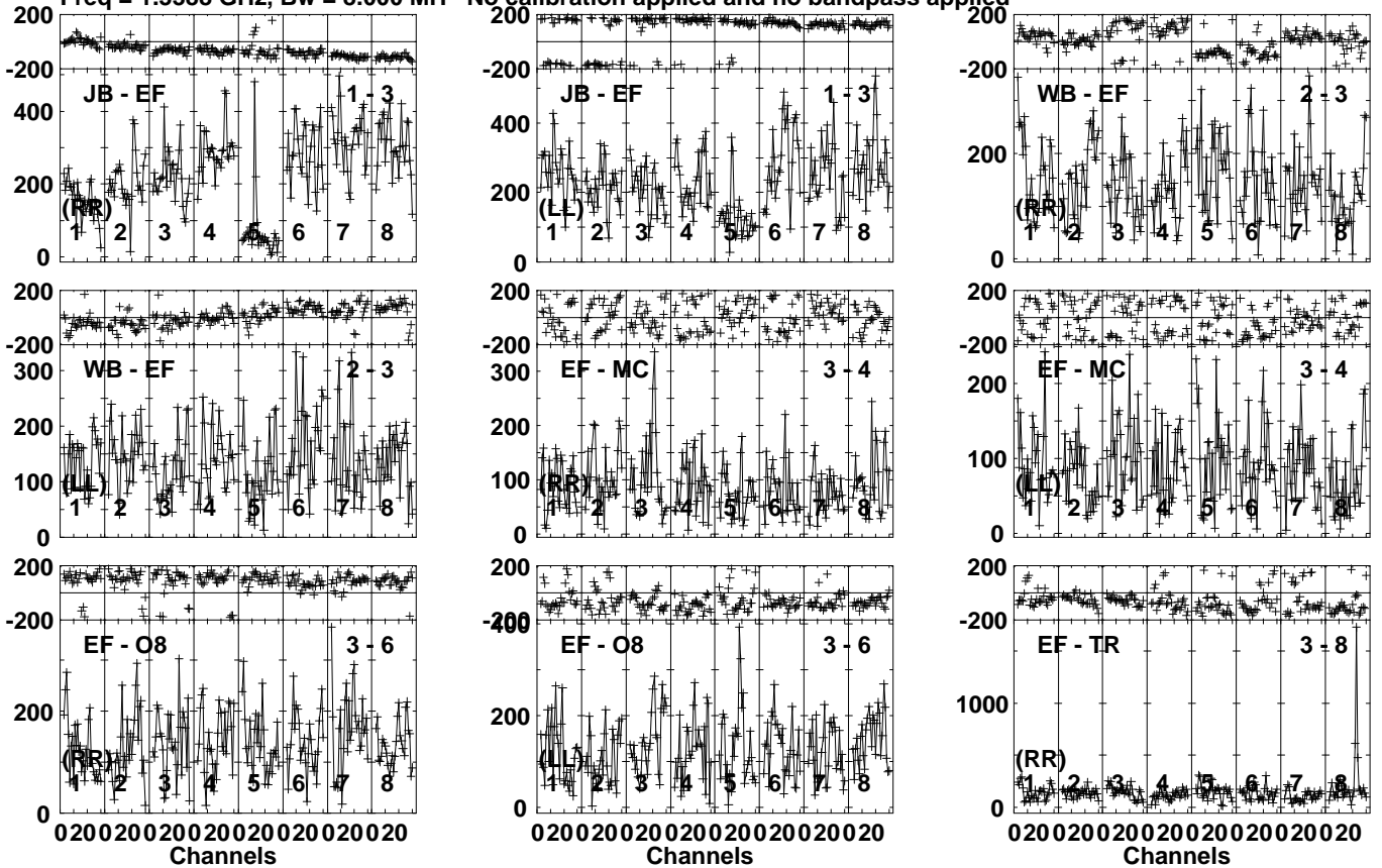
Lower frame: Micro Ampl Jy Top frame: Phas deg Vector averaged cross-power spectrum Several baselines displayed Timerange: 00/21:57:01 to 00/22:01:59
