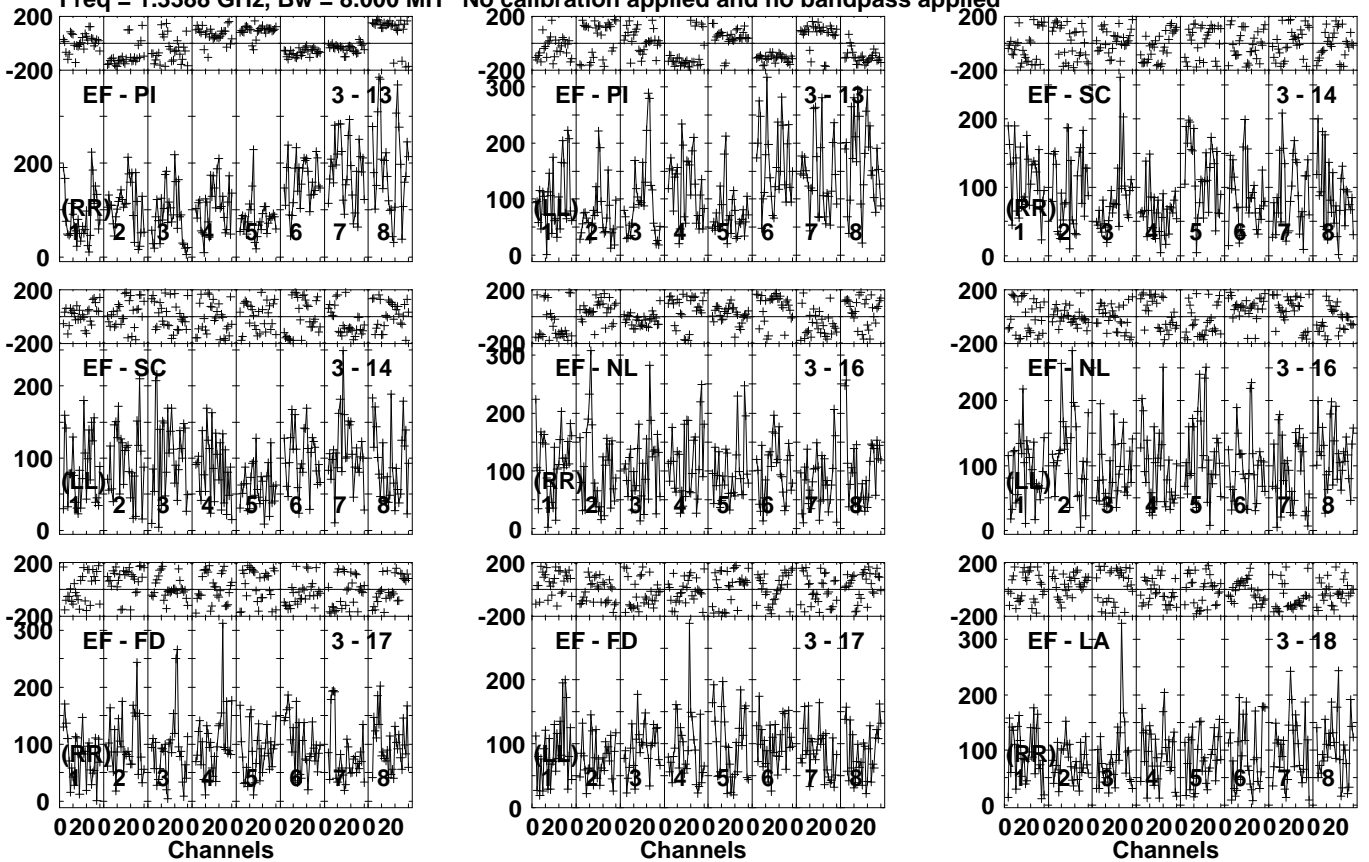
Lower frame: Micro Ampl Jy Top frame: Phas deg Vector averaged cross-power spectrum Several baselines displayed Timerange: 00/18:24:01 to 00/18:28:59
