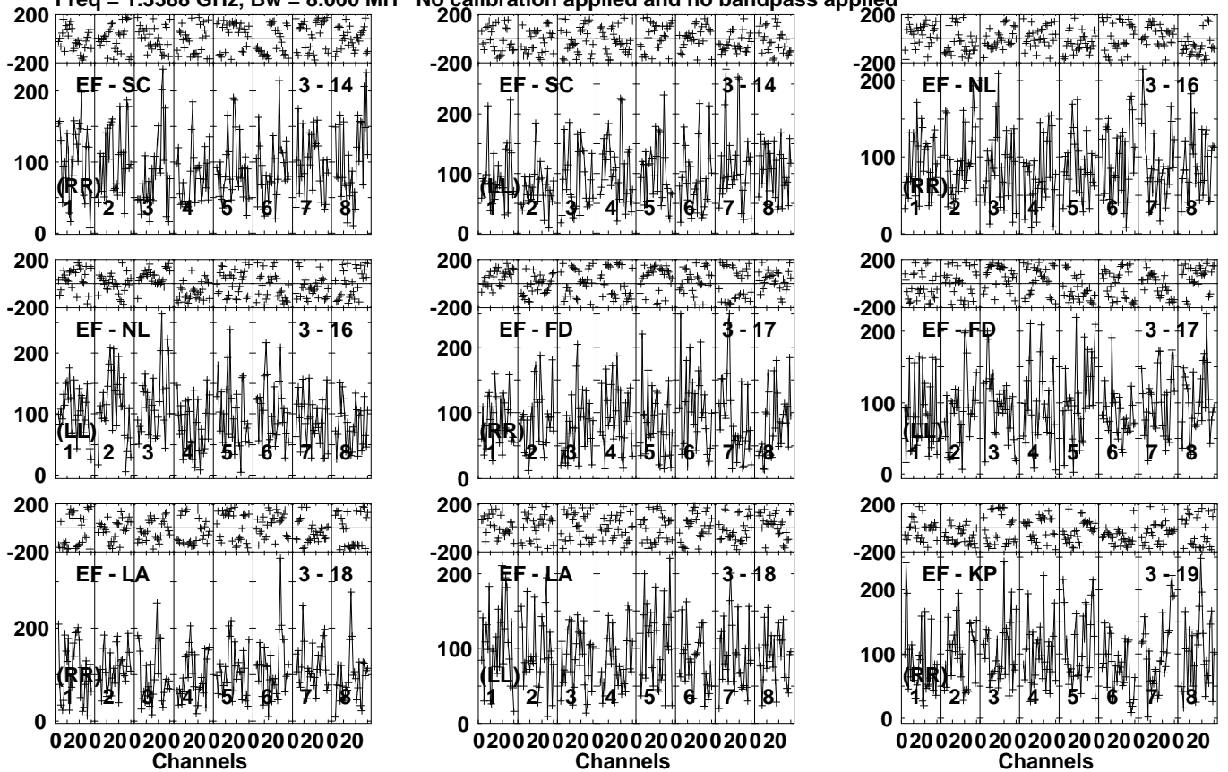
Lower frame: Micro Ampl Jy Top frame: Phas deg Vector averaged cross-power spectrum Several baselines displayed Timerange: 01/00:15:01 to 01/00:19:59
