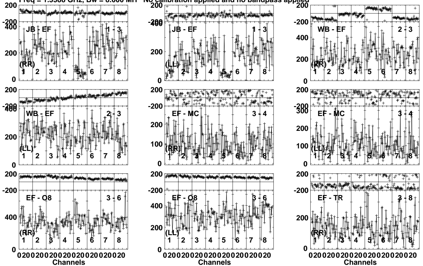
Lower frame: Micro Ampl Jy Top frame: Phas deg Vector averaged cross-power spectrum Several baselines displayed Timerange: 00:16:46:01 to 00:16:50:59
