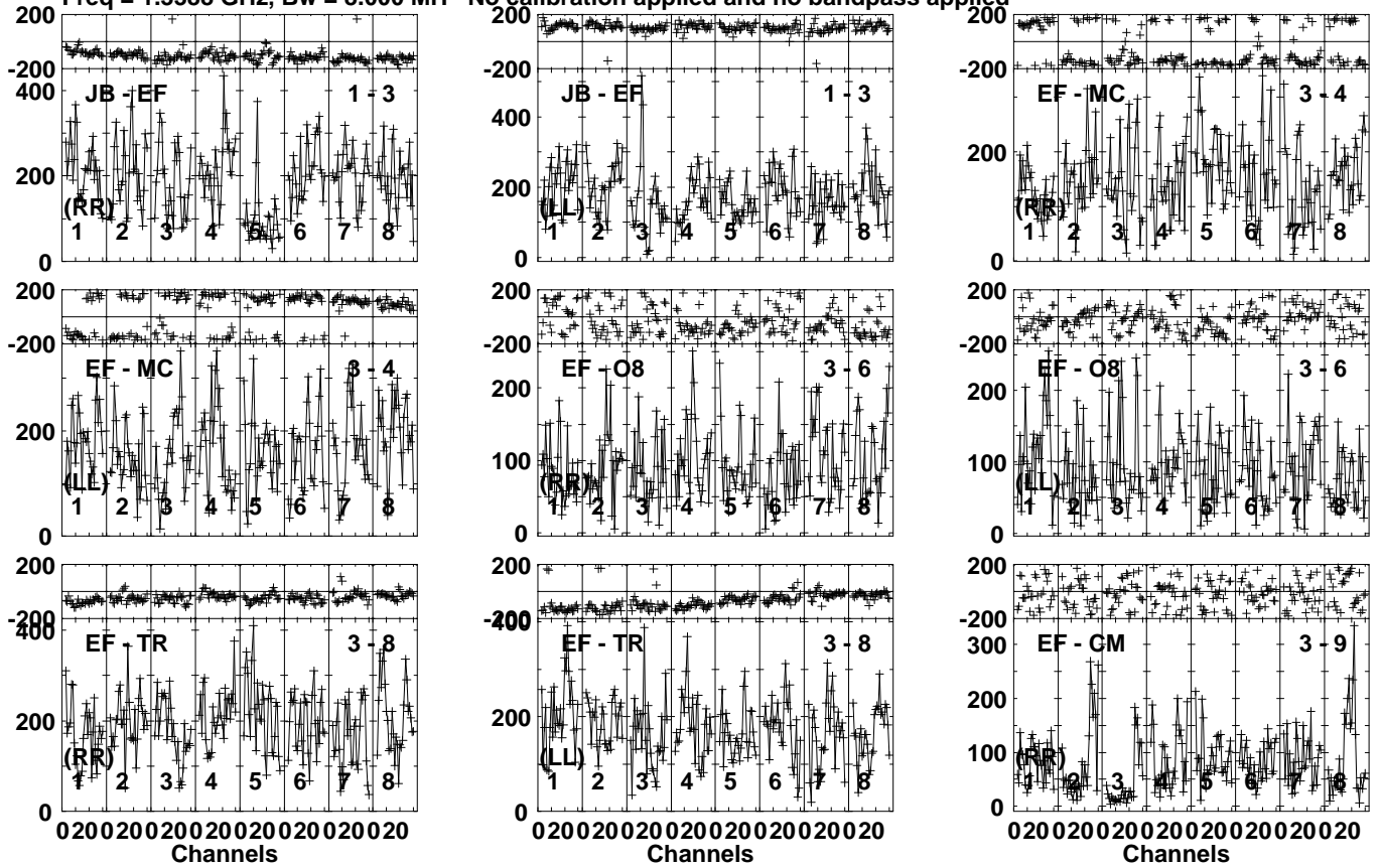
Lower frame: Micro Ampl Jy Top frame: Phas deg Vector averaged cross-power spectrum Several baselines displayed Timerange: 01/02:19:01 to 01/02:23:59
