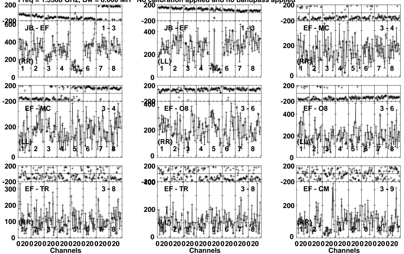
Lower frame: Micro Ampl Jy Top frame: Phas deg Vector averaged cross-power spectrum Several baselines displayed Timerange: 00/23:28:01 to 00/23:32:59
