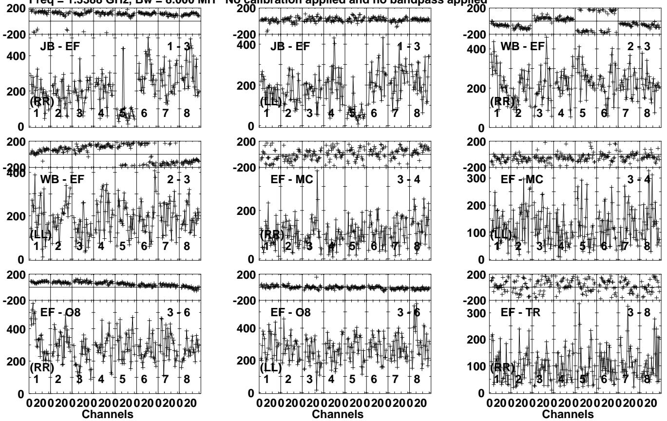
Lower frame: Micro Ampl Jy Top frame: Phas deg Vector averaged cross-power spectrum Several baselines displayed Timerange: 00/17:35:01 to 00/17:39:59
