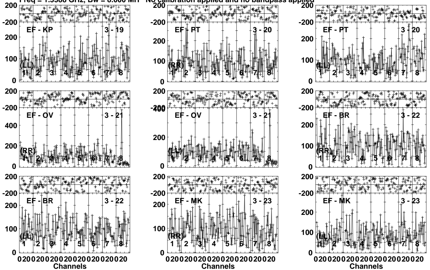
Lower frame: Micro Ampl Jy Top frame: Phas deg Vector averaged cross-power spectrum Several baselines displayed Timerange: 01/00:36:01 to 01/00:40:59
