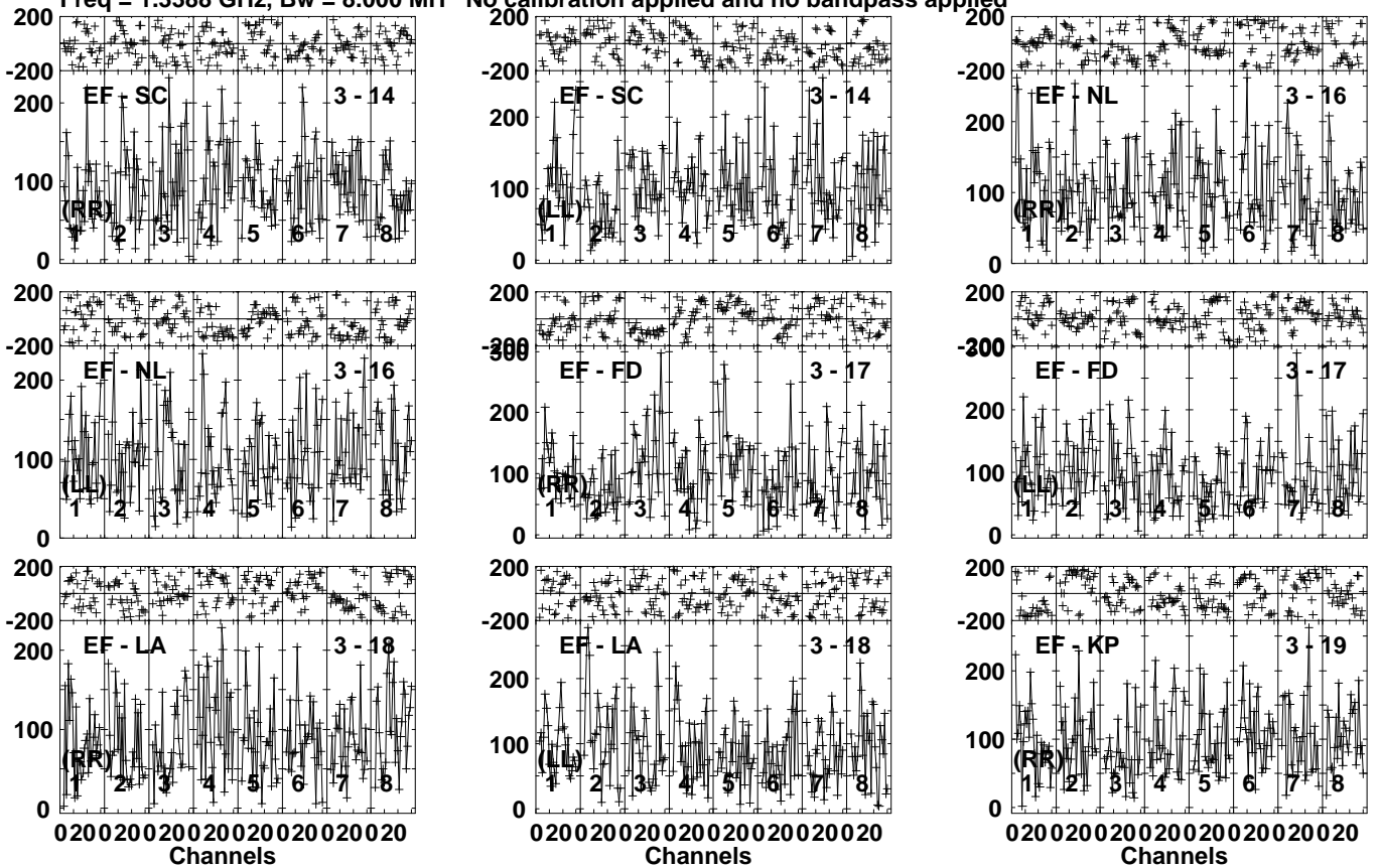
Lower frame: Micro Ampl Jy Top frame: Phas deg Vector averaged cross-power spectrum Several baselines displayed Timerange: 01/00:29:01 to 01/00:33:59
