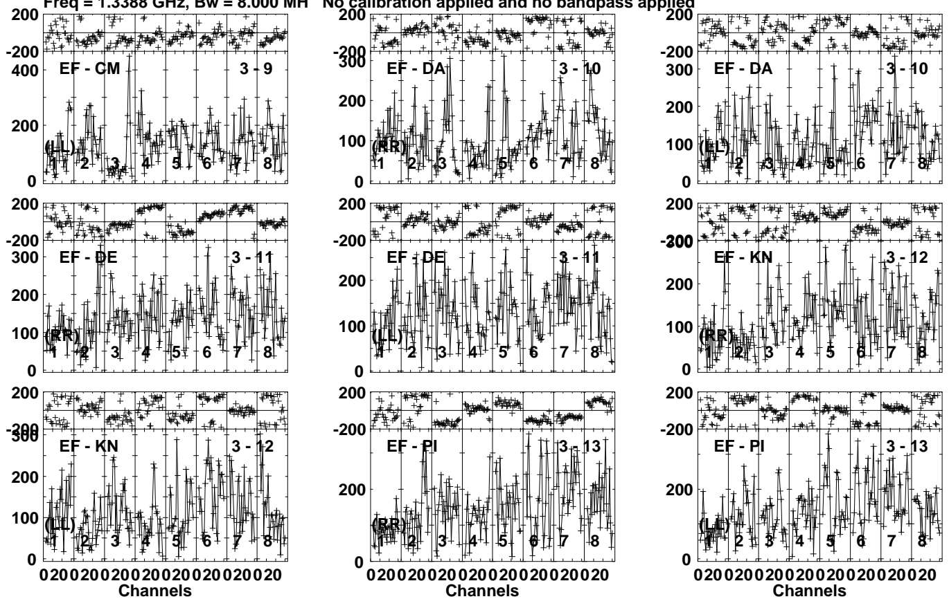
Lower frame: Micro Ampl Jy Top frame: Phas deg Vector averaged cross-power spectrum Several baselines displayed Timerange: 01/01:46:01 to 01/01:50:59
