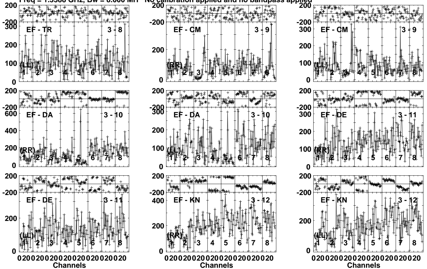
Lower frame: Micro Ampl Jy Top frame: Phas deg Vector averaged cross-power spectrum Several baselines displayed Timerange: 00/17:42:01 to 00/17:46:59
