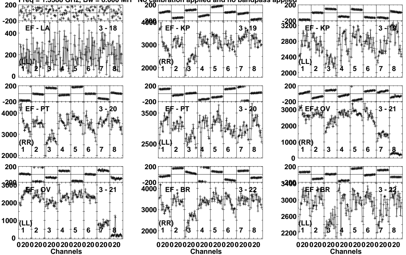
Lower frame: Micro Ampl Jy Top frame: Phas deg Vector averaged cross-power spectrum Several baselines displayed Timerange: 00/17:05:31 to 00/17:06:59
