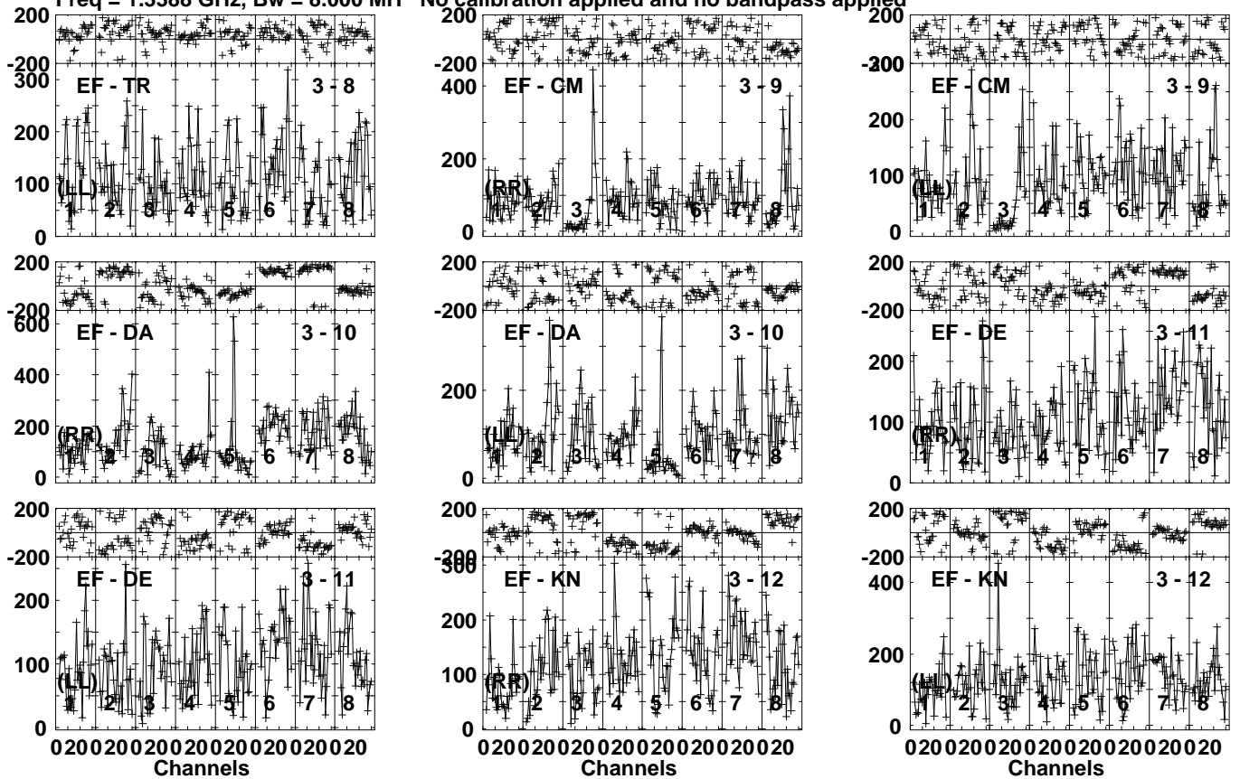
Lower frame: Micro Ampl Jy Top frame: Phas deg Vector averaged cross-power spectrum Several baselines displayed Timerange: 00/18:03:01 to 00/18:07:59
