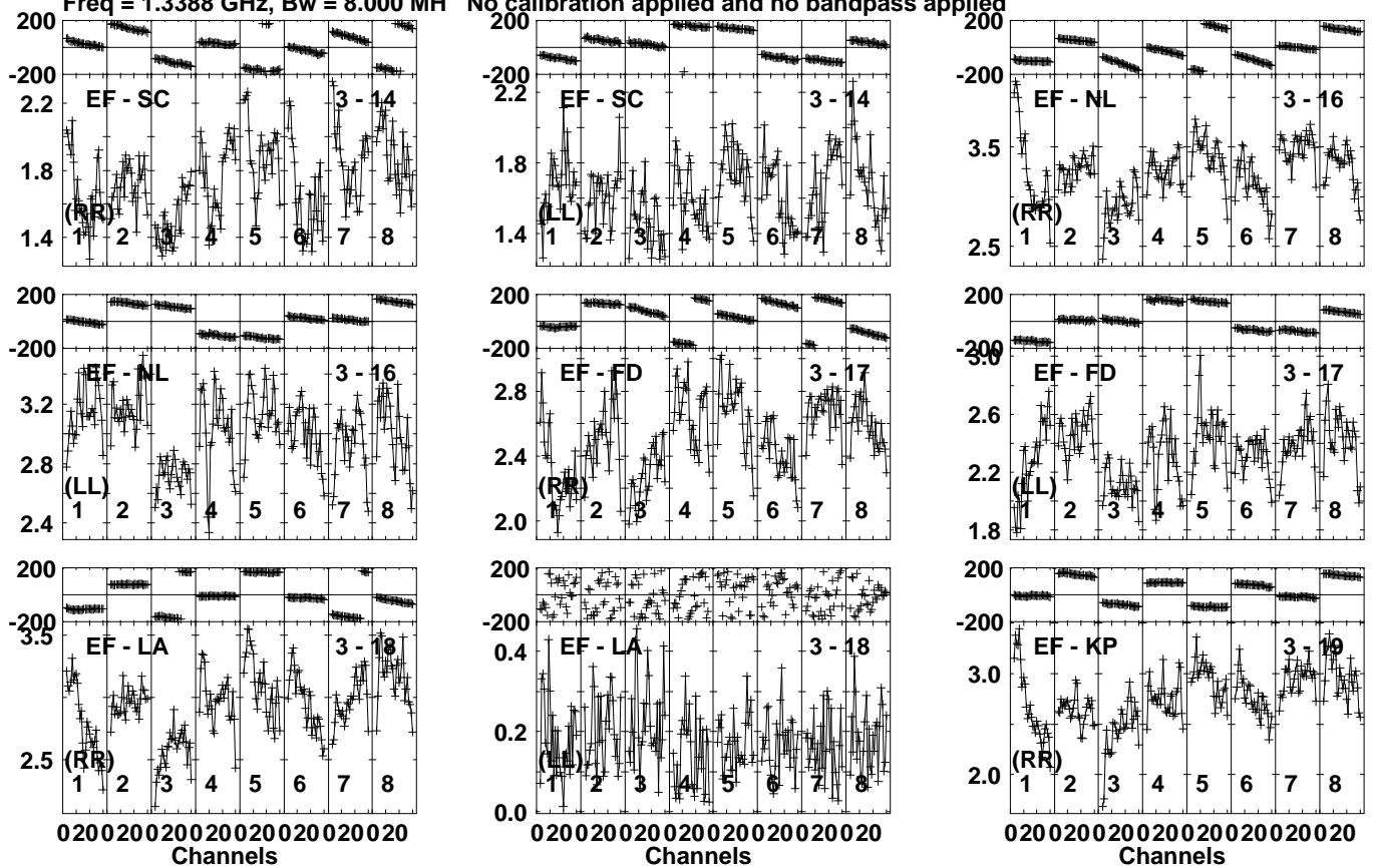
Lower frame: Milli Amp Jy Top frame: Phas deg Vector averaged cross-power spectrum Several baselines displayed Timerange: 01/03:06:31 to 01/03:07:59
