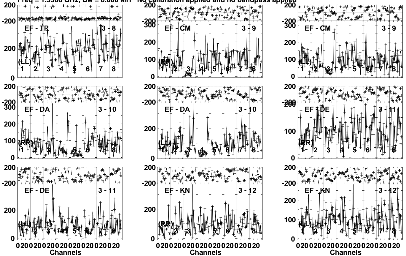
Lower frame: Micro Ampl Jy Top frame: Phas deg Vector averaged cross-power spectrum Several baselines displayed Timerange: 00/18:45:01 to 00/18:49:59
