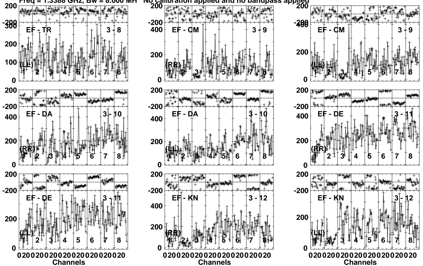
Lower frame: Micro Ampl Jy Top frame: Phas deg Vector averaged cross-power spectrum Several baselines displayed Timerange: 00/22:39:01 to 00/22:43:59
