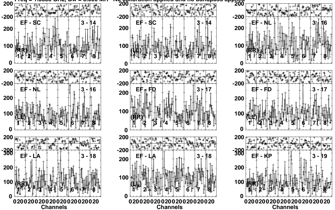
Lower frame: Micro Ampl Jy Top frame: Phas deg Vector averaged cross-power spectrum Several baselines displayed Timerange: 01/02:47:01 to 01/02:51:59
