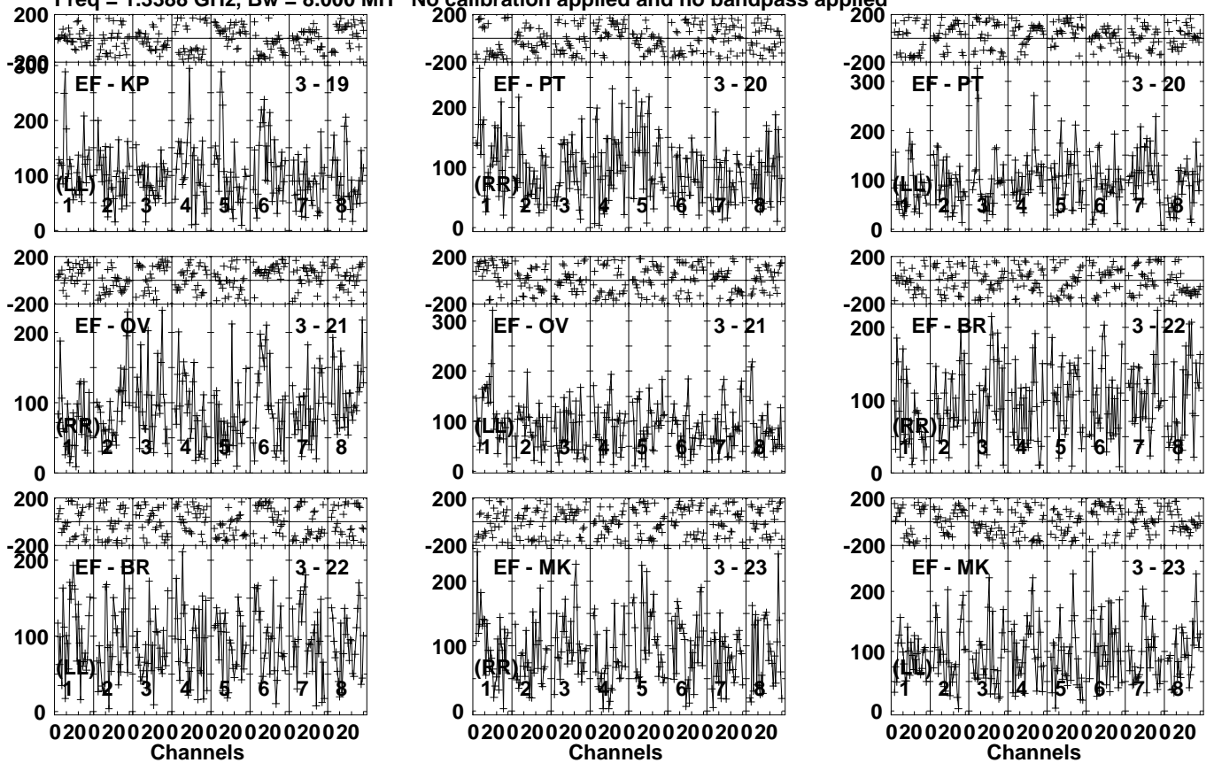
Lower frame: Micro Ampl Jy Top frame: Phas deg Vector averaged cross-power spectrum Several baselines displayed Timerange: 01/02:54:01 to 01/02:58:59
