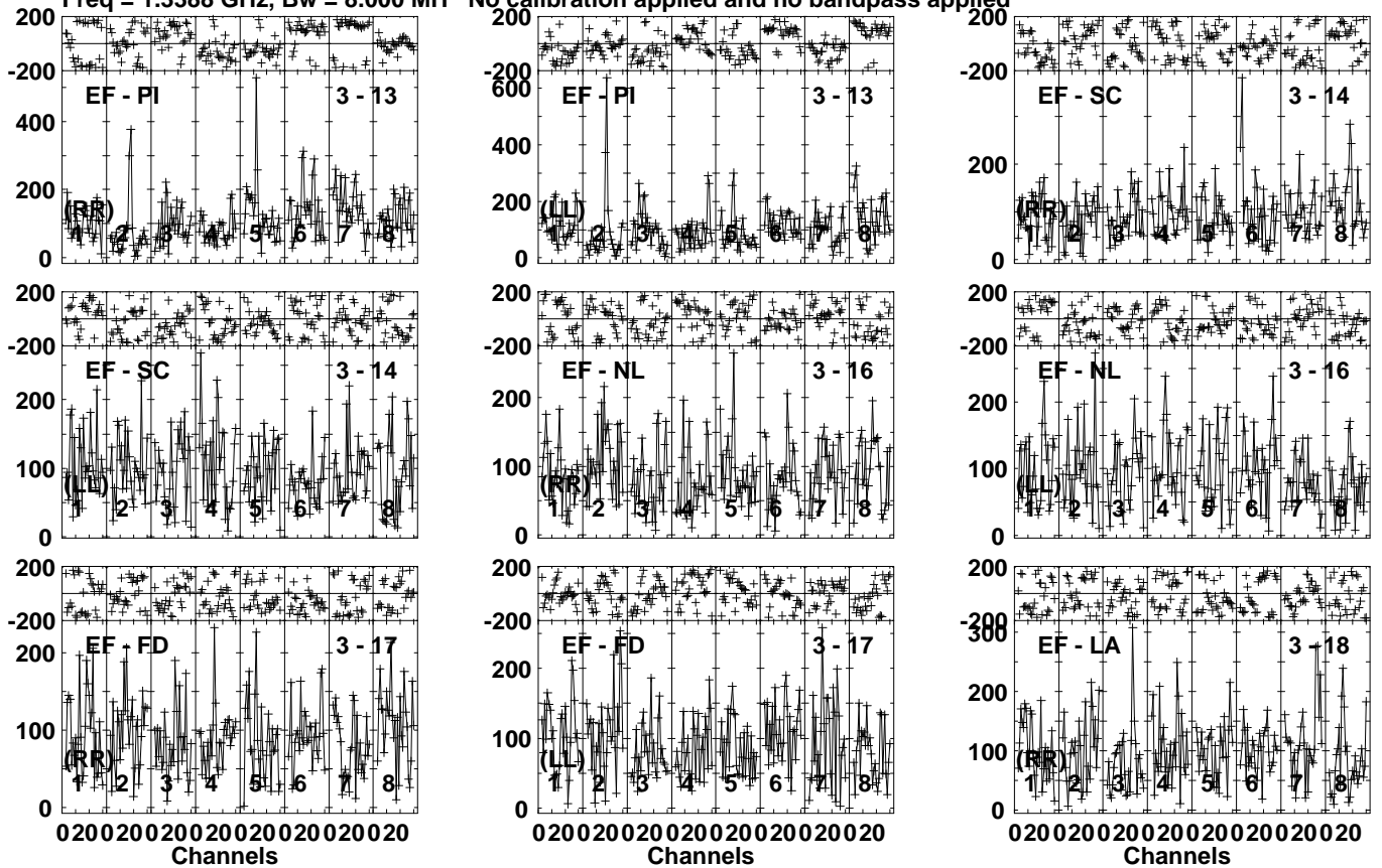
Lower frame: Micro Ampl Jy Top frame: Phas deg Vector averaged cross-power spectrum Several baselines displayed Timerange: 00/21:03:01 to 00/21:07:59
