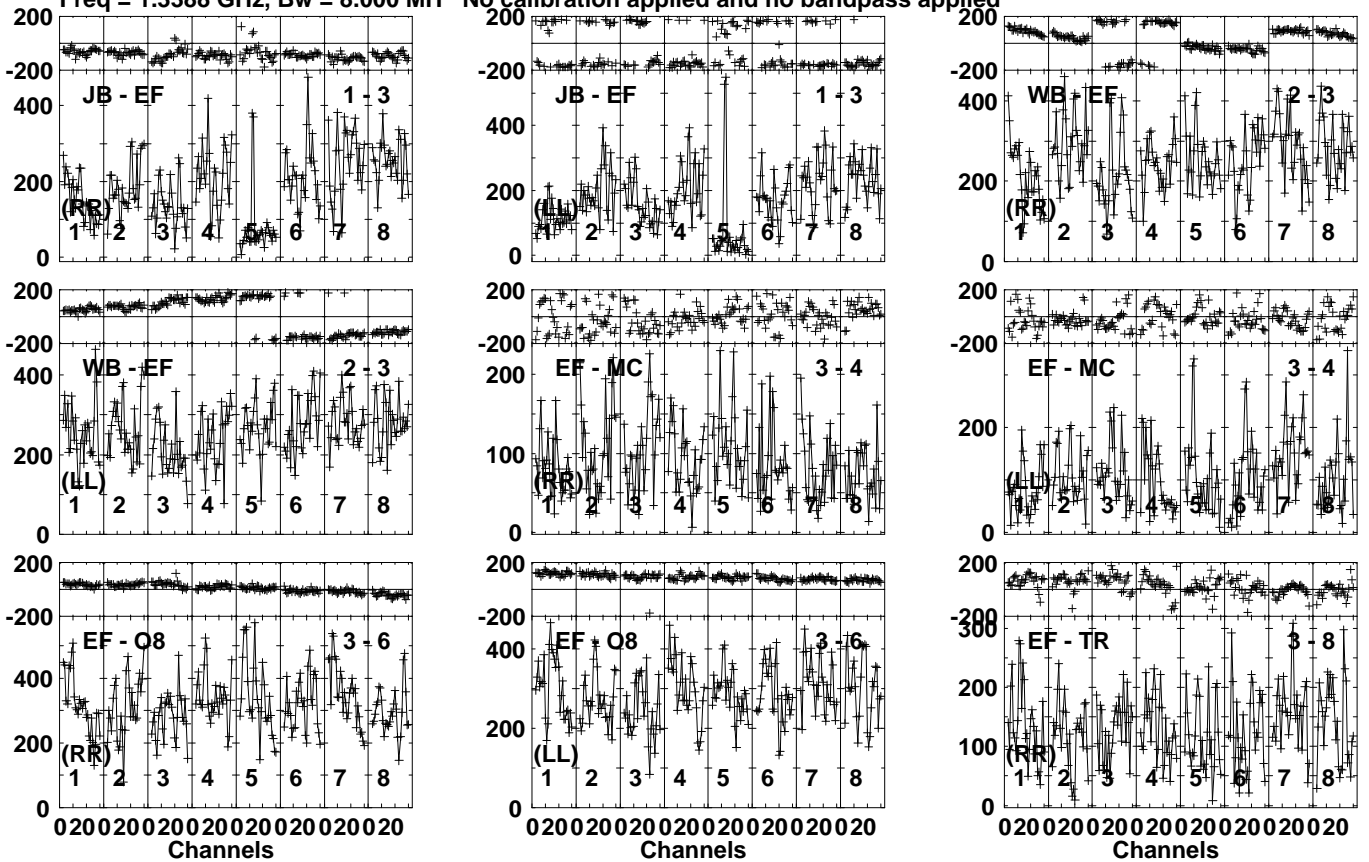
Lower frame: Micro Ampl Jy Top frame: Phas deg Vector averaged cross-power spectrum Several baselines displayed Timerange: 00/16:10:01 to 00/16:15:29
