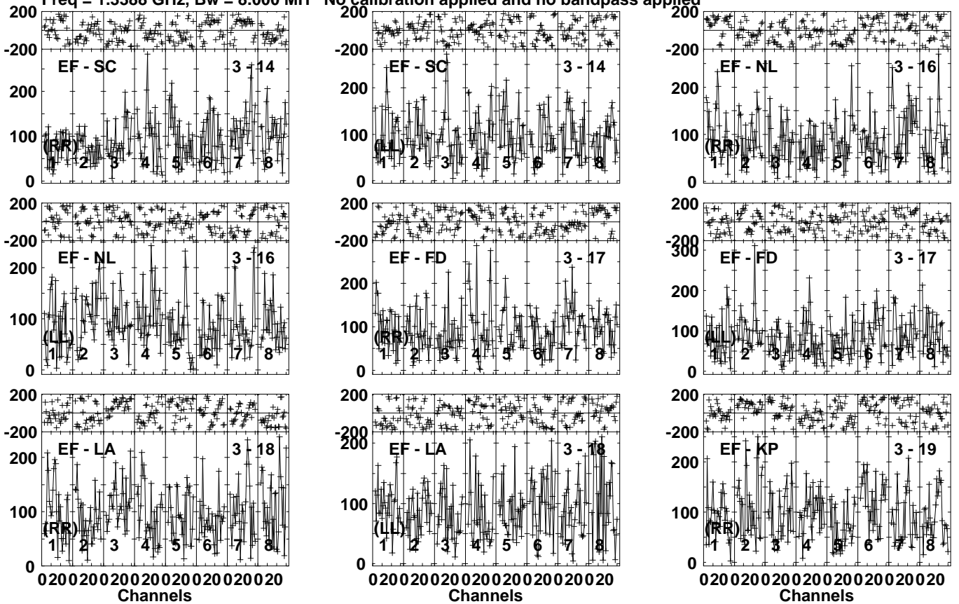
Lower frame: Micro Ampl Jy Top frame: Phas deg Vector averaged cross-power spectrum Several baselines displayed Timerange: 01/03:01:01 to 01/03:05:59
