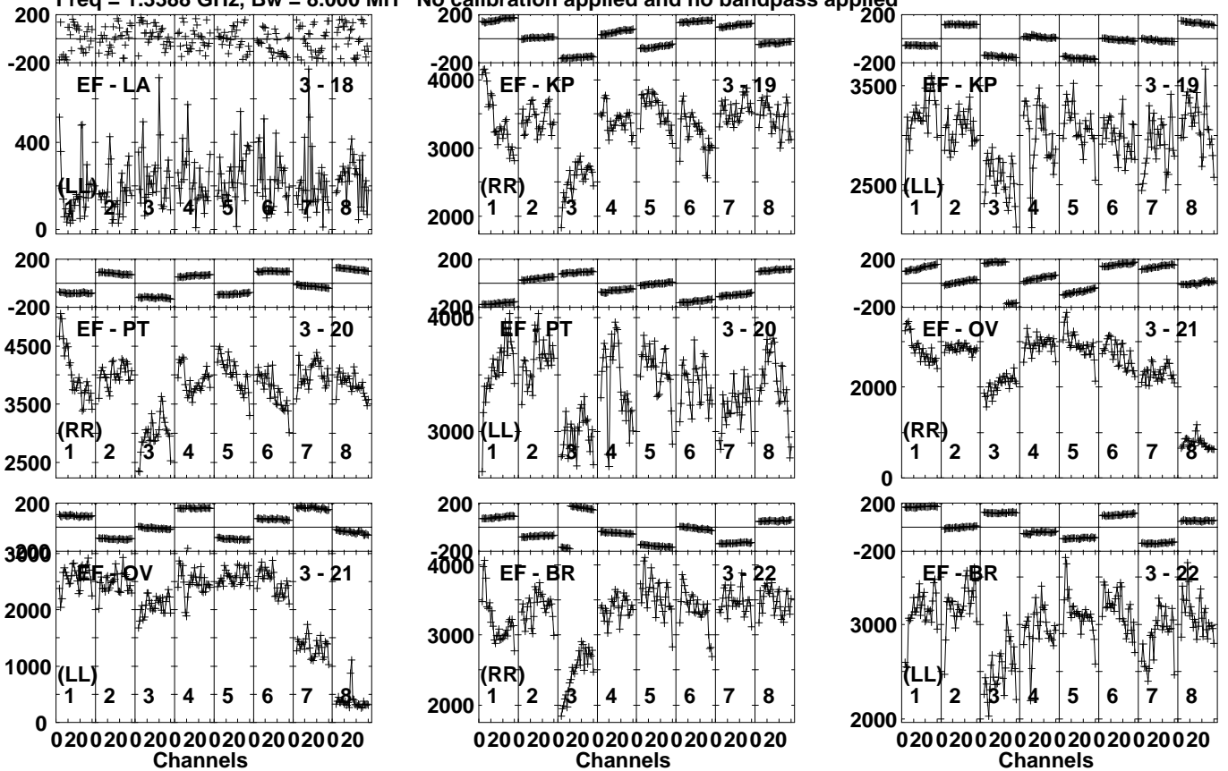
Lower frame: Micro Ampl Jy Top frame: Phas deg Vector averaged cross-power spectrum Several baselines displayed Timerange: 00/17:26:31 to 00/17:27:59
