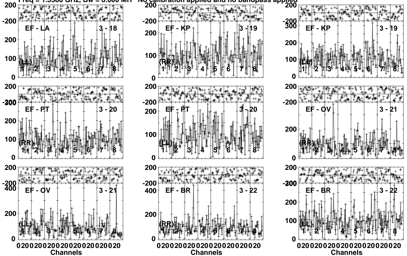
Lower frame: Micro Ampl Jy Top frame: Phas deg Vector averaged cross-power spectrum Several baselines displayed Timerange: 00/17:28:01 to 00/17:32:59
