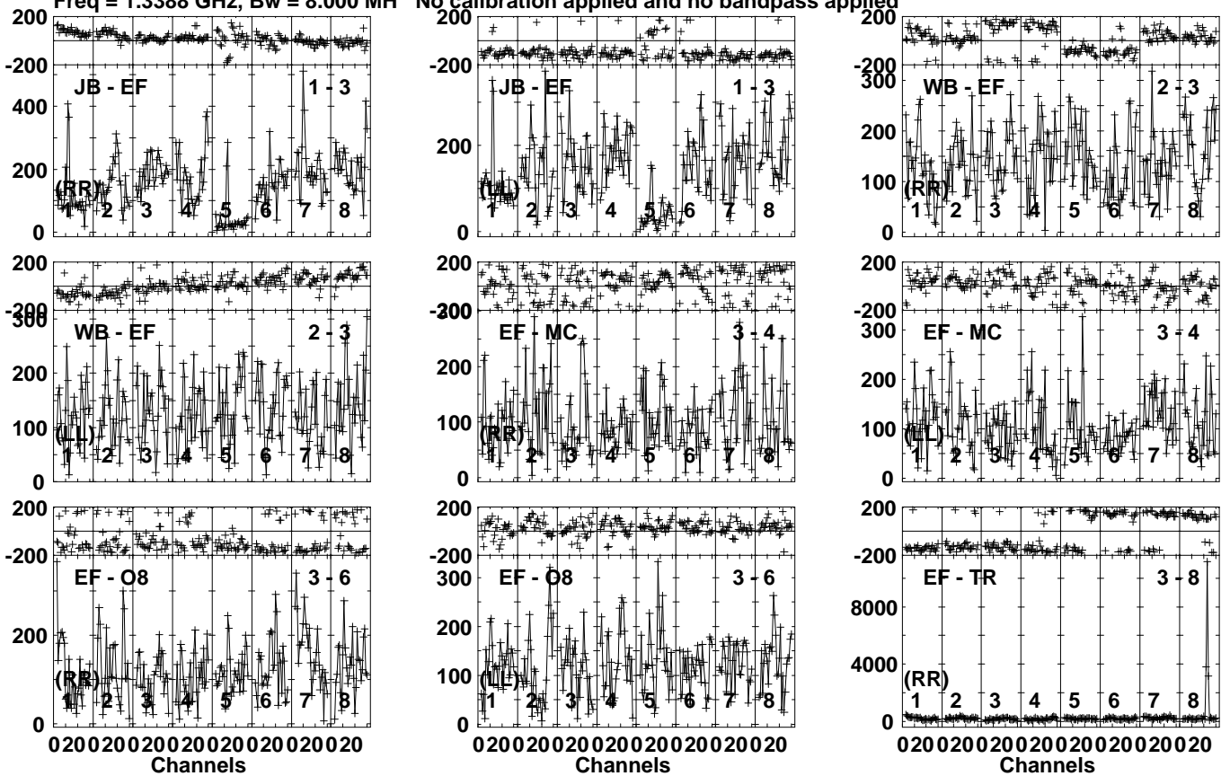
Lower frame: Micro Ampl Jy Top frame: Phas deg Vector averaged cross-power spectrum Several baselines displayed Timerange: 00/21:17:01 to 00/21:21:59
