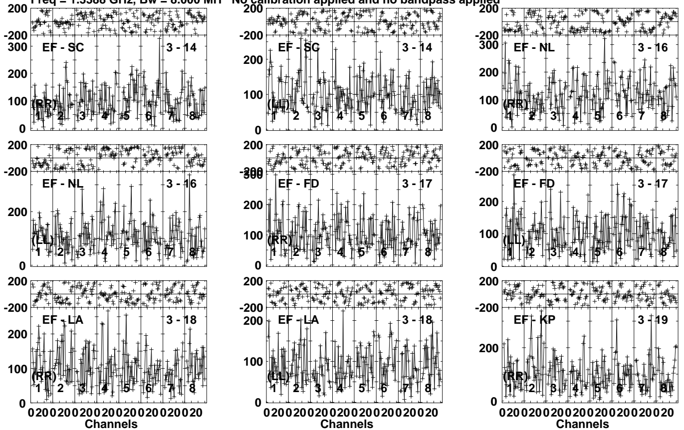
Lower frame: Micro Ampl Jy Top frame: Phas deg Vector averaged cross-power spectrum Several baselines displayed Timerange: 00/23:35:01 to 00/23:39:59
