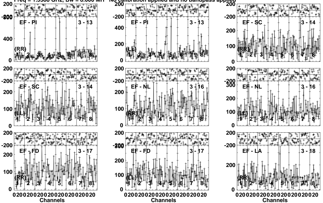
Lower frame: Micro Ampl Jy Top frame: Phas deg Vector averaged cross-power spectrum Several baselines displayed Timerange: 00/20:35:01 to 00/20:39:59
