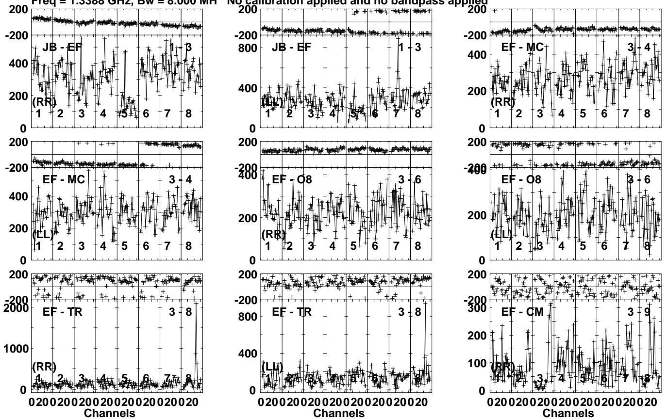
Lower frame: Micro Ampl Jy Top frame: Phas deg Vector averaged cross-power spectrum Several baselines displayed Timerange: 01/00:22:01 to 01/00:26:59
