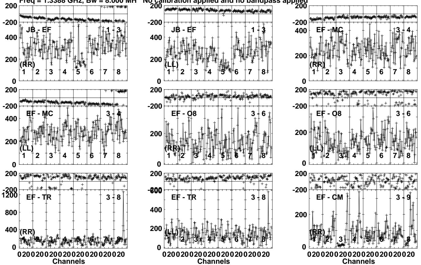
Lower frame: Micro Ampl Jy Top frame: Phas deg Vector averaged cross-power spectrum Several baselines displayed Timerange: 01/00:57:01 to 01/01:01:59
