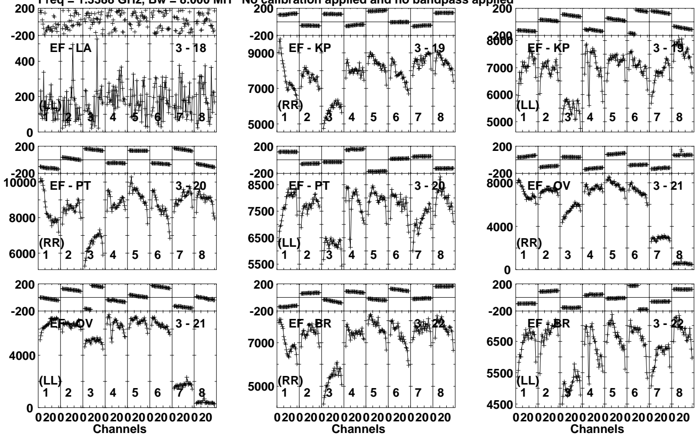
Lower frame: Micro Ampl Jy Top frame: Phas deg Vector averaged cross-power spectrum Several baselines displayed Timerange: 00/20:19:31 to 00/20:20:59
