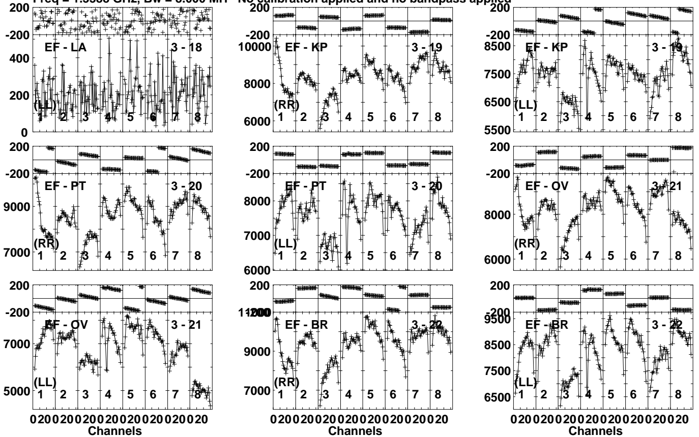
Lower frame: Micro Ampl Jy Top frame: Phas deg Vector averaged cross-power spectrum Several baselines displayed Timerange: 00/21:55:31 to 00/21:56:59
