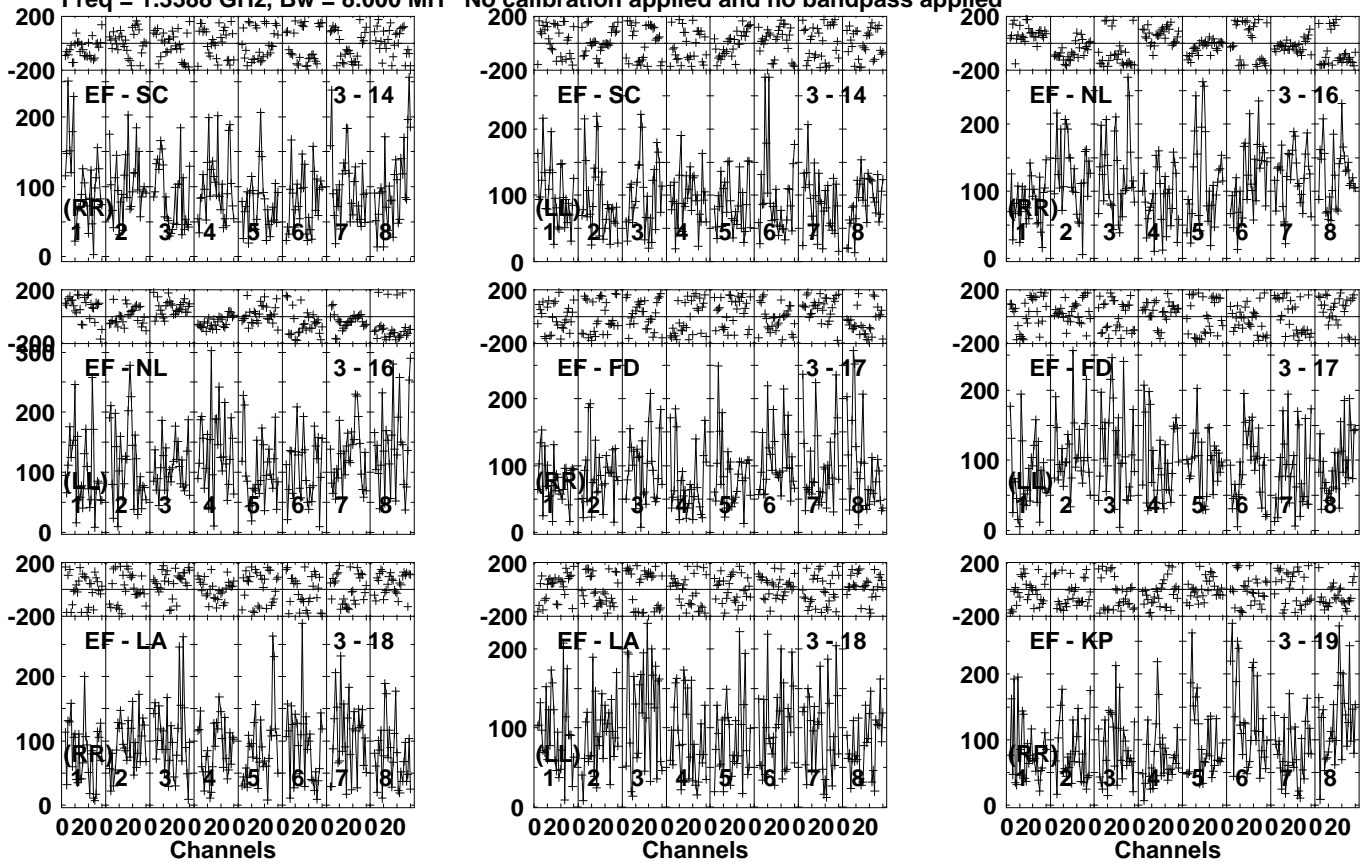
Lower frame: Micro Ampl Jy Top frame: Phas deg Vector averaged cross-power spectrum Several baselines displayed Timerange: 01/01:25:01 to 01/01:29:59
