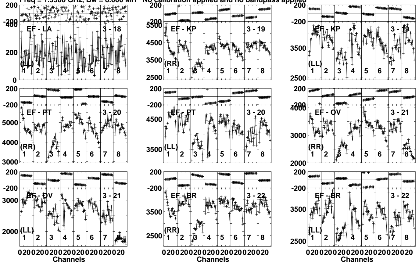
Lower frame: Micro Ampl Jy Top frame: Phas deg Vector averaged cross-power spectrum Several baselines displayed Timerange: 00/18:01:31 to 00/18:02:59
