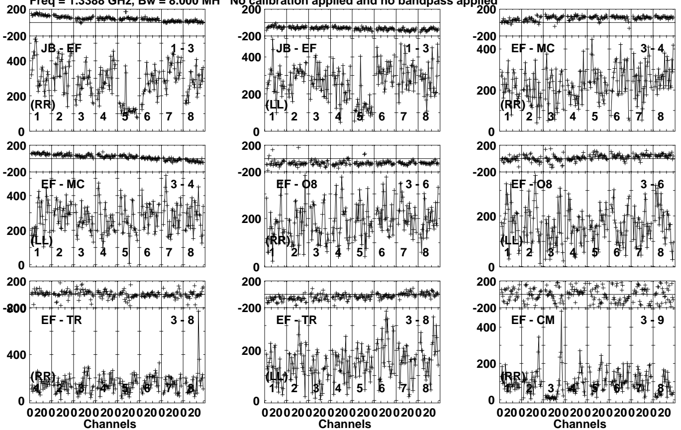
Lower frame: Micro Ampl Jy Top frame: Phas deg Vector averaged cross-power spectrum Several baselines displayed Timerange: 01/01:18:01 to 01/01:22:59
