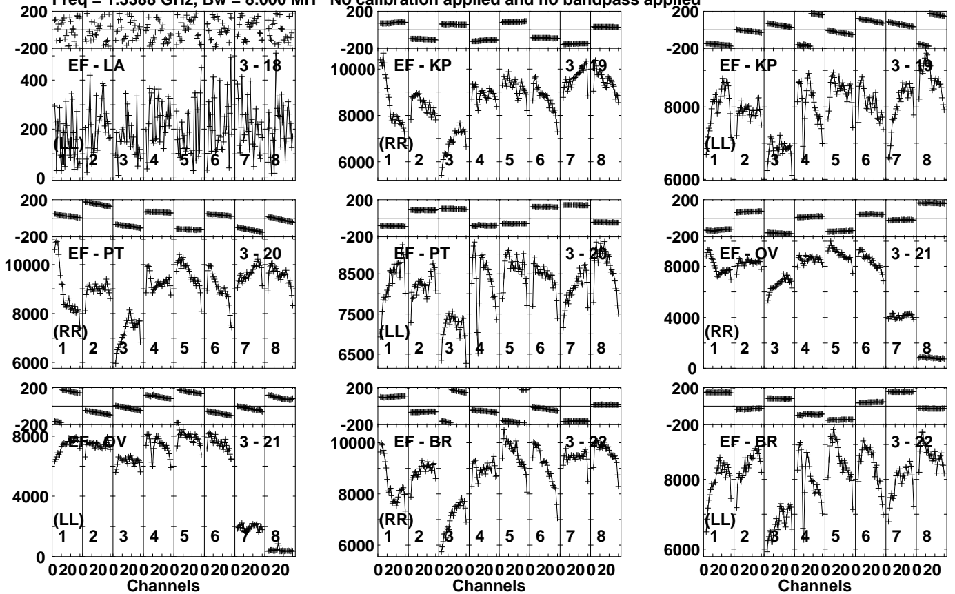
Lower frame: Micro Ampl Jy Top frame: Phas deg Vector averaged cross-power spectrum Several baselines displayed Timerange: 00/21:22:31 to 00/21:23:59
