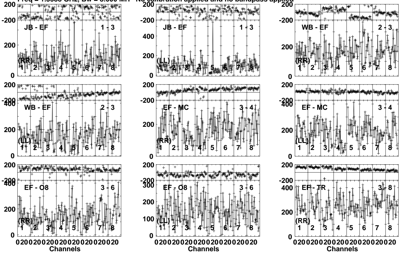
Lower frame: Micro Ampl Jy Top frame: Phas deg Vector averaged cross-power spectrum Several baselines displayed Timerange: 00:19:46:01 to 00:19:50:59
