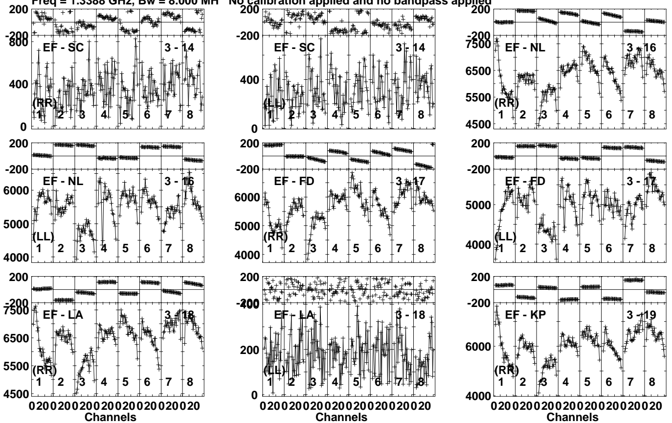
Lower frame: Micro Ampl Jy Top frame: Phas deg Vector averaged cross-power spectrum Several baselines displayed Timerange: 00/23:33:31 to 00/23:34:59
