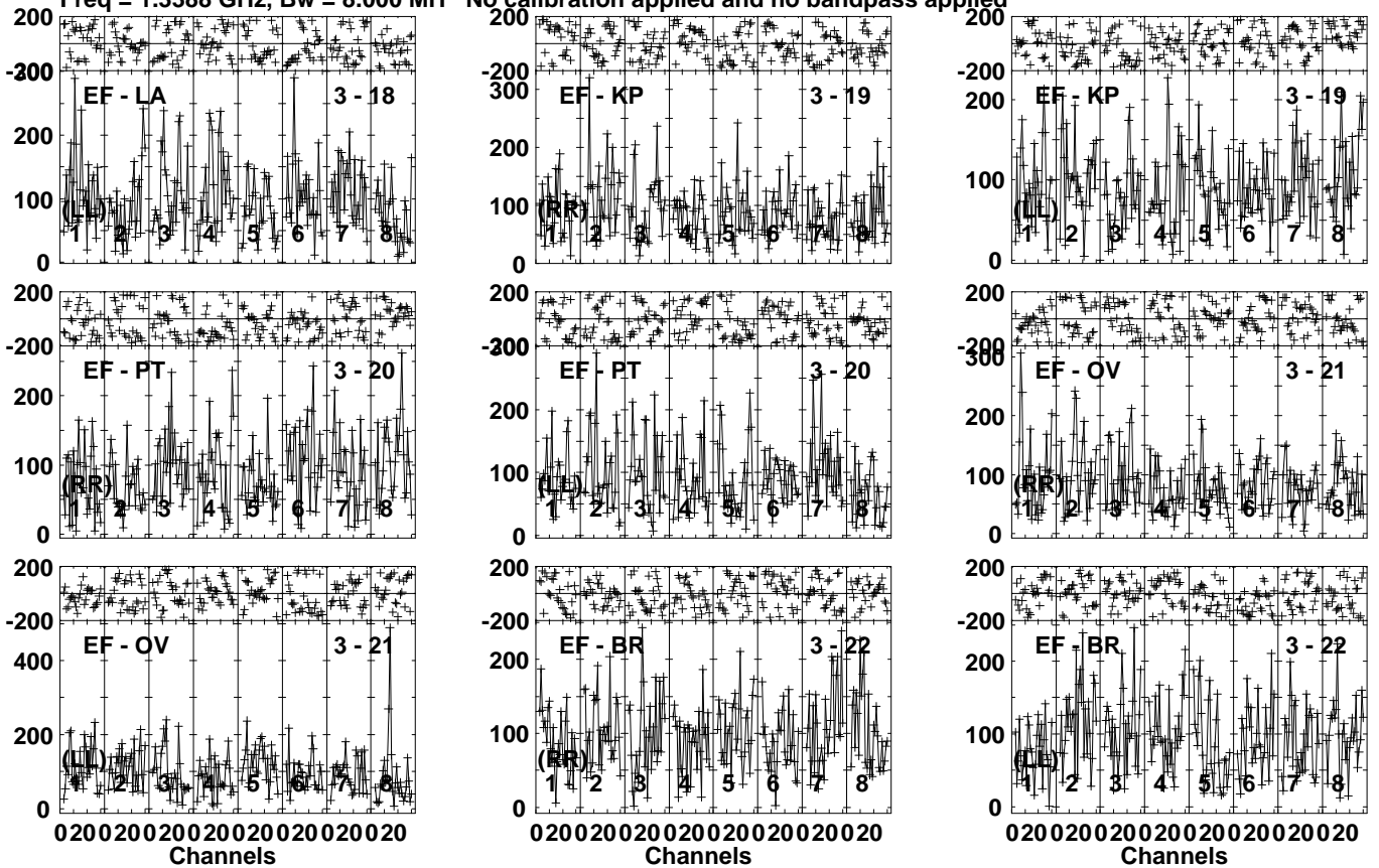
Lower frame: Micro Ampl Jy Top frame: Phas deg Vector averaged cross-power spectrum Several baselines displayed Timerange: 00/21:36:01 to 00/21:40:59
