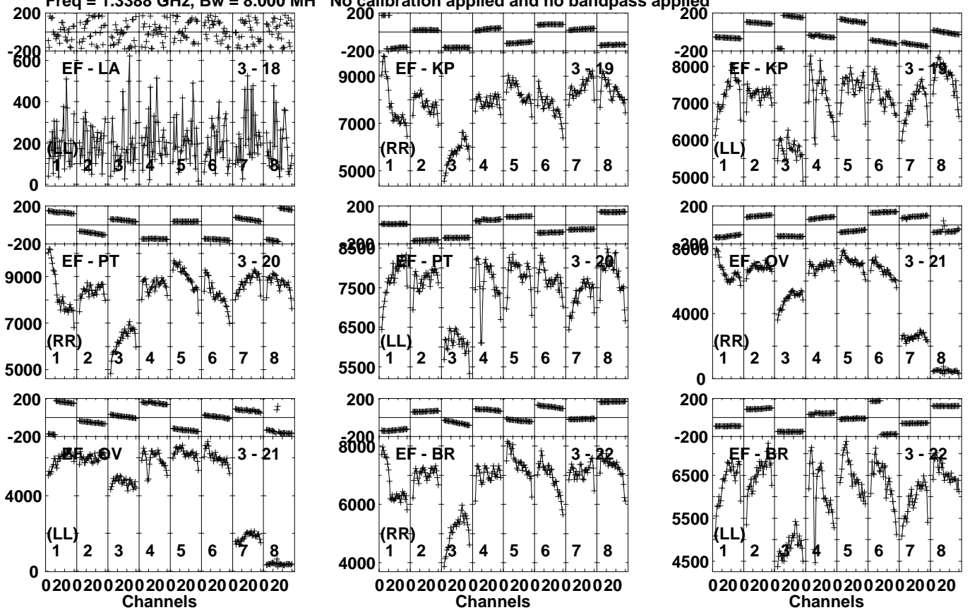
Lower frame: Micro Ampl Jy Top frame: Phas deg Vector averaged cross-power spectrum Several baselines displayed Timerange: 00/19:58:31 to 00/19:59:59
