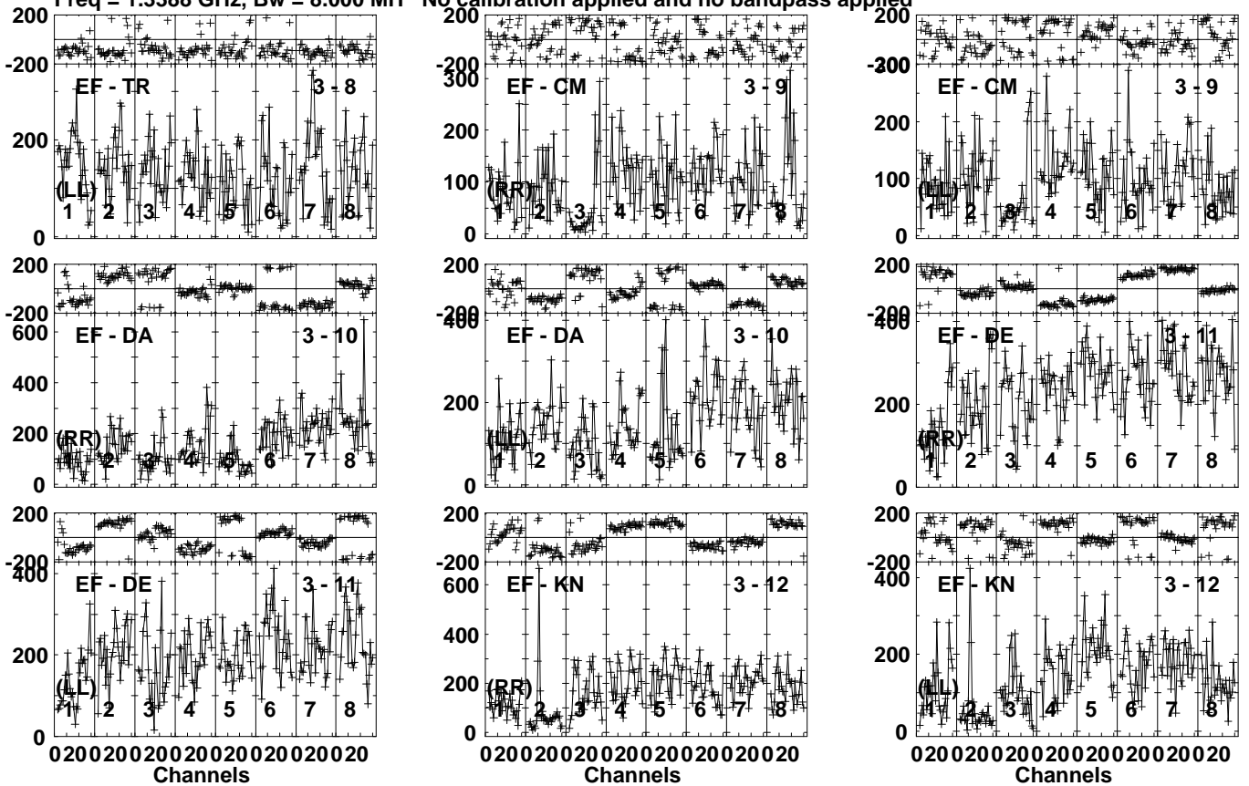
Lower frame: Micro Ampl Jy Top frame: Phas deg Vector averaged cross-power spectrum Several baselines displayed Timerange: 00/22:11:01 to 00/22:15:59
