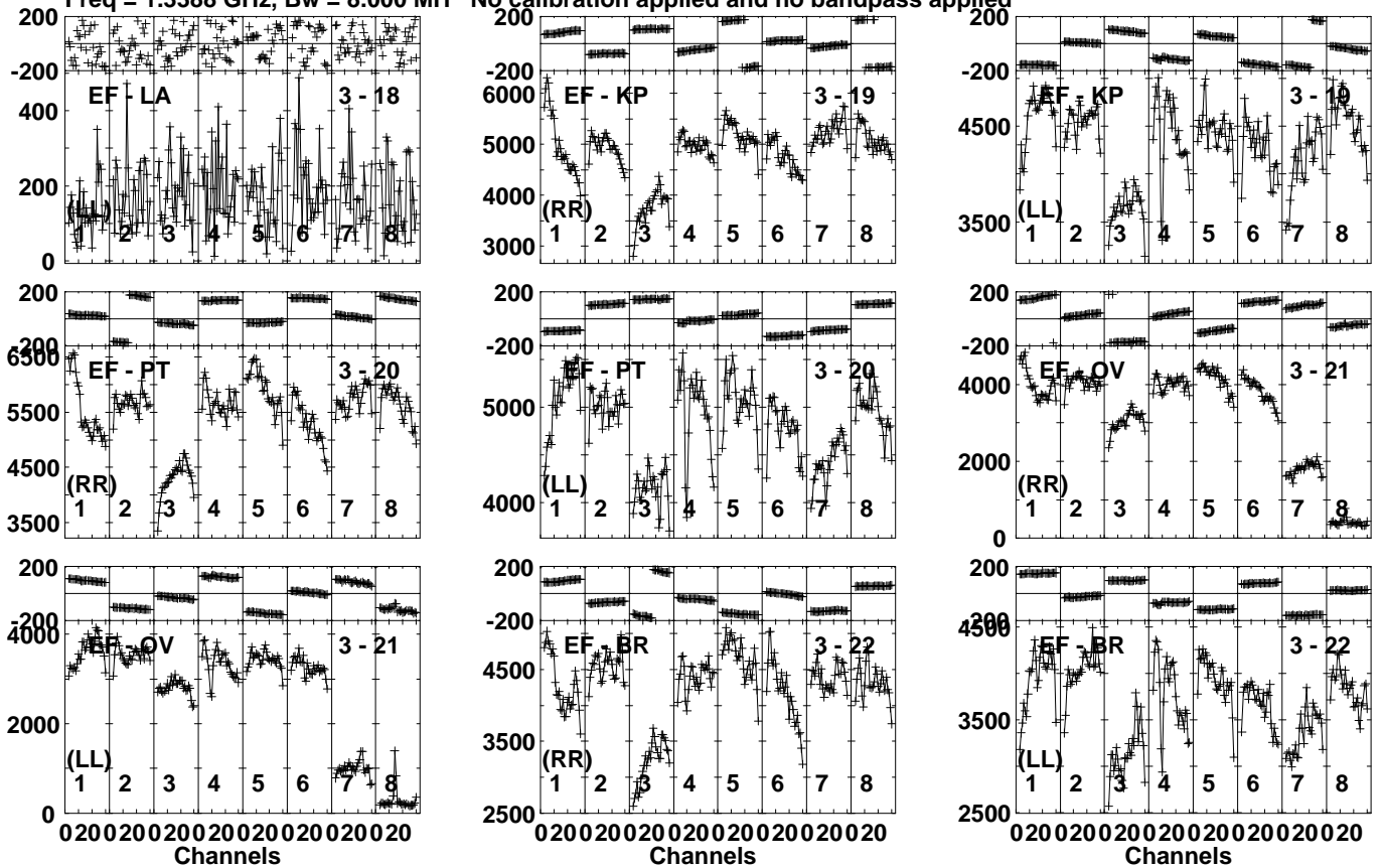
Lower frame: Micro Ampl Jy Top frame: Phas deg Vector averaged cross-power spectrum Several baselines displayed Timerange: 00/18:29:31 to 00/18:30:59
