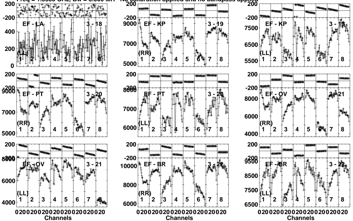
Lower frame: Micro Ampl Jy Top frame: Phas deg Vector averaged cross-power spectrum Several baselines displayed Timerange: 00/22:23:31 to 00/22:24:59
