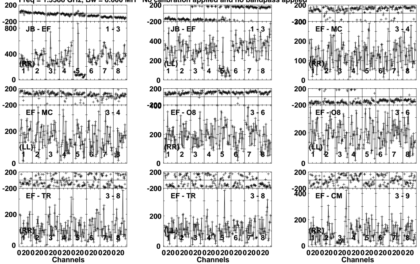
Lower frame: Micro Ampl Jy Top frame: Phas deg Vector averaged cross-power spectrum Several baselines displayed Timerange: 00/23:07:01 to 00/23:11:59
