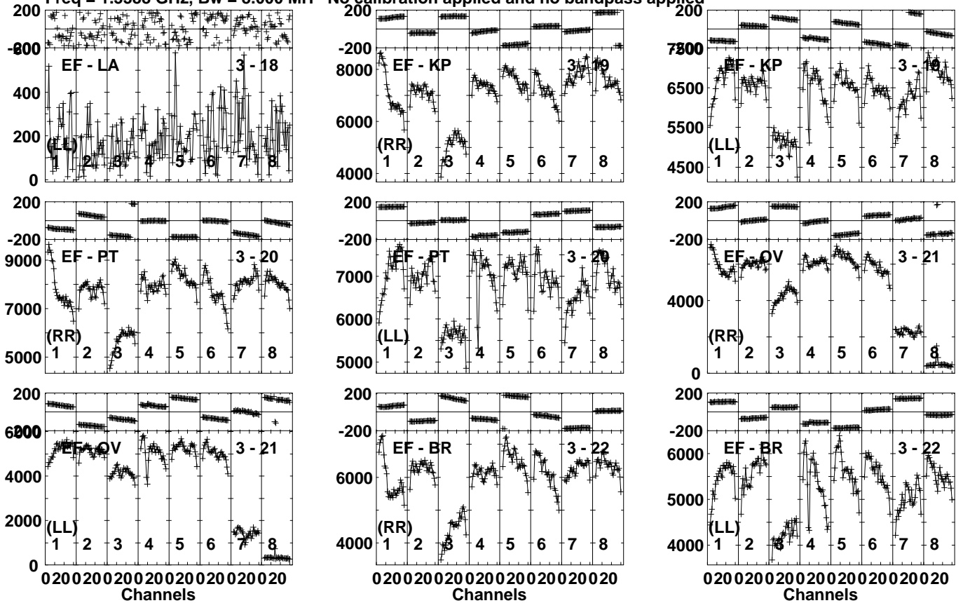
Lower frame: Micro Ampl Jy Top frame: Phas deg Vector averaged cross-power spectrum Several baselines displayed Timerange: 00/19:37:31 to 00/19:38:59
