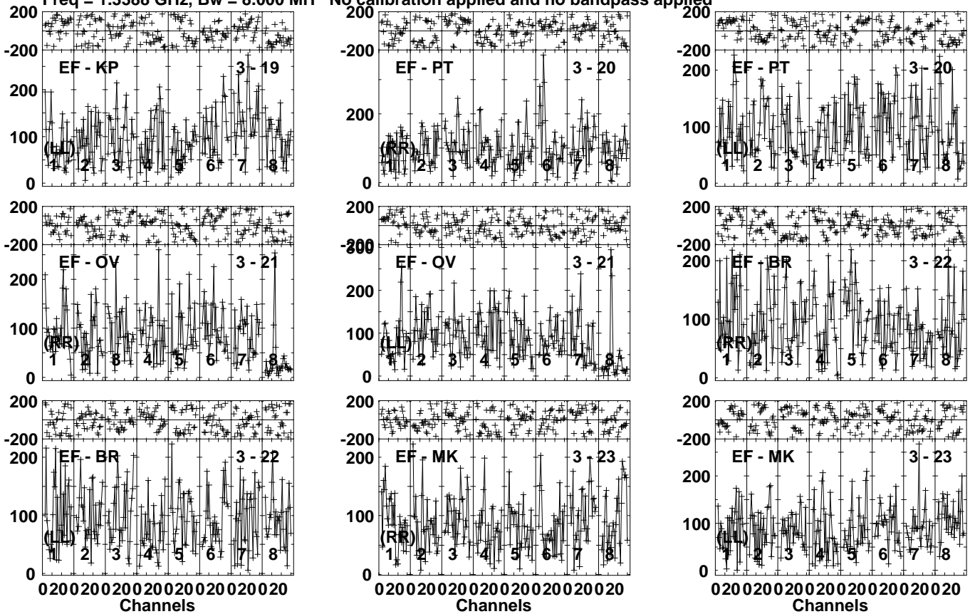
Lower frame: Micro Ampl Jy Top frame: Phas deg Vector averaged cross-power spectrum Several baselines displayed Timerange: 01/01:04:01 to 01/01:08:59
