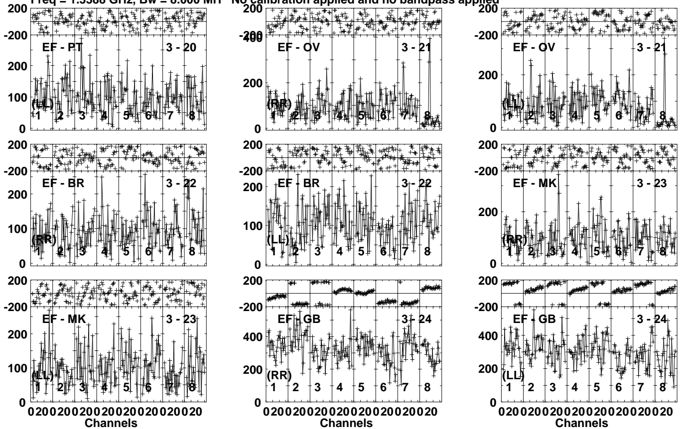
Lower frame: Micro Ampl Jy Top frame: Phas deg Vector averaged cross-power spectrum Several baselines displayed Timerange: 00/22:53:01 to 00/22:57:59
